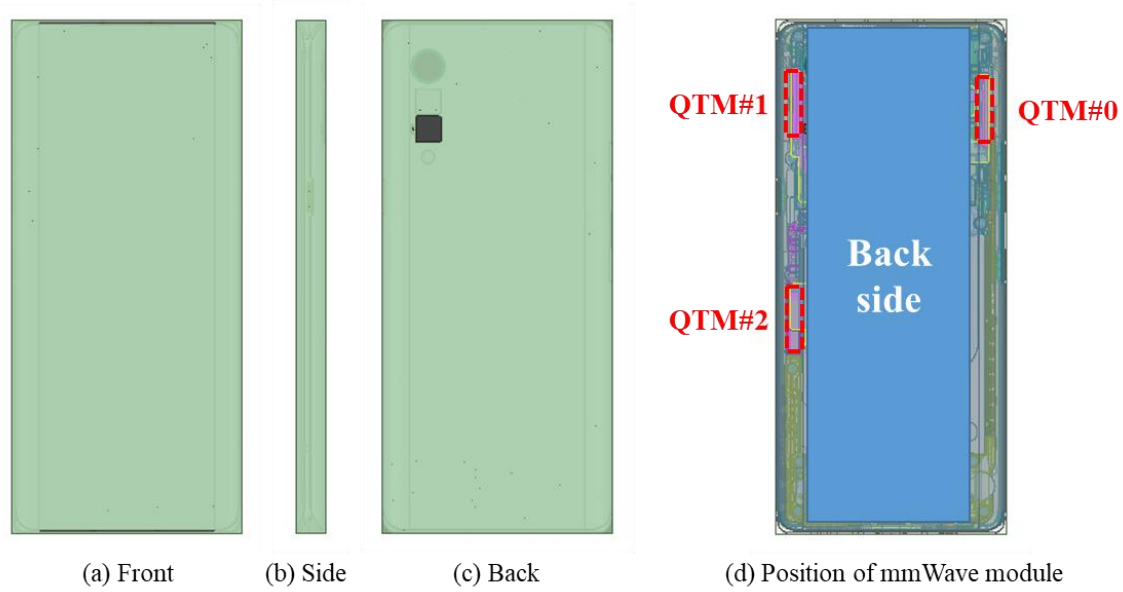
Figure 2. HFSS simulation model which is mounted three mmWave antenna modules
