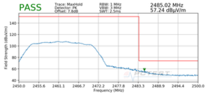
Plot 7-8. Radiated Restricted Upper Band Edge Measurement SISO ANT2 (Peak)
