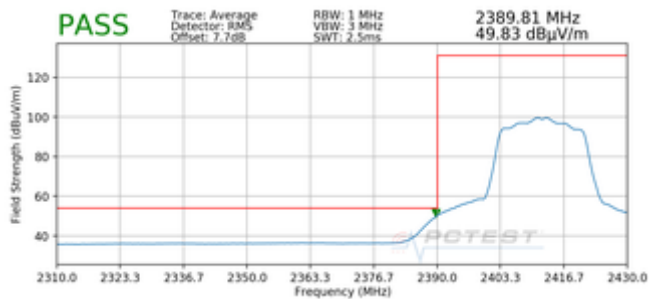
Plot 7-1. Radiated Restricted Lower Band Edge Measurement SISO ANT1 (Average)
