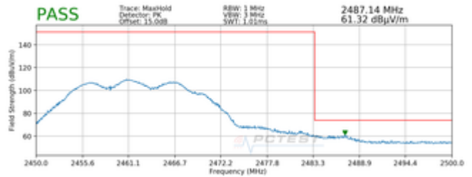
Plot 7-14. Radiated Restricted Upper Band Edge Measurement MIMO (Peak) (w/ Dual Display)
