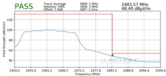
Plot 7-3. Radiated Restricted Upper Band Edge Measurement SISO ANT1 (Average)
