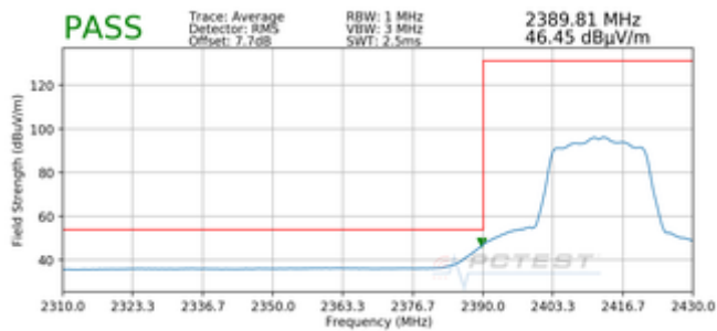
Plot 7-5. Radiated Restricted Lower Band Edge Measurement SISO ANT2 (Average)
