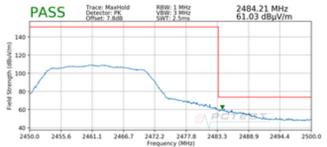
Plot 7-4. Radiated Restricted Upper Band Edge Measurement SISO ANT1 (Peak)
