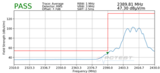
Plot 7-9. Radiated Restricted Lower Band Edge Measurement MIMO (Average)
