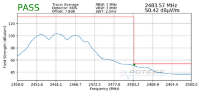
Plot 7-11. Radiated Restricted Upper Band Edge Measurement MIMO (Average)
