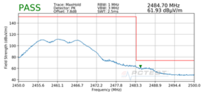
Plot 7-12. Radiated Restricted Upper Band Edge Measurement MIMO (Peak)
