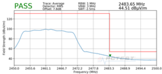
Plot 7-7. Radiated Restricted Upper Band Edge Measurement SISO ANT2 (Average)
