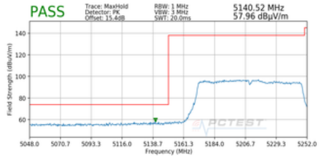
Plot 7-16. Radiated Lower Band Edge Plot SISO ANT1 (Peak – UNII Band 1)
