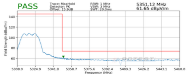
Plot 7-46. Radiated Upper Band Edge Plot MIMO (Peak – UNII Band 2A)
