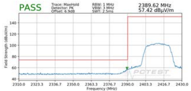
Plot 7-78. Radiated Restricted Lower Band Edge Measurement SISO ANT2 (Peak)
