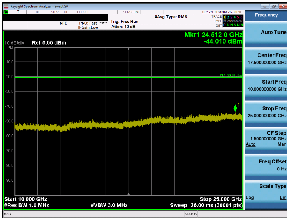
Plot 7-58. Conducted Spurious Plot SISO ANT2 (802.11b – Ch. 6)
