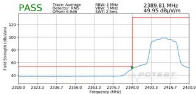
Plot 7-73. Radiated Restricted Lower Band Edge Measurement SISO ANT1 (Average)
