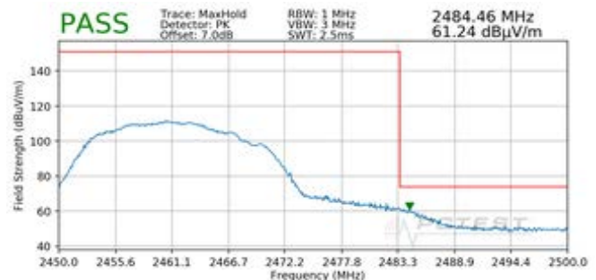
Plot 7-84. Radiated Restricted Upper Band Edge Measurement MIMO (Peak)
