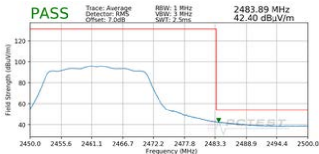
Plot 7-79. Radiated Restricted Upper Band Edge Measurement SISO ANT2 (Average)
