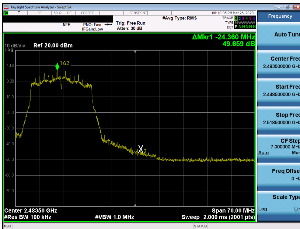
Plot 7-42. Band Edge Plot SISO ANT1 (802.11n (2.4GHz) – Ch. 11)
