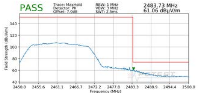
Plot 7-76. Radiated Restricted Upper Band Edge Measurement SISO ANT1 (Peak)
