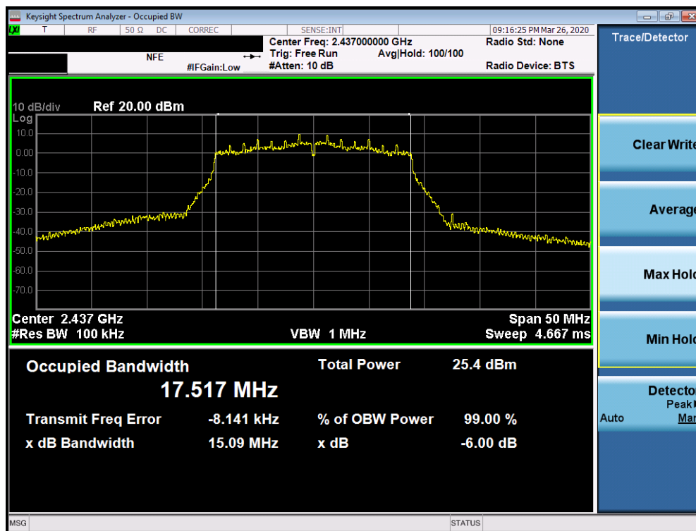
Plot 7-17. 6dB Bandwidth Plot SISO ANT1 (802.11n (2.4GHz) – Ch. 6)
