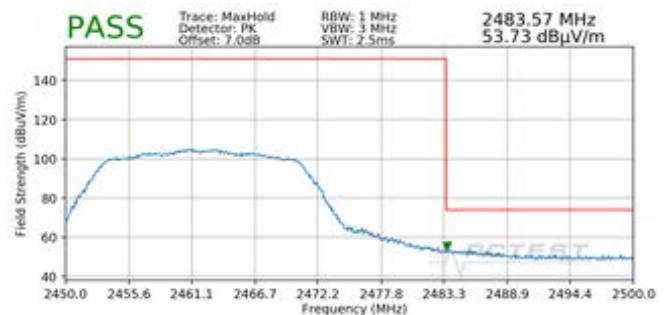
Plot 7-80. Radiated Restricted Upper Band Edge Measurement SISO ANT2 (Peak)
