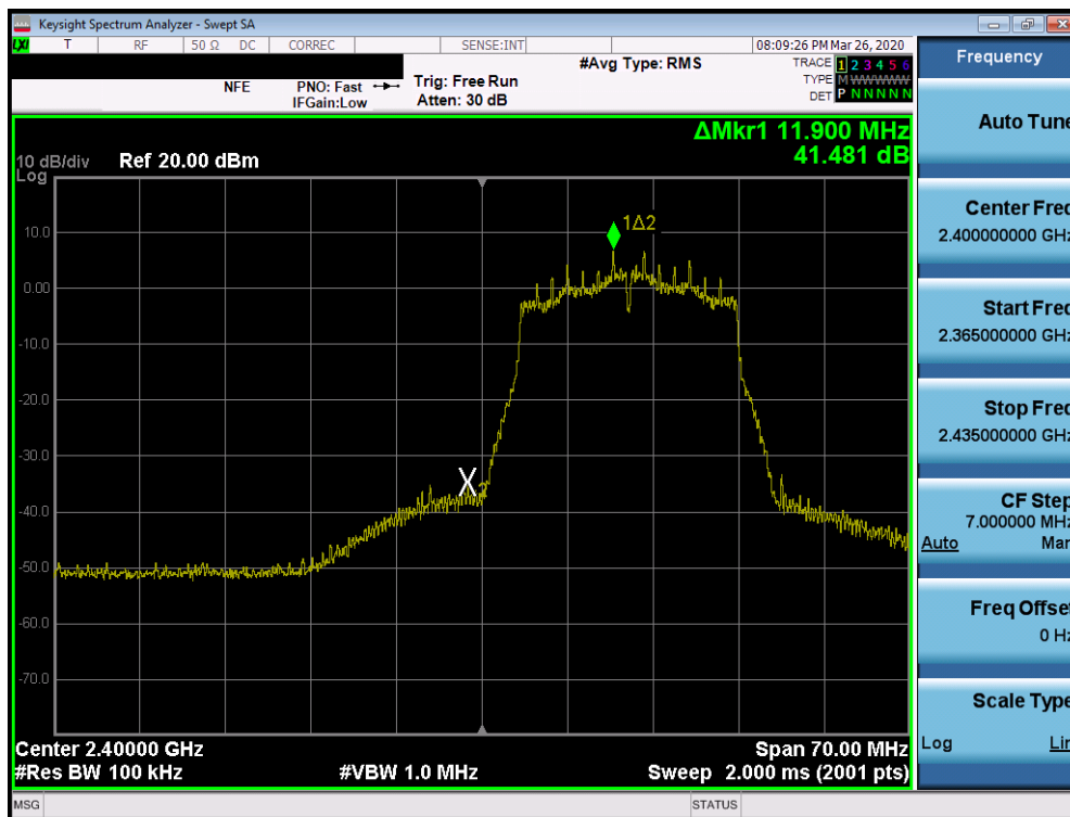
Plot 7-41. Band Edge Plot SISO ANT1 (802.11n (2.4GHz) – Ch. 1)
