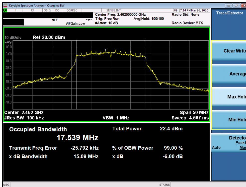
Plot 7-18. 6dB Bandwidth Plot SISO ANT1 (802.11n (2.4GHz) – Ch. 11)
