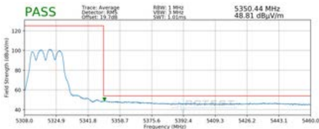
Plot 7-220. Radiated Upper Band Edge Plot MIMO (Average – UNII Band 2A)
