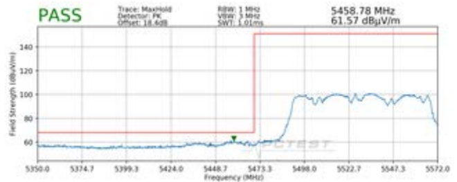
Plot 7-237. Radiated Lower Band Edge Plot MIMO (Peak – UNII Band 2C)
