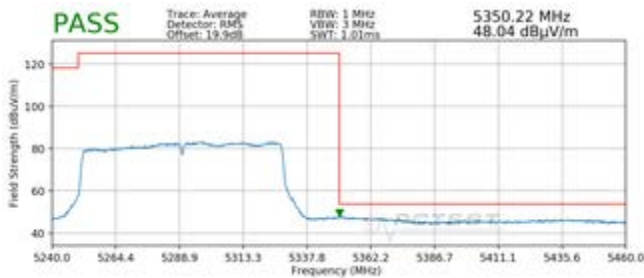
Plot 7-213. Radiated Upper Band Edge Plot SISO ANT2 (Average - UNII Band 2A)
