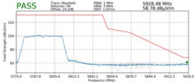
Plot 7-210. Radiated Upper Band Edge Plot SISO ANT2 (Peak - UNII Band 3)
