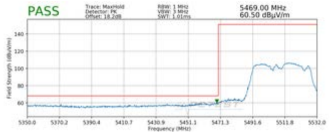
Plot 7-230. Radiated Lower Band Edge Plot MIMO (Peak – UNII Band 2C)
