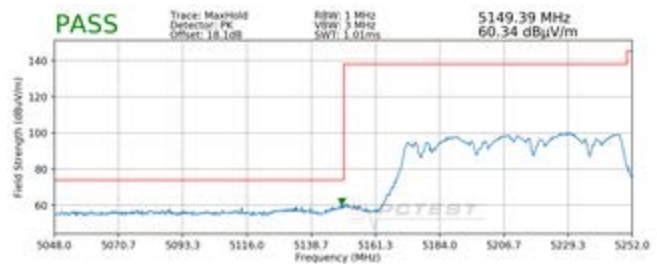
Plot 7-233. Radiated Lower Band Edge Plot MIMO (Peak – UNII Band 1)
