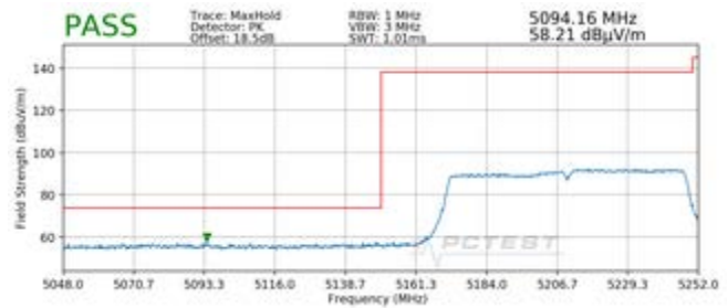
Plot 7-212. Radiated Lower Band Edge Plot SISO ANT2 (Peak - UNII Band 1)
