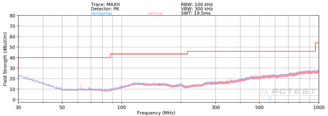
Plot 7-239. Radiated Spurious Plot below 1GHz MIMO-CDD (802.11a – U3 Ch. 157)
