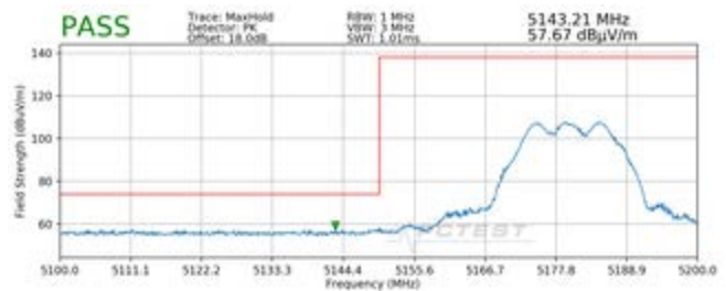
Plot 7-219. Radiated Lower Band Edge Plot MIMO (Peak – UNII Band 1)
