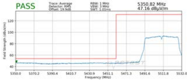
Plot 7-208. Radiated Lower Band Edge Plot SISO ANT2 (Average - UNII Band 2C)
