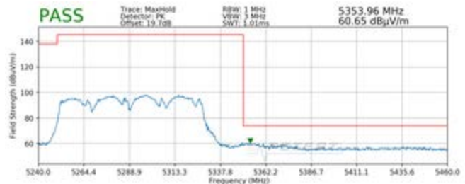
Plot 7-235. Radiated Upper Band Edge Plot MIMO (Peak – UNII Band 2A)
