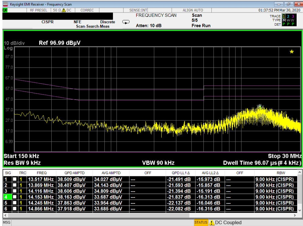
Plot 7-243. Line Conducted Plot with 802.11a UNII Band 2A (L1)
