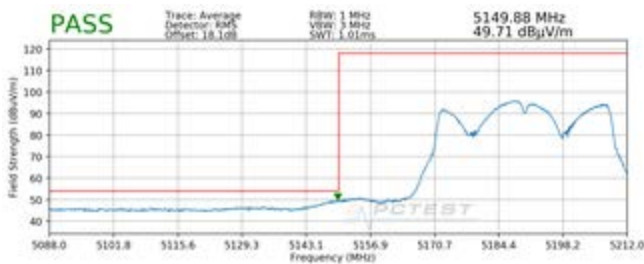
Plot 7-225. Radiated Lower Band Edge Plot MIMO (Average – UNII Band 1)
