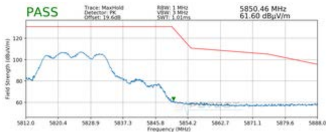
Plot 7-224. Radiated Upper Band Edge Plot MIMO (Peak – UNII Band 3)
