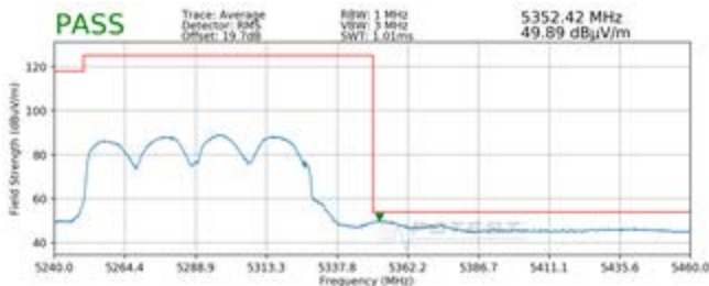
Plot 7-234. Radiated Upper Band Edge Plot MIMO (Average – UNII Band 2A)
