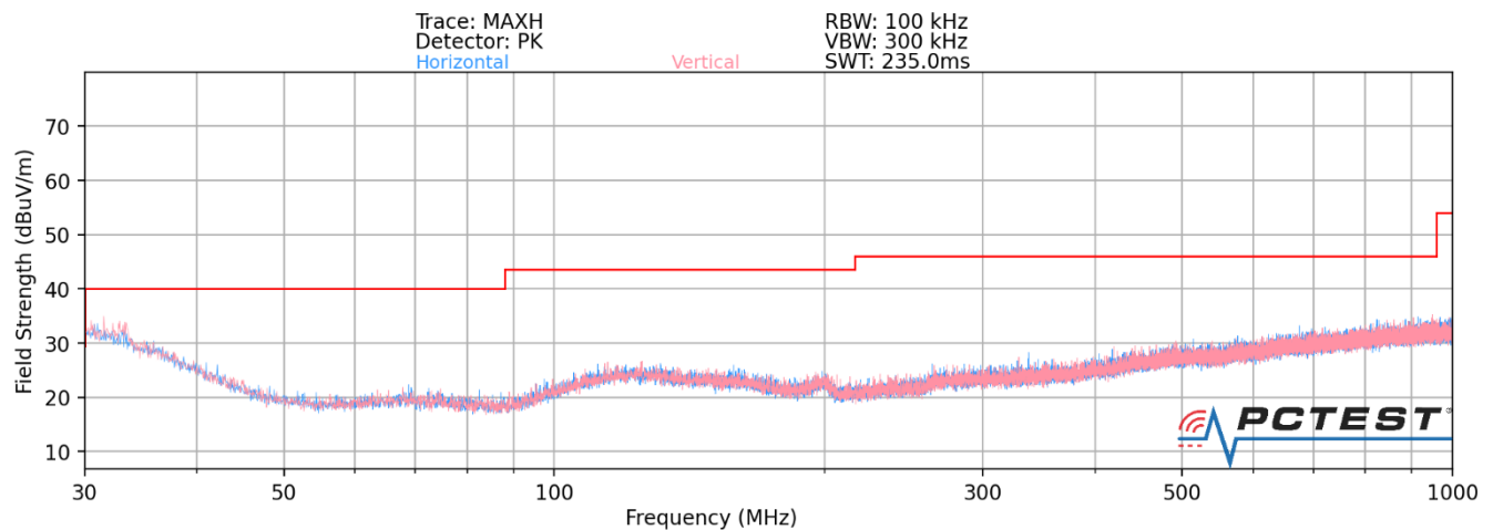
Plot 7-240. Radiated Spurious Plot below 1GHz (2.4GHz – 5GHz)
