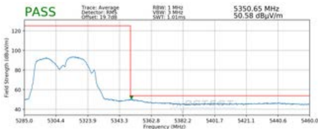
Plot 7-227. Radiated Upper Band Edge Plot MIMO (Average – UNII Band 2A)
