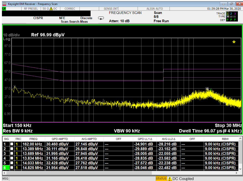
Plot 7-244. Line Conducted Plot with 802.11a UNII Band 2A (N)
