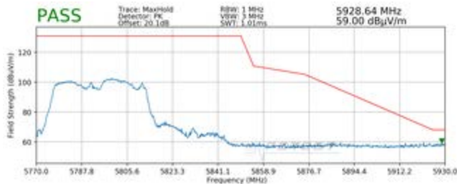
Plot 7-231. Radiated Upper Band Edge Plot MIMO (Peak – UNII Band 3)
