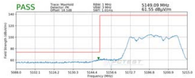
Plot 7-226. Radiated Lower Band Edge Plot MIMO (Peak – UNII Band 1)
