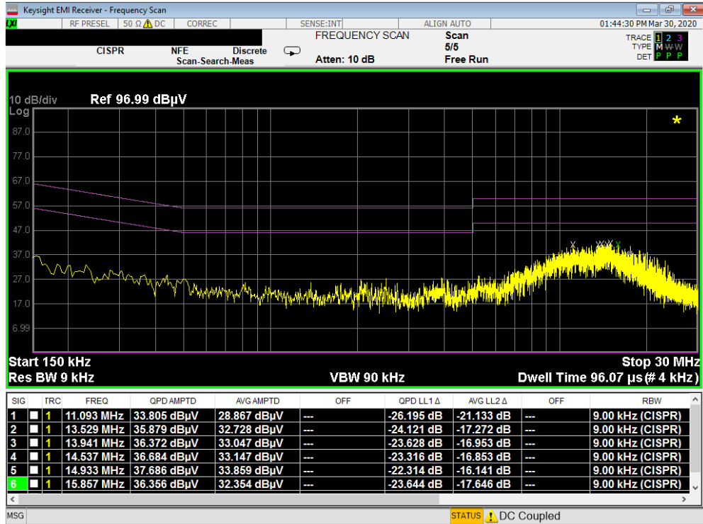
Plot 7-247. Line Conducted Plot with 802.11a UNII Band 3 (L1)
