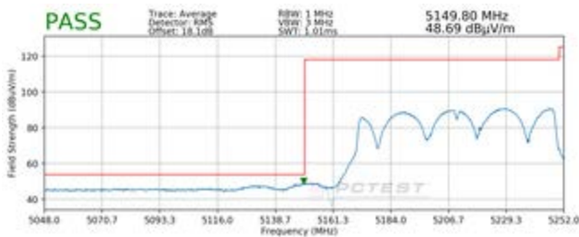
Plot 7-232. Radiated Lower Band Edge Plot MIMO (Average – UNII Band 1)
