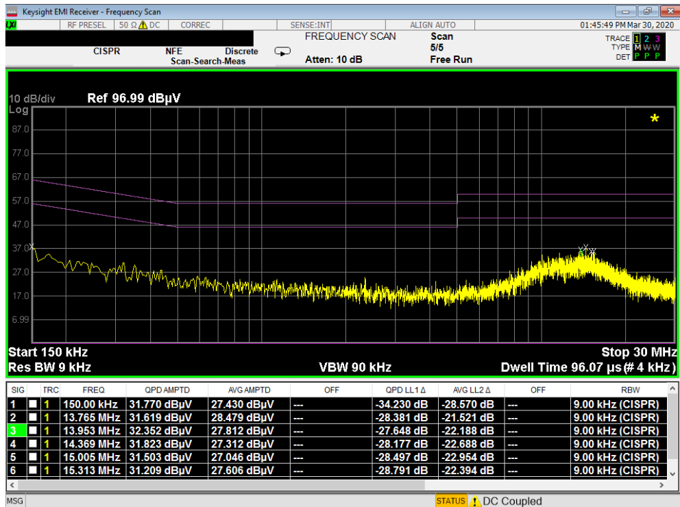
Plot 7-248. Line Conducted Plot with 802.11a UNII Band 3 (N)
