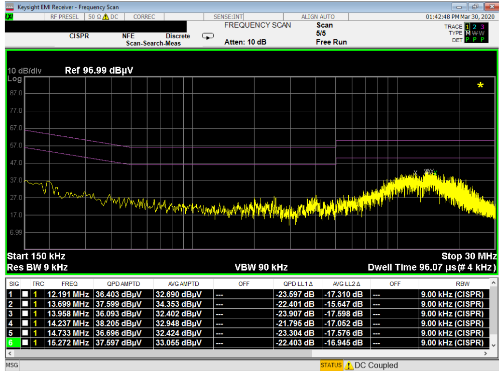
Plot 7-245. Line Conducted Plot with 802.11a UNII Band 2C (L1)
