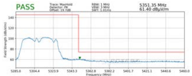
Plot 7-228. Radiated Upper Band Edge Plot MIMO (Peak – UNII Band 2A)
