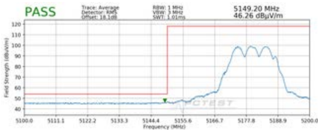
Plot 7-218. Radiated Lower Band Edge Plot MIMO (Average – UNII Band 1)
