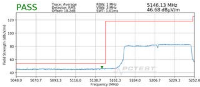
Plot 7-211. Radiated Lower Band Edge Plot SISO ANT2 (Average - UNII Band 1)
