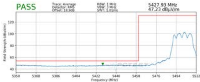
Plot 7-222. Radiated Lower Band Edge Plot MIMO (Average – UNII Band 2C)
