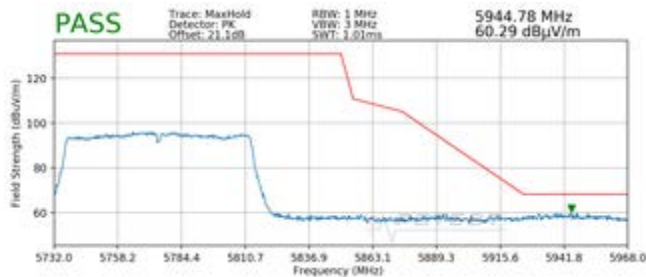
Plot 7-217. Radiated Upper Band Edge Plot SISO ANT2 (Peak - UNII Band 3)
