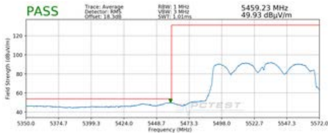
Plot 7-236. Radiated Lower Band Edge Plot MIMO (Average – UNII Band 2C)
