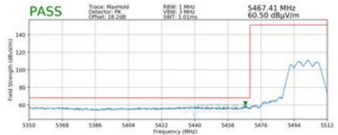
Plot 7-223. Radiated Lower Band Edge Plot MIMO (Peak – UNII Band 2C)
