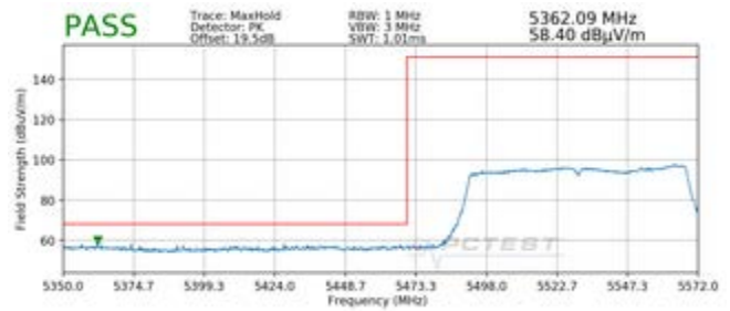
Plot 7-216. Radiated Lower Band Edge Plot SISO ANT2 (Peak - UNII Band 2C)
