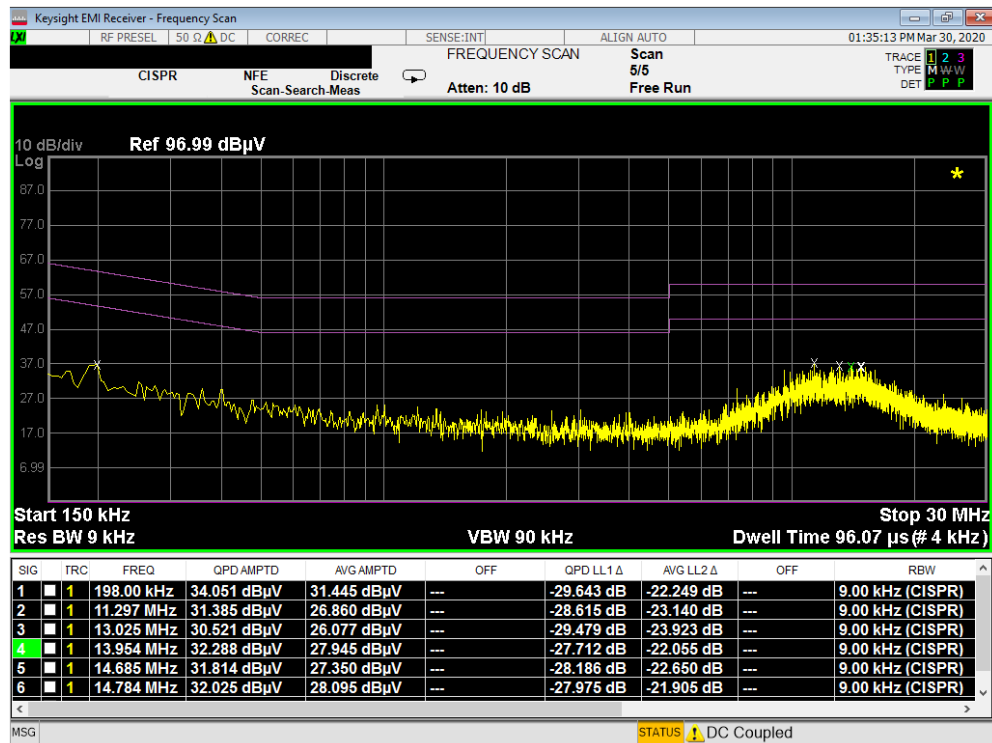
Plot 7-242. Line Conducted Plot with 802.11a UNII Band 1 (N)
