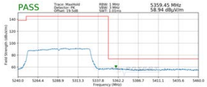
Plot 7-214. Radiated Upper Band Edge Plot SISO ANT2 (Peak - UNII Band 2A)
