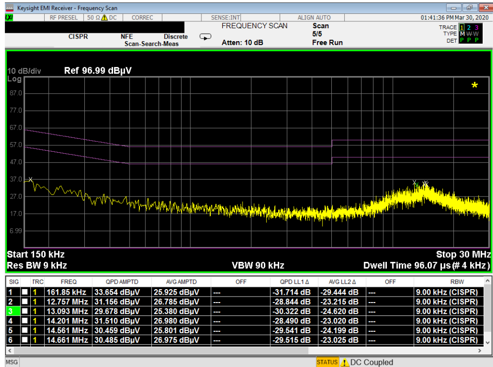
Plot 7-246. Line Conducted Plot with 802.11a UNII Band 2C (N)
