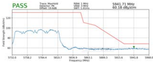
Plot 7-238. Radiated Upper Band Edge Plot MIMO (Peak – UNII Band 3)
