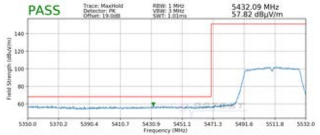
Plot 7-209. Radiated Lower Band Edge Plot SISO ANT2 (Peak - UNII Band 2C)
