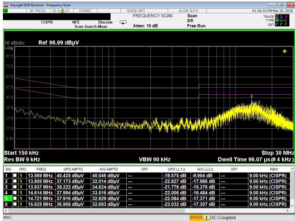
Plot 7-241. Line Conducted Plot with 802.11a UNII Band 1 (L1)
