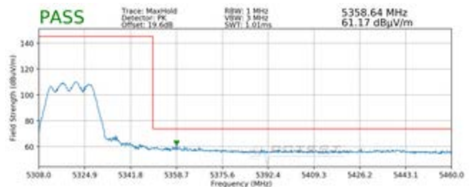
Plot 7-221. Radiated Upper Band Edge Plot MIMO (Peak – UNII Band 2A)
