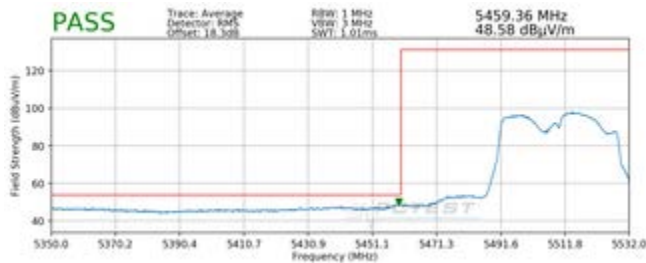
Plot 7-229. Radiated Lower Band Edge Plot MIMO (Average – UNII Band 2C)
