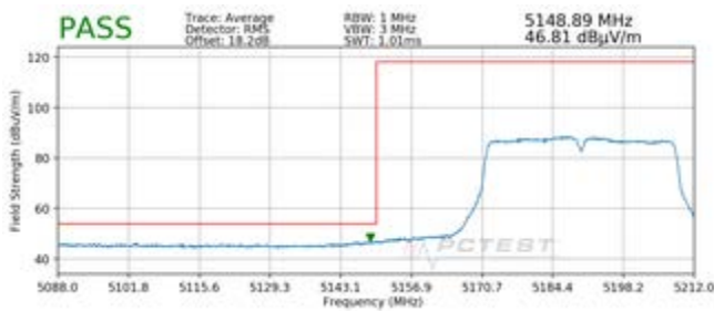
Plot 7-204. Radiated Lower Band Edge Plot SISO ANT2 (Average - UNII Band 1)
