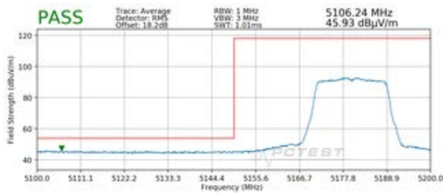
Plot 7-197. Radiated Lower Band Edge Plot SISO ANT2 (Average - UNII Band 1)
