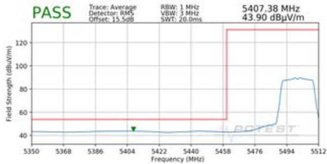
Plot 7-180. Radiated Lower Band Edge Plot SISO ANT1 (Average – UNII Band 2C)
