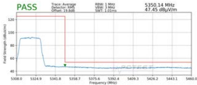
Plot 7-199. Radiated Upper Band Edge Plot SISO ANT2 (Average - UNII Band 2A)
