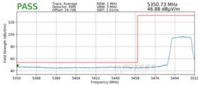
Plot 7-201. Radiated Lower Band Edge Plot SISO ANT2 (Average - UNII Band 2C)
