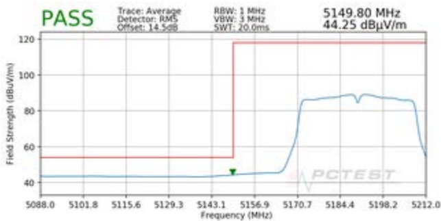
Plot 7-183. Radiated Lower Band Edge Plot SISO ANT1 (Average – UNII Band 1)
