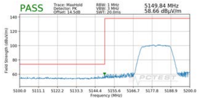
Plot 7-177. Radiated Lower Band Edge Plot SISO ANT1 (Peak – UNII Band 1)
