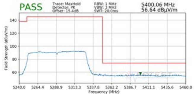
Plot 7-193. Radiated Upper Band Edge Plot SISO ANT1 (Peak – UNII Band 2A)
