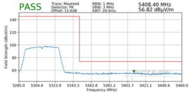
Plot 7-186. Radiated Upper Band Edge Plot SISO ANT1 (Peak – UNII Band 2A)
