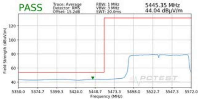
Plot 7-194. Radiated Lower Band Edge Plot SISO ANT1 (Average – UNII Band 2C)
