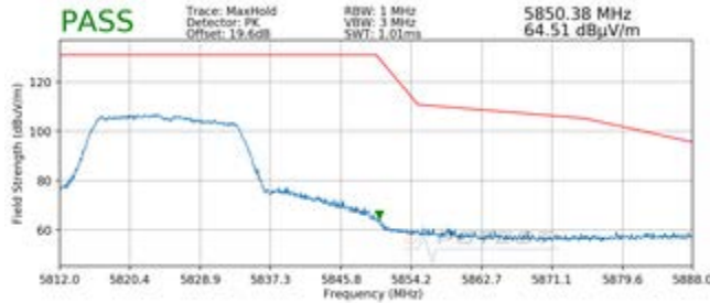
Plot 7-203. Radiated Upper Band Edge Plot SISO ANT2 (Peak - UNII Band 3)
