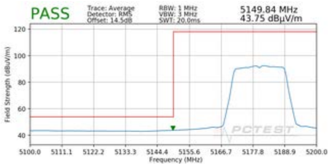
Plot 7-176. Radiated Lower Band Edge Plot SISO ANT1 (Average – UNII Band 1)
