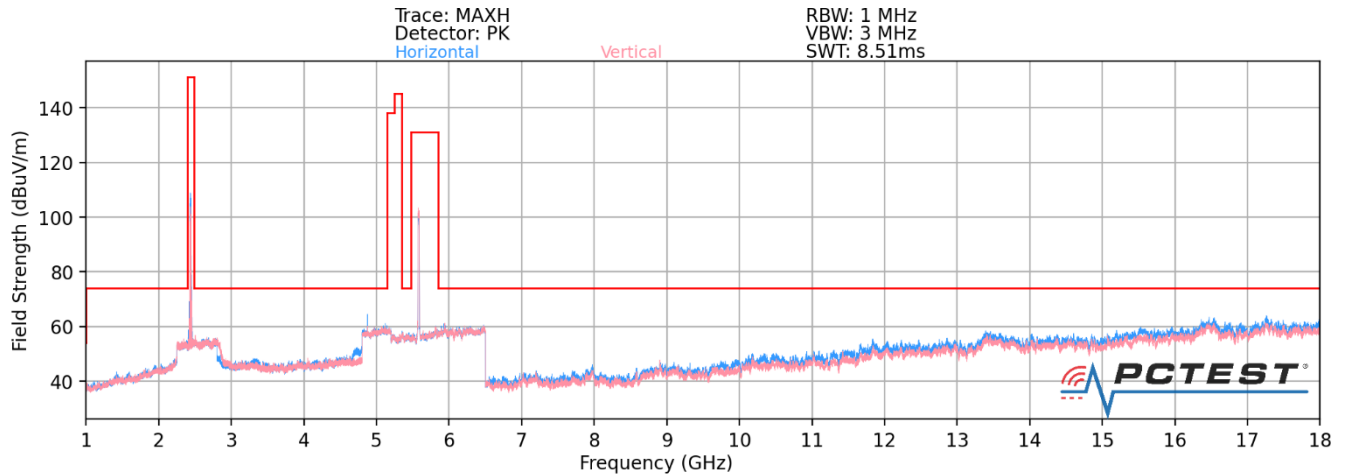
Plot 7-173. Radiated Spurious Plot above 1GHz (2.4GHz – 5GHz)
