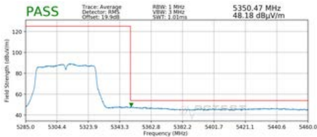
Plot 7-206. Radiated Upper Band Edge Plot SISO ANT2 (Average - UNII Band 2A)
