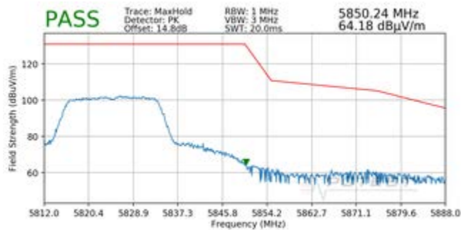
Plot 7-182. Radiated Upper Band Edge Plot SISO ANT1 (Peak – UNII Band 3)
