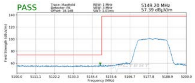
Plot 7-198. Radiated Lower Band Edge Plot SISO ANT2 (Peak - UNII Band 1)
