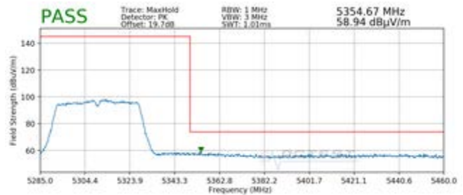
Plot 7-207. Radiated Upper Band Edge Plot SISO ANT2 (Peak - UNII Band 2A)
