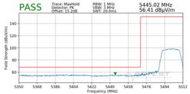
Plot 7-181. Radiated Lower Band Edge Plot SISO ANT1 (Peak – UNII Band 2C)
