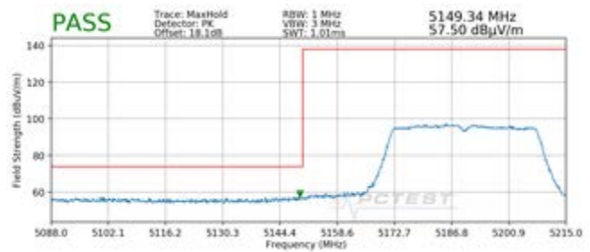
Plot 7-205. Radiated Lower Band Edge Plot SISO ANT2 (Peak - UNII Band 1)
