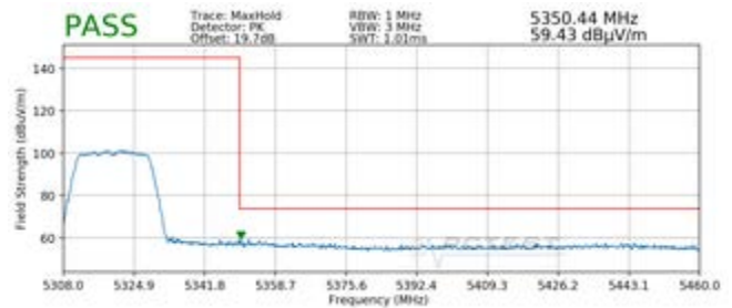
Plot 7-200. Radiated Upper Band Edge Plot SISO ANT2 (Peak - UNII Band 2A)
