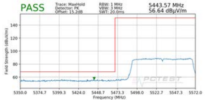
Plot 7-195. Radiated Lower Band Edge Plot SISO ANT1 (Peak – UNII Band 2C)
