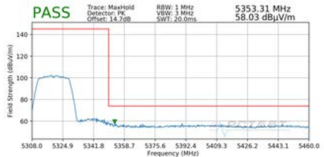
Plot 7-179. Radiated Upper Band Edge Plot SISO ANT1 (Peak – UNII Band 2A)
