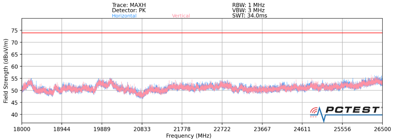
Plot 7-174. Radiated Spurious Plot above 18GHz (2.4GHz – 5GHz)
