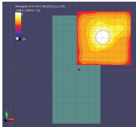
Figure 12-2 4cm 2 psPD distribution measured at input.power.limit of 4.4 dBm on the back surface for n260 beam 31
