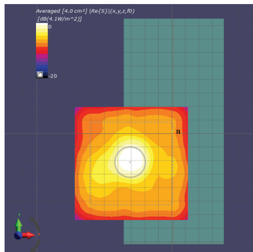
Figure 12-2 4cm 2 psPD distribution measured at input.power.limit of 4.4 dBm on the back surface for n260 beam 31
