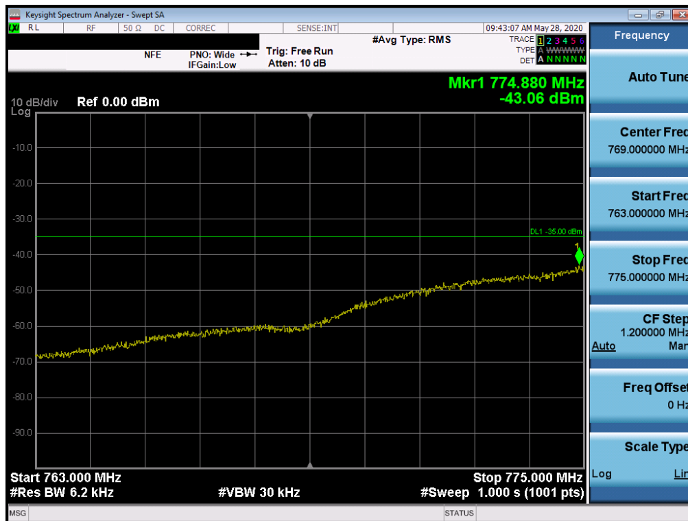
Plot 7-132. Lower Emission Mask Plot (LTE Band 13 - 10MHz QPSK – Full RB Configuration)
