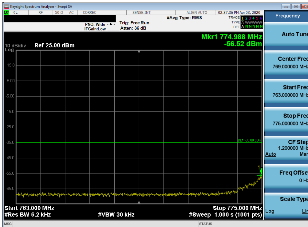
Plot 7-136. Lower Emission Mask Plot (LTE Band 13 - 5MHz QPSK – Full RB Configuration)
