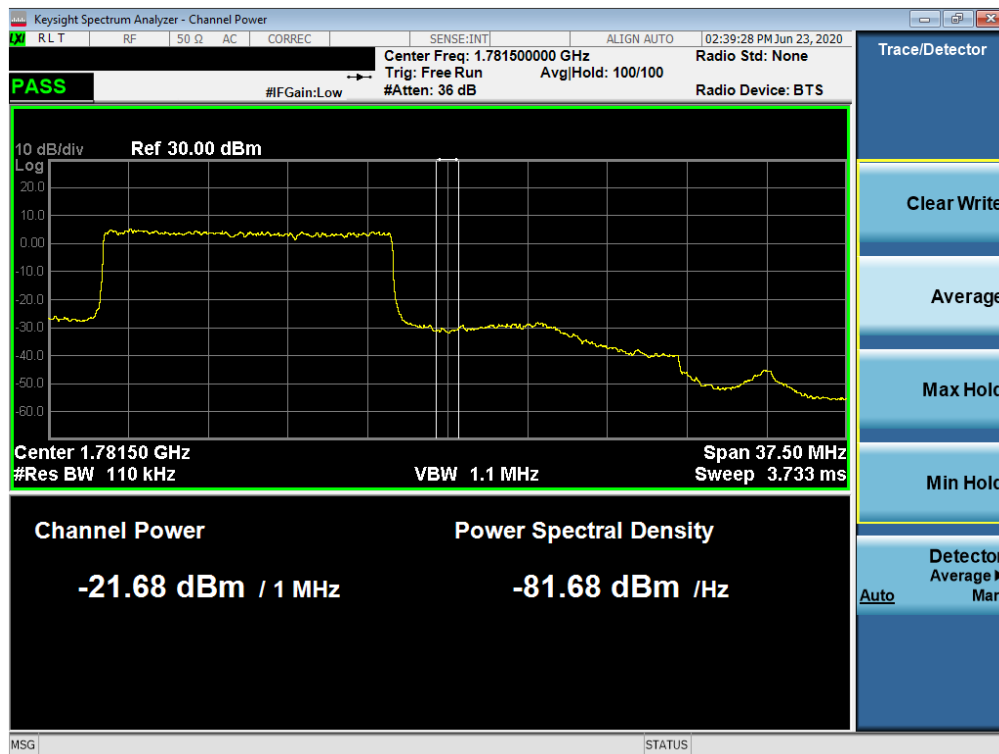
Plot 7-146. Upper Extended Band Edge Plot (NR Band n66 – 15.0MHz - Full RB)
