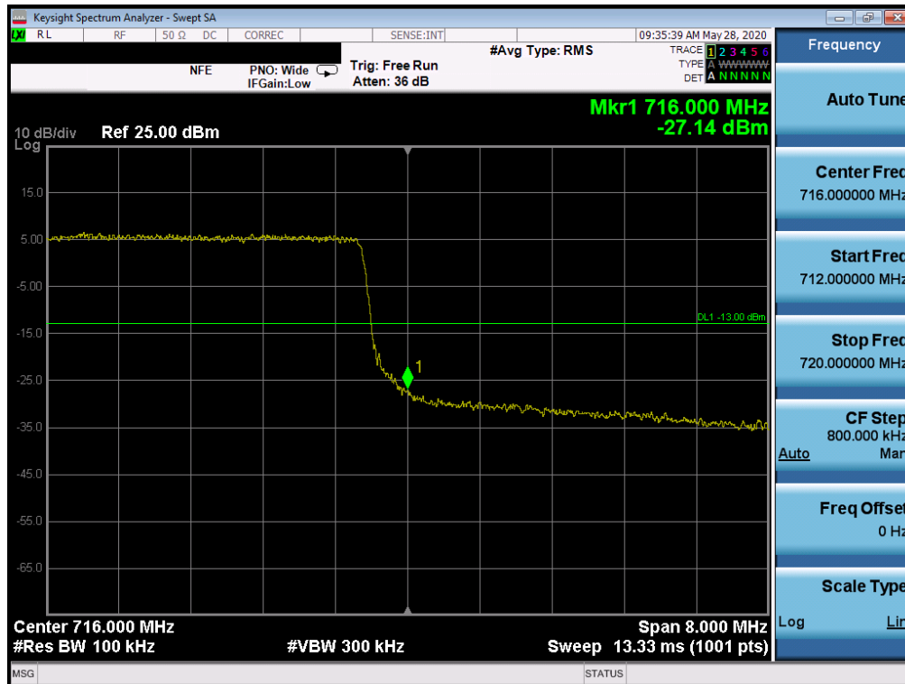
Plot 7-124. Upper Band Edge Plot (LTE Band 12 - 10MHz QPSK – Full RB Configuration)
