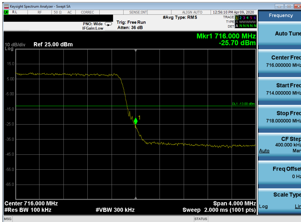
Plot 7-126. Upper Band Edge Plot (LTE Band 12 - 5MHz QPSK – Full RB Configuration)
