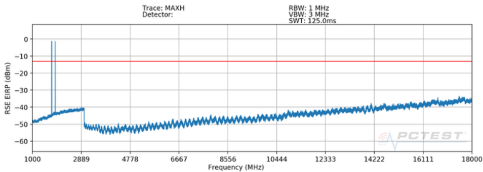
Plot 7-163. Radiated Spurious Plot (ENDC n66-LB2)
