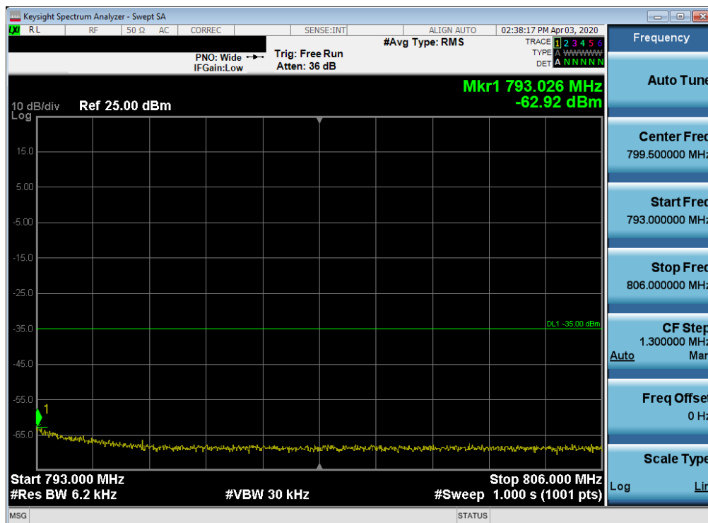
Plot 7-138. Upper Emission Mask Plot (LTE Band 13 - 5MHz QPSK – Full RB Configuration)
