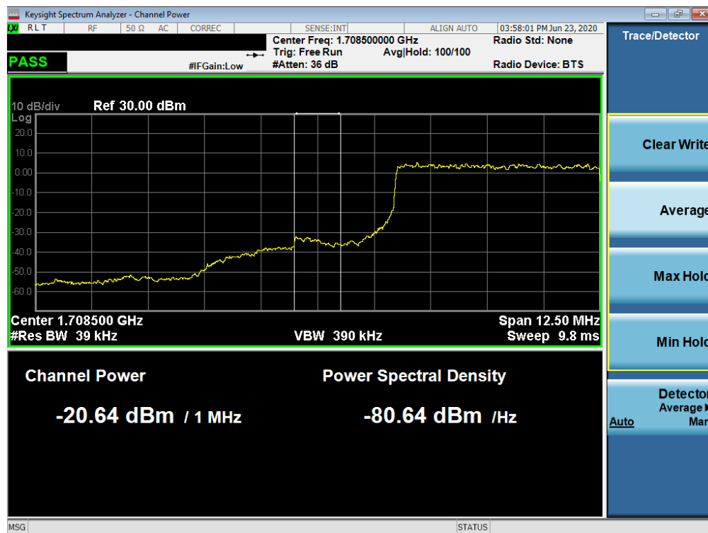
Plot 7-152. Lower Extended Band Edge Plot (NR Band n66 – 5.0MHz - Full RB)
