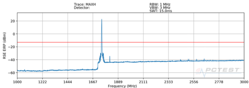
Plot 7-164. Radiated Spurious Plot (ENDC n66-LB5)
