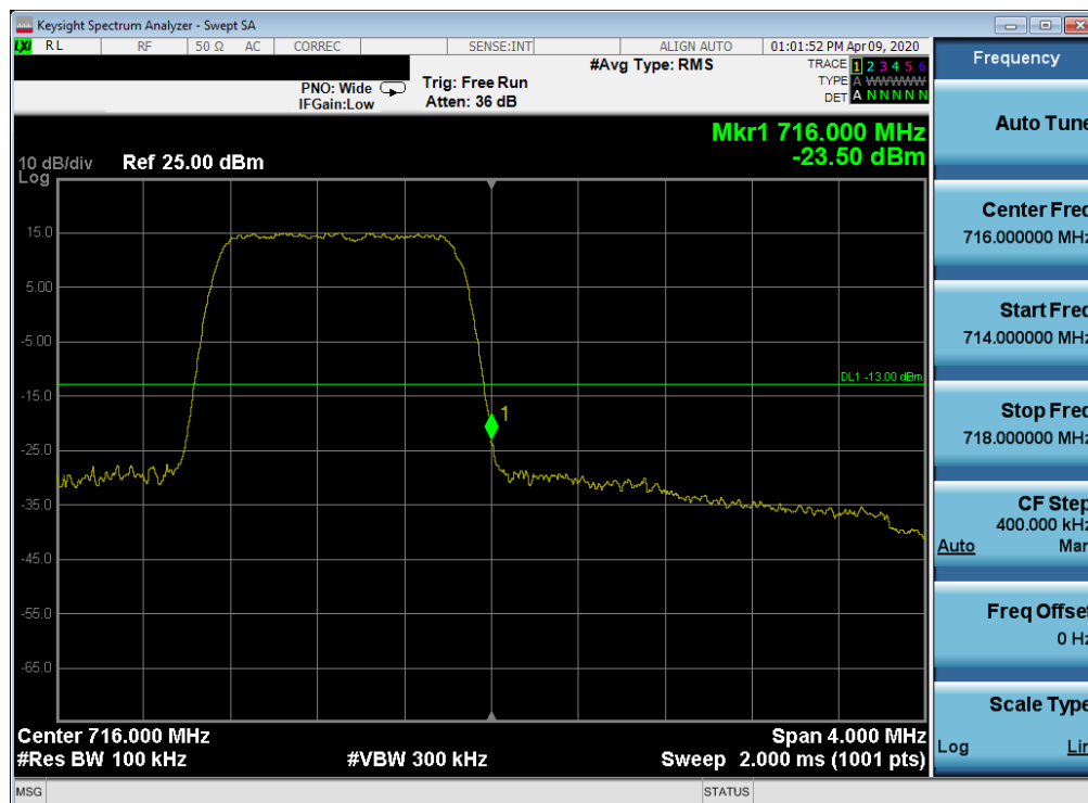
Plot 7-130. Upper Band Edge Plot (LTE Band 12 – 1.4MHz QPSK – Full RB Configuration)
