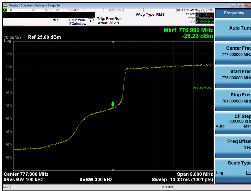
Plot 7-131. Lower Band Edge Plot (LTE Band 13 - 10MHz QPSK – Full RB Configuration)
