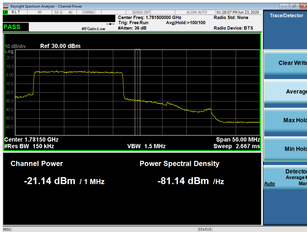
Plot 7-142. Upper Extended Band Edge Plot (NR Band n66 – 20.0MHz - Full RB)
