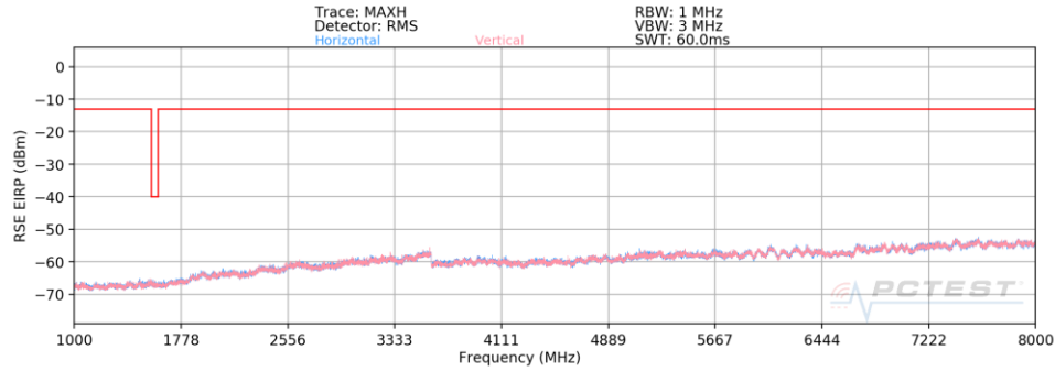
Plot 7-161. Radiated Spurious Plot (LTE Band 13)
