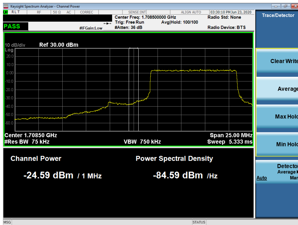
Plot 7-148. Lower Extended Band Edge Plot (NR Band n66 – 10.0MHz - Full RB)
