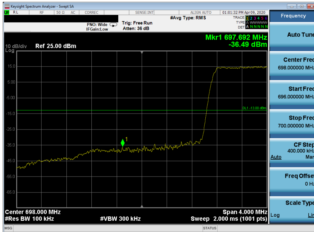
Plot 7-129. Lower Band Edge Plot (LTE Band 12 – 1.4MHz QPSK – Full RB Configuration)
