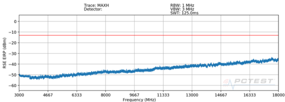
Plot 7-165. Radiated Spurious Plot (ENDC n66-LB5)
