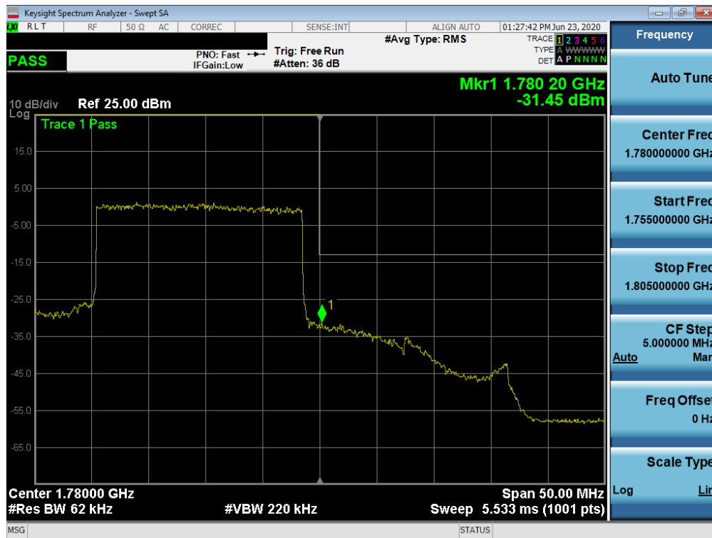
Plot 7-141. Upper Band Edge Plot (NR Band n66 – 20.0MHz - Full RB)
