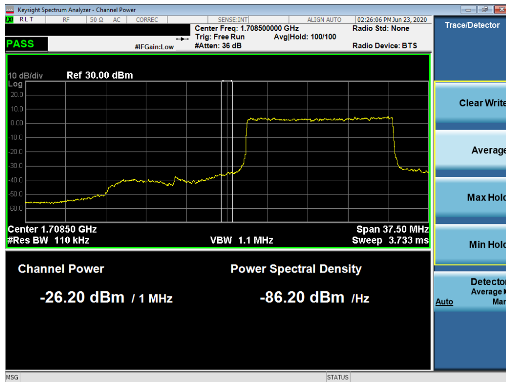
Plot 7-144. Lower Extended Band Edge Plot (NR Band n66 – 15.0MHz - Full RB)
