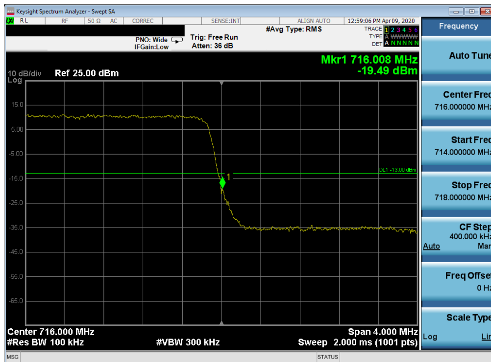
Plot 7-128. Upper Band Edge Plot (LTE Band 12 - 3MHz QPSK – Full RB Configuration)
