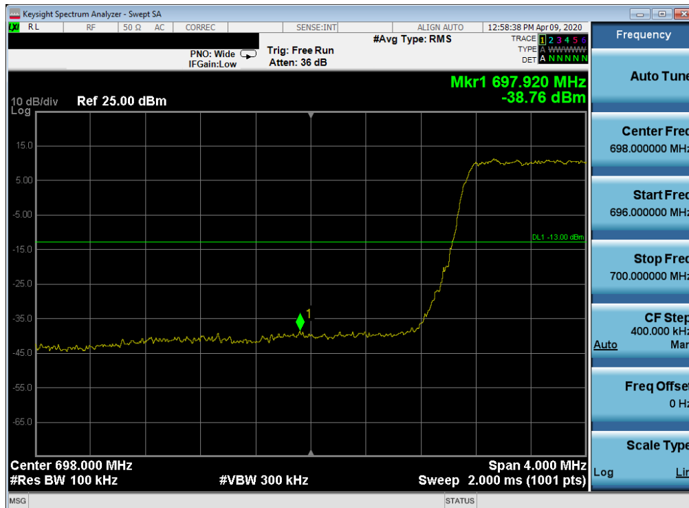
Plot 7-127. Lower Band Edge Plot (LTE Band 12 - 3MHz QPSK – Full RB Configuration)
