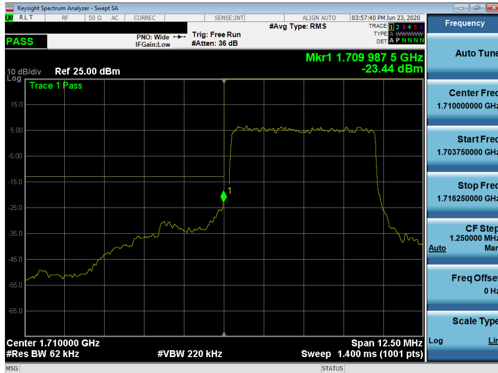
Plot 7-151. Lower Band Edge Plot (NR Band n66 – 5.0MHz - Full RB)
