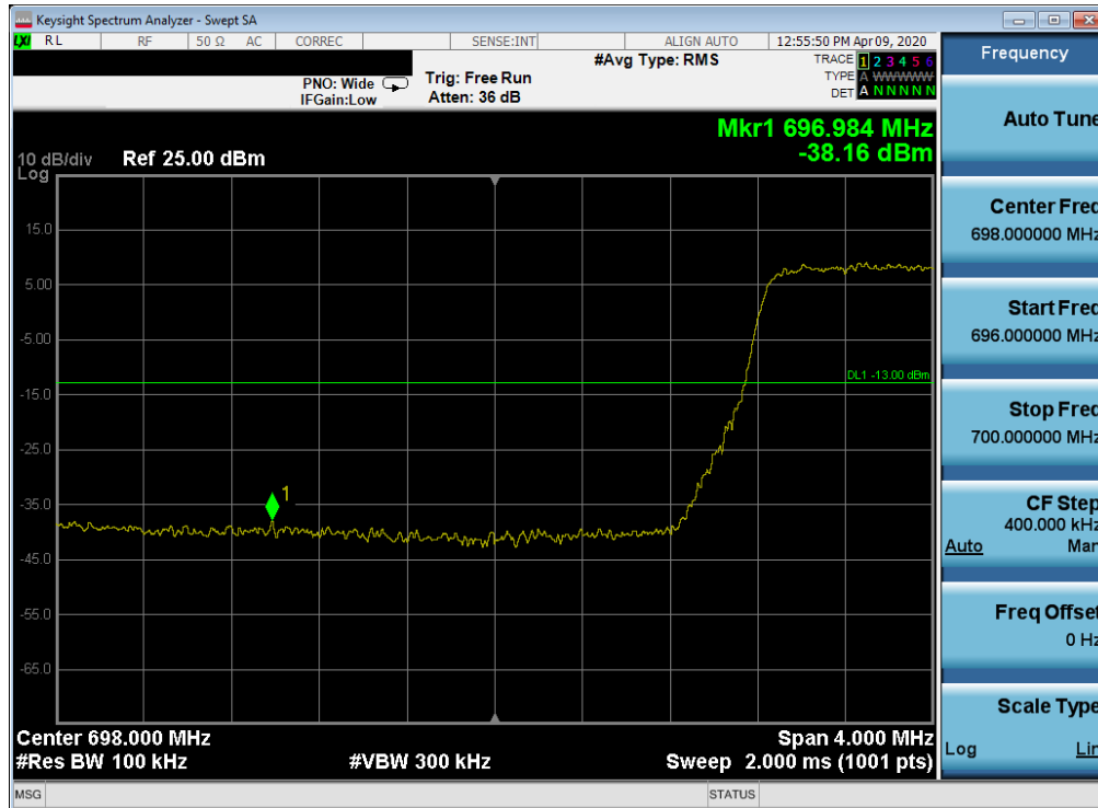
Plot 7-125. Lower Band Edge Plot (LTE Band 12 - 5MHz QPSK – Full RB Configuration)
