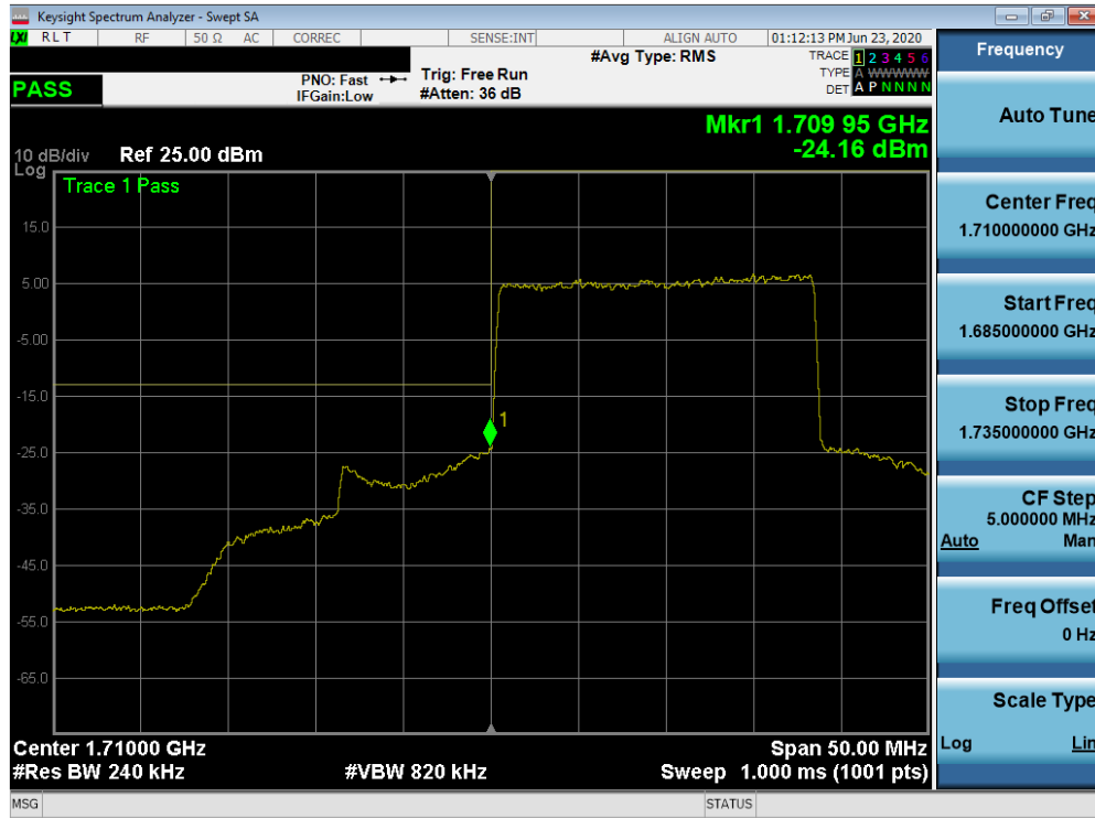
Plot 7-139. Lower Band Edge Plot (NR Band n66 – 20.0MHz - Full RB)
