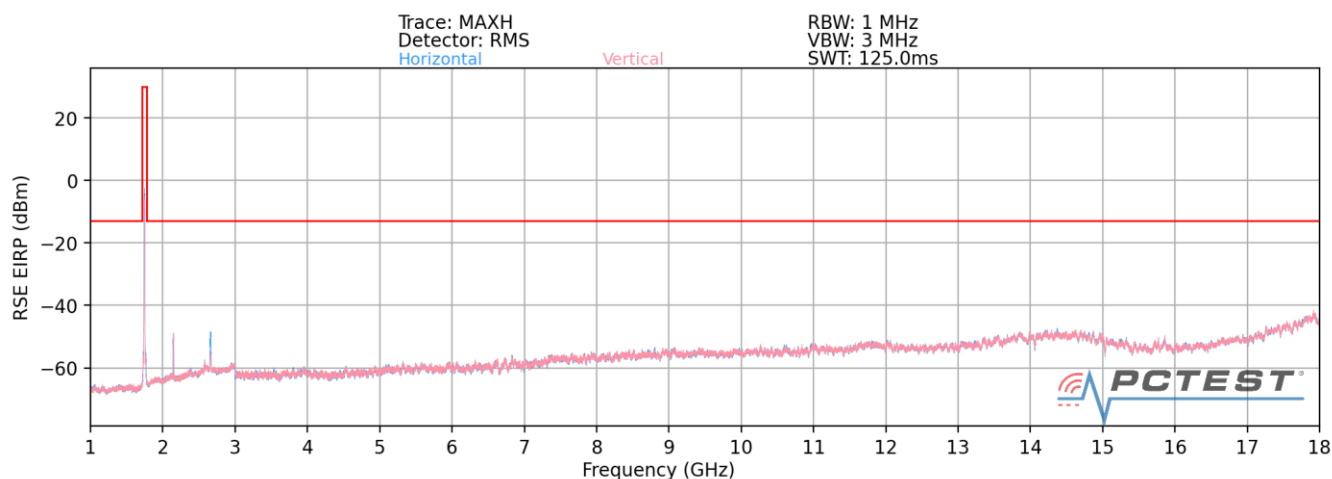
Plot 7-159. Radiated Spurious Plot (LTE Band 66/4)
