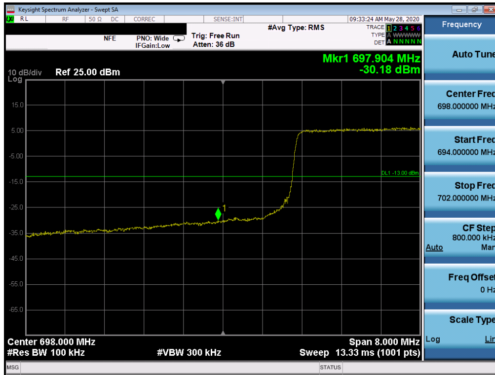
Plot 7-123. Lower Band Edge Plot (LTE Band 12 - 10MHz QPSK – Full RB Configuration)
