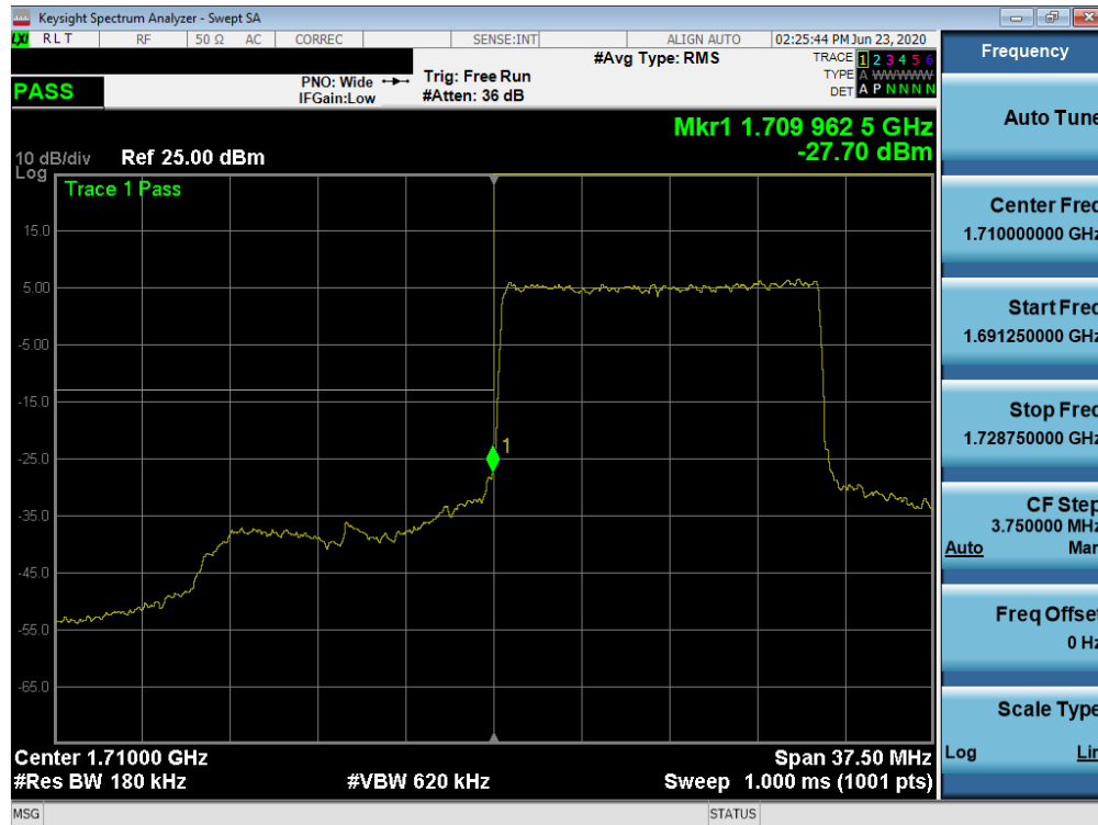
Plot 7-143. Lower Band Edge Plot (NR Band n66 – 15.0MHz - Full RB)
