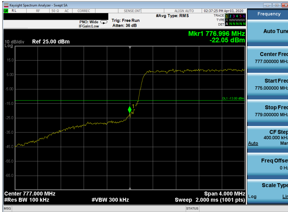
Plot 7-135. Lower Band Edge Plot (LTE Band 13 - 5MHz QPSK – Full RB Configuration)
