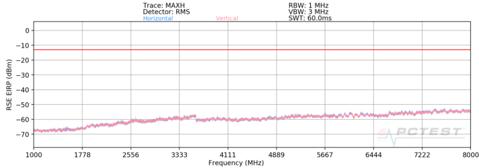
Plot 7-160. Radiated Spurious Plot (LTE Band 12)
