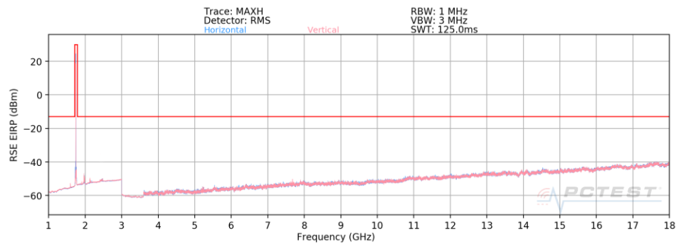
Plot 7-162. Radiated Spurious Plot (NR Band n66)
