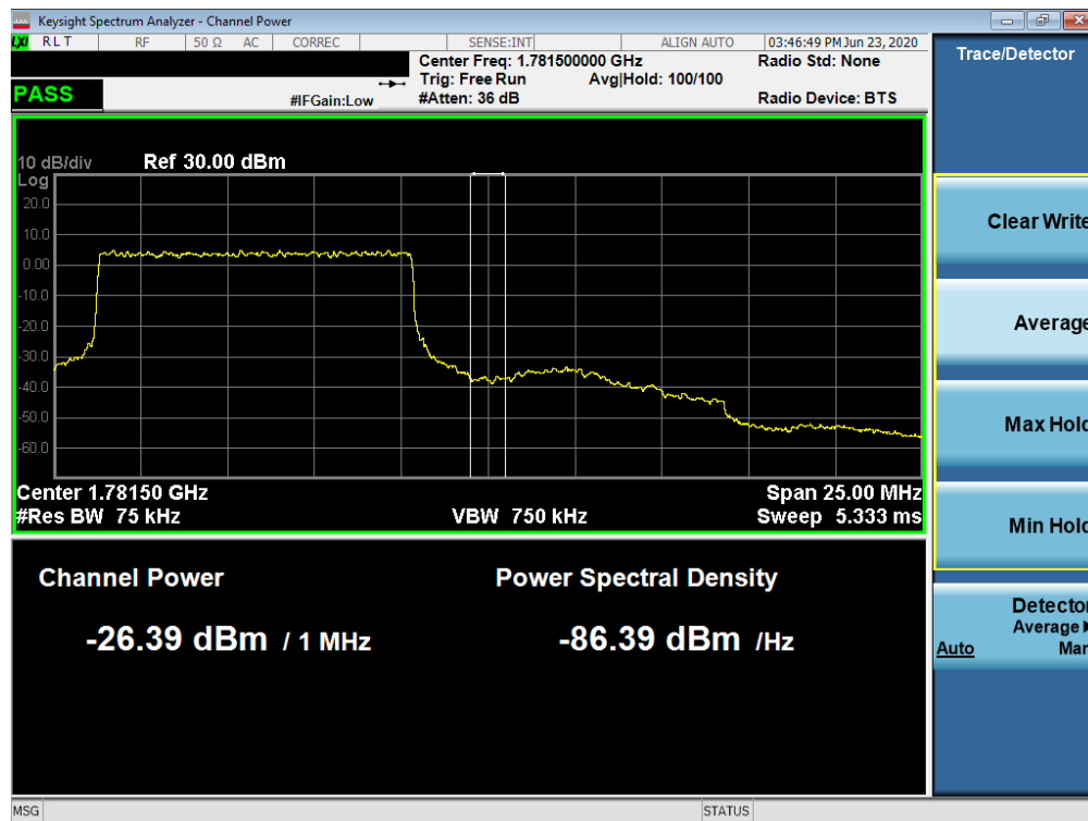
Plot 7-150. Upper Extended Band Edge Plot (NR Band n66 – 10.0MHz - Full RB)
