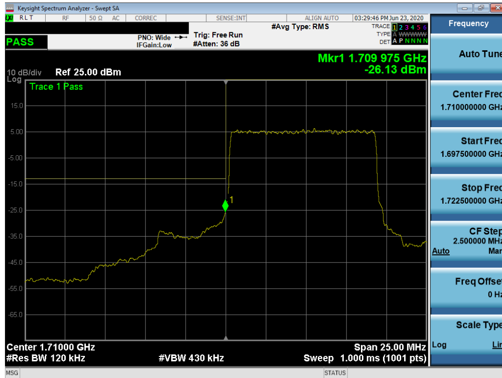
Plot 7-147. Lower Band Edge Plot (NR Band n66 – 10.0MHz - Full RB)
