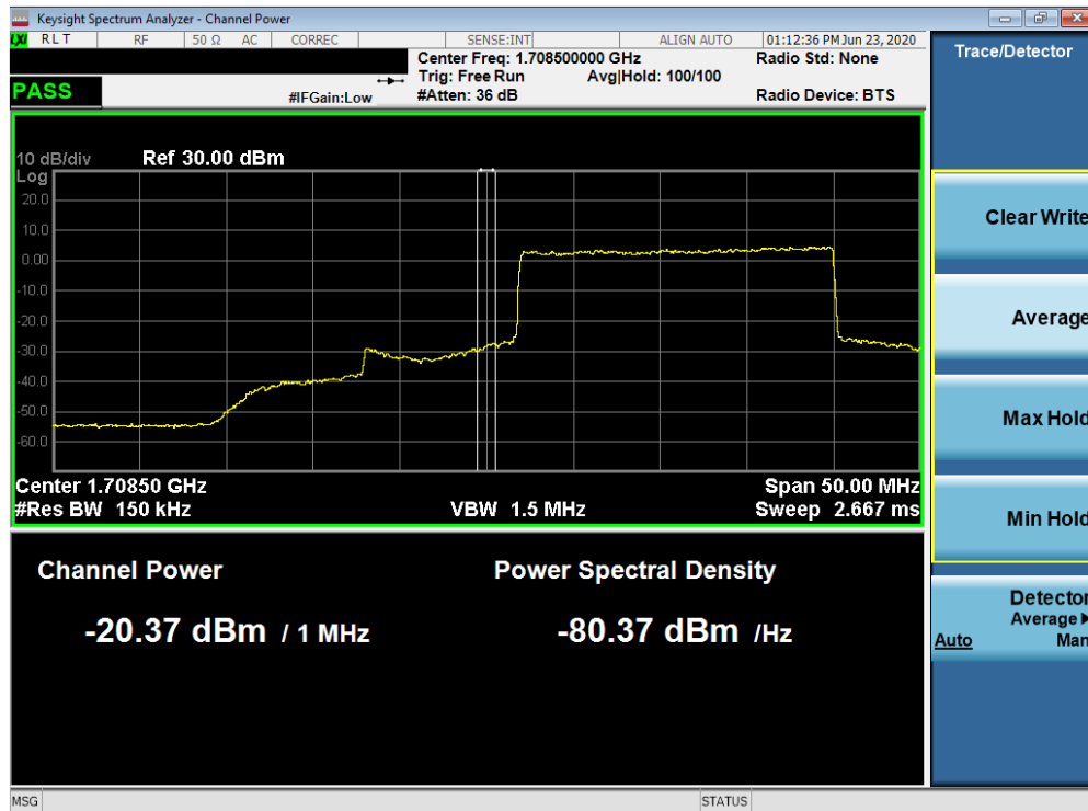
Plot 7-140. Lower Extended Band Edge Plot (NR Band n66 – 20.0MHz - Full RB)
