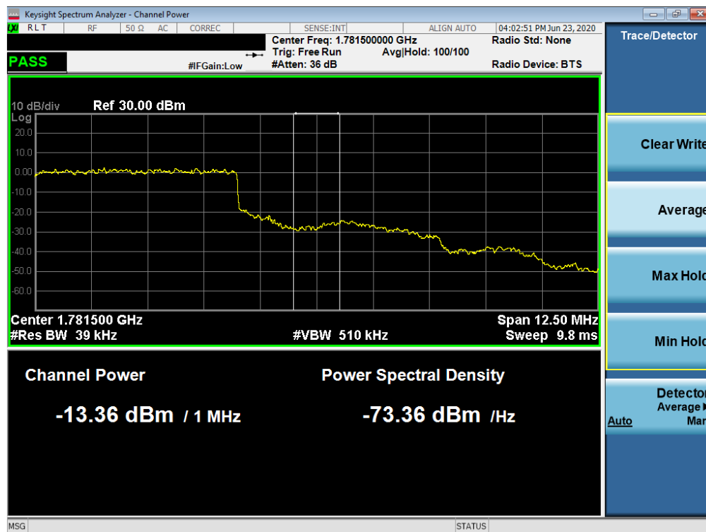
Plot 7-154. Upper Extended Band Edge Plot (NR Band n66 – 5.0MHz - Full RB)
