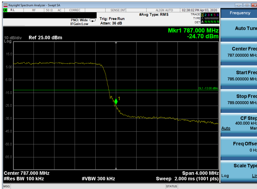
Plot 7-137. Upper Band Edge Plot (LTE Band 13 - 5MHz QPSK – Full RB Configuration)
