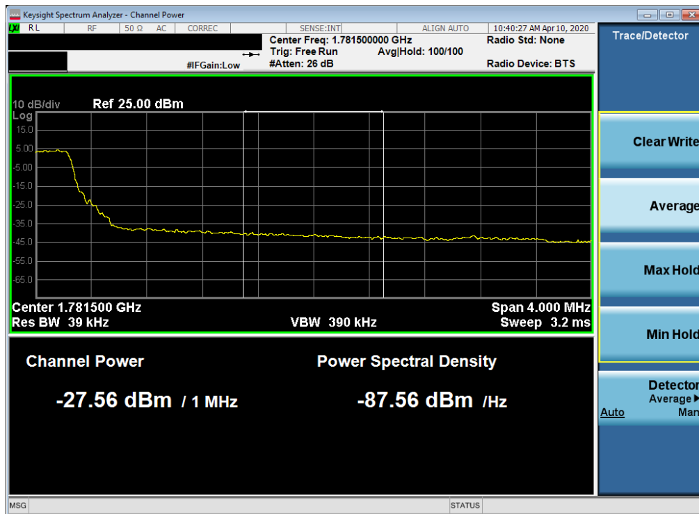
Plot 7-110. Upper Extended Band Edge Plot (LTE Band 66 - 5MHz QPSK – Full RB Configuration)
