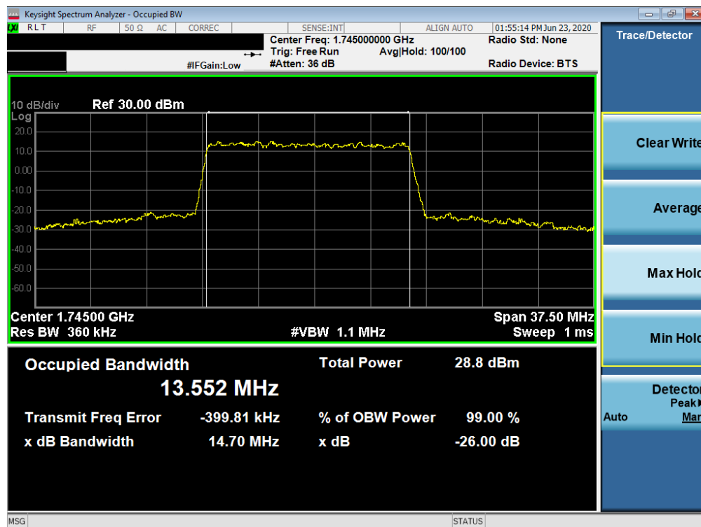
Plot 7-46. Occupied Bandwidth Plot (NR Band n66 - 15.0MHz CP-OFDM 256QAM - Full RB)
