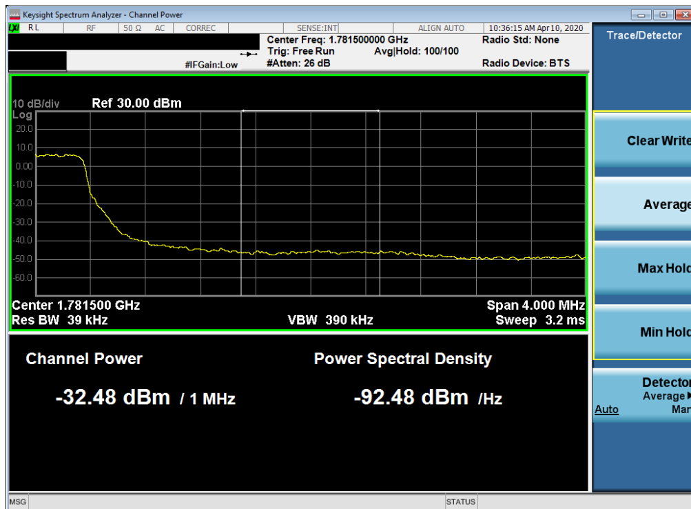
Plot 7-116. Upper Extended Band Edge Plot (LTE Band 66 - 3MHz QPSK – Full RB Configuration)
