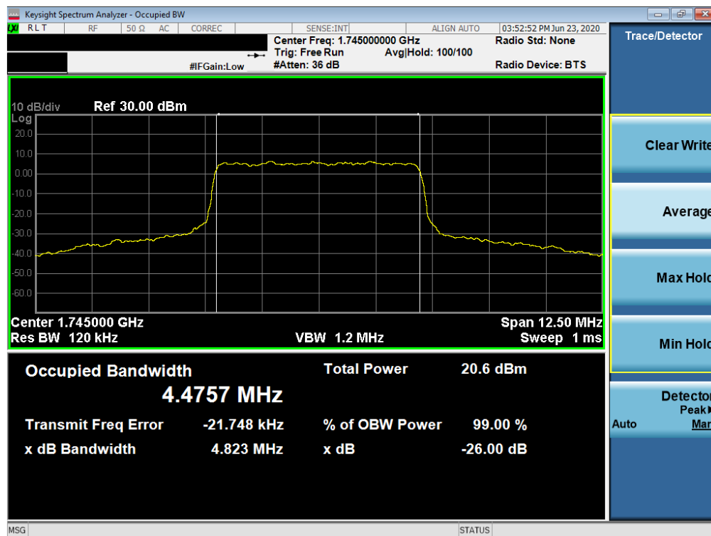
Plot 7-56. Occupied Bandwidth Plot (NR Band n66 - 5.0MHz CP-OFDM 256QAM - Full RB)
