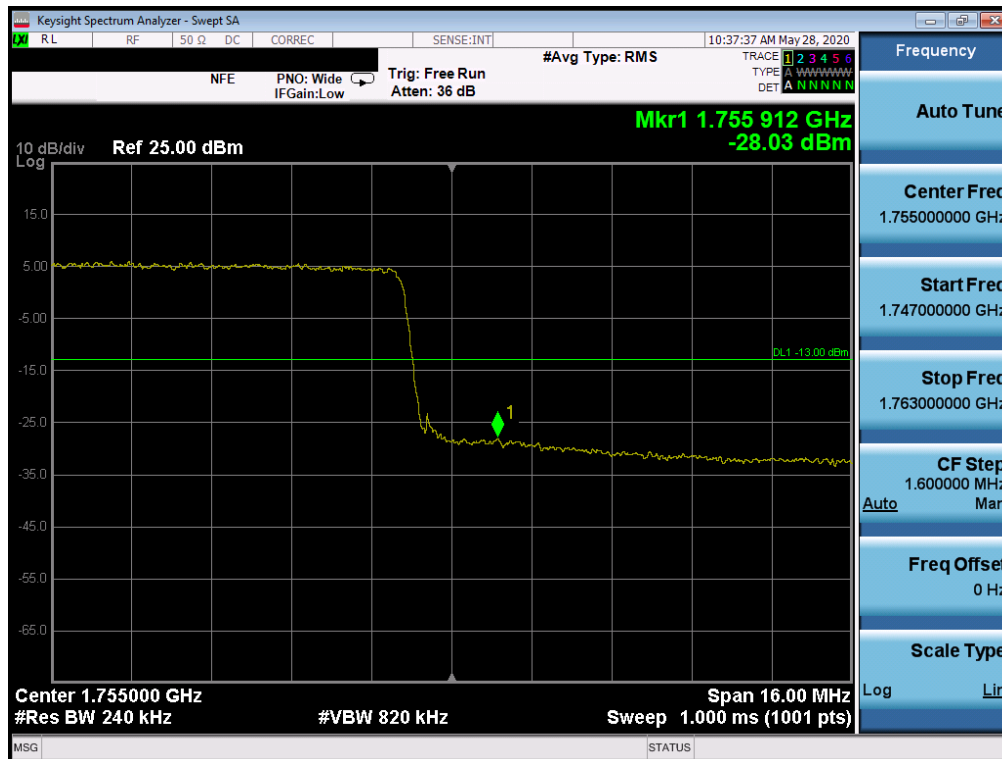
Plot 7-89. Upper Band Edge Plot (LTE Band 4 - 20MHz QPSK - Full RB Configuration)
