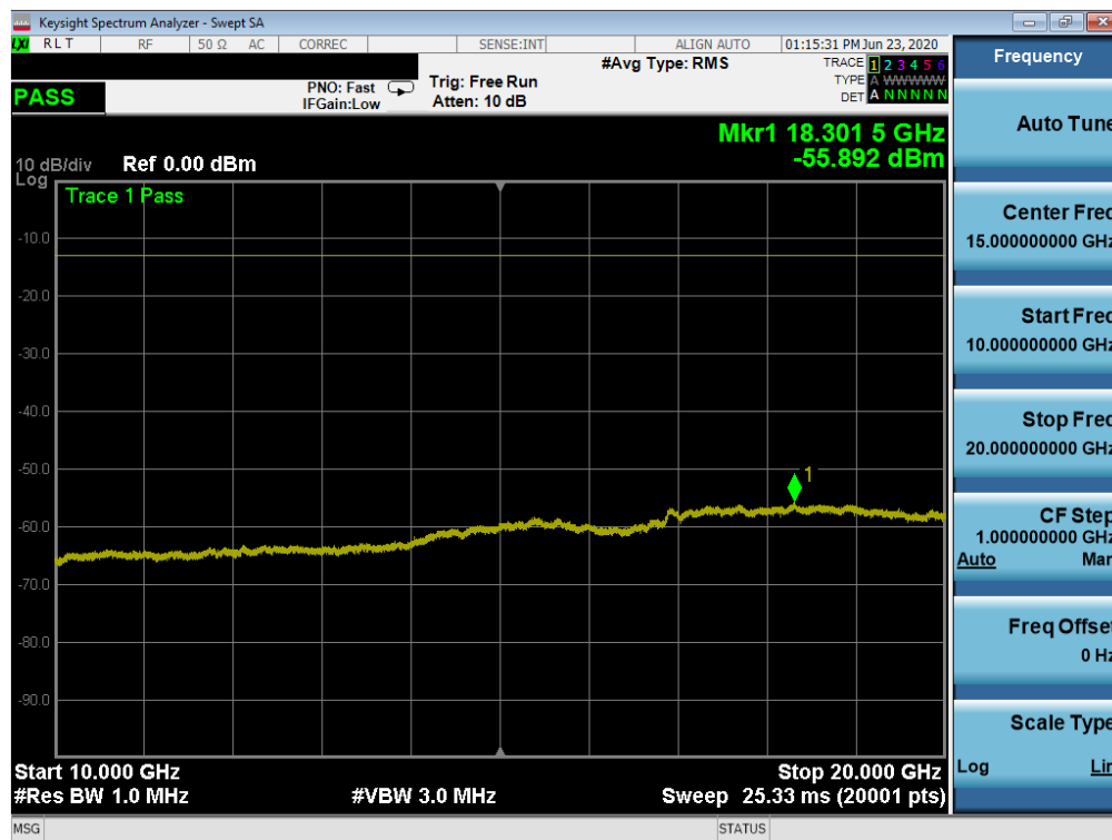
Plot 7-80. Conducted Spurious Plot (NR Band n66 - 20.0MHz - RB Size 1, RB Offset 0 - Low Channel)
