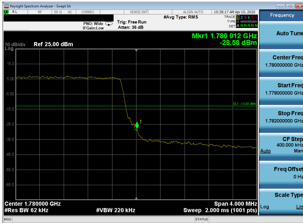
Plot 7-109. Upper Band Edge Plot (LTE Band 66 - 5MHz QPSK – Full RB Configuration)
