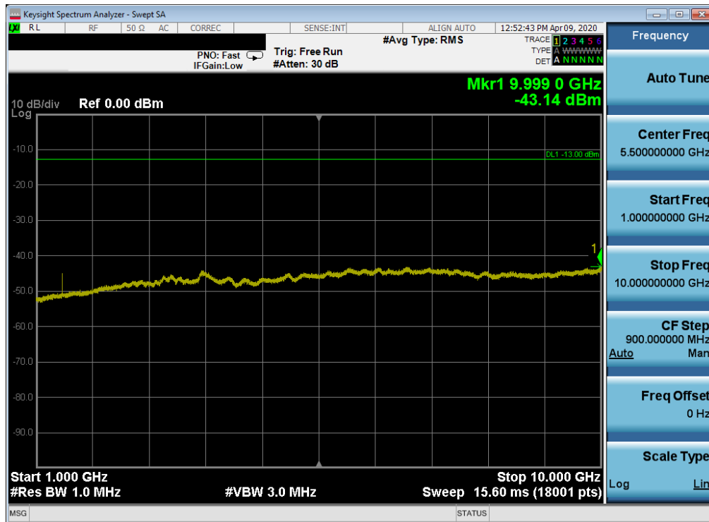
Plot 7-74. Conducted Spurious Plot (LTE Band 12 - 10MHz QPSK - RB Size 1, RB Offset 0 - High Channel)
