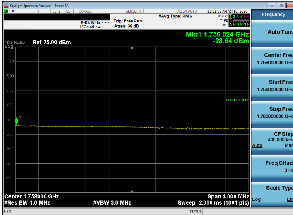
Plot 7-96. Upper Extended Band Edge Plot (LTE Band 4 - 15MHz QPSK – Full RB Configuration)
