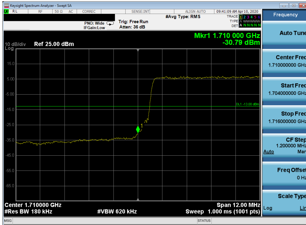
Plot 7-93. Lower Band Edge Plot (LTE Band 66/4 - 15MHz QPSK – Full RB Configuration)
