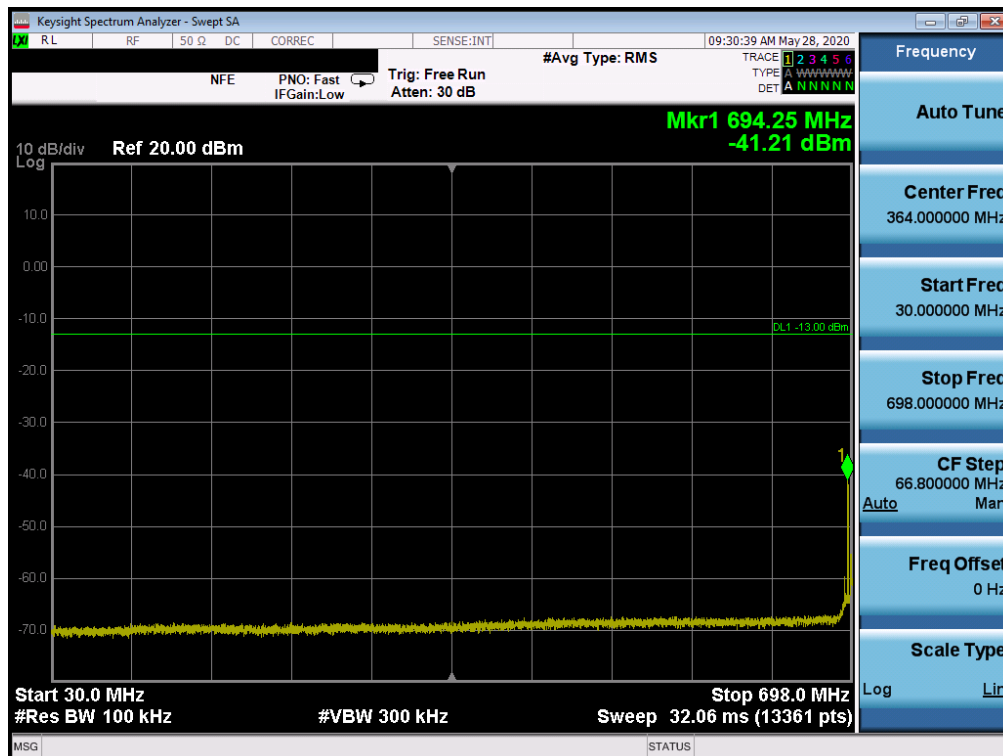
Plot 7-69. Conducted Spurious Plot (LTE Band 12 - 10MHz QPSK - RB Size 1, RB Offset 0 - Mid Channel)
