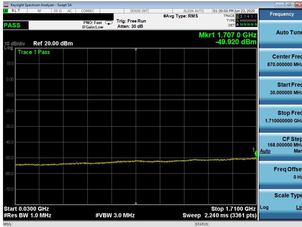
Plot 7-84. Conducted Spurious Plot (NR Band n66 - 20.0MHz - RB Size 1, RB Offset 0 - High Channel)
