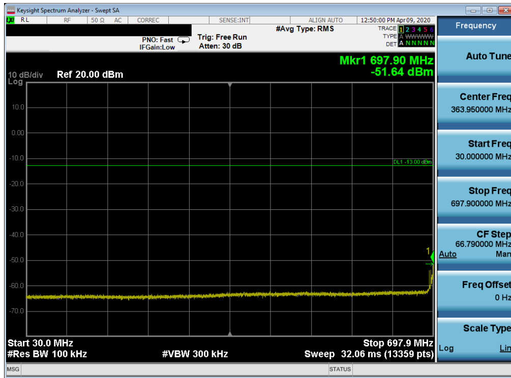
Plot 7-66. Conducted Spurious Plot (LTE Band 12 - 10MHz QPSK - RB Size 1, RB Offset 0 - Low Channel)
