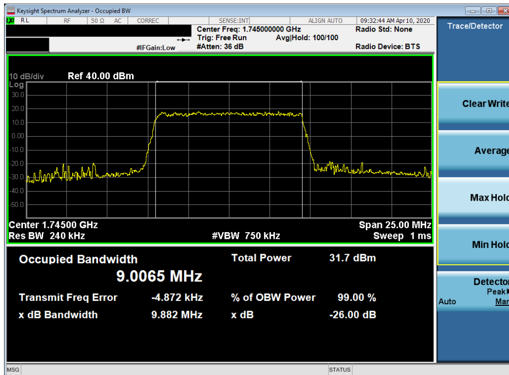
Plot 7-8. Occupied Bandwidth Plot (LTE Band 66/4 - 10MHz 16-QAM - Full RB Configuration)
