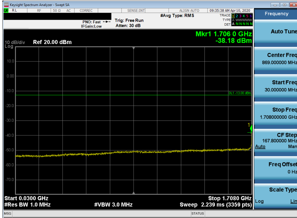
Plot 7-57. Conducted Spurious Plot (LTE Band 66/4 - 20MHz QPSK - RB Size 1, RB Offset 0 - Low Channel)
