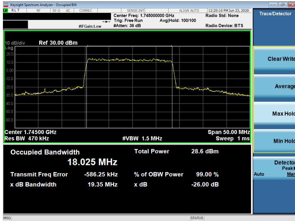
Plot 7-41. Occupied Bandwidth Plot (NR Band n66 - 20.0MHz CP-OFDM 256QAM - Full RB)
