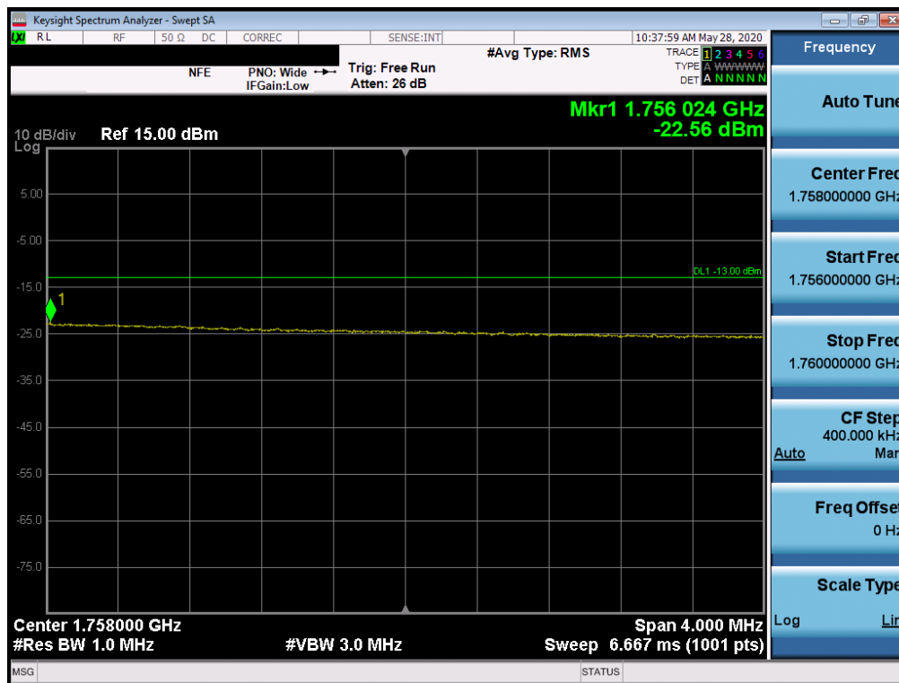
Plot 7-90. Upper Extended Band Edge Plot (LTE Band 4 - 20MHz QPSK - Full RB Configuration)
