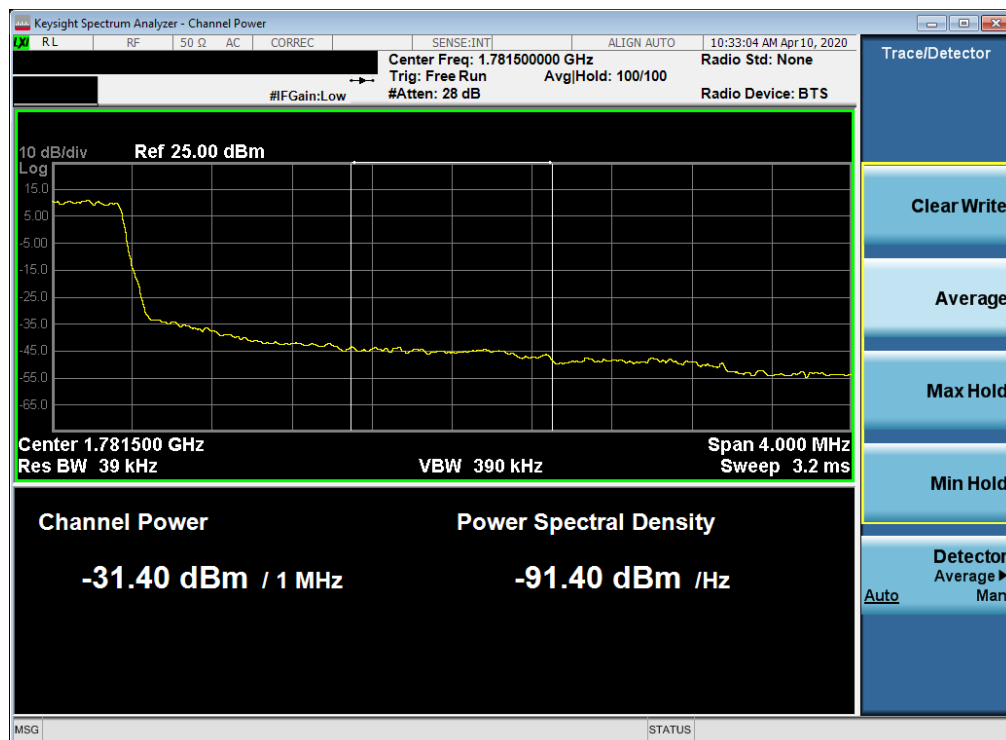
Plot 7-122. Upper Extended Band Edge Plot (LTE Band 66 – 1.4MHz QPSK – Full RB Configuration)
