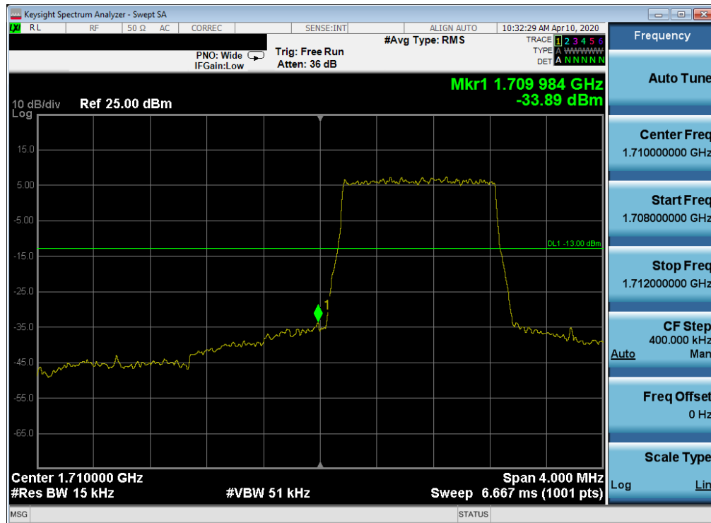
Plot 7-117. Lower Band Edge Plot (LTE Band 66/4 – 1.4MHz QPSK – Full RB Configuration)
