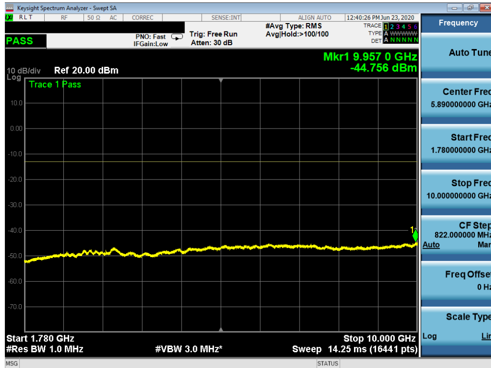
Plot 7-82. Conducted Spurious Plot (NR Band n66 - 20.0MHz - RB Size 1, RB Offset 0 - Mid Channel)
