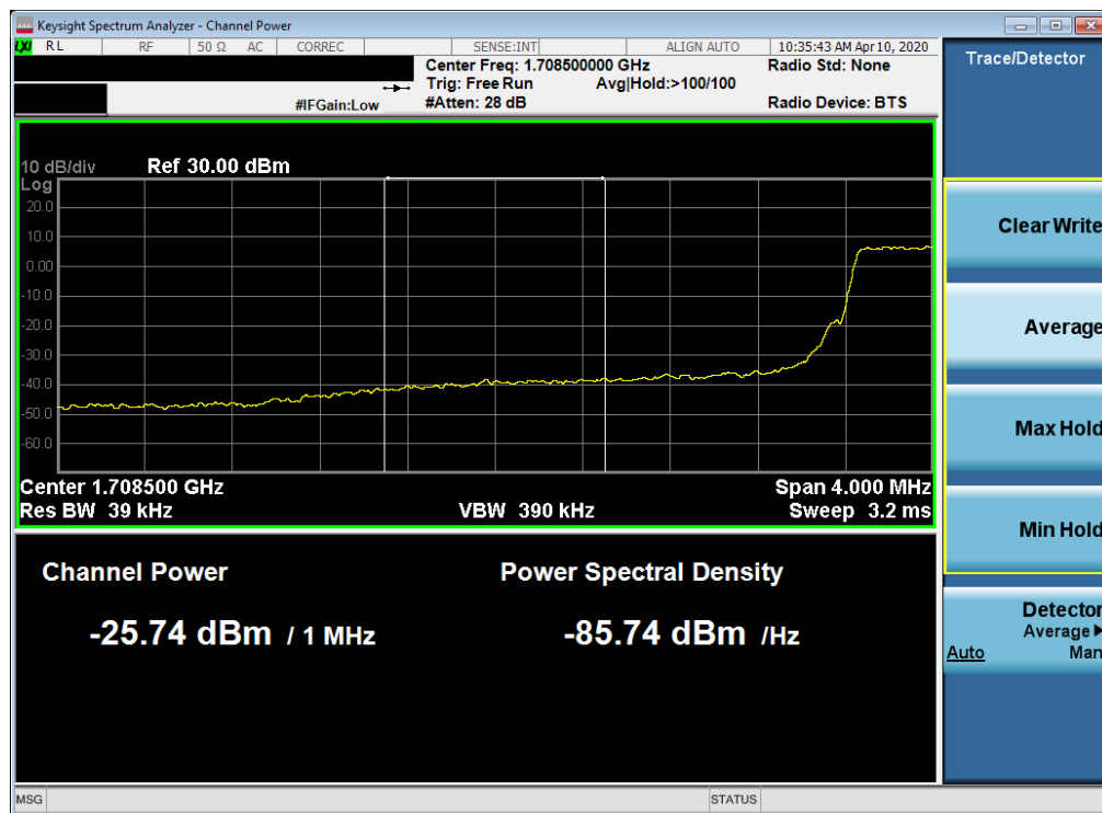
Plot 7-112. Lower Extended Band Edge Plot (LTE Band 66/4 - 3MHz QPSK – Full RB Configuration)
