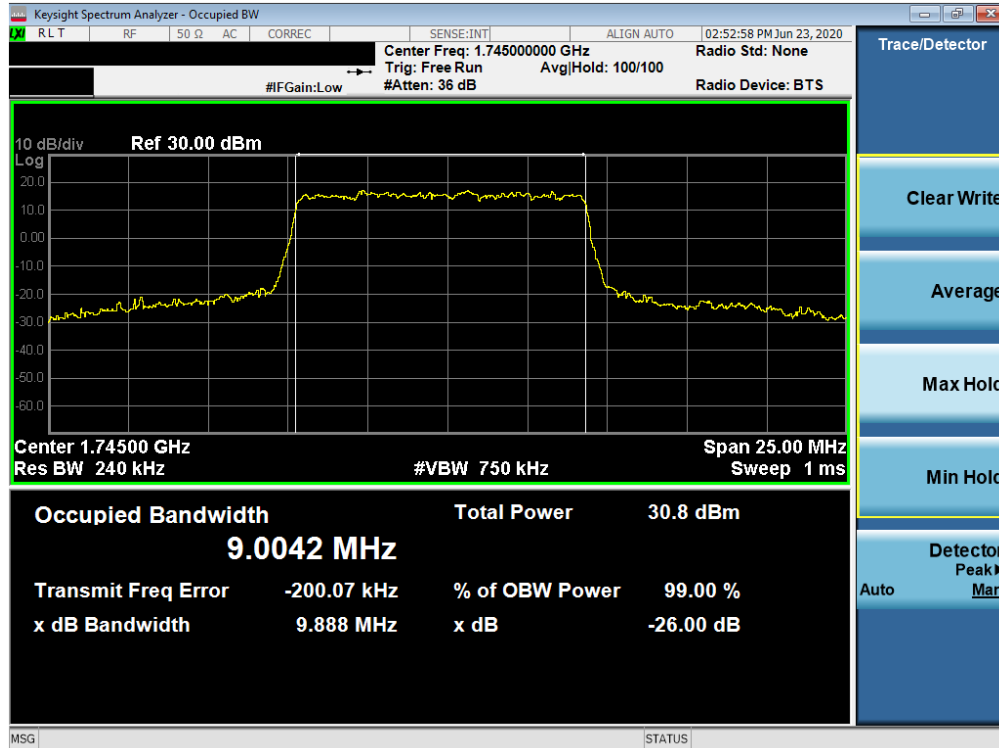
Plot 7-49. Occupied Bandwidth Plot (NR Band n66 - 10.0MHz CP-OFDM 16QAM - Full RB)
