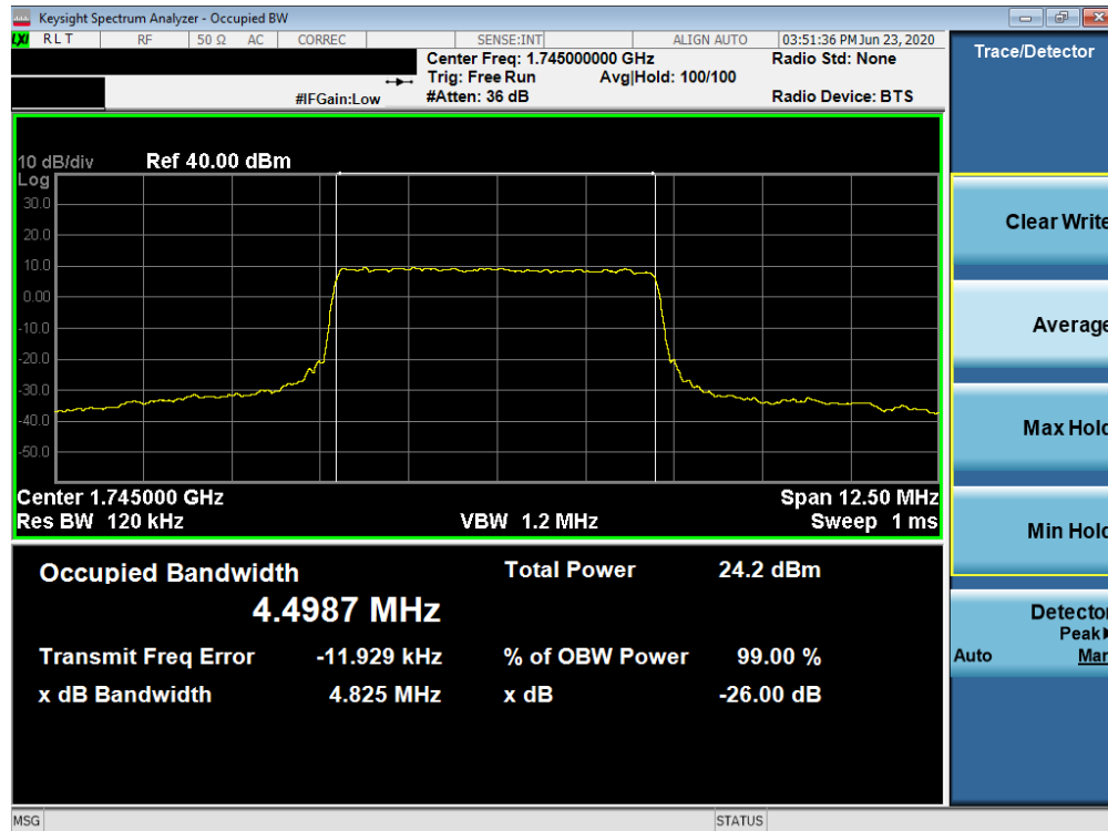
Plot 7-53. Occupied Bandwidth Plot (NR Band n66 - 5.0MHz CP-OFDM QPSK - Full RB)
