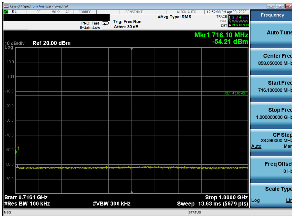
Plot 7-73. Conducted Spurious Plot (LTE Band 12 - 10MHz QPSK - RB Size 1, RB Offset 0 - High Channel)
