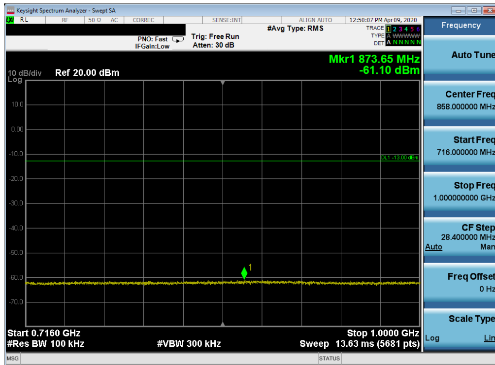
Plot 7-67. Conducted Spurious Plot (LTE Band 12 - 10MHz QPSK - RB Size 1, RB Offset 0 - Low Channel)
