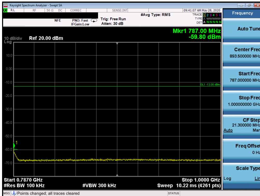
Plot 7-76. Conducted Spurious Plot (LTE Band 13 - 10MHz QPSK - RB Size 1, RB Offset 0)
