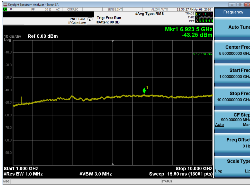
Plot 7-68. Conducted Spurious Plot (LTE Band 12 - 10MHz QPSK - RB Size 1, RB Offset 0 - Low Channel)
