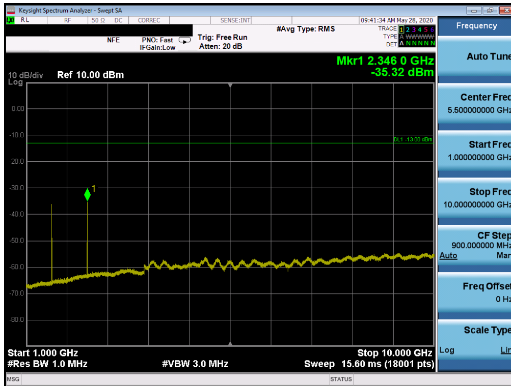
Plot 7-77. Conducted Spurious Plot (LTE Band 13 - 10MHz QPSK - RB Size 1, RB Offset 0)
