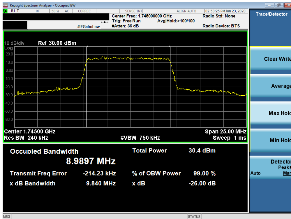
Plot 7-50. Occupied Bandwidth Plot (NR Band n66 - 10.0MHz CP-OFDM 64QAM - Full RB)
