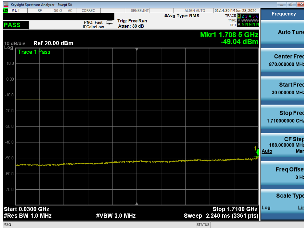
Plot 7-78. Conducted Spurious Plot (NR Band n66 -20.0MHz - RB Size 1, RB Offset 0 - Low Channel)
