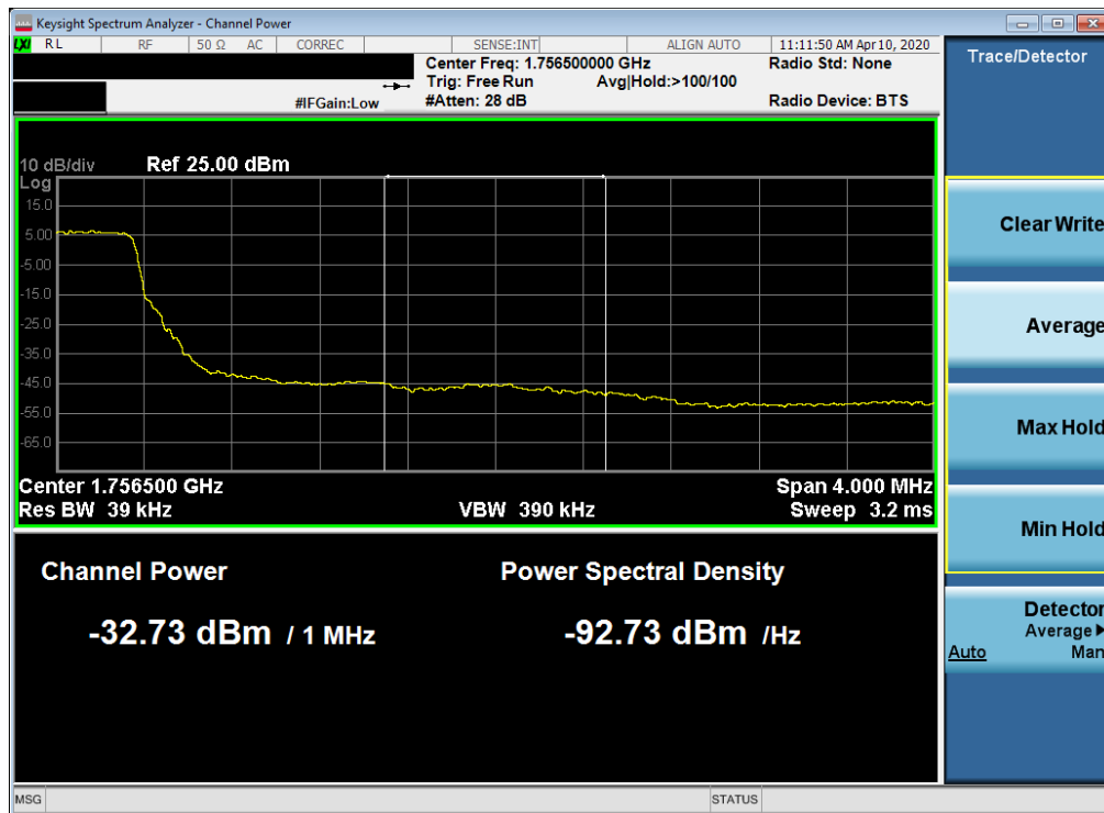
Plot 7-114. Upper Extended Band Edge Plot (LTE Band 4 - 3MHz QPSK – Full RB Configuration)
