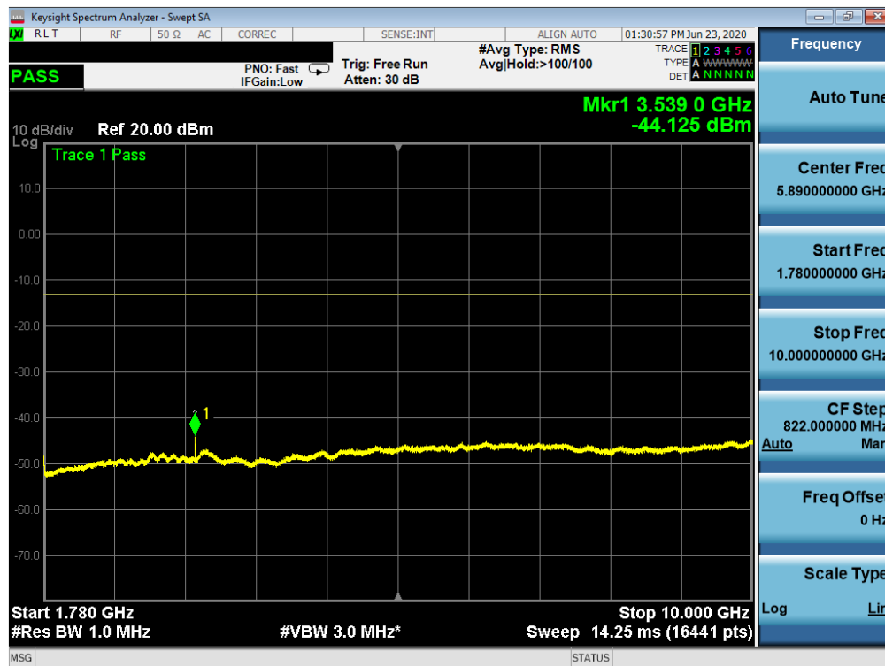
Plot 7-85. Conducted Spurious Plot (NR Band n66 - 20.0MHz - RB Size 1, RB Offset 0 - High Channel)
