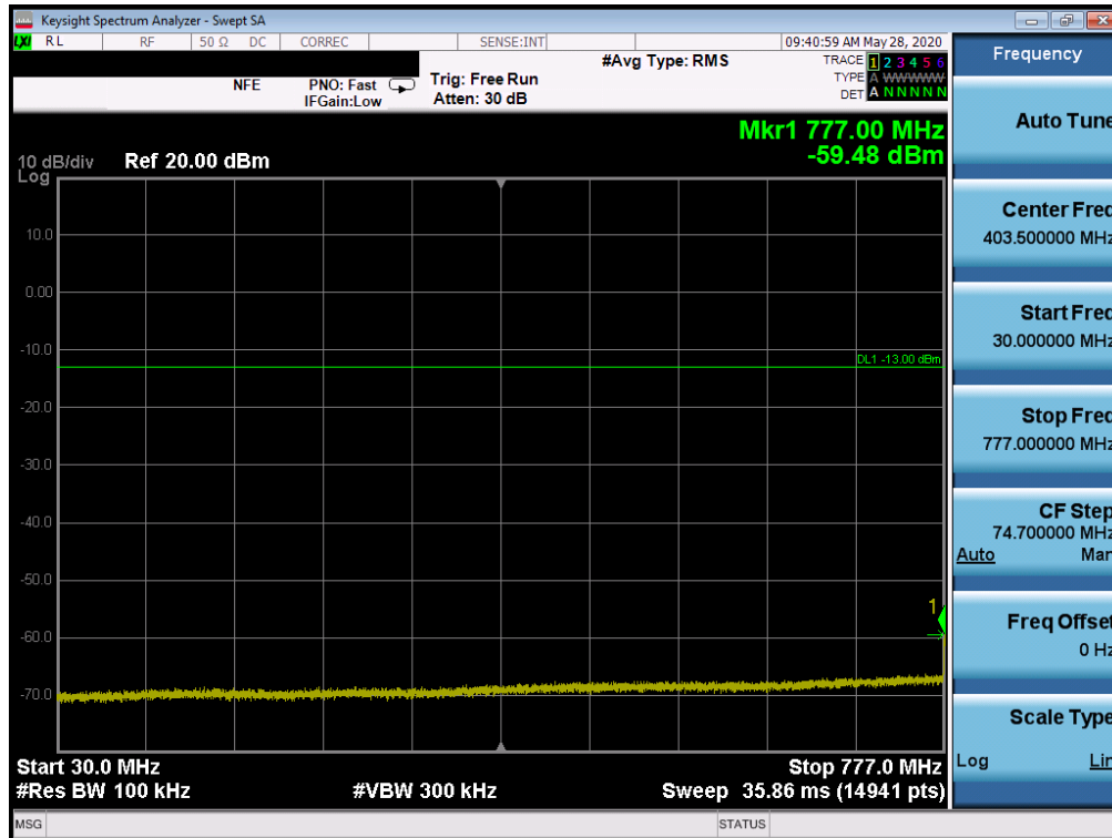
Plot 7-75. Conducted Spurious Plot (LTE Band 13 - 10MHz QPSK - RB Size 1, RB Offset 0)
