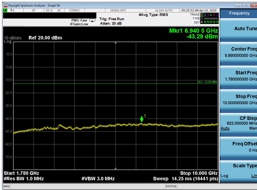
Plot 7-58. Conducted Spurious Plot (LTE Band 66/4 - 20MHz QPSK - RB Size 1, RB Offset 0 - Low Channel)
