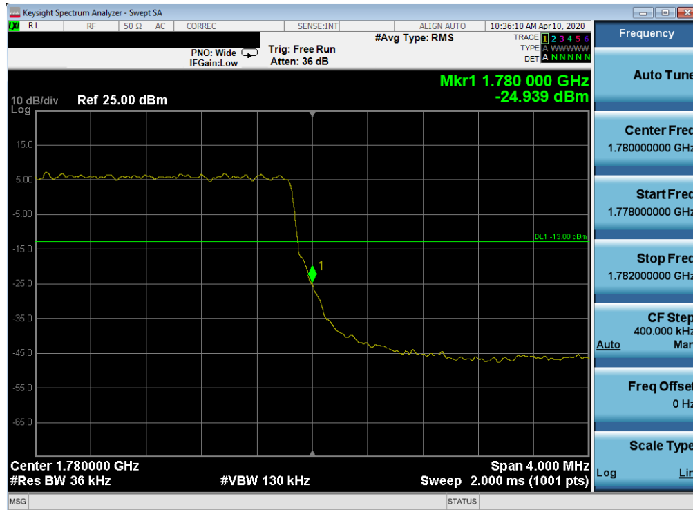
Plot 7-115. Upper Band Edge Plot (LTE Band 66 - 3MHz QPSK – Full RB Configuration)
