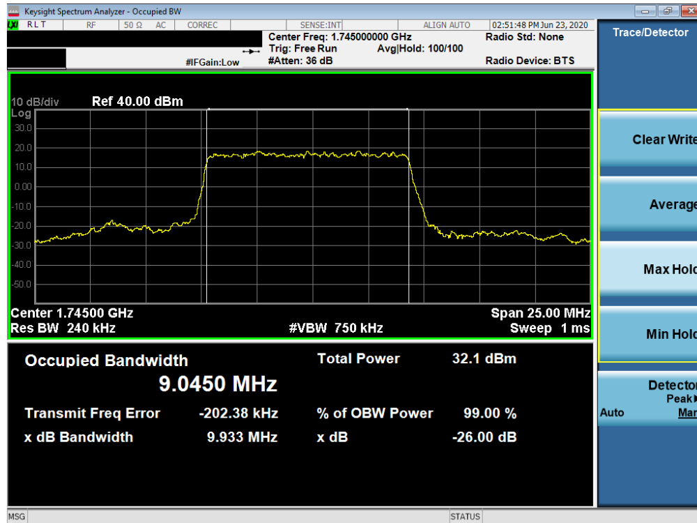
Plot 7-47. Occupied Bandwidth Plot (NR Band n66 - 10.0MHz DFT-s-OFDM BPSK - Full RB)
