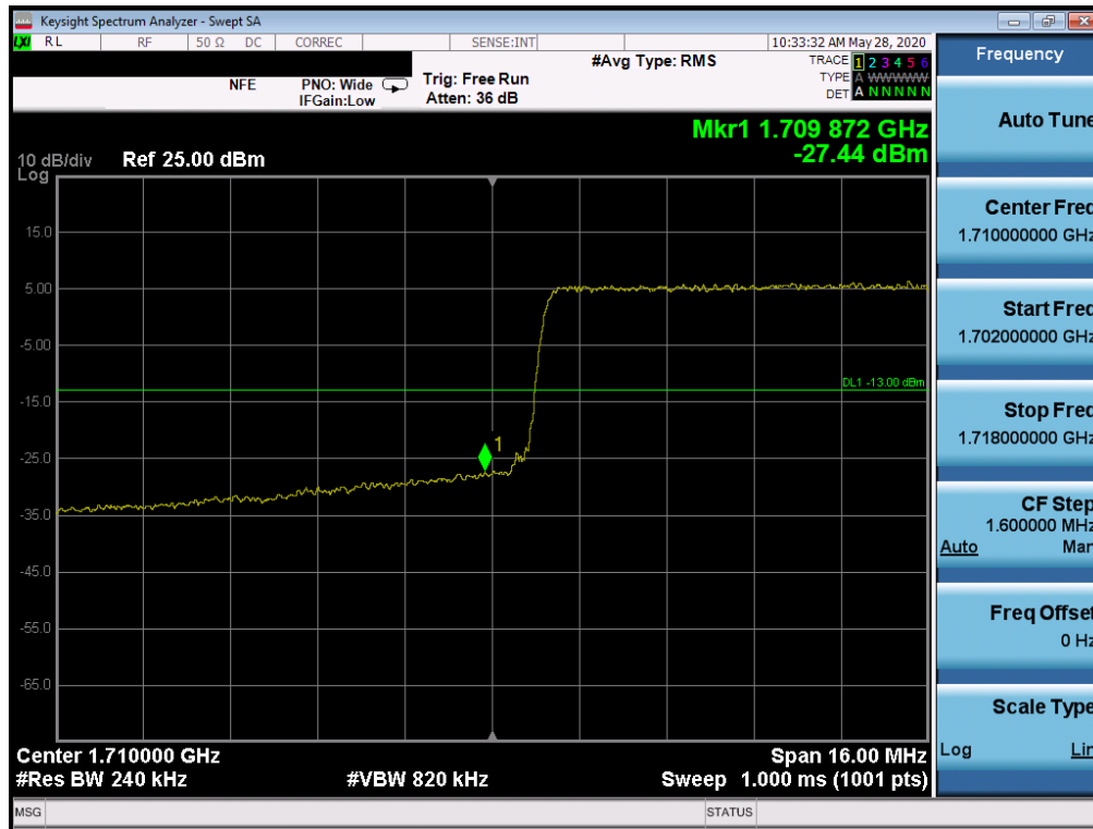
Plot 7-87. Lower Band Edge Plot (LTE Band 66/4 - 20MHz QPSK – Full RB Configuration)
