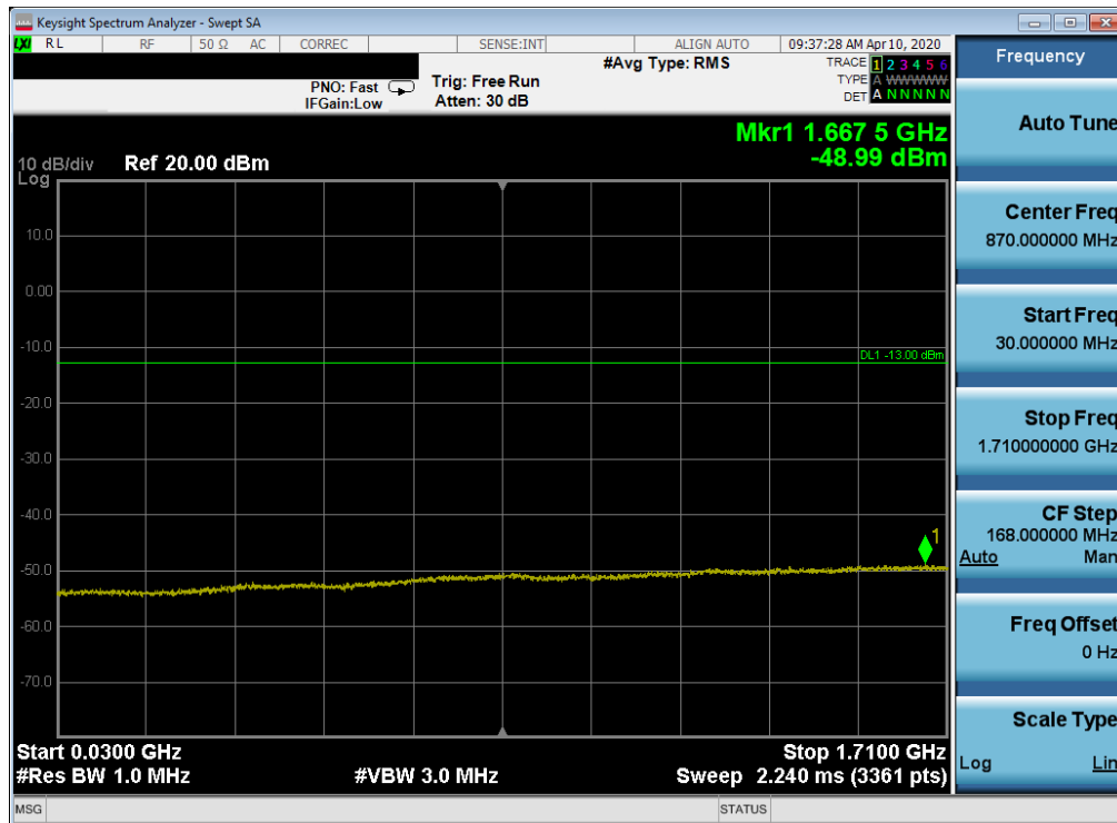
Plot 7-63. Conducted Spurious Plot (LTE Band 66/4 - 20MHz QPSK - RB Size 1, RB Offset 0 - High Channel)
