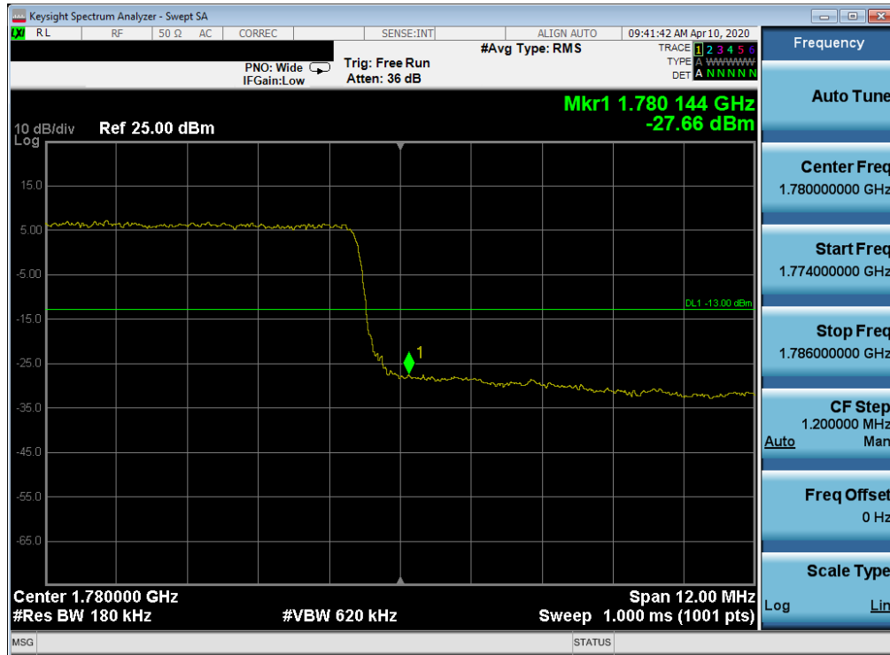
Plot 7-97. Upper Band Edge Plot (LTE Band 66 - 15MHz QPSK – Full RB Configuration)
