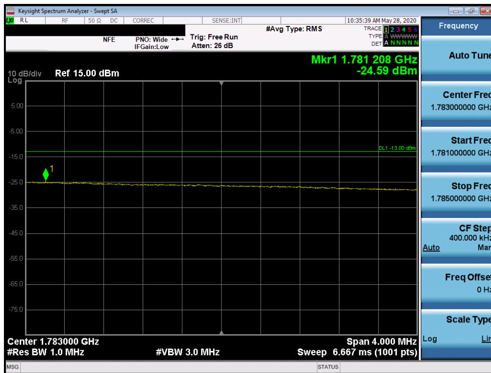
Plot 7-92. Channel Edge Plot (LTE Band 66 - 20MHz QPSK – Full RB Configuration)
