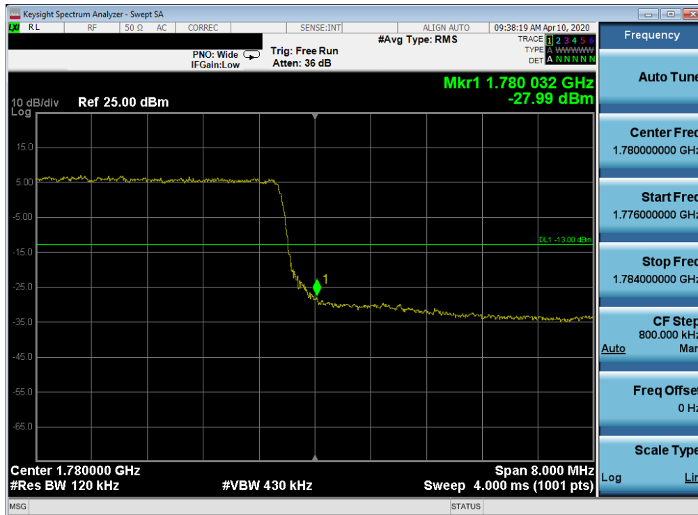
Plot 7-103. Upper Band Edge Plot (LTE Band 66 - 10MHz QPSK – Full RB Configuration)
