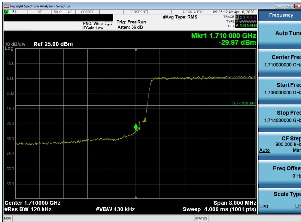
Plot 7-99. Lower Band Edge Plot (LTE Band 66/4 - 10MHz QPSK – Full RB Configuration)
