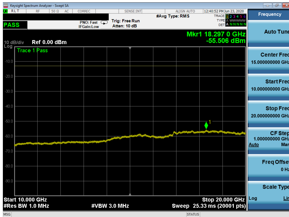
Plot 7-83. Conducted Spurious Plot (NR Band n66 - 20.0MHz - RB Size 1, RB Offset 0 - Mid Channel)
