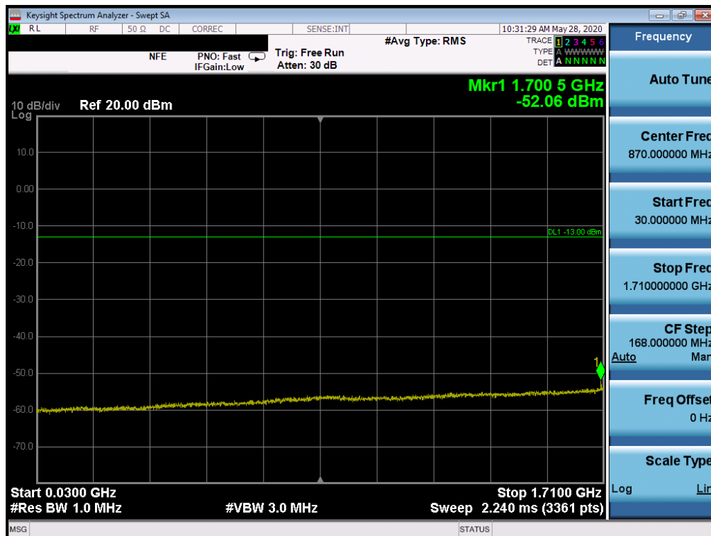
Plot 7-60. Conducted Spurious Plot (LTE Band 66/4 - 20MHz QPSK - RB Size 1, RB Offset 0 - Mid Channel)
