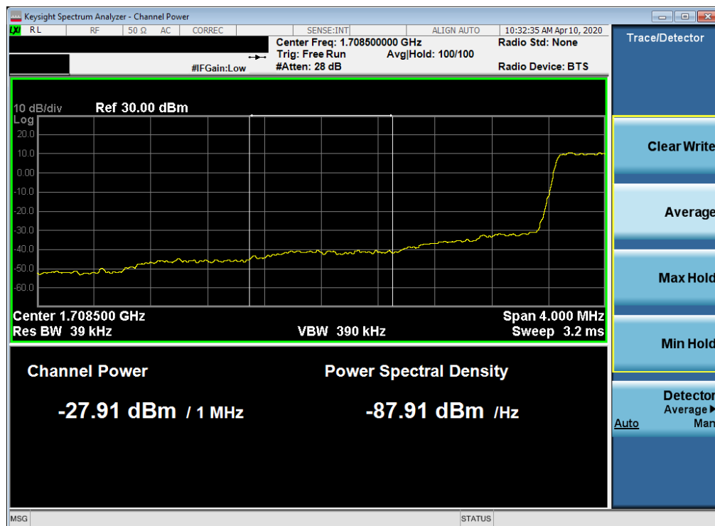
Plot 7-118. Lower Extended Band Edge Plot (LTE Band 66/4 – 1.4MHz QPSK – Full RB Configuration)
