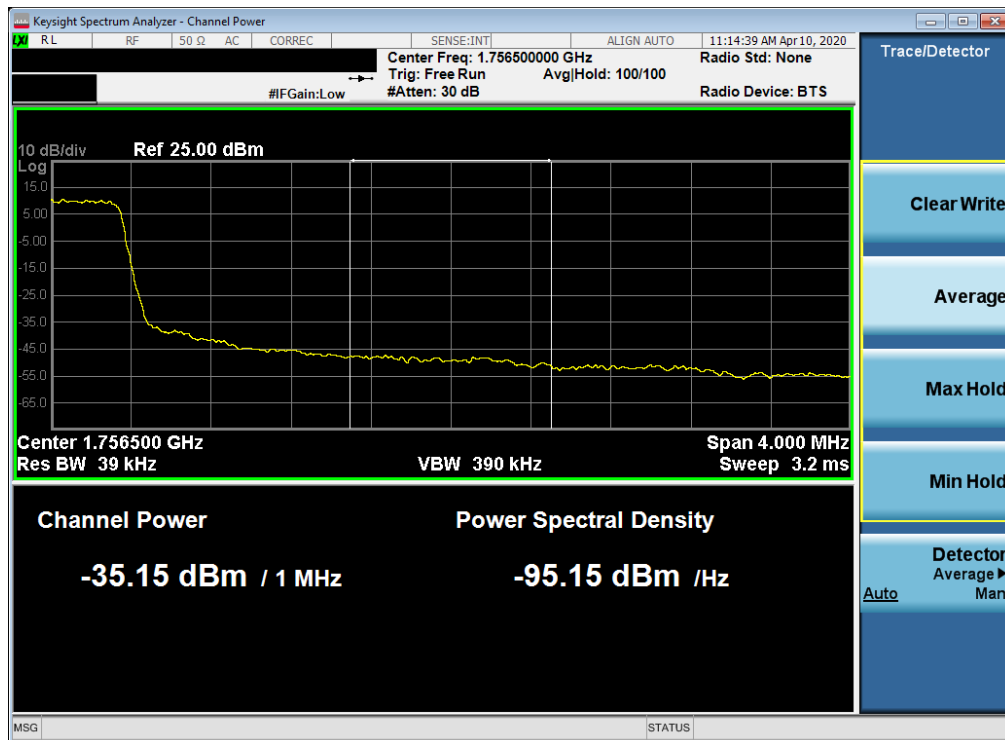
Plot 7-120. Upper Extended Band Edge Plot (LTE Band 4 – 1.4MHz QPSK – Full RB Configuration)
