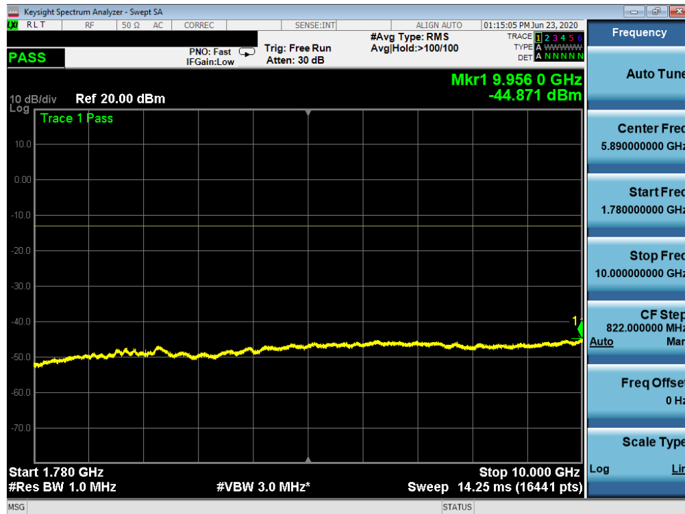
Plot 7-79. Conducted Spurious Plot (NR Band n66 - 20.0MHz - RB Size 1, RB Offset 0 - Low Channel)
