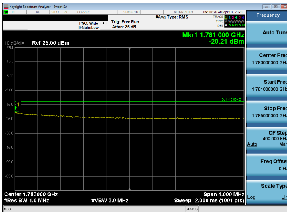
Plot 7-104. Upper Extended Band Edge Plot (LTE Band 66 - 10MHz QPSK – Full RB Configuration)
