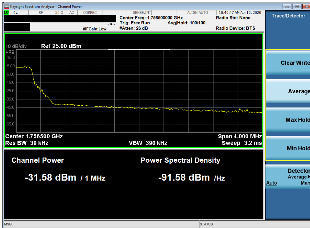
Plot 7-108. Upper Extended Band Edge Plot (LTE Band 4 - 5MHz QPSK – Full RB Configuration)
