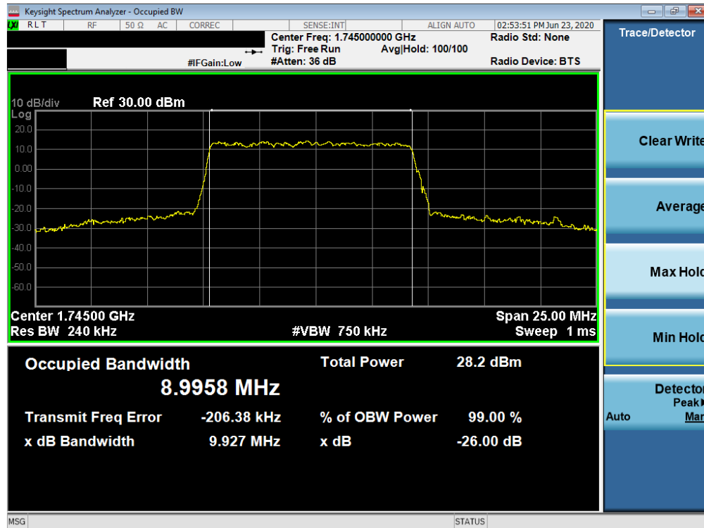
Plot 7-51. Occupied Bandwidth Plot (NR Band n66 - 10.0MHz CP-OFDM 256QAM - Full RB)
