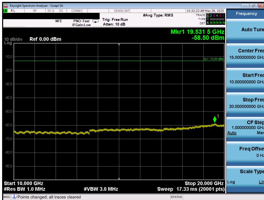
Plot 7-62. Conducted Spurious Plot (LTE Band 66/4 - 20MHz QPSK - RB Size 1, RB Offset 0 - Mid Channel)
