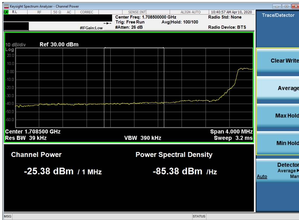
Plot 7-106. Lower Extended Band Edge Plot (LTE Band 66/4 - 5MHz QPSK – Full RB Configuration)
