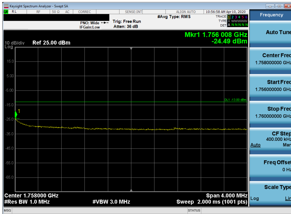
Plot 7-102. Upper Extended Band Edge Plot (LTE Band 4 - 10MHz QPSK – Full RB Configuration)
