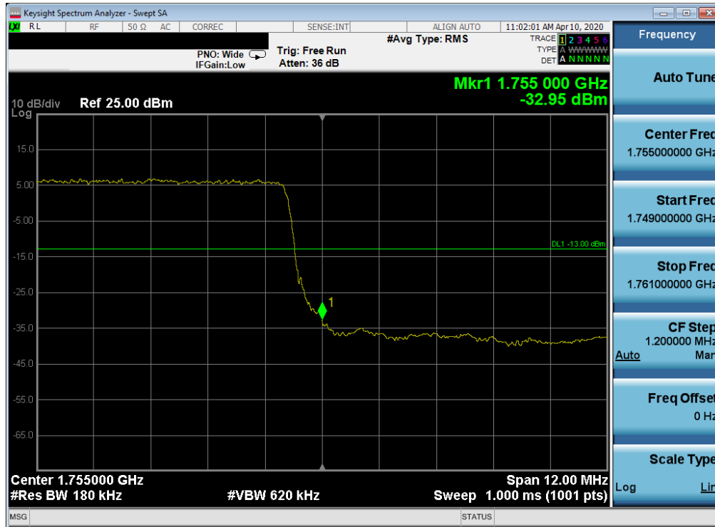
Plot 7-95. Upper Band Edge Plot (LTE Band 4 - 15MHz QPSK – Full RB Configuration)
