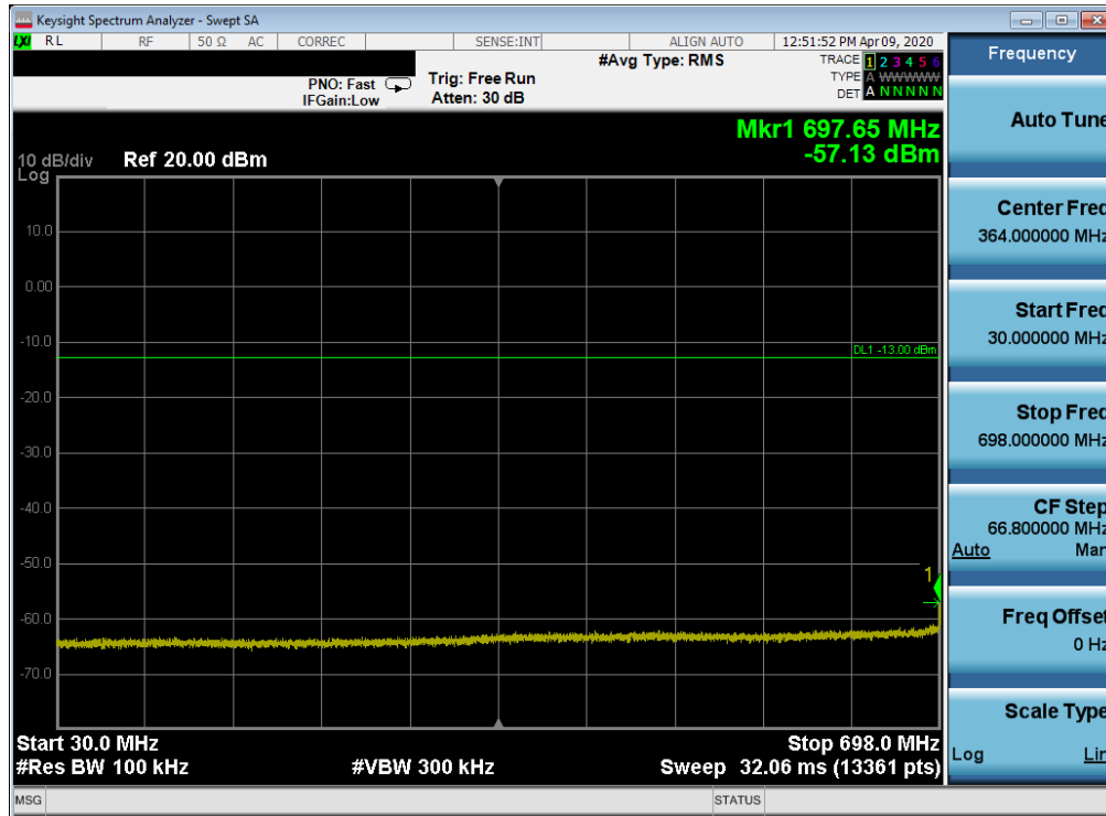
Plot 7-72. Conducted Spurious Plot (LTE Band 12 - 10MHz QPSK - RB Size 1, RB Offset 0 - High Channel)
