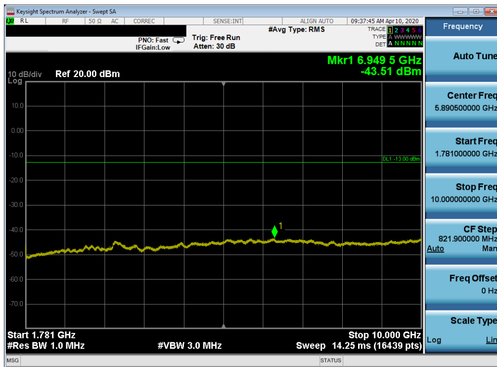
Plot 7-64. Conducted Spurious Plot (LTE Band 66/4 - 20MHz QPSK - RB Size 1, RB Offset 0 - High Channel)
