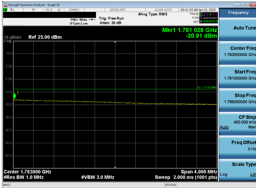
Plot 7-98. Upper Extended Band Edge Plot (LTE Band 66 - 15MHz QPSK – Full RB Configuration)
