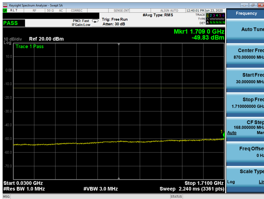
Plot 7-81. Conducted Spurious Plot (NR Band n66 - 20.0MHz - RB Size 1, RB Offset 0 - Mid Channel)
