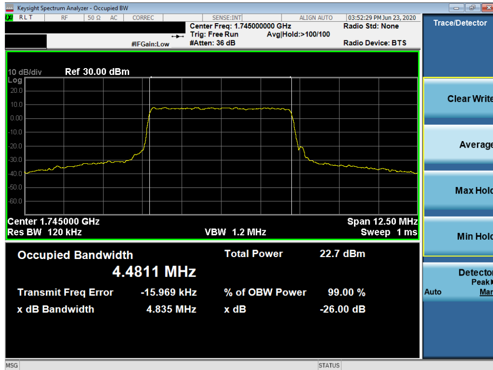
Plot 7-55. Occupied Bandwidth Plot (NR Band n66 - 5.0MHz CP-OFDM 64QAM - Full RB)
