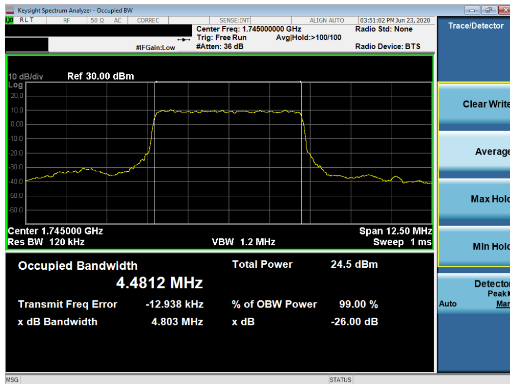
Plot 7-52. Occupied Bandwidth Plot (NR Band n66 - 5.0MHz DFT-s-OFDM BPSK - Full RB)
