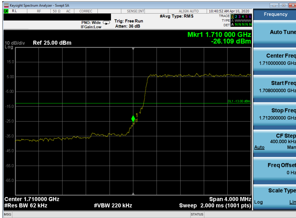
Plot 7-105. Lower Band Edge Plot (LTE Band 66/4 - 5MHz QPSK – Full RB Configuration)
