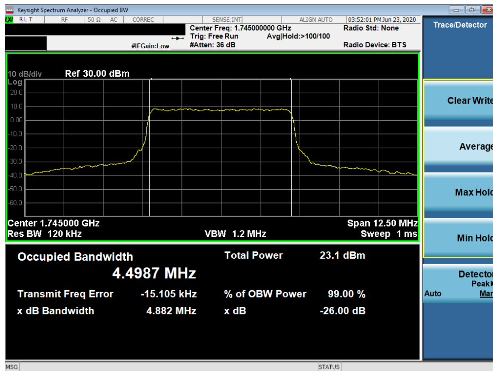
Plot 7-54. Occupied Bandwidth Plot (NR Band n66 - 5.0MHz CP-OFDM 16QAM - Full RB)
