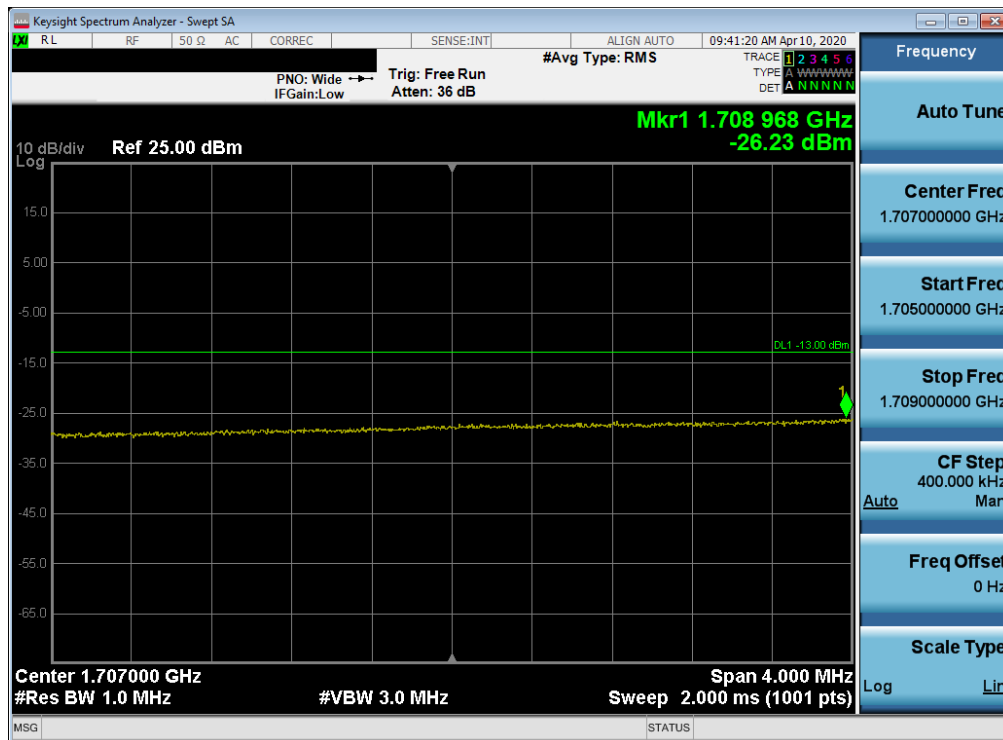
Plot 7-94. Lower Extended Band Edge Plot (LTE Band 66/4 - 15MHz QPSK – Full RB Configuration)
