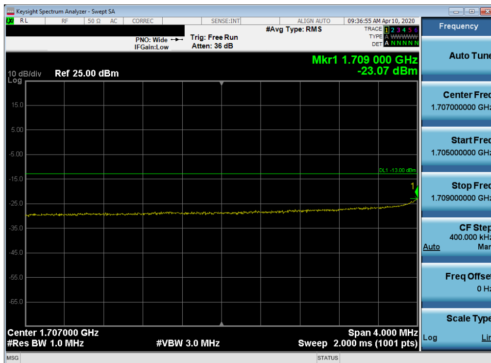
Plot 7-100. Lower Extended Band Edge Plot (LTE Band 66/4 - 10MHz QPSK – Full RB Configuration)
