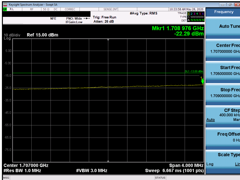
Plot 7-88. Lower Extended Band Edge Plot (LTE Band 66/4 - 20MHz QPSK – Full RB Configuration)
