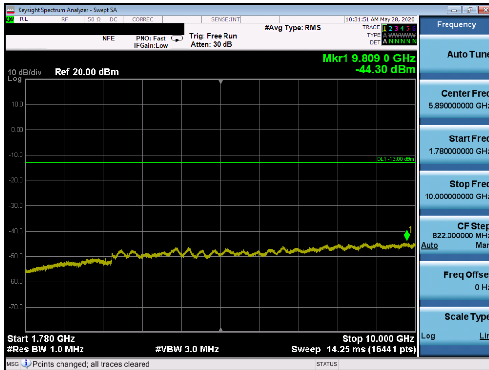
Plot 7-61. Conducted Spurious Plot (LTE Band 66/4 - 20MHz QPSK - RB Size 1, RB Offset 0 - Mid Channel)
