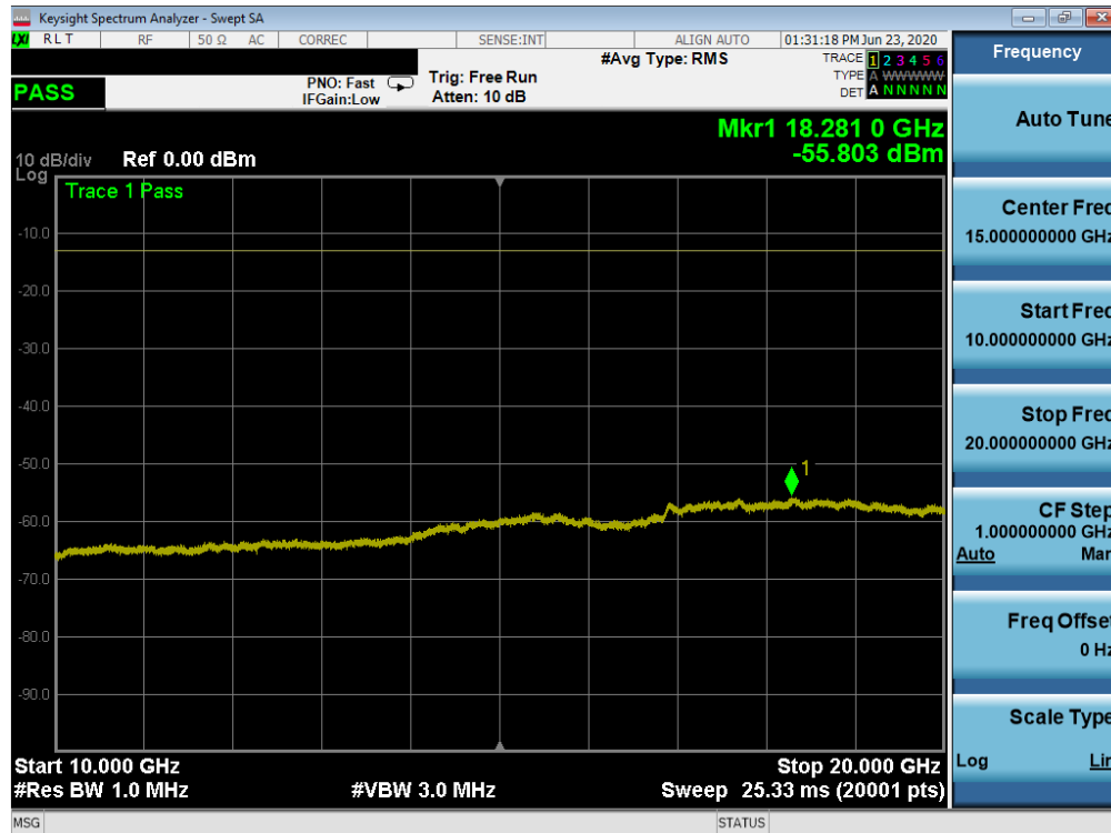
Plot 7-86. Conducted Spurious Plot (NR Band n66 - 20.0MHz - RB Size 1, RB Offset 0 - High Channel)
