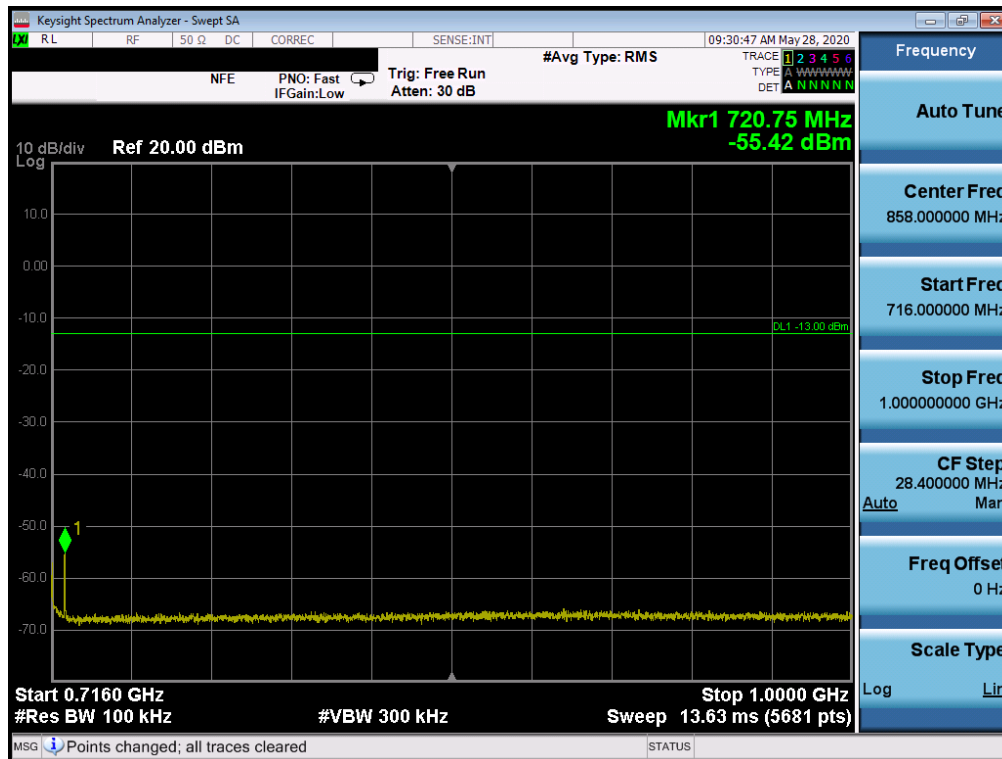
Plot 7-70. Conducted Spurious Plot (LTE Band 12 - 10MHz QPSK - RB Size 1, RB Offset 0 - Mid Channel)
