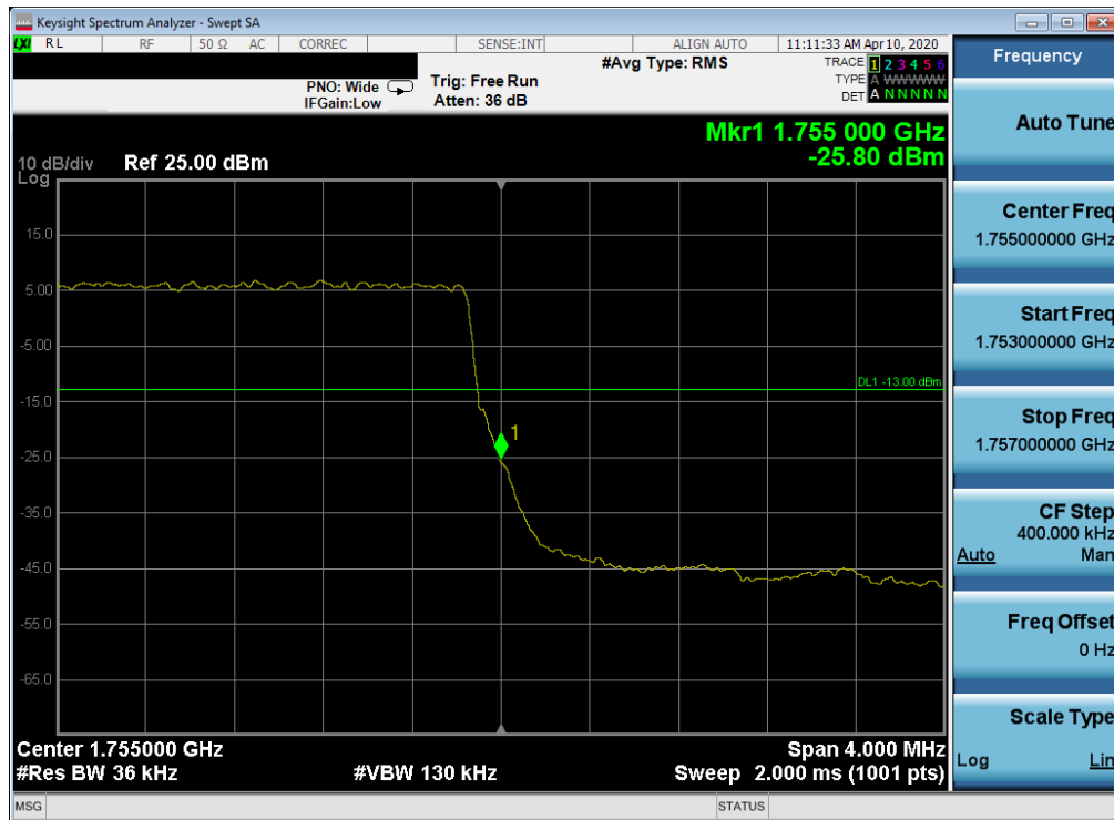
Plot 7-113. Upper Band Edge Plot (LTE Band 4 - 3MHz QPSK – Full RB Configuration)
