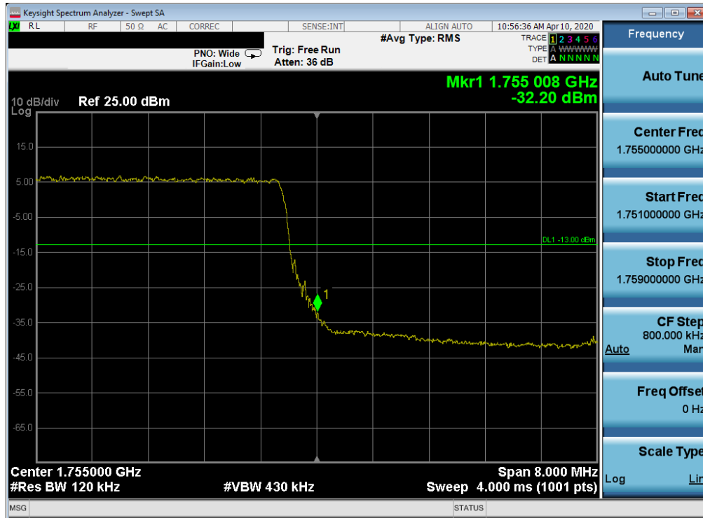
Plot 7-101. Upper Band Edge Plot (LTE Band 4 - 10MHz QPSK – Full RB Configuration)
