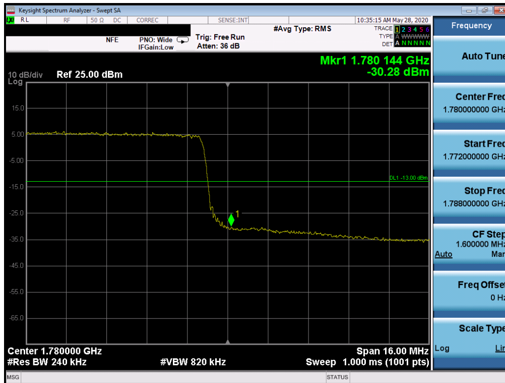
Plot 7-91. Upper Band Edge Plot (LTE Band 66 - 20MHz QPSK – Full RB Configuration)
