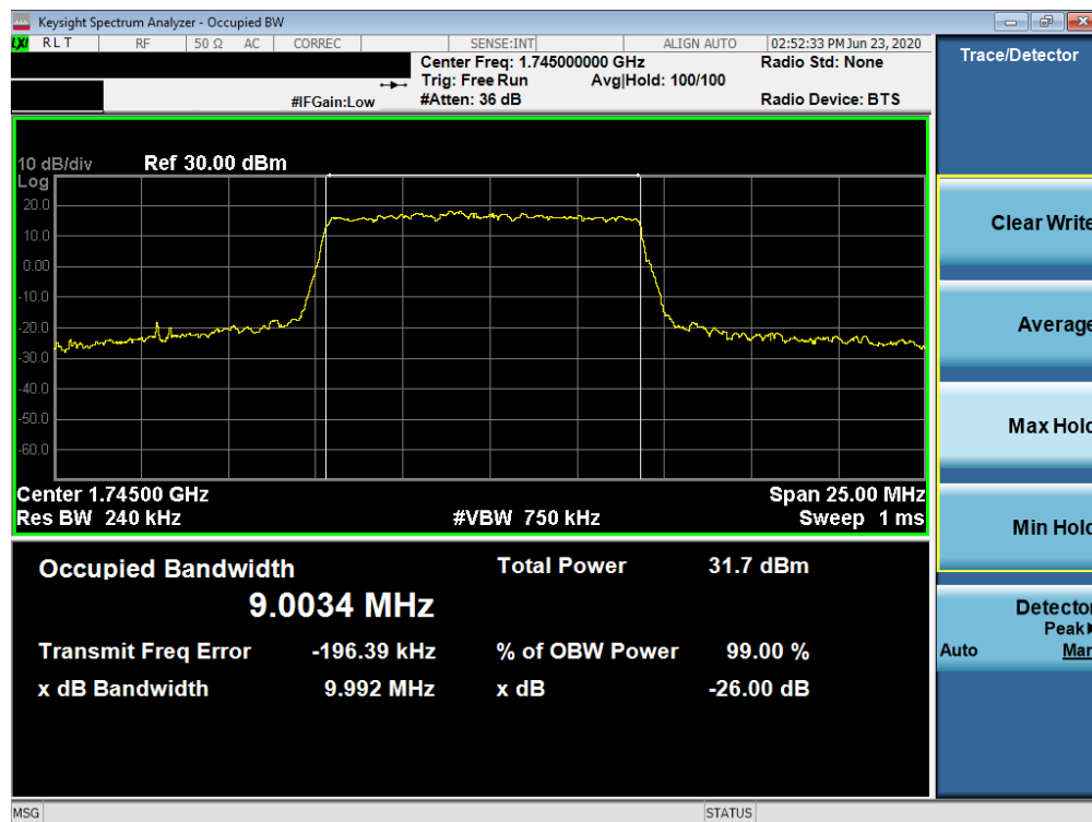
Plot 7-48. Occupied Bandwidth Plot (NR Band n66 - 10.0MHz CP-OFDM QPSK - Full RB)
