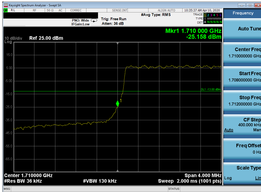
Plot 7-111. Lower Band Edge Plot (LTE Band 66/4 - 3MHz QPSK – Full RB Configuration)
