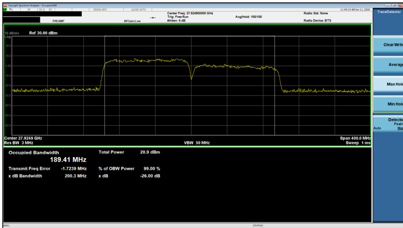
Plot 7-15. Ant 2 Occupied Bandwidth Plot (100MHz-2CC – 64QAM – Mid Channel)
