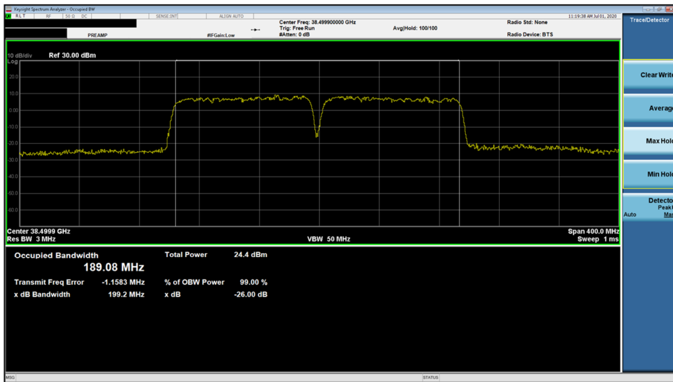
Plot 7-32. Ant 2 Occupied Bandwidth Plot (100MHz-2CC – pi/2-BPSK – Mid Channel)
