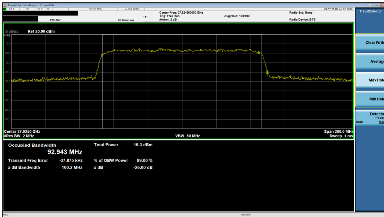
Plot 7-11. Ant 2 Occupied Bandwidth Plot (100MHz-1CC – 64QAM – Mid Channel)
