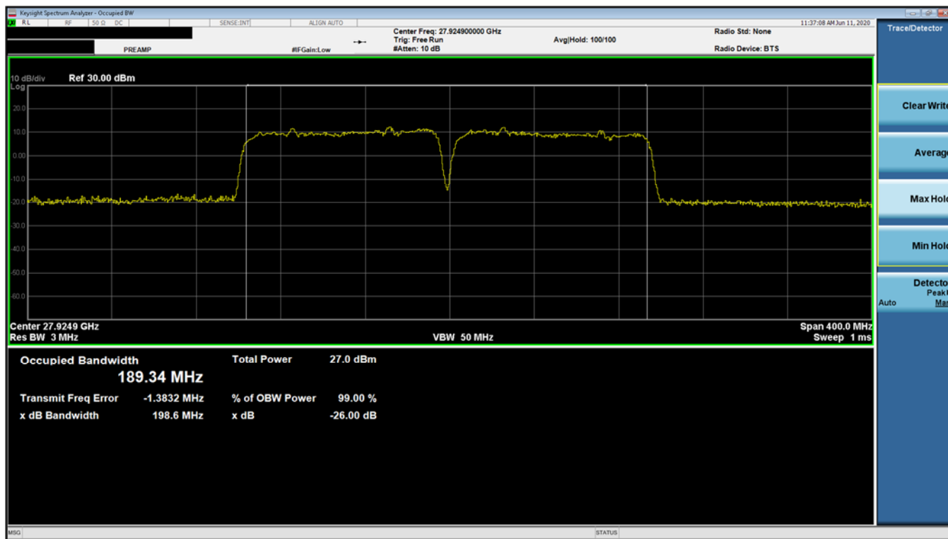
Plot 7-16. Ant 2 Occupied Bandwidth Plot (100MHz-2CC – pi/2-BPSK – Mid Channel)
