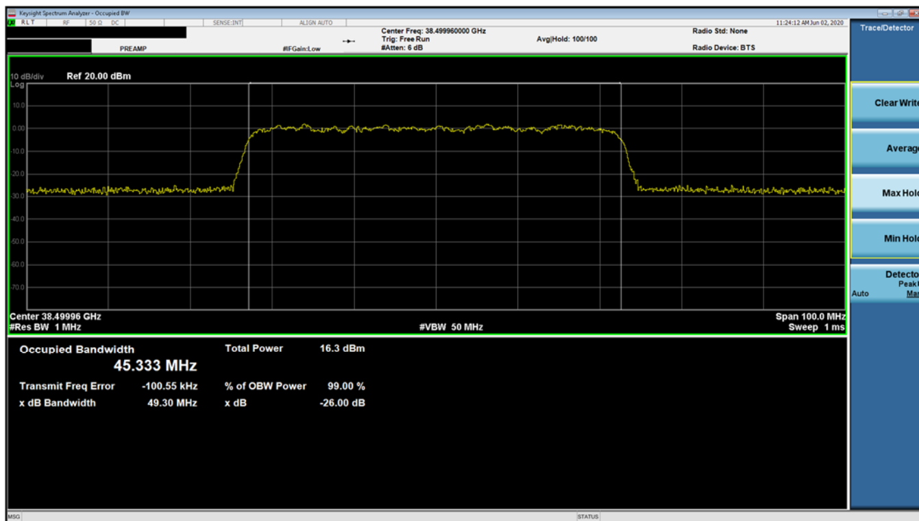
Plot 7-19. Ant 2 Occupied Bandwidth Plot (50MHz-1CC – 64QAM – Mid Channel)
