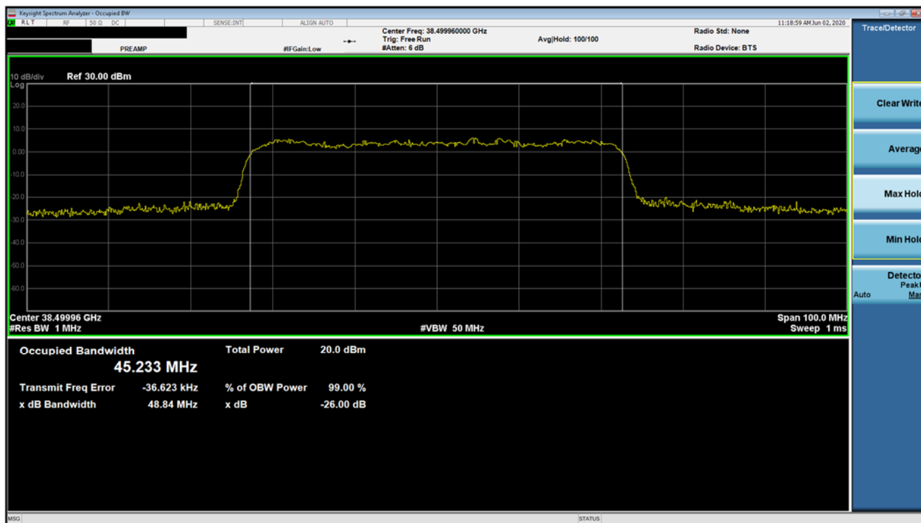
Plot 7-17. Ant 2 Occupied Bandwidth Plot (50MHz-1CC – QPSK – Mid Channel)
