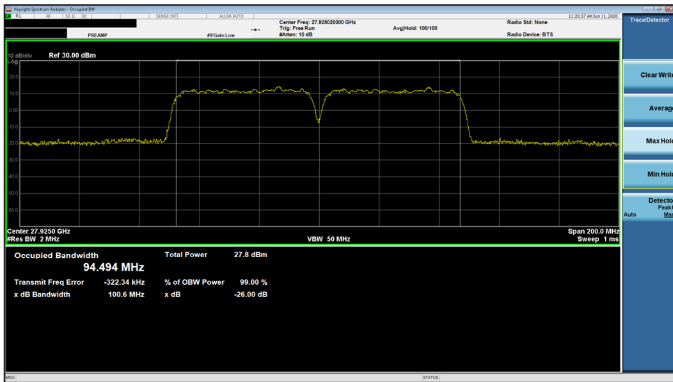
Plot 7-8. Ant 2 Occupied Bandwidth Plot (50MHz-2CC – pi/2-BPSK – Mid Channel)
