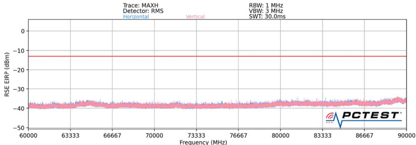
Plot 7-35. Ant 2-n260 Radiated Spurious Plot (1CC QPSK Mid Channel V Beam – ENDC Anchor Band 2)
