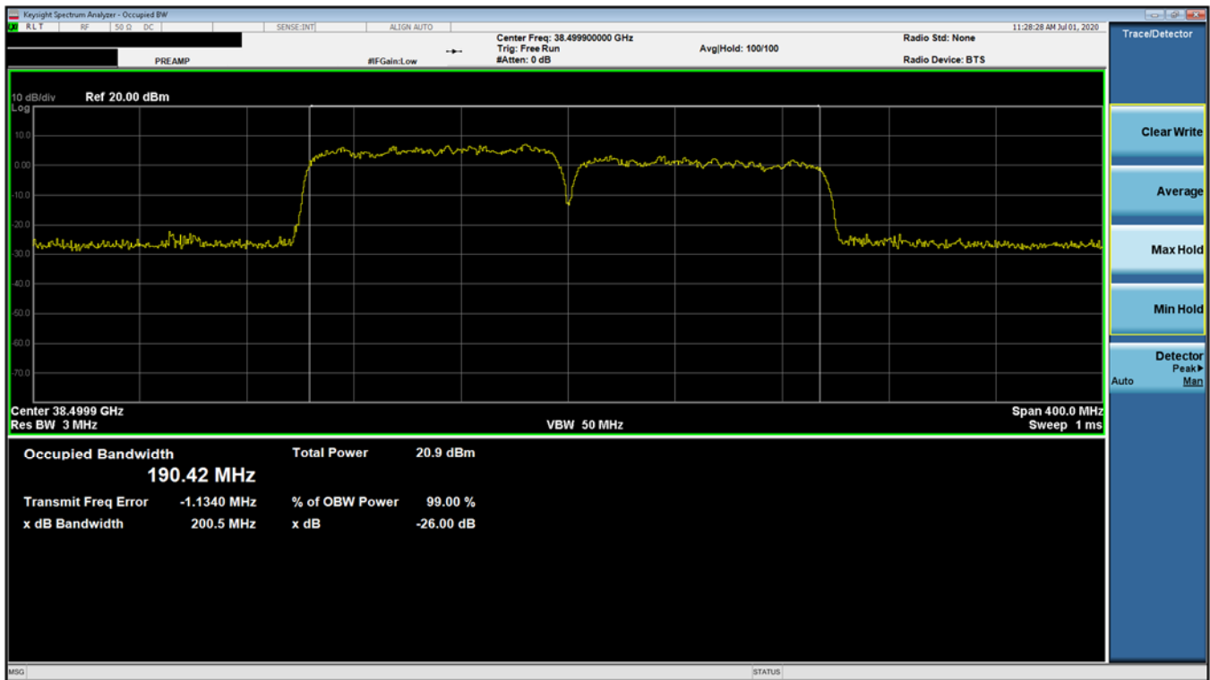
Plot 7-30. Ant 2 Occupied Bandwidth Plot (100MHz-2CC – 16QAM – Mid Channel)
