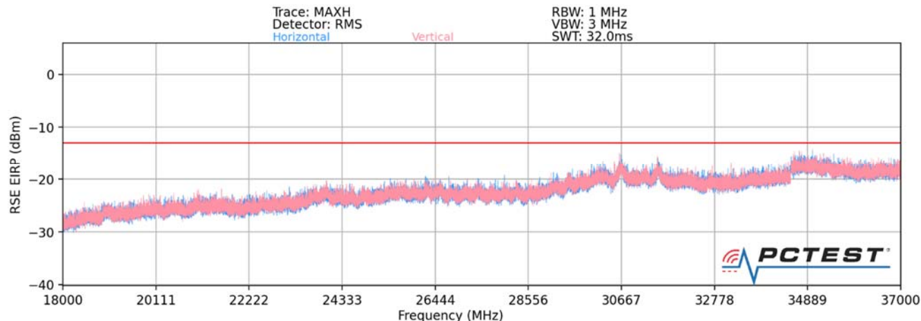
Plot 7-49. Ant 3-n260 Radiated Spurious Plot (1CC QPSK Mid Channel MIMO – ENDC Anchor Band 2)
