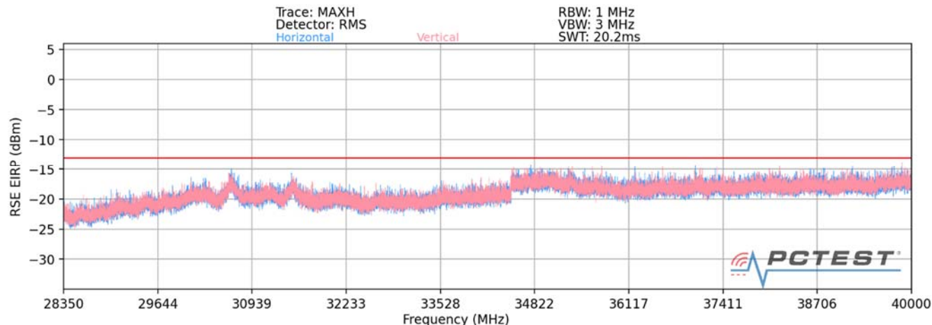
Plot 7-36. Ant 3-n261 Radiated Spurious Plot (1CC QPSK Mid Channel V Beam – ENDC Anchor B2)
