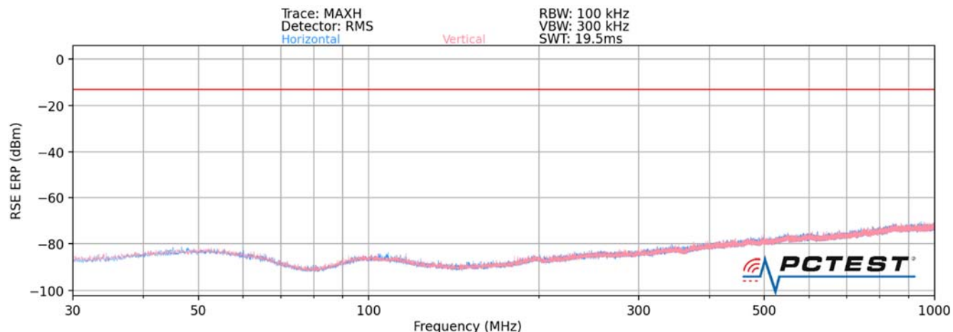
Plot 7-47. Ant 3-n260 Radiated Spurious Plot (1CC QPSK Mid Channel MIMO – ENDC Anchor Band 2)
