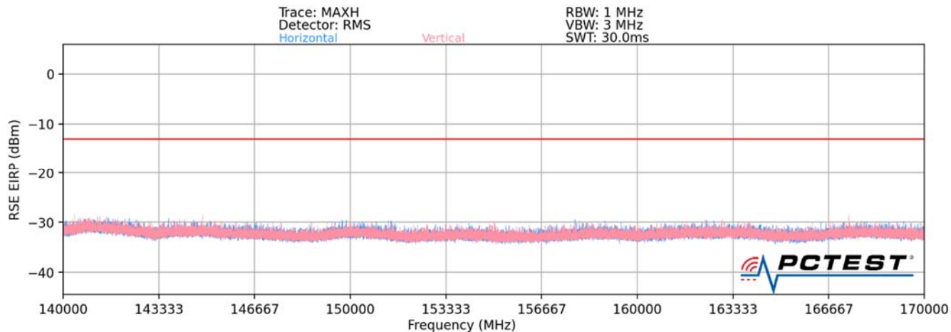
Plot 7-53. Ant 3-n260 Radiated Spurious Plot (1CC QPSK Mid Channel MIMO – ENDC Anchor Band 2)
