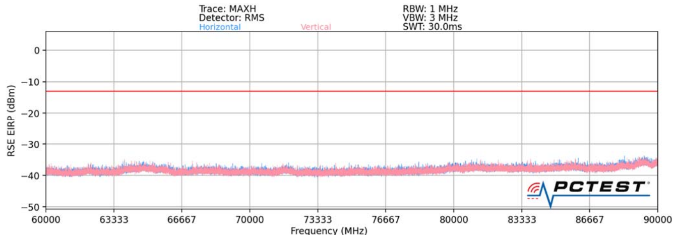
Plot 7-51. Ant 3-n260 Radiated Spurious Plot (1CC QPSK Mid Channel MIMO – ENDC Anchor Band 2)
