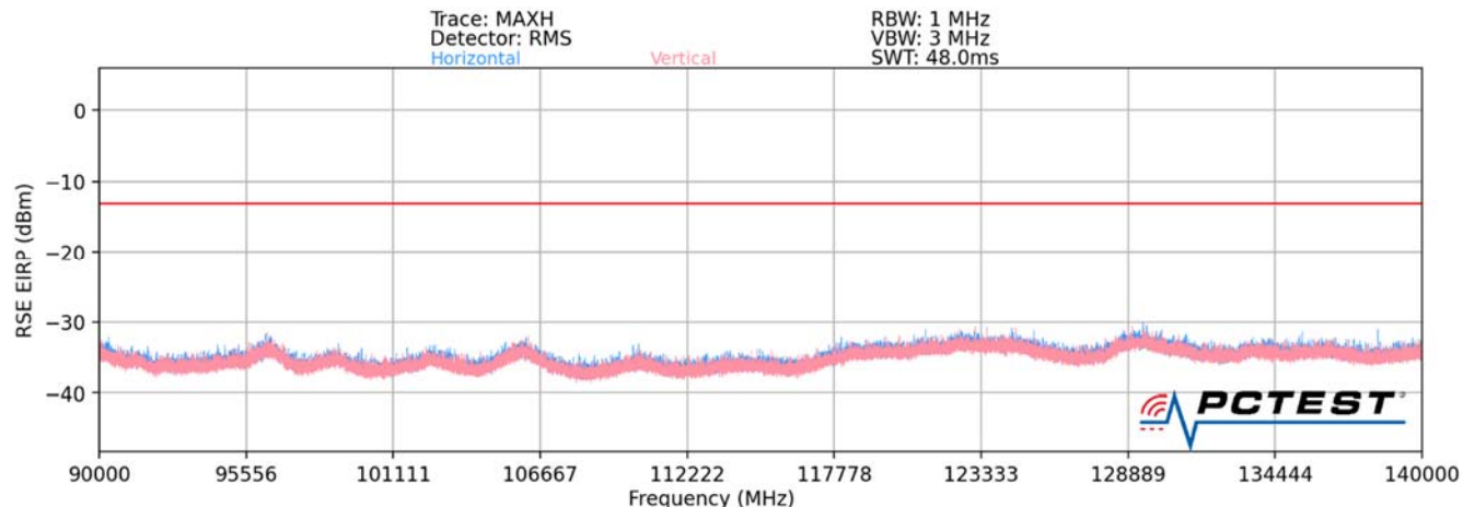
Plot 7-52. Ant 3-n260 Radiated Spurious Plot (1CC QPSK Mid Channel MIMO – ENDC Anchor Band 2)
