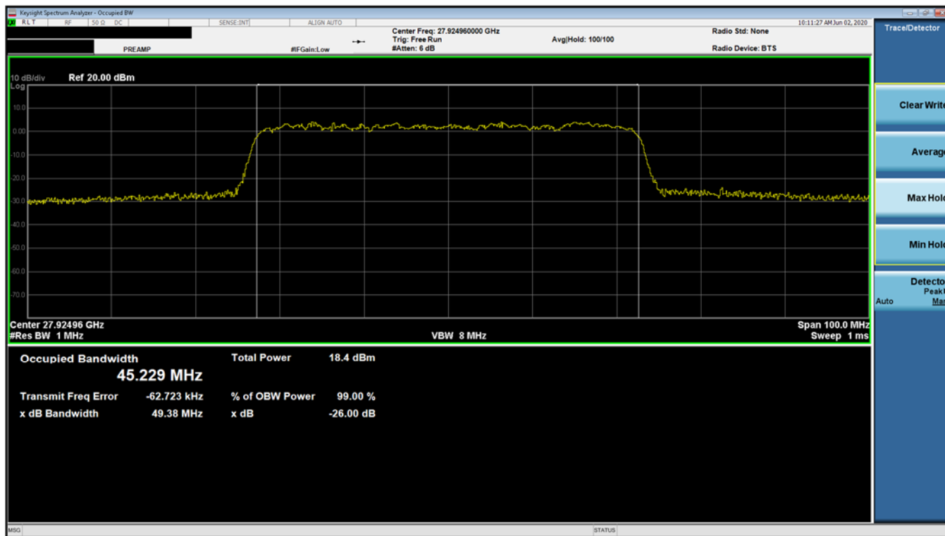
Plot 7-3. Ant 2 Occupied Bandwidth Plot (50MHz-1CC – 64QAM – Mid Channel)
