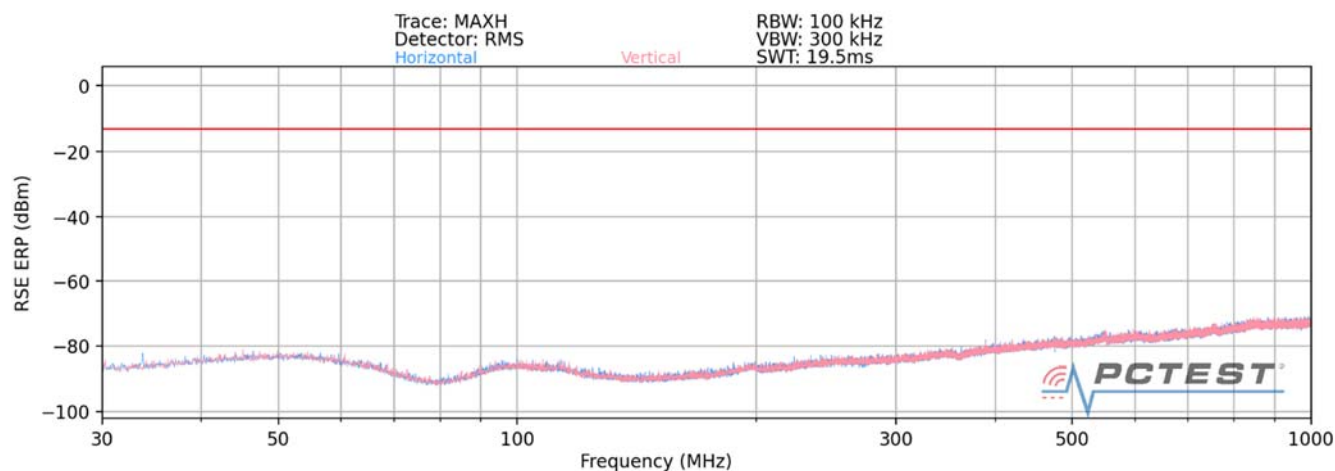
Plot 7-34. Ant 3- n261 Radiated Spurious Plot (1CC QPSK Mid Channel V Beam – ENDC Anchor Band 2)
