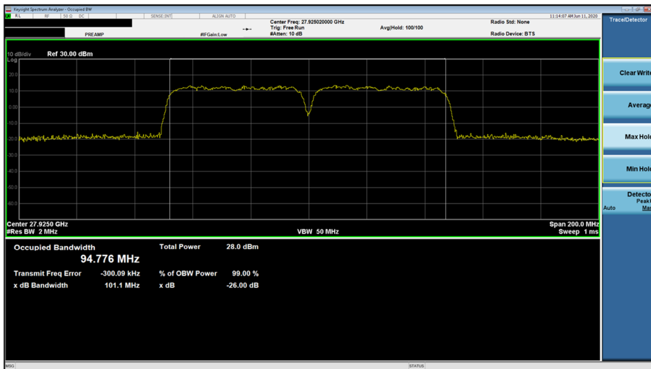
Plot 7-5. Ant 2 Occupied Bandwidth Plot (50MHz-2CC – QPSK – Mid Channel)
