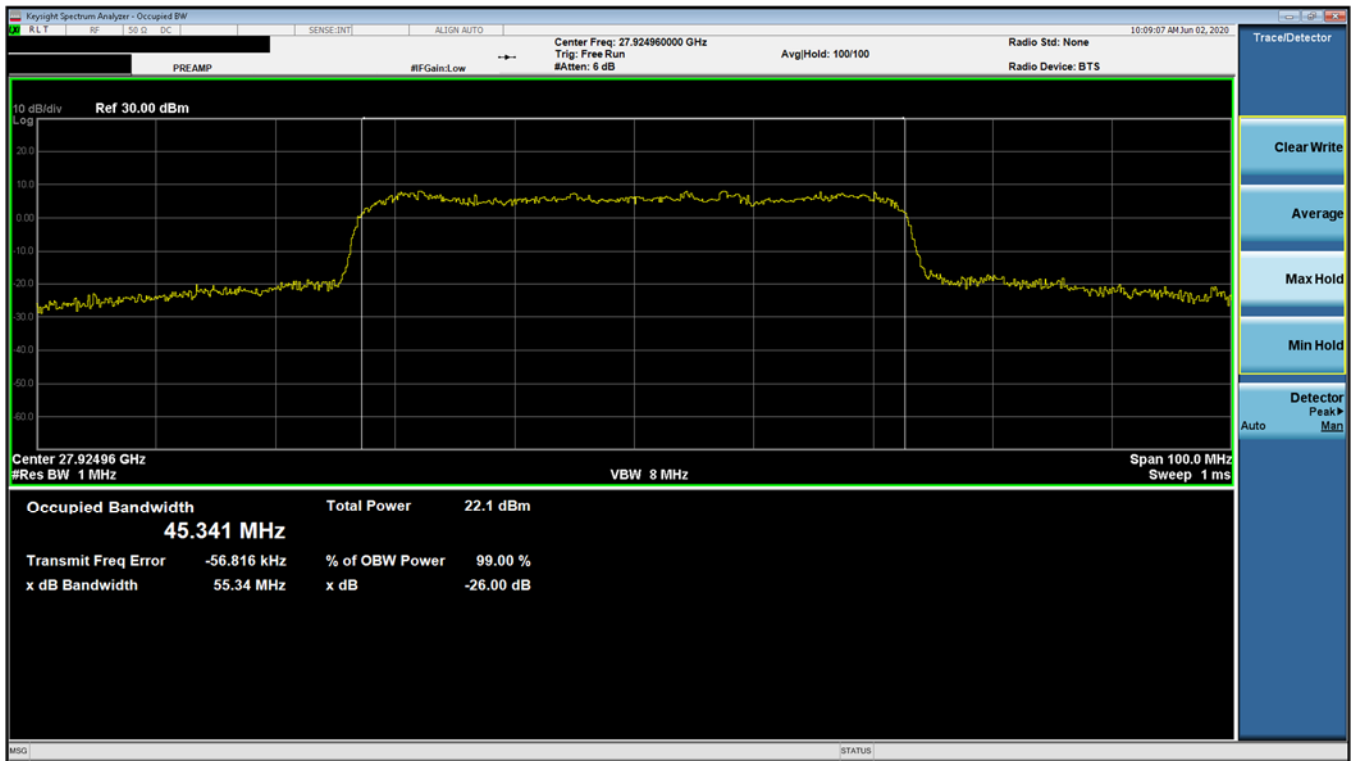
Plot 7-1. Ant 2 Occupied Bandwidth Plot (50MHz-1CC – QPSK – Mid Channel)
