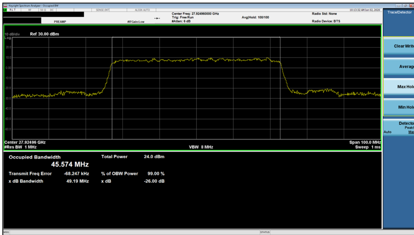
Plot 7-4. Ant 2 Occupied Bandwidth Plot (50MHz-1CC – pi/2-BPSK – Mid Channel)
