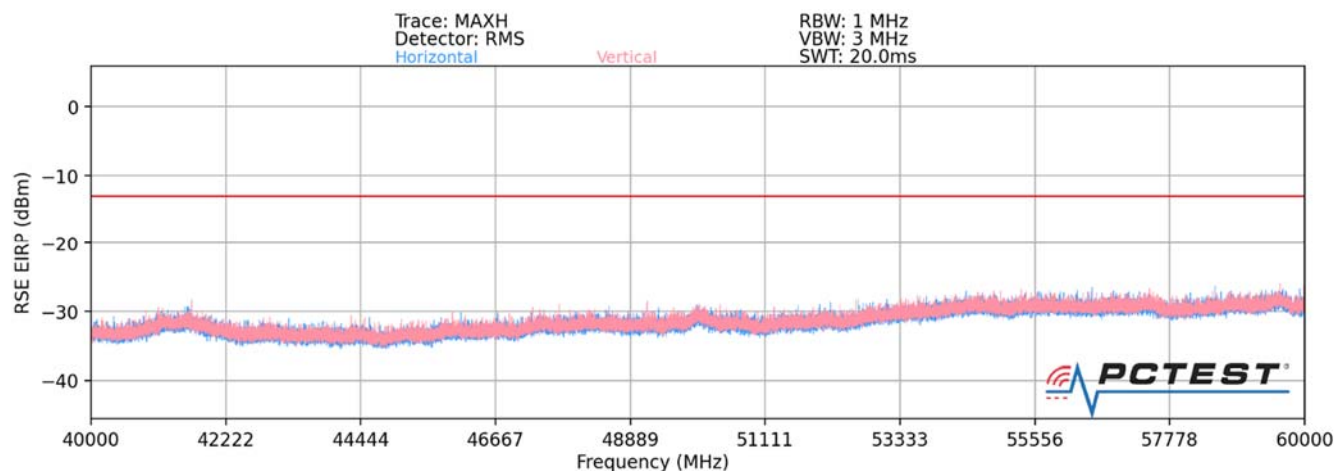
Plot 7-50. Ant 3-n260 Radiated Spurious Plot (1CC QPSK Mid Channel MIMO – ENDC Anchor Band 2)
