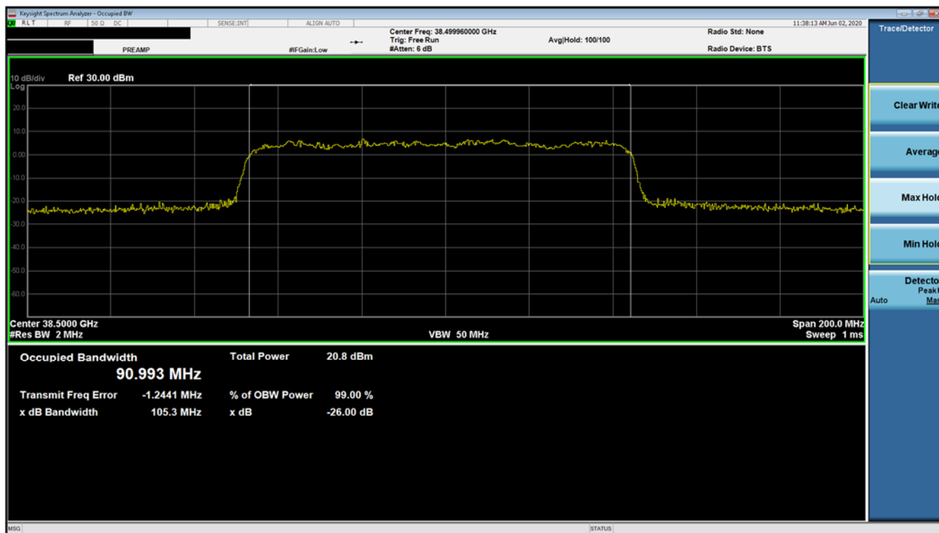
Plot 7-25. Ant 2 Occupied Bandwidth Plot (100MHz-1CC – QPSK – Mid Channel)
