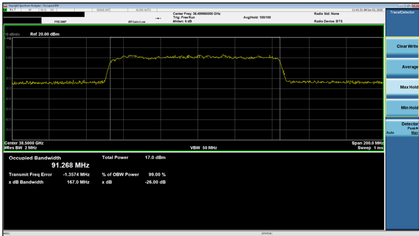
Plot 7-27. Ant 2 Occupied Bandwidth Plot (100MHz-1CC – 64QAM – Mid Channel)
