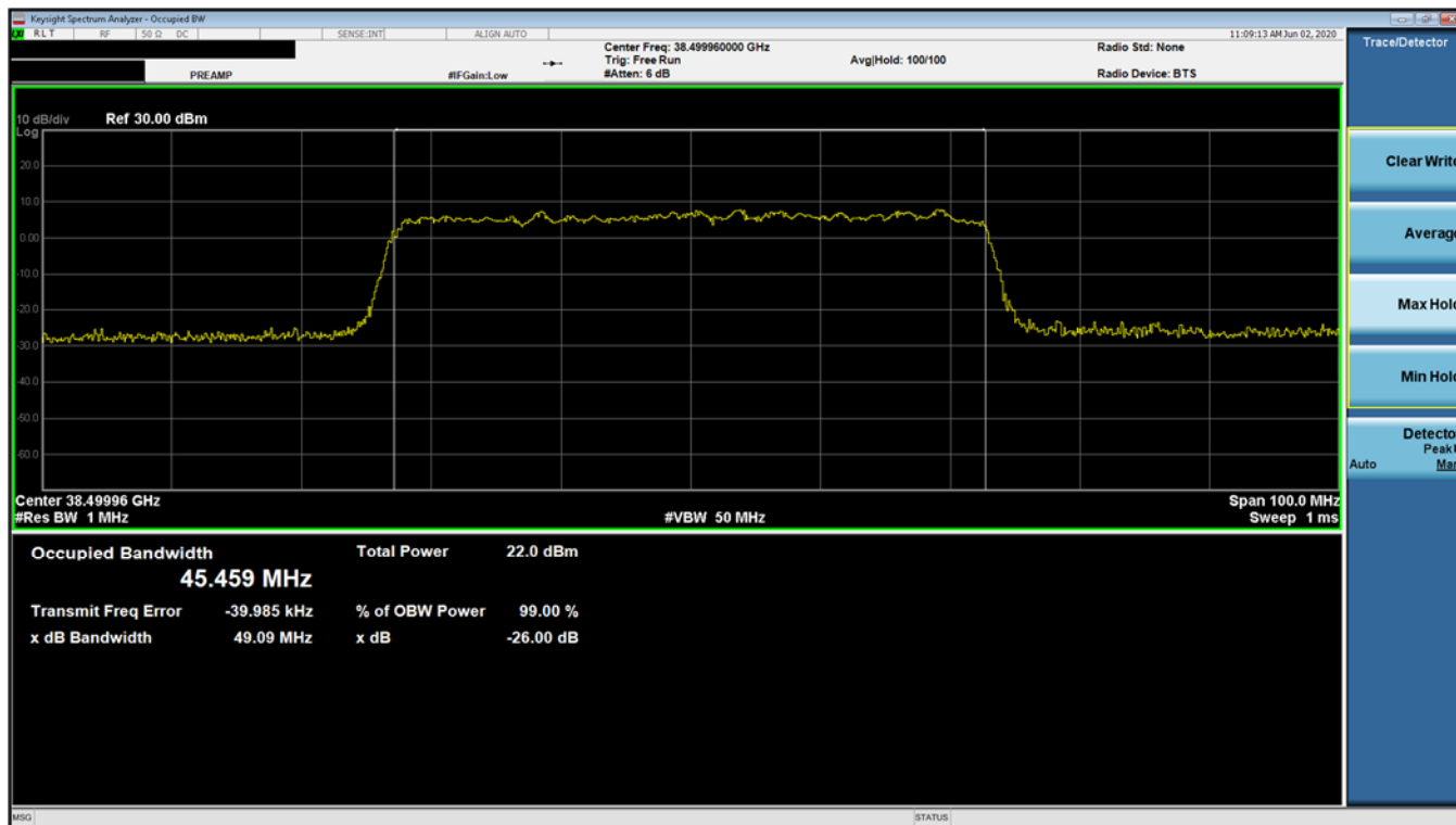
Plot 7-20. Ant 2 Occupied Bandwidth Plot (50MHz-1CC – pi/2-BPSK – Mid Channel)
