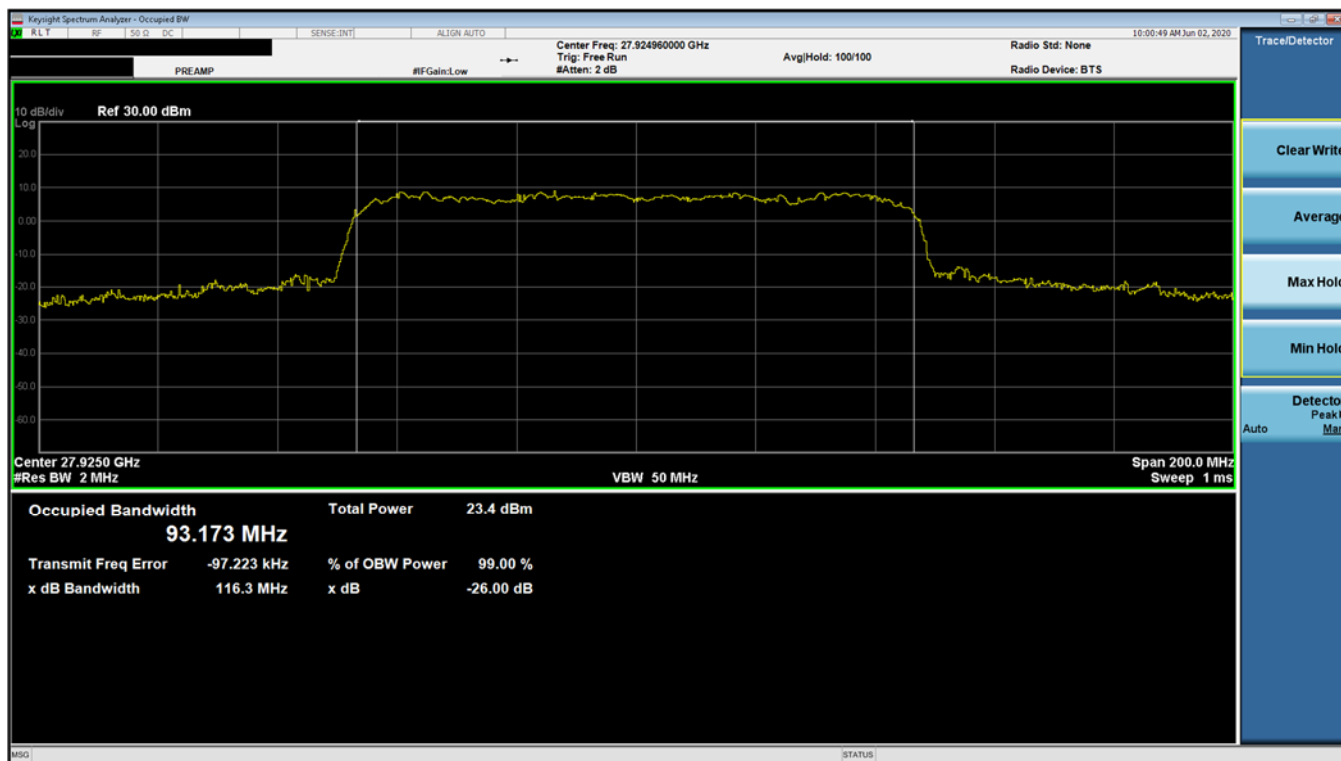
Plot 7-9. Ant 2 Occupied Bandwidth Plot (100MHz-1CC – QPSK – Mid Channel)
