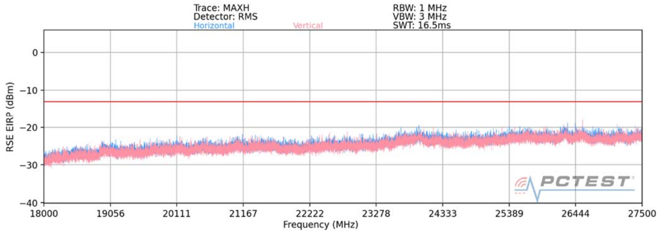
Plot 7-35. Ant 3-n261 Radiated Spurious Plot (1CC QPSK Mid Channel V Beam – ENDC Anchor B2)
