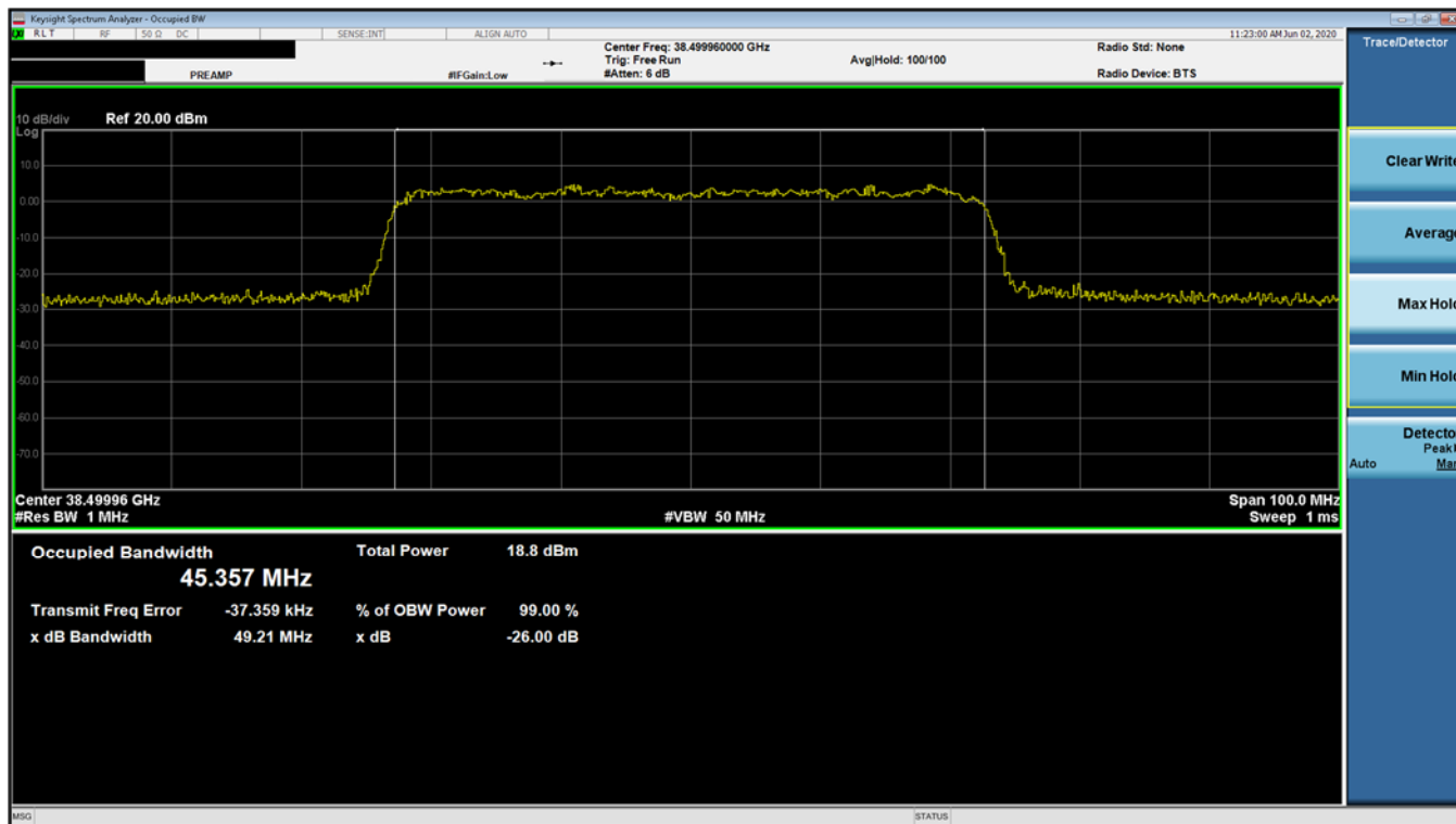
Plot 7-18. Ant 2 Occupied Bandwidth Plot (50MHz-1CC – 16QAM – Mid Channel)
