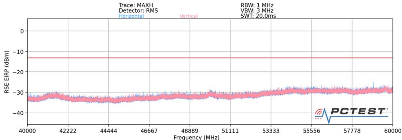
Plot 7-37. Ant 3-n261 Radiated Spurious Plot (1CC QPSK Mid Channel V Beam – ENDC Anchor B2)
