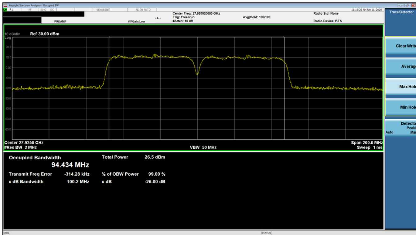
Plot 7-6. Ant 2 Occupied Bandwidth Plot (50MHz-2CC – 16QAM – Mid Channel)
