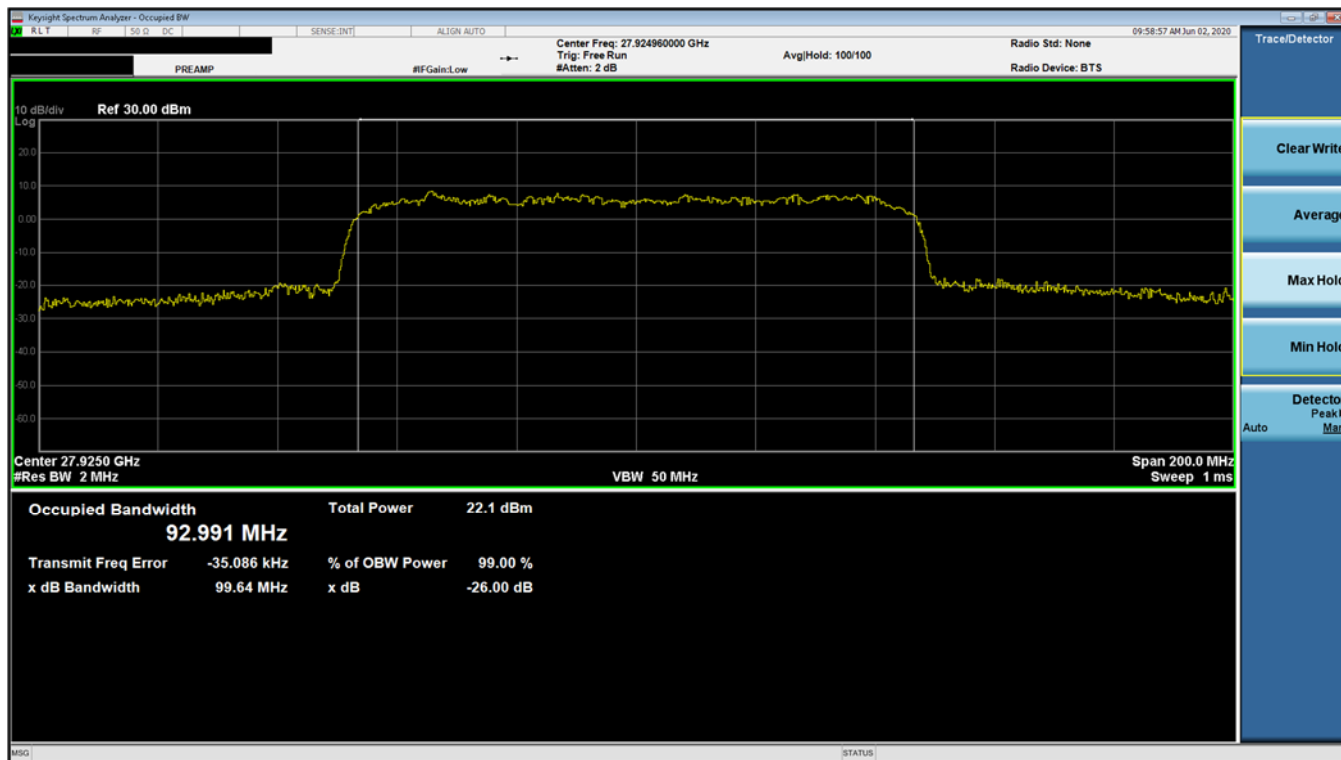
Plot 7-10. Ant 2 Occupied Bandwidth Plot (100MHz-1CC – 16QAM – Mid Channel)
