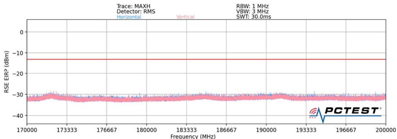
Plot 7-54. Ant 3-n260 Radiated Spurious Plot (1CC QPSK Mid Channel MIMO – ENDC Anchor Band 2)
