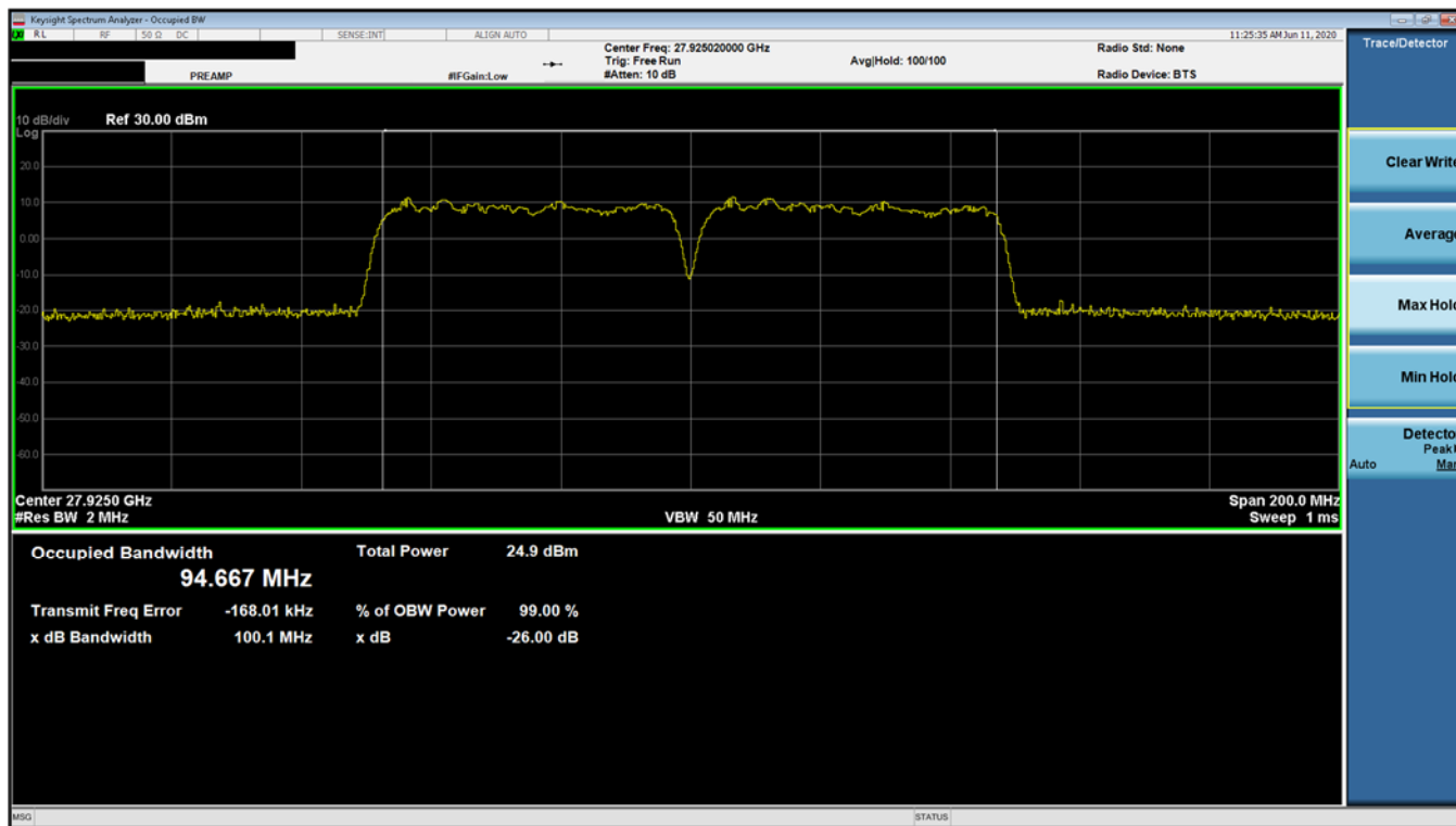
Plot 7-7. Ant 2 Occupied Bandwidth Plot (50MHz-2CC – 64QAM – Mid Channel)
