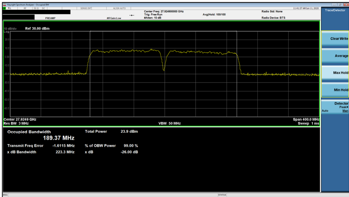
Plot 7-13. Ant 2 Occupied Bandwidth Plot (100MHz-2CC – QPSK – Mid Channel)
