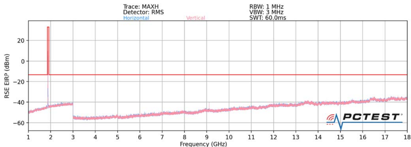
Plot 7-48. Ant 3-n260 Radiated Spurious Plot (1CC QPSK Mid Channel MIMO – ENDC Anchor Band 2)
