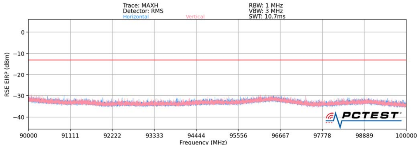
Plot 7-39. Ant 3-n261 Radiated Spurious Plot (1CC QPSK Mid Channel V Beam – ENDC Anchor B2)
