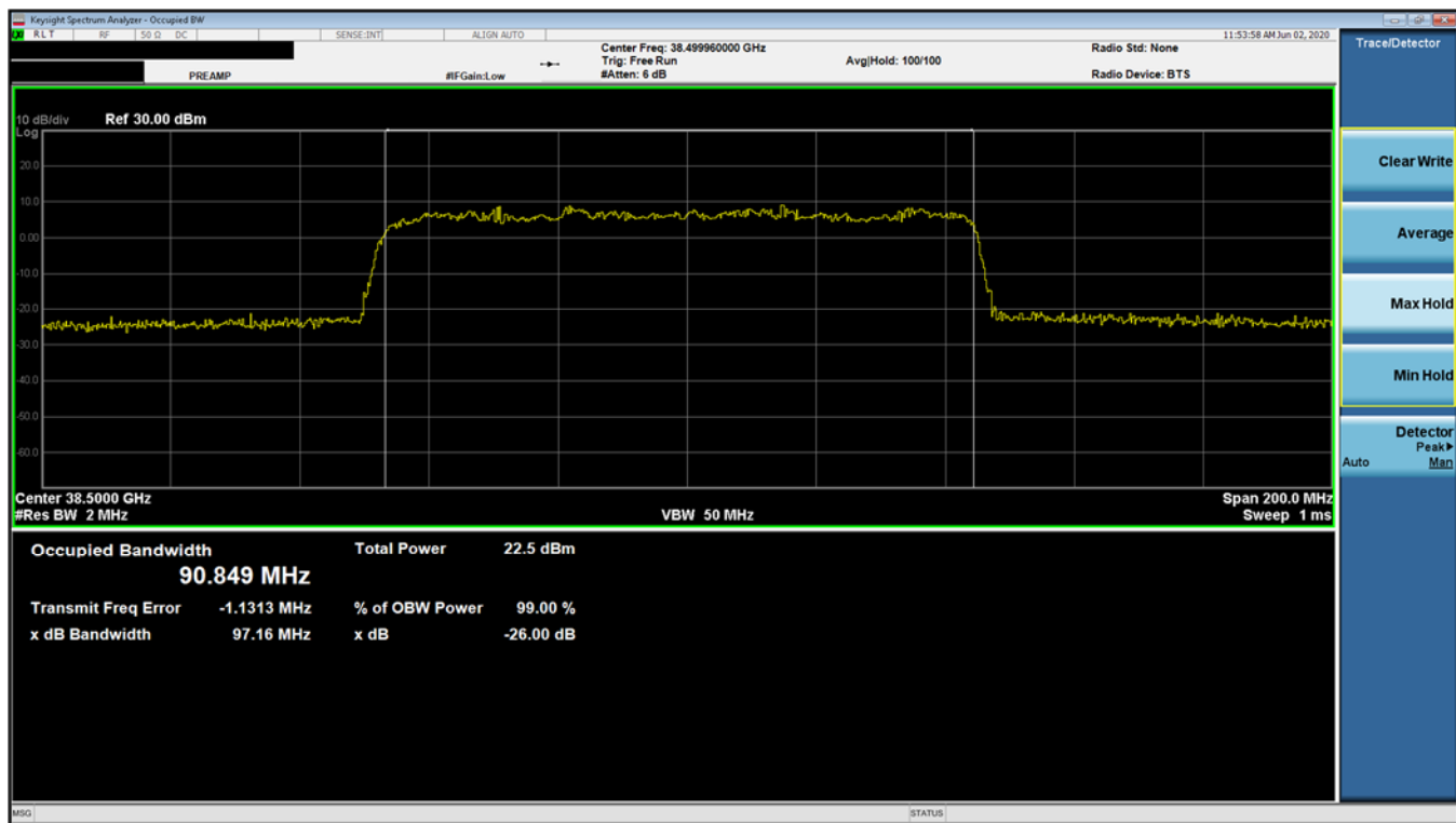
Plot 7-28. Ant 2 Occupied Bandwidth Plot (100MHz-1CC – pi/2-BPSK – Mid Channel)
