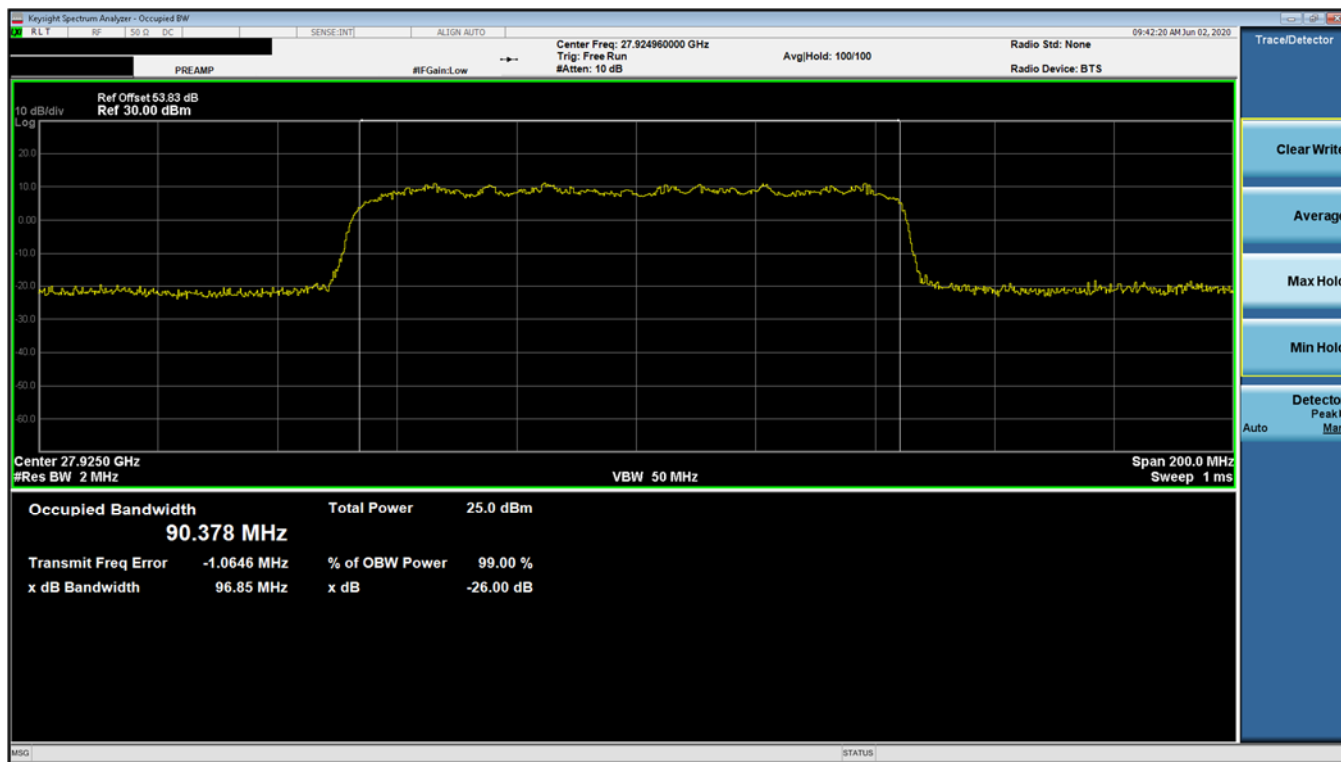
Plot 7-12. Ant 2 Occupied Bandwidth Plot (100MHz-1CC – pi/2-BPSK – Mid Channel)
