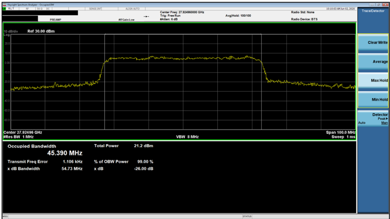
Plot 7-2. Ant 2 Occupied Bandwidth Plot (50MHz-1CC – 16QAM – Mid Channel)
