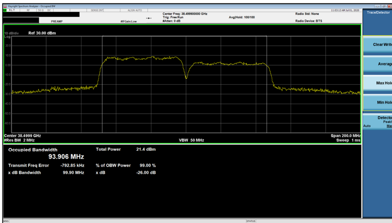
Plot 7-21. Ant 2 Occupied Bandwidth Plot (50MHz-2CC – QPSK – Mid Channel)
