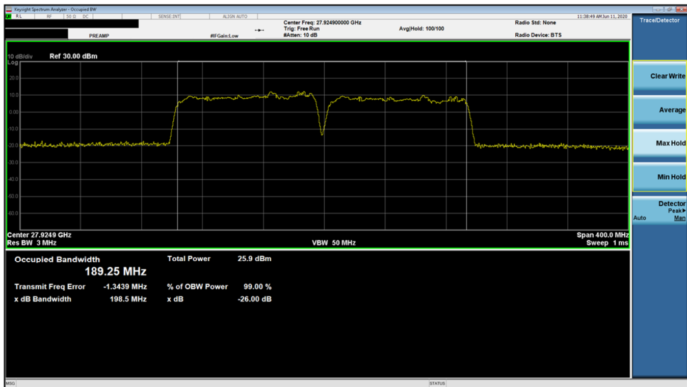
Plot 7-14. Ant 2 Occupied Bandwidth Plot (100MHz-2CC – 16QAM – Mid Channel)
