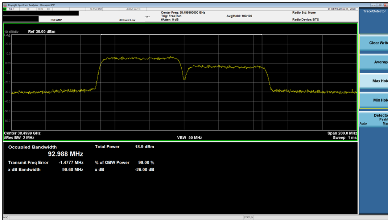
Plot 7-22. Ant 2 Occupied Bandwidth Plot (50MHz-2CC – 16QAM – Mid Channel)
