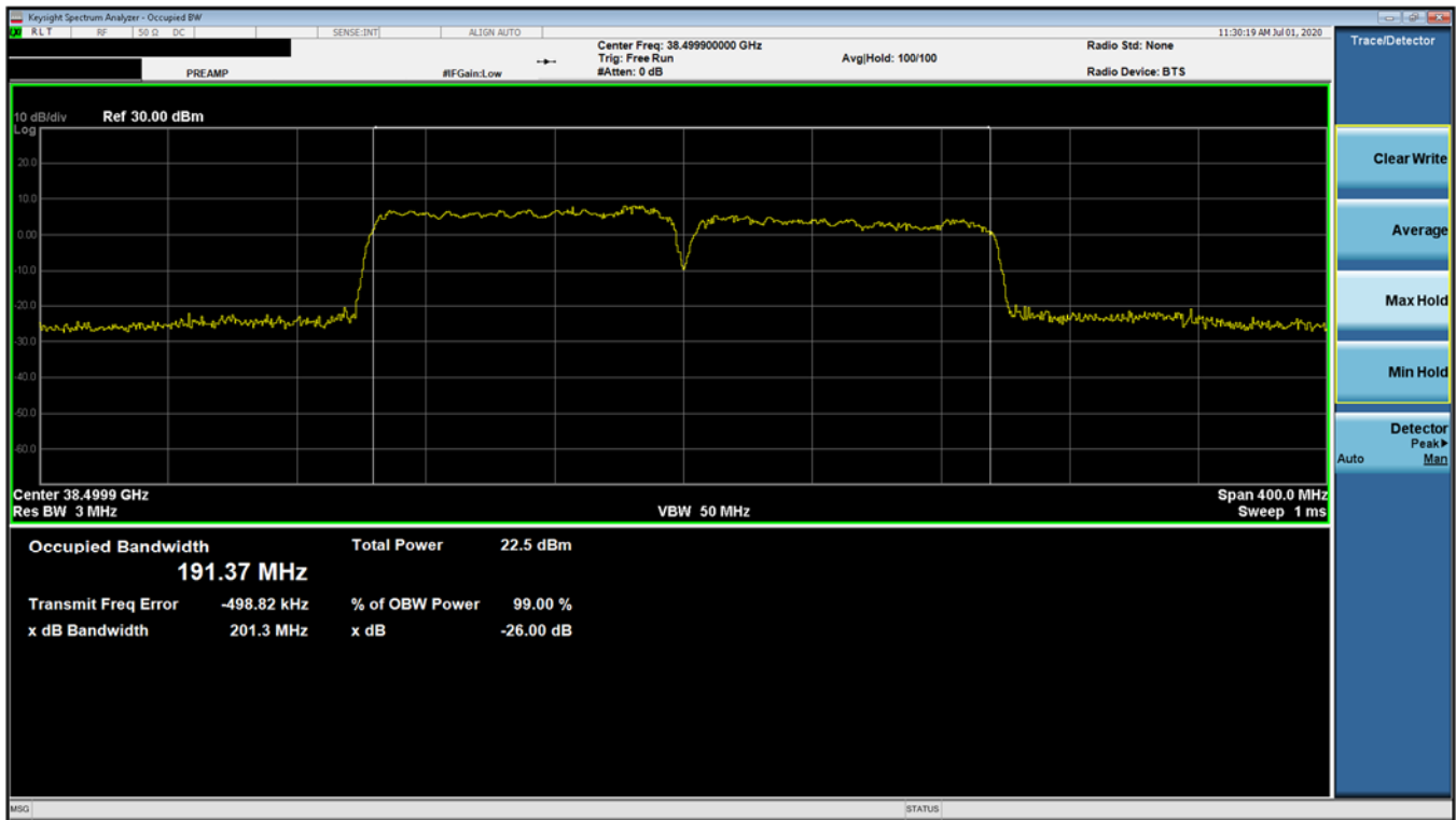
Plot 7-29. Ant 2 Occupied Bandwidth Plot (100MHz-2CC – QPSK – Mid Channel)
