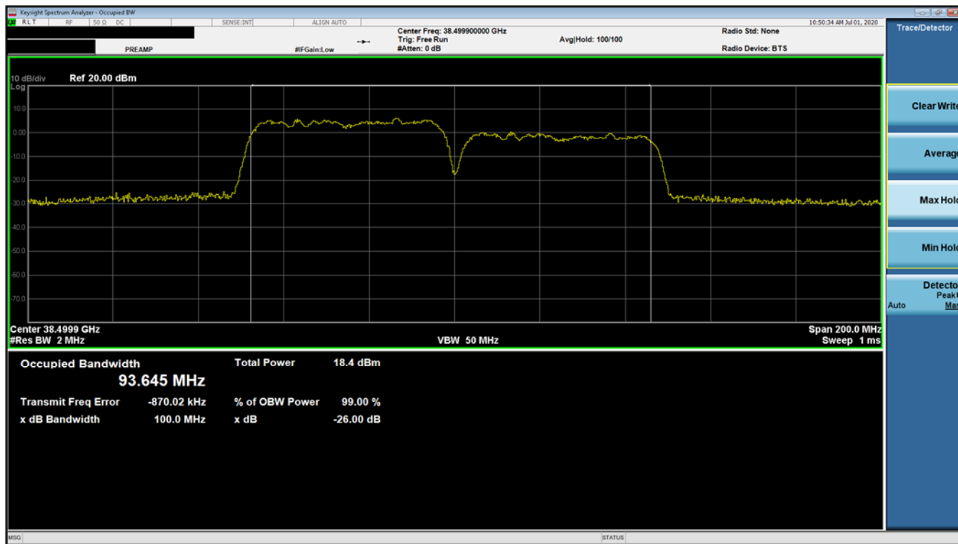
Plot 7-24. Ant 2 Occupied Bandwidth Plot (50MHz-2CC – pi/2-BPSK – Mid Channel)
