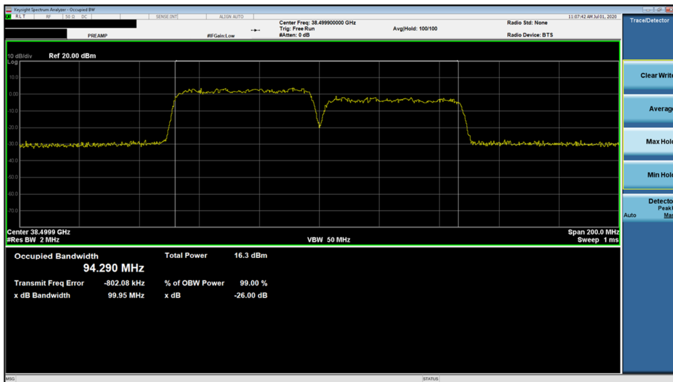
Plot 7-23. Ant 2 Occupied Bandwidth Plot (50MHz-2CC – 64QAM – Mid Channel)
