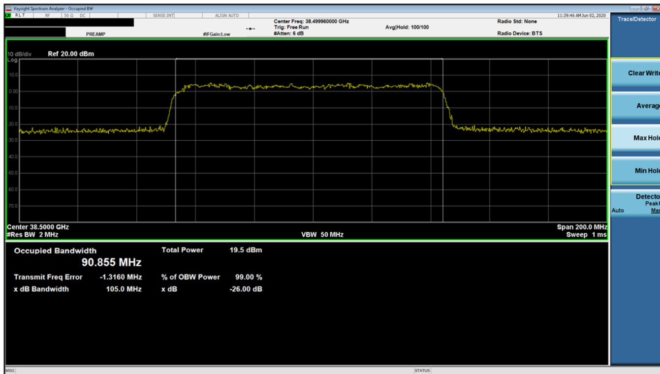
Plot 7-26. Ant 2 Occupied Bandwidth Plot (100MHz-1CC – 16QAM – Mid Channel)
