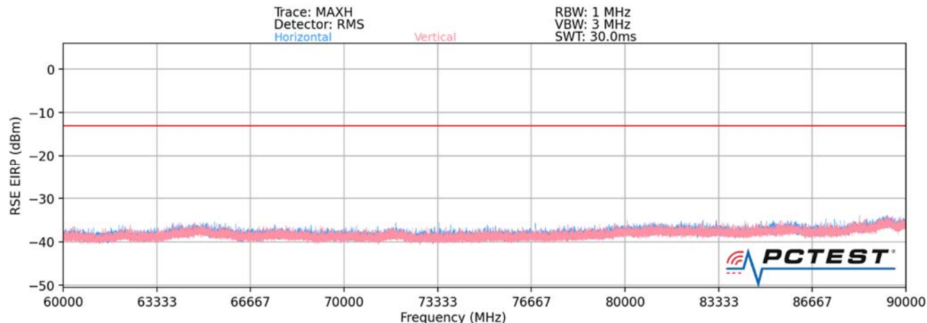
Plot 7-38. Ant 3-n261 Radiated Spurious Plot (1CC QPSK Mid Channel V Beam – ENDC Anchor B2)
