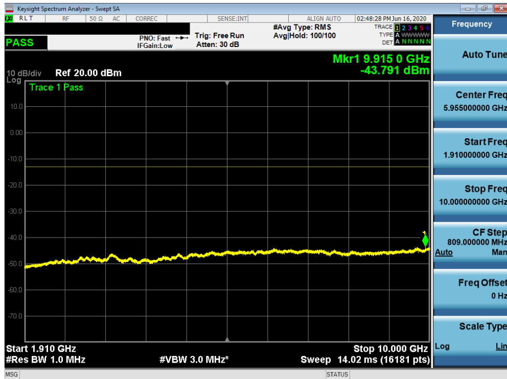
Plot 7-53. Conducted Spurious Plot (NR Band n2 - 20.0MHz - RB Size 1, RB Offset 0 - Low Channel)
