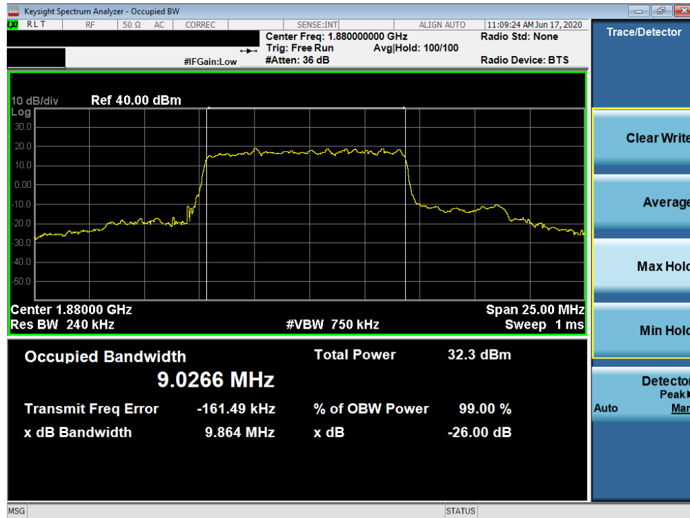
Plot 7-29. Occupied Bandwidth Plot (NR Band n2 - 10.0MHz DFT-s-OFDM BPSK - Full RB)
