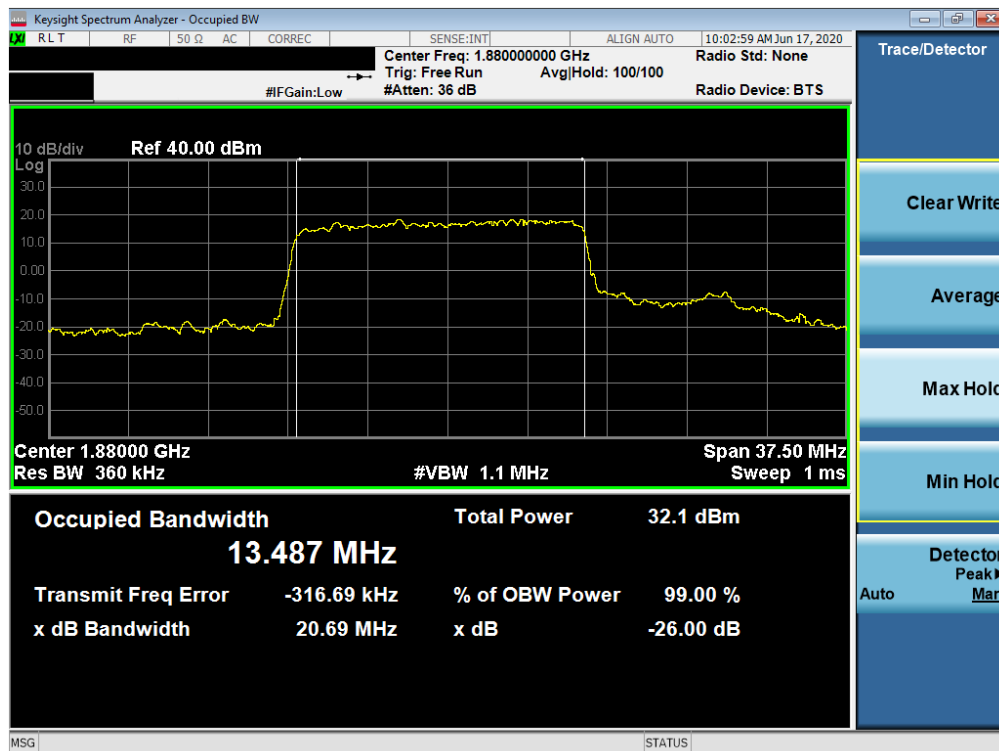
Plot 7-24. Occupied Bandwidth Plot (NR Band n2 - 15.0MHz DFT-s-OFDM BPSK - Full RB)
