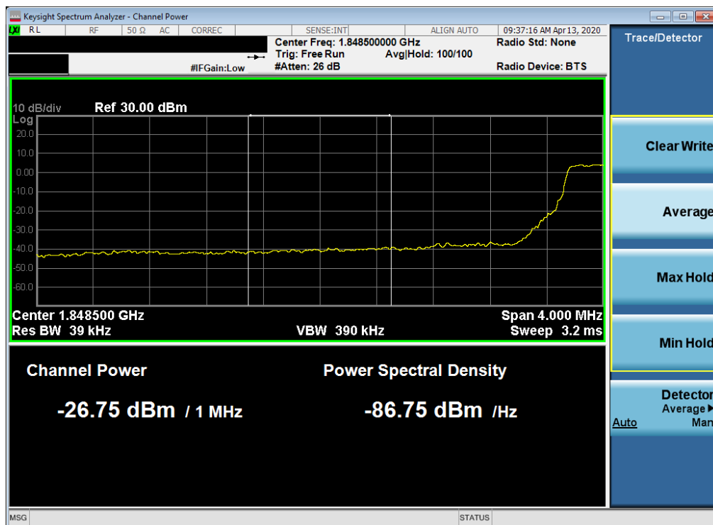
Plot 7-101. Extended Lower Band Edge Plot (LTE Band 2 - 5MHz QPSK – Full RB Configuration)
