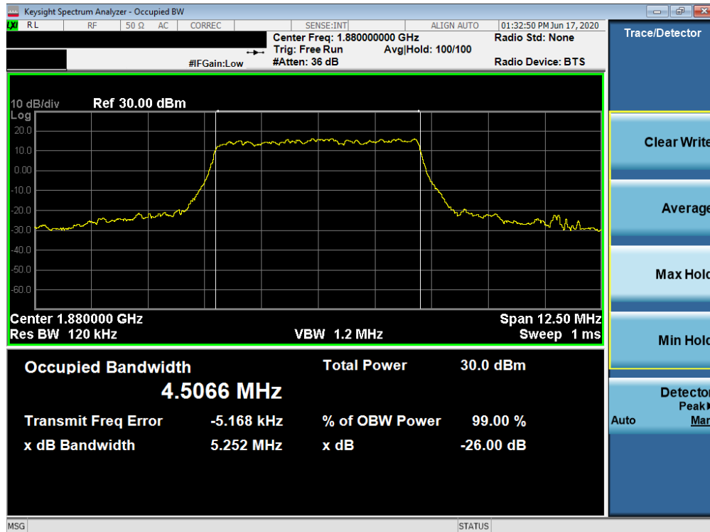
Plot 7-37. Occupied Bandwidth Plot (NR Band n2 - 5.0MHz CP-OFDM 64QAM - Full RB)
