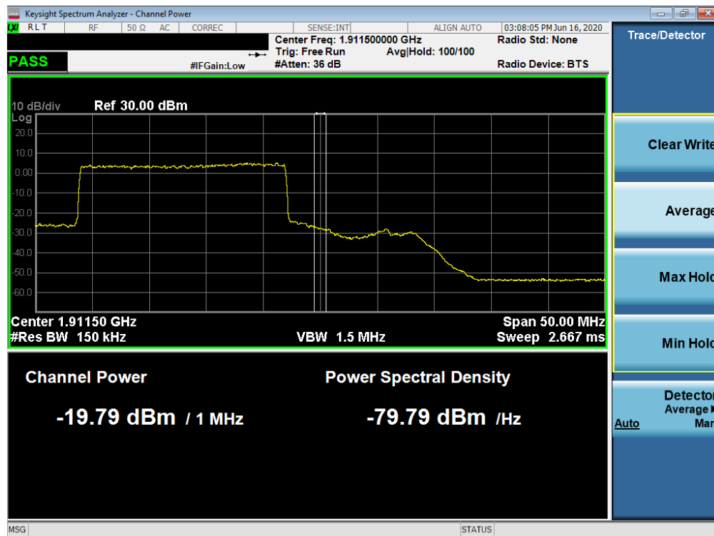
Plot 7-115. Upper Extended Band Edge Plot (NR Band n2 – 20.0MHz - Full RB)
