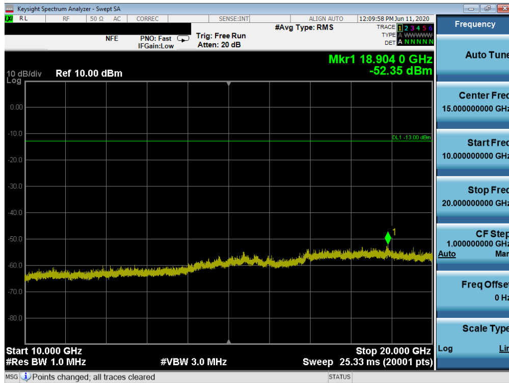
Plot 7-81. Conducted Spurious Plot (CDMA Ch. 25)
