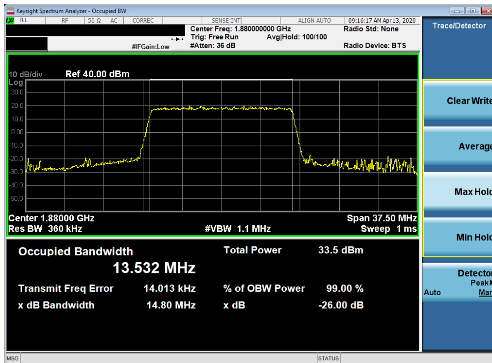
Plot 7-4. Occupied Bandwidth Plot (LTE Band 2 - 15MHz QPSK - Full RB Configuration)
