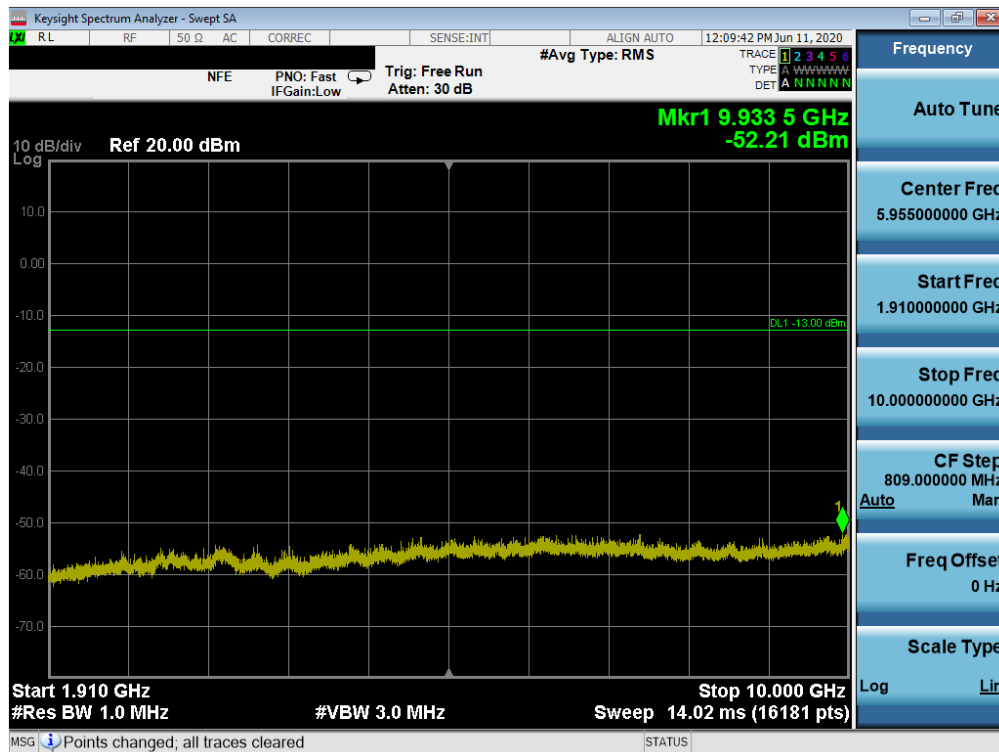
Plot 7-80. Conducted Spurious Plot (CDMA Ch. 25)
