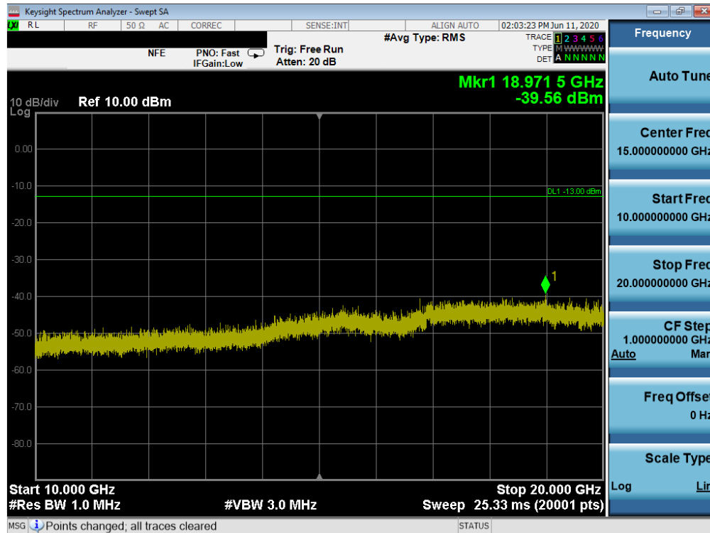
Plot 7-69. Conducted Spurious Plot (GPRS Ch. 810)
