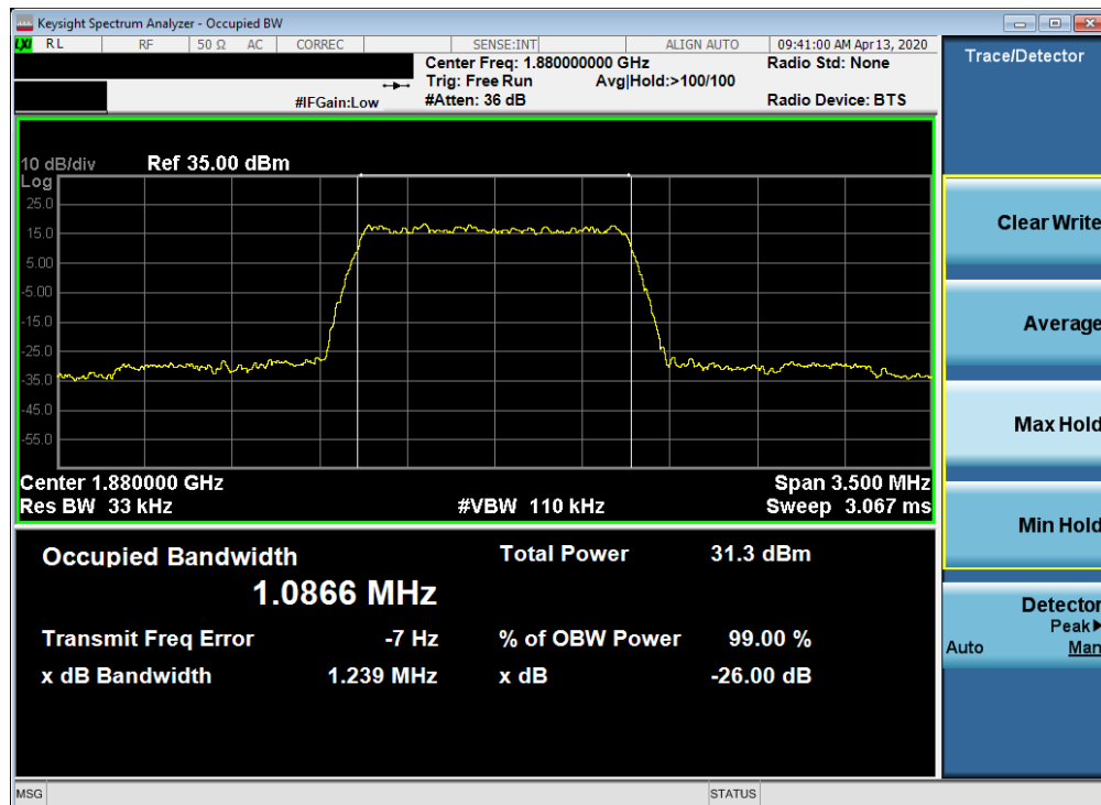
Plot 7-18. Occupied Bandwidth Plot (LTE Band 2 - 1.4MHz 64-QAM - Full RB Configuration)
