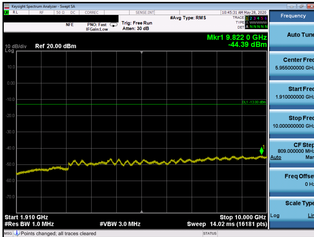
Plot 7-47. Conducted Spurious Plot (LTE Band 2 - 20MHz QPSK - RB Size 1, RB Offset 0 - Mid Channel)
