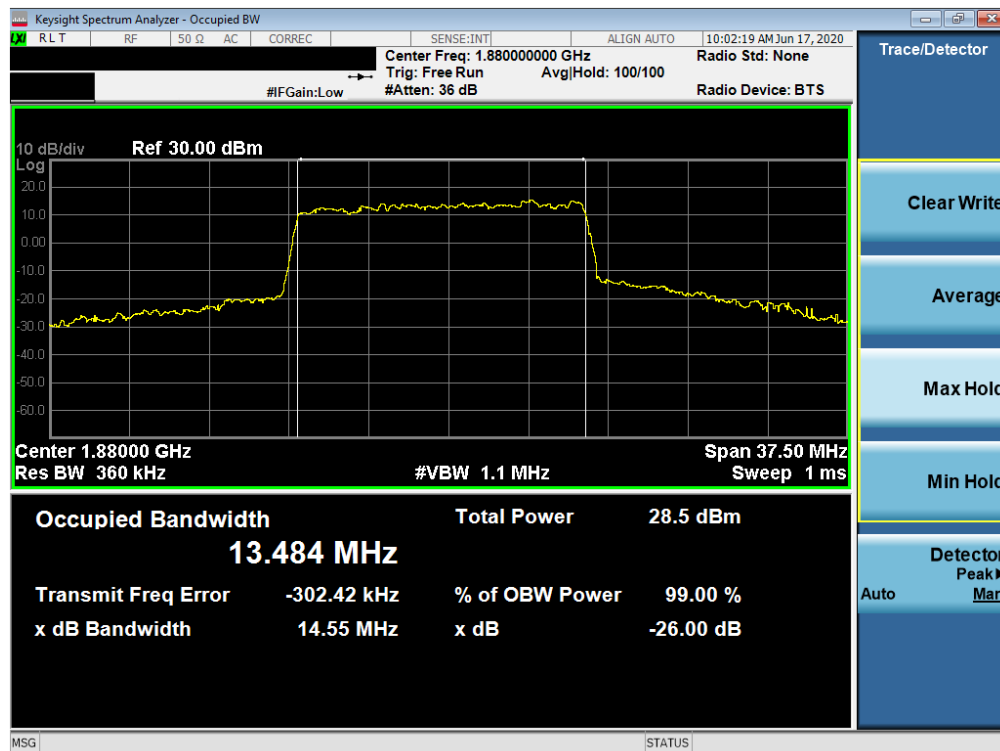
Plot 7-28. Occupied Bandwidth Plot (NR Band n2 - 15.0MHz CP-OFDM 256QAM - Full RB)
