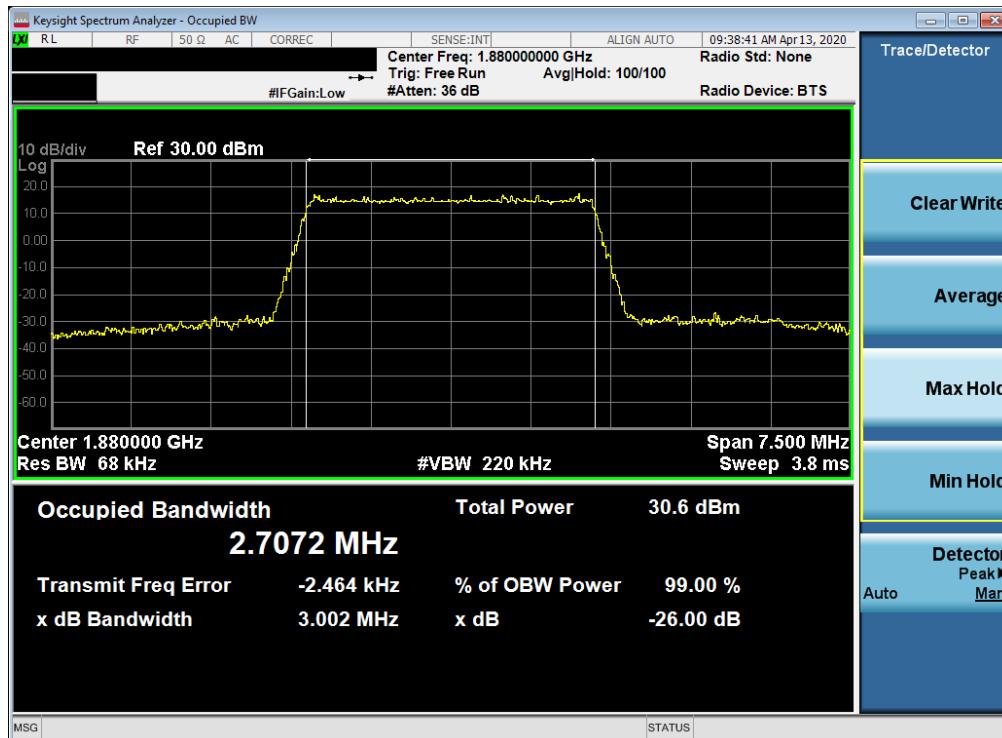
Plot 7-15. Occupied Bandwidth Plot (LTE Band 2 - 3MHz 64-QAM - Full RB Configuration)
