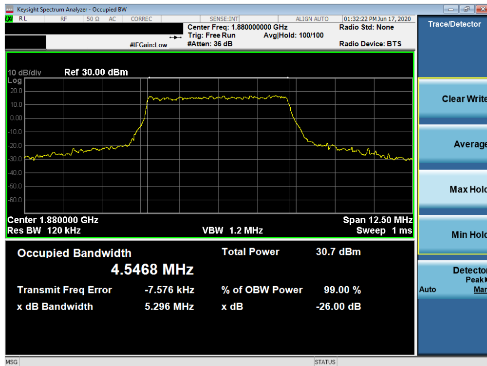
Plot 7-36. Occupied Bandwidth Plot (NR Band n2 - 5.0MHz CP-OFDM 16QAM - Full RB)
