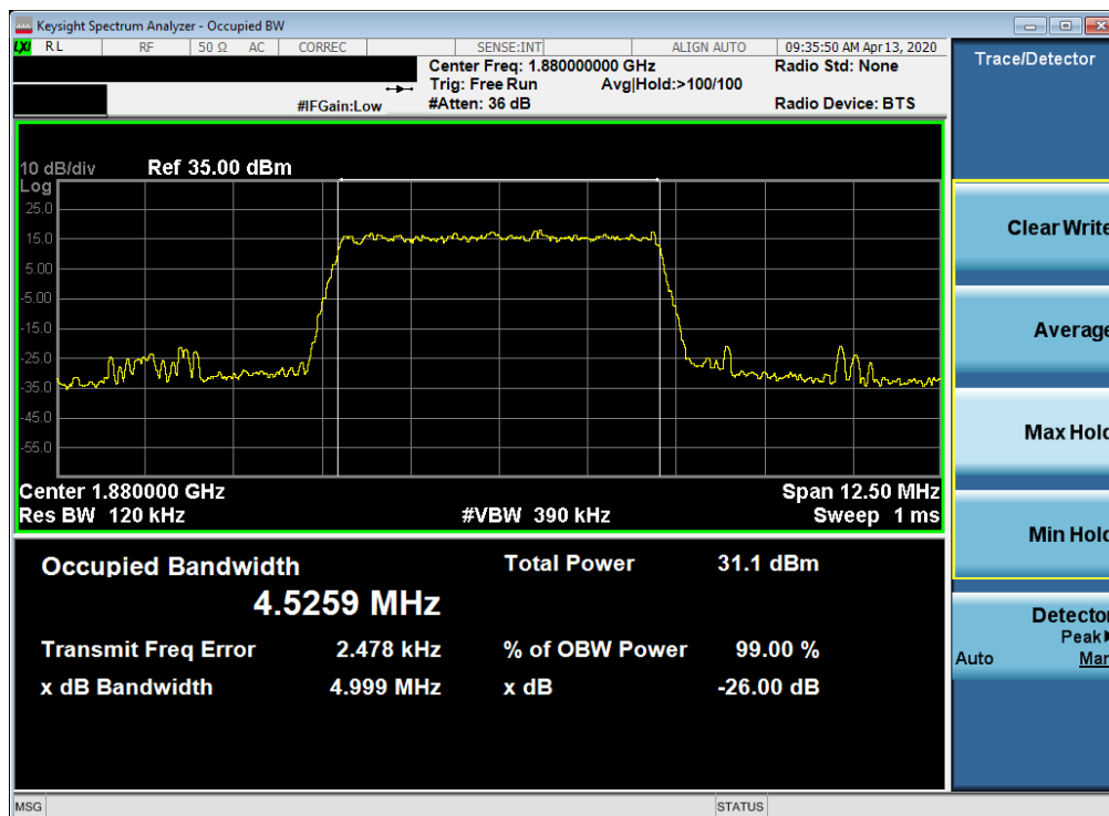
Plot 7-12. Occupied Bandwidth Plot (LTE Band 2 - 5MHz 64-QAM - Full RB Configuration)
