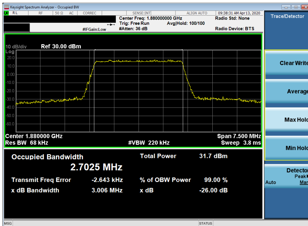
Plot 7-14. Occupied Bandwidth Plot (LTE Band 2 - 3MHz 16-QAM - Full RB Configuration)
