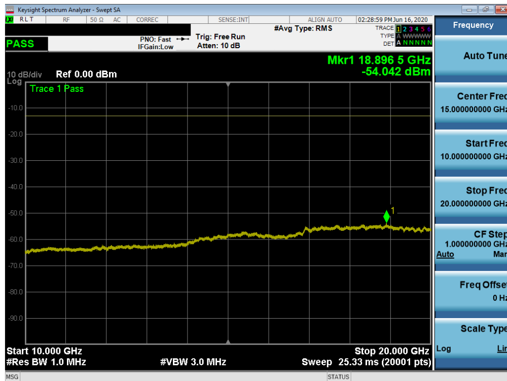
Plot 7-57. Conducted Spurious Plot (NR Band n2 - 20.0MHz - RB Size 1, RB Offset 0 - Mid Channel)
