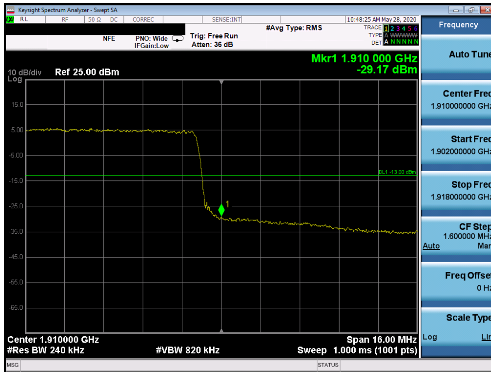
Plot 7-90. Upper Band Edge Plot (LTE Band 2 - 20MHz QPSK – Full RB Configuration)
