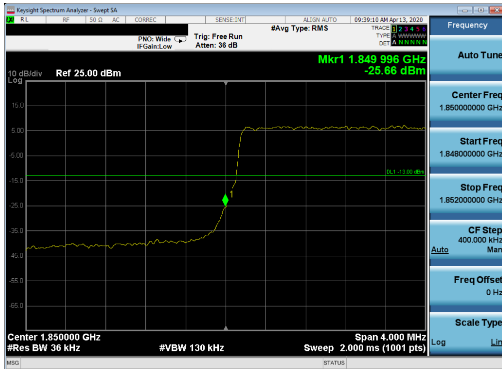
Plot 7-104. Lower Band Edge Plot (LTE Band 2 - 3MHz QPSK – Full RB Configuration)
