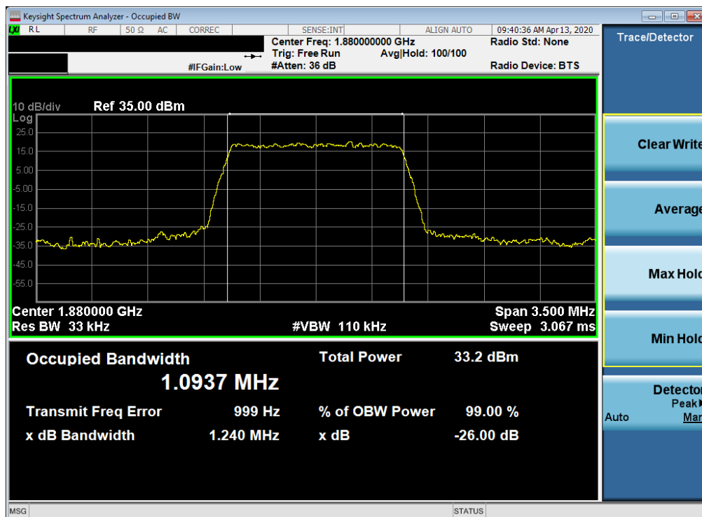
Plot 7-16. Occupied Bandwidth Plot (LTE Band 2 - 1.4MHz QPSK - Full RB Configuration)
