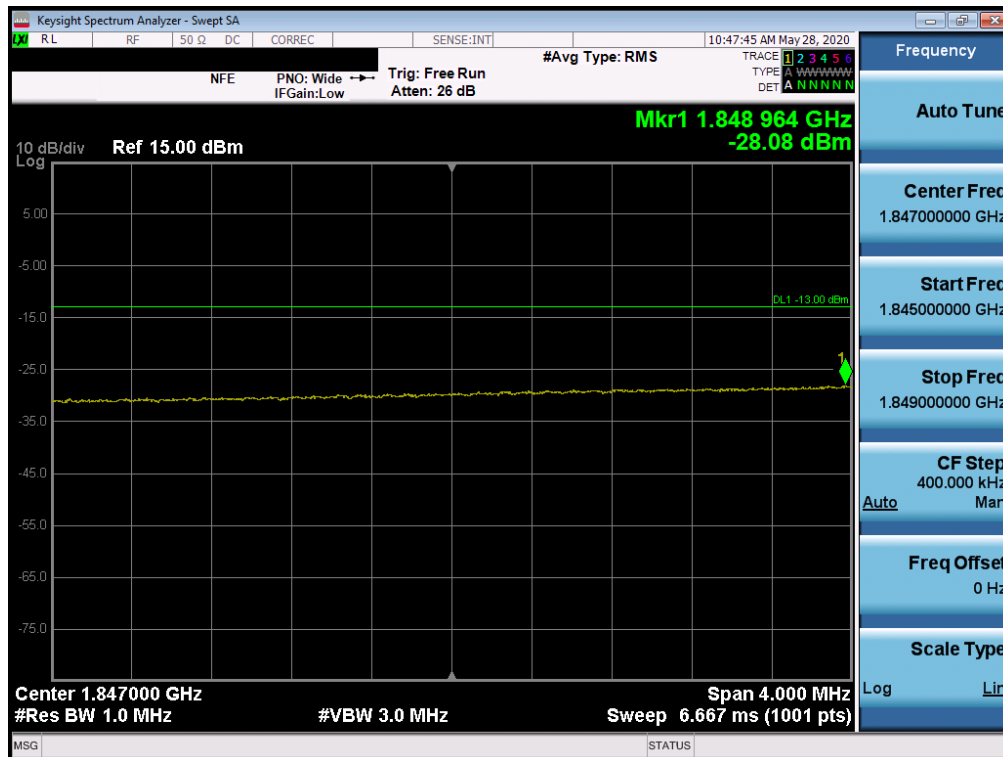
Plot 7-89. Extended Lower Band Edge Plot (LTE Band 2 - 20MHz QPSK - Full RB Configuration)
