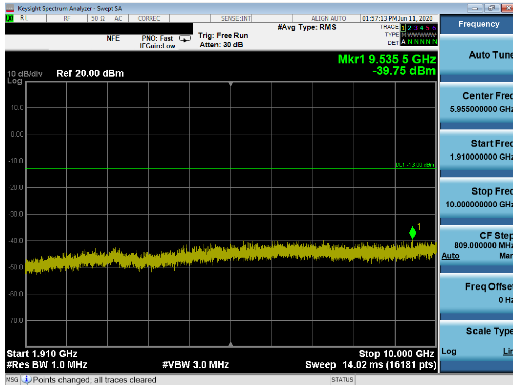
Plot 7-65. Conducted Spurious Plot (GPRS Ch. 661)
