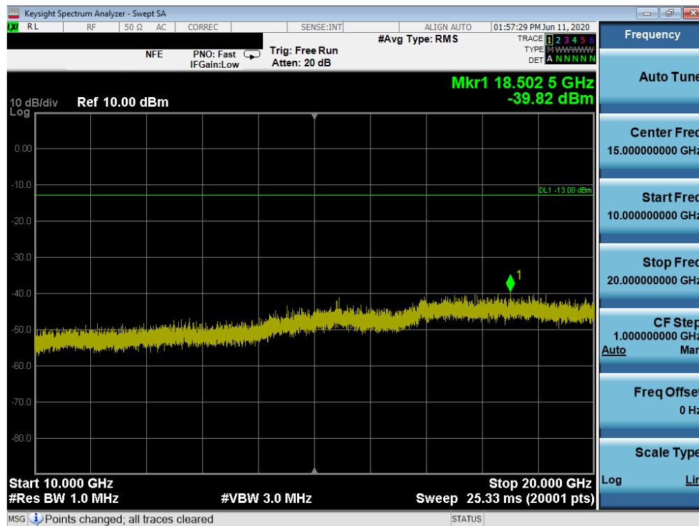
Plot 7-66. Conducted Spurious Plot (GPRS Ch. 661)
