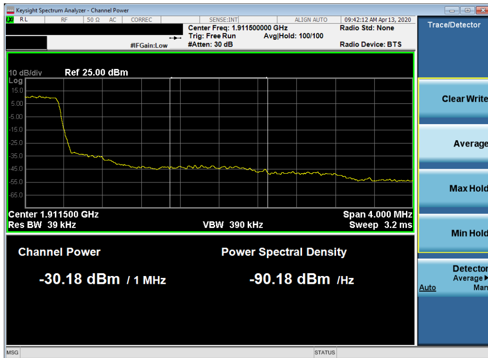
Plot 7-111. Extended Upper Band Edge Plot (LTE Band 2 – 1.4MHz QPSK – Full RB Configuration)
