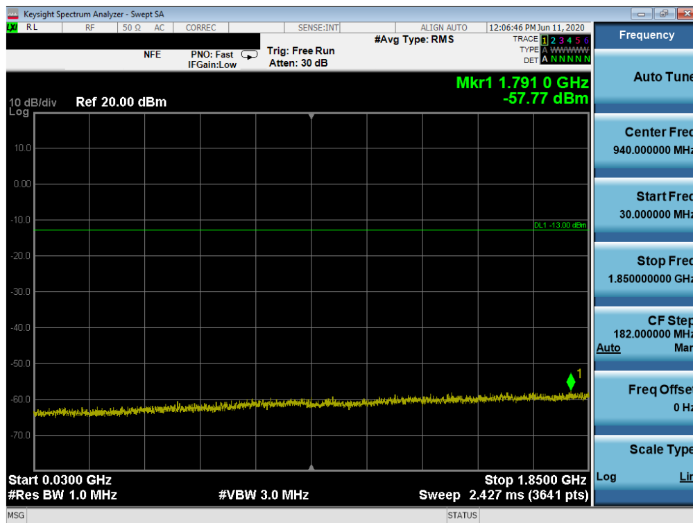
Plot 7-82. Conducted Spurious Plot (CDMA Ch. 600)
