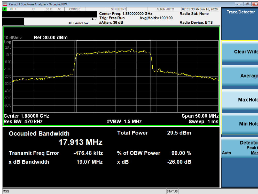
Plot 7-23. Occupied Bandwidth Plot (NR Band n2 - 20.0MHz CP-OFDM 256QAM - Full RB)
