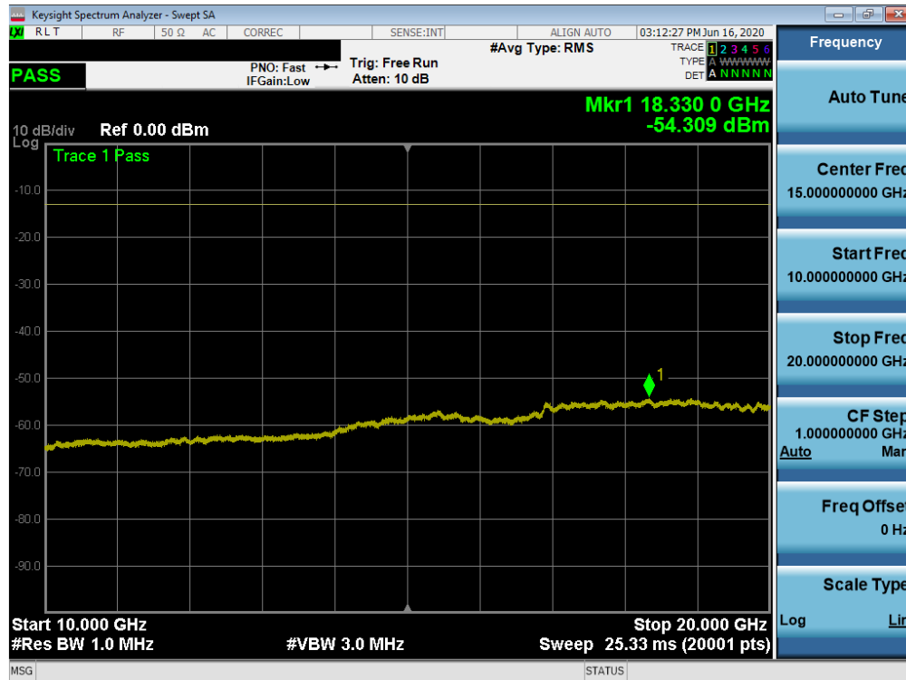
Plot 7-60. Conducted Spurious Plot (NR Band n2 - 20.0MHz - RB Size 1, RB Offset 0 - High Channel)
