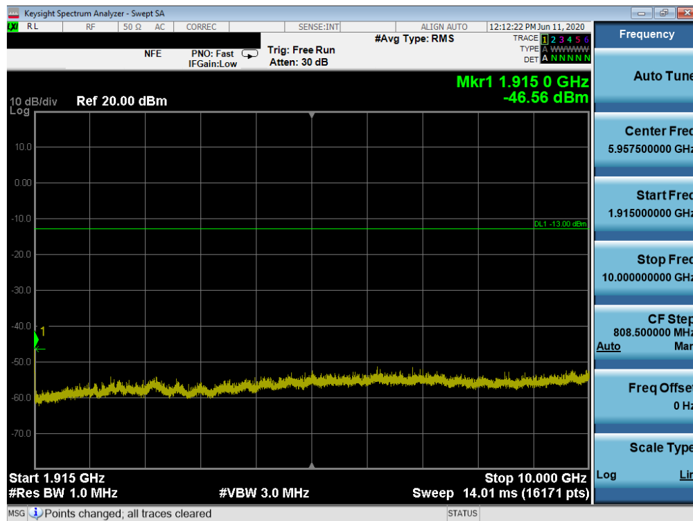
Plot 7-86. Conducted Spurious Plot (CDMA Ch. 1175)
