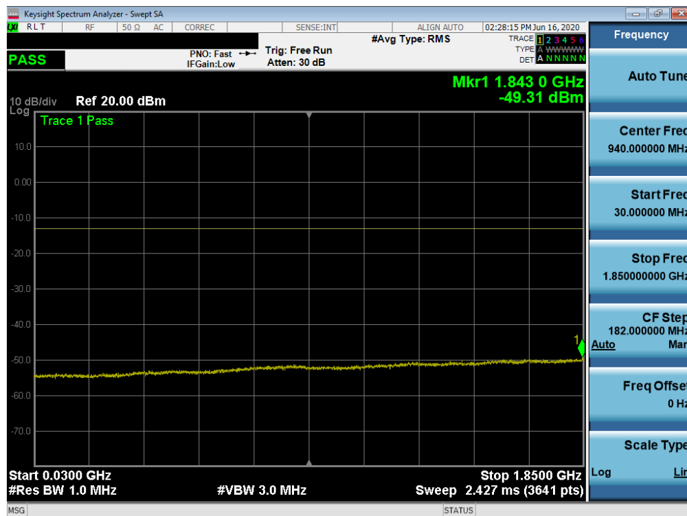
Plot 7-55. Conducted Spurious Plot (NR Band n2 - 20.0MHz - RB Size 1, RB Offset 0 - Mid Channel)
