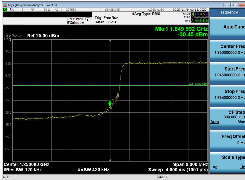
Plot 7-96. Lower Band Edge Plot (LTE Band 2 - 10MHz QPSK – Full RB Configuration)
