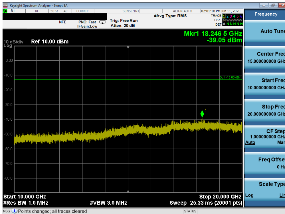
Plot 7-63. Conducted Spurious Plot (GPRS Ch. 512)
