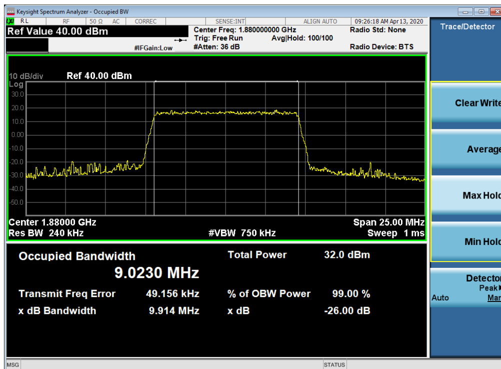
Plot 7-8. Occupied Bandwidth Plot (LTE Band 2 - 10MHz 16-QAM - Full RB Configuration)
