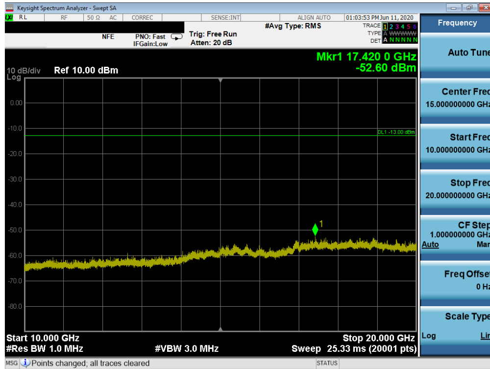
Plot 7-78. Conducted Spurious Plot (WCDMA Ch. 9538)
