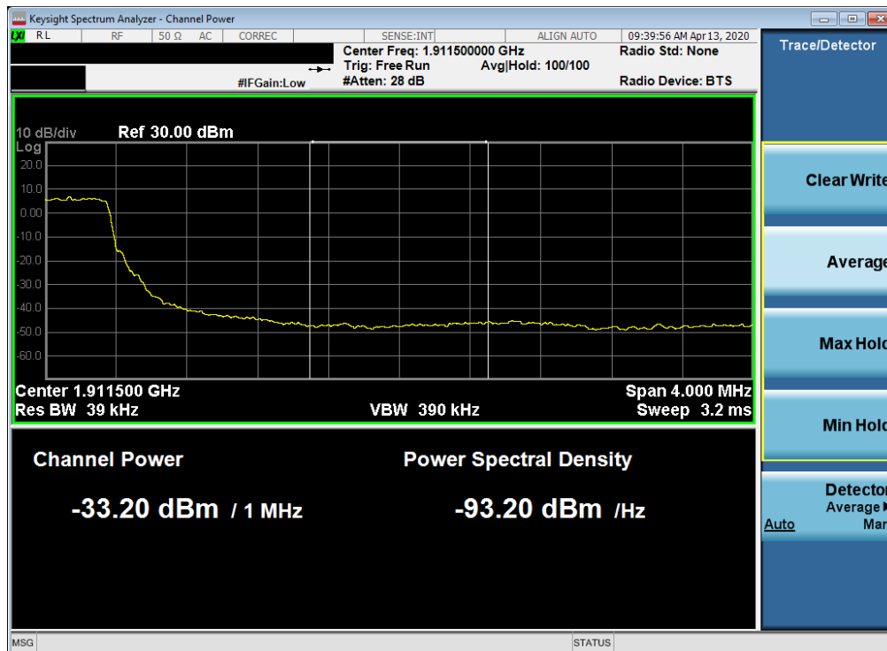
Plot 7-107. Extended Upper Band Edge Plot (LTE Band 2 - 3MHz QPSK – Full RB Configuration)
