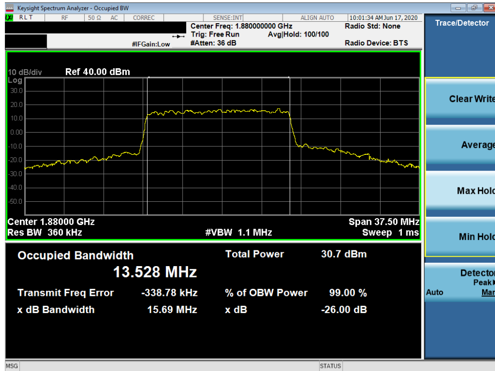
Plot 7-27. Occupied Bandwidth Plot (NR Band n2 - 15.0MHz CP-OFDM 64QAM - Full RB)
