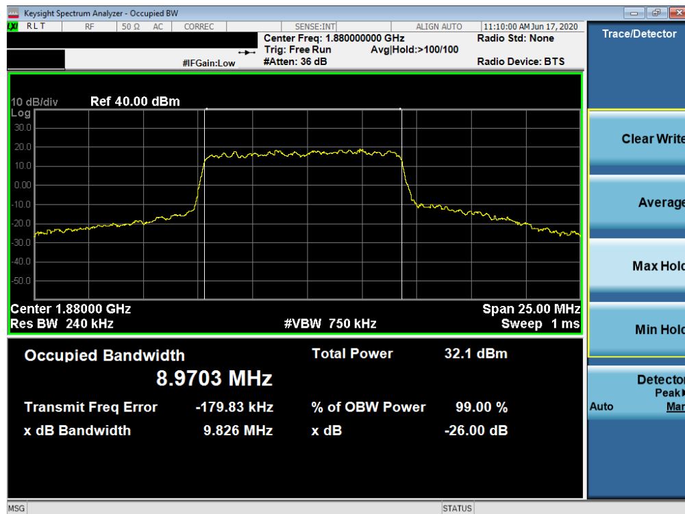
Plot 7-30. Occupied Bandwidth Plot (NR Band n2 - 10.0MHz CP-OFDM QPSK - Full RB)
