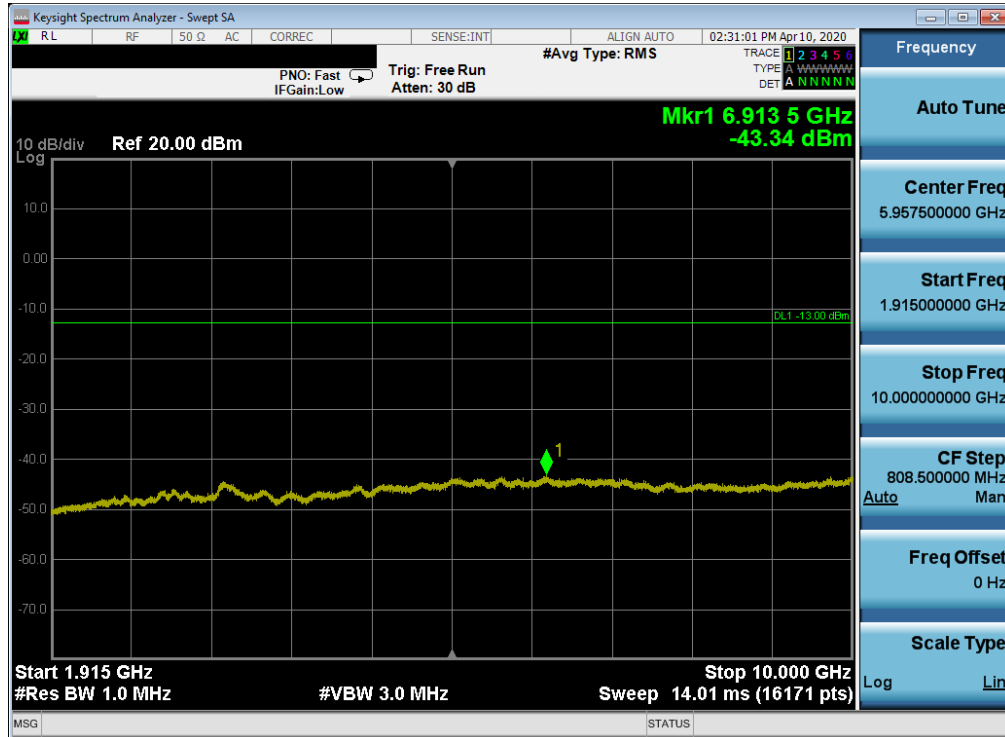
Plot 7-44. Conducted Spurious Plot (LTE Band 2 - 20MHz QPSK - RB Size 1, RB Offset 0 - Low Channel)
