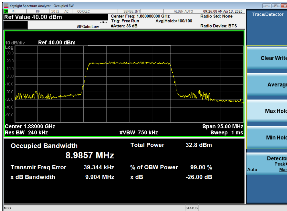
Plot 7-7. Occupied Bandwidth Plot (LTE Band 2 - 10MHz QPSK - Full RB Configuration)
