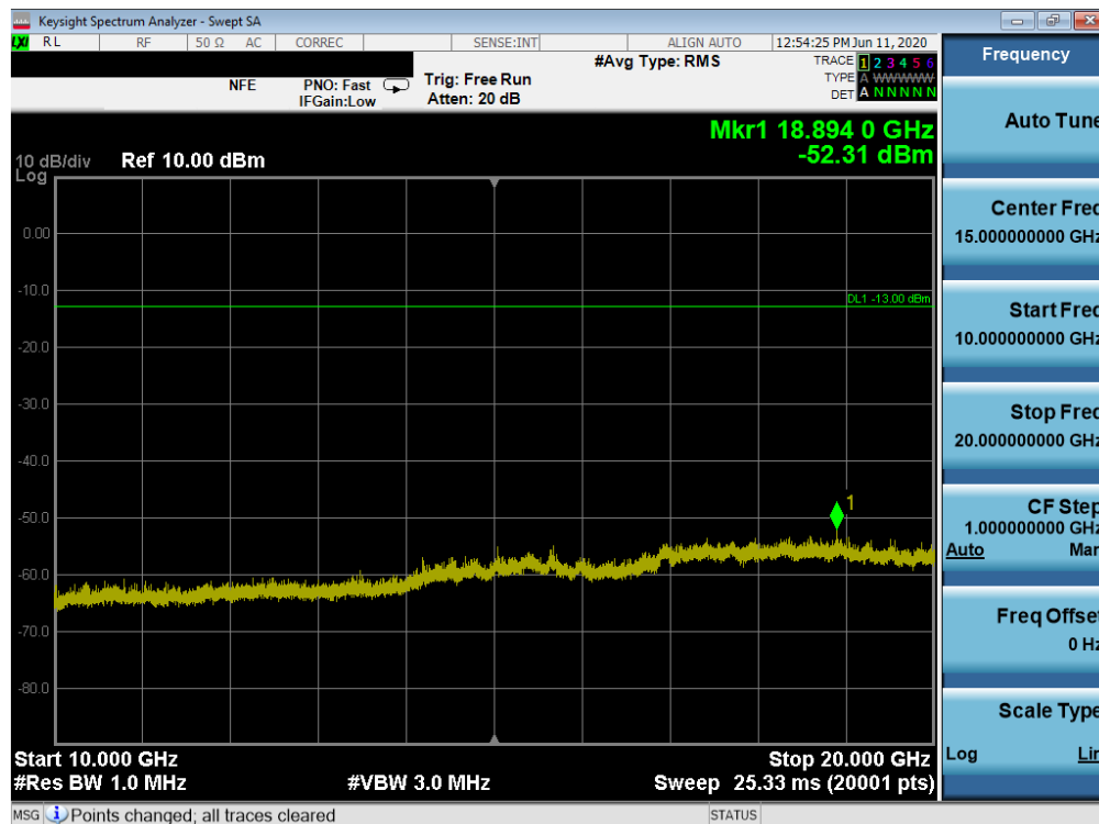
Plot 7-75. Conducted Spurious Plot (WCDMA Ch. 9400)
