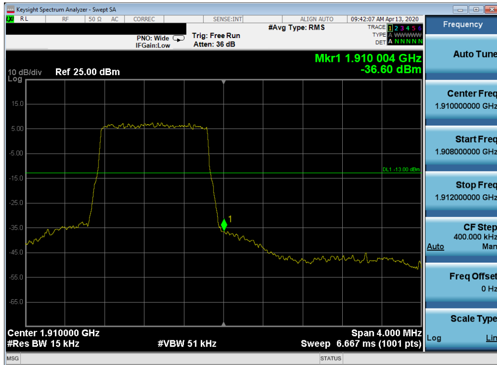
Plot 7-110. Upper Band Edge Plot (LTE Band 2 – 1.4MHz QPSK – Full RB Configuration)
