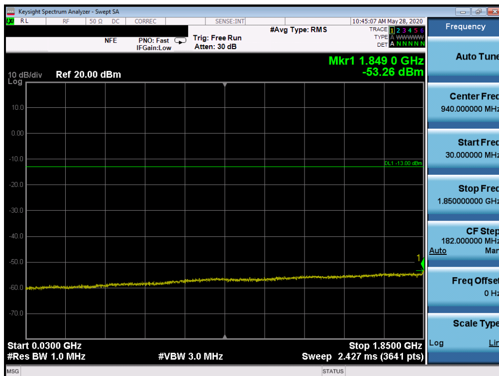
Plot 7-46. Conducted Spurious Plot (LTE Band 2 - 20MHz QPSK - RB Size 1, RB Offset 0 - Mid Channel)
