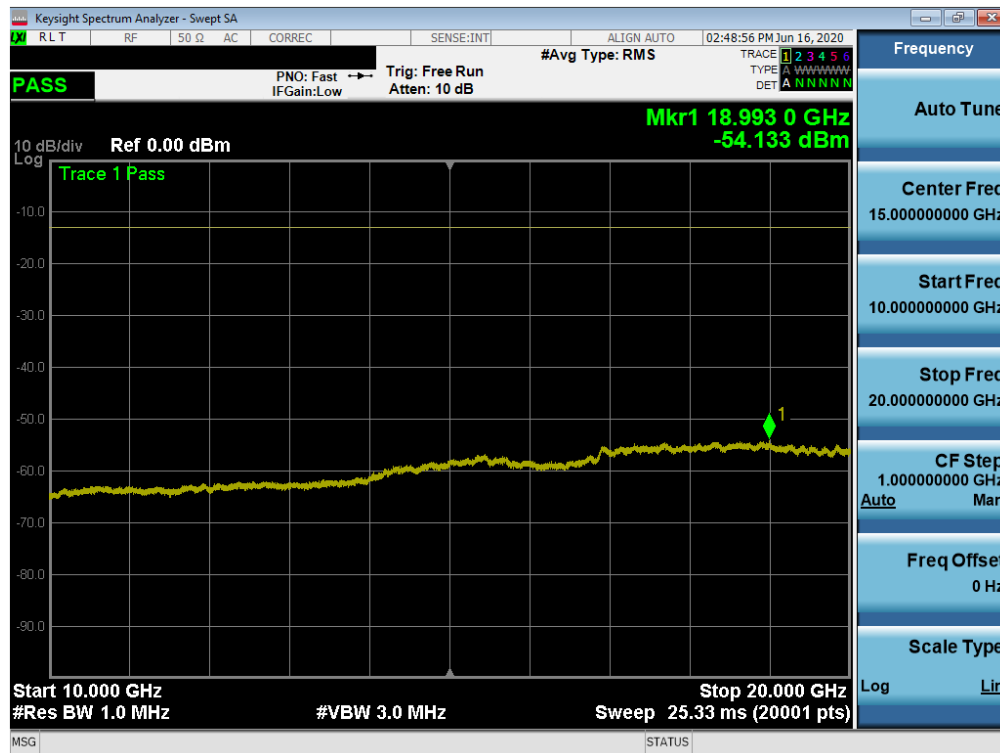
Plot 7-54. Conducted Spurious Plot (NR Band n2 - 20.0MHz - RB Size 1, RB Offset 0 - Low Channel)
