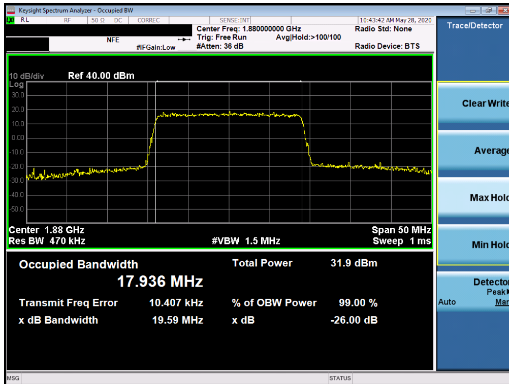
Plot 7-3. Occupied Bandwidth Plot (LTE Band 2 - 20MHz 64-QAM - Full RB Configuration)
