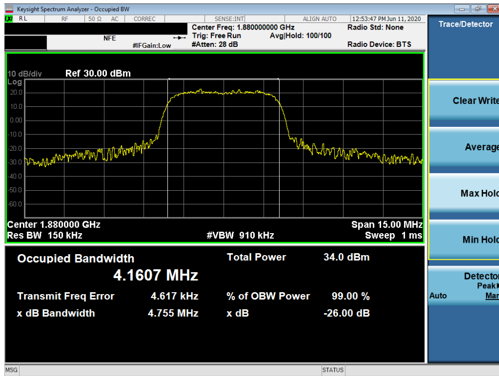
Plot 7-41. Occupied Bandwidth Plot (WCDMA, Ch. 9400)
