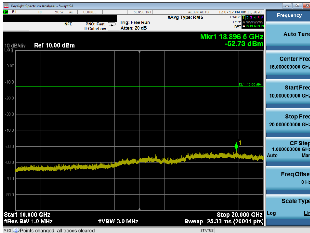
Plot 7-84. Conducted Spurious Plot (CDMA Ch. 600)
