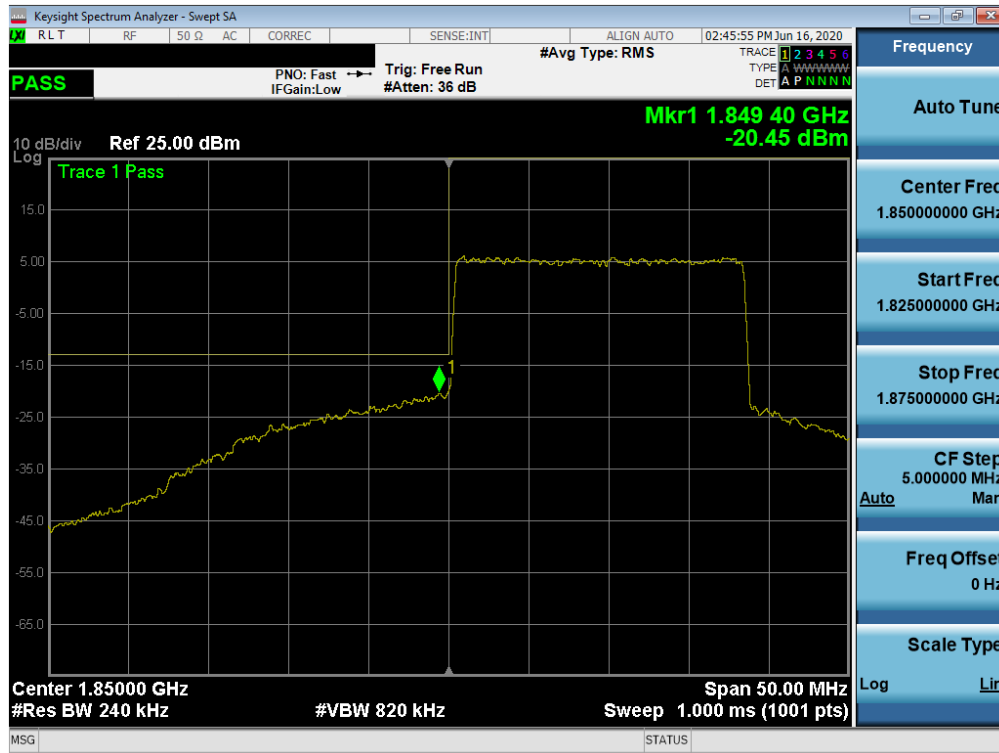
Plot 7-112. Lower Band Edge Plot (NR Band n2 – 20.0MHz - Full RB)
