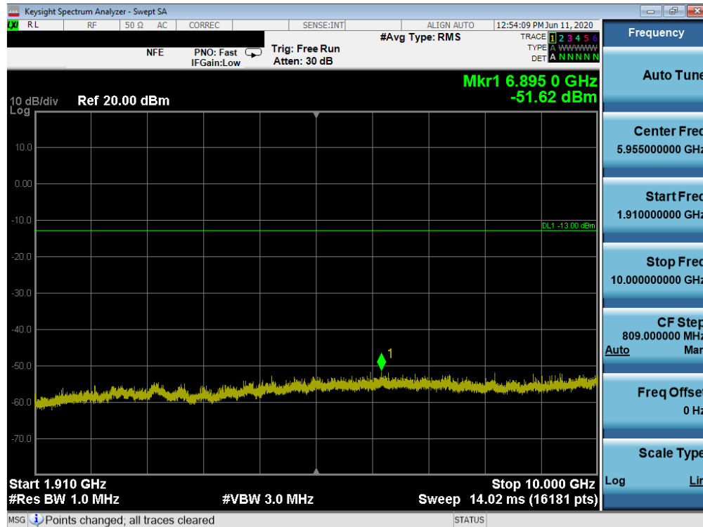
Plot 7-74. Conducted Spurious Plot (WCDMA Ch. 9400)
