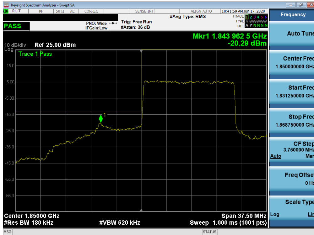
Plot 7-116. Lower Band Edge Plot (NR Band n2 – 15.0MHz - Full RB)
