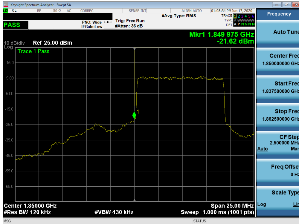
Plot 7-120. Lower Band Edge Plot (NR Band n2 – 10.0MHz - Full RB)
