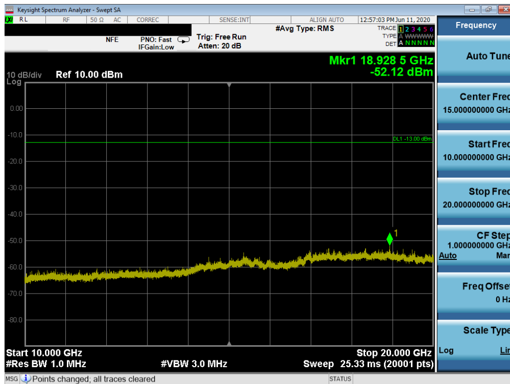
Plot 7-72. Conducted Spurious Plot (WCDMA Ch. 9262)
