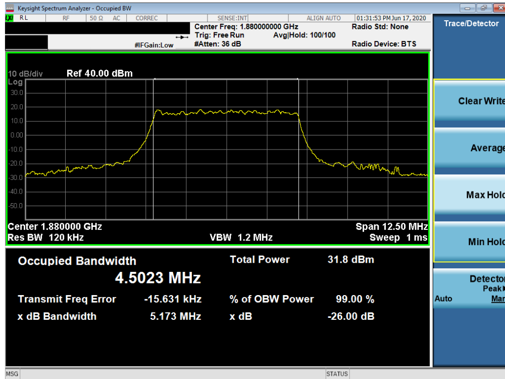
Plot 7-35. Occupied Bandwidth Plot (NR Band n2 - 5.0MHz CP-OFDM QPSK - Full RB)
