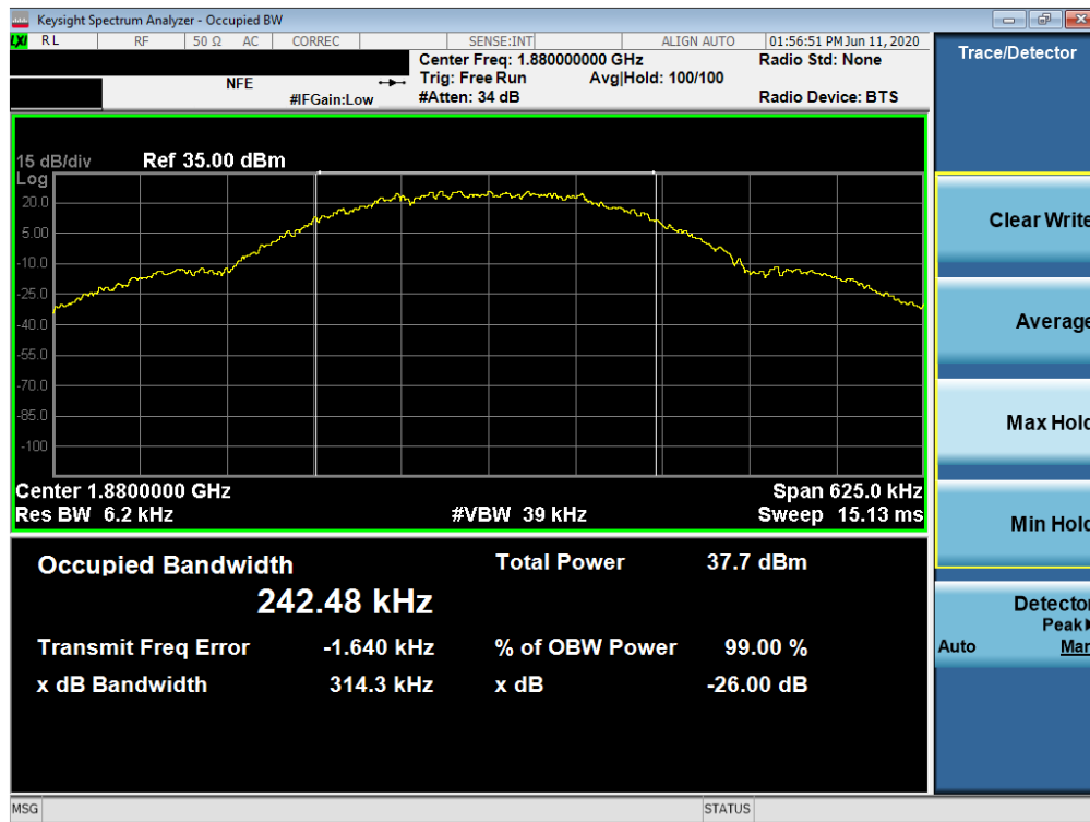
Plot 7-39. Occupied Bandwidth Plot (GPRS, Ch. 661)
