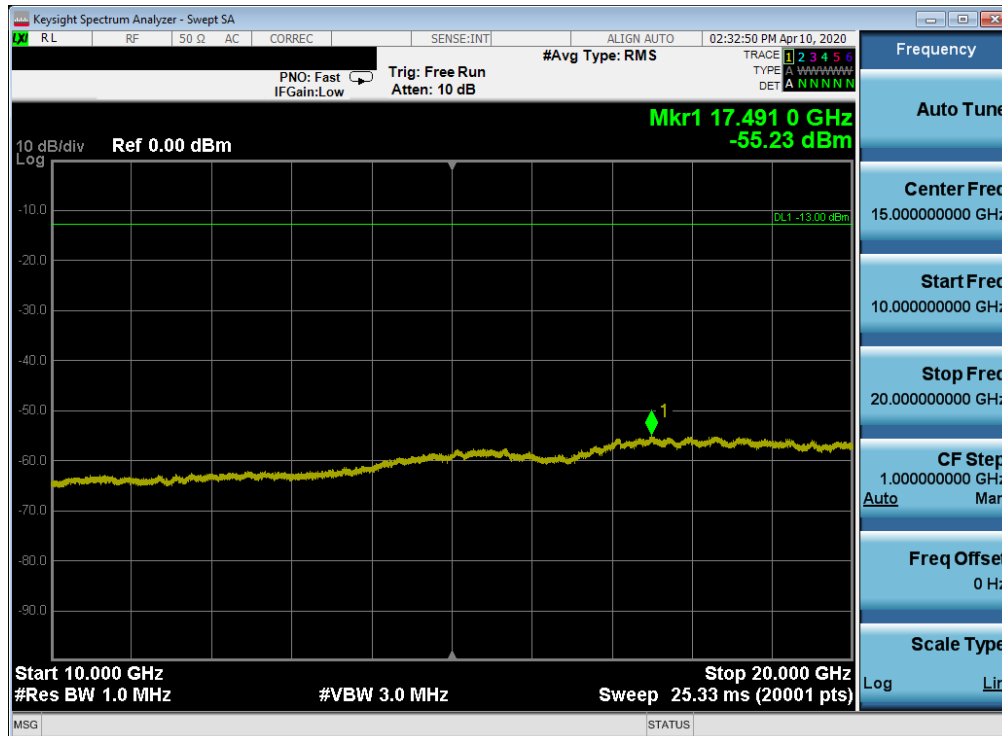
Plot 7-51. Conducted Spurious Plot (LTE Band 2 - 20MHz QPSK - RB Size 1, RB Offset 0 - High Channel)
