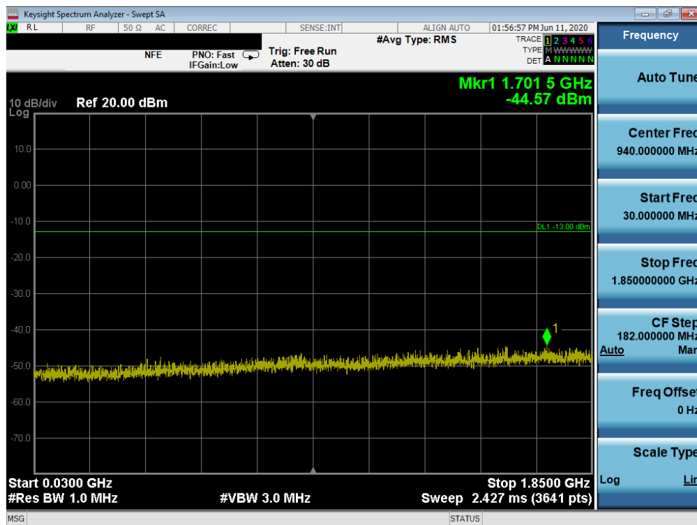
Plot 7-64. Conducted Spurious Plot (GPRS Ch. 661)
