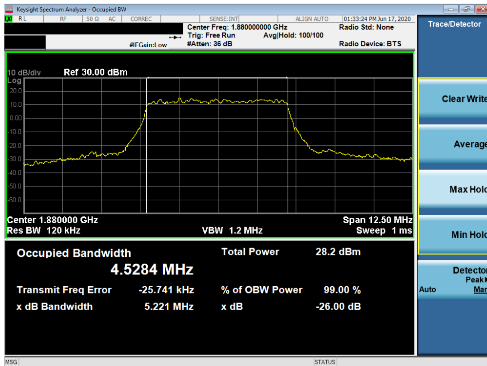
Plot 7-38. Occupied Bandwidth Plot (NR Band n2 - 5.0MHz CP-OFDM 256QAM - Full RB)
