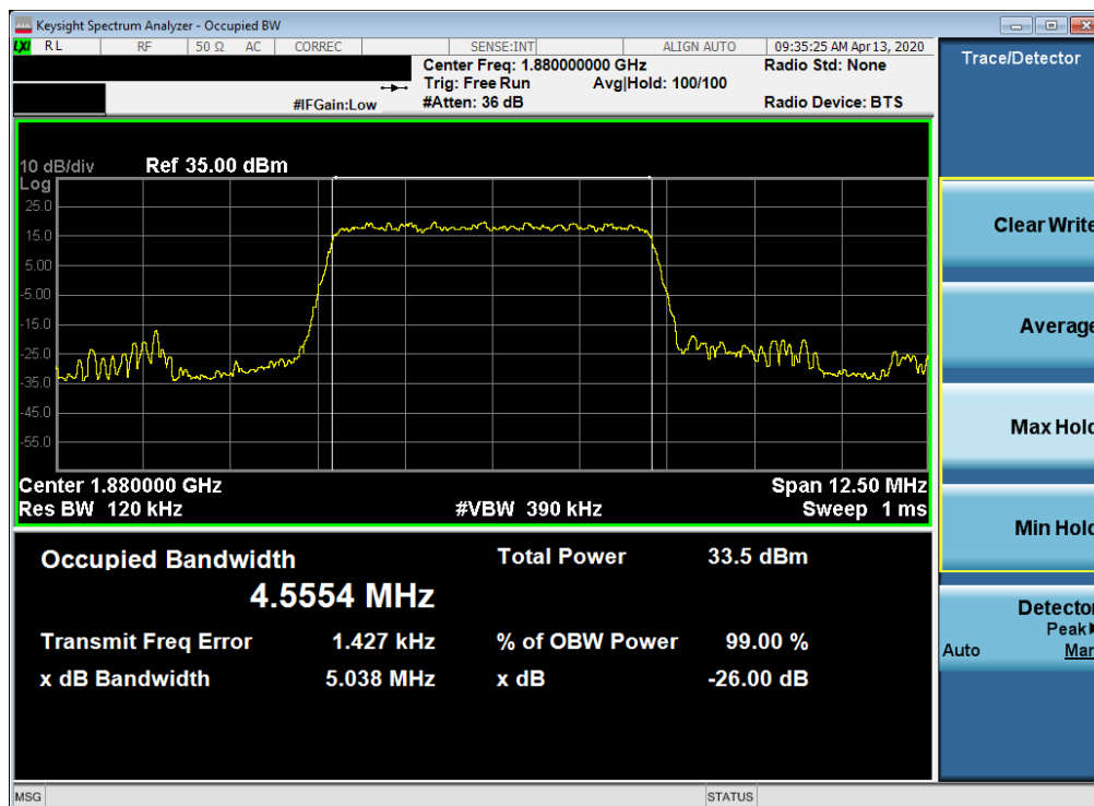
Plot 7-10. Occupied Bandwidth Plot (LTE Band 2 - 5MHz QPSK - Full RB Configuration)
