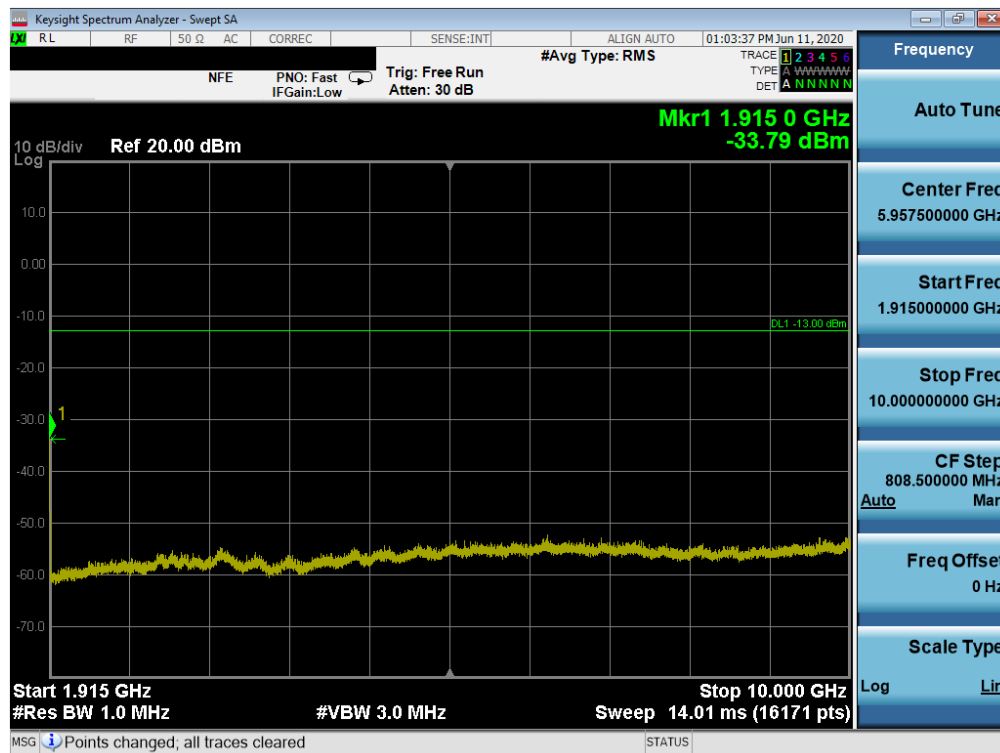
Plot 7-77. Conducted Spurious Plot (WCDMA Ch. 9538)
