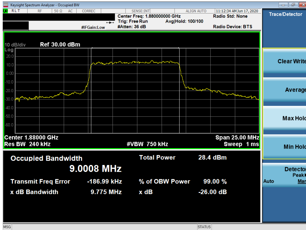
Plot 7-33. Occupied Bandwidth Plot (NR Band n2 - 10.0MHz CP-OFDM 256QAM - Full RB)
