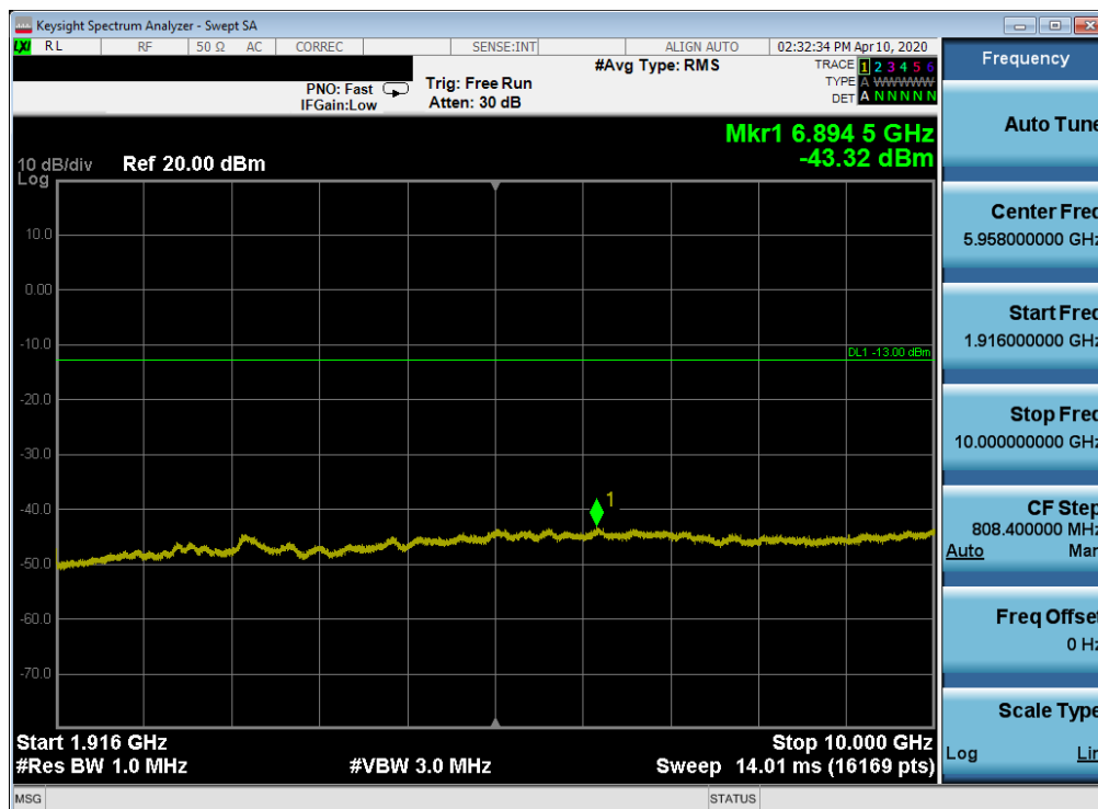
Plot 7-50. Conducted Spurious Plot (LTE Band 2 - 20MHz QPSK - RB Size 1, RB Offset 0 - High Channel)
