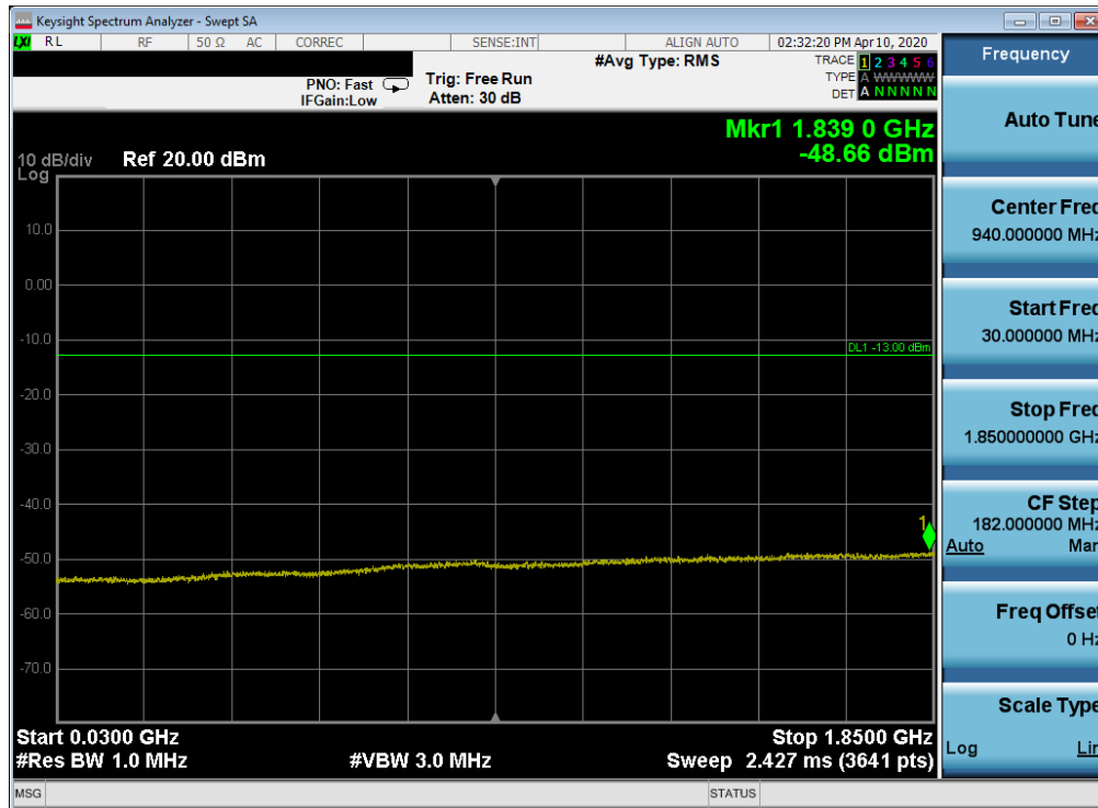
Plot 7-49. Conducted Spurious Plot (LTE Band 2 - 20MHz QPSK - RB Size 1, RB Offset 0 - High Channel)
