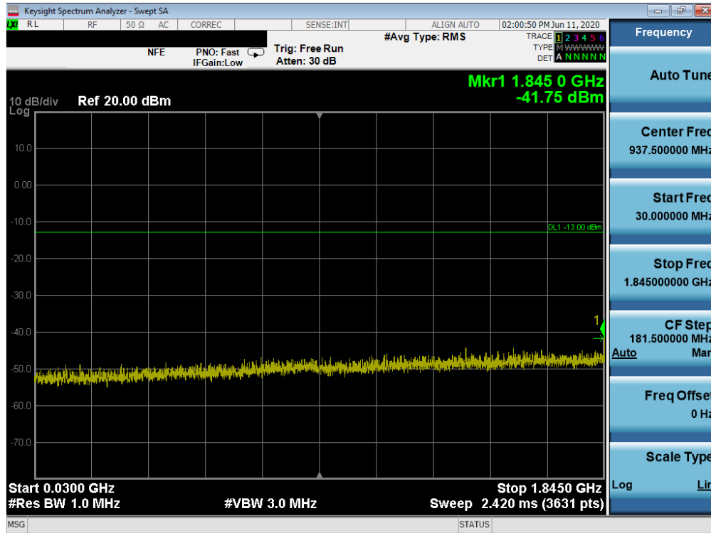
Plot 7-61. Conducted Spurious Plot (GPRS Ch. 512)
