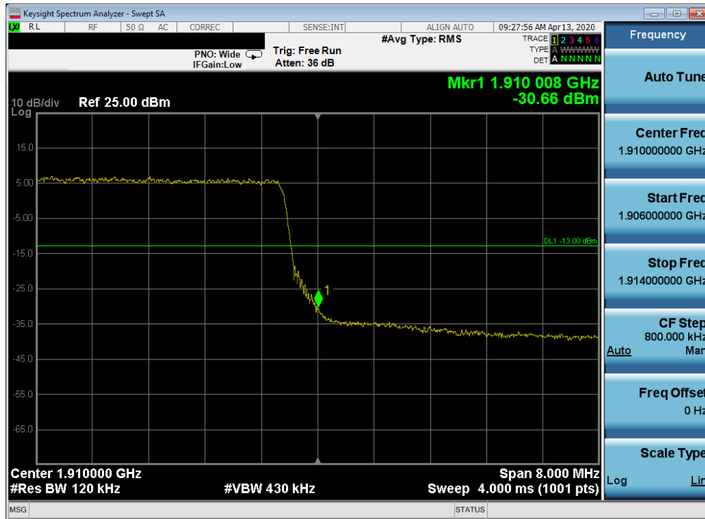
Plot 7-98. Upper Band Edge Plot (LTE Band 2 - 10MHz QPSK – Full RB Configuration)
