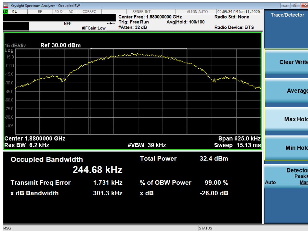
Plot 7-40. Occupied Bandwidth Plot (EDGE, Ch. 661)
