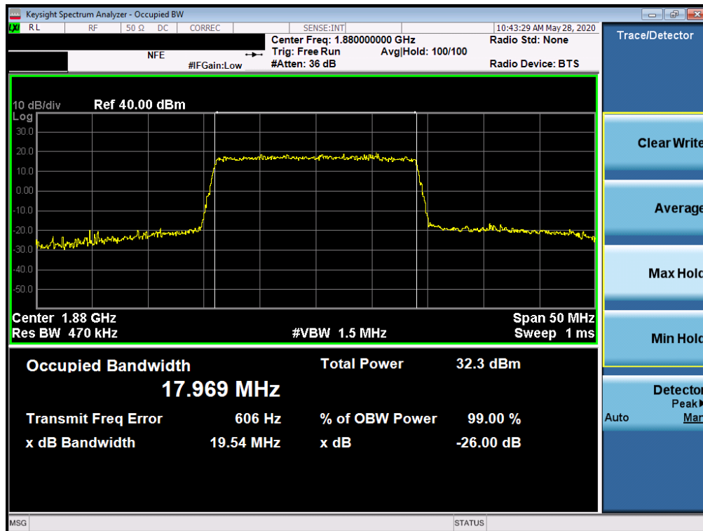
Plot 7-2. Occupied Bandwidth Plot (LTE Band 2 - 20MHz 16-QAM - Full RB Configuration)
