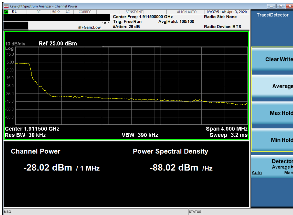
Plot 7-103. Extended Upper Band Edge Plot (LTE Band 2 - 5MHz QPSK – Full RB Configuration)
