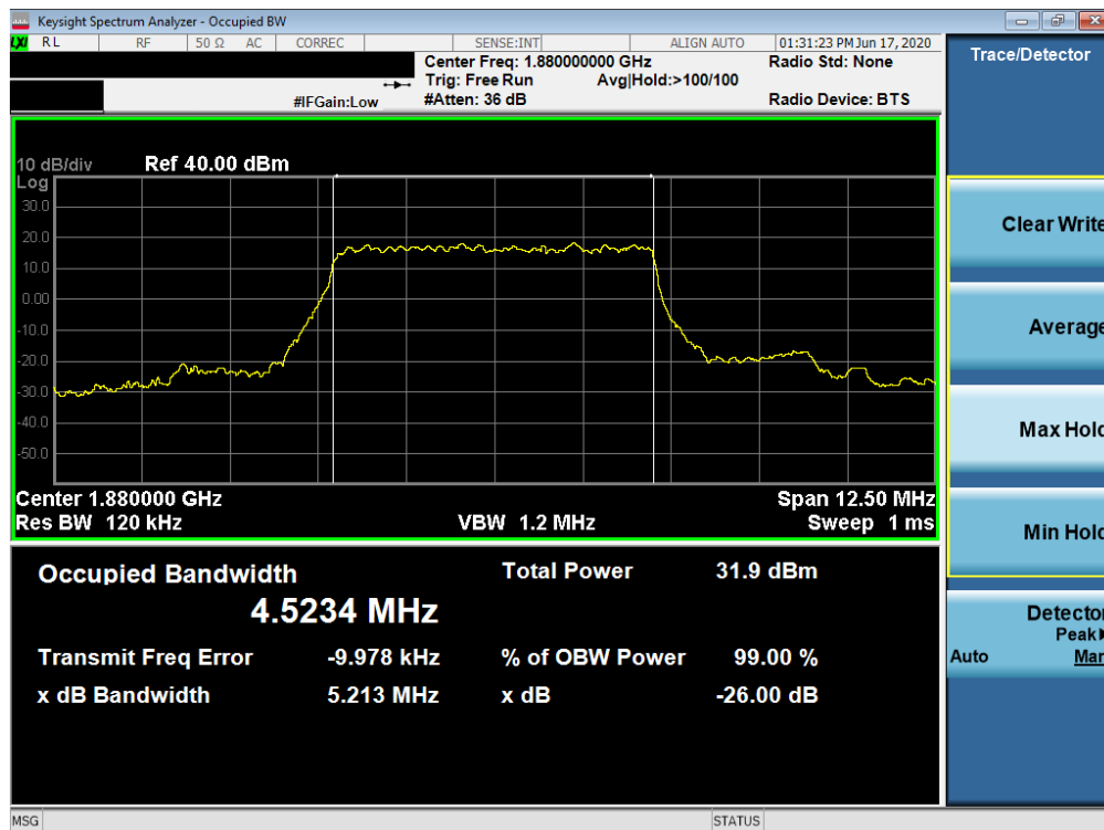
Plot 7-34. Occupied Bandwidth Plot (NR Band n2 - 5.0MHz DFT-s-OFDM BPSK - Full RB)
