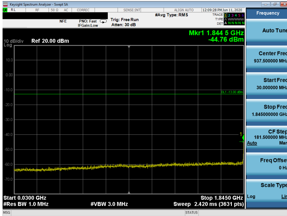
Plot 7-79. Conducted Spurious Plot (CDMA Ch. 25)
