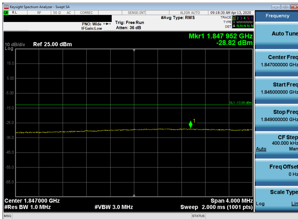
Plot 7-93. Extended Lower Band Edge Plot (LTE Band 2 - 15MHz QPSK – Full RB Configuration)
