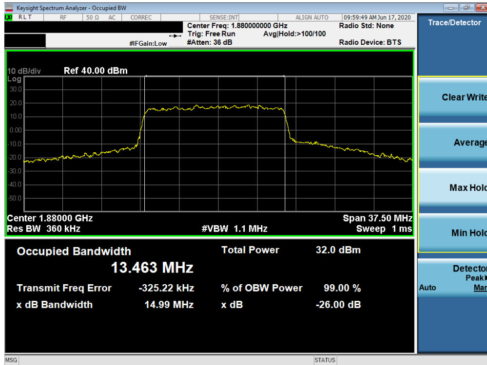
Plot 7-25. Occupied Bandwidth Plot (NR Band n2 - 15.0MHz CP-OFDM QPSK - Full RB)
