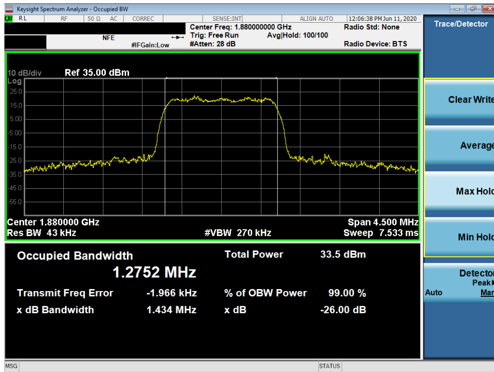
Plot 7-42. Occupied Bandwidth Plot (CDMA, Ch. 600)
