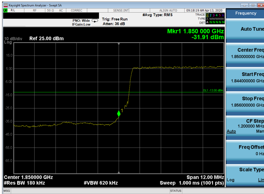
Plot 7-92. Lower Band Edge Plot (LTE Band 2 - 15MHz QPSK – Full RB Configuration)
