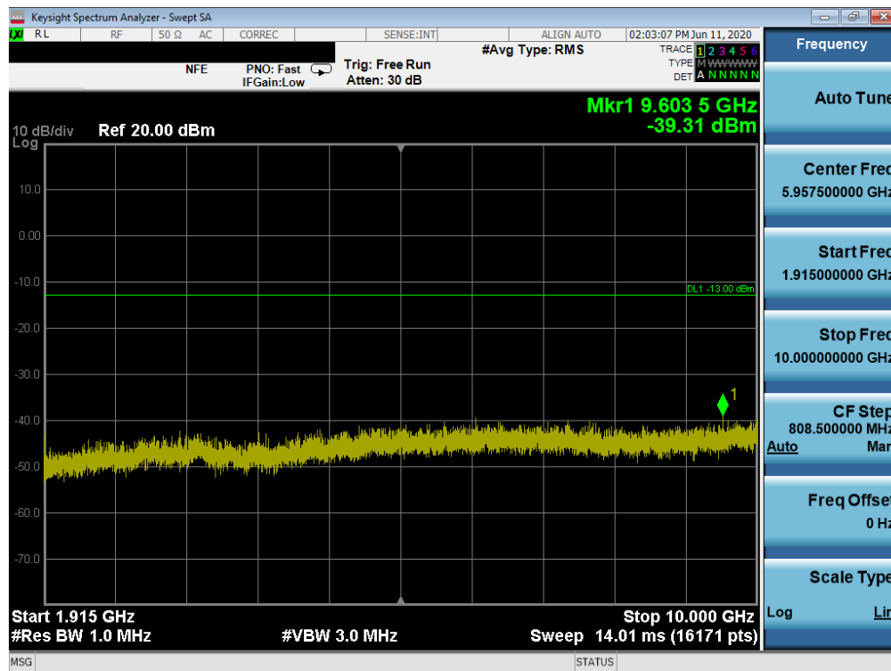
Plot 7-68. Conducted Spurious Plot (GPRS Ch. 810)
