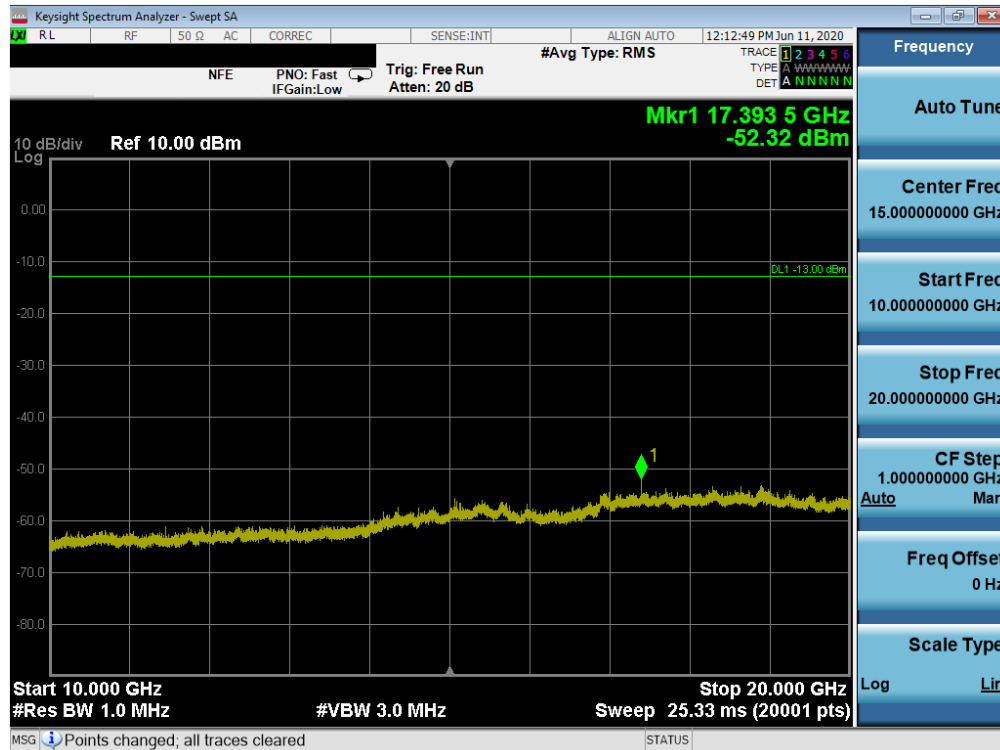
Plot 7-87. Conducted Spurious Plot (CDMA Ch. 1175)
