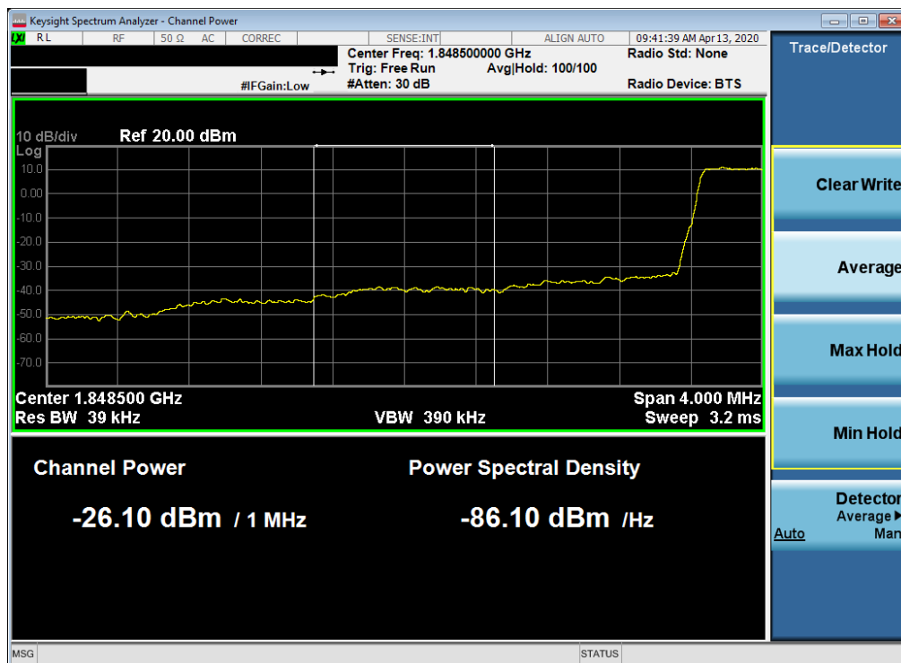
Plot 7-109. Extended Lower Band Edge Plot (LTE Band 2 – 1.4MHz QPSK – Full RB Configuration)
