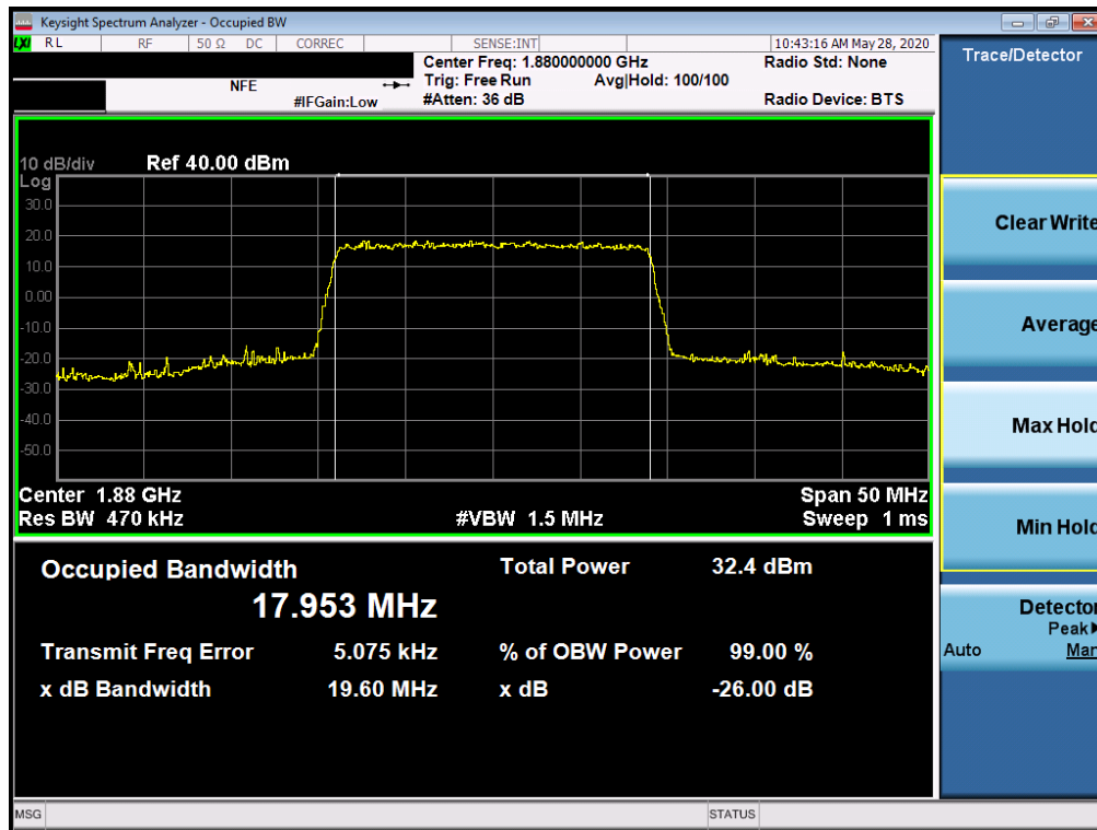
Plot 7-1. Occupied Bandwidth Plot (LTE Band 2 - 20MHz QPSK - Full RB Configuration)
