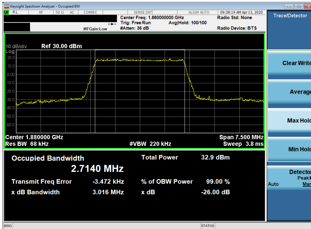
Plot 7-13. Occupied Bandwidth Plot (LTE Band 2 - 3MHz QPSK - Full RB Configuration)
