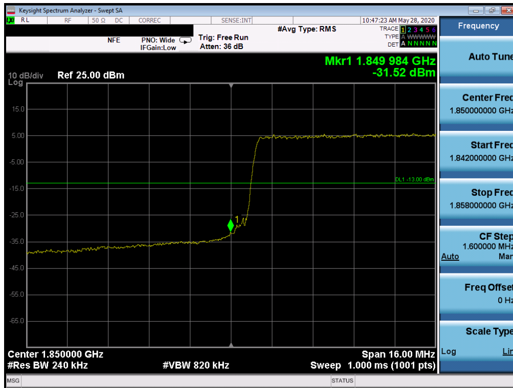
Plot 7-88. Lower Band Edge Plot (LTE Band 2 - 20MHz QPSK - Full RB Configuration)
