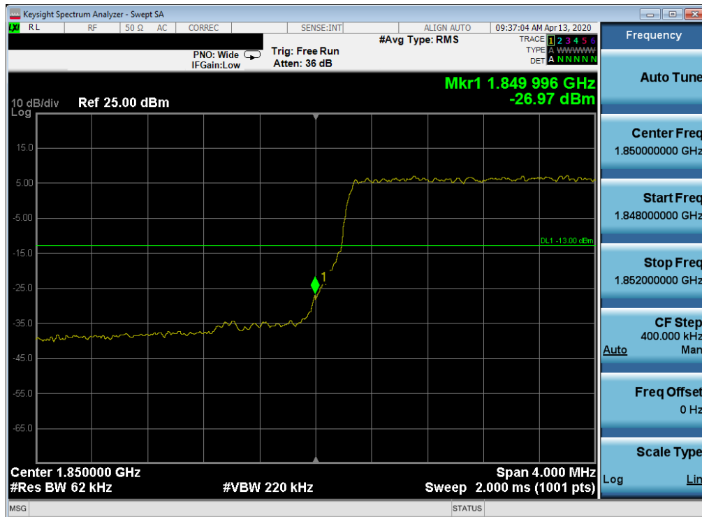
Plot 7-100. Lower Band Edge Plot (LTE Band 2 - 5MHz QPSK – Full RB Configuration)
