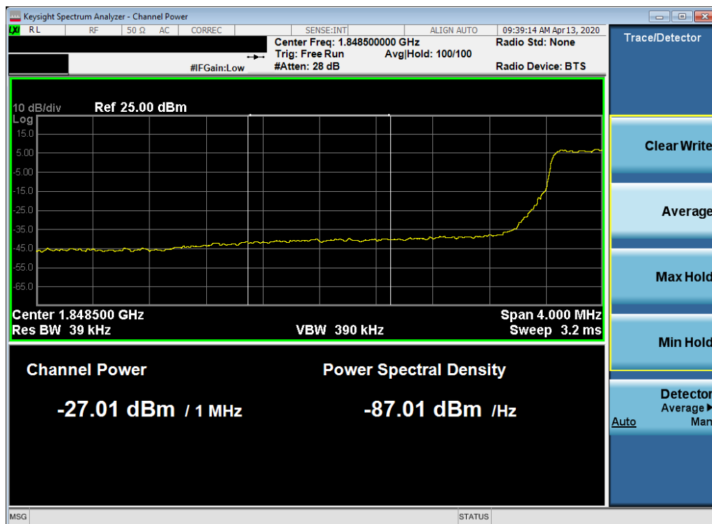
Plot 7-105. Extended Lower Band Edge Plot (LTE Band 2 - 3MHz QPSK – Full RB Configuration)
