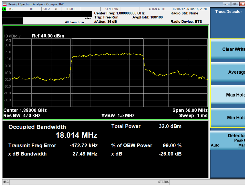
Plot 7-19. Occupied Bandwidth Plot (NR Band n2 - 20.0MHz DFT-s-OFDM BPSK - Full RB)
