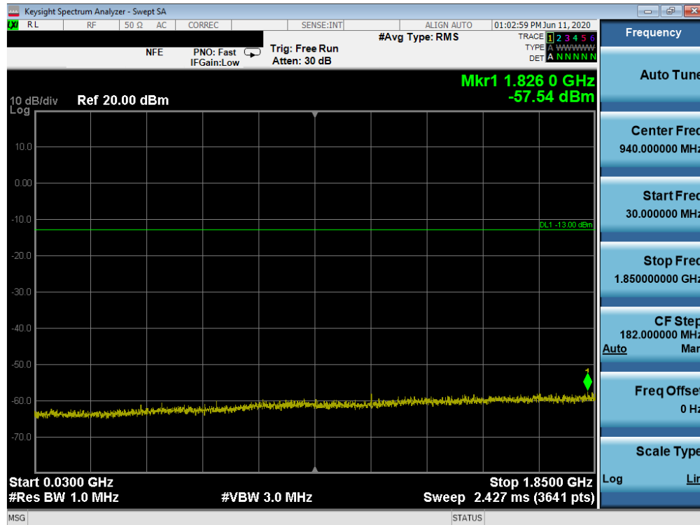
Plot 7-76. Conducted Spurious Plot (WCDMA Ch. 9538)
