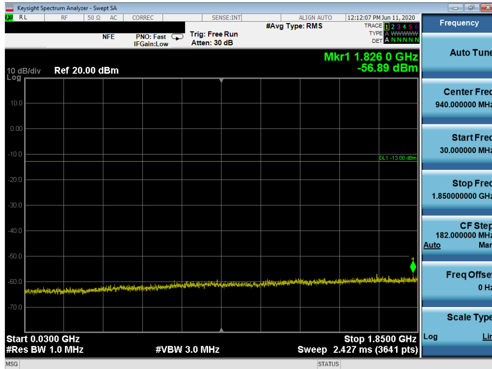
Plot 7-85. Conducted Spurious Plot (CDMA Ch. 1175)
