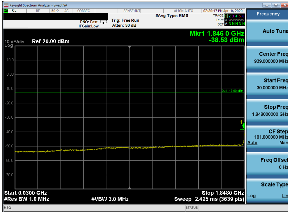
Plot 7-43. Conducted Spurious Plot (LTE Band 2 - 20MHz QPSK - RB Size 1, RB Offset 0 - Low Channel)
