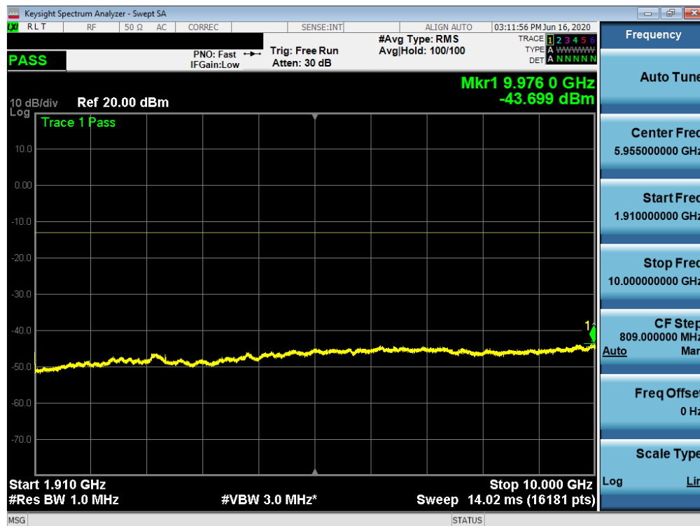
Plot 7-59. Conducted Spurious Plot (NR Band n2 - 20.0MHz - RB Size 1, RB Offset 0 - High Channel)
