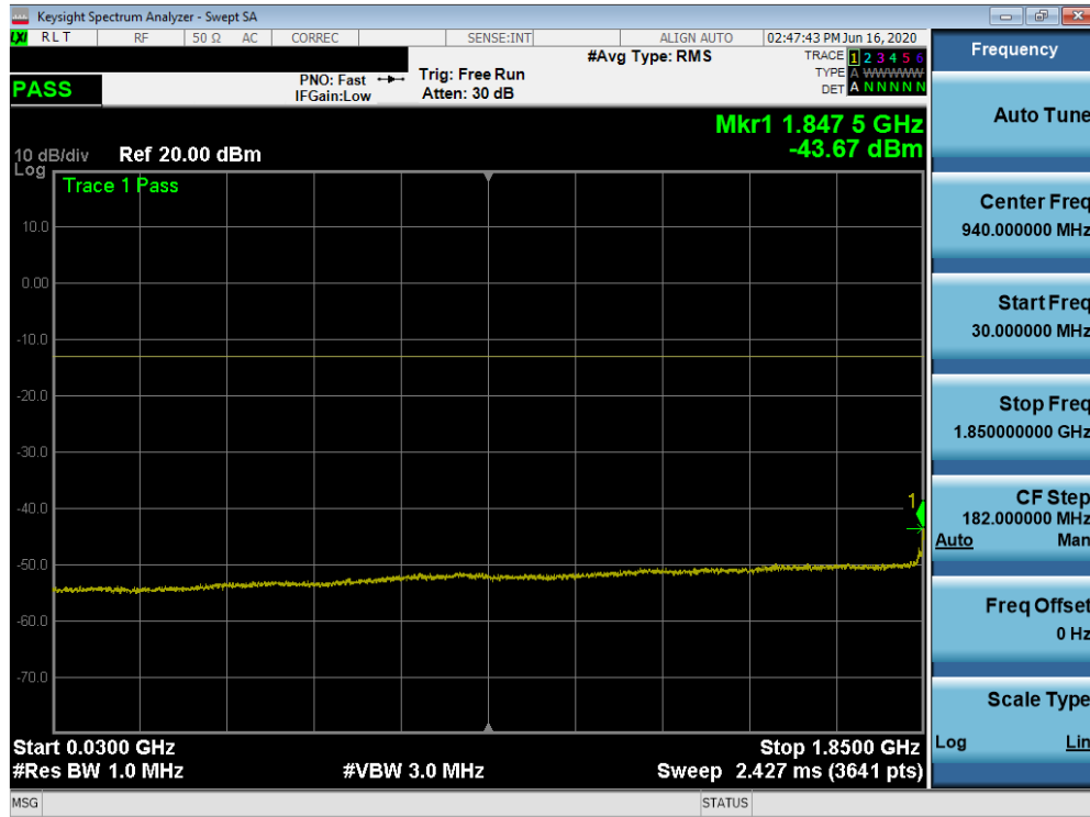
Plot 7-52. Conducted Spurious Plot (NR Band n2 -20.0MHz - RB Size 1, RB Offset 0 - Low Channel)
