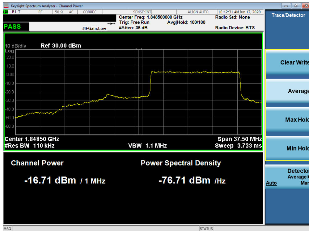
Plot 7-117. Lower Extended Band Edge Plot (NR Band n2 – 15.0MHz - Full RB)
