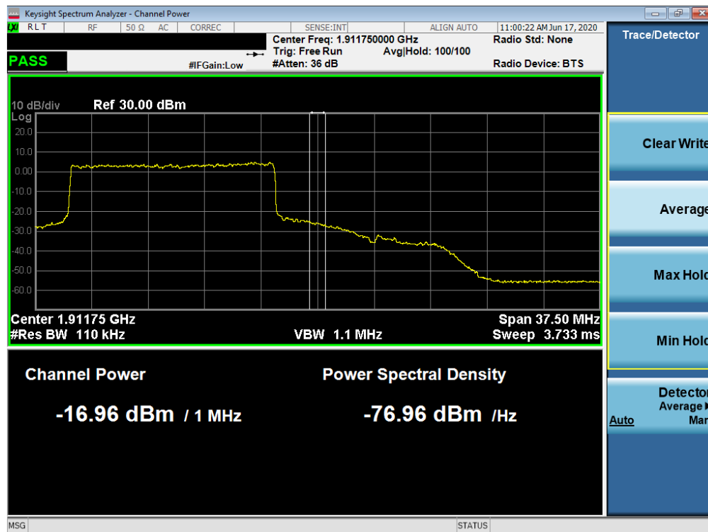
Plot 7-119. Upper Extended Band Edge Plot (NR Band n2 – 15.0MHz - Full RB)
