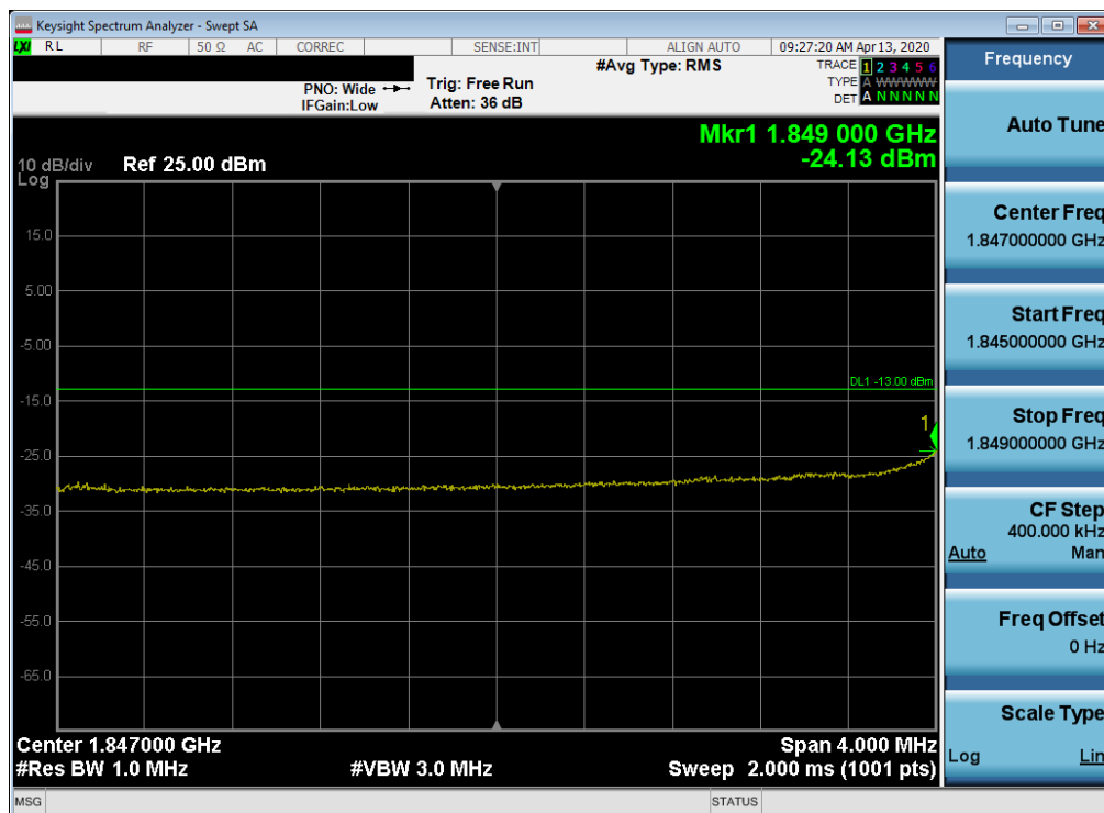
Plot 7-97. Extended Lower Band Edge Plot (LTE Band 2 - 10MHz QPSK – Full RB Configuration)
