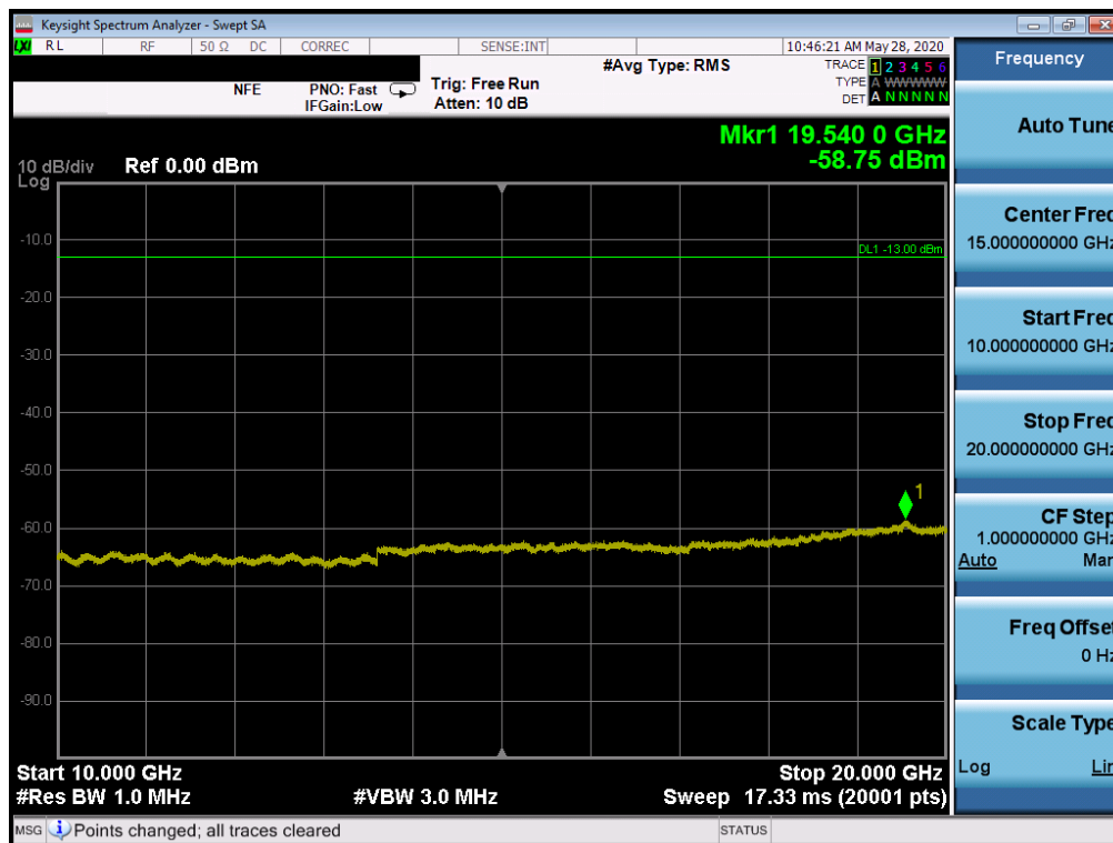
Plot 7-48. Conducted Spurious Plot (LTE Band 2 - 20MHz QPSK - RB Size 1, RB Offset 0 - Mid Channel)
