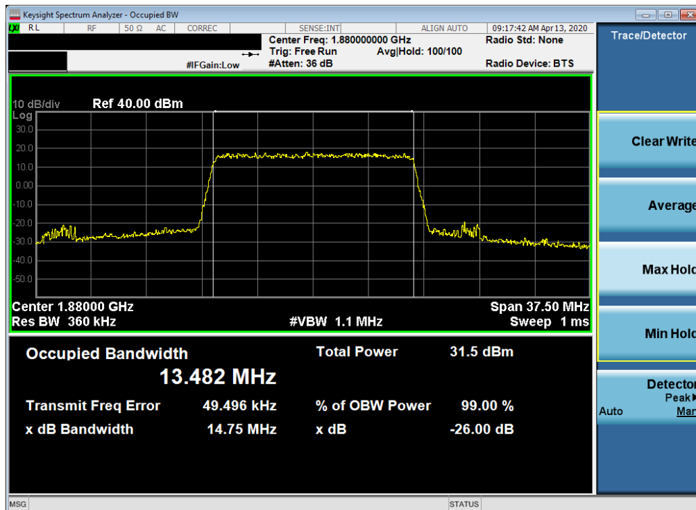
Plot 7-6. Occupied Bandwidth Plot (LTE Band 2 - 15MHz 64-QAM - Full RB Configuration)
