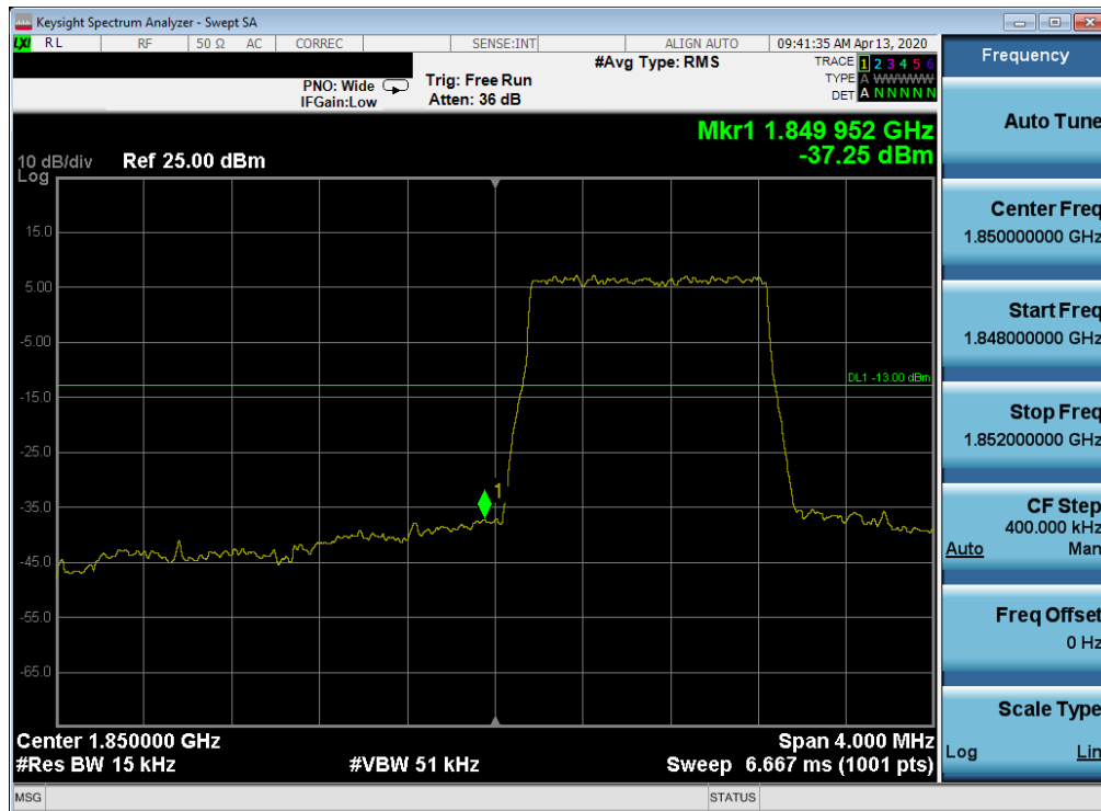
Plot 7-108. Lower Band Edge Plot (LTE Band 2 – 1.4MHz QPSK – Full RB Configuration)
