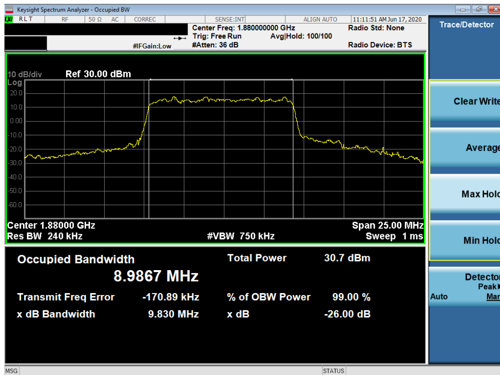
Plot 7-32. Occupied Bandwidth Plot (NR Band n2 - 10.0MHz CP-OFDM 64QAM - Full RB)
