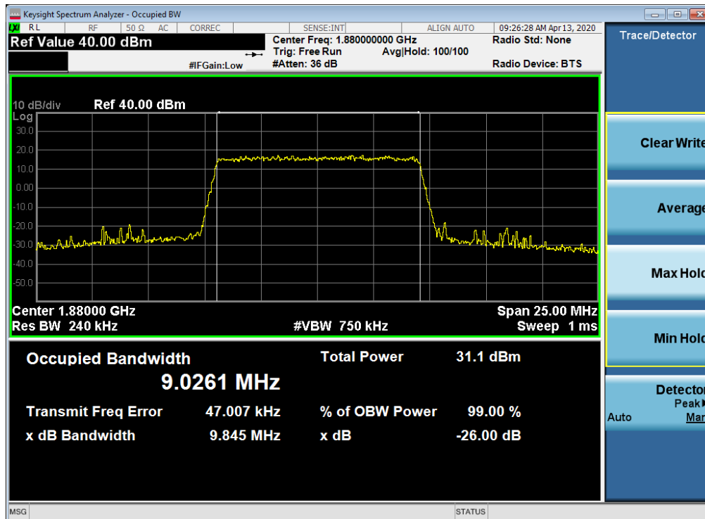
Plot 7-9. Occupied Bandwidth Plot (LTE Band 2 - 10MHz 64-QAM - Full RB Configuration)
