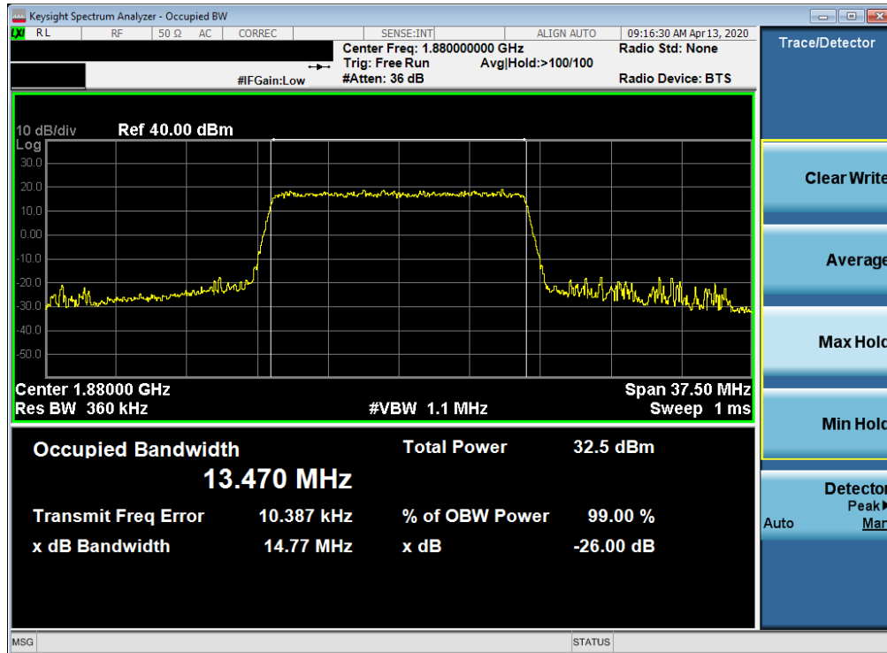
Plot 7-5. Occupied Bandwidth Plot (LTE Band 2 - 15MHz 16-QAM - Full RB Configuration)
