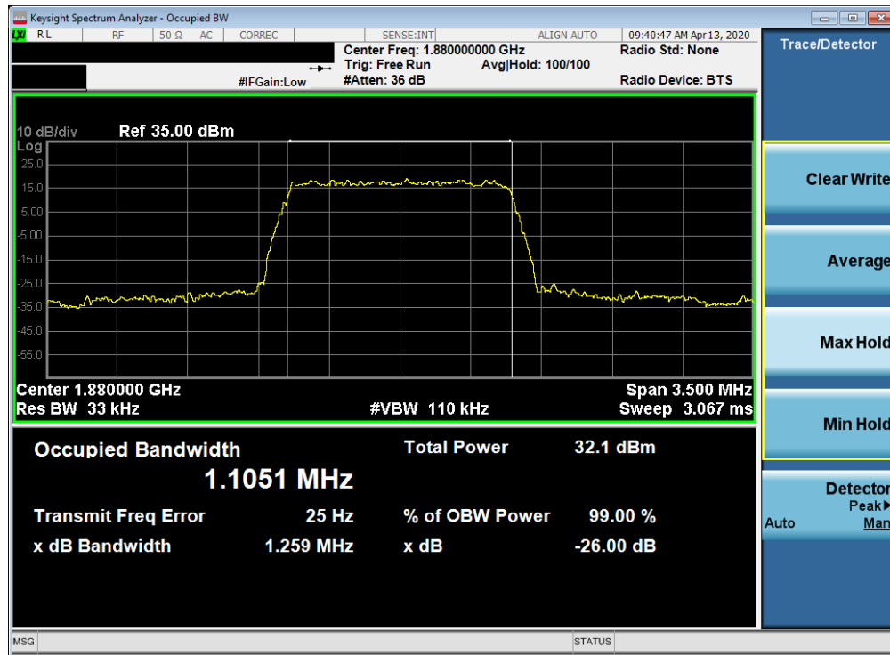
Plot 7-17. Occupied Bandwidth Plot (LTE Band 2 - 1.4MHz 16-QAM - Full RB Configuration)
