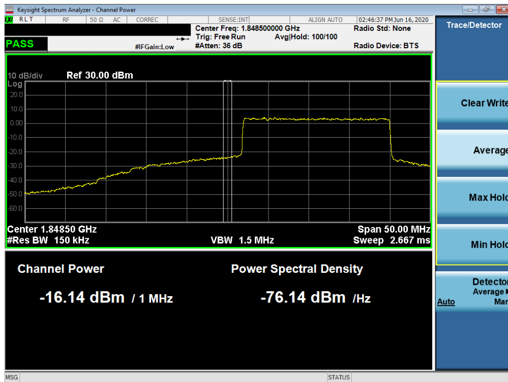
Plot 7-113. Lower Extended Band Edge Plot (NR Band n2 – 20.0MHz - Full RB)
