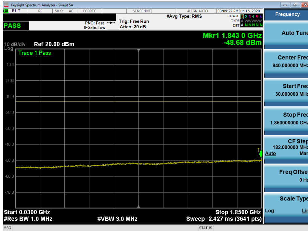
Plot 7-58. Conducted Spurious Plot (NR Band n2 - 20.0MHz - RB Size 1, RB Offset 0 - High Channel)
