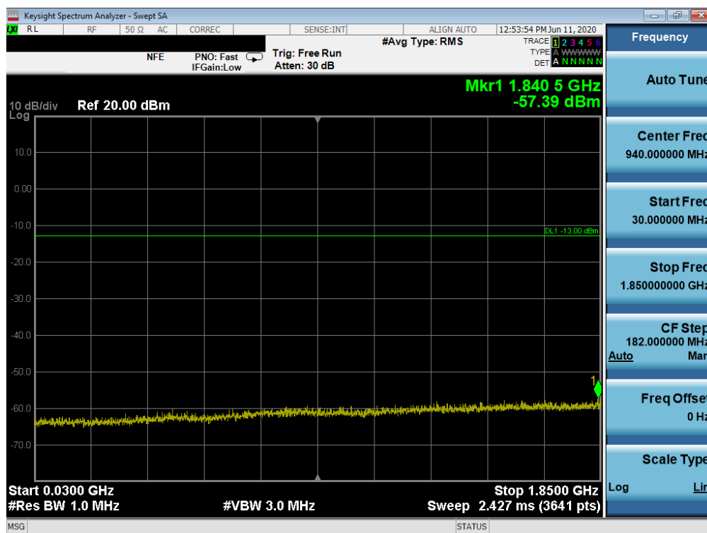
Plot 7-73. Conducted Spurious Plot (WCDMA Ch. 9400)
