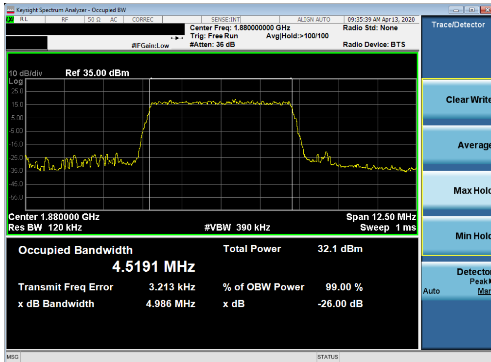
Plot 7-11. Occupied Bandwidth Plot (LTE Band 2 - 5MHz 16-QAM - Full RB Configuration)
