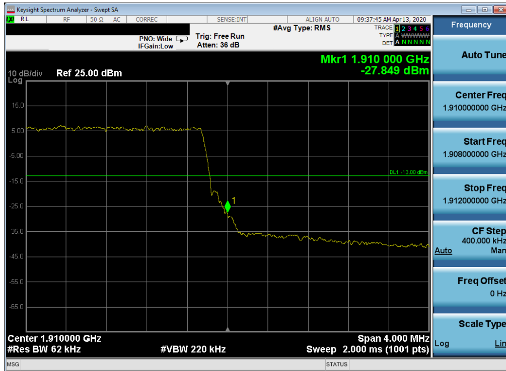
Plot 7-102. Upper Band Edge Plot (LTE Band 2 - 5MHz QPSK – Full RB Configuration)
