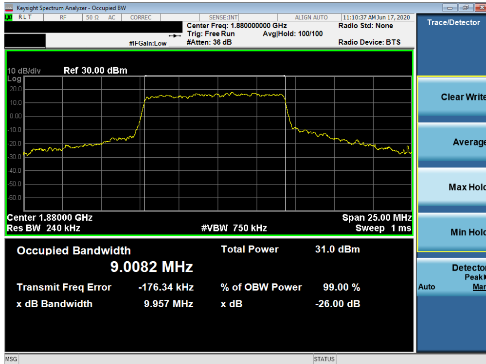
Plot 7-31. Occupied Bandwidth Plot (NR Band n2 - 10.0MHz CP-OFDM 16QAM - Full RB)
