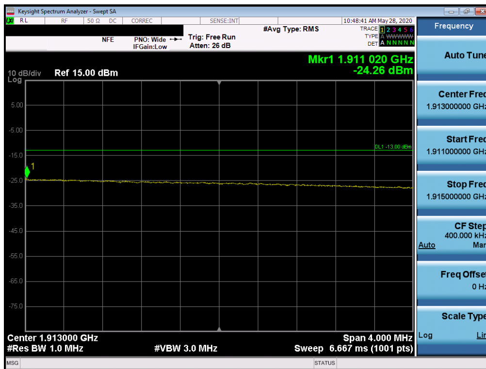
Plot 7-91. Extended Upper Band Edge Plot (LTE Band 2 - 20MHz QPSK – Full RB Configuration)
