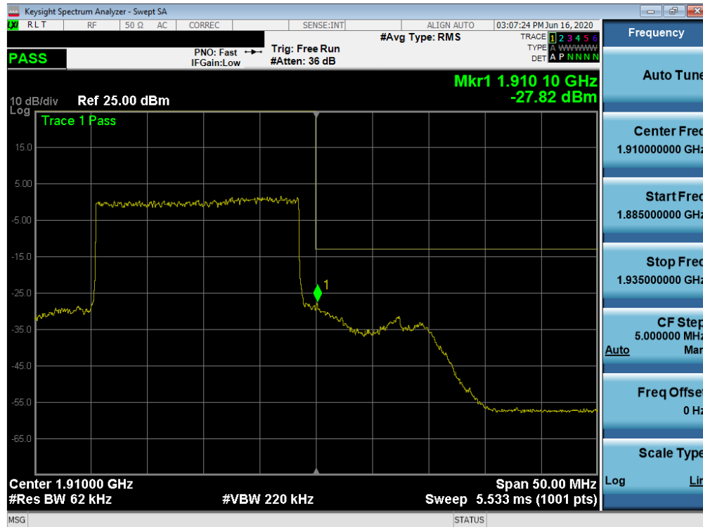
Plot 7-114. Upper Band Edge Plot (NR Band n2 – 20.0MHz - Full RB)
