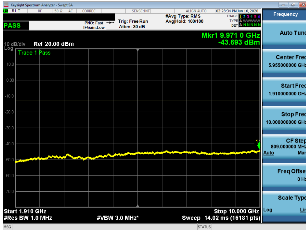
Plot 7-56. Conducted Spurious Plot (NR Band n2 - 20.0MHz - RB Size 1, RB Offset 0 - Mid Channel)
