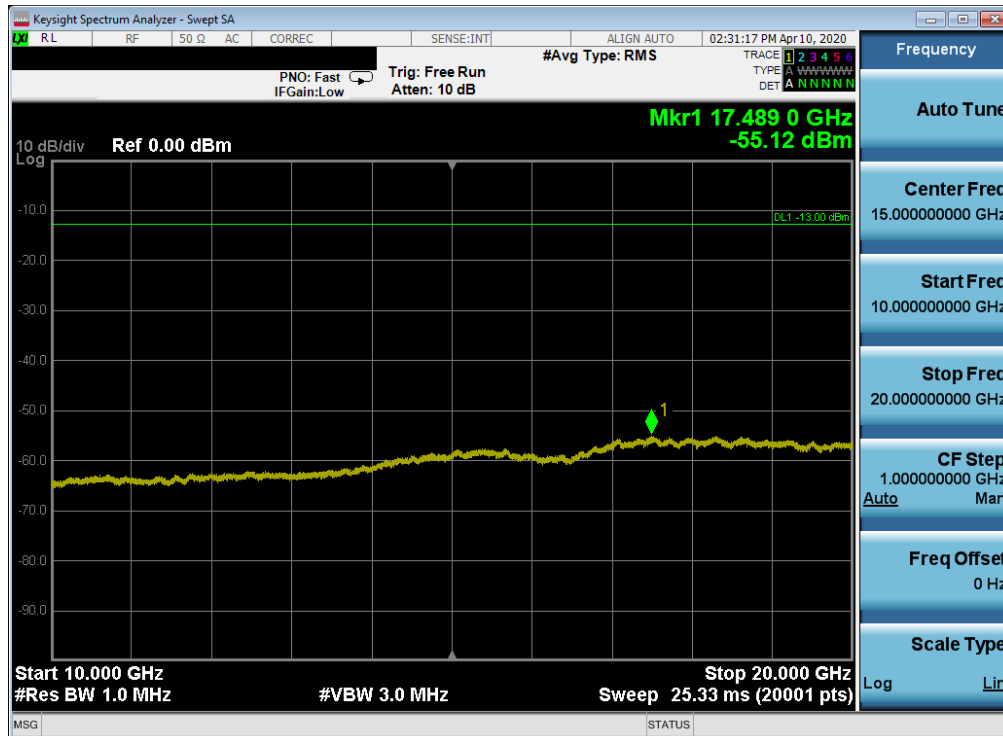
Plot 7-45. Conducted Spurious Plot (LTE Band 2 - 20MHz QPSK - RB Size 1, RB Offset 0 - Low Channel)
