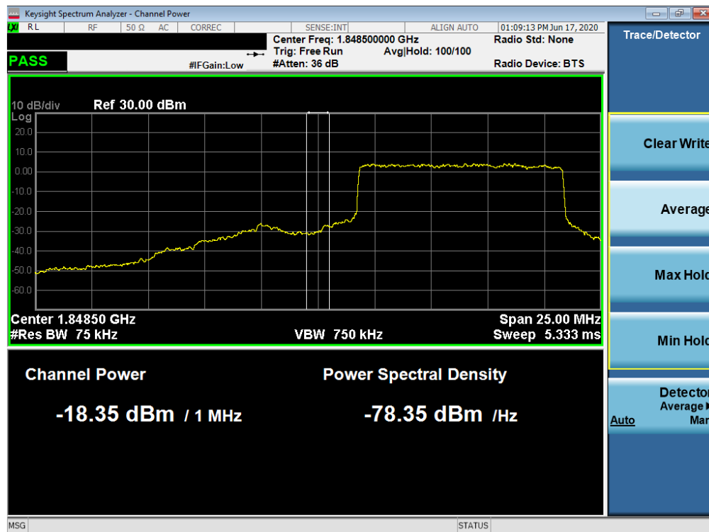
Plot 7-121. Lower Extended Band Edge Plot (NR Band n2 – 10.0MHz - Full RB)
