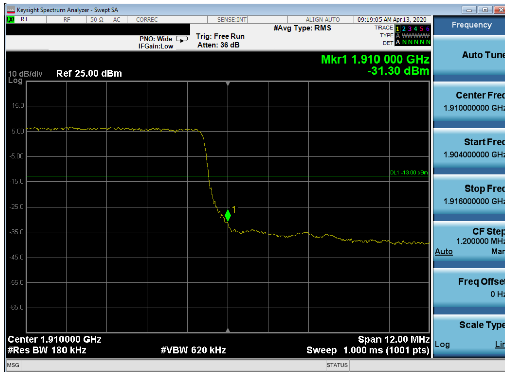
Plot 7-94. Upper Band Edge Plot (LTE Band 2 - 15MHz QPSK – Full RB Configuration)
