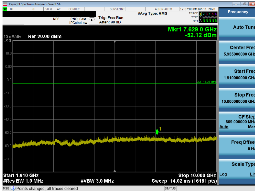
Plot 7-83. Conducted Spurious Plot (CDMA Ch. 600)
