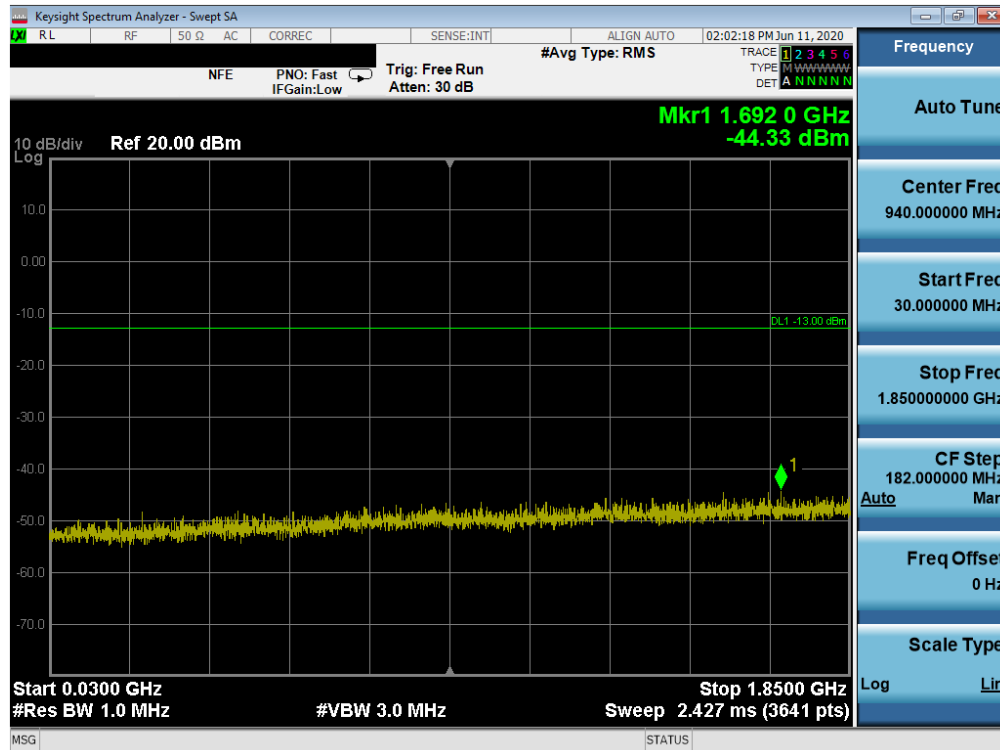
Plot 7-67. Conducted Spurious Plot (GPRS Ch. 810)
