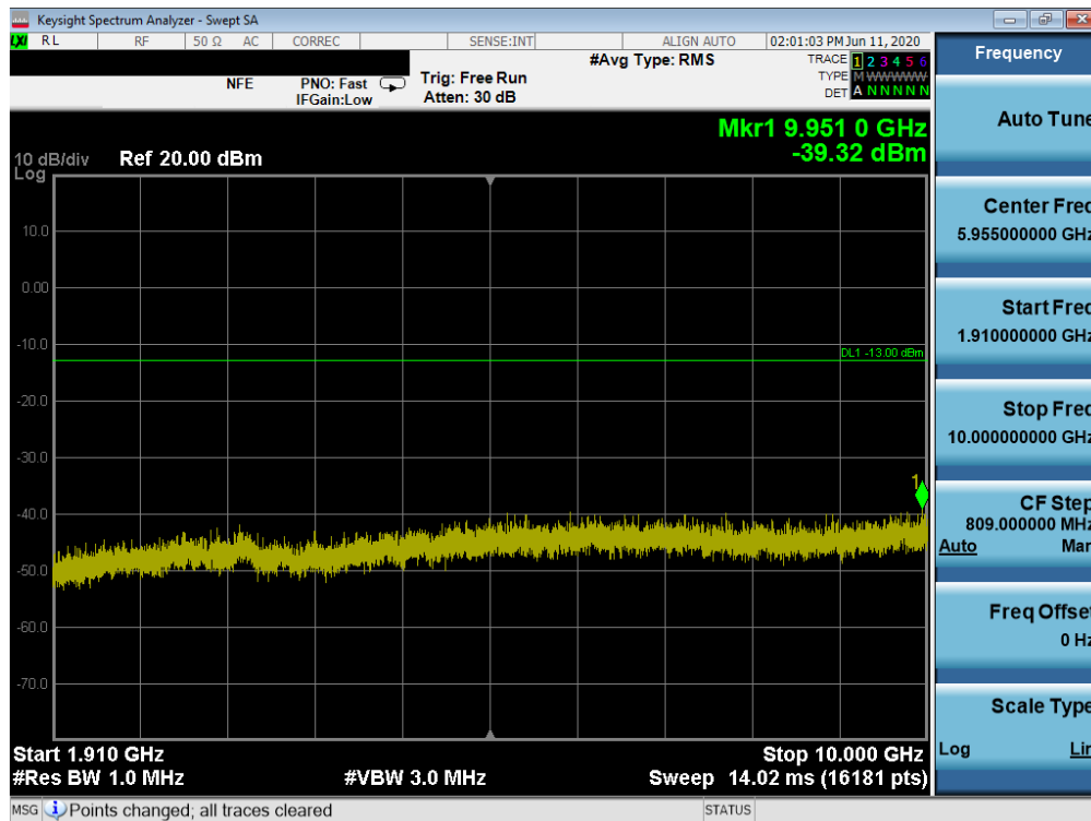
Plot 7-62. Conducted Spurious Plot (GPRS Ch. 512)
