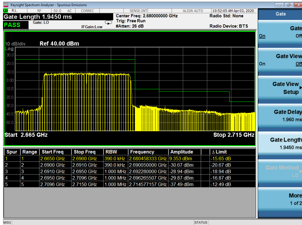
Plot 7-467. Upper ACP Plot (Band 41 - 20MHz QPSK - Full RB Configuration)
