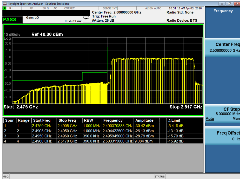
Plot 7-466. Lower ACP Plot (Band 41 - 20MHz QPSK - Full RB Configuration)
