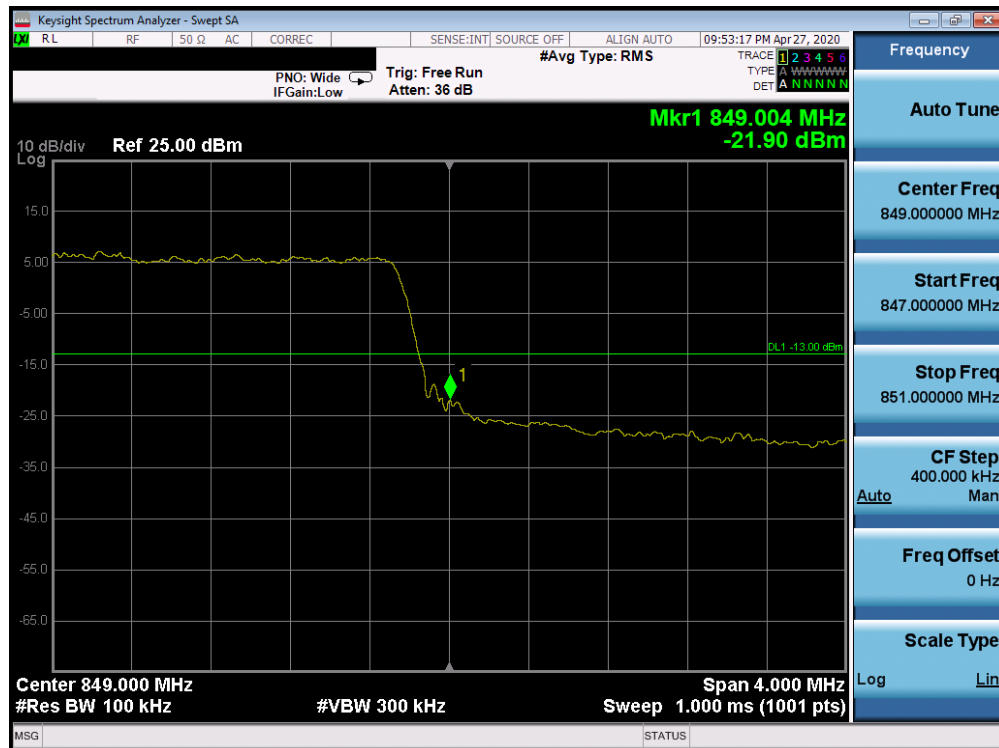
Plot 7-485. Upper 5G sub6 Band Edge Plot (5G sub6 n5 - 5.0MHz QPSK - Full RB Configuration)
