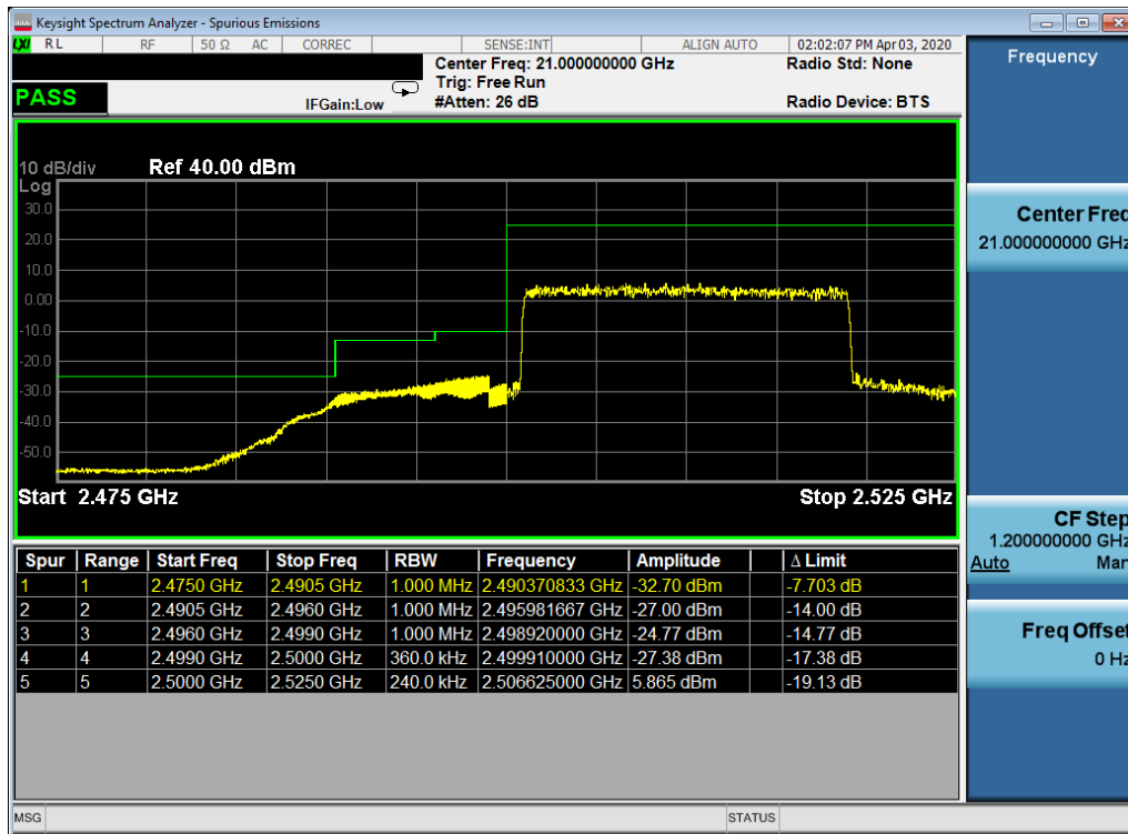
Plot 7-458. Lower ACP Plot (Band 7 - 20MHz QPSK - Full RB Configuration)
