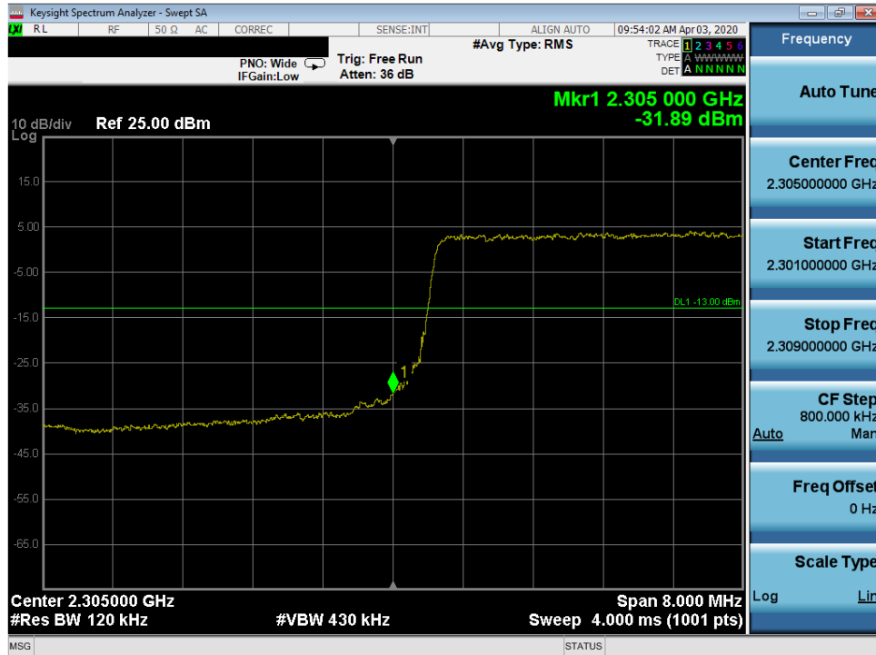
Plot 7-448. Lower Band Edge Plot (Band 30 - 10.0MHz QPSK - Full RB Configuration)
