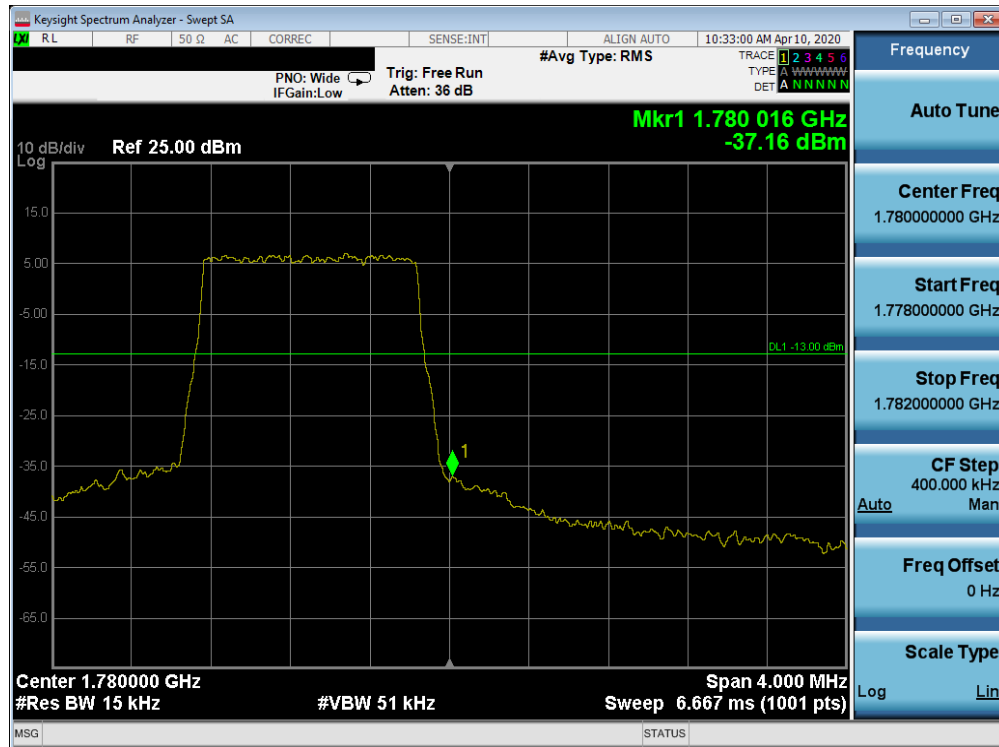
Plot 7-376. Upper Band Edge Plot (Band 66 - 1.4MHz QPSK - Full RB Configuration)
