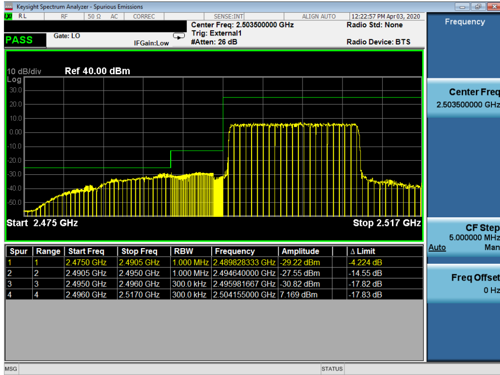
Plot 7-472. Lower ACP Plot (Band 41 - 15MHz QPSK - Full RB Configuration)
