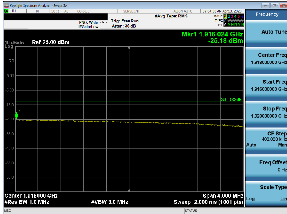
Plot 7-443. Upper Extended Band Edge Plot (Band 25 - 20.0MHz QPSK - Full RB Configuration)
