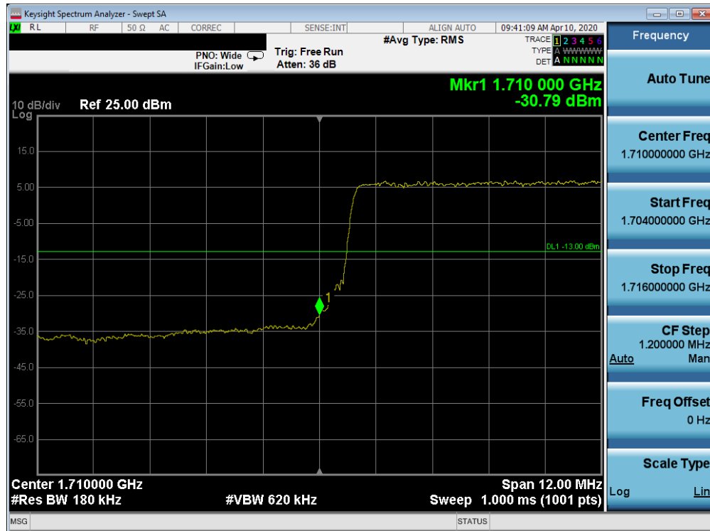
Plot 7-396. Lower Band Edge Plot (Band 66/4 - 15.0MHz QPSK - Full RB Configuration)
