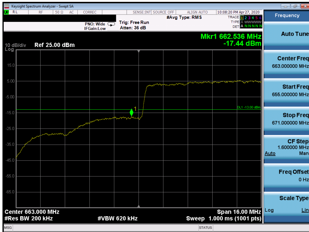
Plot 7-482. Lower 5G sub6 Band Edge Plot (5G sub6 n71 - 20.0MHz QPSK - Full RB Configuration)
