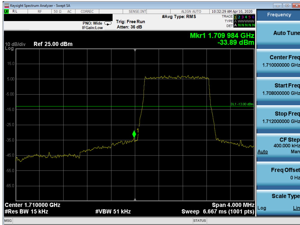
Plot 7-372. Lower Band Edge Plot (Band 66/4 - 1.4MHz QPSK - Full RB Configuration)
