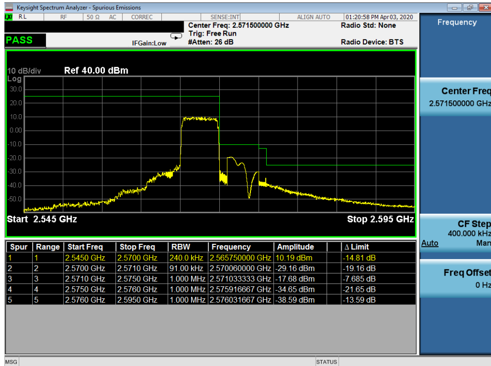
Plot 7-453. Upper ACP Plot (Band 7 - 5MHz QPSK - Full RB Configuration)
