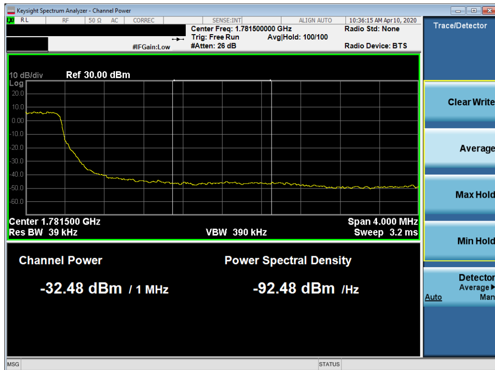
Plot 7-383. Upper Extended Band Edge Plot (Band 66 - 3.0MHz QPSK - Full RB Configuration)
