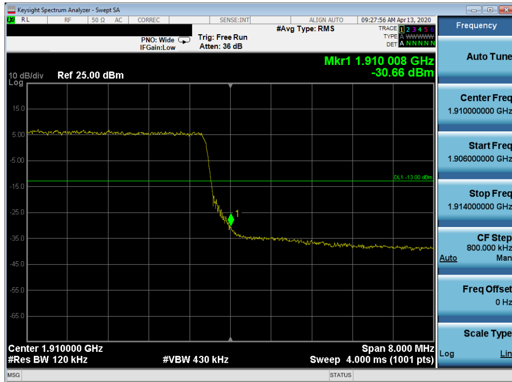
Plot 7-428. Upper Band Edge Plot (Band 2 - 10.0MHz QPSK - Full RB Configuration)
