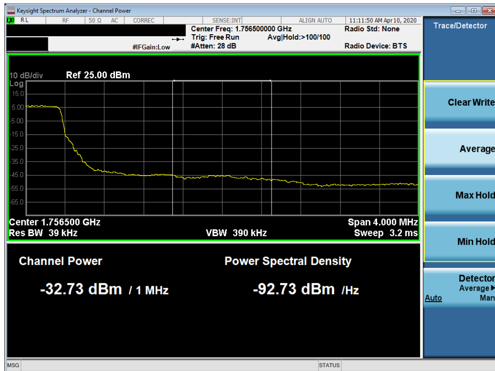
Plot 7-381. Upper Extended Band Edge Plot (Band 4 - 3.0MHz QPSK - Full RB Configuration)
