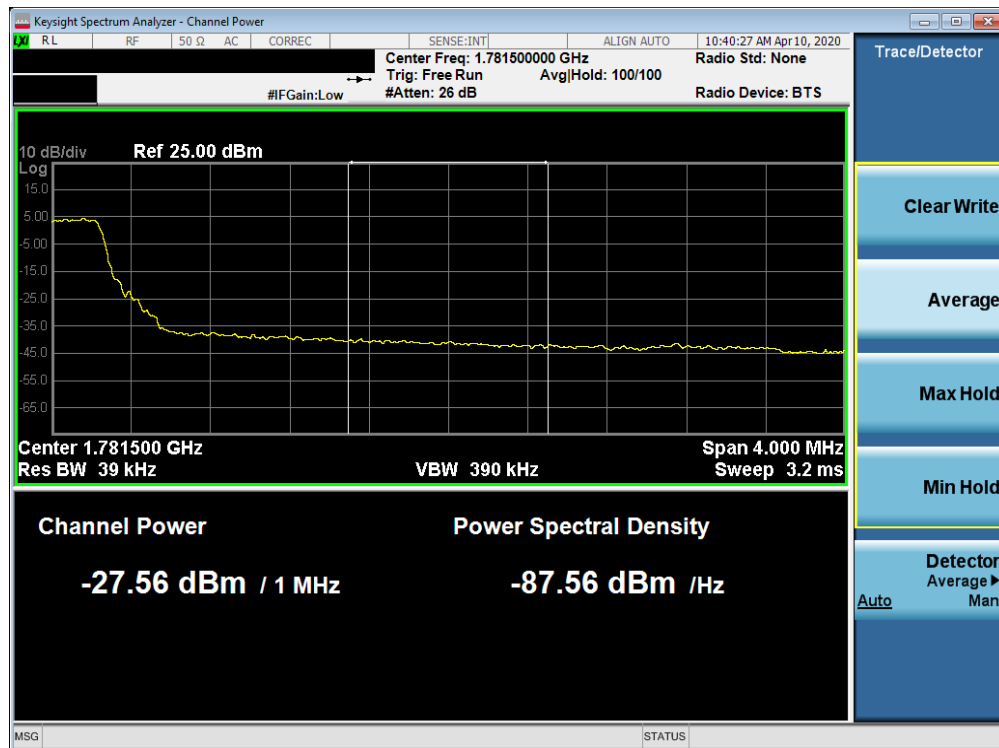
Plot 7-389. Upper Extended Band Edge Plot (Band 66 - 5.0MHz QPSK - Full RB Configuration)
