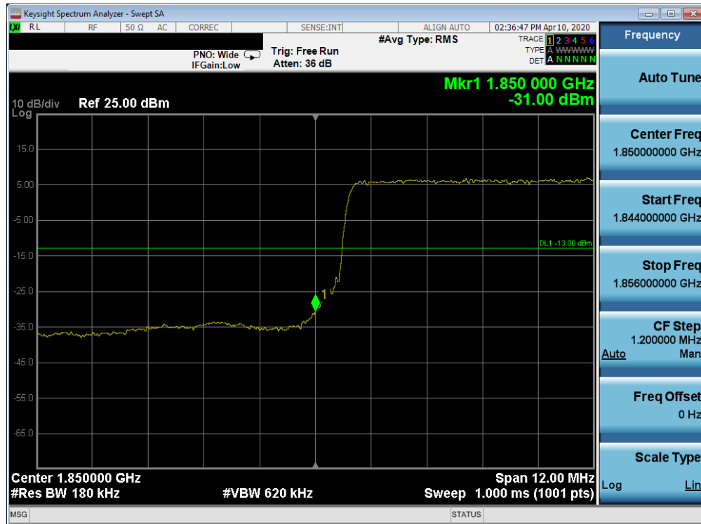
Plot 7-432. Lower Band Edge Plot (Band 25/2 - 15.0MHz QPSK - Full RB Configuration)
