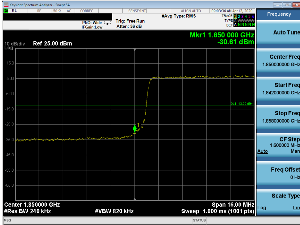
Plot 7-438. Lower Band Edge Plot (Band 25/2 - 20.0MHz QPSK - Full RB Configuration)
