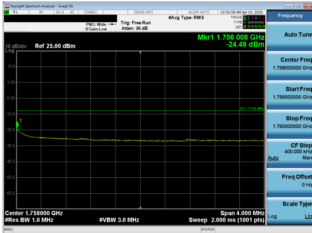
Plot 7-393. Upper Extended Band Edge Plot (Band 4 - 10.0MHz QPSK - Full RB Configuration)
