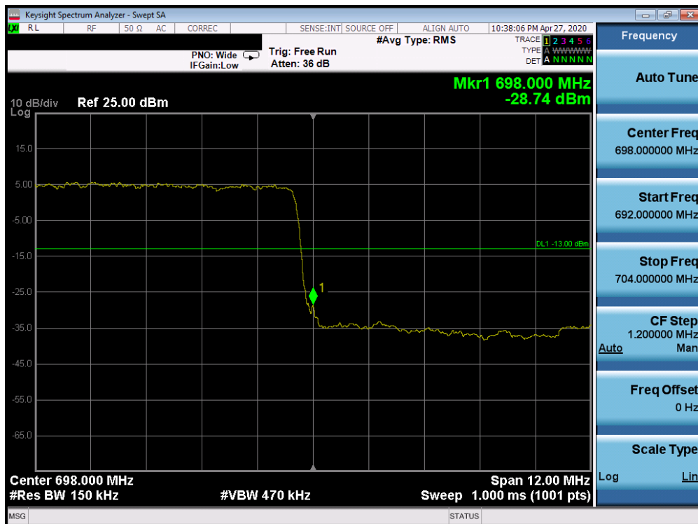
Plot 7-481. Upper 5G sub6 Band Edge Plot (5G sub6 n71 - 15.0MHz QPSK - Full RB Configuration)
