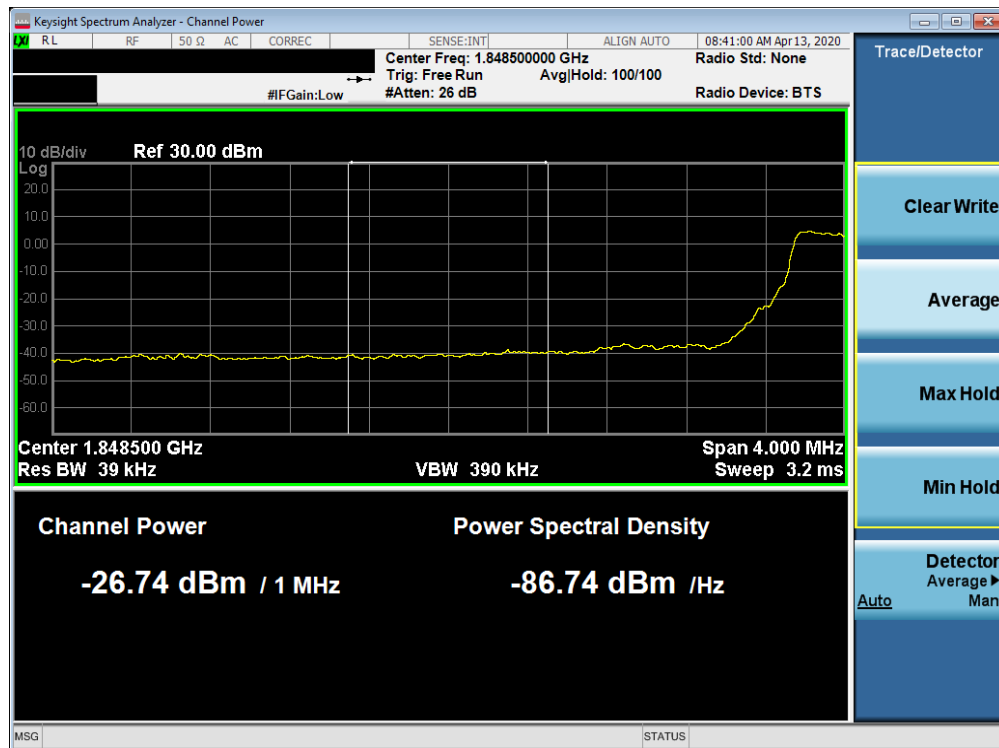
Plot 7-421. Lower Extended Band Edge Plot (Band 25/2 - 5.0MHz QPSK - Full RB Configuration)
