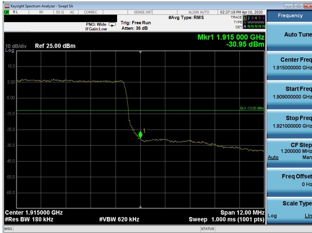
Plot 7-436. Upper Band Edge Plot (Band 25 - 15.0MHz QPSK - Full RB Configuration)
