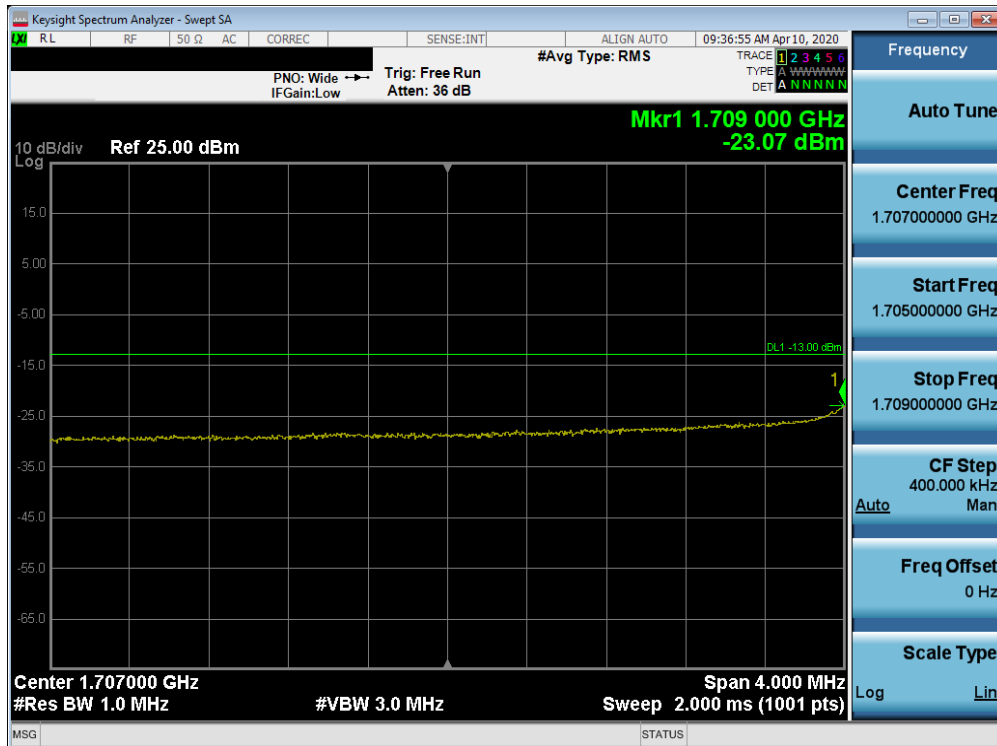
Plot 7-391. Lower Extended Band Edge Plot (Band 66/4 - 10.0MHz QPSK - Full RB Configuration)
