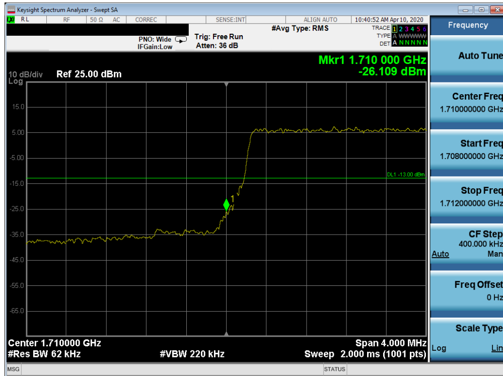
Plot 7-384. Lower Band Edge Plot (Band 66/4 - 5.0MHz QPSK - Full RB Configuration)
