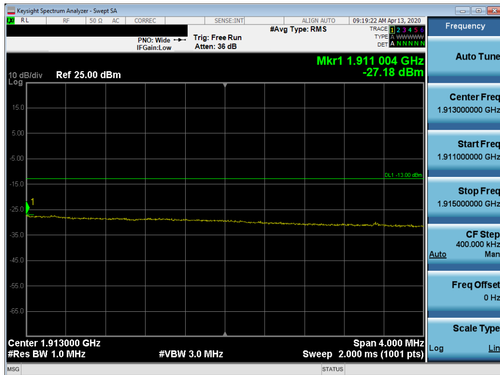
Plot 7-435. Upper Extended Band Edge Plot (Band 2 - 15.0MHz QPSK - Full RB Configuration)
