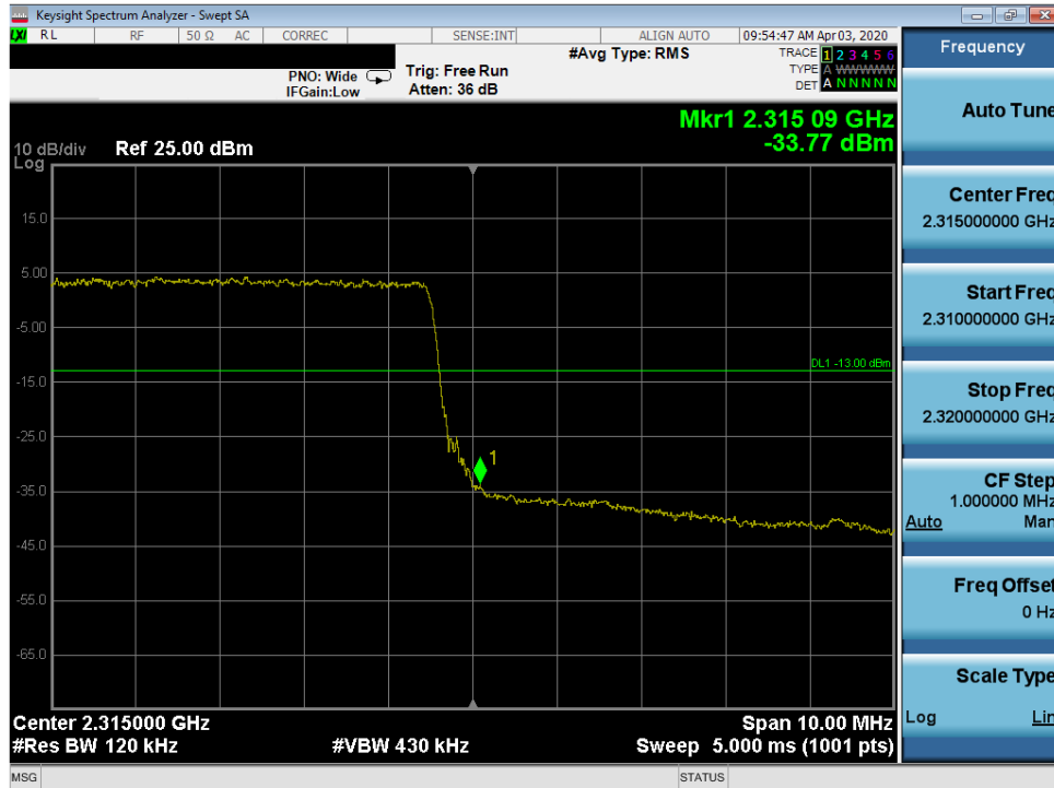
Plot 7-450. Upper Band Edge Plot (Band 30 - 10.0MHz QPSK - Full RB Configuration)
