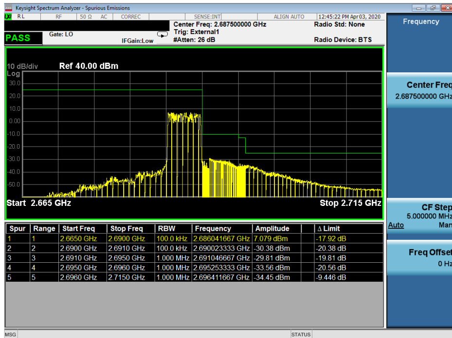
Plot 7-469. Upper ACP Plot (Band 41 - 5MHz QPSK - Full RB Configuration)
