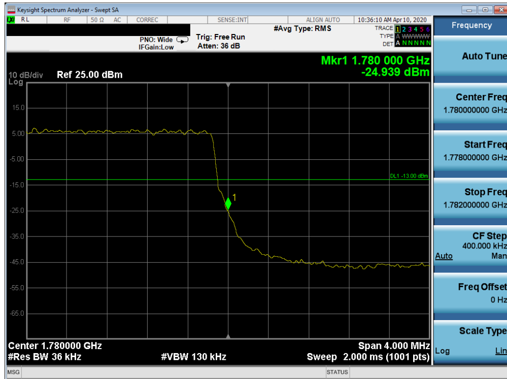
Plot 7-382. Upper Band Edge Plot (Band 66 - 3.0MHz QPSK - Full RB Configuration)
