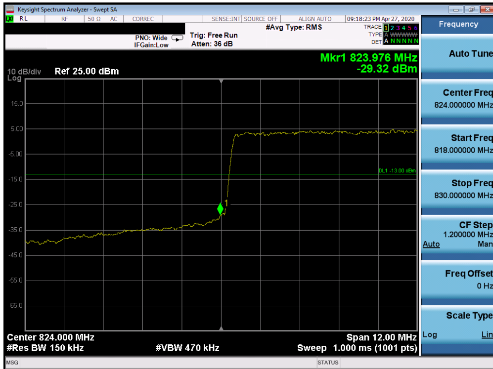
Plot 7-488. Lower 5G sub6 Band Edge Plot (5G sub6 n5 – 15MHz QPSK - Full RB Configuration)
