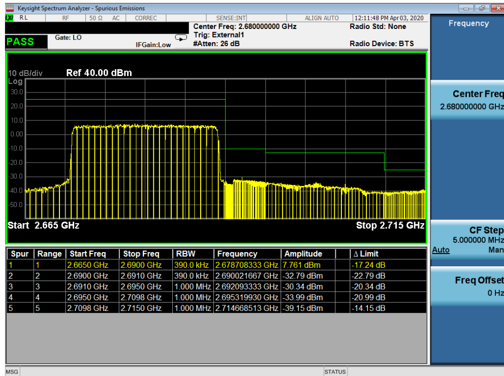
Plot 7-475. Upper ACP Plot (Band 41 - 20MHz QPSK - Full RB Configuration)
