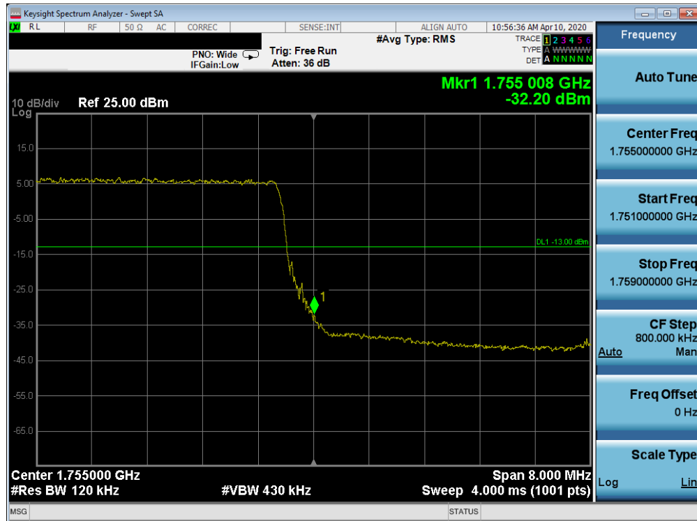
Plot 7-392. Upper Band Edge Plot (Band 4 - 10.0MHz QPSK - Full RB Configuration)
