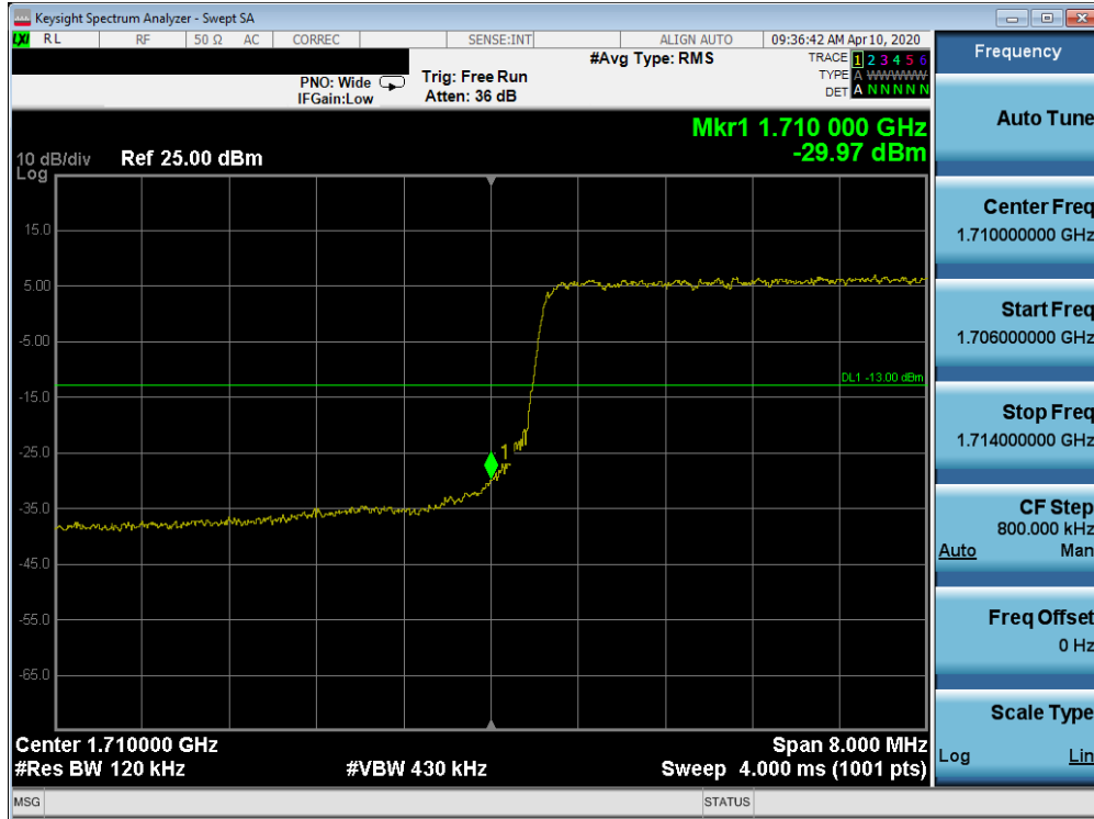
Plot 7-390. Lower Band Edge Plot (Band 66/4 - 10.0MHz QPSK - Full RB Configuration)
