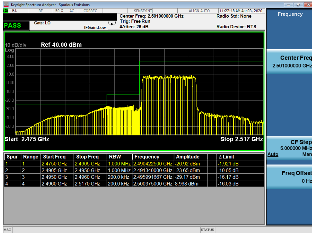
Plot 7-462. Lower ACP Plot (Band 41 - 10MHz QPSK - Full RB Configuration)
