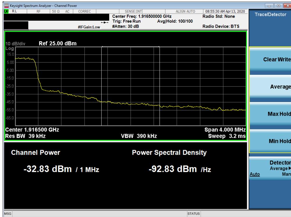
Plot 7-413. Upper Extended Band Edge Plot (Band 25 - 1.4MHz QPSK - Full RB Configuration)
