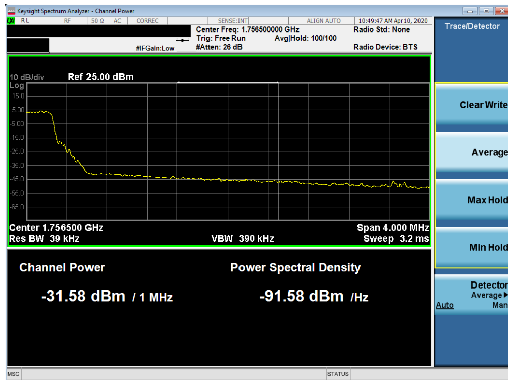
Plot 7-387. Upper Extended Band Edge Plot (Band 4 - 5.0MHz QPSK - Full RB Configuration)
