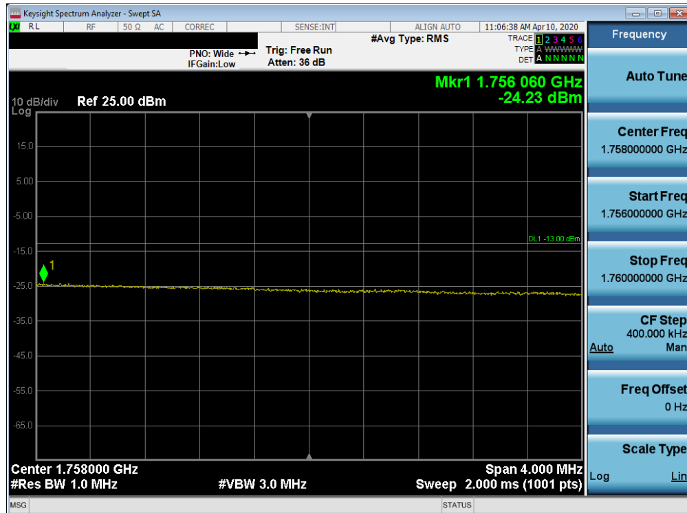
Plot 7-405. Upper Extended Band Edge Plot (Band 4 - 20.0MHz QPSK - Full RB Configuration)
