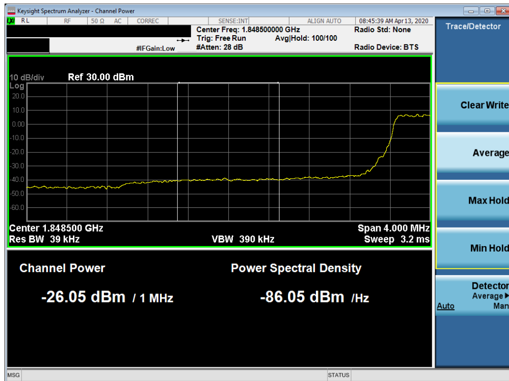
Plot 7-415. Lower Extended Band Edge Plot (Band 25/2 - 3.0MHz QPSK - Full RB Configuration)
