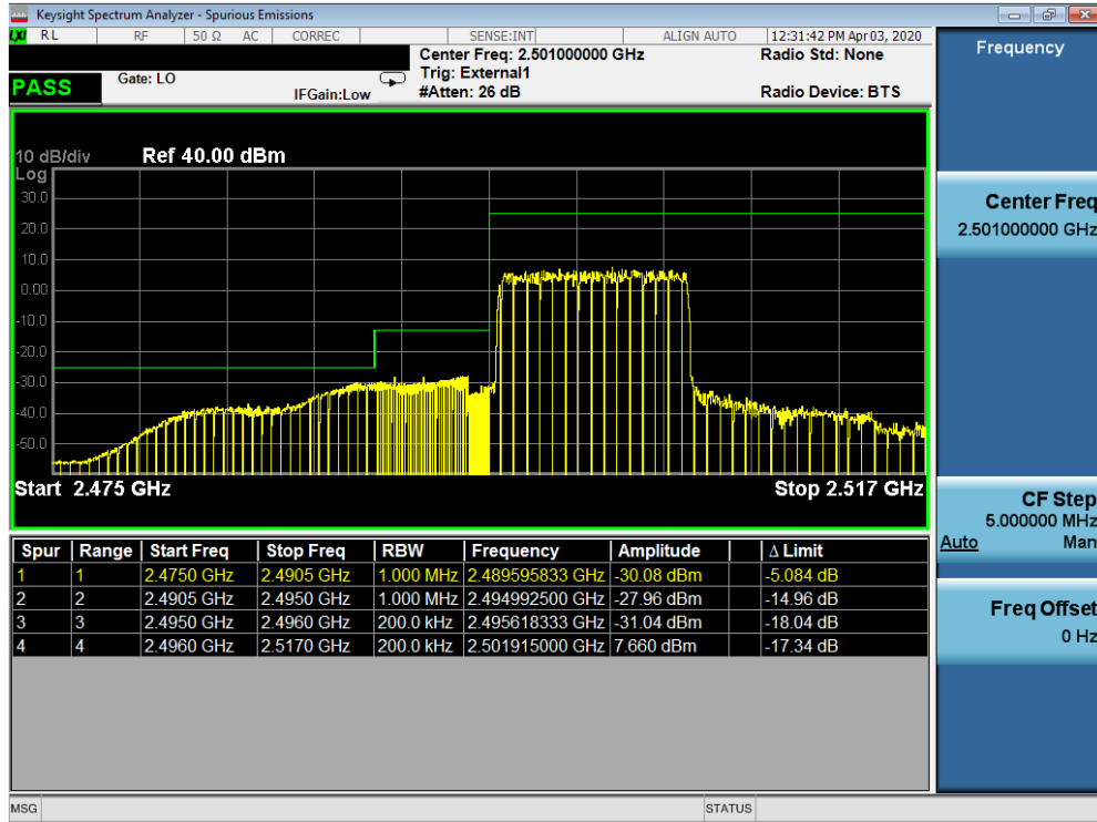
Plot 7-470. Lower ACP Plot (Band 41 - 10MHz QPSK - Full RB Configuration)
