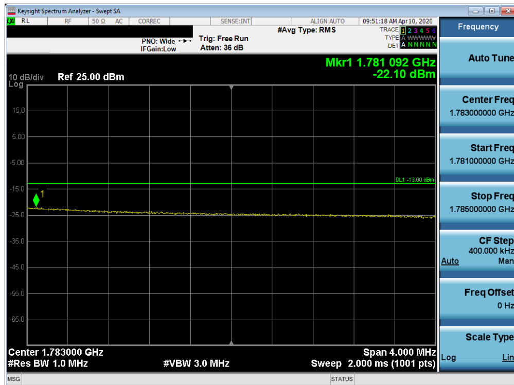
Plot 7-407. Upper Extended Band Edge Plot (Band 66 - 20.0MHz QPSK - Full RB Configuration)
