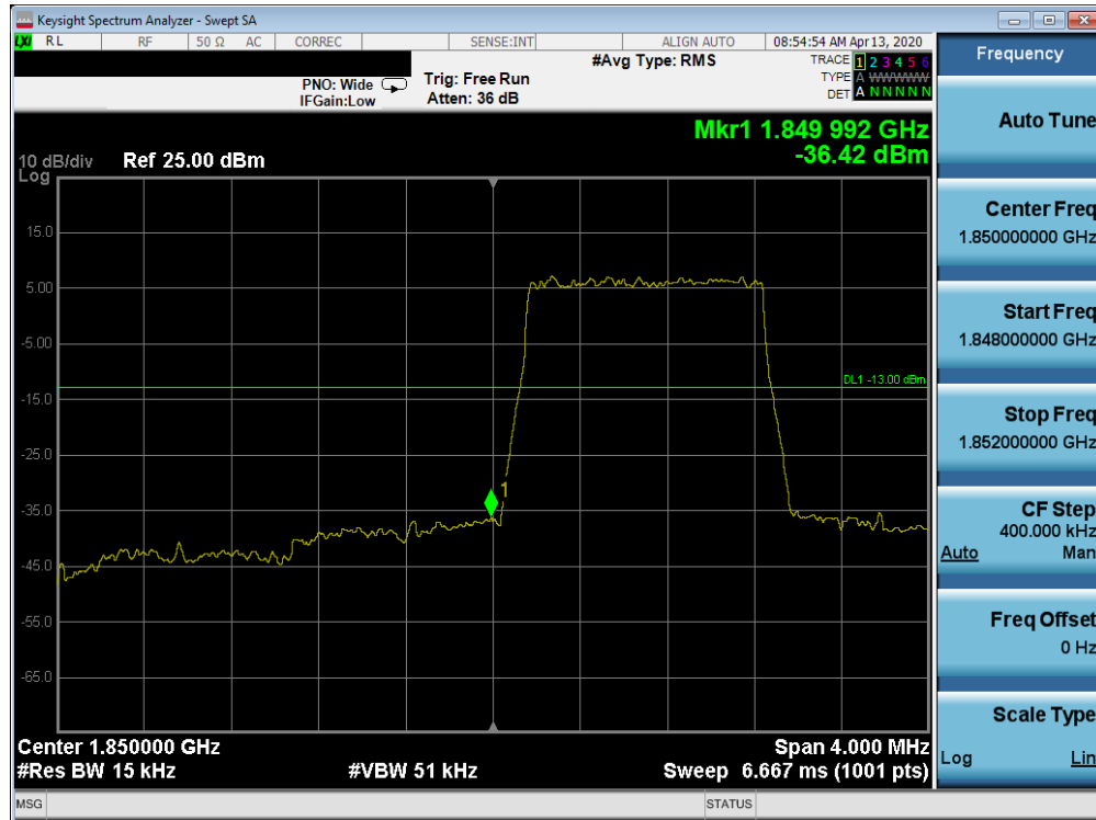
Plot 7-408. Lower Band Edge Plot (Band 25/2 - 1.4MHz QPSK - Full RB Configuration)
