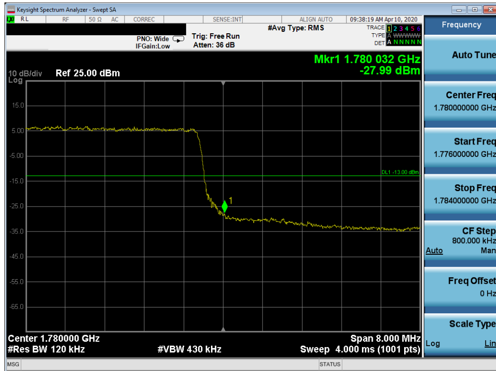
Plot 7-394. Upper Band Edge Plot (Band 66 - 10.0MHz QPSK - Full RB Configuration)
