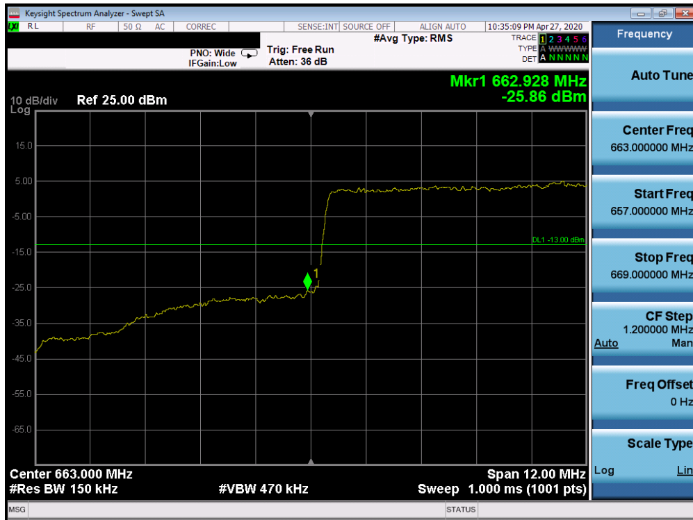
Plot 7-480. Lower 5G sub6 Band Edge Plot (5G sub6 n71 - 15.0MHz QPSK - Full RB Configuration)
