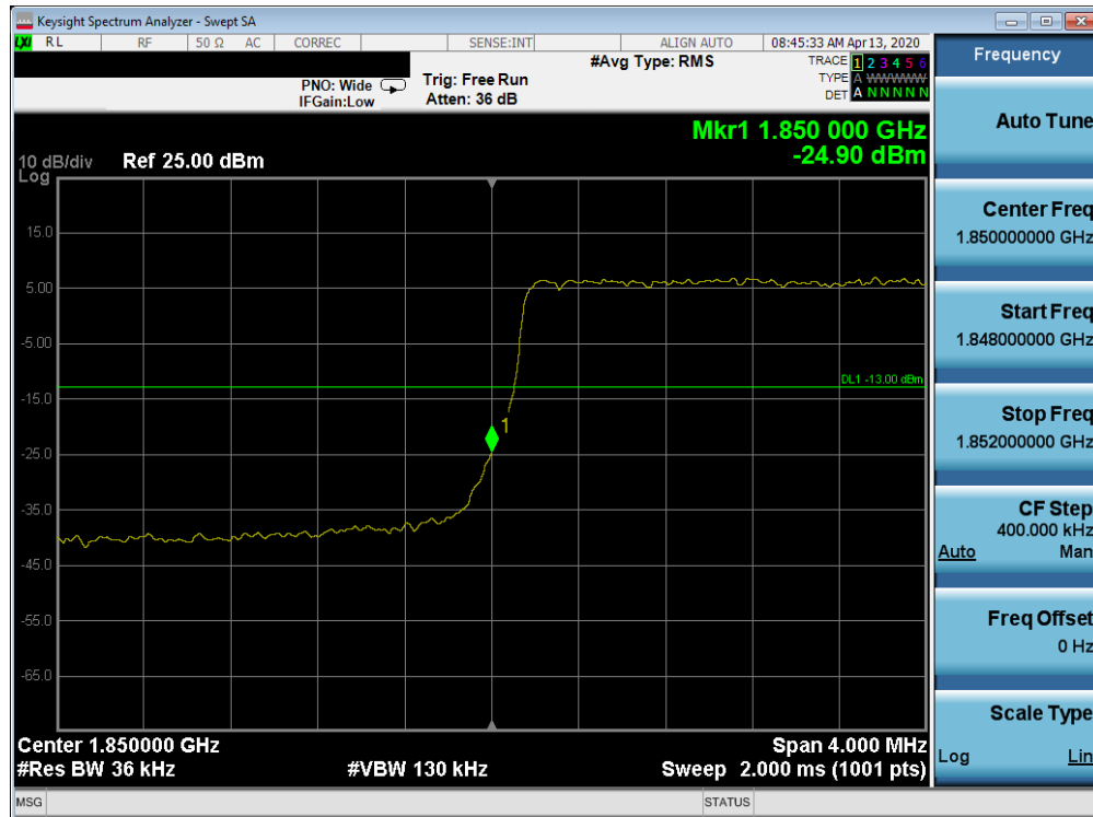
Plot 7-414. Lower Band Edge Plot (Band 25/2 - 3.0MHz QPSK - Full RB Configuration)
