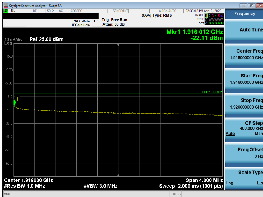
Plot 7-431. Upper Extended Band Edge Plot (Band 25 - 10.0MHz QPSK - Full RB Configuration)
