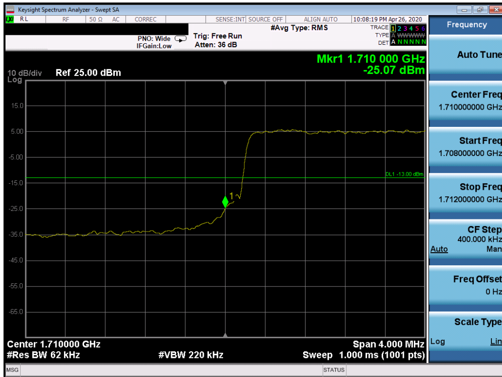
Plot 7-492. Lower 5G sub6 Band Edge Plot (5G sub6 n66 - 5.0MHz QPSK - Full RB Configuration)
