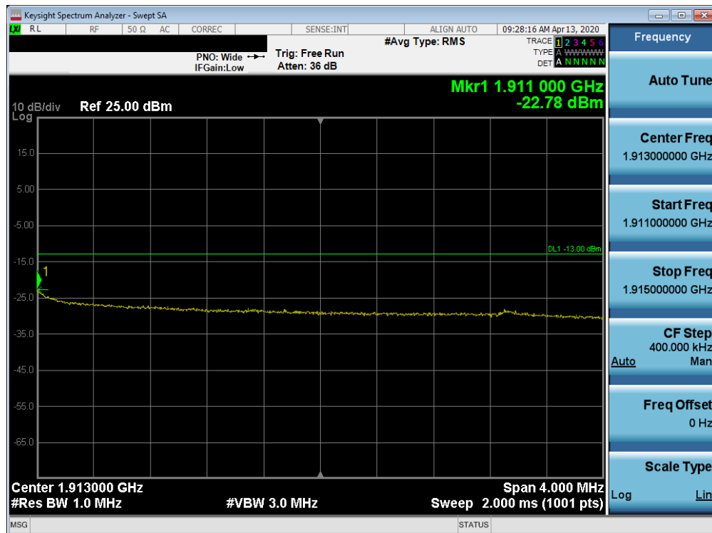
Plot 7-429. Upper Extended Band Edge Plot (Band 2 - 10.0MHz QPSK - Full RB Configuration)
