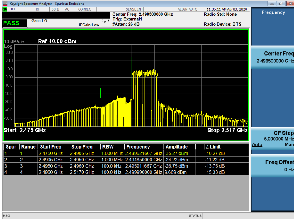
Plot 7-460. Lower ACP Plot (Band 41 - 5MHz QPSK - Full RB Configuration)
