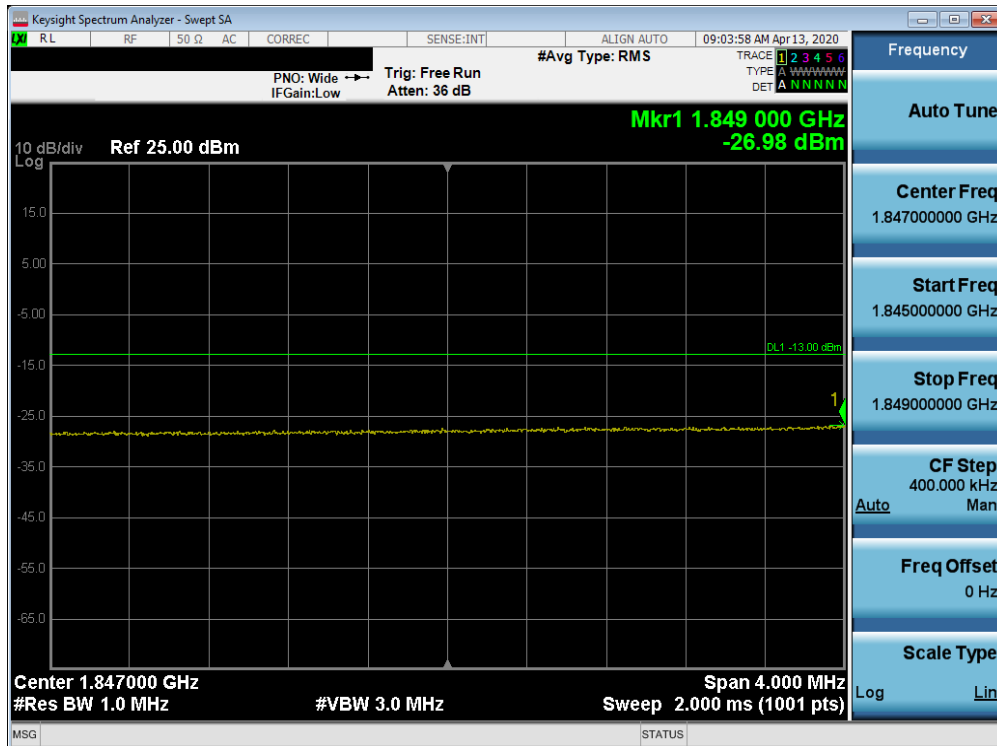
Plot 7-439. Lower Extended Band Edge Plot (Band 25/2 - 20.0MHz QPSK - Full RB Configuration)
