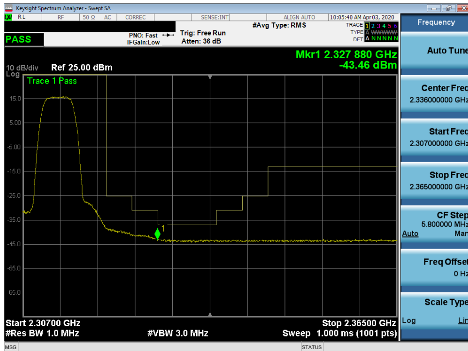
Plot 7-447. Upper Extended Band Edge Plot (Band 30 - 5.0MHz QPSK - Full RB Configuration)
