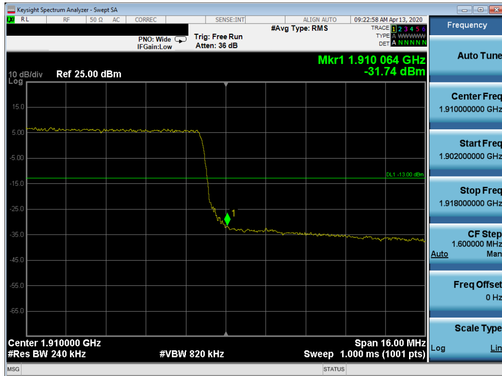
Plot 7-440. Upper Band Edge Plot (Band 2 - 20.0MHz QPSK - Full RB Configuration)
