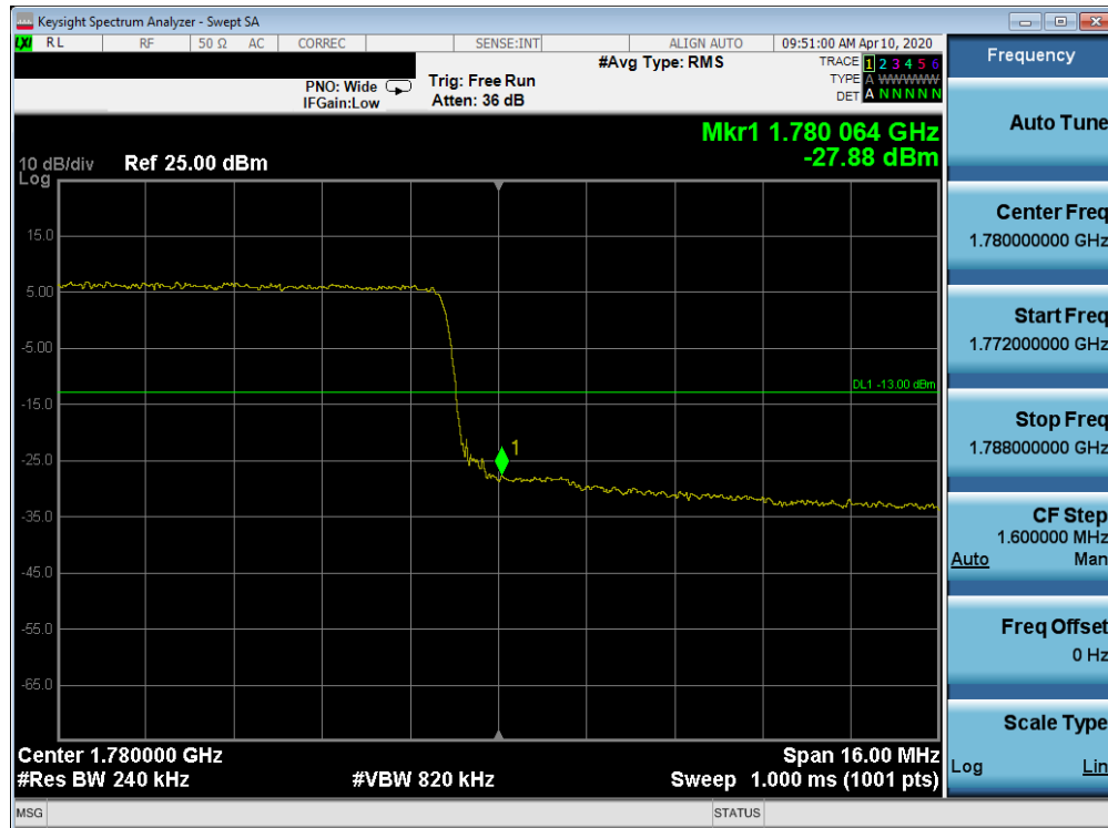
Plot 7-406. Upper Band Edge Plot (Band 66 - 20.0MHz QPSK - Full RB Configuration)
