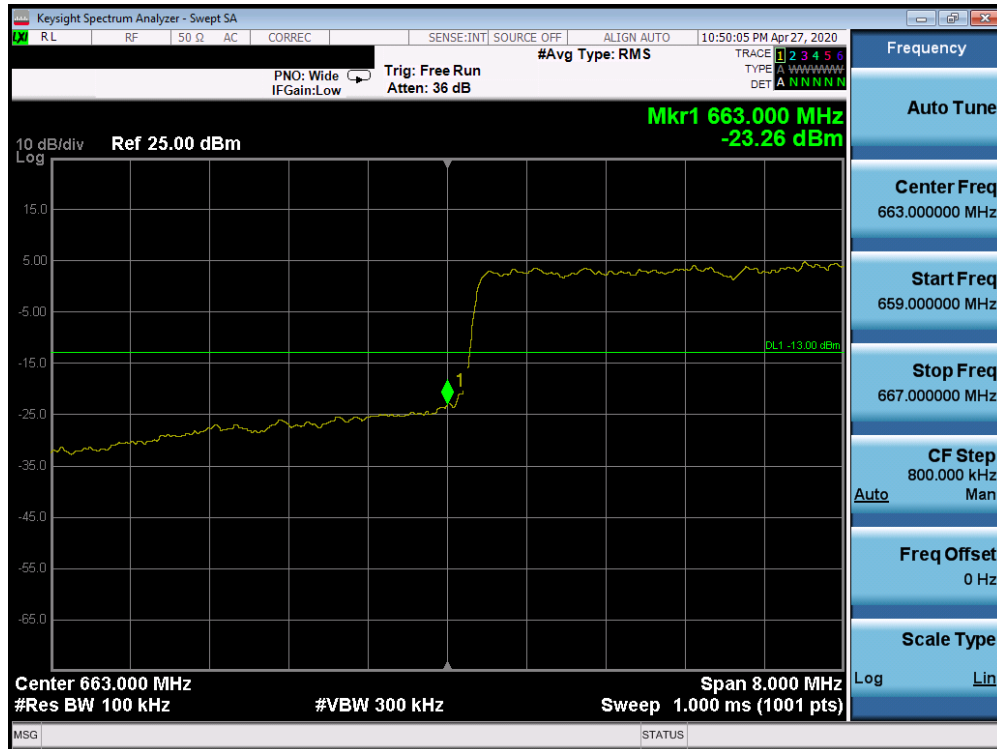
Plot 7-478. Lower 5G sub6 Band Edge Plot (5G sub6 n71 - 10.0MHz QPSK - Full RB Configuration)
