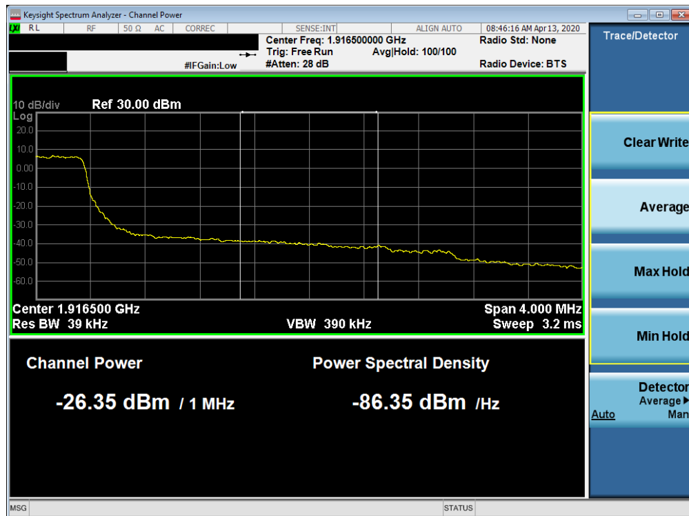
Plot 7-419. Upper Extended Band Edge Plot (Band 25 - 3.0MHz QPSK - Full RB Configuration)
