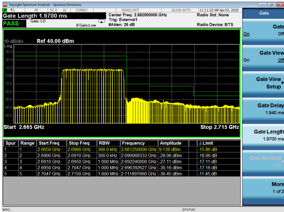
Plot 7-465. Upper ACP Plot (Band 41 - 15MHz QPSK - Full RB Configuration)
