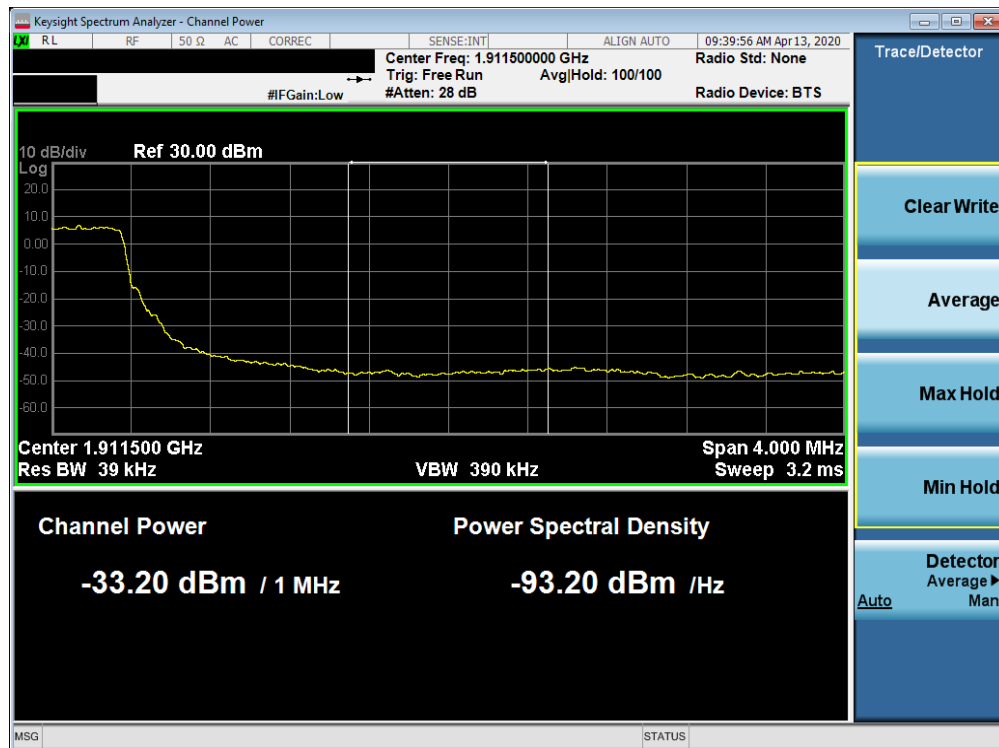
Plot 7-417. Upper Extended Band Edge Plot (Band 2 - 3.0MHz QPSK - Full RB Configuration)
