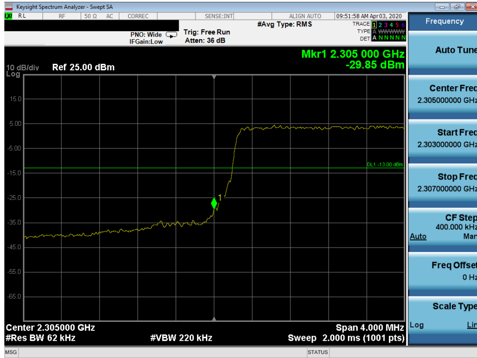
Plot 7-444. Lower Band Edge Plot (Band 30 - 5.0MHz QPSK - Full RB Configuration)
