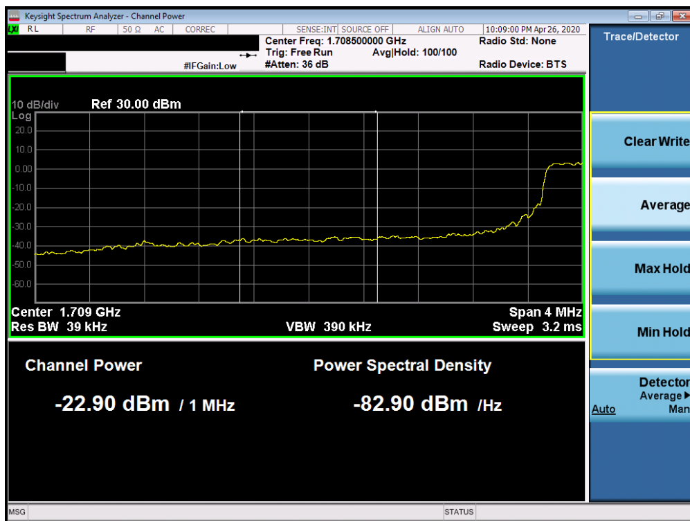
Plot 7-493. Lower Extended 5G sub6 Band Edge Plot (5G sub6 n66 - 5.0MHz QPSK - Full RB Configuration)
