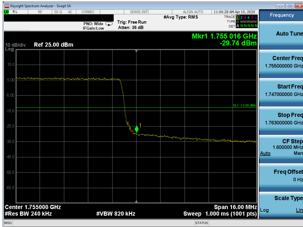
Plot 7-404. Upper Band Edge Plot (Band 4 - 20.0MHz QPSK - Full RB Configuration)
