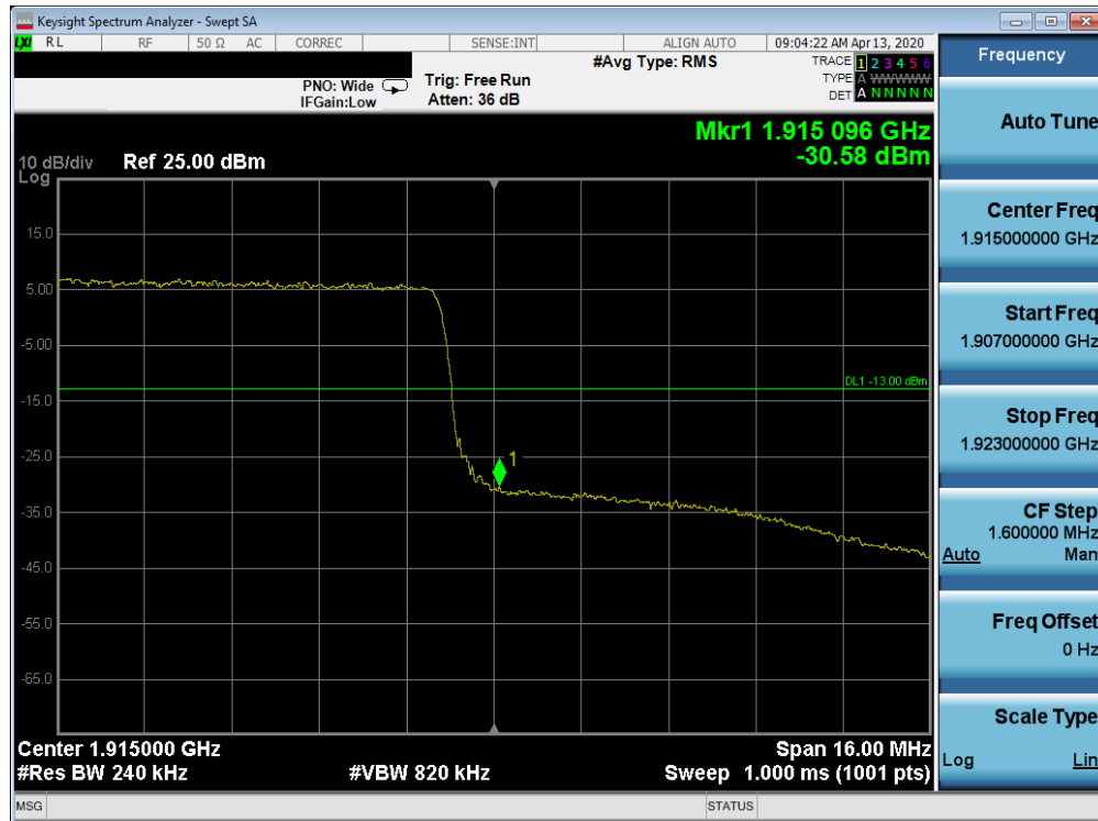
Plot 7-442. Upper Band Edge Plot (Band 25 - 20.0MHz QPSK - Full RB Configuration)
