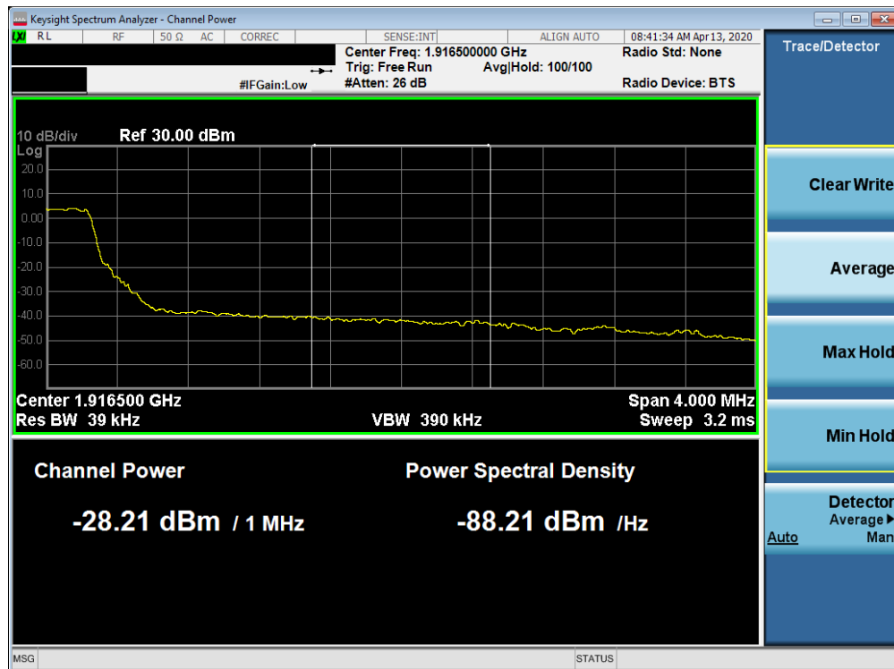
Plot 7-425. Upper Extended Band Edge Plot (Band 25 - 5.0MHz QPSK - Full RB Configuration)
