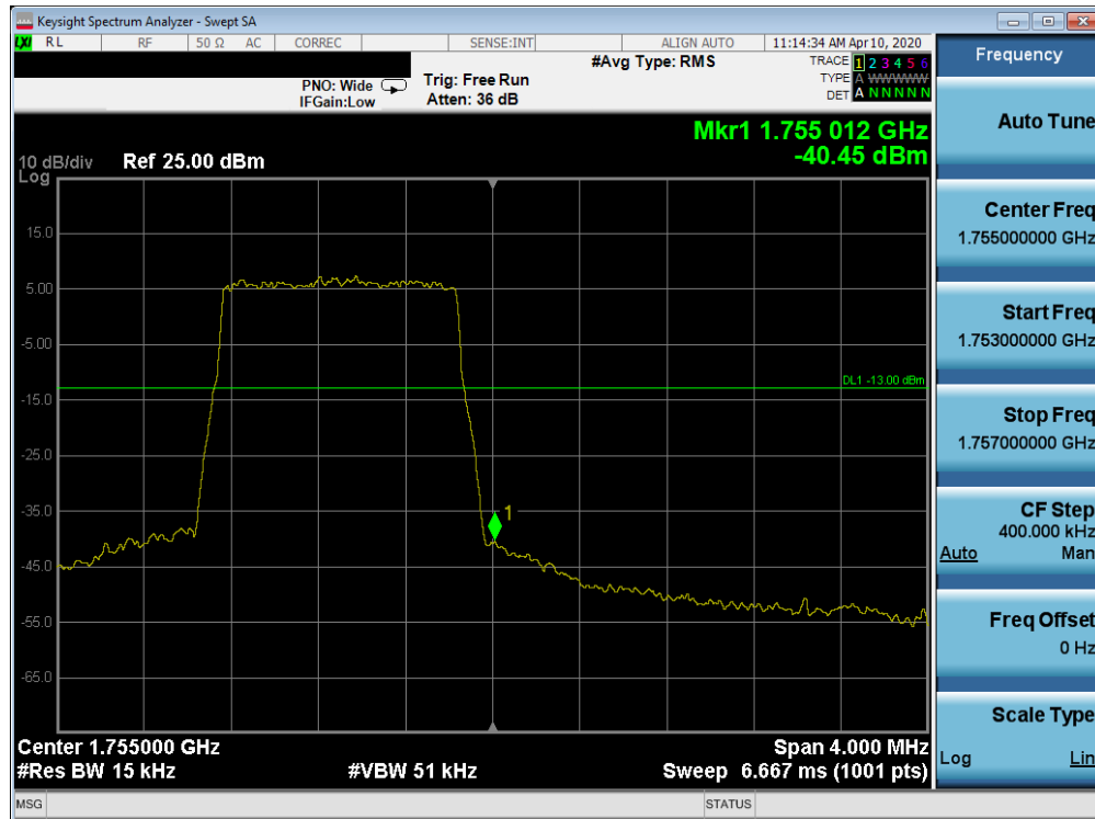
Plot 7-374. Upper Band Edge Plot (Band 4 - 1.4MHz QPSK - Full RB Configuration)
