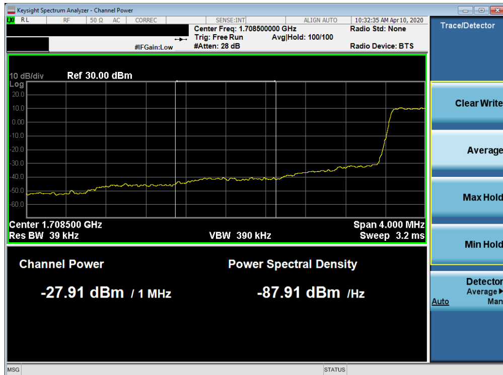
Plot 7-373. Lower Extended Band Edge Plot (Band 66/4 - 1.4MHz QPSK - Full RB Configuration)
