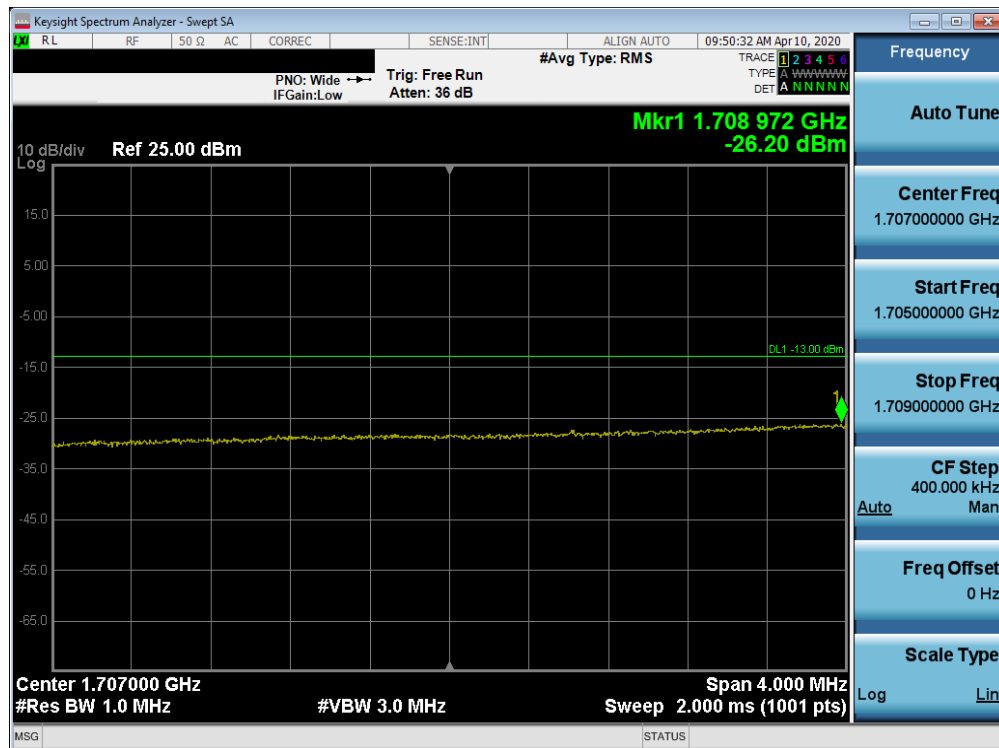
Plot 7-403. Lower Extended Band Edge Plot (Band 66/4 - 20.0MHz QPSK - Full RB Configuration)
