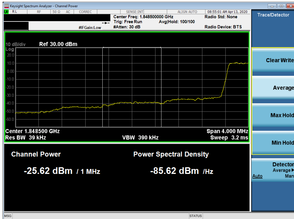
Plot 7-409. Lower Extended Band Edge Plot (Band 25/2 - 1.4MHz QPSK - Full RB Configuration)
