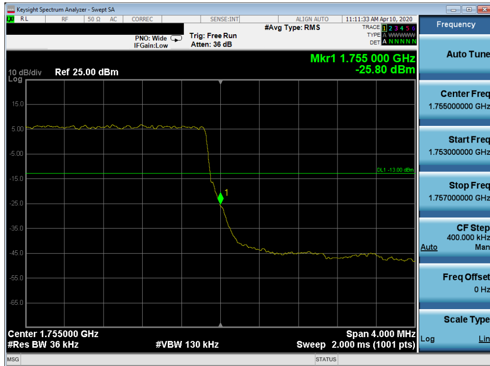
Plot 7-380. Upper Band Edge Plot (Band 4 - 3.0MHz QPSK - Full RB Configuration)
