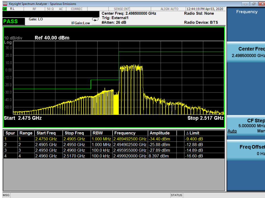
Plot 7-468. Lower ACP Plot (Band 41 - 5MHz QPSK - Full RB Configuration)
