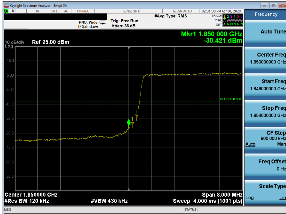
Plot 7-426. Lower Band Edge Plot (Band 25/2 - 10.0MHz QPSK - Full RB Configuration)
