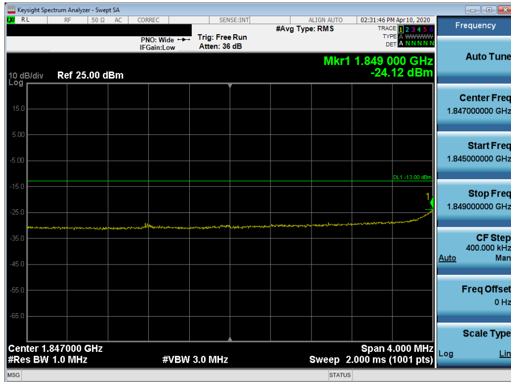
Plot 7-427. Lower Extended Band Edge Plot (Band 25/2 - 10.0MHz QPSK - Full RB Configuration)
