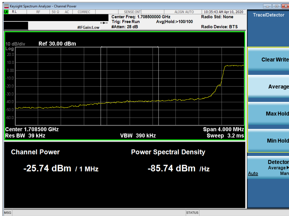
Plot 7-379. Lower Extended Band Edge Plot (Band 66/4 - 3.0MHz QPSK - Full RB Configuration)
