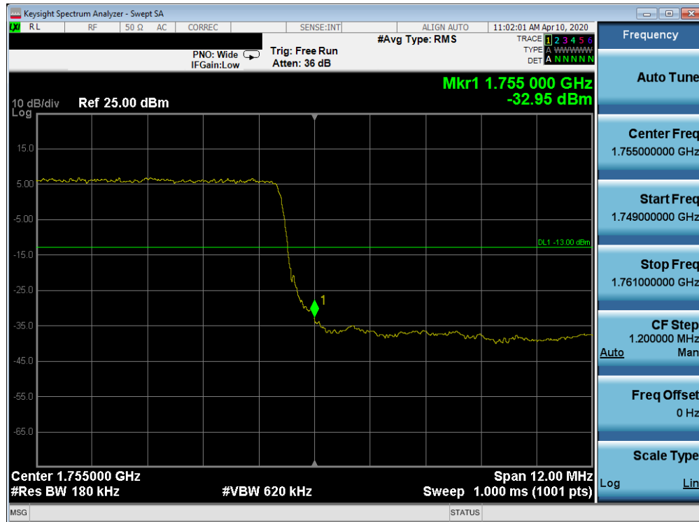
Plot 7-398. Upper Band Edge Plot (Band 4 - 15.0MHz QPSK - Full RB Configuration)
