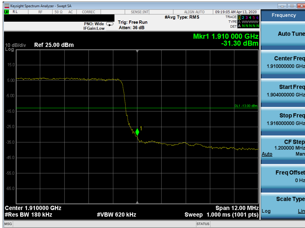
Plot 7-434. Upper Band Edge Plot (Band 2 - 15.0MHz QPSK - Full RB Configuration)
