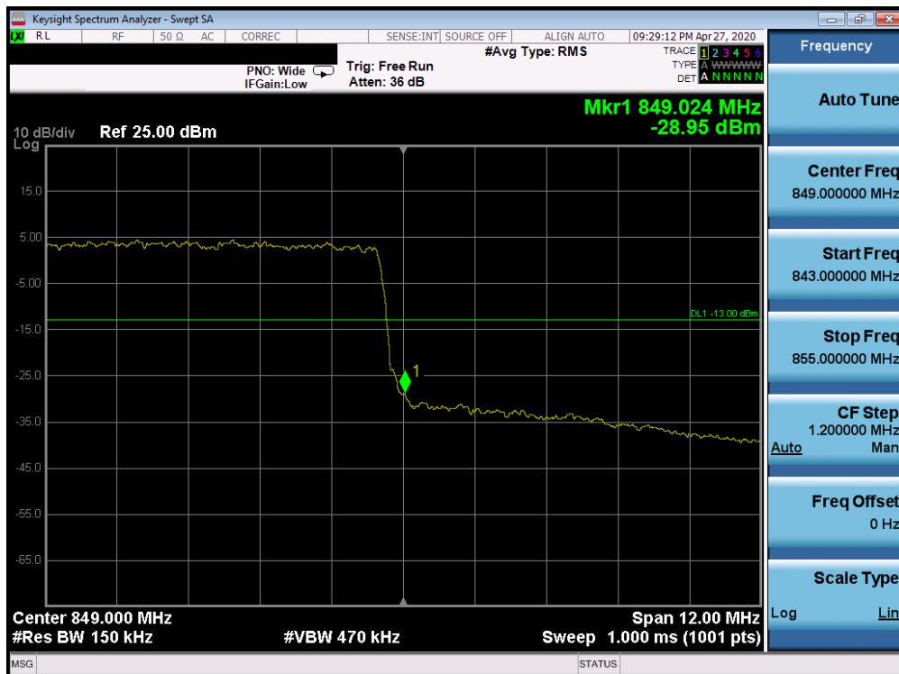
Plot 7-489. Upper 5G sub6 Band Edge Plot (5G sub6 n5 – 15MHz QPSK - Full RB Configuration)
