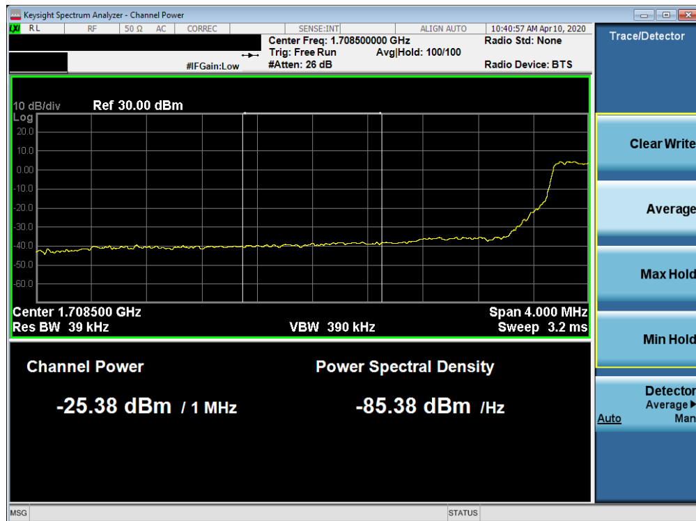
Plot 7-385. Lower Extended Band Edge Plot (Band 66/4 - 5.0MHz QPSK - Full RB Configuration)
