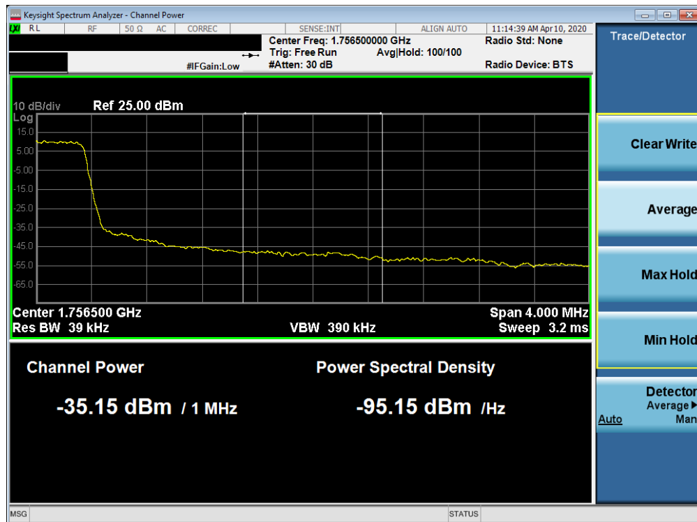
Plot 7-375. Upper Extended Band Edge Plot (Band 4 - 1.4MHz QPSK - Full RB Configuration)
