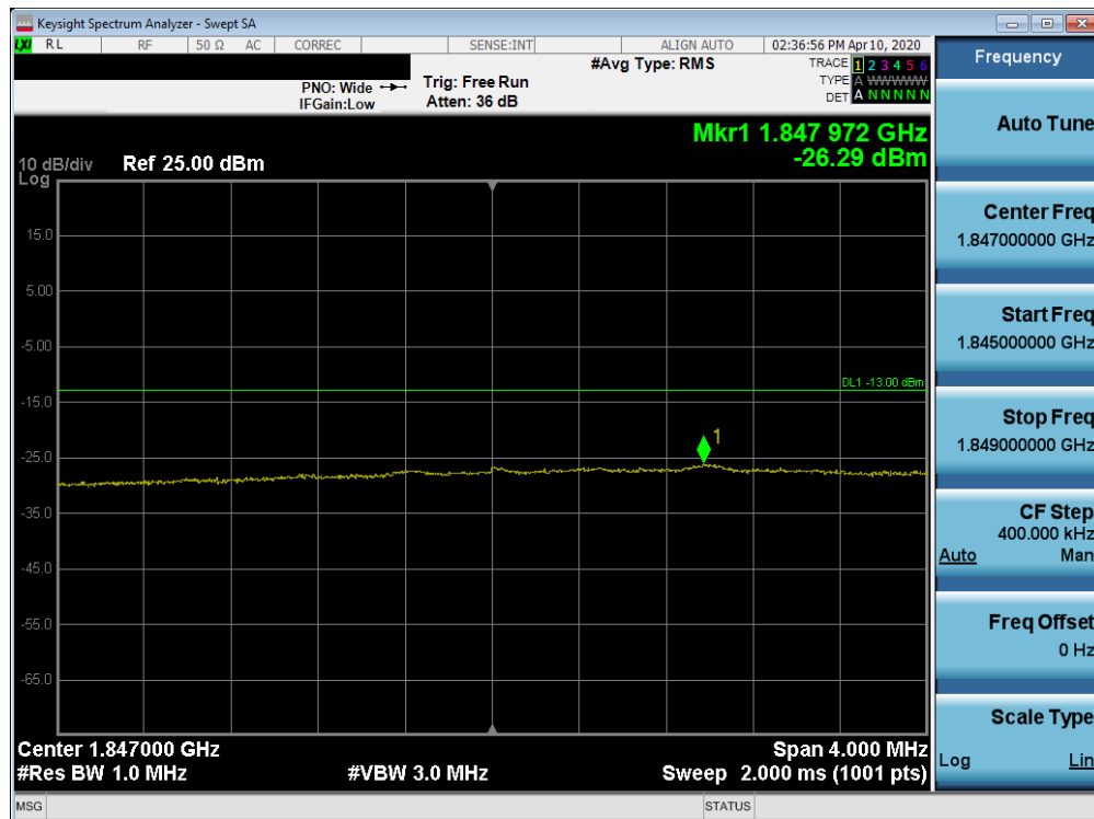
Plot 7-433. Lower Extended Band Edge Plot (Band 25/2 - 15.0MHz QPSK - Full RB Configuration)
