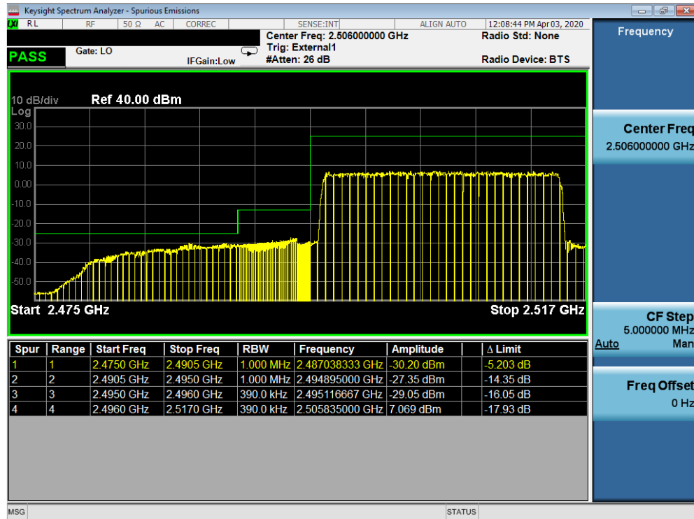
Plot 7-474. Lower ACP Plot (Band 41 - 20MHz QPSK - Full RB Configuration)
