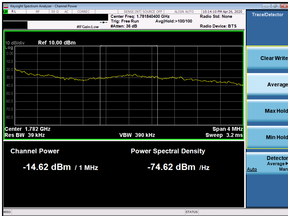
Plot 7-495. Upper Extended 5G sub6 Band Edge Plot (5G sub6 n66 - 5.0MHz QPSK - Full RB Configuration)
