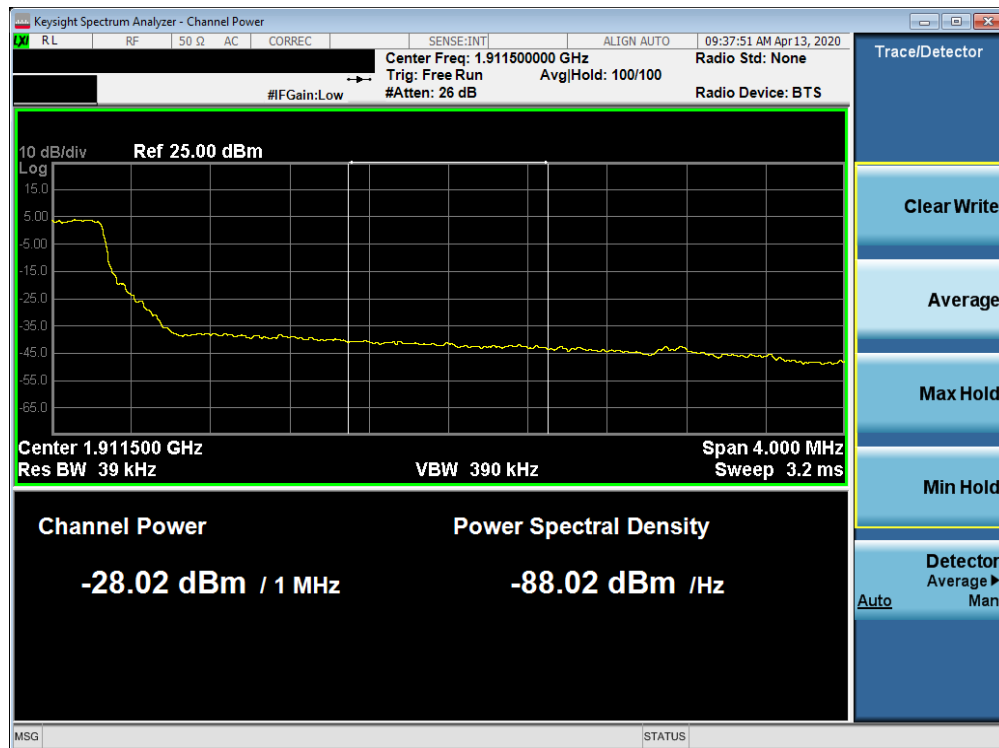
Plot 7-423. Upper Extended Band Edge Plot (Band 2 - 5.0MHz QPSK - Full RB Configuration)
