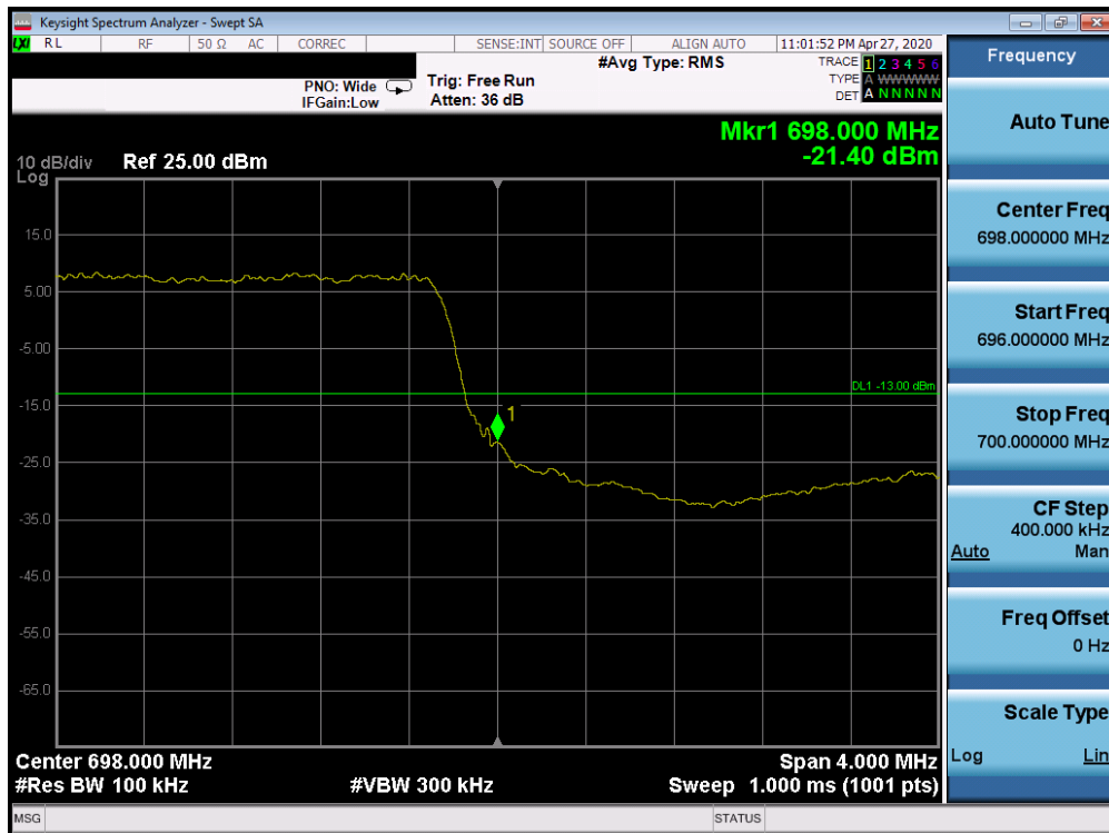
Plot 7-477. Upper 5G sub6 Band Edge Plot (5G sub6 n71 - 5.0MHz QPSK - Full RB Configuration)
