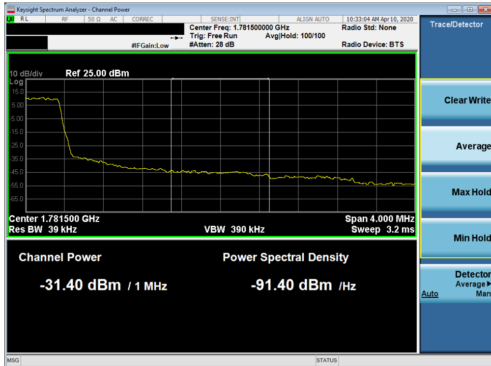
Plot 7-377. Upper Extended Band Edge Plot (Band 66 - 1.4MHz QPSK - Full RB Configuration)
