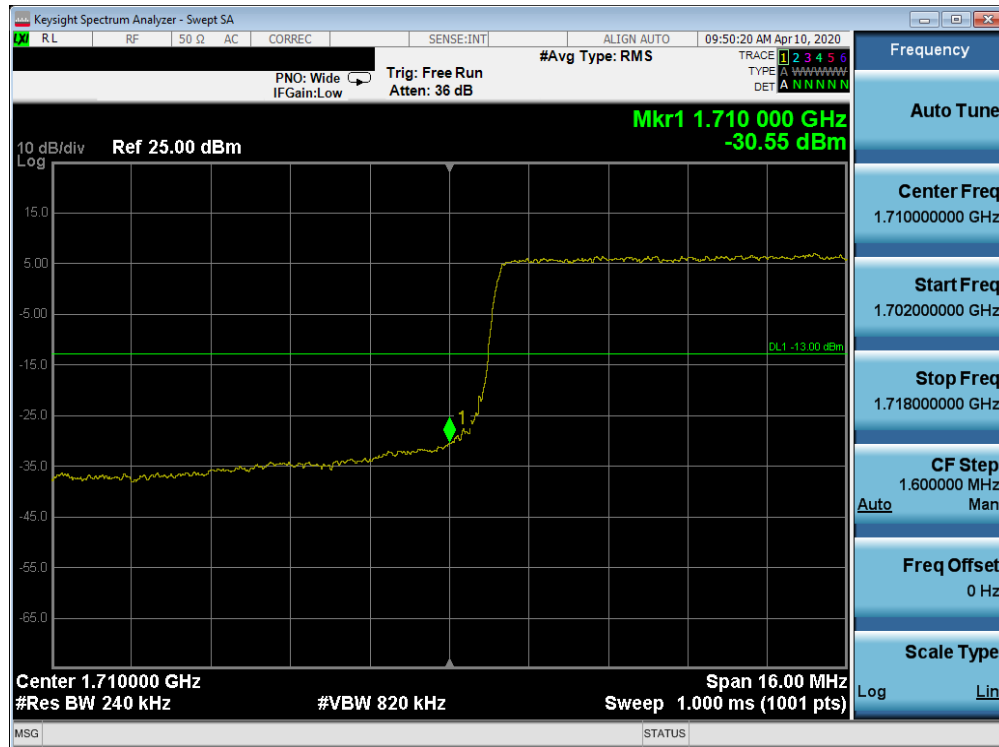
Plot 7-402. Lower Band Edge Plot (Band 66/4 - 20.0MHz QPSK - Full RB Configuration)
