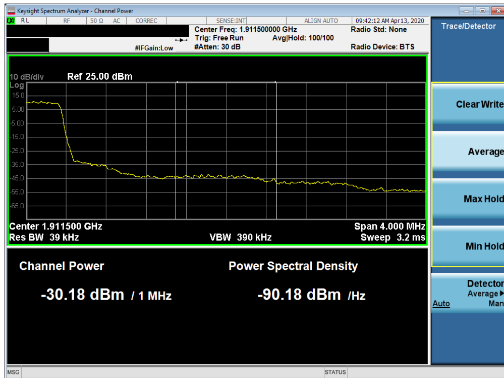
Plot 7-411. Upper Extended Band Edge Plot (Band 2 - 1.4MHz QPSK - Full RB Configuration)
