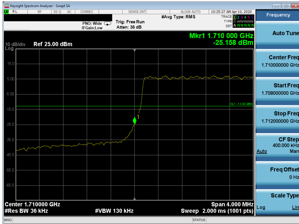
Plot 7-378. Lower Band Edge Plot (Band 66/4 - 3.0MHz QPSK - Full RB Configuration)
