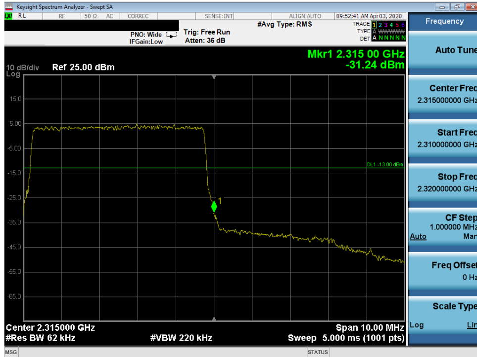
Plot 7-446. Upper Band Edge Plot (Band 30 - 5.0MHz QPSK - Full RB Configuration)
