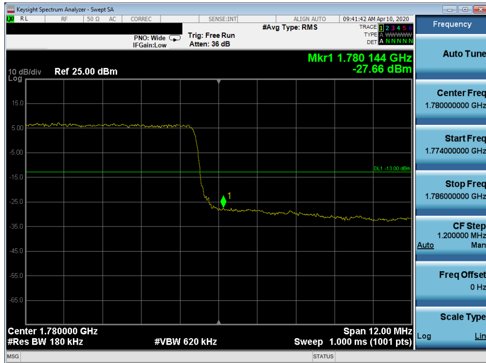
Plot 7-400. Upper Band Edge Plot (Band 66 - 15.0MHz QPSK - Full RB Configuration)
