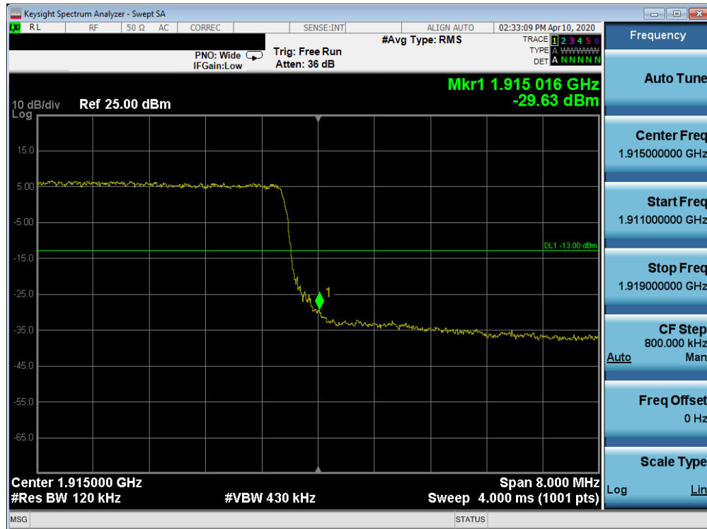
Plot 7-430. Upper Band Edge Plot (Band 25 - 10.0MHz QPSK - Full RB Configuration)
