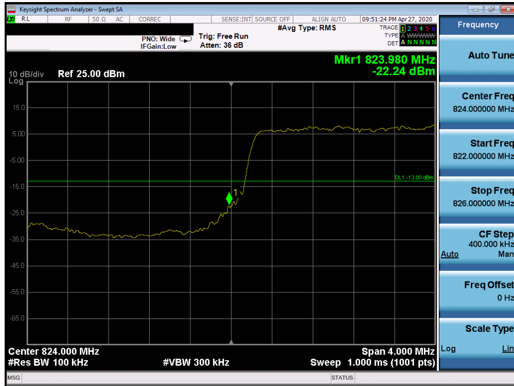
Plot 7-484. Lower 5G sub6 Band Edge Plot (5G sub6 n5 - 5.0MHz QPSK - Full RB Configuration)
