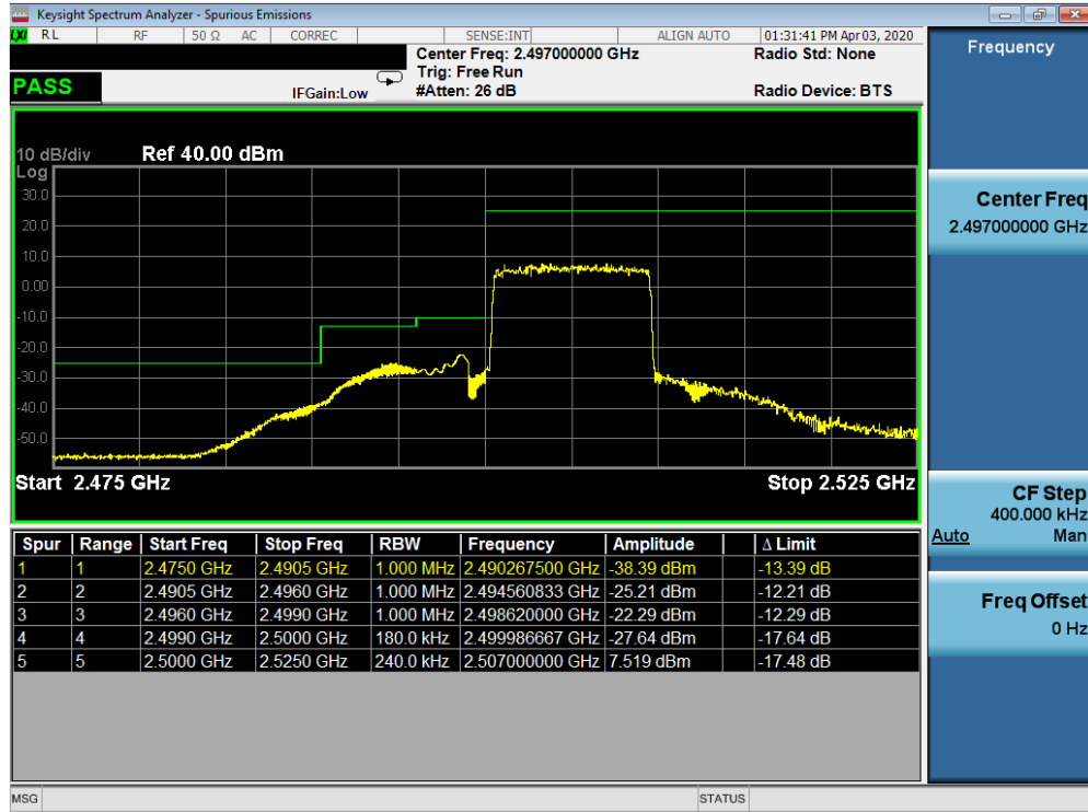
Plot 7-454. Lower ACP Plot (Band 7 - 10MHz QPSK - Full RB Configuration)
