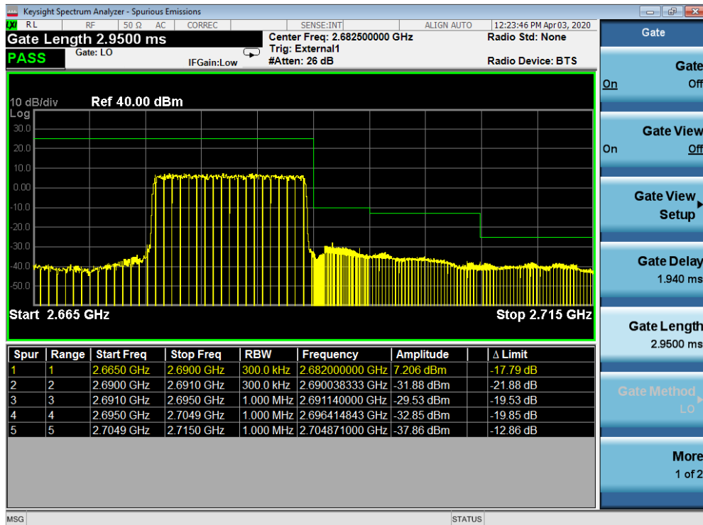
Plot 7-473. Upper ACP Plot (Band 41 - 15MHz QPSK - Full RB Configuration)
