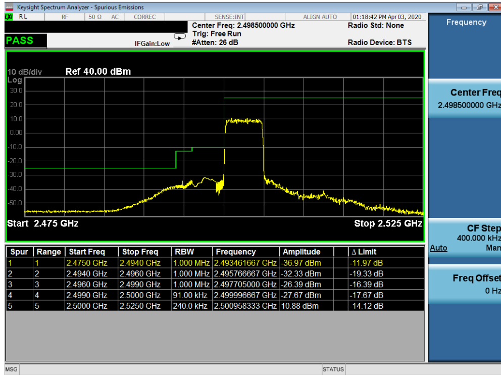
Plot 7-452. Lower ACP Plot (Band 7 - 5MHz QPSK - Full RB Configuration)
