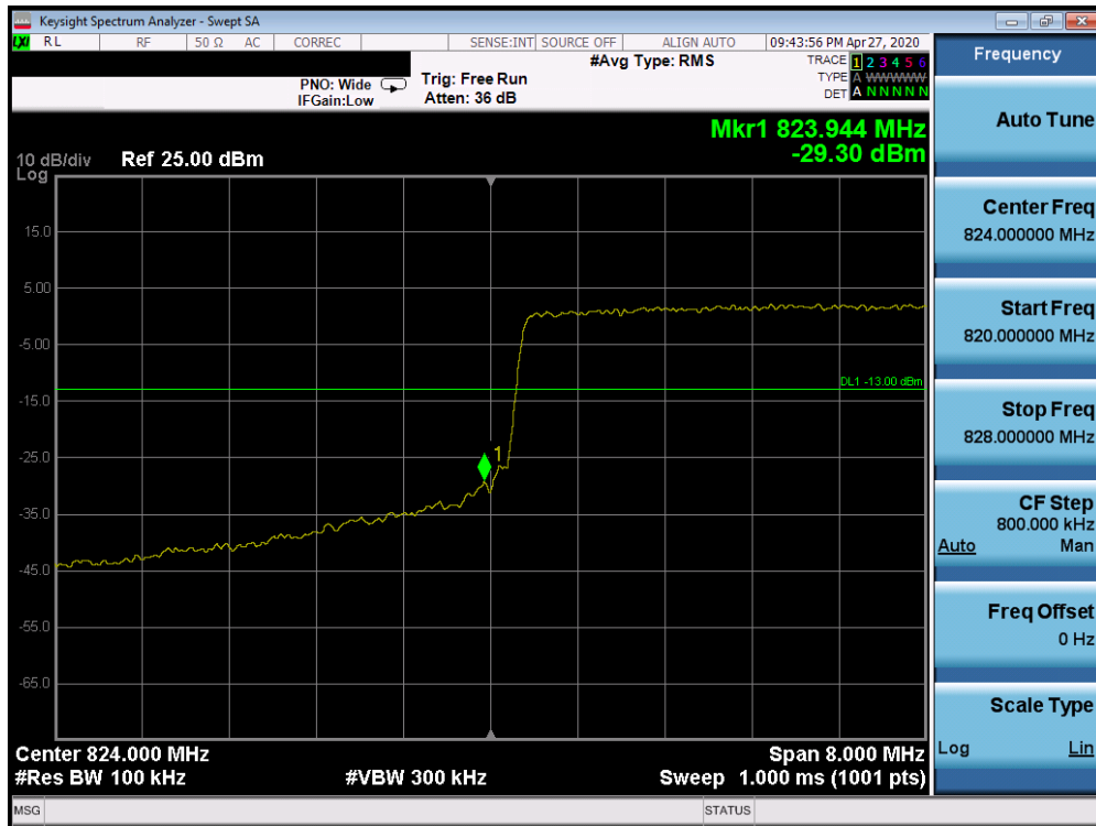
Plot 7-486. Lower 5G sub6 Band Edge Plot (5G sub6 n5 – 10MHz QPSK - Full RB Configuration)
