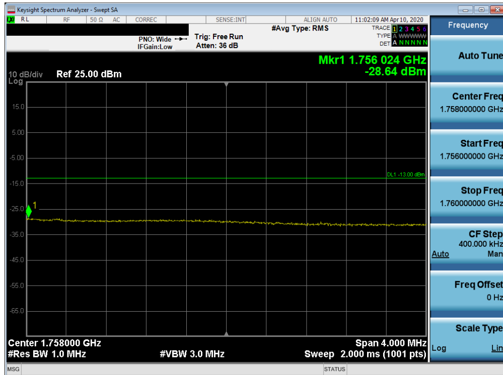
Plot 7-399. Upper Extended Band Edge Plot (Band 4 - 15.0MHz QPSK - Full RB Configuration)
