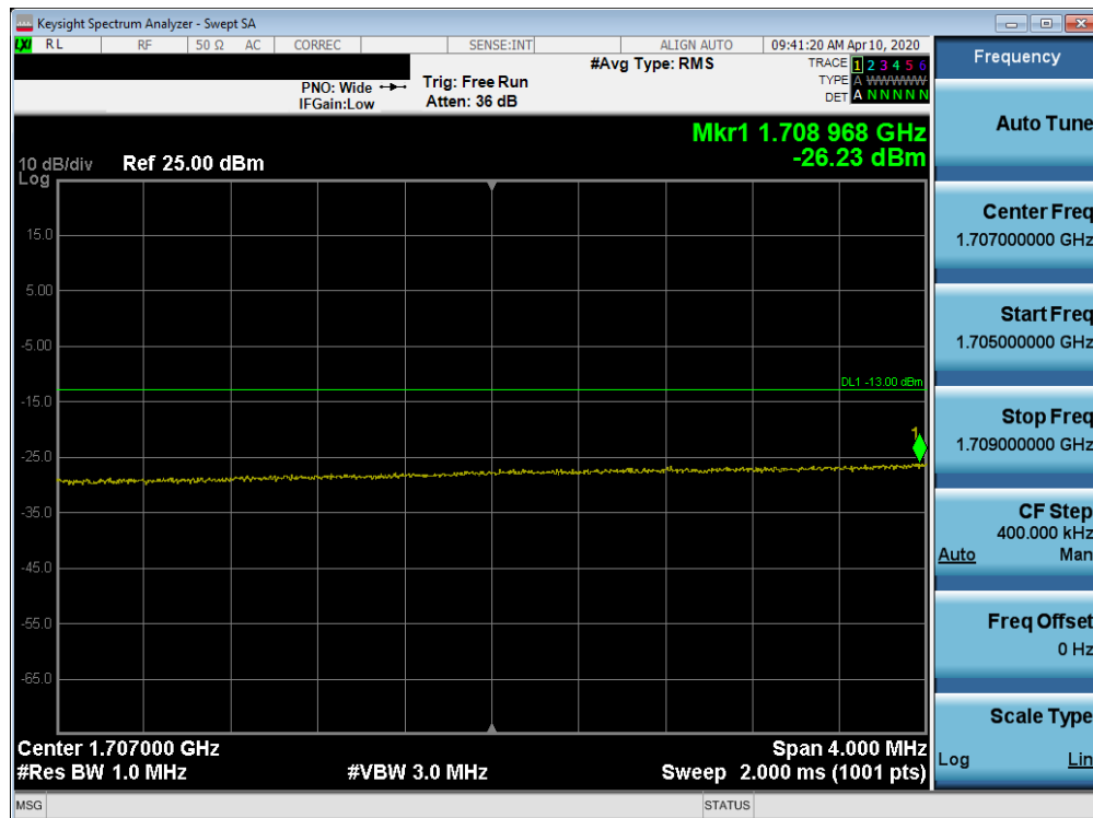
Plot 7-397. Lower Extended Band Edge Plot (Band 66/4 - 15.0MHz QPSK - Full RB Configuration)
