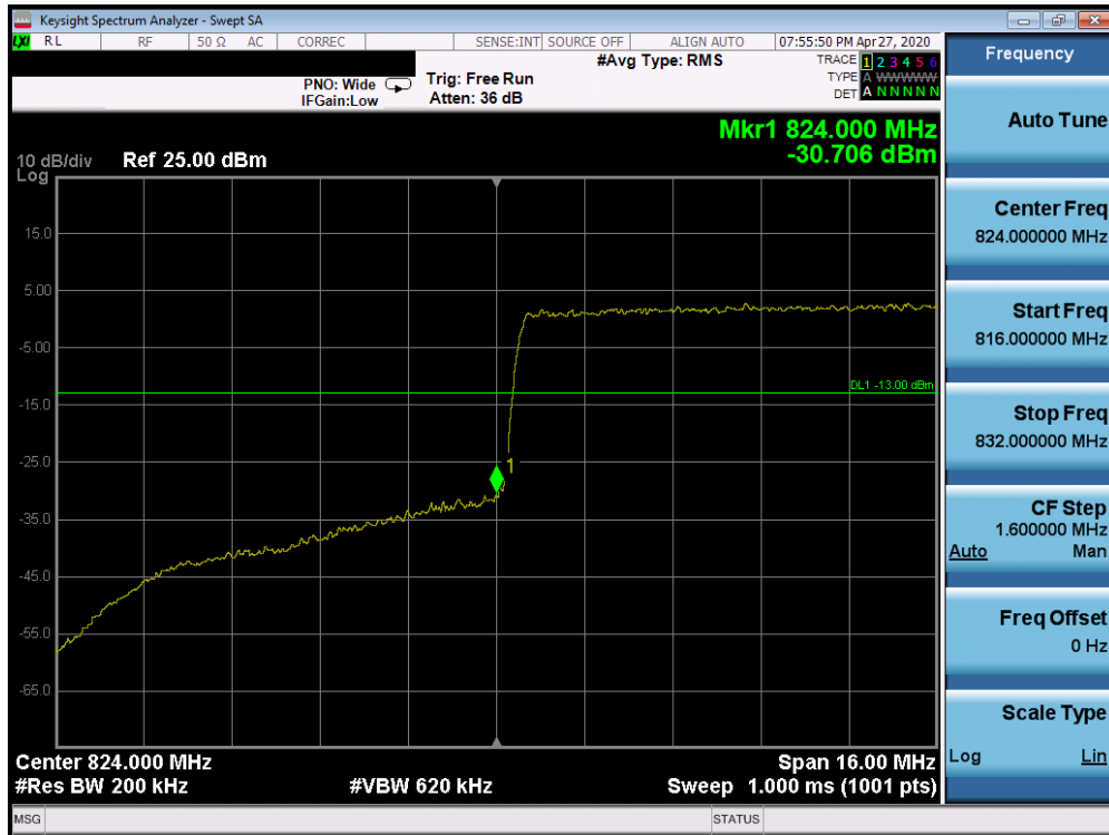
Plot 7-490. Lower 5G sub6 Band Edge Plot (5G sub6 n5 – 20MHz QPSK - Full RB Configuration)
