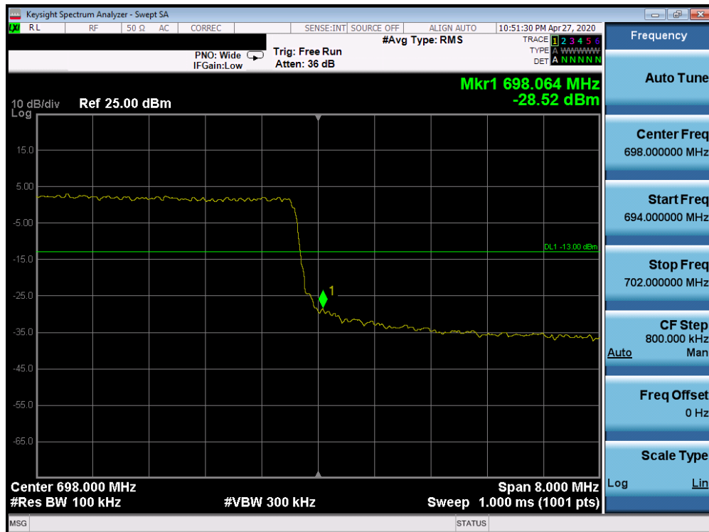
Plot 7-479. Upper 5G sub6 Band Edge Plot (5G sub6 n71 - 10.0MHz QPSK - Full RB Configuration)
