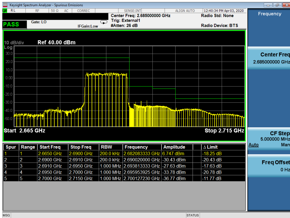
Plot 7-471. Upper ACP Plot (Band 41 - 10MHz QPSK - Full RB Configuration)
