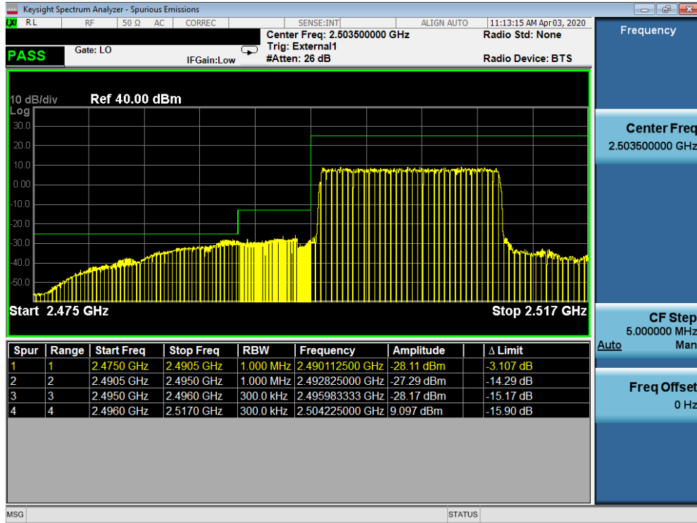
Plot 7-464. Lower ACP Plot (Band 41 - 15MHz QPSK - Full RB Configuration)
