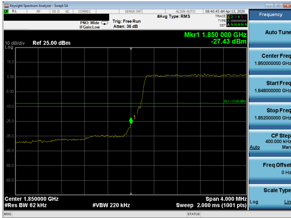
Plot 7-420. Lower Band Edge Plot (Band 25/2 - 5.0MHz QPSK - Full RB Configuration)
