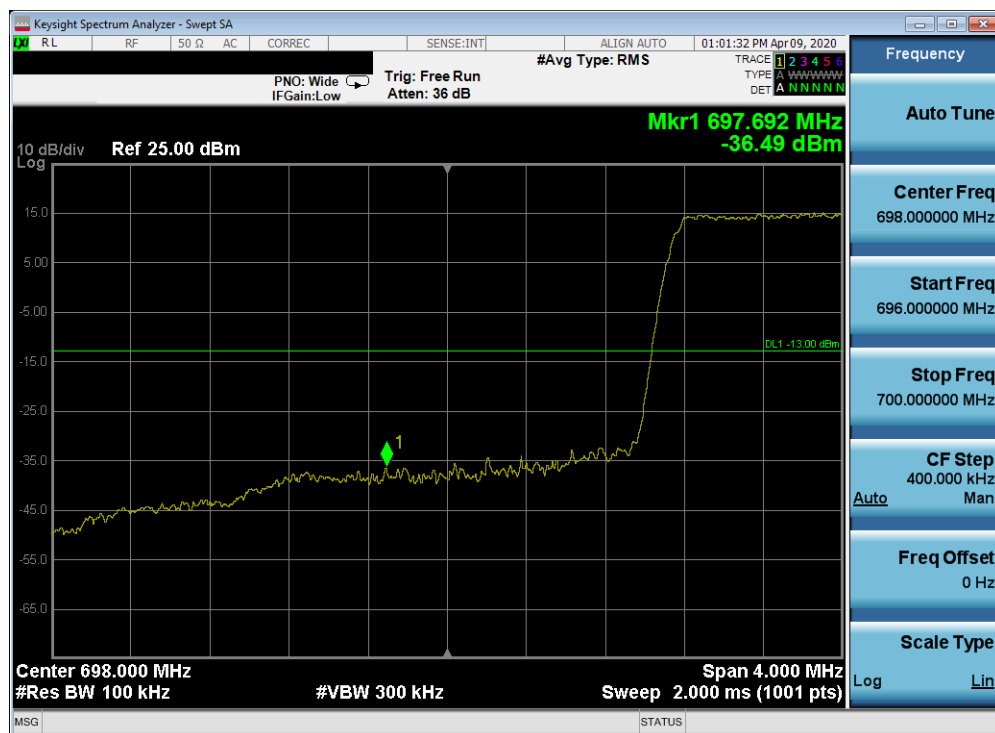
Plot 7-346. Lower Band Edge Plot (Band 12 - 1.4MHz QPSK - Full RB Configuration)
