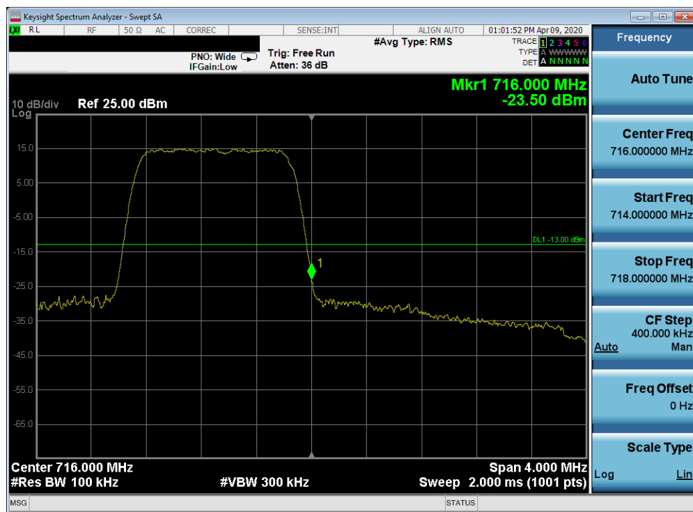
Plot 7-347. Upper Band Edge Plot (Band 12 - 1.4MHz QPSK - Full RB Configuration)
