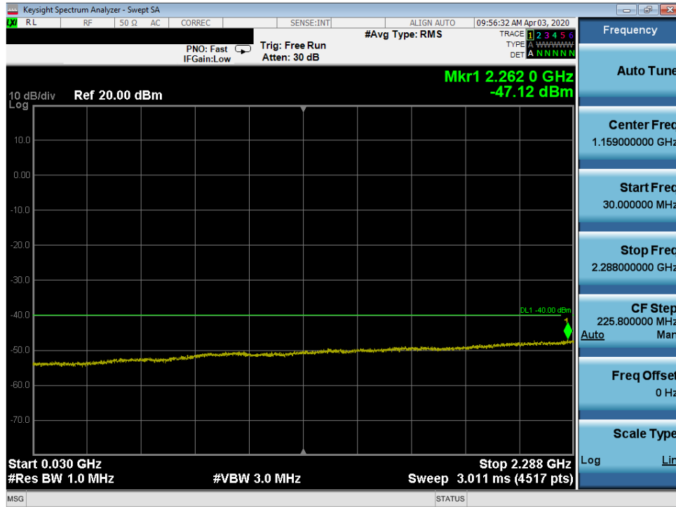
Plot 7-272. Conducted Spurious Plot (Band 30 - 10.0MHz QPSK - RB Size 1, RB Offset 0)
