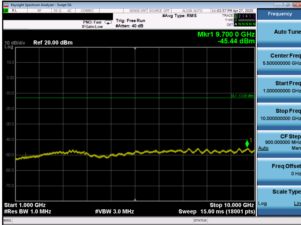
Plot 7-301. Conducted Spurious Plot (5G sub6 n71 - 5.0MHz QPSK - RB Size 1, RB Offset 0 - High Channel)
