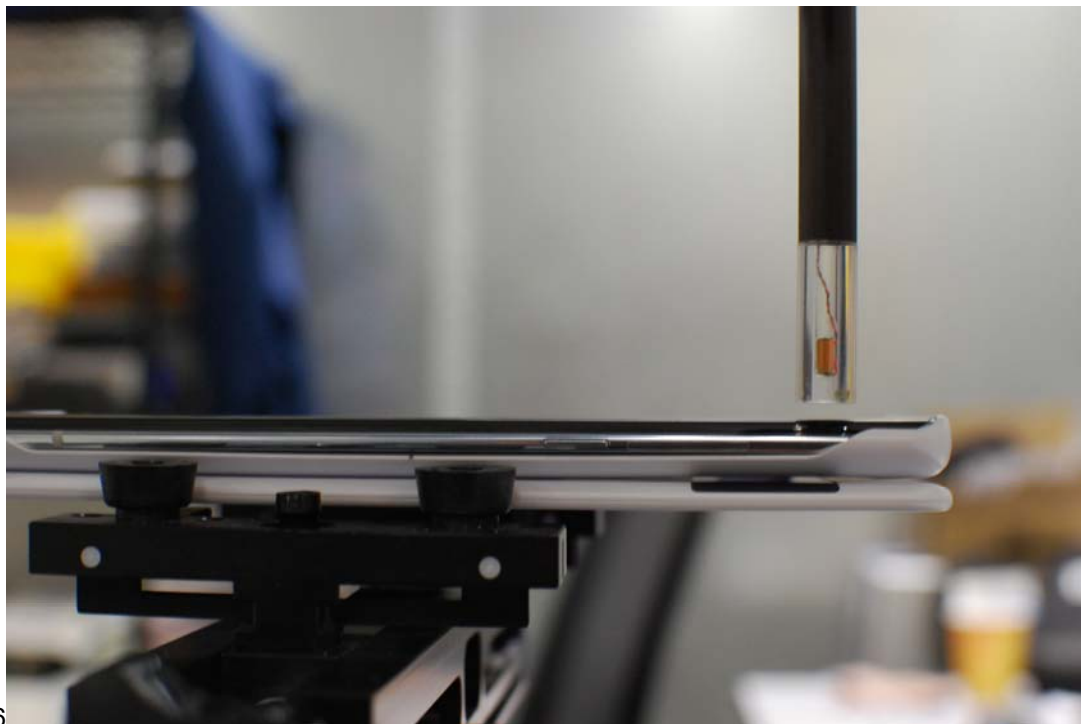
Figure 16-4 Test Setup for Wireless Device with Dual Display Cover - Open
