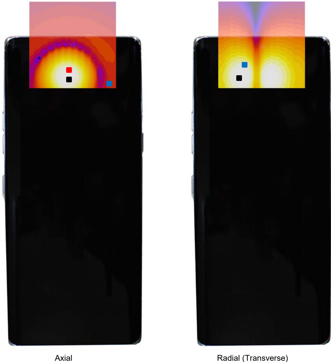
Figure 16-7 T-Coil Scan Overlay Magnetic Field Distributions
