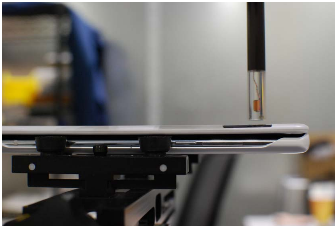
Figure 16-5 Test Setup for Wireless Device with Dual Display Cover - Closed
