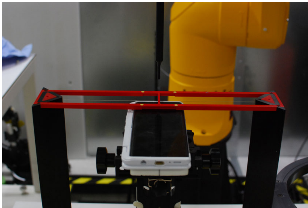
Figure 18-3 Ear Reference Point HAC Phantom Alignment – Dual Display Open
