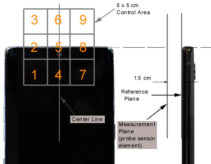
Figure 18-5 5x5 Scan grid above WD
