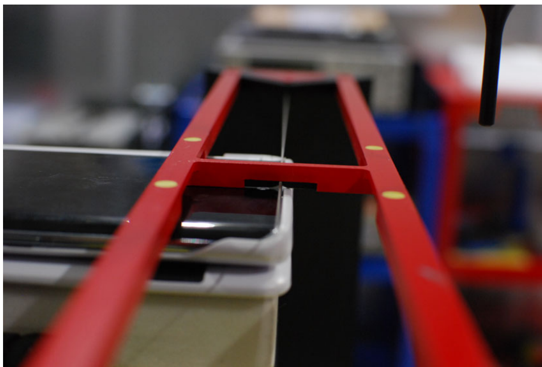
Figure 18-4 HAC Phantom Plane Alignment – Dual Display Open
