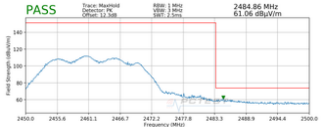
Plot 7-38. Radiated Restricted Upper Band Edge Measurement CDD (Peak)
