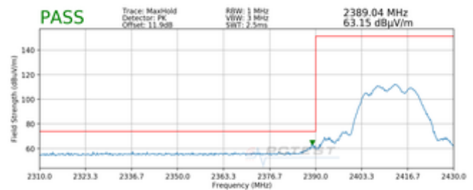
Plot 7-28. Radiated Restricted Lower Band Edge Measurement CDD (Peak)
