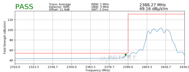
Plot 7-27. Radiated Restricted Lower Band Edge Measurement CDD (Average)
