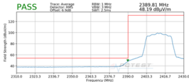
Plot 7-1. Radiated Restricted Lower Band Edge Measurement SISO ANT1 (Average)
