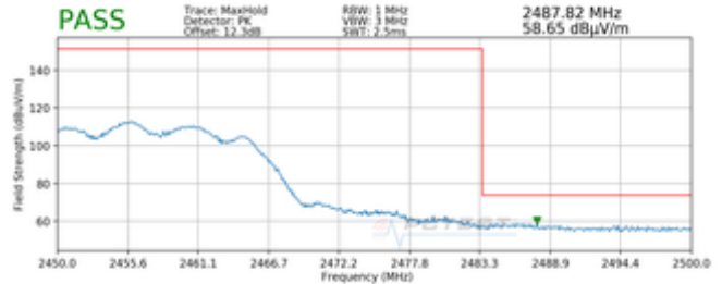
Plot 7-36. Radiated Restricted Upper Band Edge Measurement CDD (Peak)
