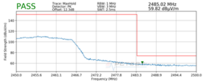
Plot 7-22. Radiated Restricted Upper Band Edge Measurement MIMO (Peak)
