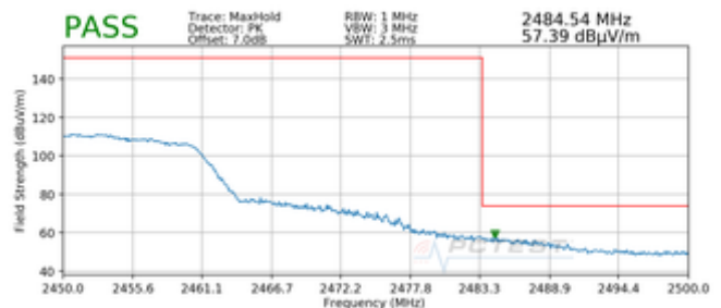
Plot 7-8. Radiated Restricted Upper Band Edge Measurement SISO ANT1 (Peak)
