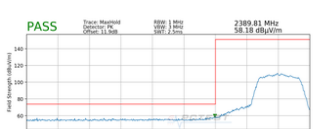
Plot 7-16. Radiated Restricted Lower Band Edge Measurement MIMO (Peak)
