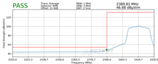
Plot 7-15. Radiated Restricted Lower Band Edge Measurement MIMO (Average)
