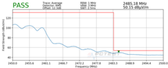
Plot 7-33. Radiated Restricted Upper Band Edge Measurement CDD (Average)
