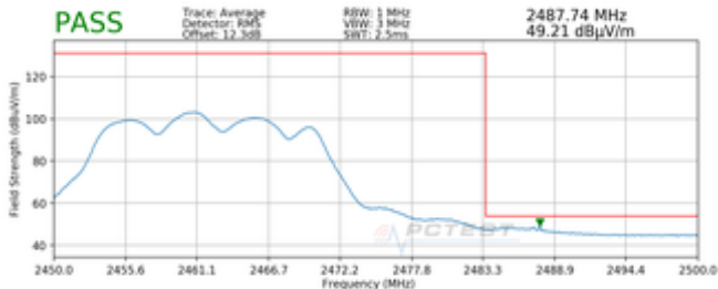
Plot 7-37. Radiated Restricted Upper Band Edge Measurement CDD (Average)
