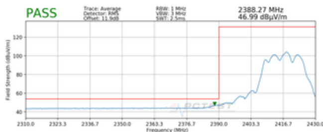
Plot 7-29. Radiated Restricted Lower Band Edge Measurement CDD (Average)
