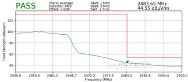
Plot 7-9. Radiated Restricted Upper Band Edge Measurement SISO ANT1 (Average)
