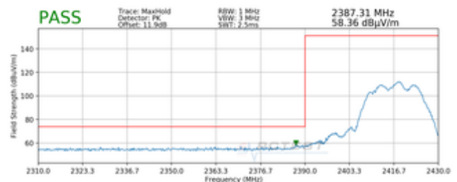
Plot 7-30. Radiated Restricted Lower Band Edge Measurement CDD (Peak)
