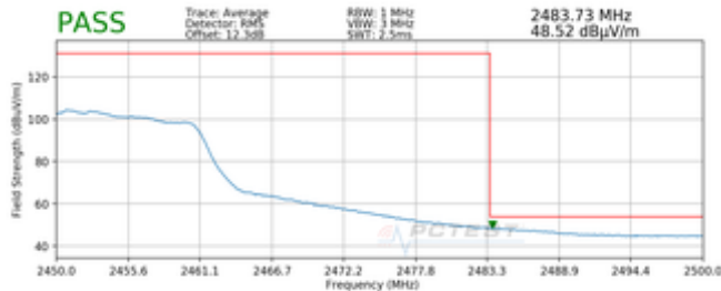
Plot 7-19. Radiated Restricted Upper Band Edge Measurement MIMO (Average)
