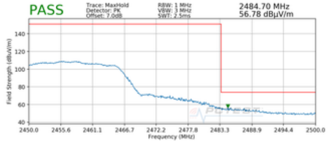
Plot 7-10. Radiated Restricted Upper Band Edge Measurement SISO ANT1 (Peak)
