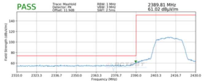
Plot 7-14. Radiated Restricted Lower Band Edge Measurement MIMO (Peak)
