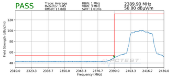
Plot 7-25. Radiated Restricted Lower Band Edge Measurement MIMO (Average) Dual Display Cover
