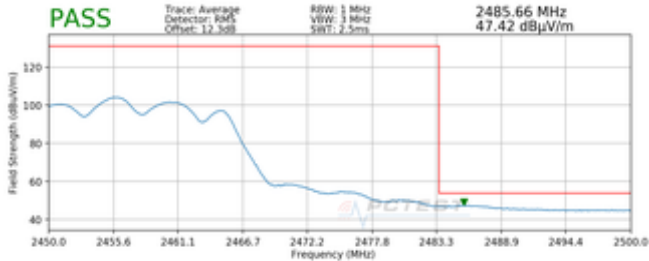
Plot 7-35. Radiated Restricted Upper Band Edge Measurement CDD (Average)
