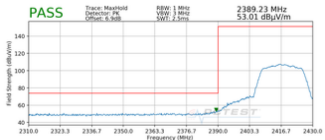
Plot 7-4. Radiated Restricted Lower Band Edge Measurement SISO ANT1 (Peak)
