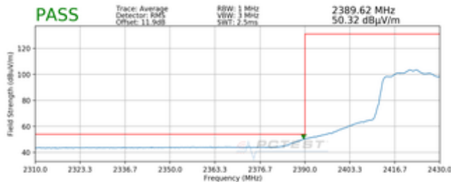
Plot 7-17. Radiated Restricted Upper Band Edge Measurement MIMO (Average)
