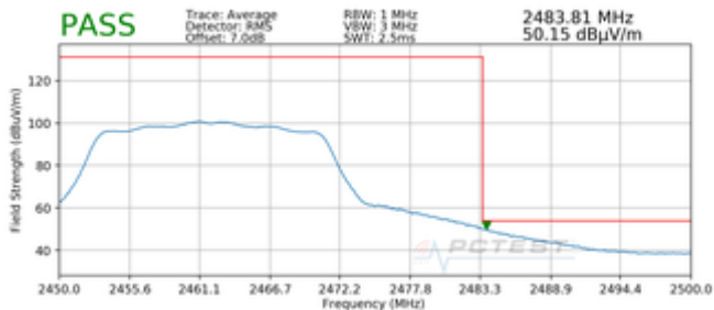
Plot 7-11. Radiated Restricted Upper Band Edge Measurement SISO ANT1 (Average)
