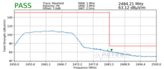
Plot 7-12. Radiated Restricted Upper Band Edge Measurement SISO ANT1 (Peak)
