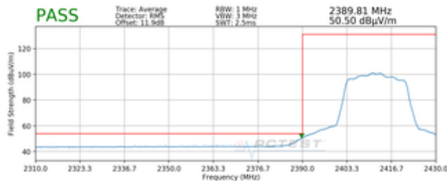
Plot 7-13. Radiated Restricted Lower Band Edge Measurement MIMO (Average)
