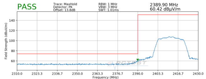
Plot 7-2. Radiated Restricted Lower Band Edge Measurement SISO ANT1 (Peak)
