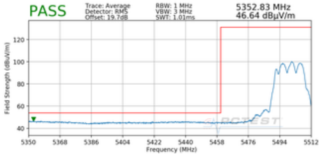
Plot 7-26. Radiated Lower Band Edge Plot CDD (Average – UNII Band 2C)
