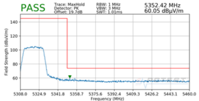
Plot 7-34. Radiated Upper Band Edge Plot MIMO (Peak – UNII Band 2A)
