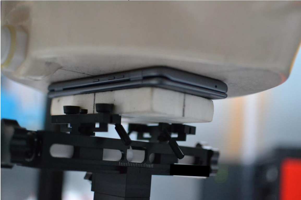
SAR Test Setup Photo 16 – Back Side with Dual Display Accessory Position #1 at 0 mm
