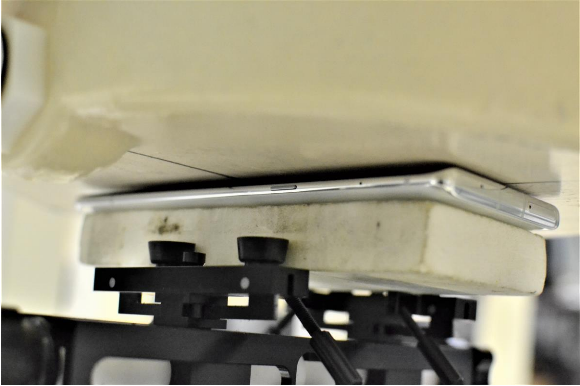
SAR Test Setup Photo 19 – Front Side at 1 mm
