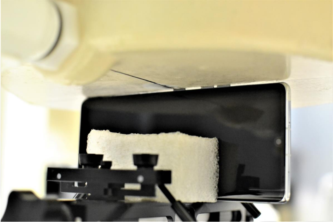
SAR Test Setup Photo 37 – Left Edge at 0 mm
