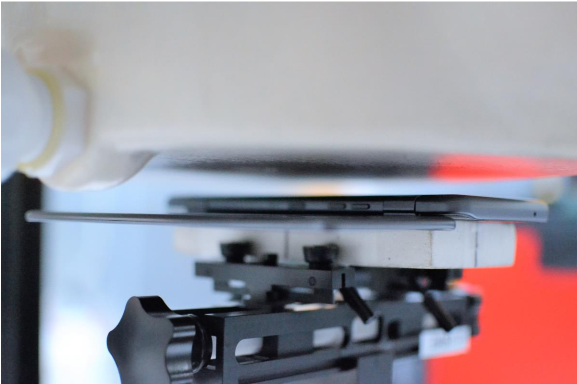
SAR Test Setup Photo 12 – Back Side with Dual Display Accessory Position #2 at 10 mm
