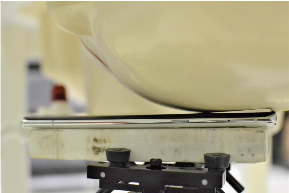
SAR Test Setup Photo 6 – Left Cheek
