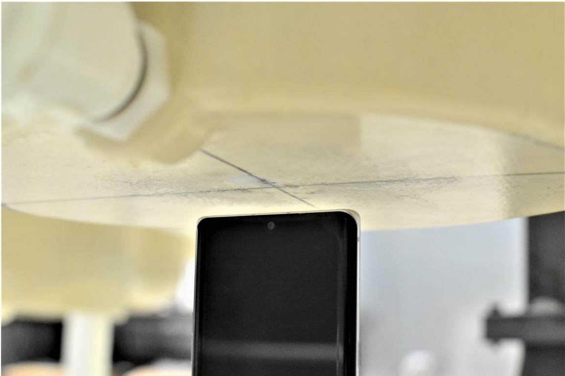
SAR Test Setup Photo 22 – Top Edge at 10 mm
