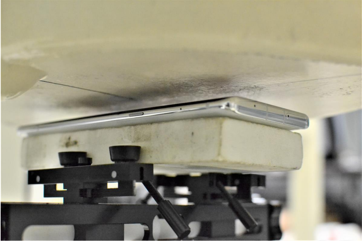
SAR Test Setup Photo 17 – Front Side at 10 mm
