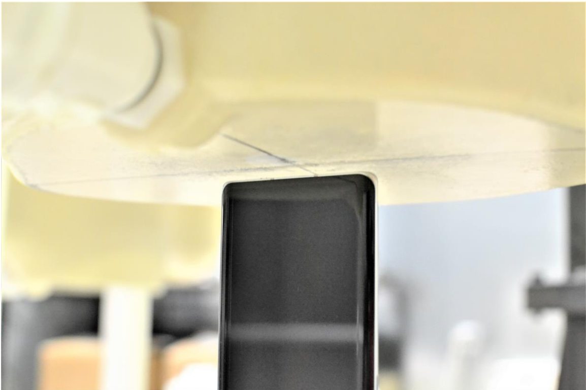
SAR Test Setup Photo 26 – Bottom Edge at 4 mm
