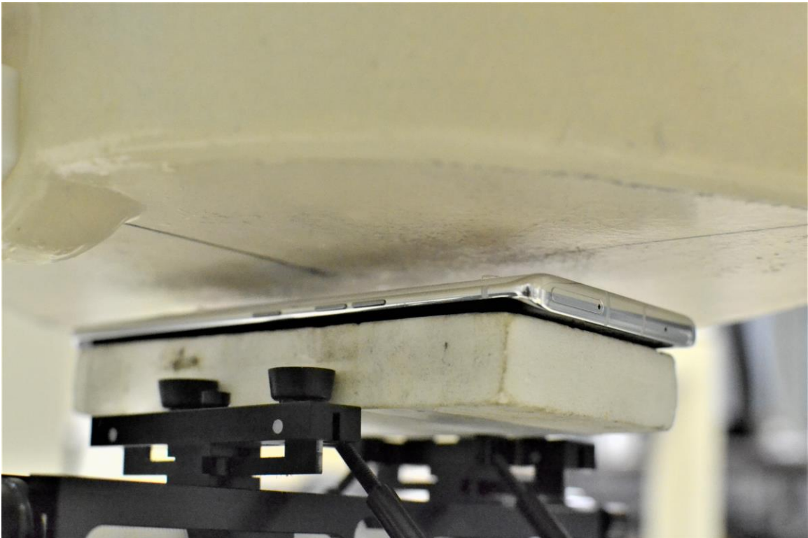
SAR Test Setup Photo 10 – Back Side at 10 mm
