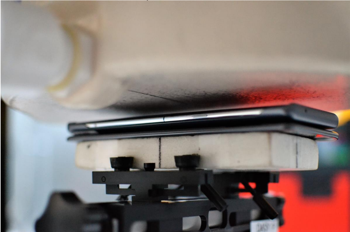
SAR Test Setup Photo 18 – Front Side with Dual Display Accessory Position #3 at 10 mm
