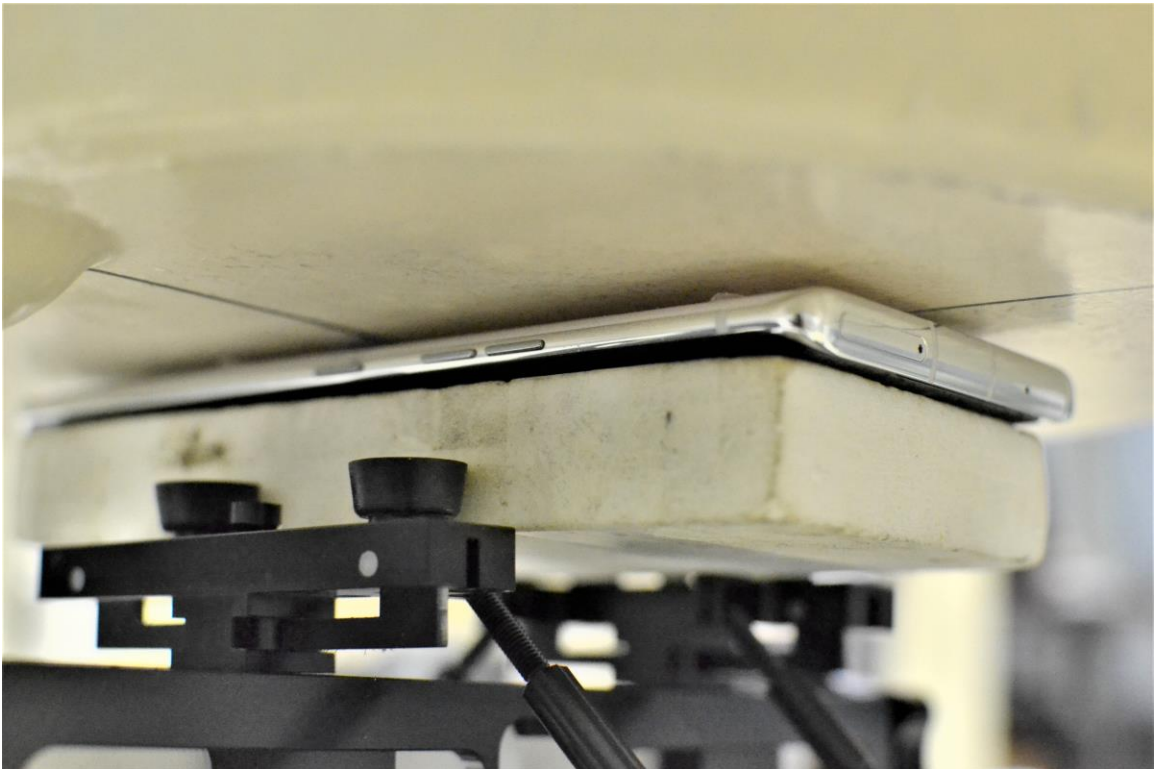
SAR Test Setup Photo 14 – Back Side at 2 mm
