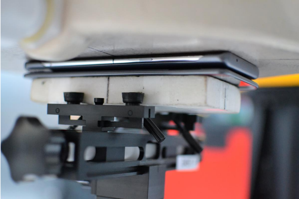
SAR Test Setup Photo 21 – Front Side with Dual Display Accessory Position #3 at 0 mm
