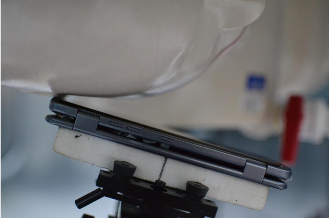
SAR Test Setup Photo 5 – Right Tilt with Dual Display Accessory Position #3
