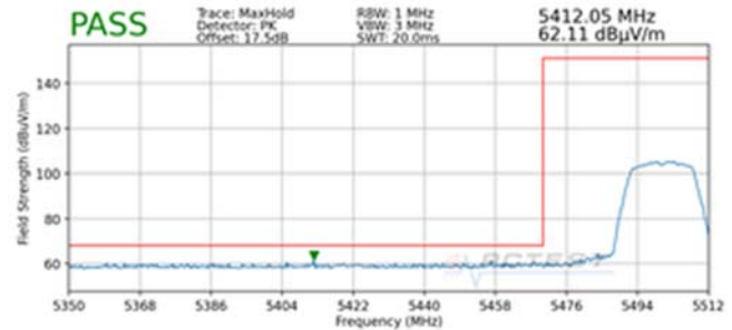
Plot 7-204. Radiated Lower Band Edge Plot SISO ANT2 (Peak – UNII Band 2C)
