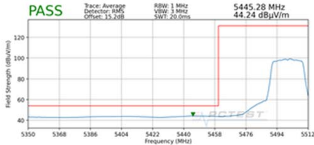
Plot 7-224. Radiated Lower Band Edge Plot MIMO (Average – UNII Band 2C)
