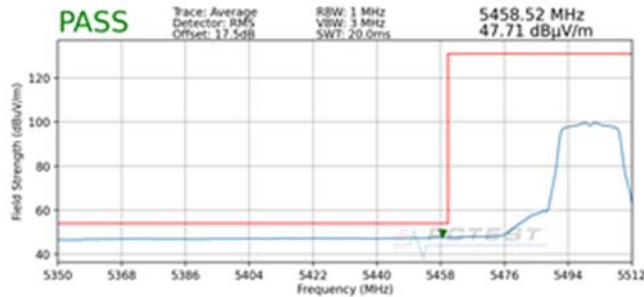
Plot 7-182. Radiated Lower Band Edge Plot SISO ANT1 (Average – UNII Band 2C)
