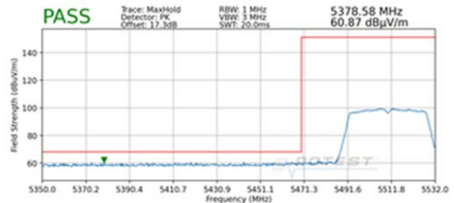
Plot 7-211. Radiated Lower Band Edge Plot SISO ANT2 (Peak – UNII Band 2C)
