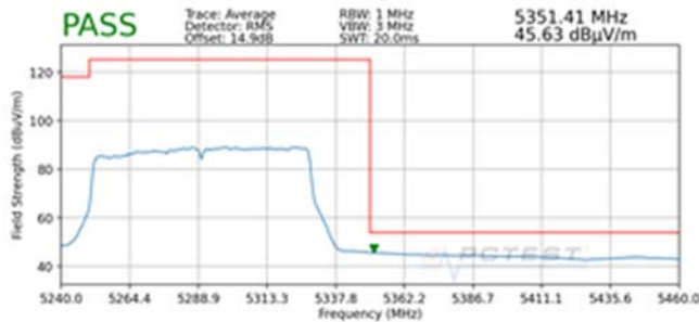
Plot 7-238. Radiated Upper Band Edge Plot MIMO (Average – UNII Band 2A)
