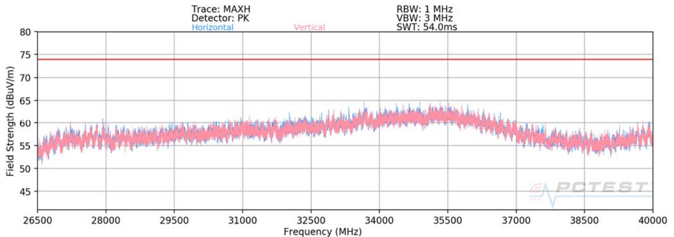
Plot 7-174. Radiated Spurious Plot 26.5GHz - 40GHz MIMO (802.11a)
