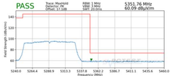
Plot 7-216. Radiated Upper Band Edge Plot SISO ANT2 (Peak – UNII Band 2A)
