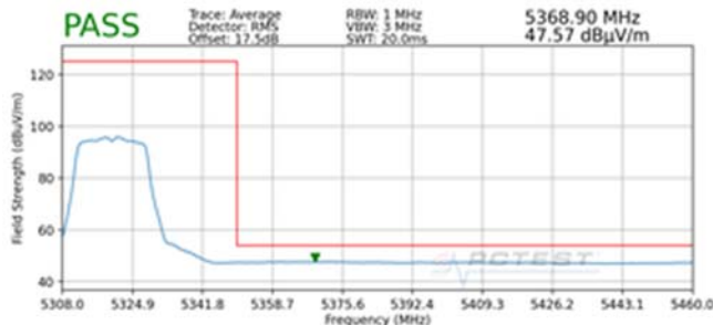
Plot 7-201. Radiated Upper Band Edge Plot SISO ANT2 (Average – UNII Band 2A)
