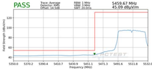
Plot 7-233. Radiated Lower Band Edge Plot MIMO (Average – UNII Band 2C)
