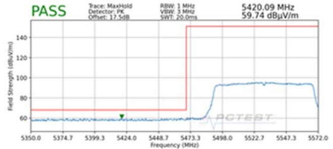
Plot 7-218. Radiated Lower Band Edge Plot SISO ANT2 (Peak – UNII Band 2C)
