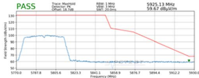
Plot 7-191. Radiated Upper Band Edge Plot SISO ANT1 (Peak – UNII Band 3)
