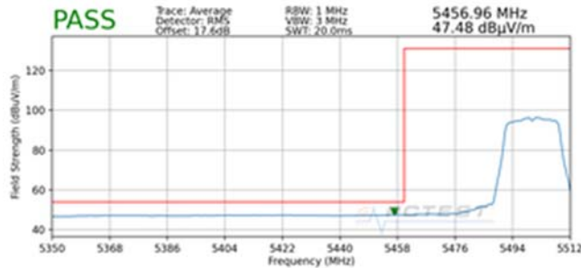
Plot 7-203. Radiated Lower Band Edge Plot SISO ANT2 (Average – UNII Band 2C)
