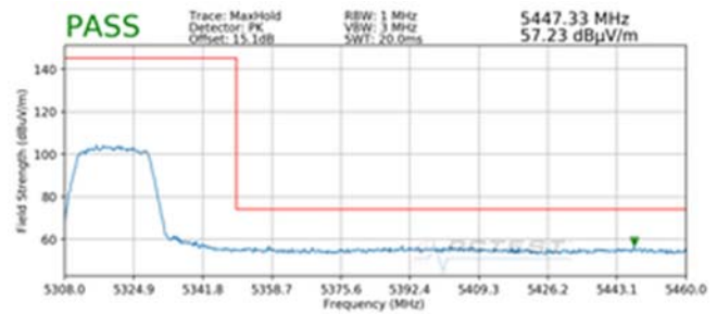
Plot 7-228. Radiated Upper Band Edge Plot MIMO (Peak – WCP)
