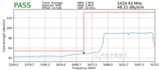
Plot 7-240. Radiated Lower Band Edge Plot MIMO (Average – UNII Band 2C)
