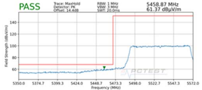
Plot 7-241. Radiated Lower Band Edge Plot MIMO (Peak – UNII Band 2C)
