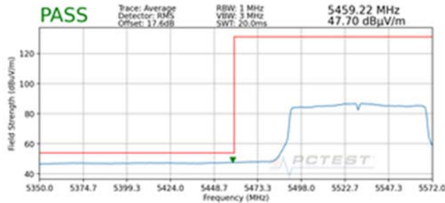
Plot 7-217. Radiated Lower Band Edge Plot SISO ANT2 (Average – UNII Band 2C)
