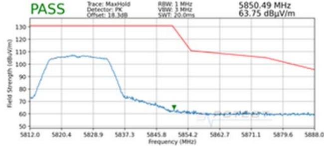
Plot 7-205. Radiated Upper Band Edge Plot SISO ANT2 (Peak – UNII Band 3)
