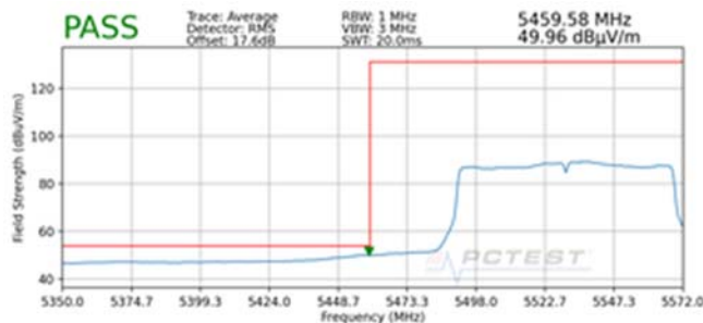
Plot 7-196. Radiated Lower Band Edge Plot SISO ANT1 (Average – UNII Band 2C)
