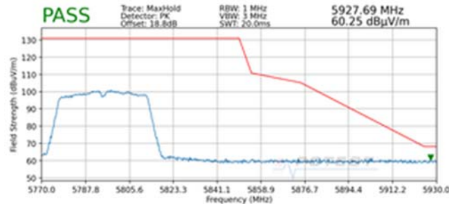
Plot 7-212. Radiated Upper Band Edge Plot SISO ANT2 (Peak – UNII Band 3)
