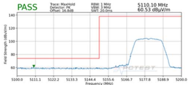
Plot 7-200. Radiated Lower Band Edge Plot SISO ANT2 (Peak – UNII Band 1)
