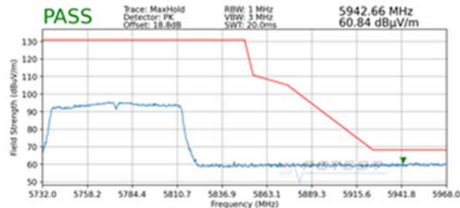
Plot 7-219. Radiated Upper Band Edge Plot SISO ANT2 (Peak – UNII Band 3)
