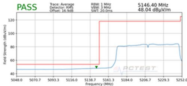
Plot 7-192. Radiated Lower Band Edge Plot SISO ANT1 (Average – UNII Band 1)
