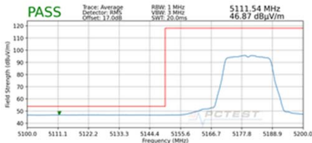
Plot 7-199. Radiated Lower Band Edge Plot SISO ANT2 (Average – UNII Band 1)
