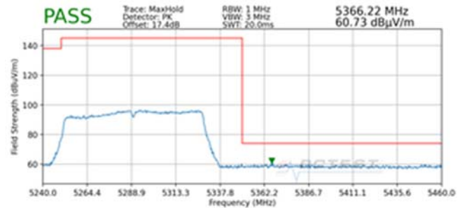
Plot 7-195. Radiated Upper Band Edge Plot SISO ANT1 (Peak – UNII Band 2A)
