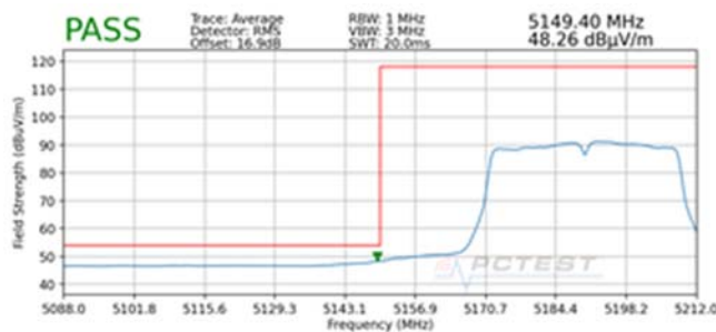
Plot 7-206. Radiated Lower Band Edge Plot SISO ANT2 (Average – UNII Band 1)
