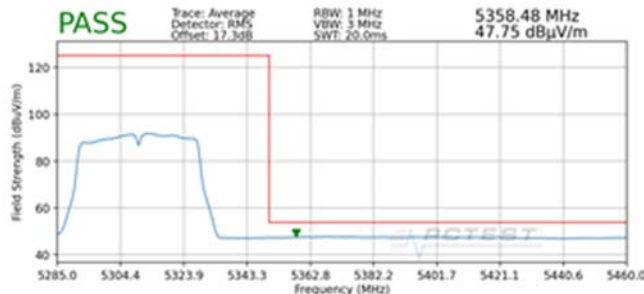
Plot 7-187. Radiated Upper Band Edge Plot SISO ANT1 (Average – UNII Band 2A)
