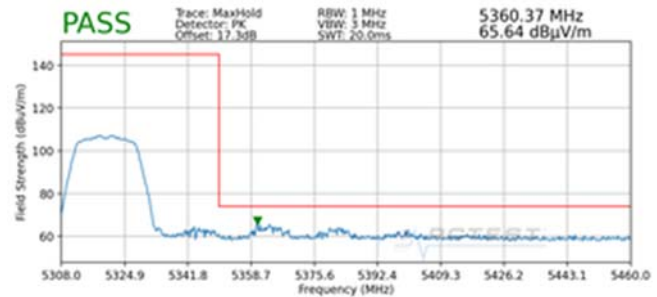
Plot 7-181. Radiated Upper Band Edge Plot SISO ANT1 (Peak – UNII Band 2A)
