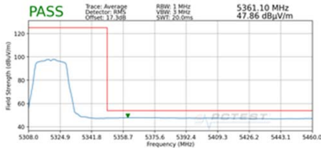
Plot 7-180. Radiated Upper Band Edge Plot SISO ANT1 (Average – UNII Band 2A)
