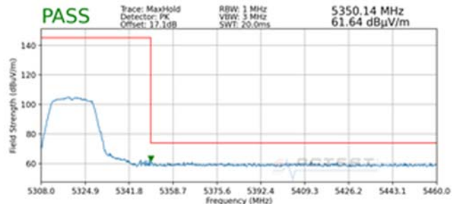
Plot 7-202. Radiated Upper Band Edge Plot SISO ANT2 (Peak – UNII Band 2A)
