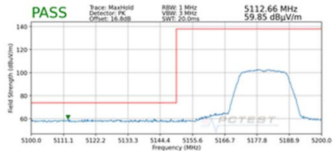
Plot 7-179. Radiated Lower Band Edge Plot SISO ANT1 (Peak – UNII Band 1)
