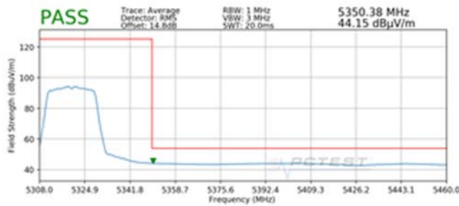
Plot 7-227. Radiated Upper Band Edge Plot MIMO (Average – WCP)
