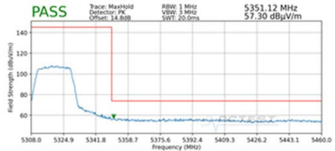
Plot 7-223. Radiated Upper Band Edge Plot MIMO (Peak – UNII Band 2A)
