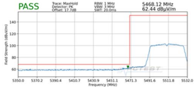
Plot 7-190. Radiated Lower Band Edge Plot SISO ANT1 (Peak – UNII Band 2C)
