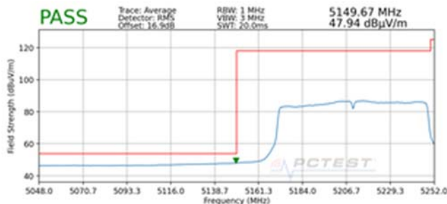
Plot 7-213. Radiated Lower Band Edge Plot SISO ANT2 (Average – UNII Band 1)
