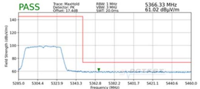
Plot 7-209. Radiated Upper Band Edge Plot SISO ANT2 (Peak – UNII Band 2A)
