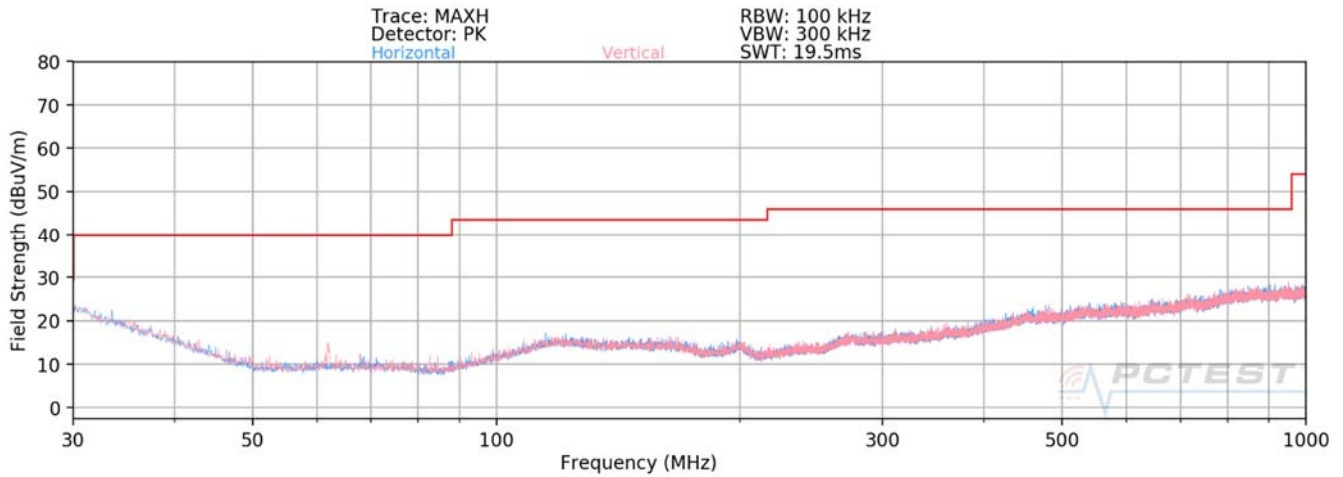
Plot 7-243. Radiated Spurious Plot below 1GHz MIMO (802.11a – U3 Ch. 157)
