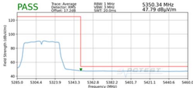
Plot 7-208. Radiated Upper Band Edge Plot SISO ANT2 (Average – UNII Band 2A)
