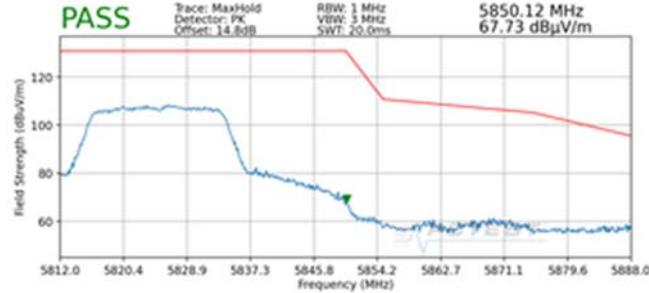
Plot 7-226. Radiated Upper Band Edge Plot MIMO (Peak – UNII Band 3)
