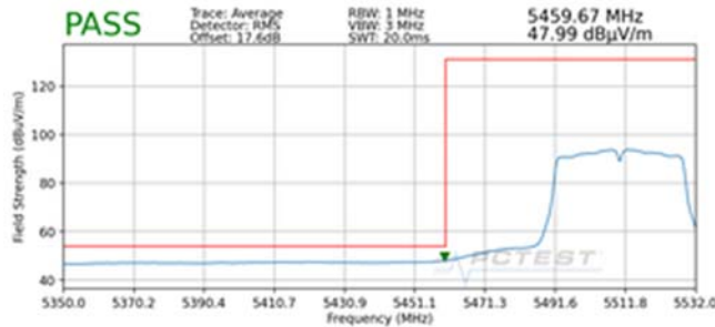
Plot 7-189. Radiated Lower Band Edge Plot SISO ANT1 (Average – UNII Band 2C)
