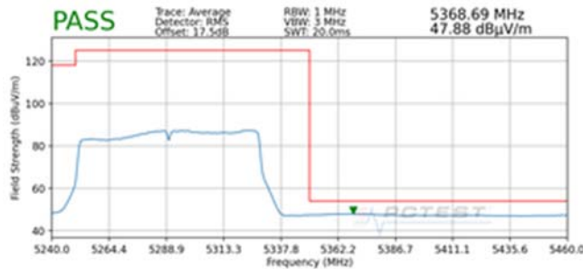
Plot 7-194. Radiated Upper Band Edge Plot SISO ANT1 (Average – UNII Band 2A)
