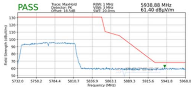
Plot 7-198. Radiated Upper Band Edge Plot SISO ANT1 (Peak – UNII Band 3)
