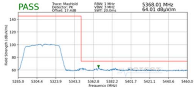
Plot 7-188. Radiated Upper Band Edge Plot SISO ANT1 (Peak – UNII Band 2A)
