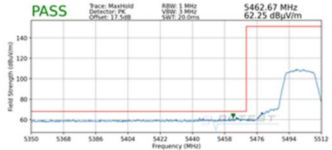
Plot 7-183. Radiated Lower Band Edge Plot SISO ANT1 (Peak – UNII Band 2C)
