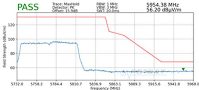
Plot 7-242. Radiated Upper Band Edge Plot MIMO (Peak – UNII Band 3)
