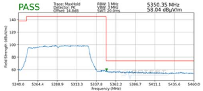
Plot 7-239. Radiated Upper Band Edge Plot MIMO (Peak – UNII Band 2A)
