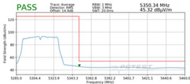
Plot 7-231. Radiated Upper Band Edge Plot MIMO (Average – UNII Band 2A)
