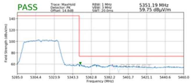
Plot 7-232. Radiated Upper Band Edge Plot MIMO (Peak – UNII Band 2A)
