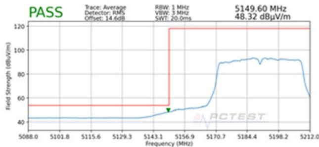
Plot 7-229. Radiated Lower Band Edge Plot MIMO (Average – UNII Band 1)
