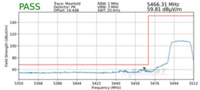
Plot 7-225. Radiated Lower Band Edge Plot MIMO (Peak – UNII Band 2C)
