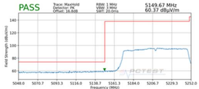
Plot 7-214. Radiated Lower Band Edge Plot SISO ANT2 (Peak – UNII Band 1)
