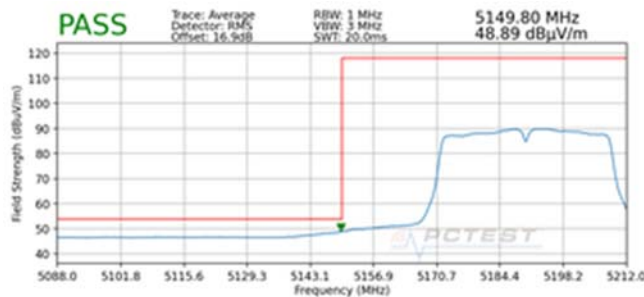
Plot 7-185. Radiated Lower Band Edge Plot SISO ANT1 (Average – UNII Band 1)
