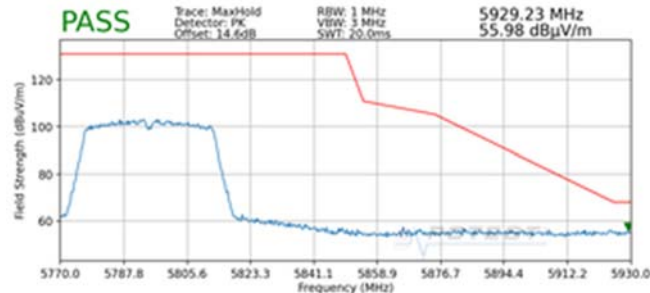
Plot 7-235. Radiated Upper Band Edge Plot MIMO (Peak – UNII Band 3)
