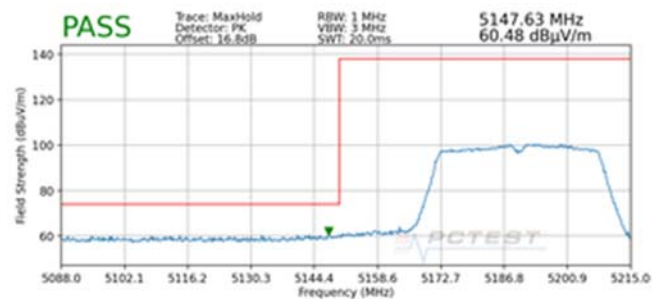
Plot 7-207. Radiated Lower Band Edge Plot SISO ANT2 (Peak – UNII Band 1)
