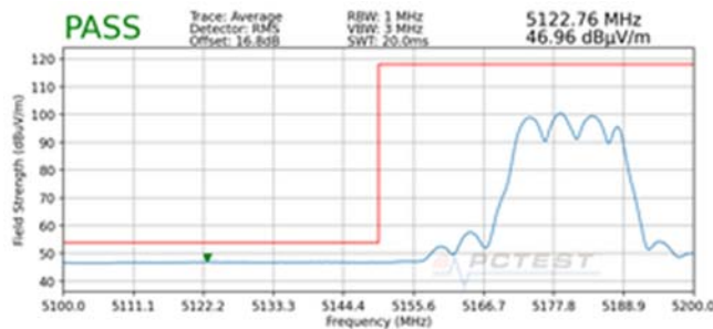
Plot 7-220. Radiated Lower Band Edge Plot MIMO (Average – UNII Band 1)
