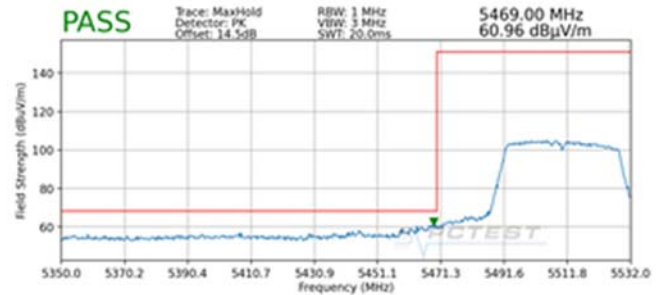
Plot 7-234. Radiated Lower Band Edge Plot MIMO (Peak – UNII Band 2C)
