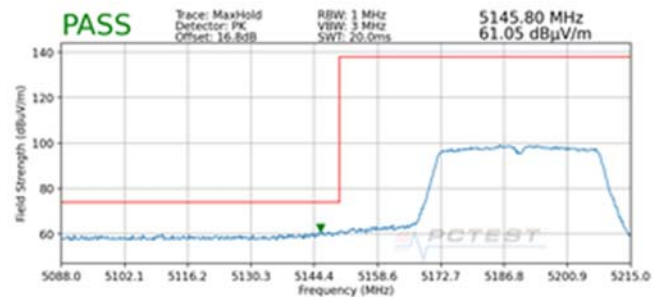
Plot 7-186. Radiated Lower Band Edge Plot SISO ANT1 (Peak – UNII Band 1)
