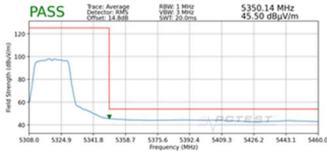
Plot 7-222. Radiated Upper Band Edge Plot MIMO (Average – UNII Band 2A)
