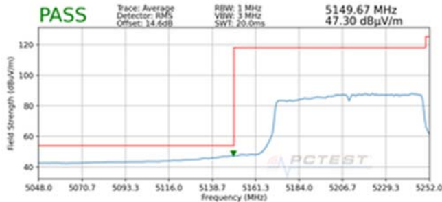
Plot 7-236. Radiated Lower Band Edge Plot MIMO (Average – UNII Band 1)
