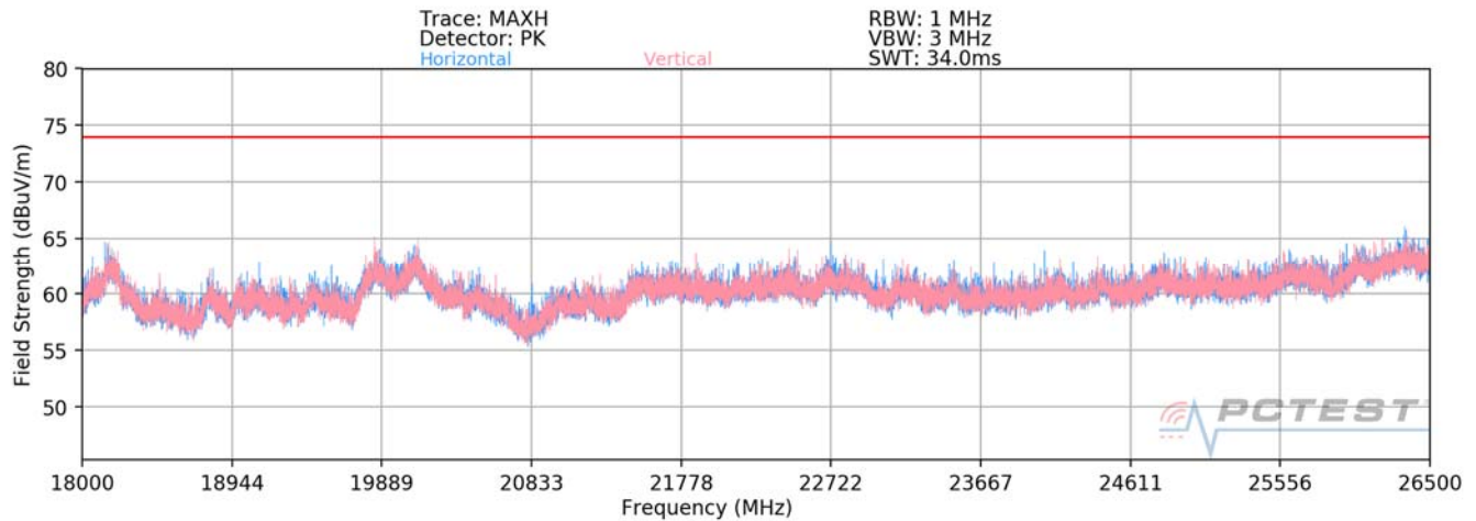
Plot 7-173. Radiated Spurious Plot above 18GHz - 26.5GHz MIMO (802.11a)
