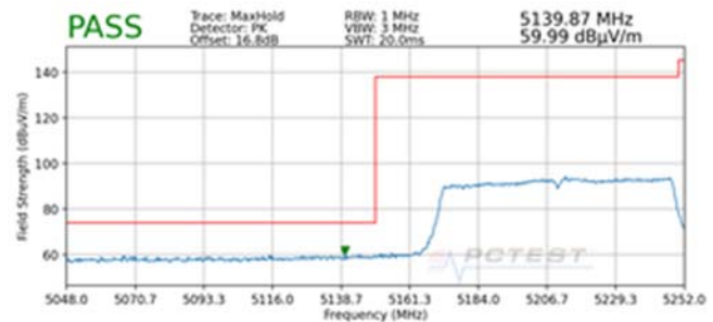
Plot 7-193. Radiated Lower Band Edge Plot SISO ANT1 (Peak – UNII Band 1)
