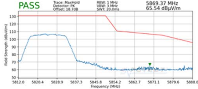
Plot 7-184. Radiated Upper Band Edge Plot SISO ANT1 (Peak – UNII Band 3)
