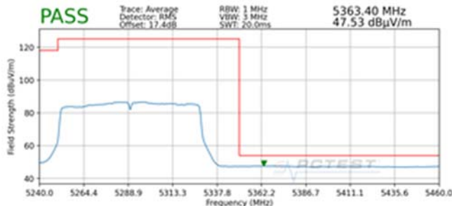
Plot 7-215. Radiated Upper Band Edge Plot SISO ANT2 (Average – UNII Band 2A)
