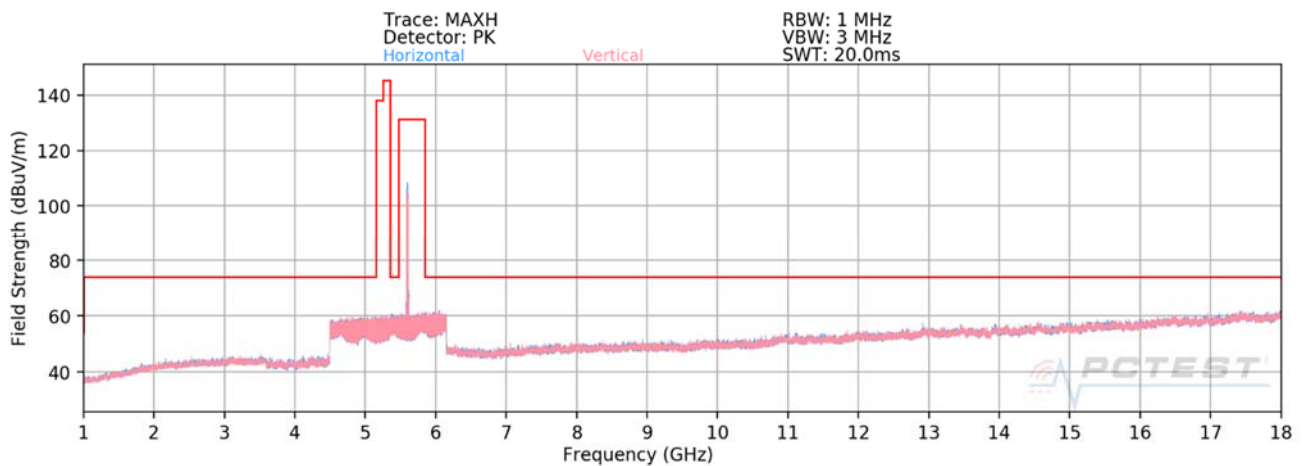
Plot 7-171. Radiated Spurious Plot above 1GHz MIMO (802.11a – U2C Ch. 116120)
