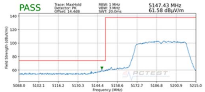
Plot 7-230. Radiated Lower Band Edge Plot MIMO (Peak – UNII Band 1)
