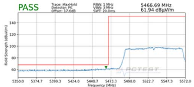
Plot 7-197. Radiated Lower Band Edge Plot SISO ANT1 (Peak – UNII Band 2C)
