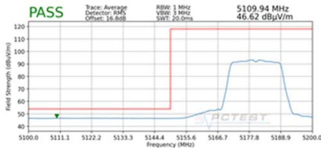
Plot 7-178. Radiated Lower Band Edge Plot SISO ANT1 (Average – UNII Band 1)
