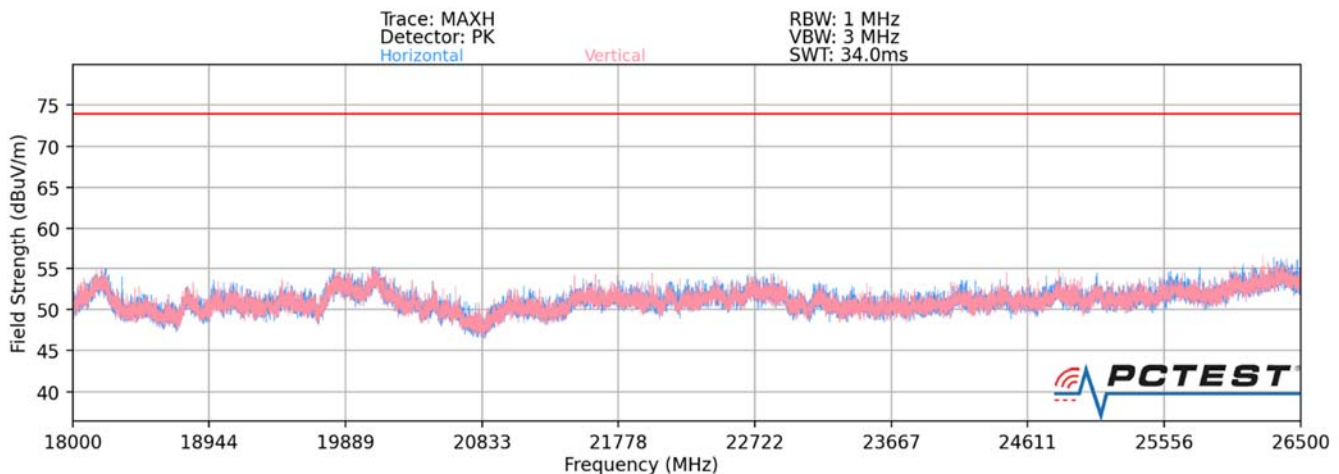
Plot 7-176. Radiated Spurious Plot above 18GHz (2.4GHz – 5GHz)
