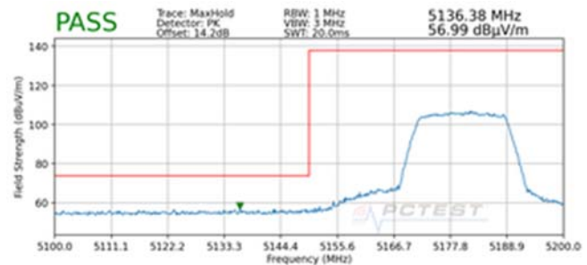
Plot 7-221. Radiated Lower Band Edge Plot MIMO (Peak – UNII Band 1)
