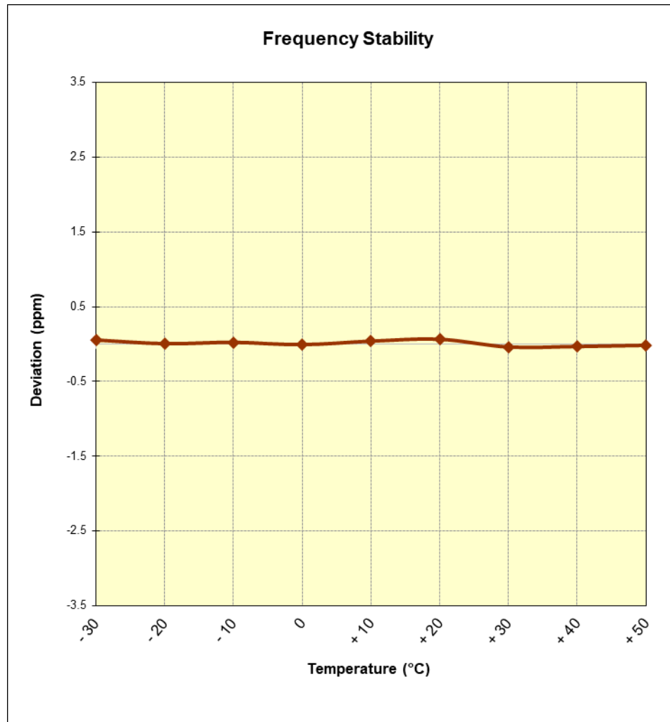
Figure 7-14. Frequency Stability Graph (PCS CDMA Mode – Ch. 600)
