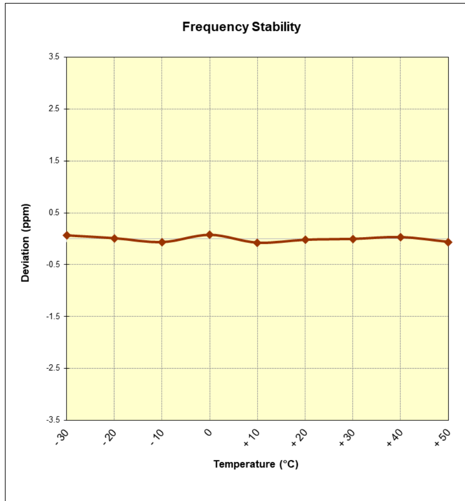
Figure 7-12. Frequency Stability Graph (AWS WCDMA Mode – Ch. 1413)
