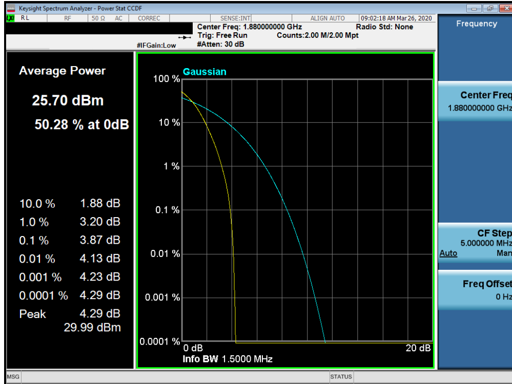
Plot 7-101. Peak-Average Ratio Plot (PCS CDMA Mode)
