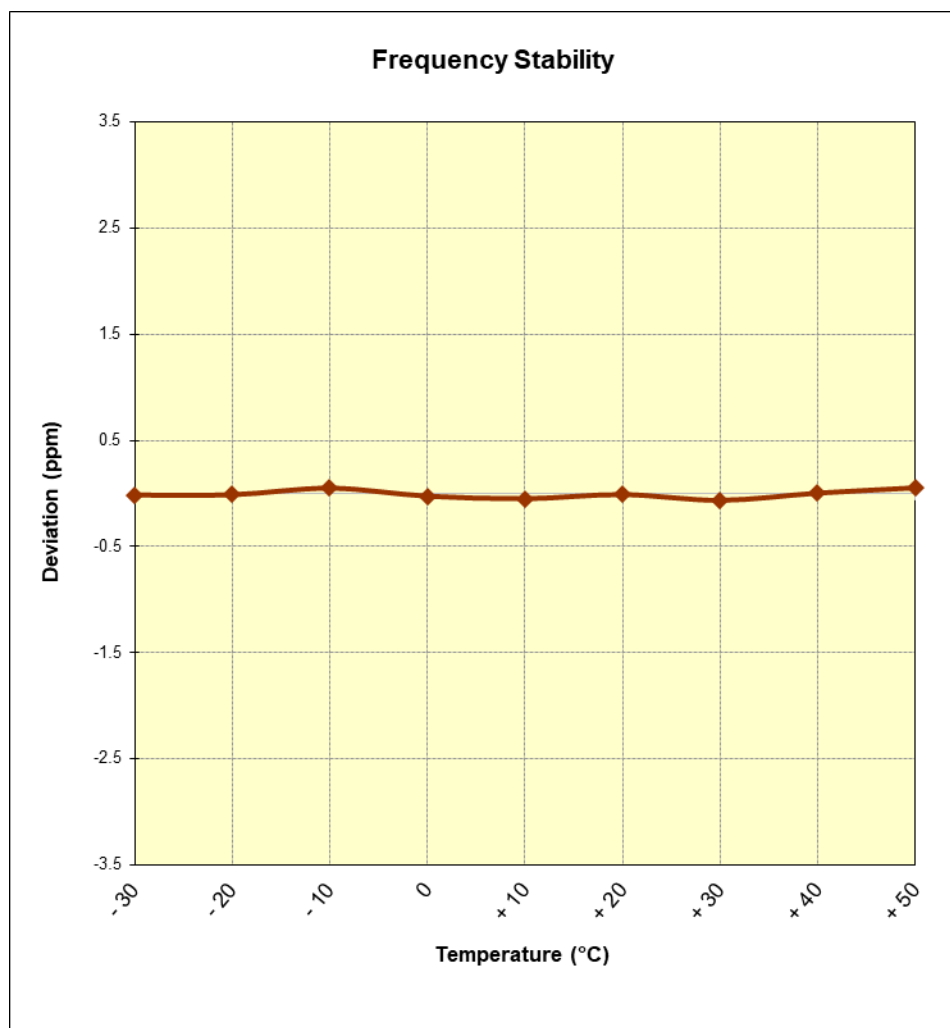
Figure 7-15. Frequency Stability Graph (PCS WCDMA Mode – Ch. 9400)
