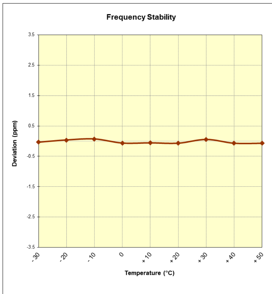
Figure 7-13. Frequency Stability Graph (PCS GPRS Mode – Ch. 661)
