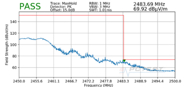
Plot 7-20. Radiated Restricted Upper Band Edge Measurement MIMO (Peak)
