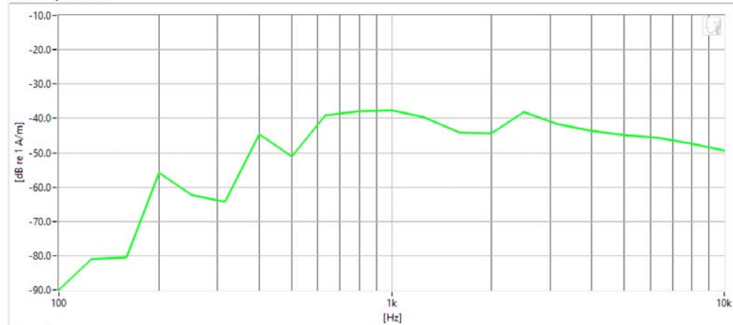
Noise Spectrum
