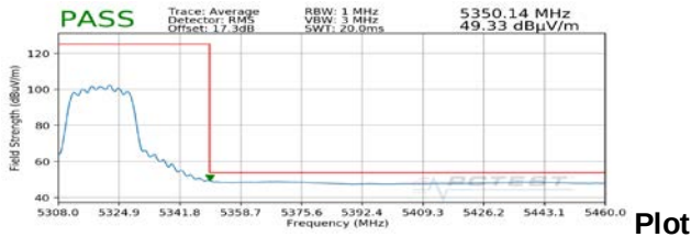
Plot 7-29. Radiated Upper Band Edge Plot MIMO (Average – UNII Band 2A) with Dual Display
