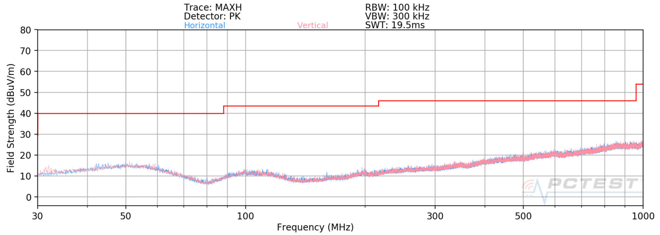
Plot 7-50. Radiated Spurious Plot below 1GHz
