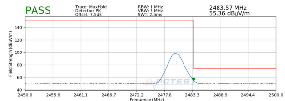
Plot 7-49. Radiated Restricted Upper Band Edge Measurement with WCP (Peak)
