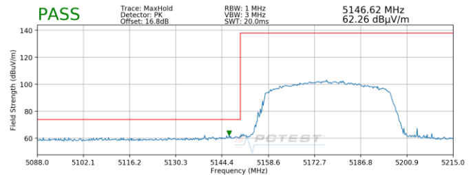
Plot 7-222. Radiated Lower Band Edge Plot MIMO (Peak – UNII Band 1)
