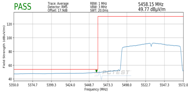
Plot 7-189. Radiated Lower Band Edge Plot SISO ANT1 (Average – UNII Band 2C)
