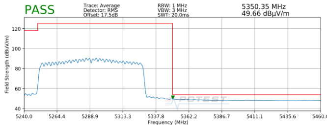
Plot 7-230. Radiated Upper Band Edge Plot MIMO (Average – UNII Band 2A)
