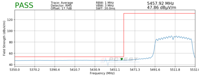
Plot 7-225. Radiated Lower Band Edge Plot MIMO (Average – UNII Band 2C)
