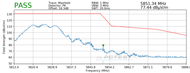
Plot 7-219. Radiated Upper Band Edge Plot MIMO (Peak – UNII Band 3)
