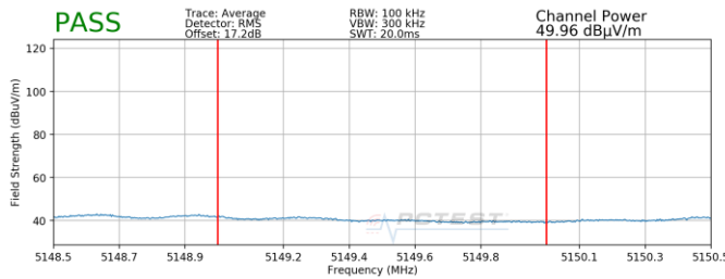
Plot 7-228. Radiated Lower Band Edge Plot MIMO (Average – UNII Band 1)
