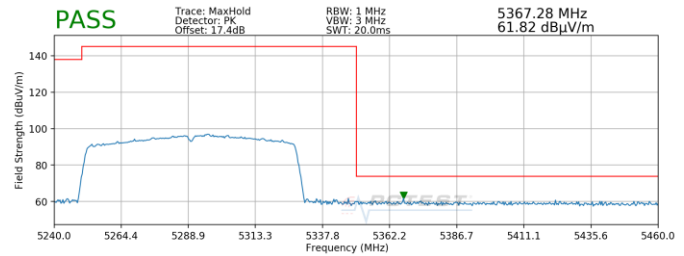
Plot 7-209. Radiated Upper Band Edge Plot SISO ANT2 (Peak – UNII Band 2A)
