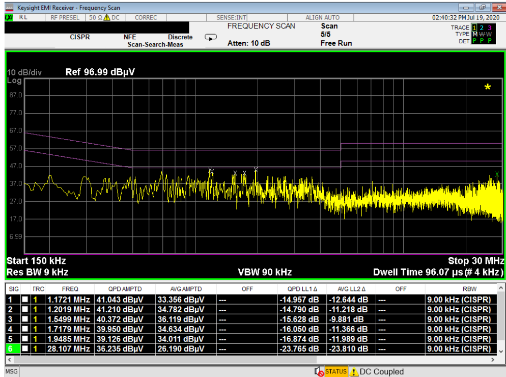
Plot 7-244. Line Conducted Plot with 802.11a UNII Band 1 with WCP (N)
