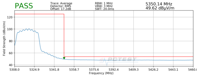
Plot 7-215. Radiated Upper Band Edge Plot MIMO (Average – UNII Band 2A)
