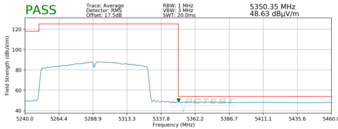
Plot 7-208. Radiated Upper Band Edge Plot SISO ANT2 (Average – UNII Band 2A)
