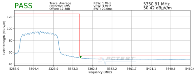
Plot 7-223. Radiated Upper Band Edge Plot MIMO (Average – UNII Band 2A)
