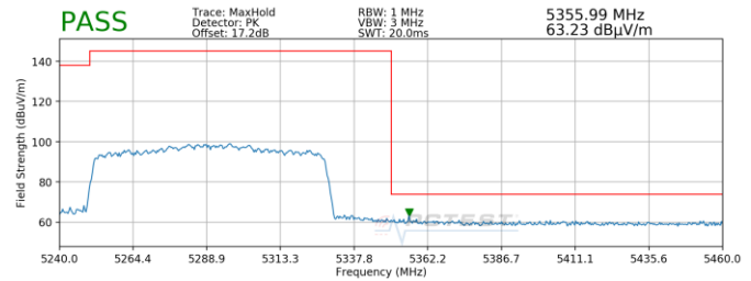
Plot 7-231. Radiated Upper Band Edge Plot MIMO (Peak – UNII Band 2A)
