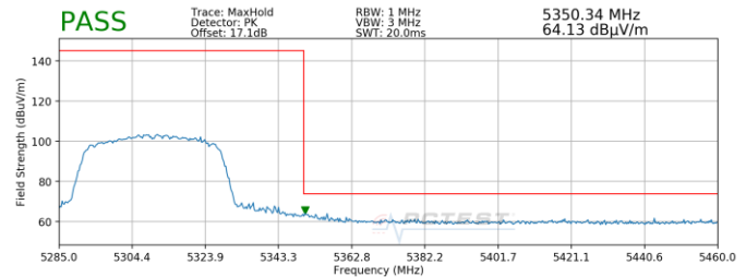
Plot 7-224. Radiated Upper Band Edge Plot MIMO (Peak – UNII Band 2A)
