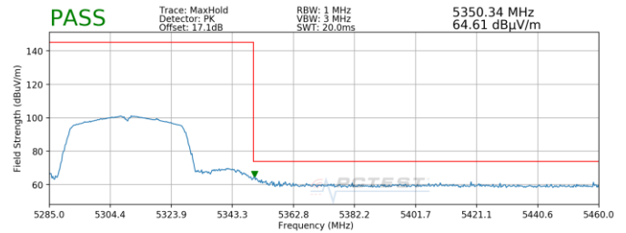
Plot 7-202. Radiated Upper Band Edge Plot SISO ANT2 (Peak – UNII Band 2A)
