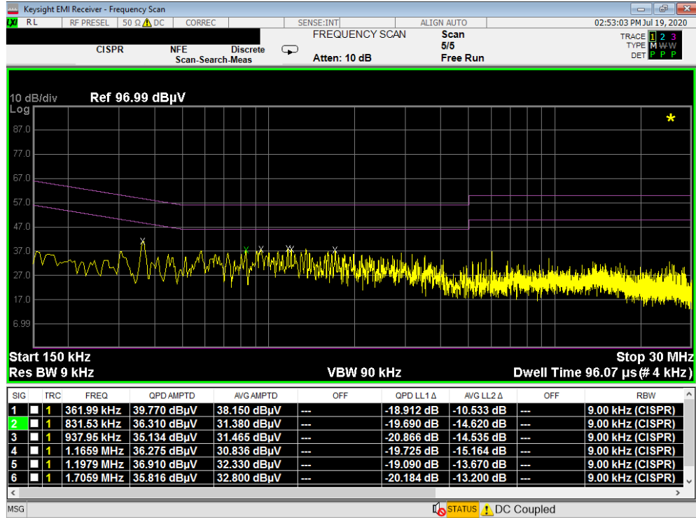
Plot 7-249. Line Conducted Plot with 802.11a UNII Band 3 with WCP (L1)
