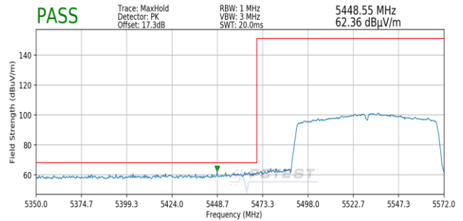
Plot 7-190. Radiated Lower Band Edge Plot SISO ANT1 (Peak – UNII Band 2C)
