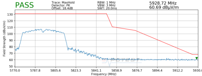
Plot 7-227. Radiated Upper Band Edge Plot MIMO (Peak – UNII Band 3)
