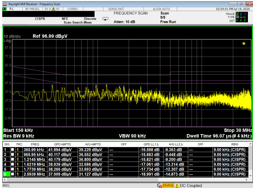
Plot 7-250. Line Conducted Plot with 802.11a UNII Band 3 with WCP (N)
