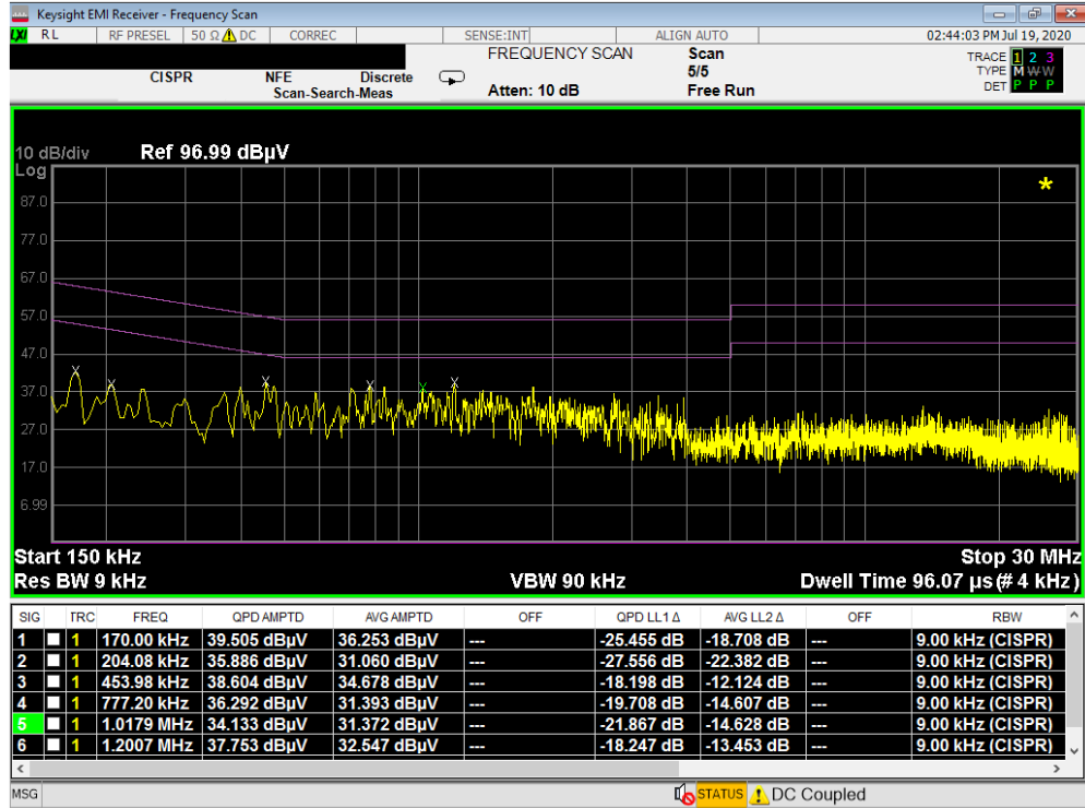
Plot 7-245. Line Conducted Plot with 802.11a UNII Band 2A with WCP (L1)
