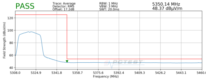
Plot 7-194. Radiated Upper Band Edge Plot SISO ANT2 (Average – UNII Band 2A)
