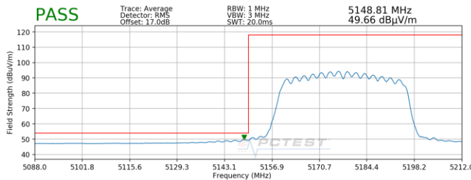
Plot 7-221. Radiated Lower Band Edge Plot MIMO (Average – UNII Band 1)
