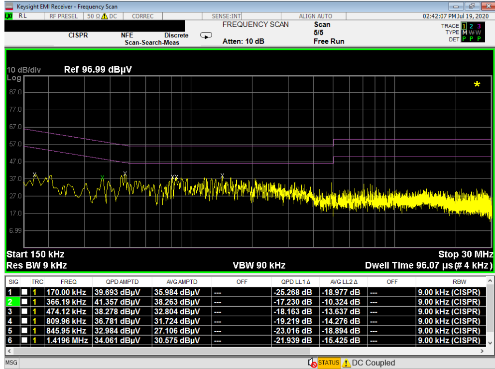
Plot 7-243. Line Conducted Plot with 802.11a UNII Band 1 with WCP (L1)
