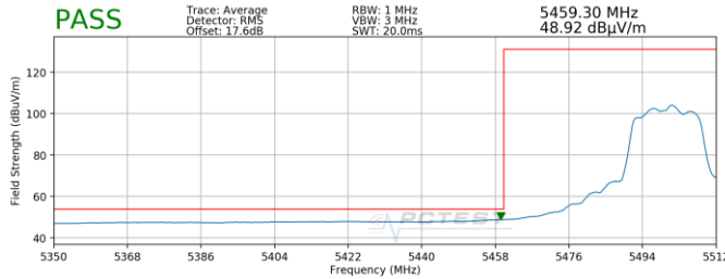
Plot 7-217. Radiated Lower Band Edge Plot MIMO (Average – UNII Band 2C)
