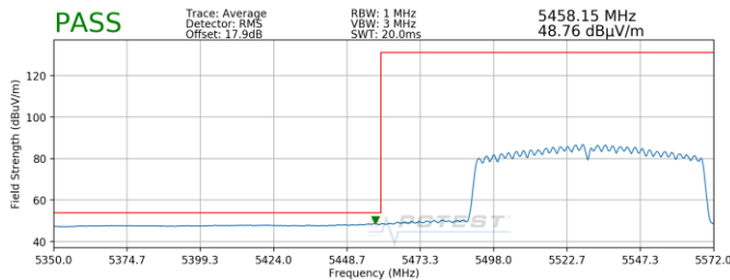
Plot 7-232. Radiated Lower Band Edge Plot MIMO (Average – UNII Band 2C)
