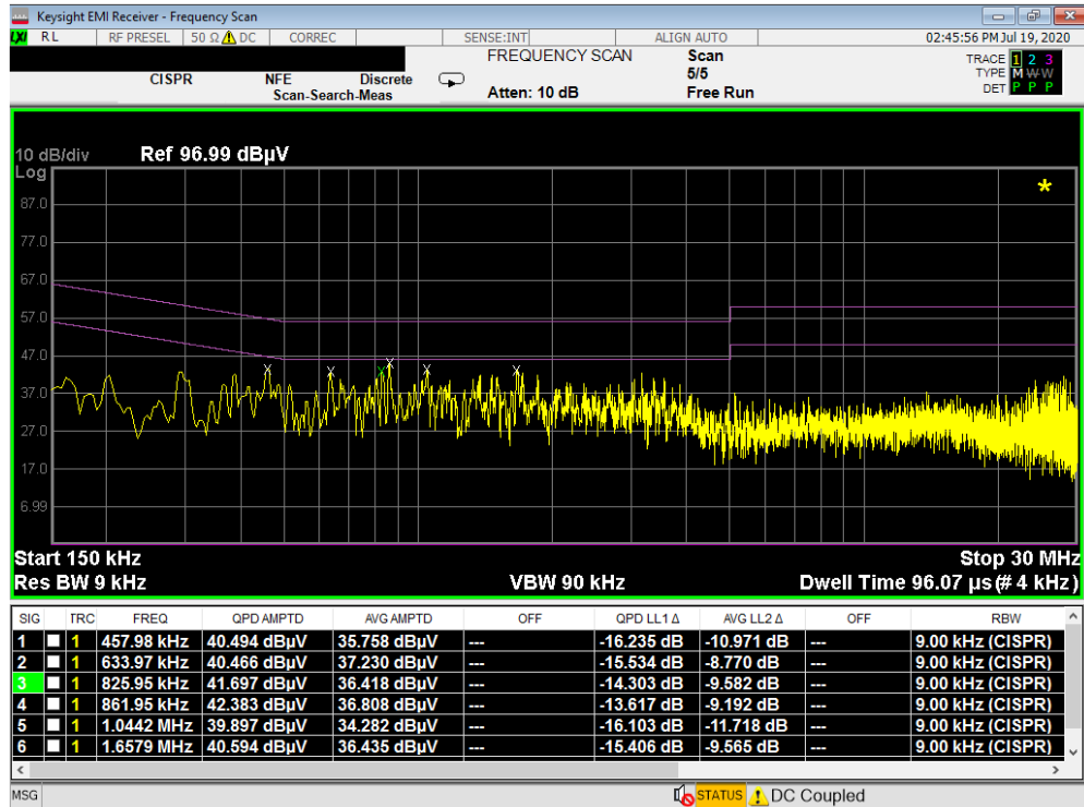
Plot 7-248. Line Conducted Plot with 802.11a UNII Band 2C with WCP (N)
