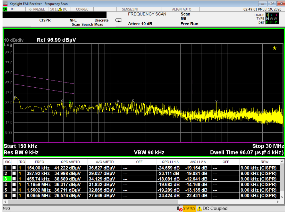
Plot 7-247. Line Conducted Plot with 802.11a UNII Band 2C with WCP (L1)
