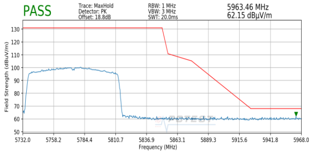
Plot 7-191. Radiated Upper Band Edge Plot SISO ANT1 (Peak – UNII Band 3)
