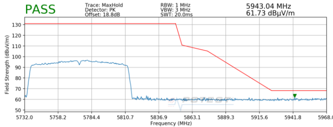
Plot 7-212. Radiated Upper Band Edge Plot SISO ANT2 (Peak - UNII Band 3)
