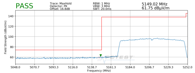
Plot 7-207. Radiated Lower Band Edge Plot SISO ANT2 (Peak – UNII Band 1)
