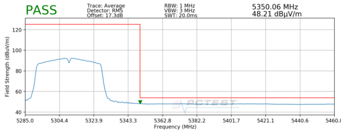
Plot 7-201. Radiated Upper Band Edge Plot SISO ANT2 (Average – UNII Band 2A)
