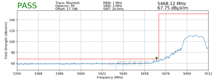
Plot 7-218. Radiated Lower Band Edge Plot MIMO (Peak – UNII Band 2C)
