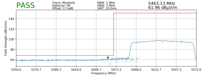
Plot 7-211. Radiated Lower Band Edge Plot SISO ANT2 (Peak - UNII Band 2C)
