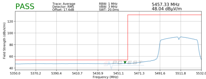
Plot 7-203. Radiated Lower Band Edge Plot SISO ANT2 (Average - UNII Band 2C)
