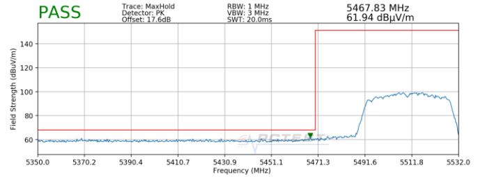
Plot 7-226. Radiated Lower Band Edge Plot MIMO (Peak – UNII Band 2C)
