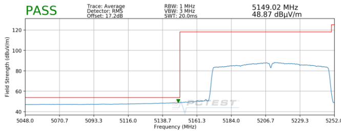
Plot 7-206. Radiated Lower Band Edge Plot SISO ANT2 (Average – UNII Band 1)
