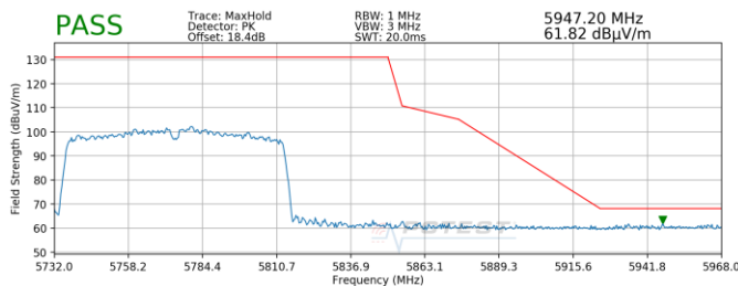
Plot 7-234. Radiated Upper Band Edge Plot MIMO (Peak – UNII Band 3)
