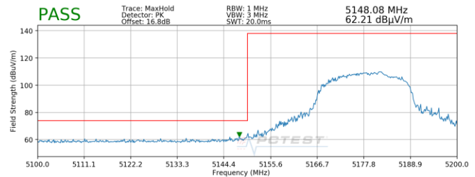
Plot 7-214. Radiated Lower Band Edge Plot MIMO (Peak – UNII Band 1)
