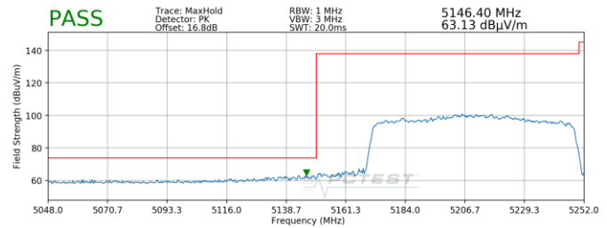
Plot 7-229. Radiated Lower Band Edge Plot MIMO (Peak – UNII Band 1)
