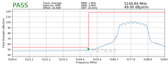
Plot 7-213. Radiated Lower Band Edge Plot MIMO (Average – UNII Band 1)
