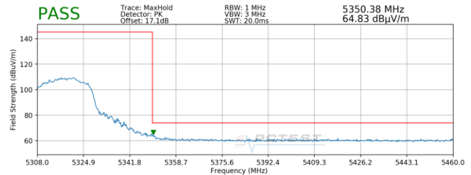
Plot 7-216. Radiated Upper Band Edge Plot MIMO (Peak – UNII Band 2A)
