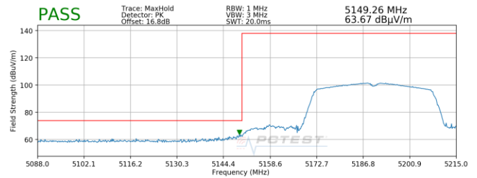
Plot 7-200. Radiated Lower Band Edge Plot SISO ANT2 (Peak – UNII Band 1)
