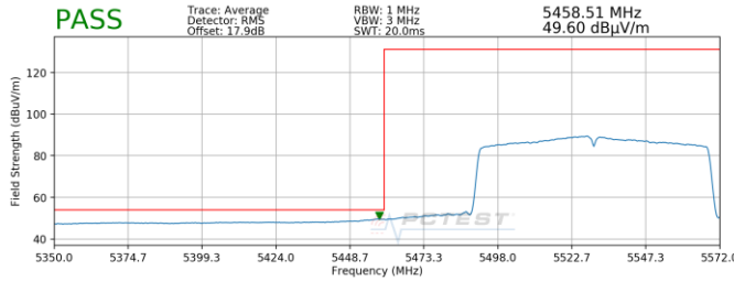
Plot 7-210. Radiated Lower Band Edge Plot SISO ANT2 (Average - UNII Band 2C)
