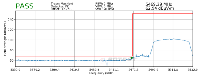
Plot 7-204. Radiated Lower Band Edge Plot SISO ANT2 (Peak - UNII Band 2C)
