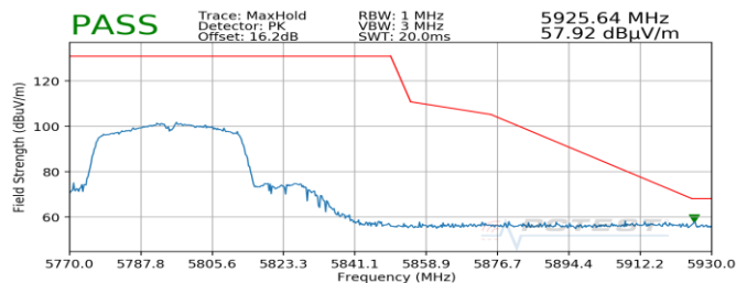
Plot 7-205. Radiated Upper Band Edge Plot SISO ANT2 (Peak - UNII Band 3)
