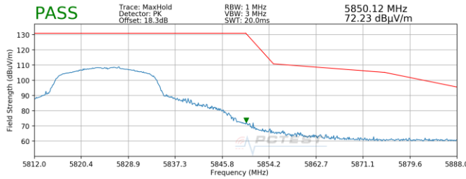
Plot 7-198. Radiated Upper Band Edge Plot SISO ANT2 (Peak - UNII Band 3)
