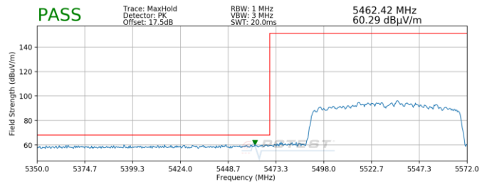
Plot 7-233. Radiated Lower Band Edge Plot MIMO (Peak – UNII Band 2C)
