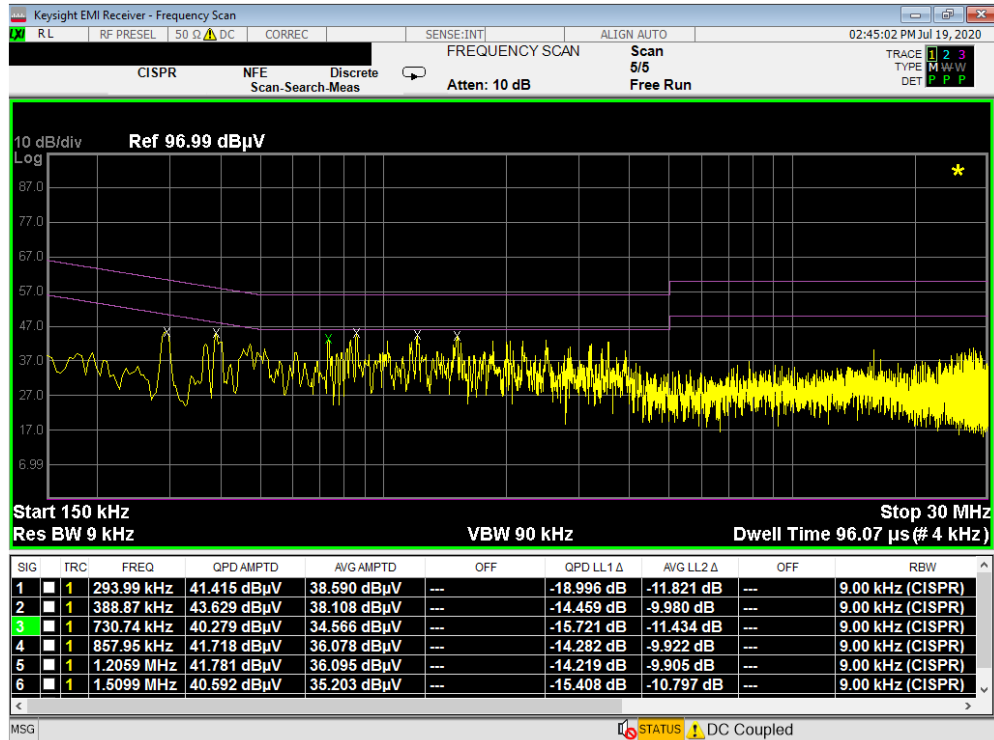
Plot 7-246. Line Conducted Plot with 802.11a UNII Band 2A with WCP (N)
