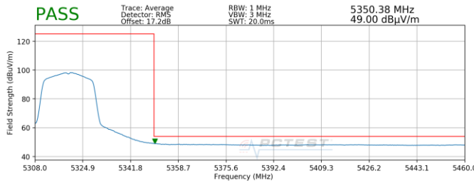
Plot 7-173. Radiated Upper Band Edge Plot SISO ANT1 (Average – UNII Band 2A)
