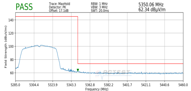
Plot 7-181. Radiated Upper Band Edge Plot SISO ANT1 (Peak – UNII Band 2A)
