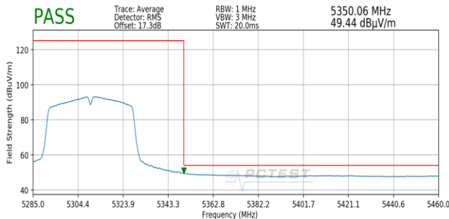
Plot 7-180. Radiated Upper Band Edge Plot SISO ANT1 (Average – UNII Band 2A)
