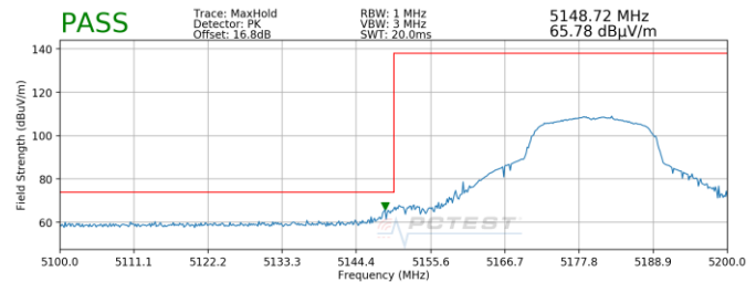
Plot 7-172. Radiated Lower Band Edge Plot SISO ANT1 (Peak – UNII Band 1)
