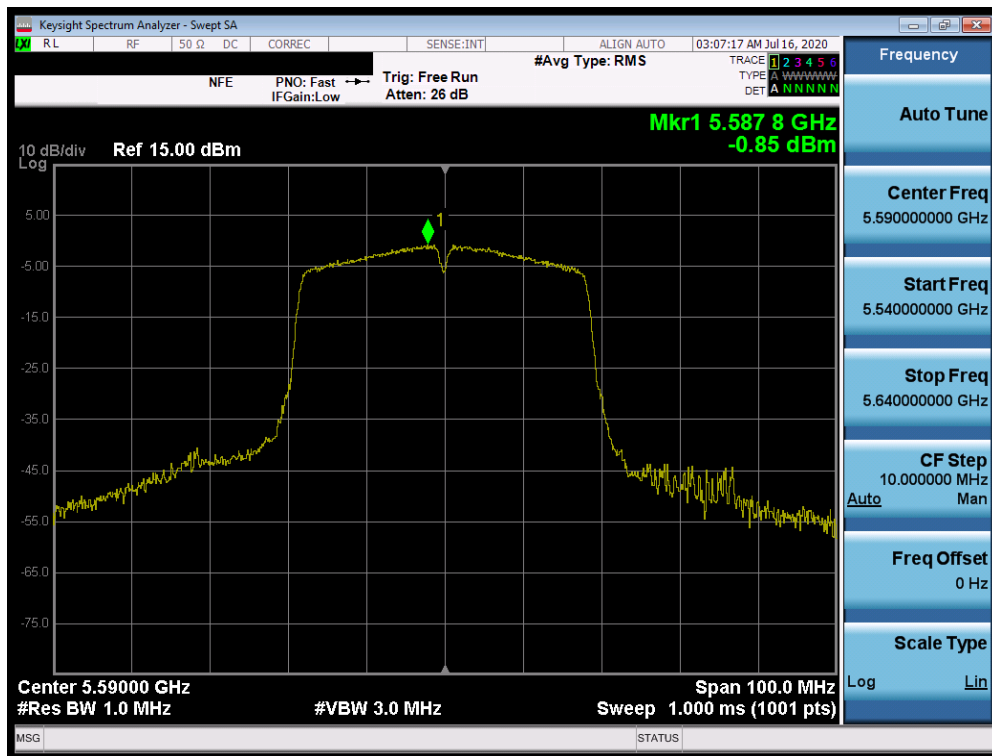
Plot 7-143. Power Spectral Density Plot SISO ANT2 (40MHz BW 802.11n (UNII Band 2C) – Ch. 118)
