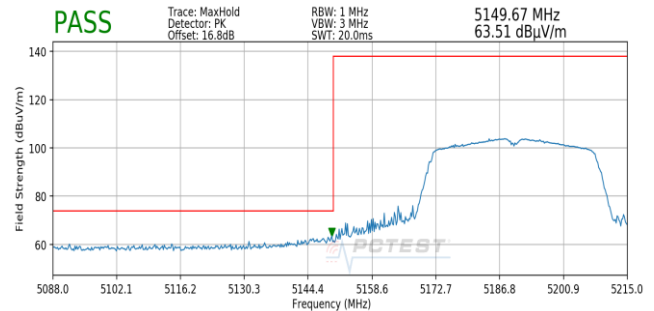
Plot 7-179. Radiated Lower Band Edge Plot SISO ANT1 (Peak – UNII Band 1)
