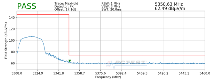
Plot 7-174. Radiated Upper Band Edge Plot SISO ANT1 (Peak – UNII Band 2A)
