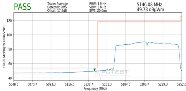
Plot 7-185. Radiated Lower Band Edge Plot SISO ANT1 (Average – UNII Band 1)
