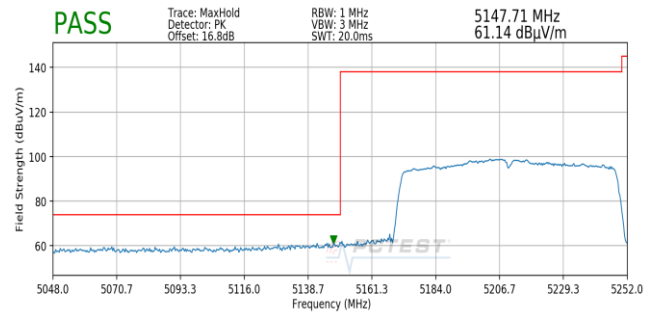
Plot 7-186. Radiated Lower Band Edge Plot SISO ANT1 (Peak – UNII Band 1)
