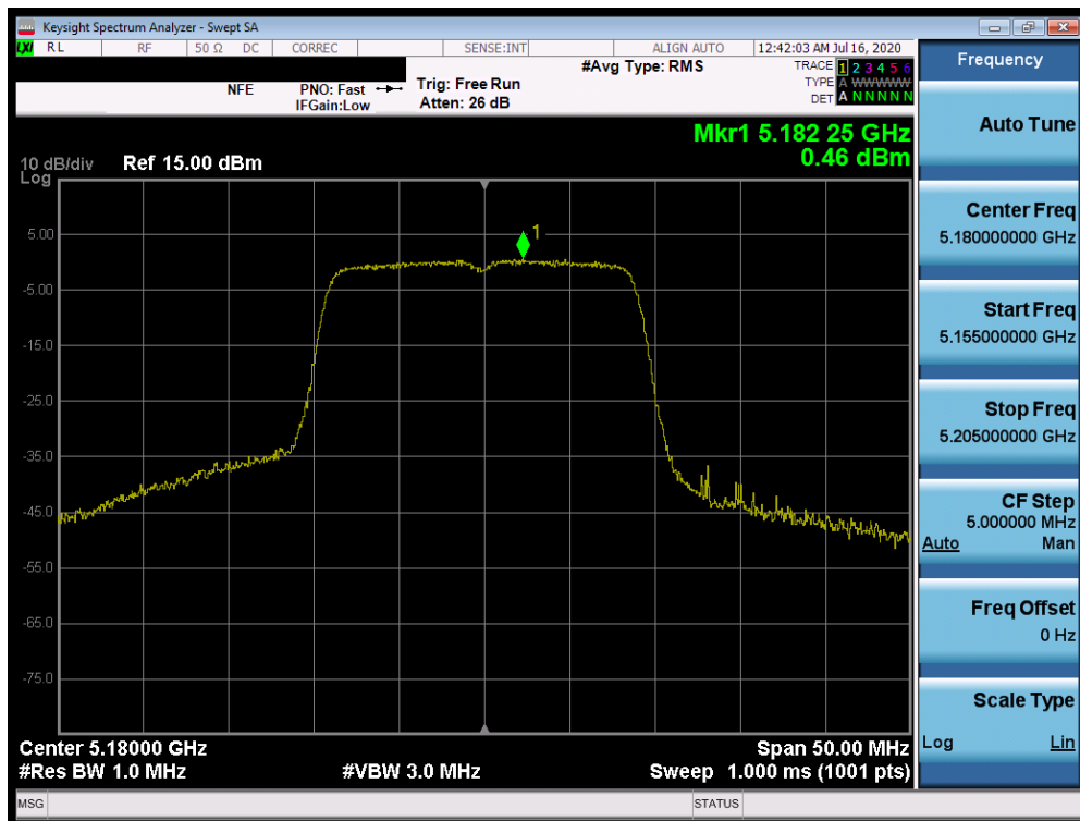
Plot 7-121. Power Spectral Density Plot SISO ANT2 (20MHz BW 802.11n (UNII Band 1) – Ch. 36)
