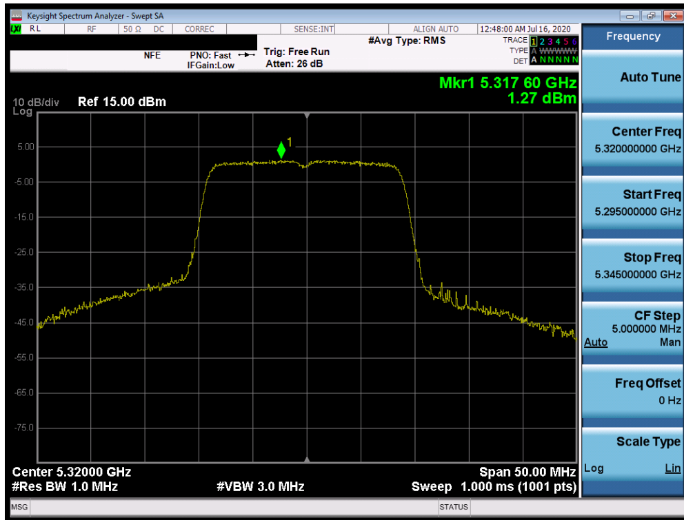
Plot 7-132. Power Spectral Density Plot SISO ANT2 (20MHz BW 802.11n (UNII Band 2A) – Ch. 64)
