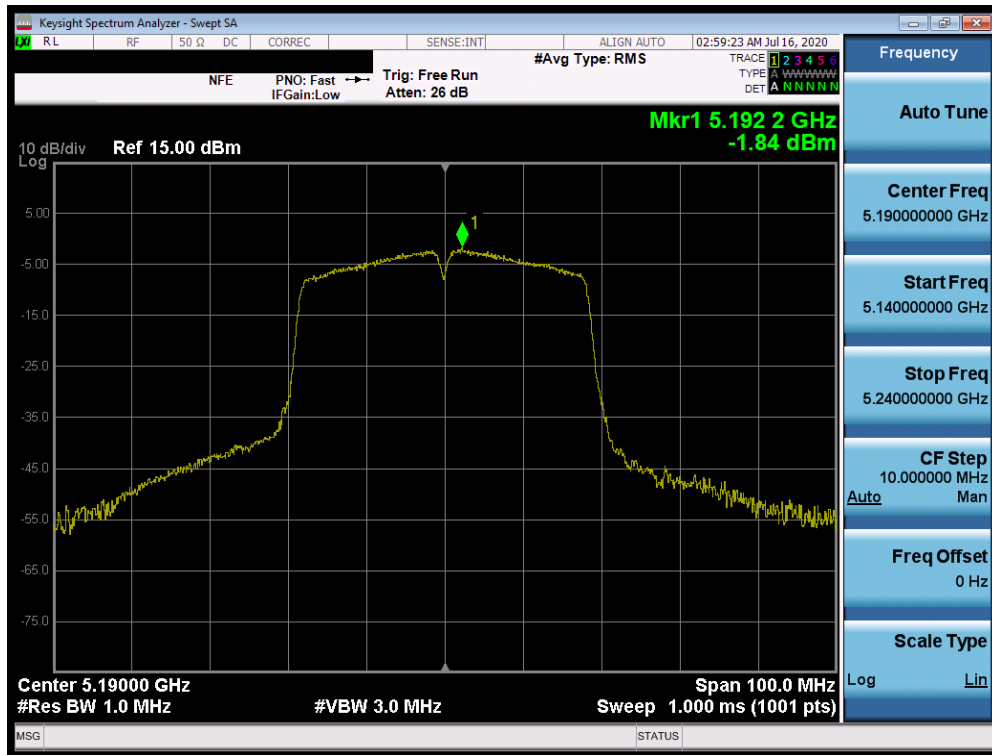
Plot 7-124. Power Spectral Density Plot SISO ANT2 (40MHz BW 802.11n (UNII Band 1) – Ch. 38)
