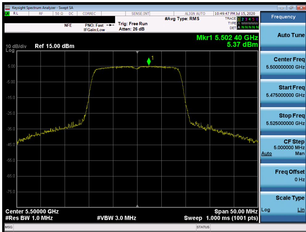
Plot 7-100. Power Spectral Density Plot SISO ANT1 (20MHz BW 802.11n (UNII Band 2C) – Ch. 100)
