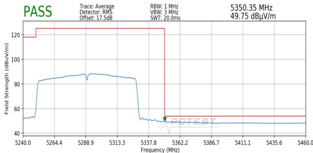
Plot 7-187. Radiated Upper Band Edge Plot SISO ANT1 (Average – UNII Band 2A)
