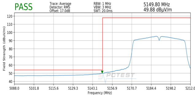
Plot 7-178. Radiated Lower Band Edge Plot SISO ANT1 (Average – UNII Band 1)
