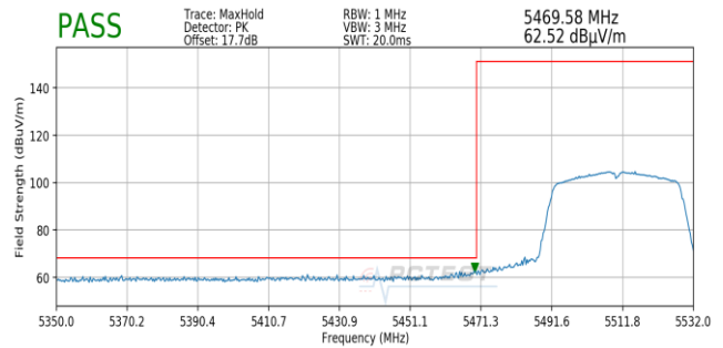
Plot 7-183. Radiated Lower Band Edge Plot SISO ANT1 (Peak – UNII Band 2C)
