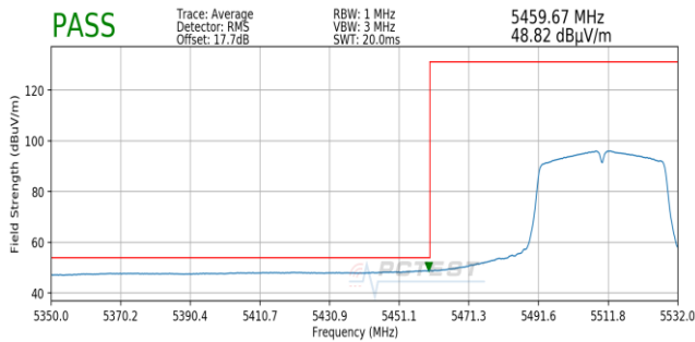
Plot 7-182. Radiated Lower Band Edge Plot SISO ANT1 (Average – UNII Band 2C)
