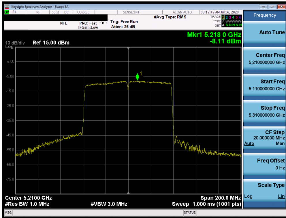
Plot 7-126. Power Spectral Density Plot SISO ANT2 (80MHz BW 802.11ac (UNII Band 1) – Ch. 42)
