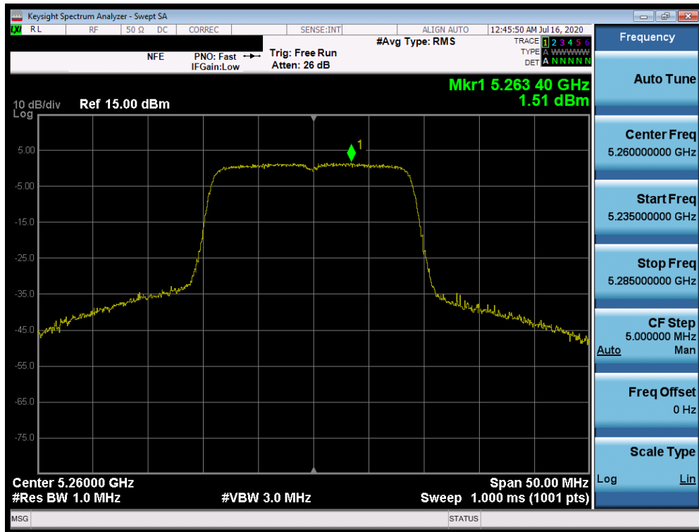
Plot 7-130. Power Spectral Density Plot SISO ANT2 (20MHz BW 802.11n (UNII Band 2A) – Ch. 52)
