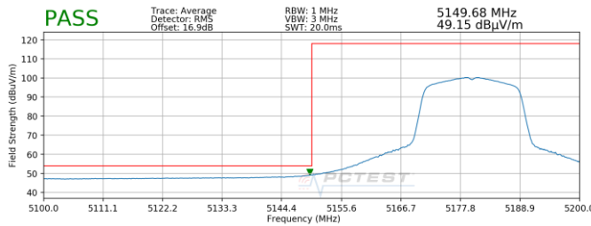
Plot 7-171. Radiated Lower Band Edge Plot SISO ANT1 (Average – UNII Band 1)
