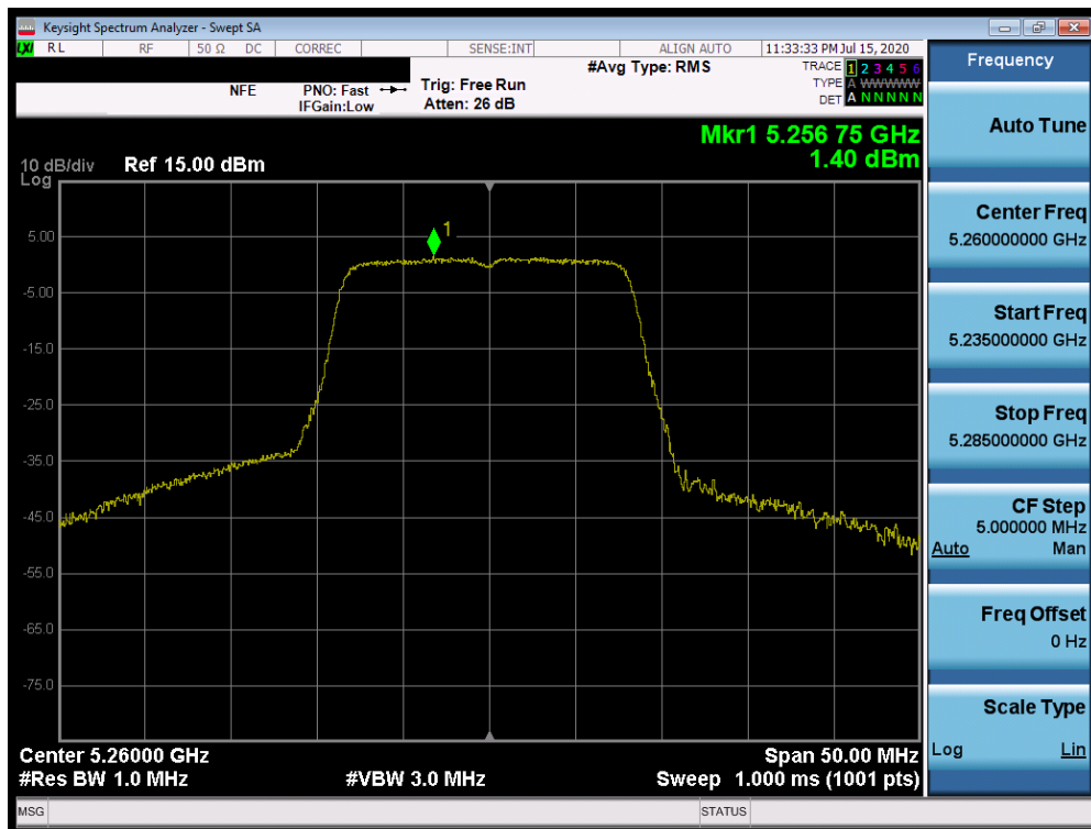
Plot 7-127. Power Spectral Density Plot SISO ANT2 (802.11a (UNII Band 2A) – Ch. 52)
