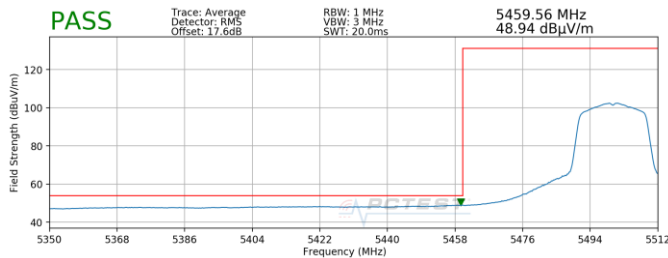
Plot 7-175. Radiated Lower Band Edge Plot SISO ANT1 (Average – UNII Band 2C)
