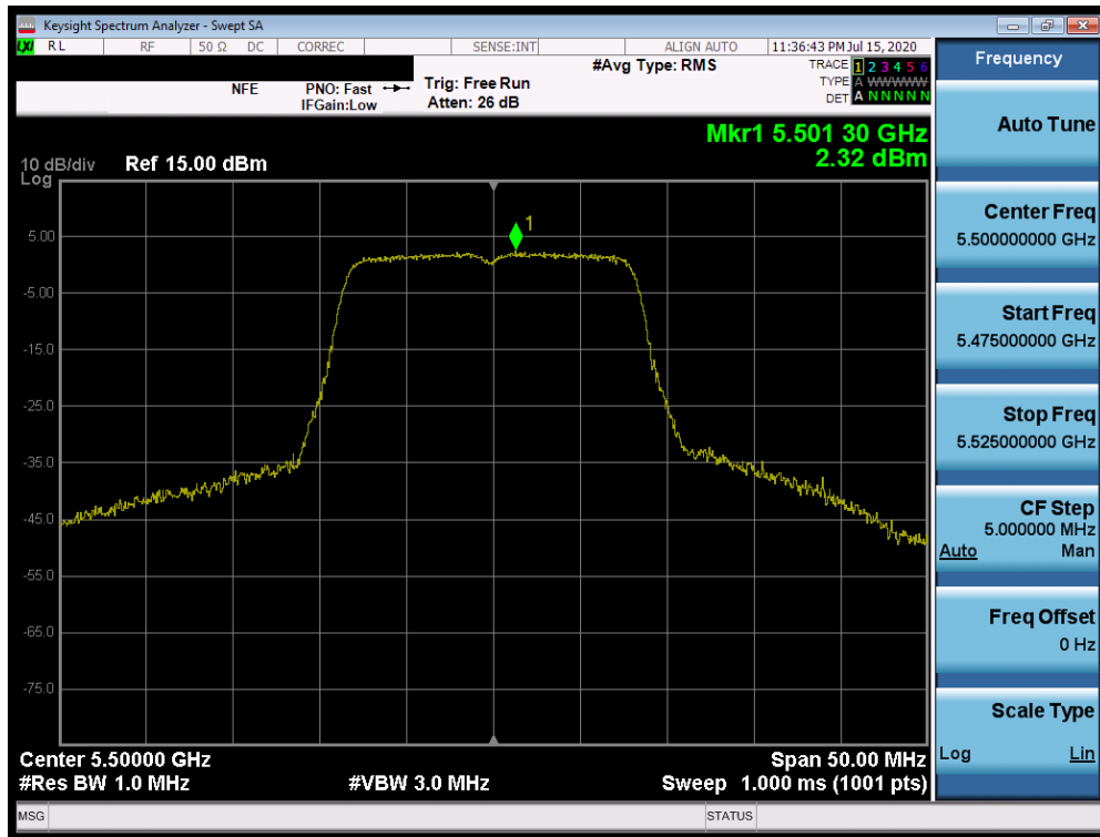
Plot 7-136. Power Spectral Density Plot SISO ANT2 (802.11a (UNII Band 2C) – Ch. 100)
