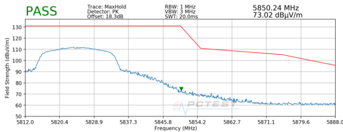
Plot 7-177. Radiated Upper Band Edge Plot SISO ANT1 (Peak – UNII Band 3)
