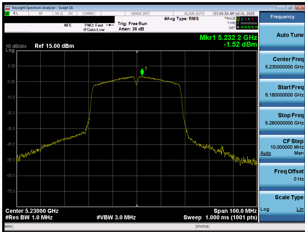
Plot 7-125. Power Spectral Density Plot SISO ANT2 (40MHz BW 802.11n (UNII Band 1) – Ch. 46)
