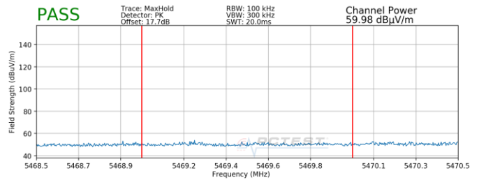
Plot 7-176. Radiated Lower Band Edge Plot SISO ANT1 (Peak – UNII Band 2C)
