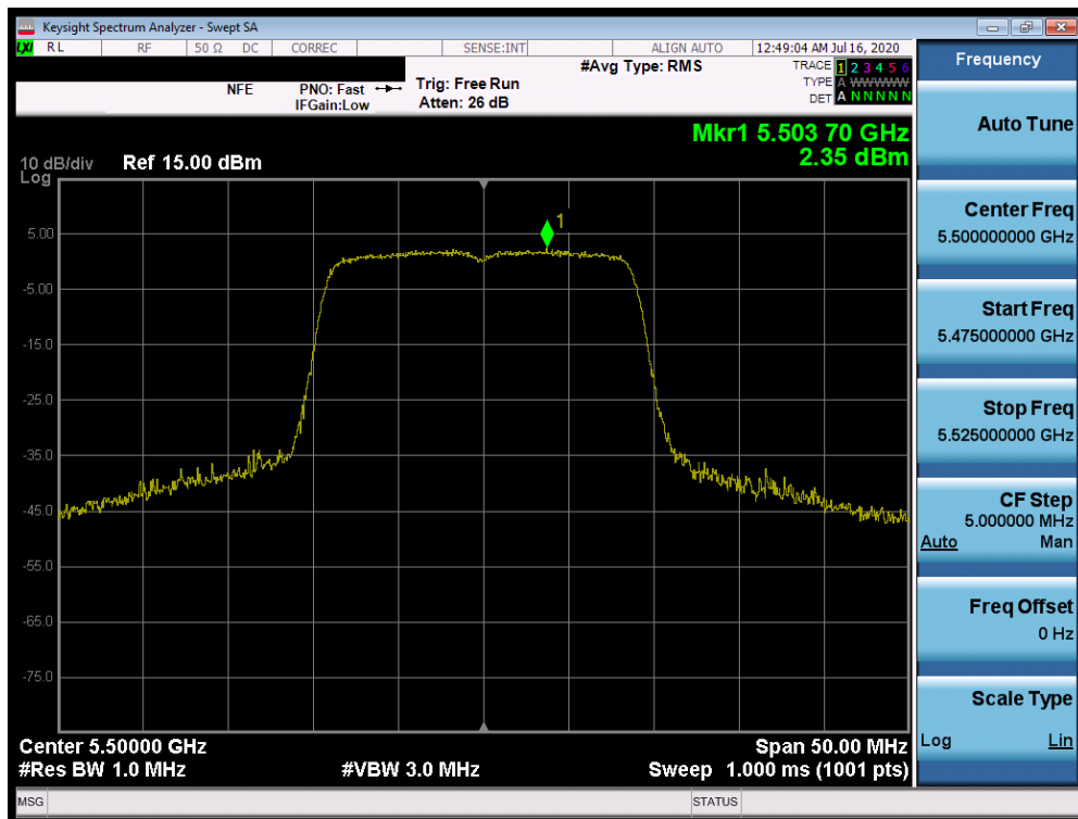
Plot 7-139. Power Spectral Density Plot SISO ANT2 (20MHz BW 802.11n (UNII Band 2C) – Ch. 100)
