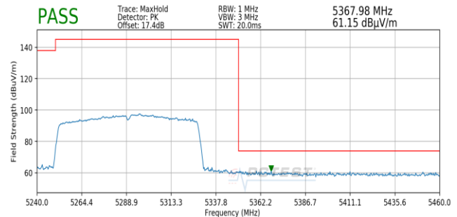
Plot 7-188. Radiated Upper Band Edge Plot SISO ANT1 (Peak – UNII Band 2A)
