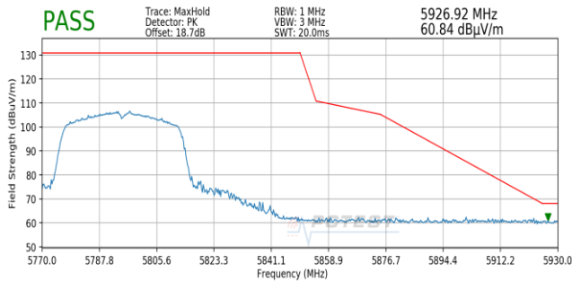
Plot 7-184. Radiated Upper Band Edge Plot SISO ANT1 (Peak – UNII Band 3)
