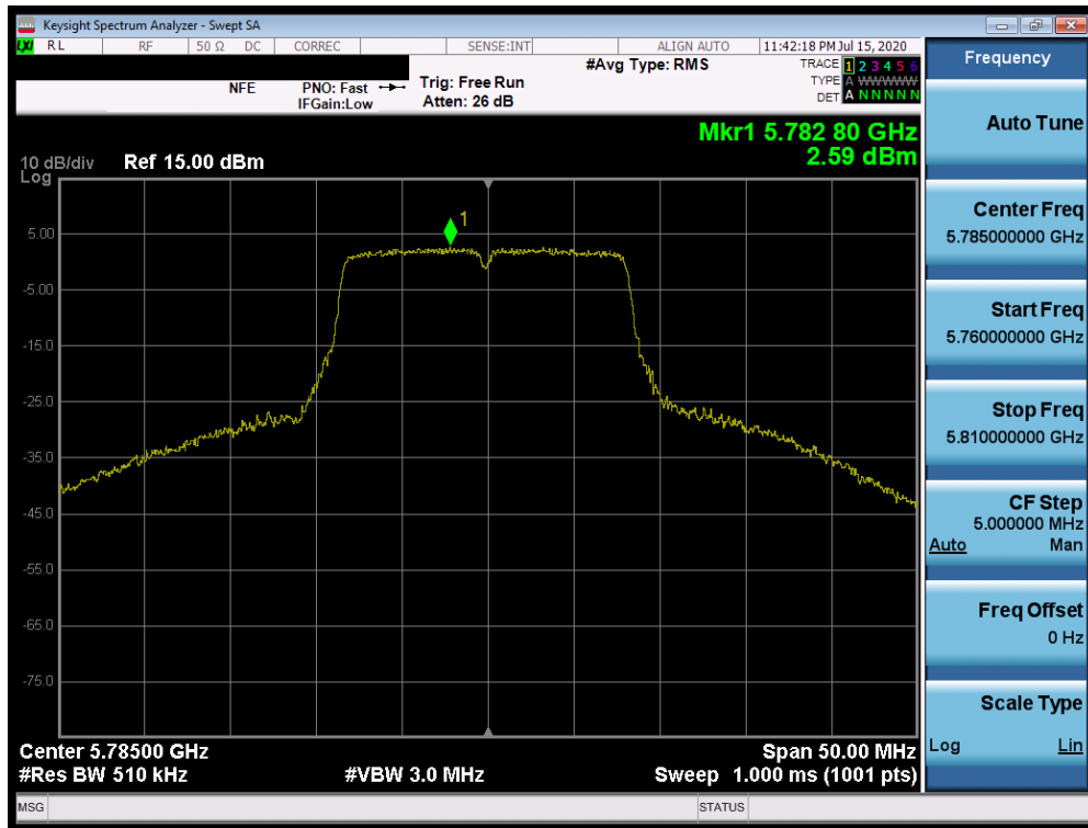
Plot 7-149. Power Spectral Density Plot SISO ANT2 (802.11a (UNII Band 3) – Ch. 157)
