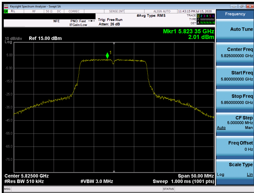
Plot 7-150. Power Spectral Density Plot SISO ANT2 (802.11a (UNII Band 3) – Ch. 165)
