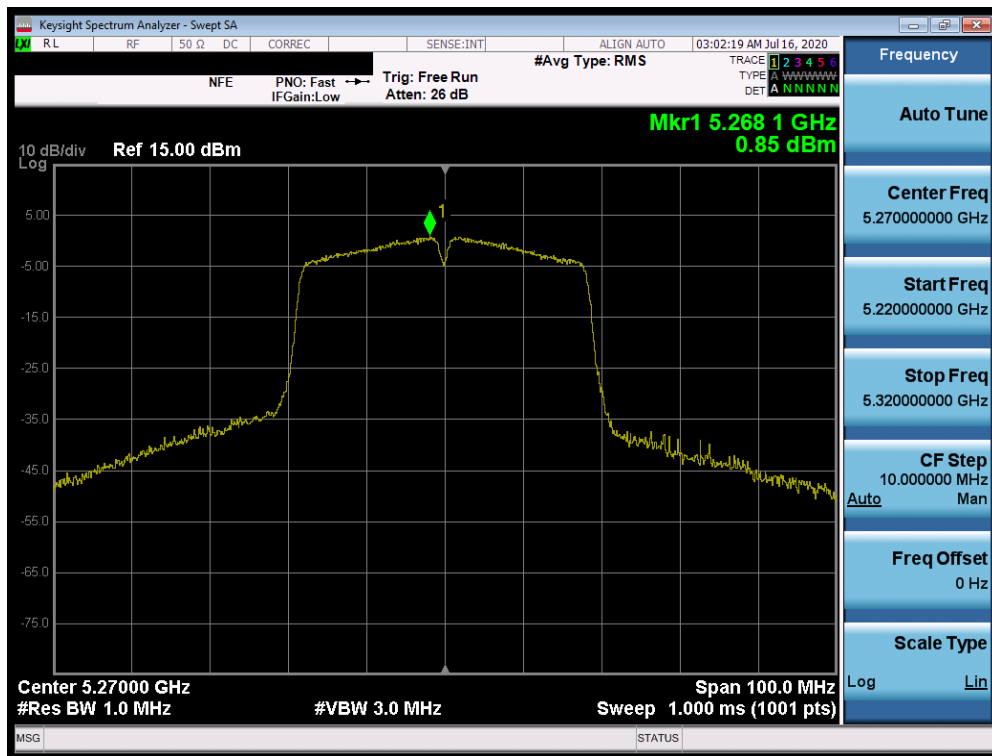
Plot 7-133. Power Spectral Density Plot SISO ANT2 (40MHz BW 802.11n (UNII Band 2A) – Ch. 54)
