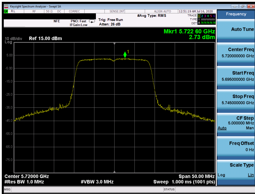
Plot 7-141. Power Spectral Density Plot SISO ANT2 (20MHz BW 802.11n (UNII Band 2C) – Ch. 144)
