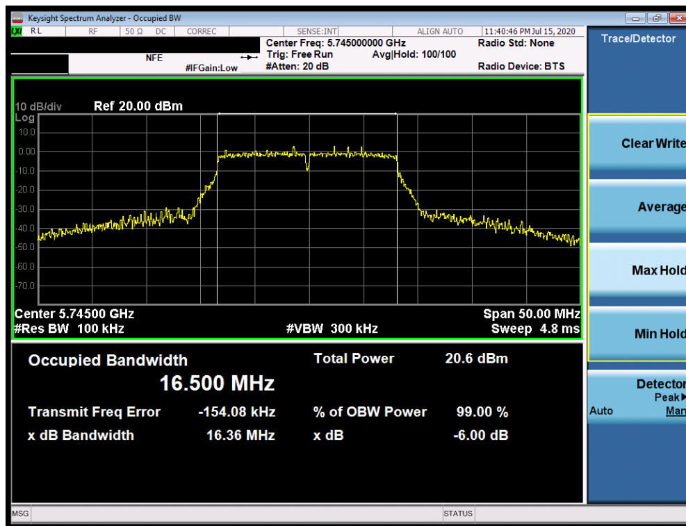
Plot 7-70. 6dB Bandwidth Plot SISO ANT2 (802.11a (UNII Band 3) - Ch. 149)
