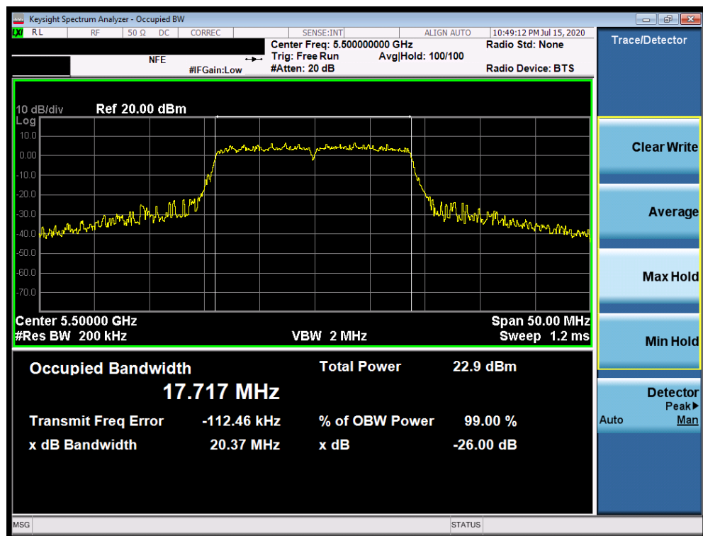
Plot 7-22. 26dB Bandwidth Plot SISO ANT1 (20MHz BW 802.11n (UNII Band 2C) – Ch. 100)
