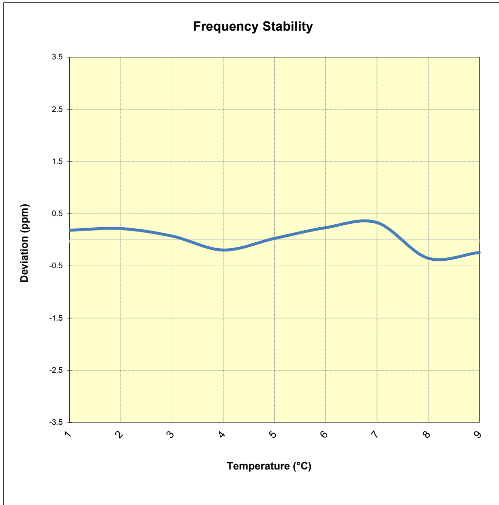
Figure 7-7. CDMA BC10 Frequency Stability Chart
