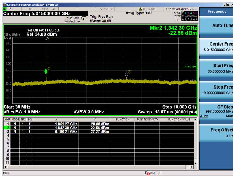
LTE Band 2 / 3MHz / QPSK - RB Size/Offset (8/4) – Low Channel
