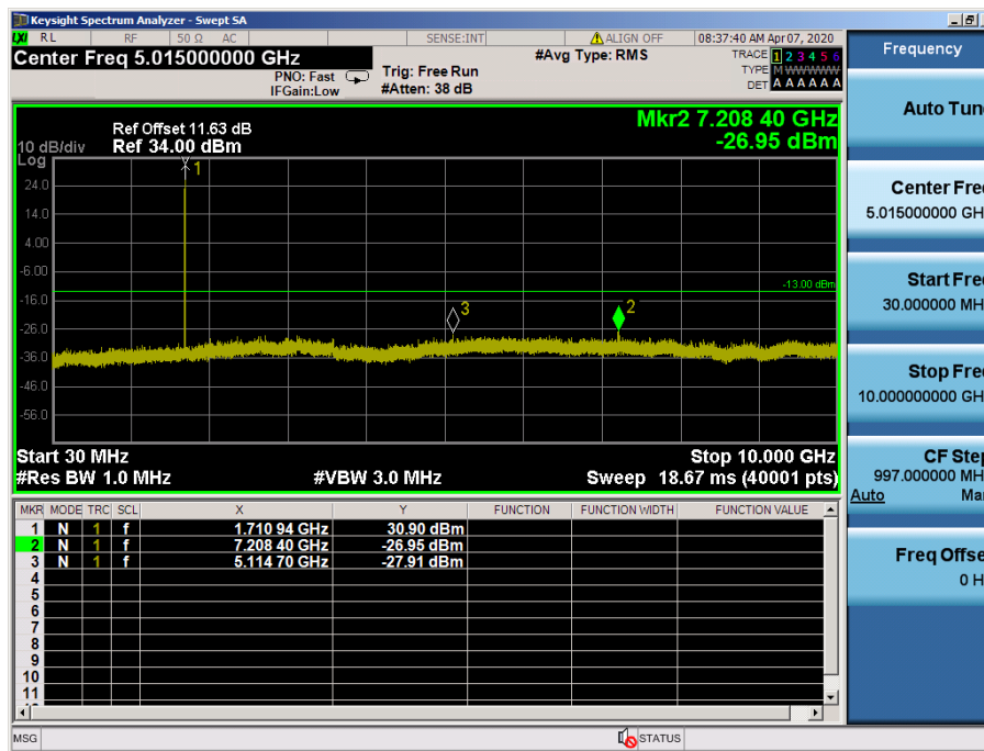
LTE Band 4 / 1.4MHz / 64QAM - RB Size/Offset (1/2) – Low Channel
