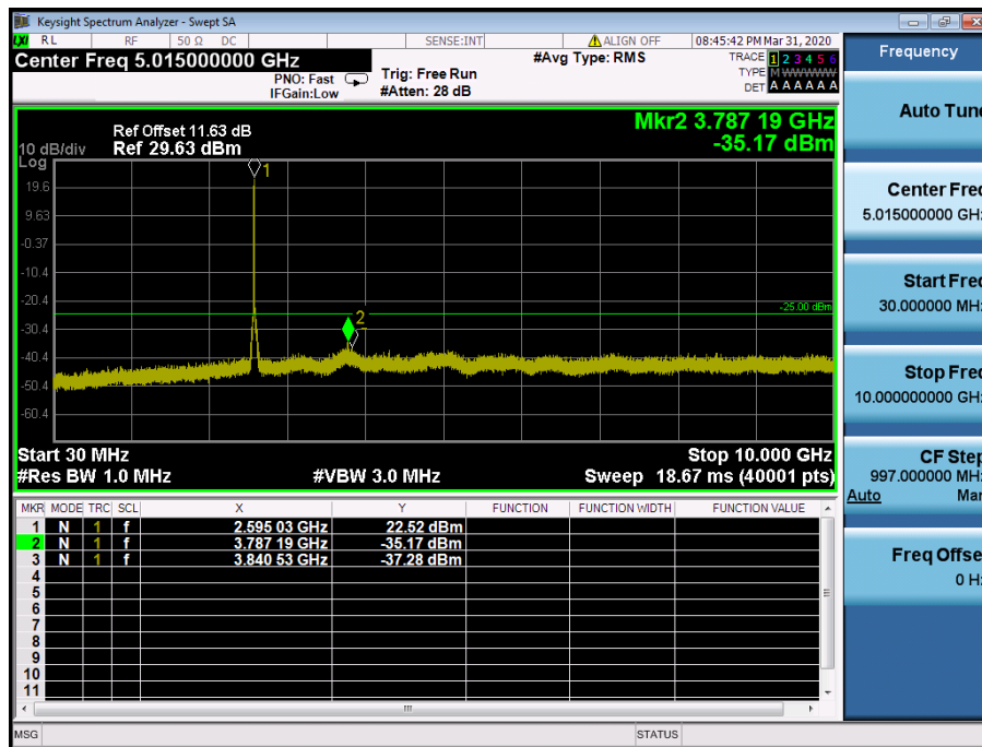
LTE Band 41 / 15MHz / 16QAM - RB Size/Offset (75/0) – Mid Channel
