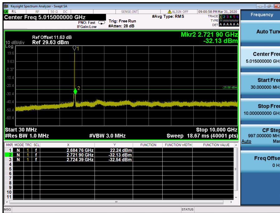
LTE Band 41 / 15MHz / 16QAM - RB Size/Offset (75/0) – High Channel
