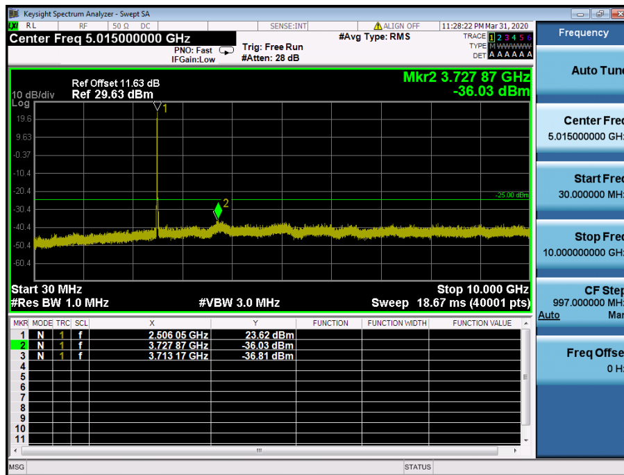
LTE Band 41 / 15MHz / 64QAM - RB Size/Offset (36/39) – Low Channel
