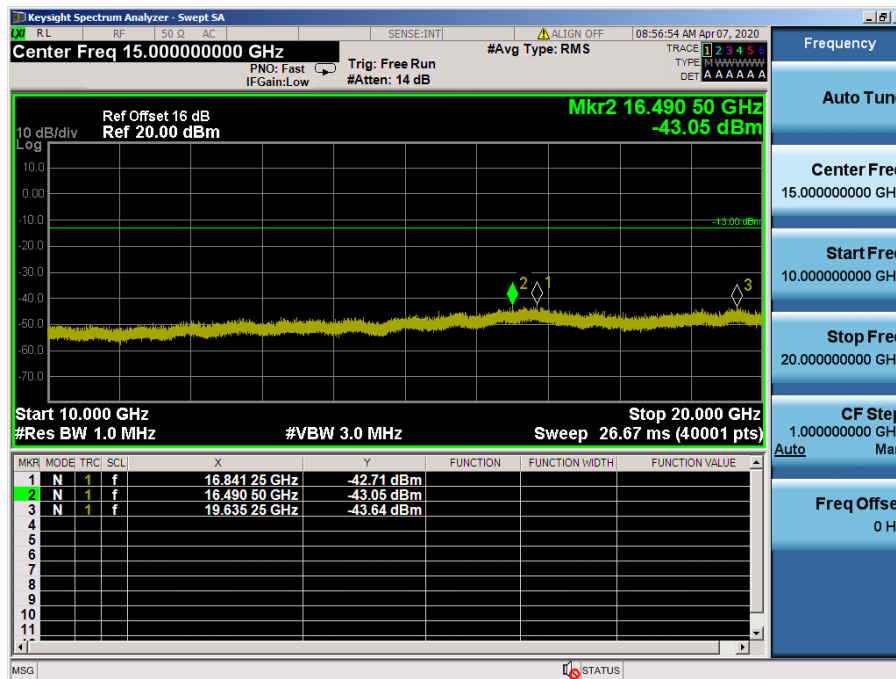
LTE Band 4 / 1.4MHz / 64QAM - RB Size/Offset (6/0) – Mid Channel
