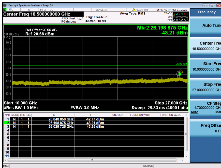
LTE Band 41 / 20MHz / QPSK - RB Size/Offset (100/0) – High Channel
