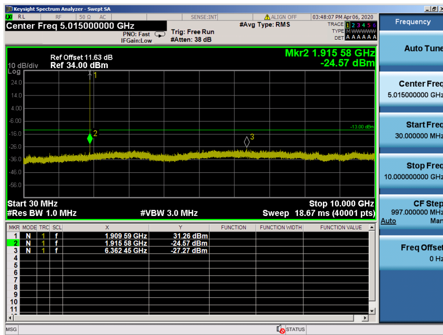
LTE Band 2 / 1.4MHz / 16QAM - RB Size/Offset (3/2) – High Channel
