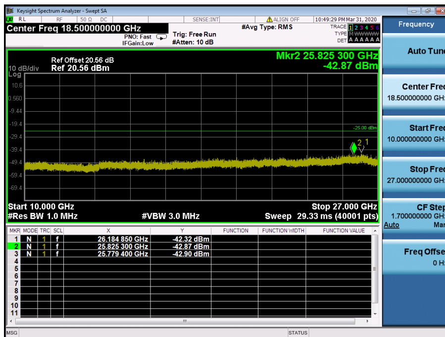
LTE Band 41 / 10MHz / 64QAM - RB Size/Offset (1/25) – Mid Channel
