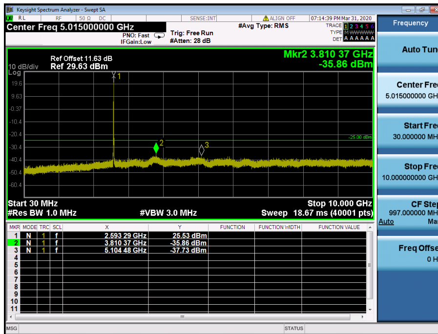
LTE Band 41 / 5MHz / 16QAM - RB Size/Offset (25/0) – Mid Channel
