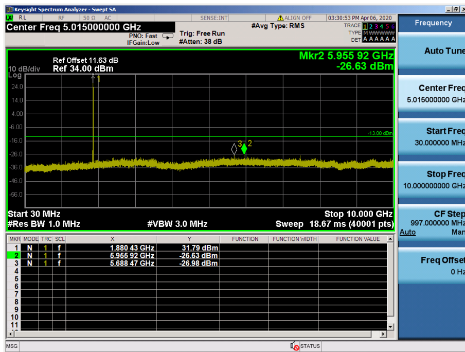
LTE Band 2 / 1.4MHz / 16QAM - RB Size/Offset (1/2) – Mid Channel
