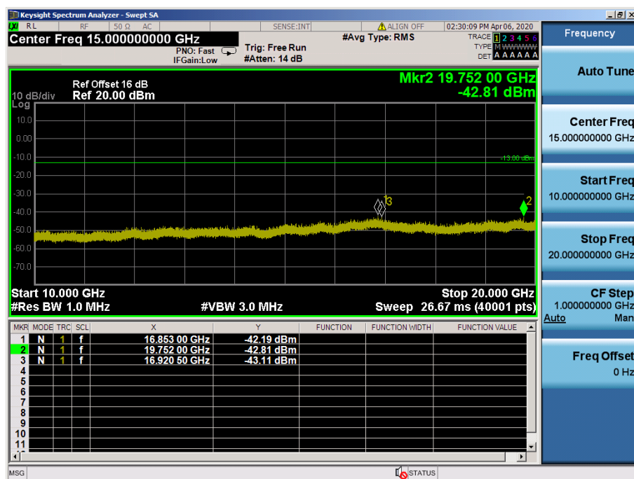
LTE Band 2 / 20MHz / QPSK - RB Size/Offset (1/0) –Low Channel
