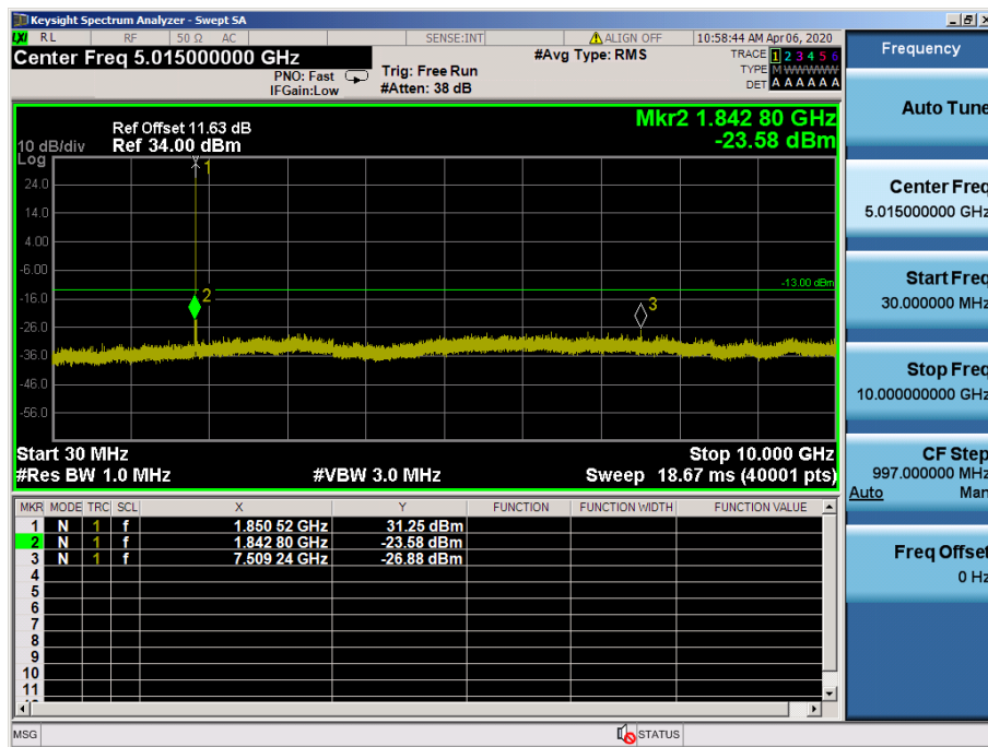
LTE Band 2 / 1.4MHz / QPSK - RB Size/Offset (3/0) – Low Channel
