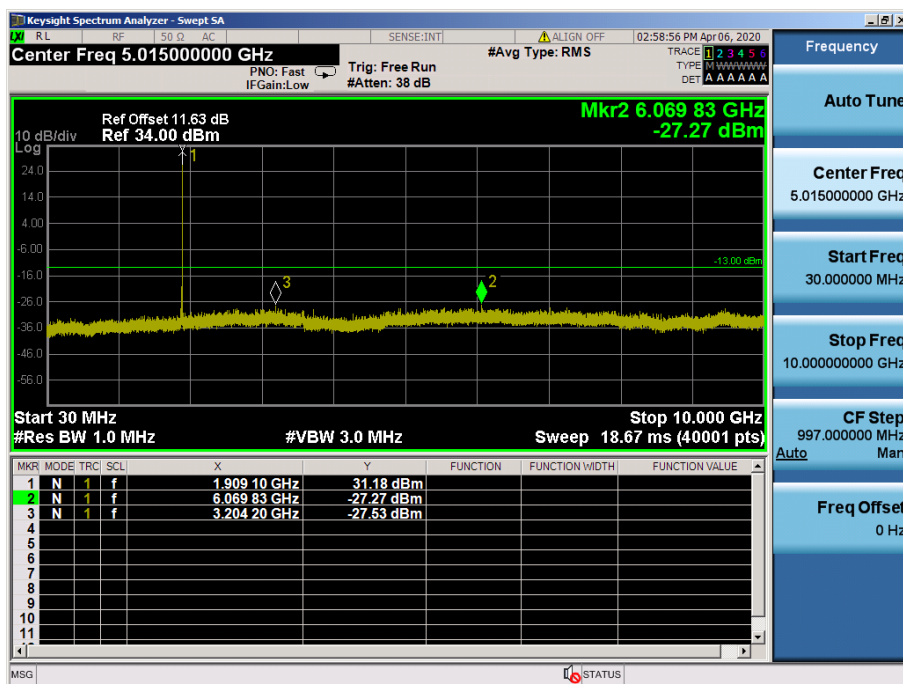
LTE Band 2 / 20MHz / QPSK - RB Size/Offset (1/99) – High Channel
