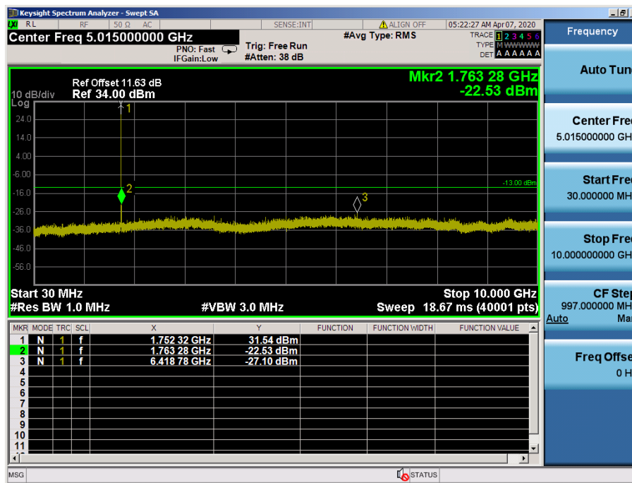
LTE Band 4 / 3MHz / 16QAM - RB Size/Offset (1/0) – High Channel
