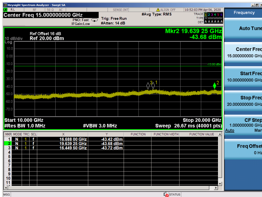
LTE Band 2 / 15MHz / 64QAM - RB Size/Offset (1/0) – High Channel
