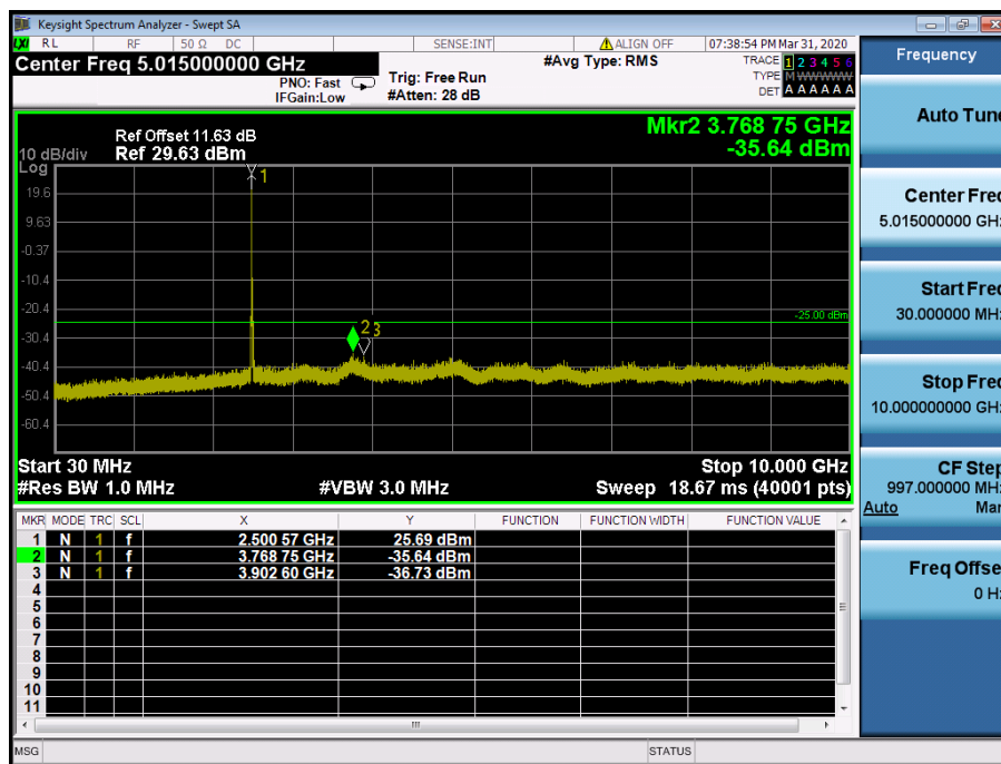
LTE Band 41 / 10MHz / 16QAM - RB Size/Offset (25/0) – Low Channel
