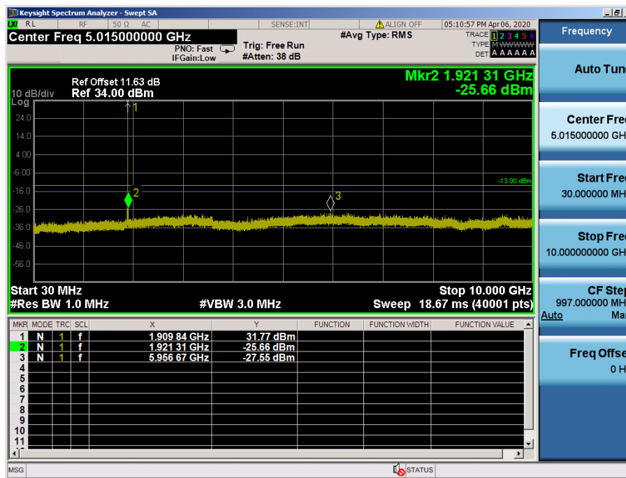
LTE Band 2 / 5MHz / 16QAM - RB Size/Offset (1/24) – High Channel
