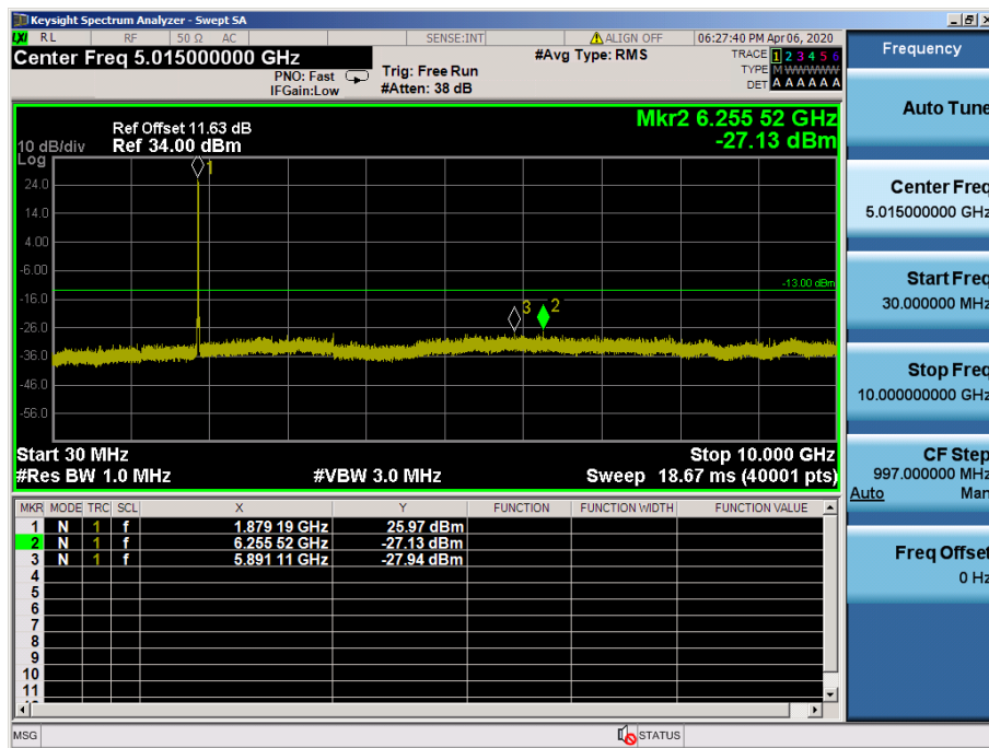
LTE Band 2 / 15MHz / 16QAM - RB Size/Offset (36/18) – Mid Channel
