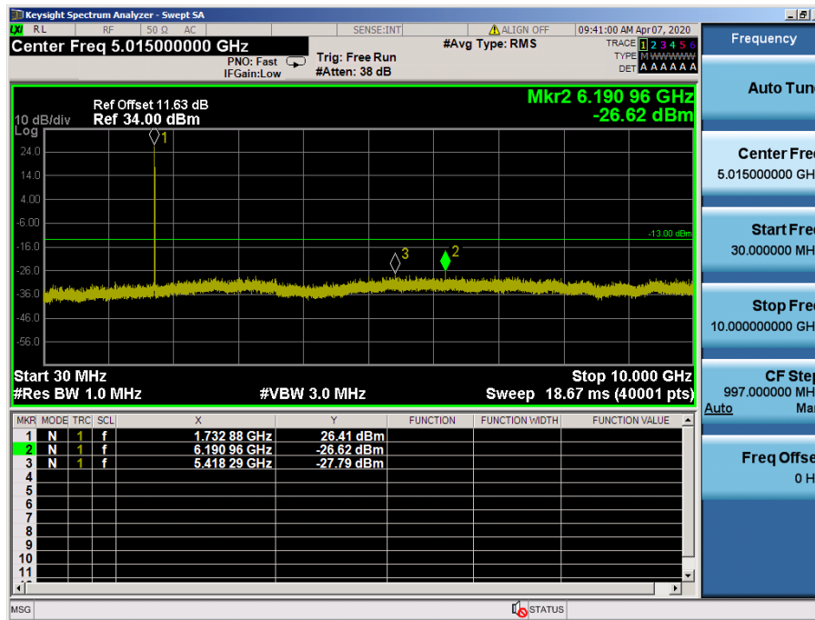
LTE Band 4 / 3MHz / 64QAM - RB Size/Offset (15/0) – Mid Channel
