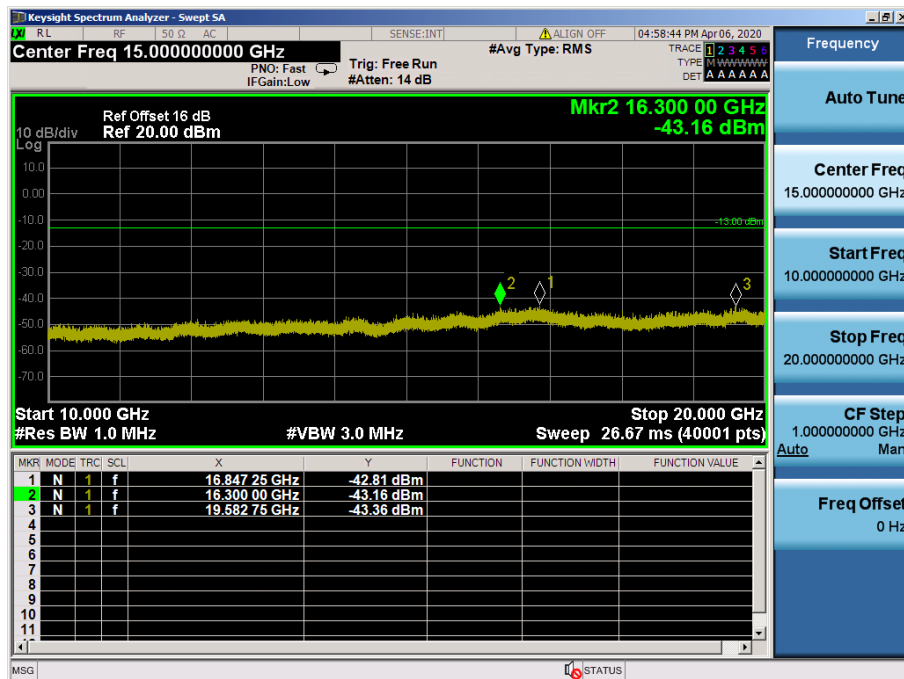
LTE Band 2 / 5MHz / 16QAM - RB Size/Offset (1/0) – Mid Channel
