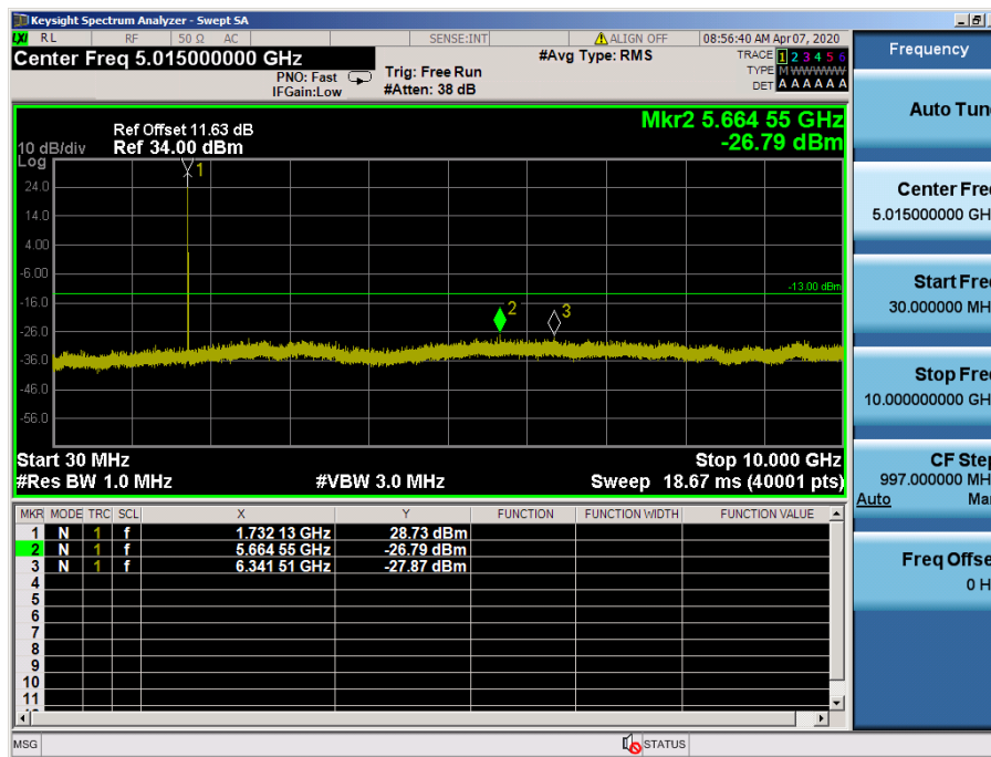
LTE Band 4 / 1.4MHz / 64QAM - RB Size/Offset (6/0) – Mid Channel
