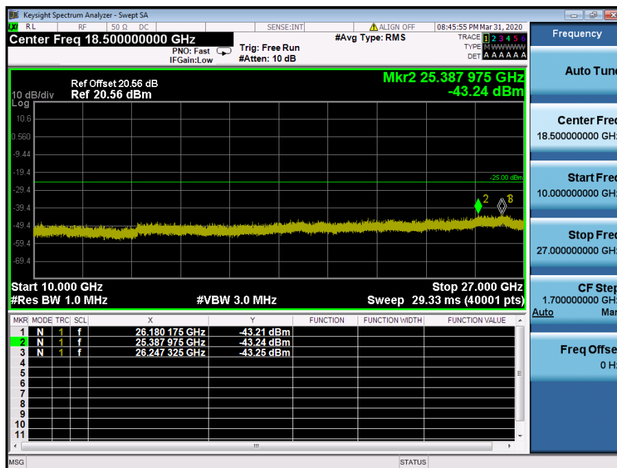
LTE Band 41 / 15MHz / 16QAM - RB Size/Offset (75/0) – Mid Channel
