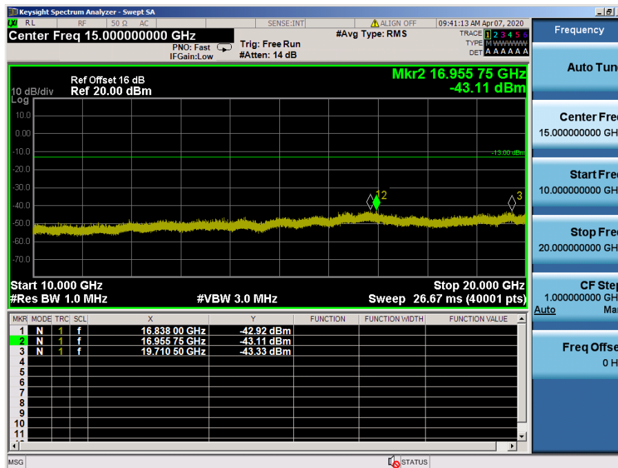
LTE Band 4 / 3MHz / 64QAM - RB Size/Offset (15/0) – Mid Channel
