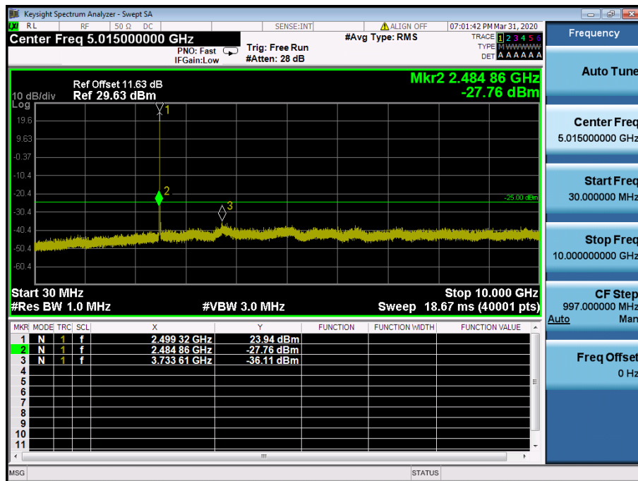
LTE Band 41 / 5MHz / 16QAM - RB Size/Offset (25/0) – Low Channel
