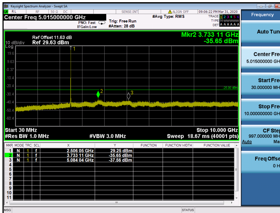
LTE Band 41 / 20MHz / 16QAM - RB Size/Offset (1/50) – Low Channel
