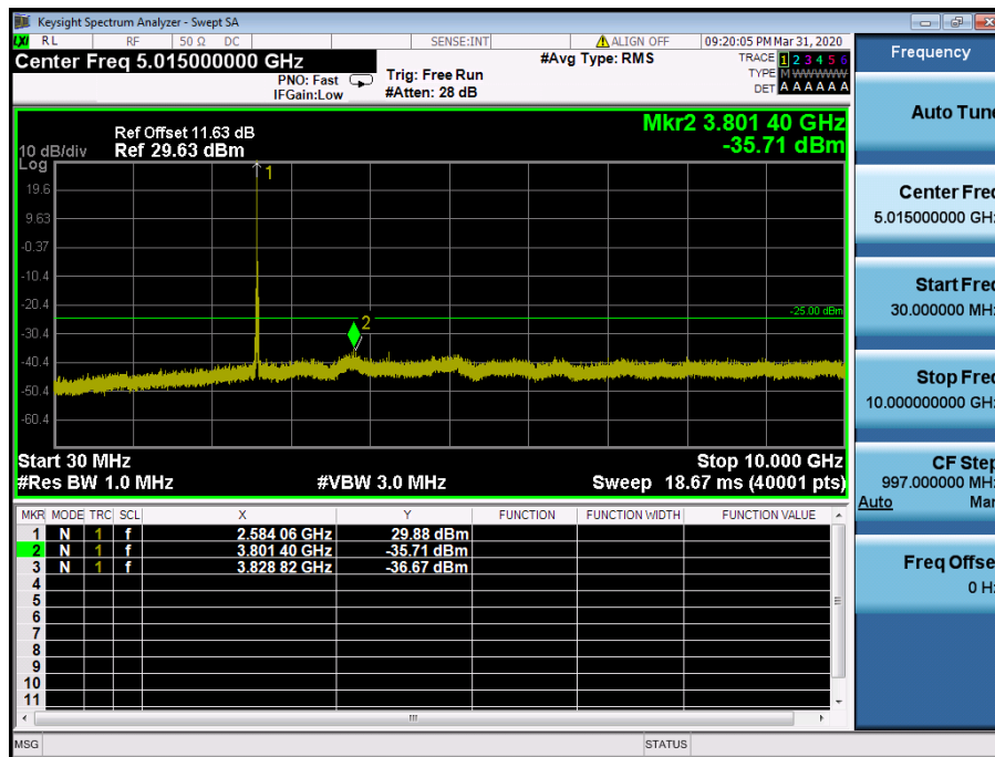
LTE Band 41 / 20MHz / 16QAM - RB Size/Offset (1/0) – Mid Channel
