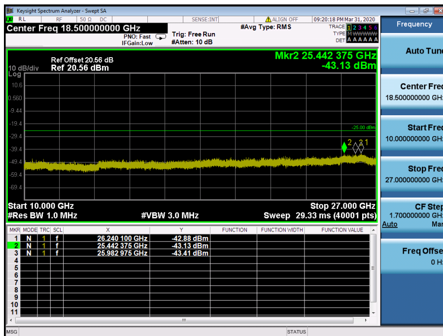
LTE Band 41 / 20MHz / 16QAM - RB Size/Offset (1/0) – Mid Channel
