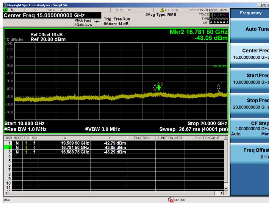
LTE Band 2 / 3MHz / 64QAM - RB Size/Offset (8/4) – High Channel
