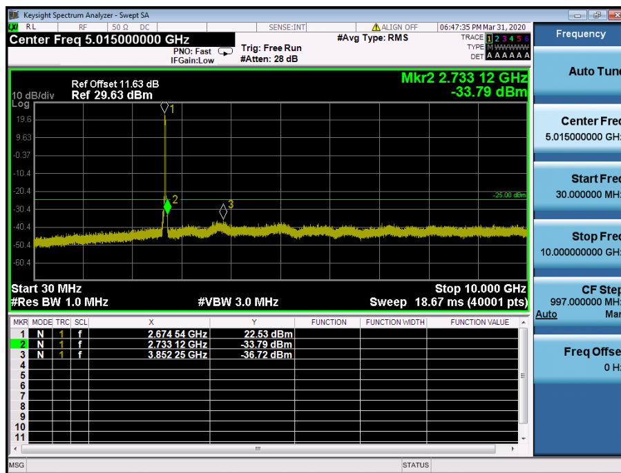
LTE Band 41 / 20MHz / QPSK - RB Size/Offset (100/0) – High Channel
