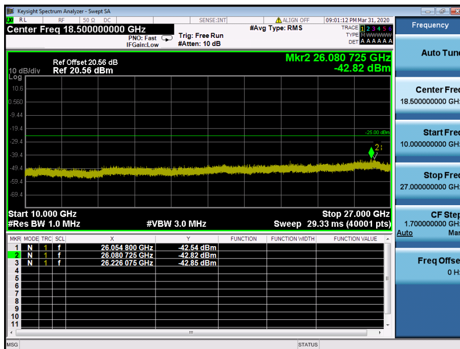
LTE Band 41 / 15MHz / 16QAM - RB Size/Offset (75/0) – High Channel
