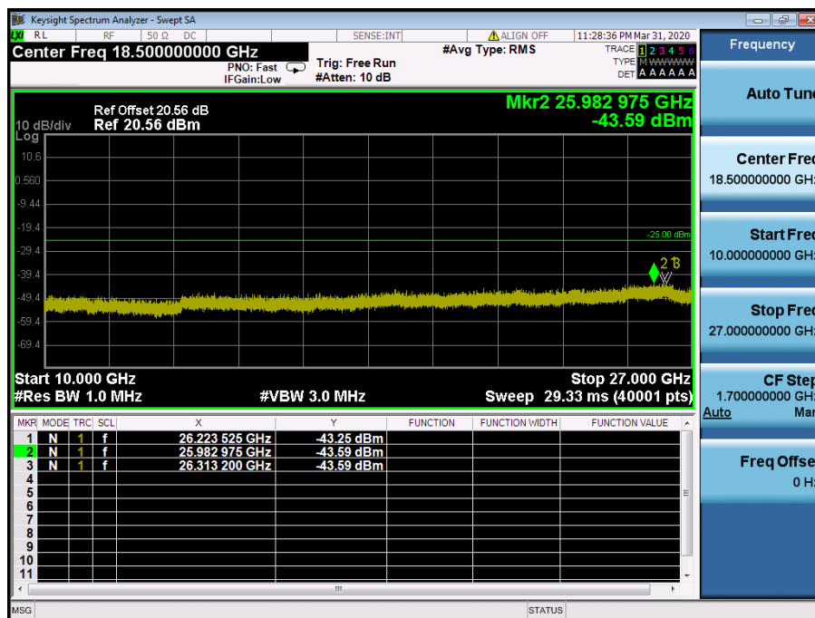
LTE Band 41 / 15MHz / 64QAM - RB Size/Offset (36/39) – Low Channel
