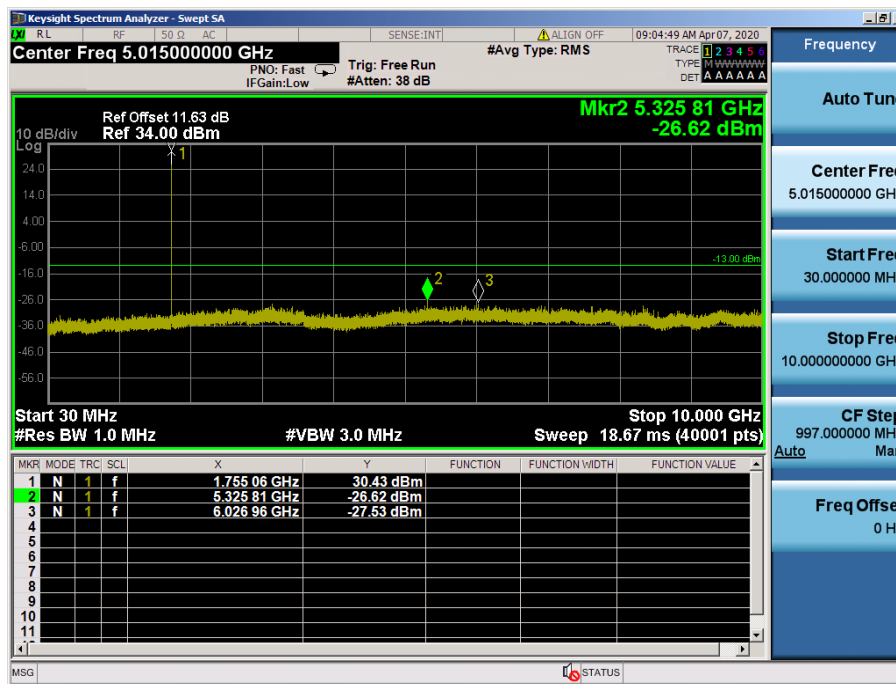
LTE Band 4 / 1.4MHz / 64QAM - RB Size/Offset (1/5) – High Channel
