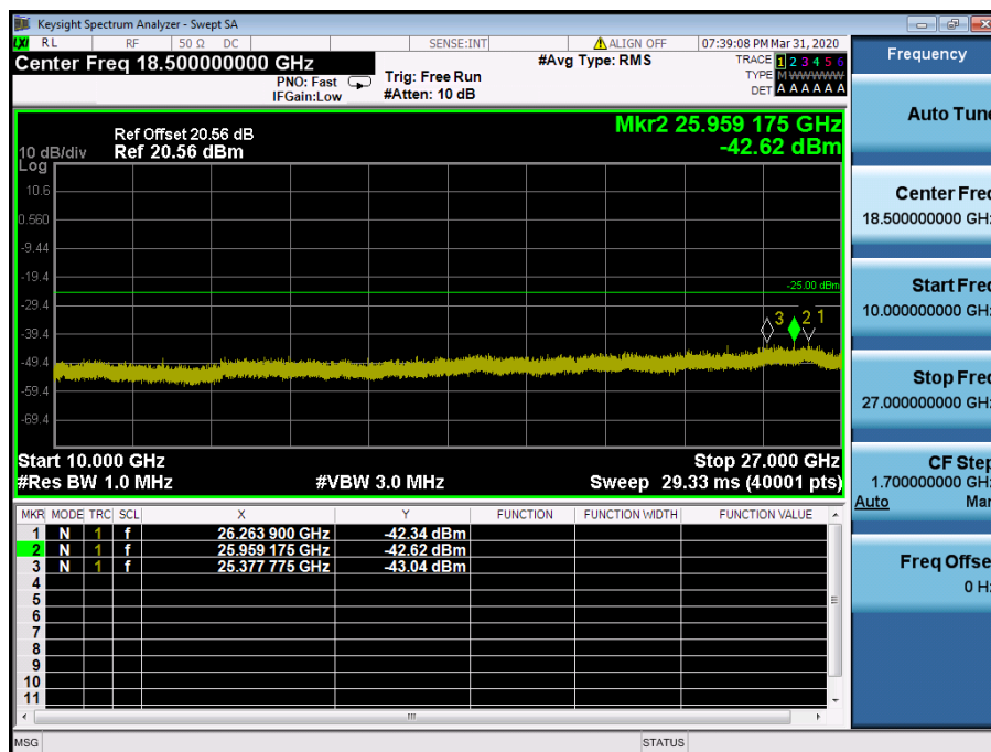
LTE Band 41 / 10MHz / 16QAM - RB Size/Offset (25/0) – Low Channel
