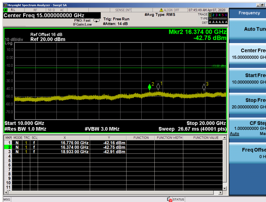
LTE Band 4 / 15MHz / 16QAM - RB Size/Offset (36/39) – High Channel
