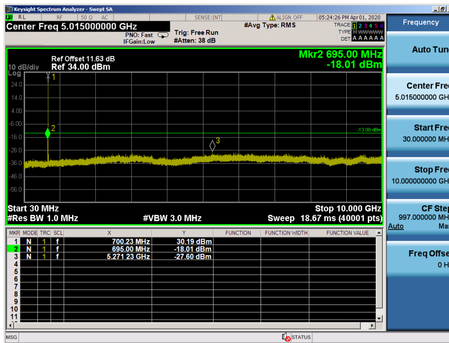
LTE Band 12 / 1.4MHz / QPSK - RB Size/Offset (6/0) – Low Channel
