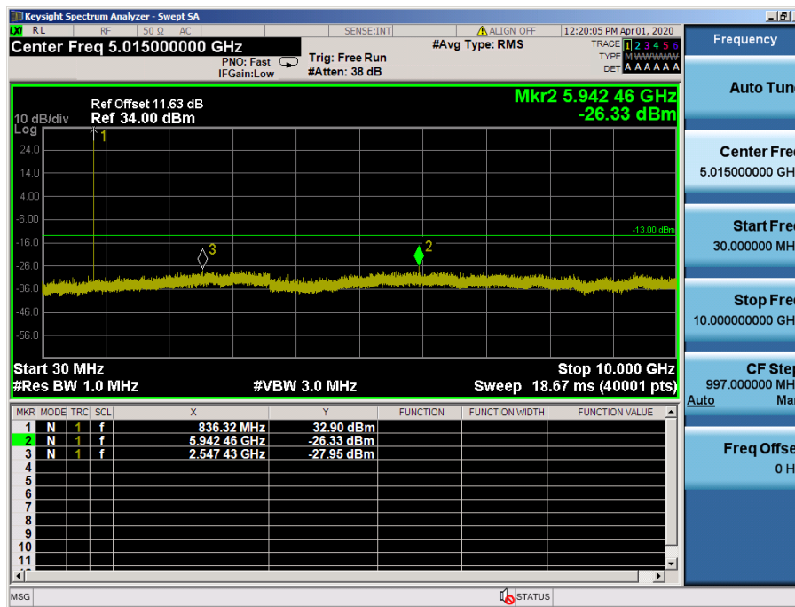
LTE Band 5 / 1.4MHz / 16QAM - RB Size/Offset (3/0) – Mid Channel
