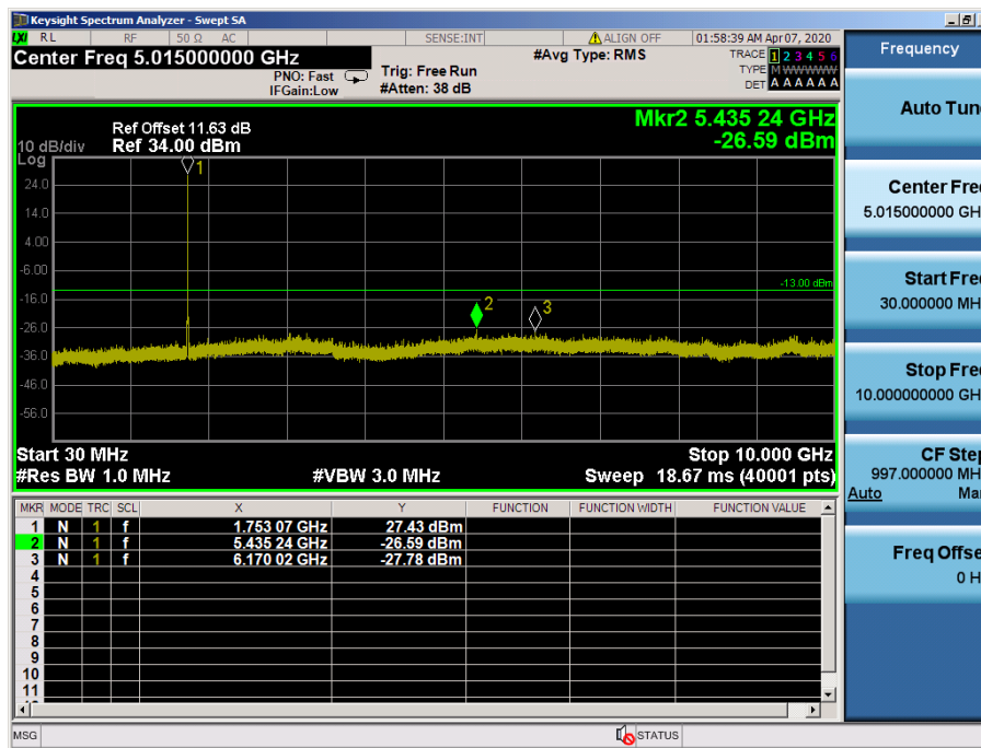
LTE Band 4 / 5MHz / QPSK - RB Size/Offset (12/13) – High Channel
