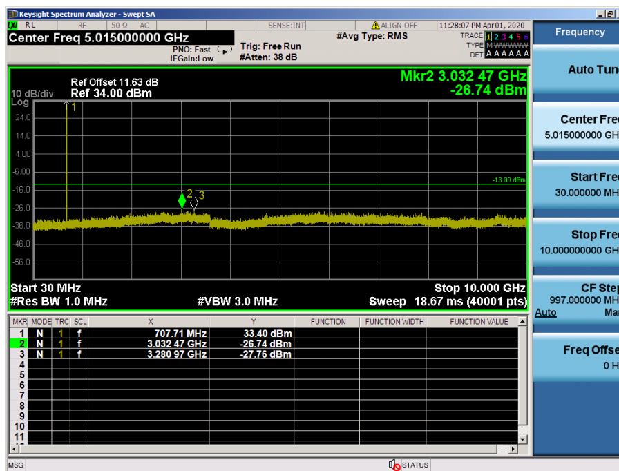
LTE Band 12, 17 / 5MHz / 64QAM - RB Size/Offset (1/12) – Mid Channel
