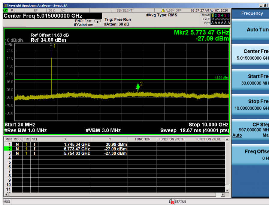
LTE Band 4 / 20MHz / QPSK - RB Size/Offset (1/50) – High Channel
