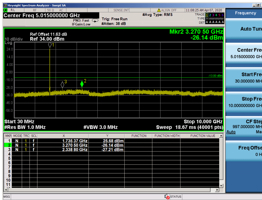
LTE Band 4 / 10MHz / 64QAM - RB Size/Offset (25/25)– Mid Channel
