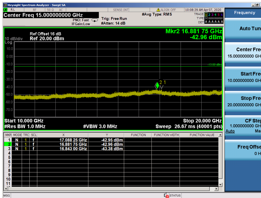
LTE Band 4 / 5MHz / 64QAM - RB Size/Offset (1/24) – Low Channel
