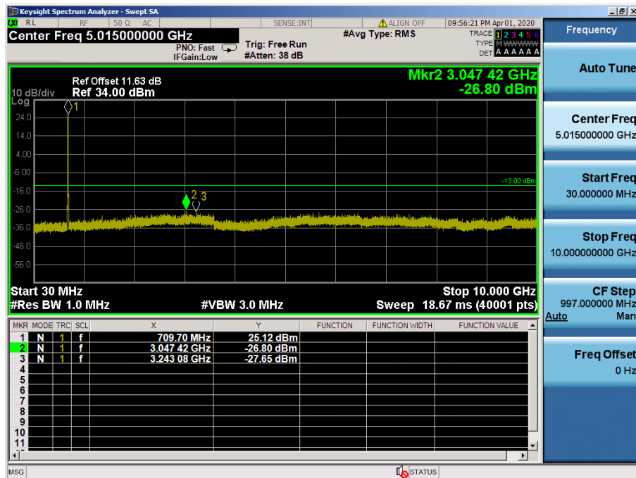
LTE Band 12, 17 / 10MHz / 16QAM - RB Size/Offset (50/0) – High Channel
