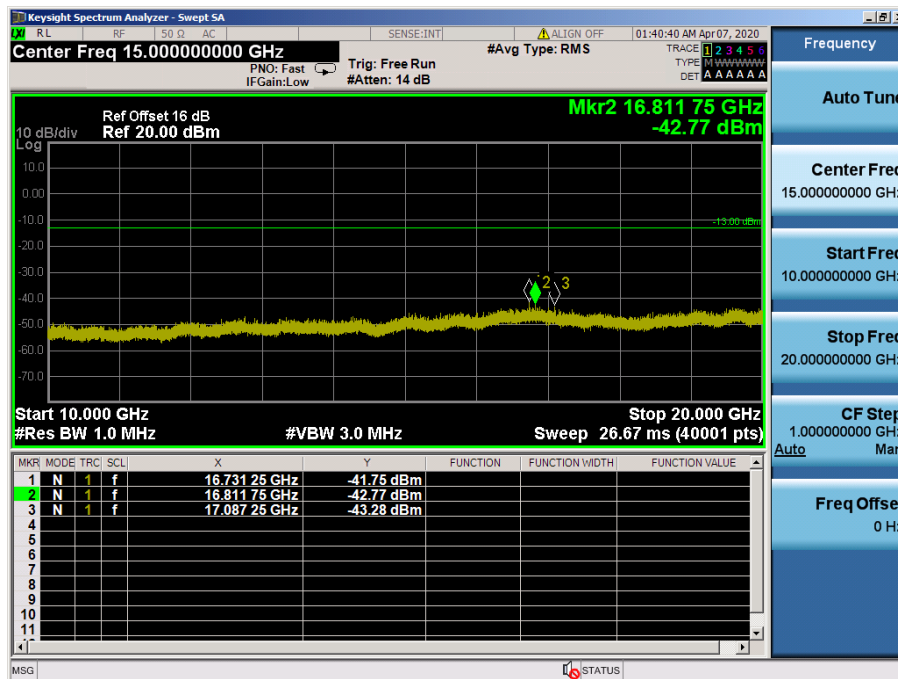
LTE Band 4 / 5MHz / QPSK - RB Size/Offset (12/0) – Mid Channel
