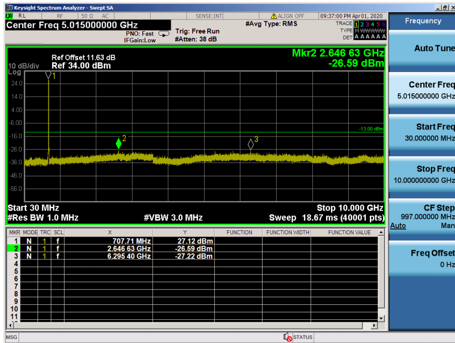
LTE Band 12, 17 / 10MHz / 16QAM - RB Size/Offset (25/25) – Low Channel
