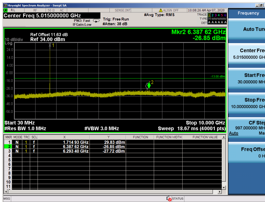
LTE Band 4 / 5MHz / 64QAM - RB Size/Offset (1/24) – Low Channel
