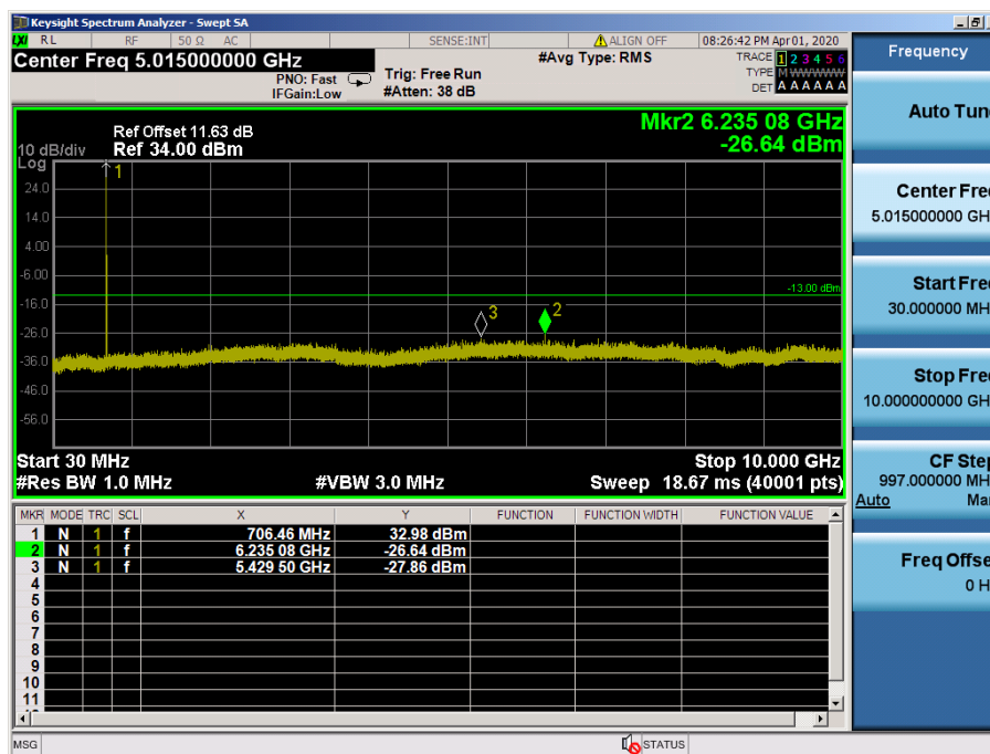
LTE Band 12 / 3MHz / 16QAM - RB Size/Offset (1/0) – Mid Channel
