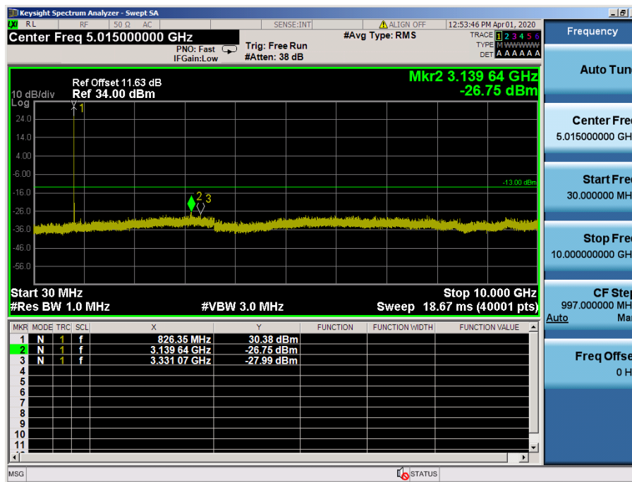
LTE Band 5 / 3MHz / 16QAM - RB Size/Offset (8/7) – Low Channel
