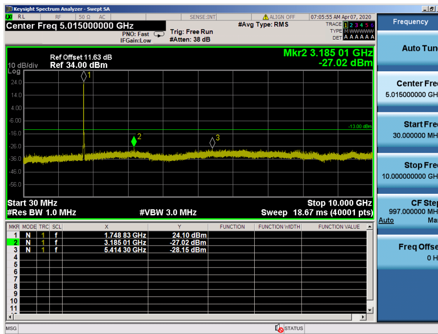
LTE Band 4 / 10MHz / 16QAM - RB Size/Offset (50/0) – High Channel
