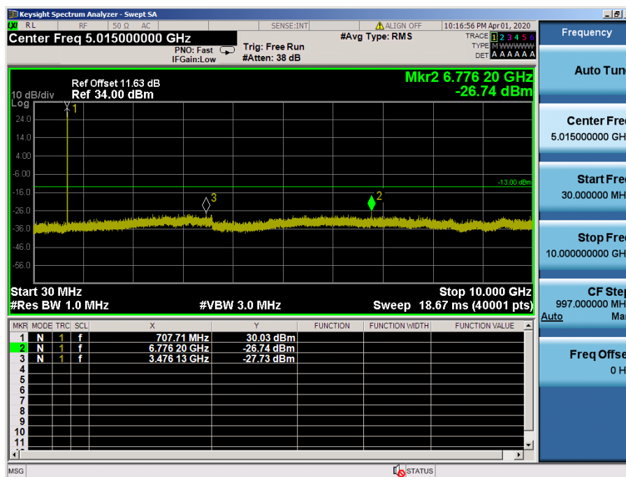
LTE Band 12 / 1.4MHz / 64QAM - RB Size/Offset (6/0) – Mid Channel
