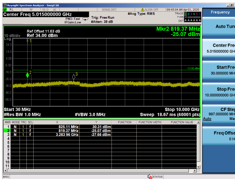
LTE Band 5 / 1.4MHz / QPSK - RB Size/Offset (6/0) – Low Channel
