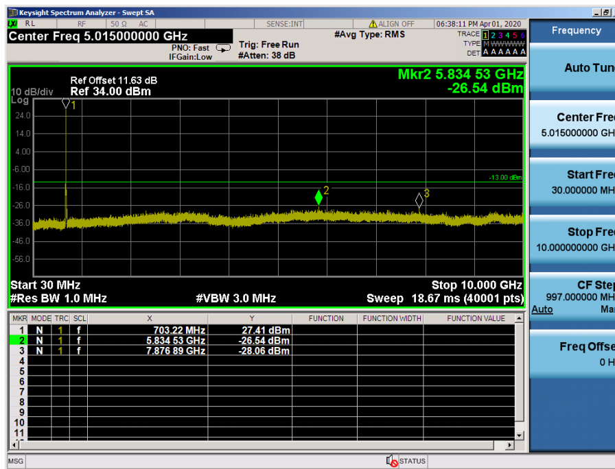
LTE Band 12, 17 / 5MHz / QPSK - RB Size/Offset (25/0) – Low Channel
