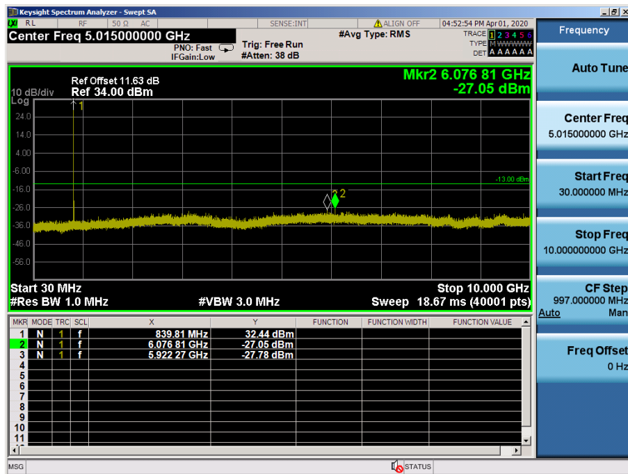
LTE Band 5 / 10MHz / 64QAM - RB Size/Offset (1/0) – High Channel
