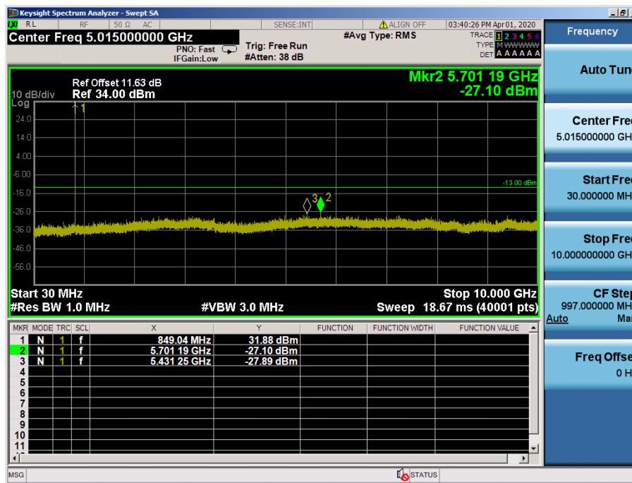
LTE Band 5 / 3MHz / 64QAM - RB Size/Offset (1/14) – High Channel
