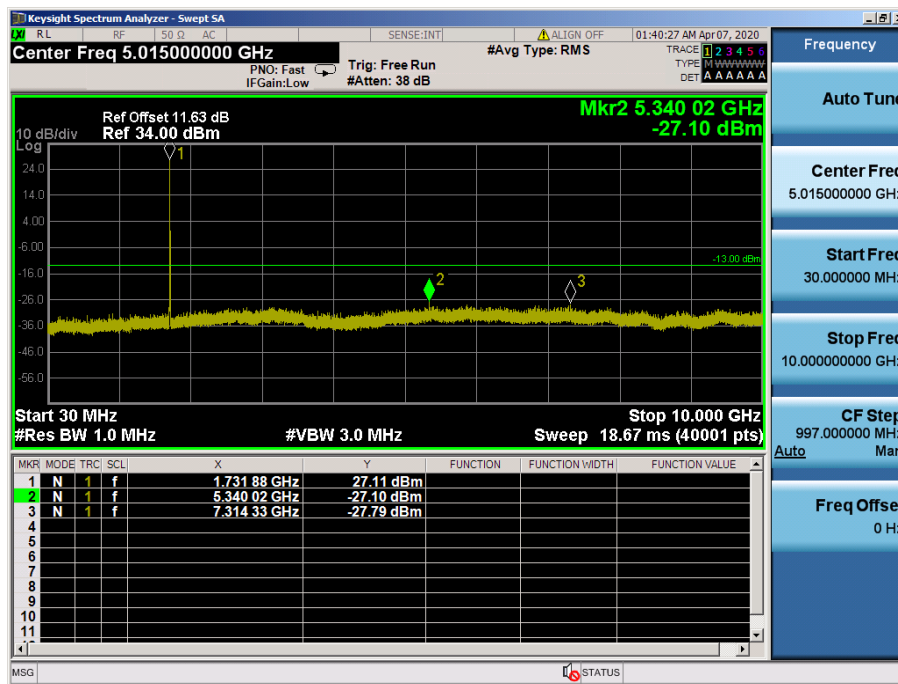
LTE Band 4 / 5MHz / QPSK - RB Size/Offset (12/0) – Mid Channel
