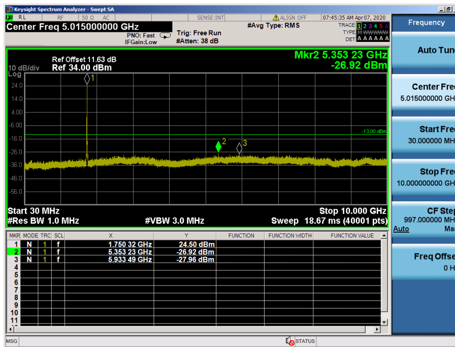
LTE Band 4 / 15MHz / 16QAM - RB Size/Offset (36/39) – High Channel
