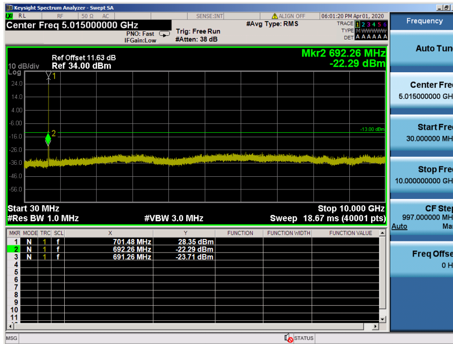
LTE Band 12 / 3MHz / QPSK - RB Size/Offset (15/0) – Low Channel
