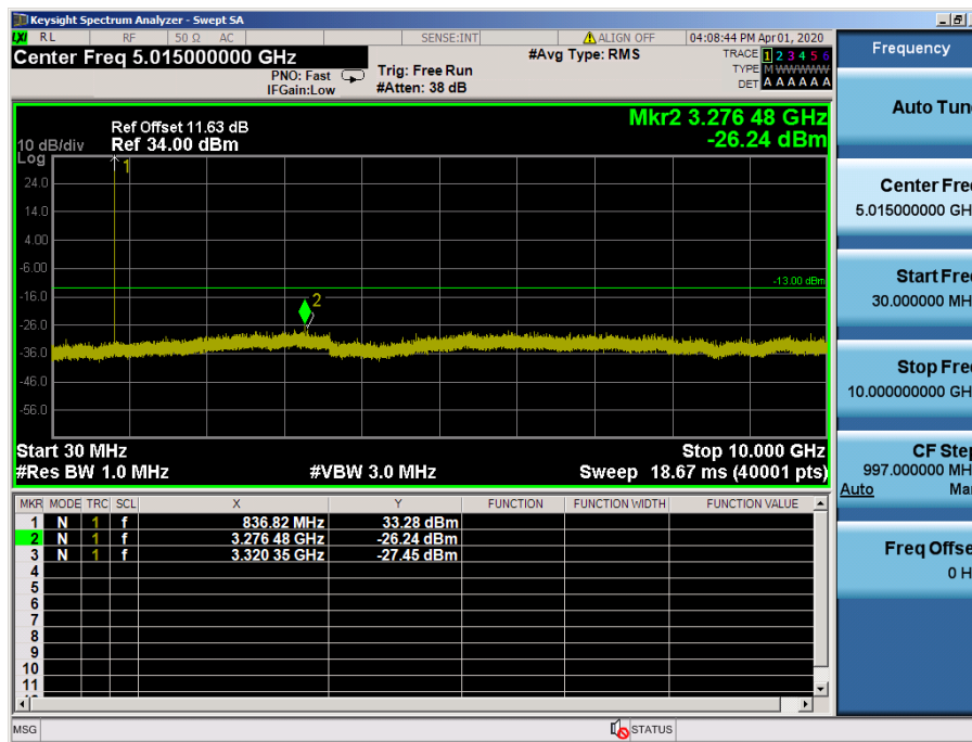
LTE Band 5 / 5MHz / 64QAM - RB Size/Offset (1/12) – Mid Channel
