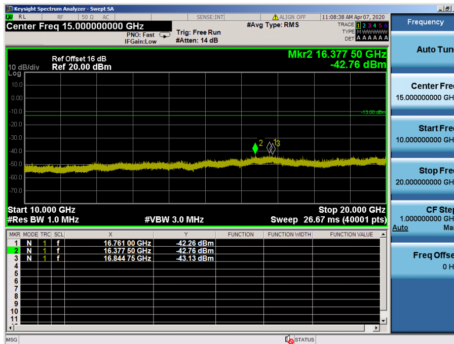
LTE Band 4 / 10MHz / 64QAM - RB Size/Offset (25/25)– Mid Channel
