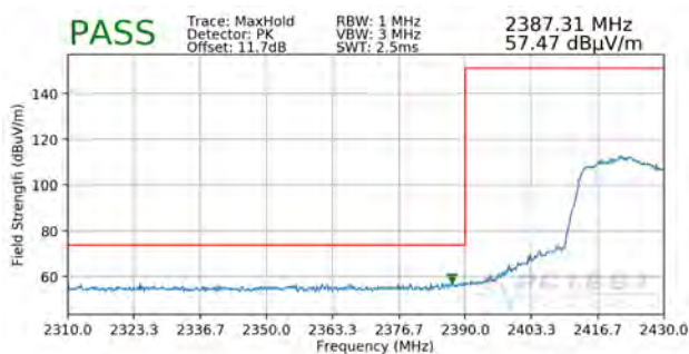
Plot 7-36. Radiated Restricted Lower Band Edge Measurement SISO ANT2 (Peak)
