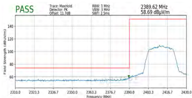
Plot 7-66. Radiated Restricted Band Edge Measurement MIMO with WCP and DS (Peak)
