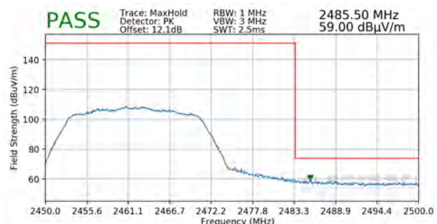
Plot 7-42. Radiated Restricted Upper Band Edge Measurement SISO ANT2 (Peak)
