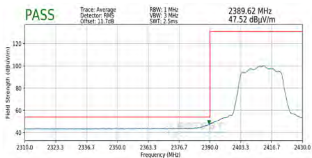
Plot 7-65. Radiated Restricted Band Edge Measurement MIMO with WCP and DS (Average)
