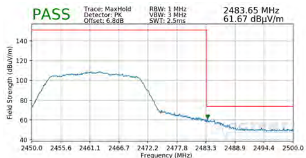
Plot 7-60. Radiated Restricted Upper Band Edge Measurement MIMO (Peak)
