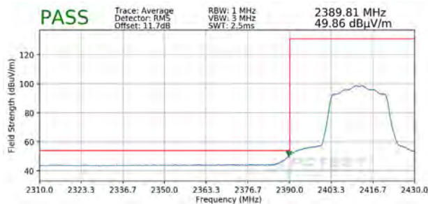
Plot 7-13. Radiated Restricted Lower Band Edge Measurement SISO ANT1 (Average)
