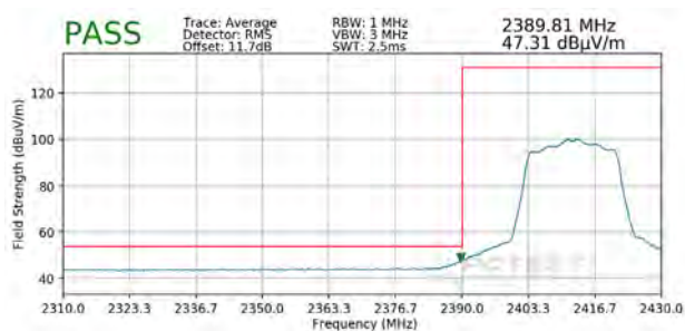
Plot 7-43. Radiated Restricted Band Edge Measurement SISO ANT2 with WCP (Average)
