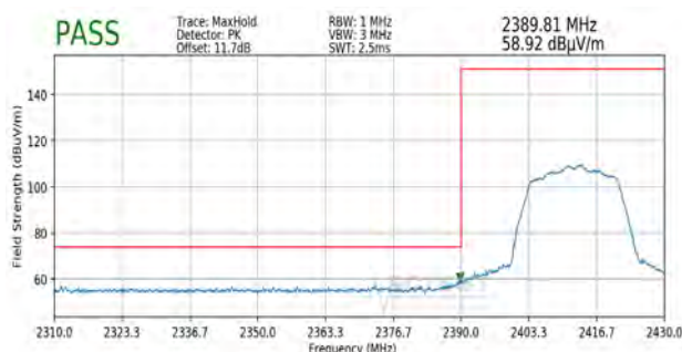
Plot 7-64. Radiated Restricted Band Edge Measurement MIMO with DS (Peak)
