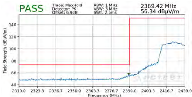
Plot 7-54. Radiated Restricted Lower Band Edge Measurement MIMO (Peak)
