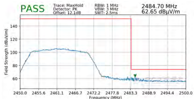
Plot 7-24. Radiated Restricted Upper Band Edge Measurement SISO ANT1 (Peak)
