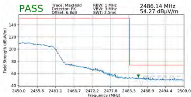
Plot 7-56. Radiated Restricted Upper Band Edge Measurement MIMO (Peak)
