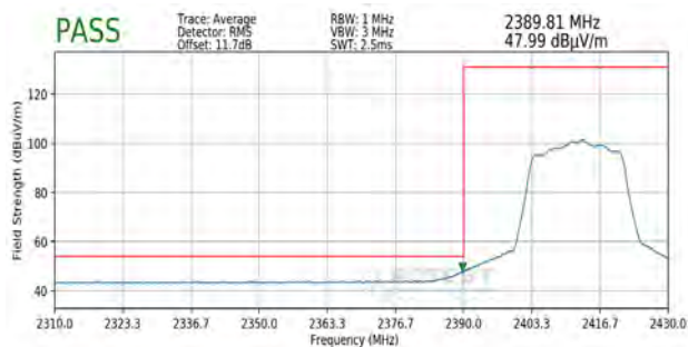
Plot 7-61. Radiated Restricted Band Edge Measurement MIMO with WCP (Average)
