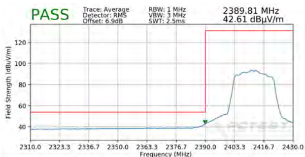
Plot 7-47. Radiated Restricted Band Edge Measurement SISO ANT2 with WCP and DS (Average)
