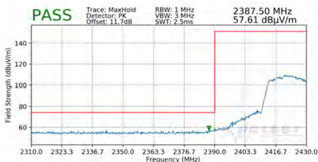
Plot 7-18. Radiated Restricted Lower Band Edge Measurement SISO ANT1 (Peak)
