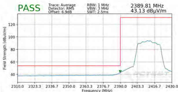
Plot 7-45. Radiated Restricted Band Edge Measurement SISO ANT2 with DS (Average)
