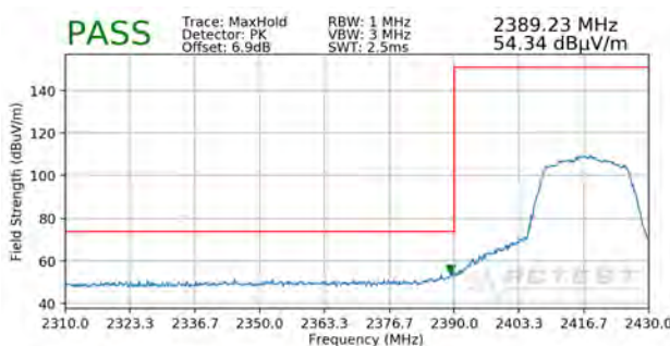
Plot 7-52. Radiated Restricted Lower Band Edge Measurement MIMO (Peak)
