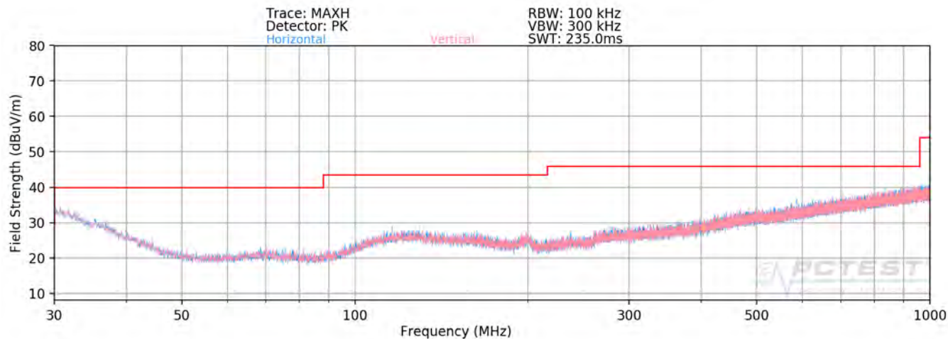
Plot 7-68. Radiated Spurious Plot below 1GHz SISO ANT2
