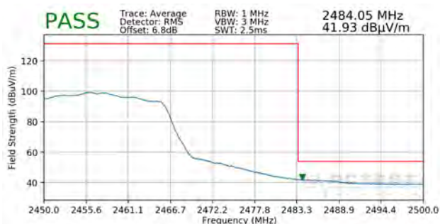
Plot 7-57. Radiated Restricted Upper Band Edge Measurement MIMO (Average)
