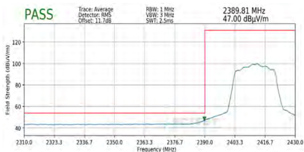
Plot 7-63. Radiated Restricted Band Edge Measurement MIMO with DS (Average)
