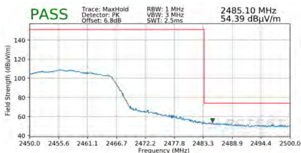
Plot 7-58. Radiated Restricted Upper Band Edge Measurement MIMO (Peak)
