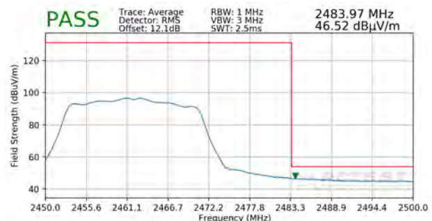
Plot 7-23. Radiated Restricted Upper Band Edge Measurement SISO ANT1 (Average)
