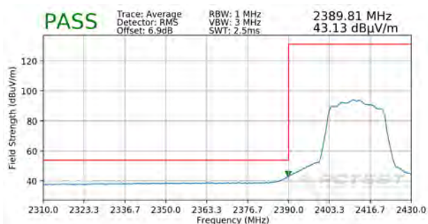
Plot 7-31. Radiated Restricted Lower Band Edge Measurement SISO ANT2 (Average)
