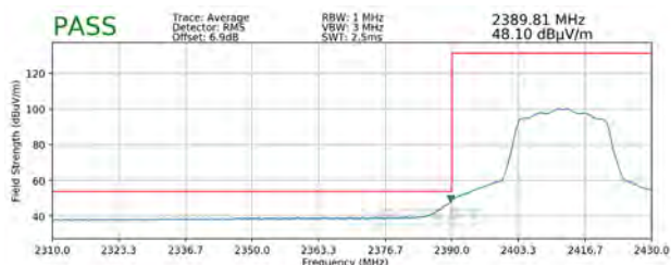
Plot 7-49. Radiated Restricted Lower Band Edge Measurement MIMO (Average)
