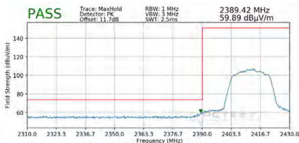
Plot 7-26. Radiated Restricted Band Edge Measurement SISO ANT1 with WCP (Peak)
