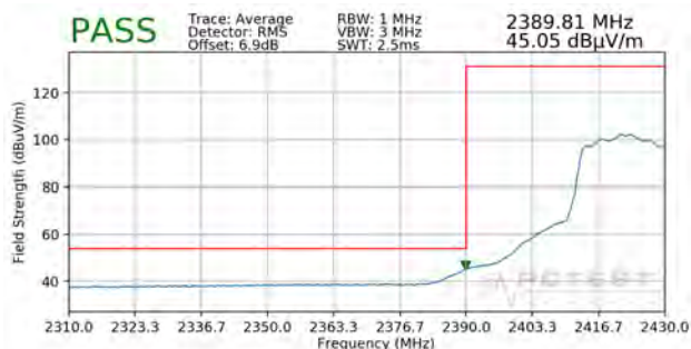
Plot 7-53. Radiated Restricted Lower Band Edge Measurement MIMO (Average)
