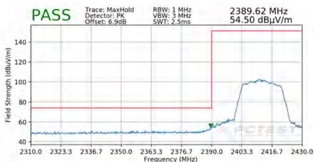
Plot 7-48. Radiated Restricted Band Edge Measurement SISO ANT2 with WCP and DS (Peak)
