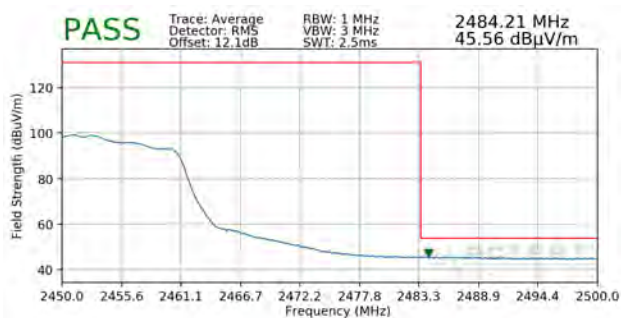
Plot 7-19. Radiated Restricted Upper Band Edge Measurement SISO ANT1 (Average)
