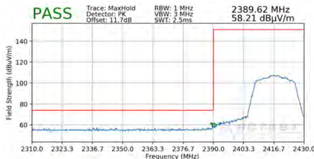
Plot 7-16. Radiated Restricted Lower Band Edge Measurement SISO ANT1 (Peak)
