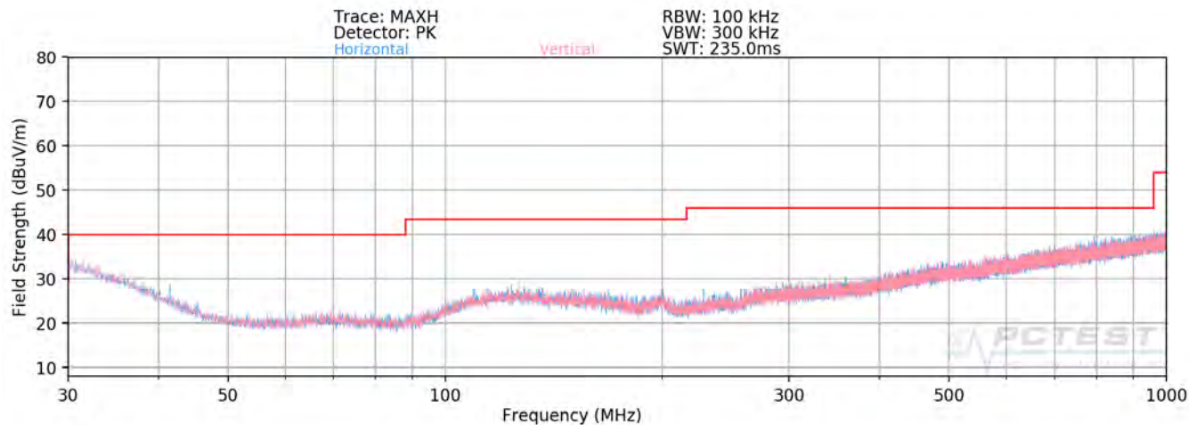
Plot 7-67. Radiated Spurious Plot below 1GHz SISO ANT1
