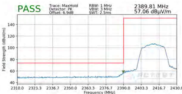
Plot 7-28. Radiated Restricted Band Edge Measurement SISO ANT1 with DS (Peak)
