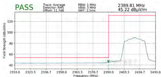
Plot 7-25. Radiated Restricted Band Edge Measurement SISO ANT1 with WCP (Average)
