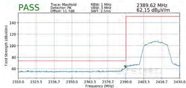
Plot 7-14. Radiated Restricted Lower Band Edge Measurement SISO ANT1 (Peak)
