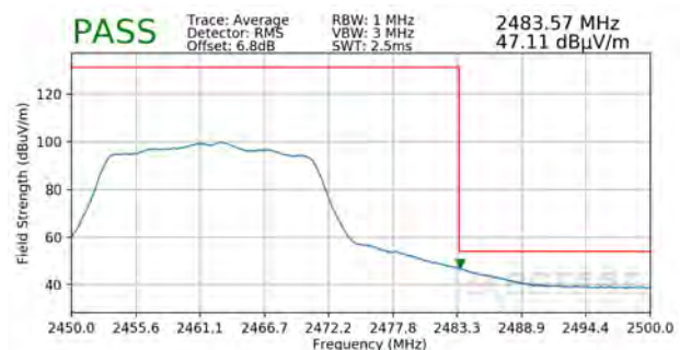
Plot 7-59. Radiated Restricted Upper Band Edge Measurement MIMO (Average)
