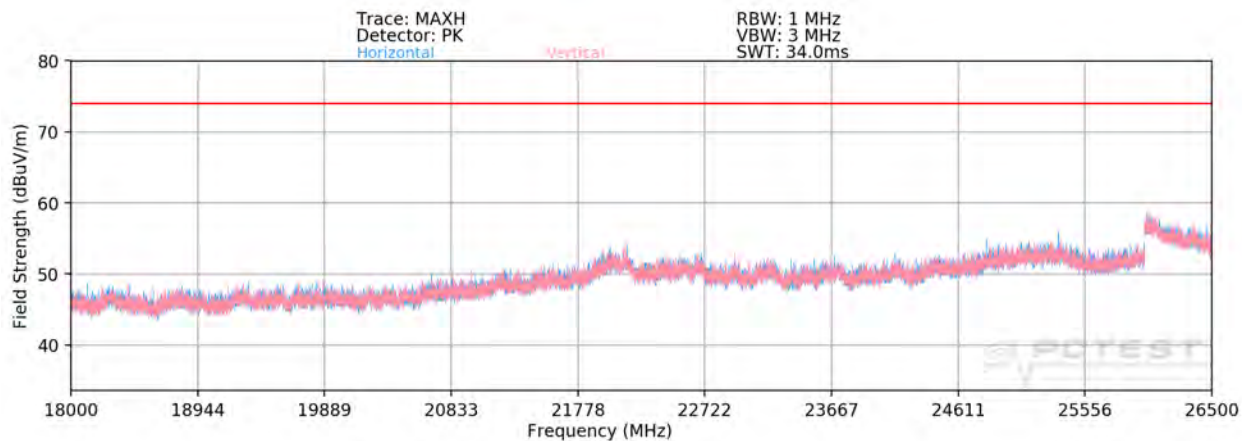
Plot 7-12. Radiated Spurious Plot above 18GHz MIMO/CDD
