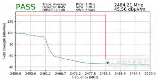
Plot 7-37. Radiated Restricted Upper Band Edge Measurement SISO ANT2 (Average)
