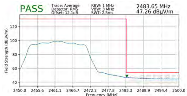
Plot 7-41. Radiated Restricted Upper Band Edge Measurement SISO ANT2 (Average)
