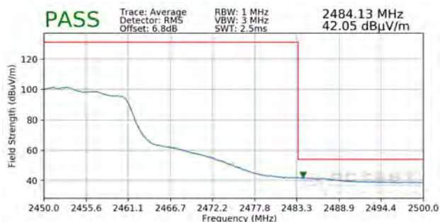
Plot 7-55. Radiated Restricted Upper Band Edge Measurement MIMO (Average)
