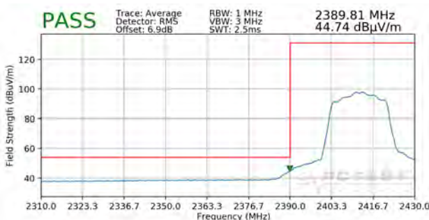
Plot 7-27. Radiated Restricted Band Edge Measurement SISO ANT1 with DS (Average)
