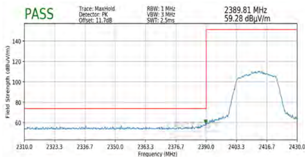
Plot 7-62. Radiated Restricted Band Edge Measurement MIMO with WCP (Peak)
