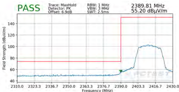
Plot 7-46. Radiated Restricted Band Edge Measurement SISO ANT2 with DS (Peak)
