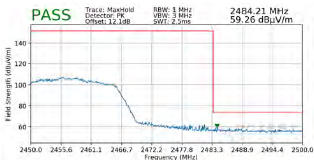
Plot 7-22. Radiated Restricted Upper Band Edge Measurement SISO ANT1 (Peak)
