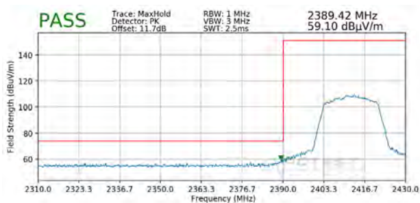
Plot 7-44. Radiated Restricted Band Edge Measurement SISO ANT2 with WCP (Peak)
