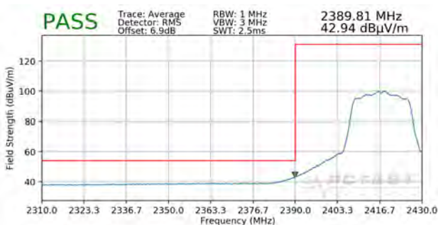
Plot 7-51. Radiated Restricted Lower Band Edge Measurement MIMO (Average)
