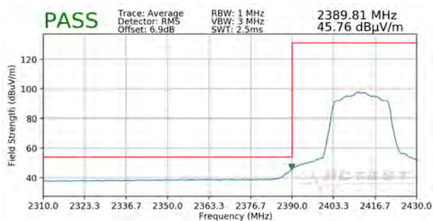
Plot 7-29. Radiated Restricted Band Edge Measurement SISO ANT1 with WCP and DS (Average)
