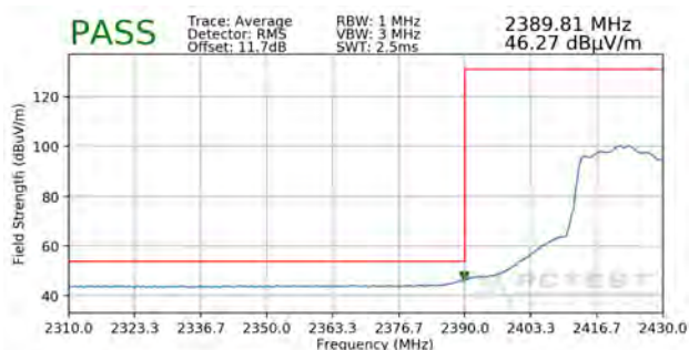
Plot 7-17. Radiated Restricted Lower Band Edge Measurement SISO ANT1 (Average)
