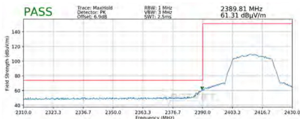
Plot 7-50. Radiated Restricted Lower Band Edge Measurement MIMO (Peak)
