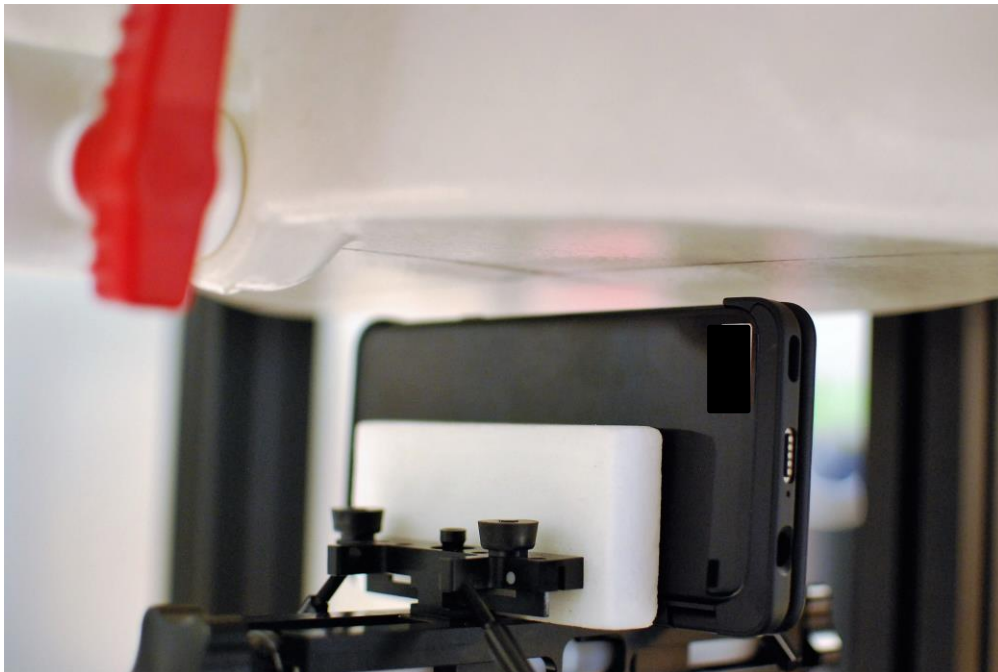
SAR Test Setup Photo 38 – Right Side at 10 mm with Dual Display Cover Position #3 (360 degrees)
