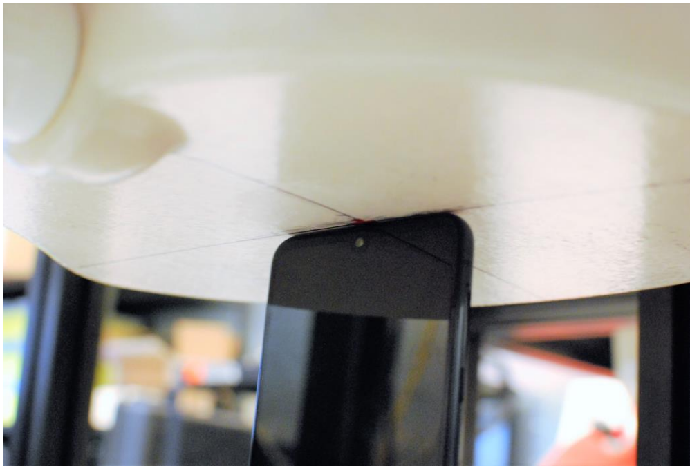
SAR Test Setup Photo 26 – Top Side at 0 mm
