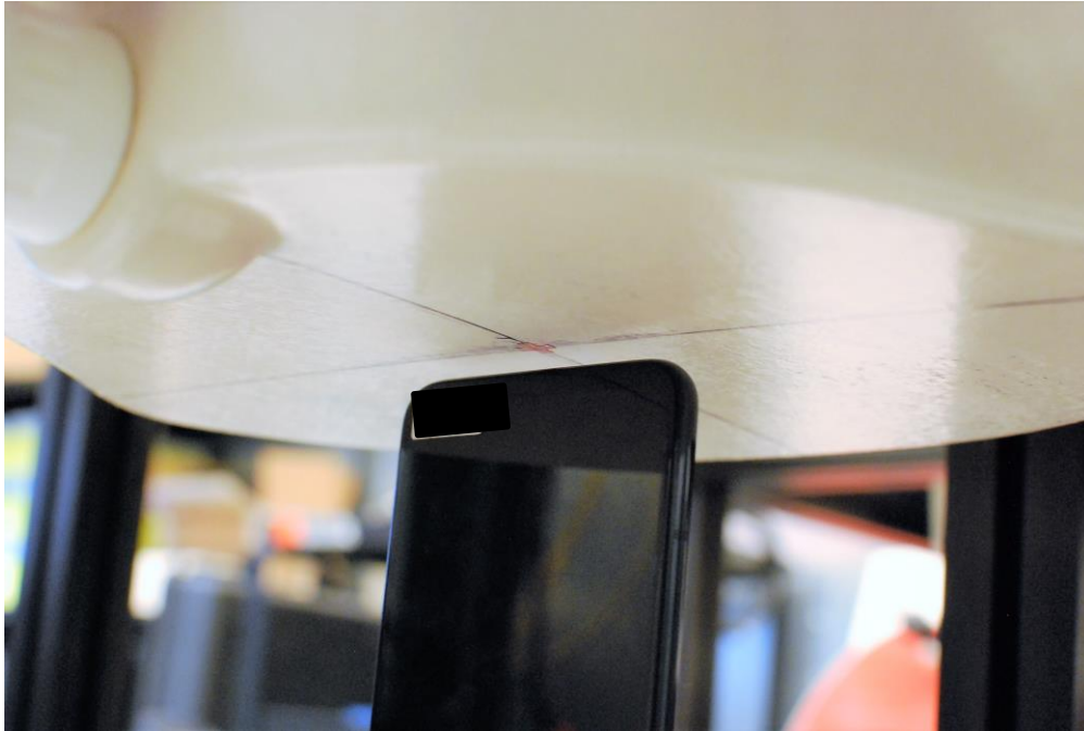
SAR Test Setup Photo 31 – Bottom Side at 3 mm
