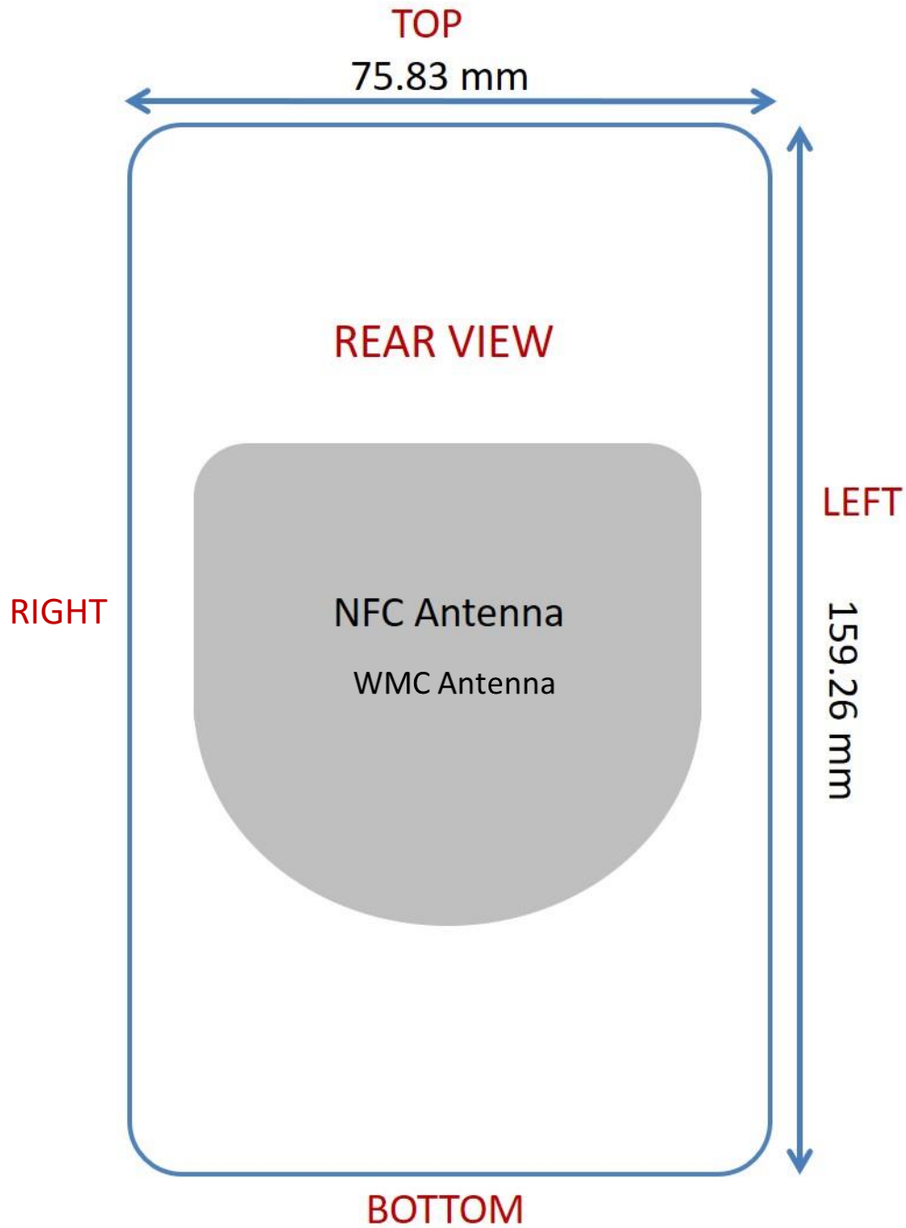
Figure F-2 NFC Antenna Locations
