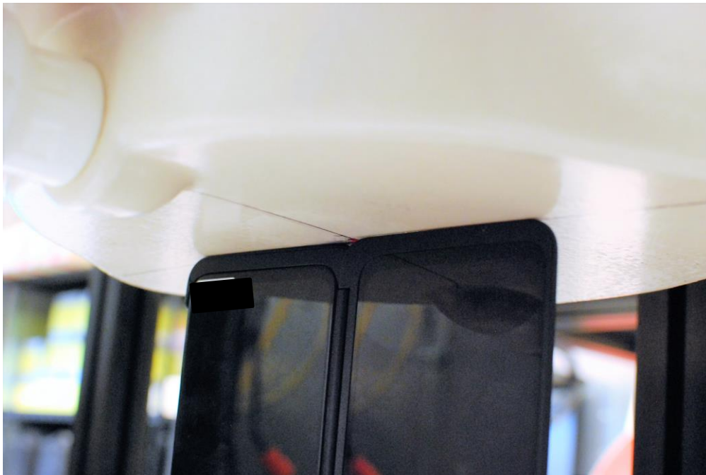
SAR Test Setup Photo 34 – Bottom Side at 0 mm with Dual Display Cover Position #2 (180 degrees)
