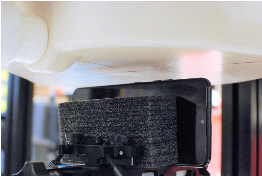
SAR Test Setup Photo 40 – Left Side at 10 mm
