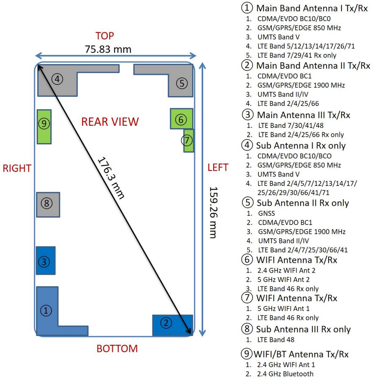
Figure F-1 DUT Antenna Locations
