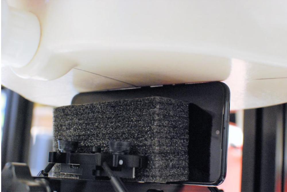
SAR Test Setup Photo 43 – Left Side at 0 mm
