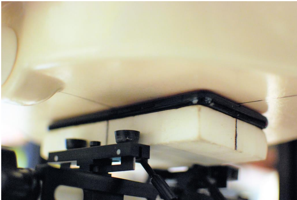
SAR Test Setup Photo 14 – Back Side at 1 mm
