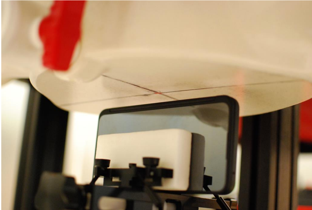
SAR Test Setup Photo 41 – Left Side at 10 mm with Dual Display Cover Position #1 (0 degrees)
