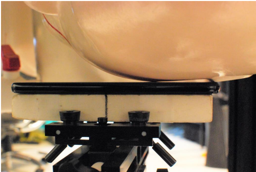
SAR Test Setup Photo 6 – Left Cheek
