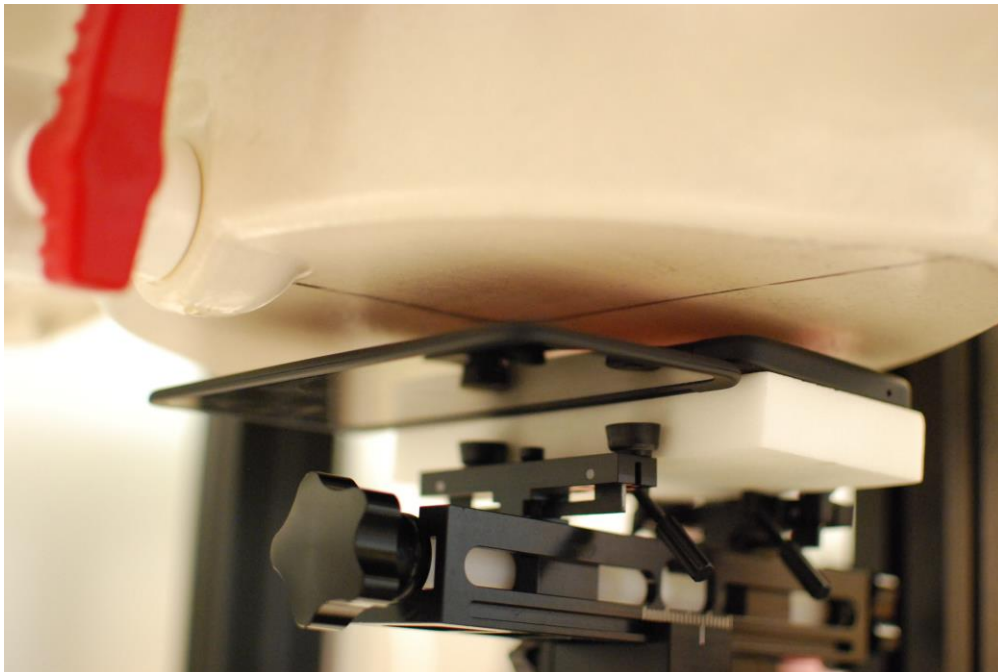
SAR Test Setup Photo 12 – Back Side at 10 mm with Dual Display Cover Position #2 (180 degrees)
