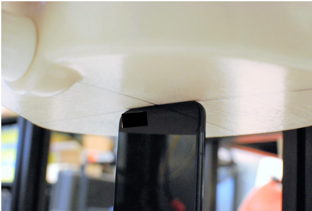
SAR Test Setup Photo 32 – Bottom Side at 0 mm
