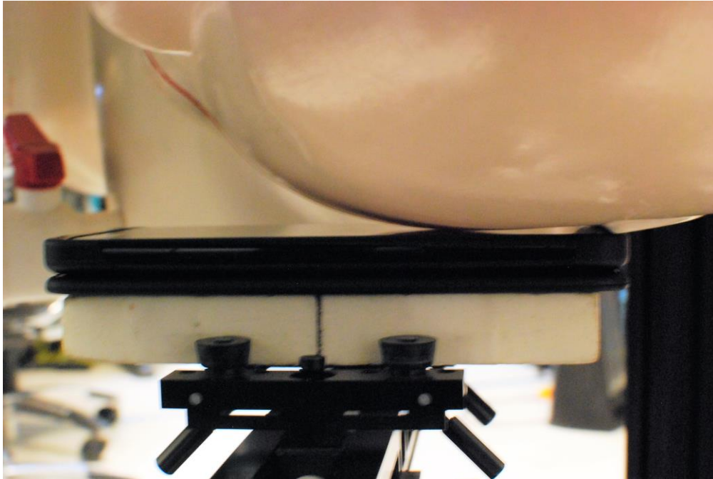
SAR Test Setup Photo 7 – Left Cheek with Dual Display Cover Position #3 (360 degrees)
