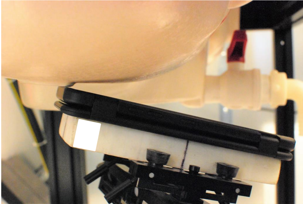
SAR Test Setup Photo 5 – Right Tilt with Dual Display Cover Position #3 (360 degrees)
