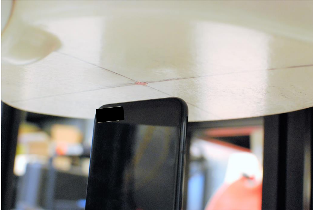
SAR Test Setup Photo 27 – Bottom Side at 10 mm
