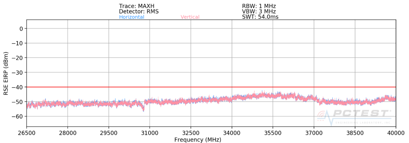
Plot 7-3. Radiated Spurious Plot 26.5 - 40GHz (Band 48)
