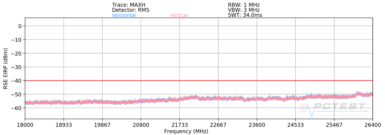
Plot 7-2. Radiated Spurious Plot 18 - 26.5GHz (Band 48)
