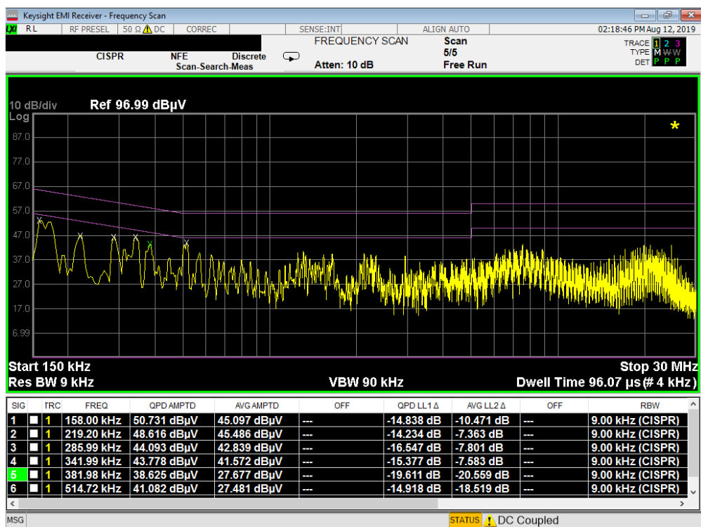
Plot 7-166. Line Conducted Plot with 802.11b (N) with WCP
