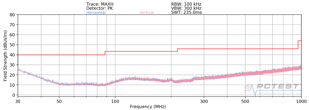
Plot 7-162. Radiated Spurious Plot below 1GHz MIMO/CDD
