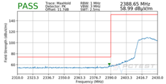
Plot 7-109. Radiated Restricted Lower Band Edge Measurement SISO ANT1 (Peak)
