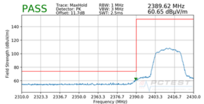
Plot 7-119. Radiated Restricted Lower Band Edge Measurement SISO ANT2 (Peak)
