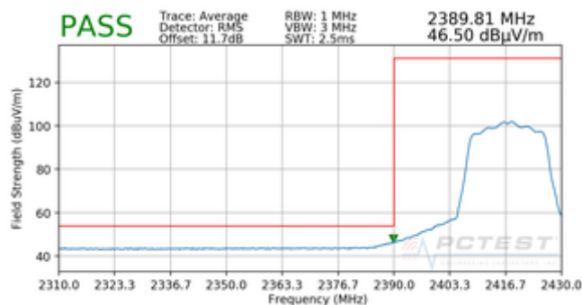
Plot 7-120. Radiated Restricted Lower Band Edge Measurement SISO ANT2 (Average)
