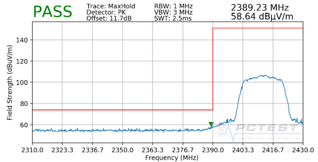
Plot 7-131. Radiated Restricted Band Edge Measurement SISO ANT2 with WCP (Peak)
