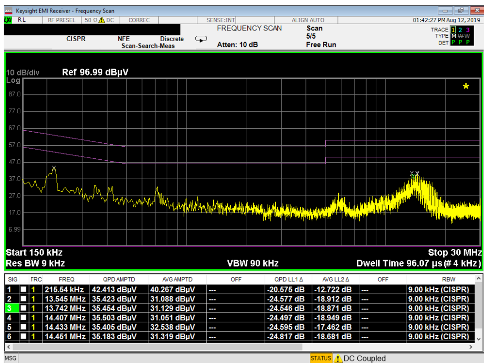
Plot 7-164. Line Conducted Plot with 802.11b (N)
