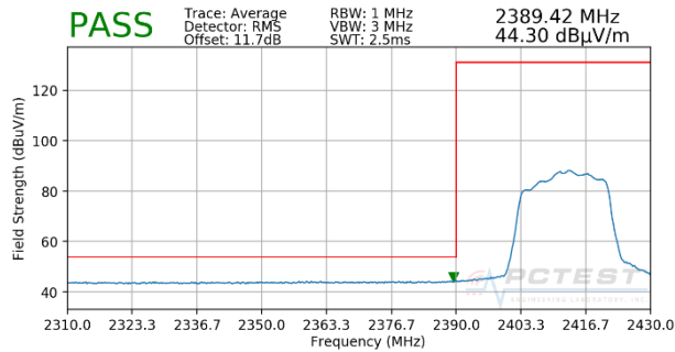
Plot 7-116. Radiated Restricted Band Edge Measurement SISO ANT1 with WCP (Average)
