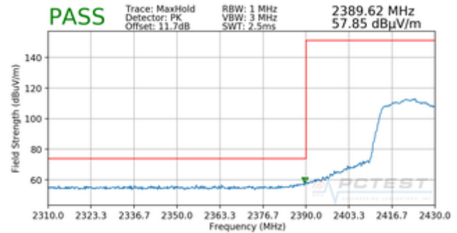
Plot 7-123. Radiated Restricted Lower Band Edge Measurement SISO ANT2 (Peak)
