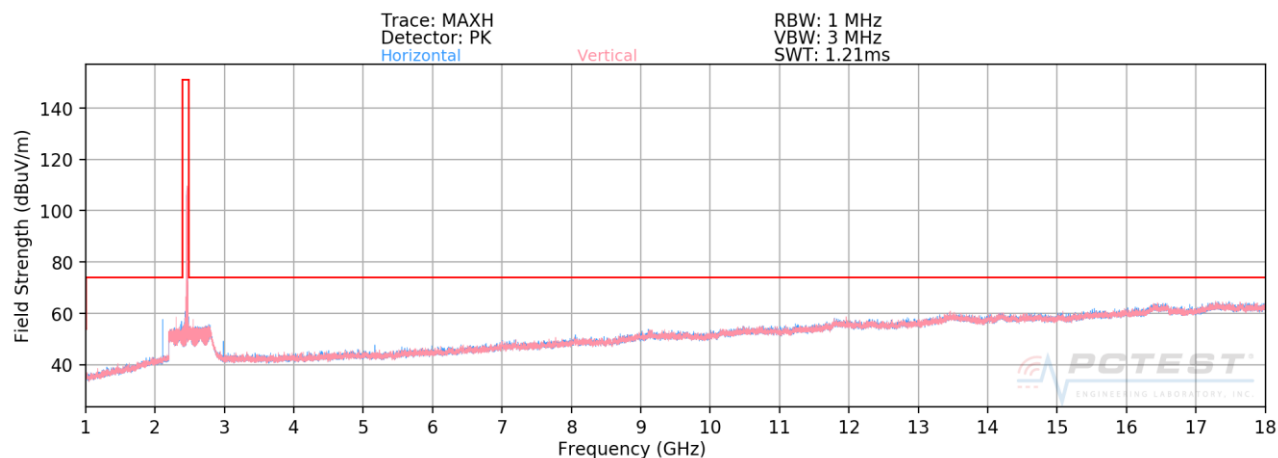
Plot 7-101. Radiated Spurious Plot above 1GHz SISO ANT2 (802.11b – Ch. 11)
