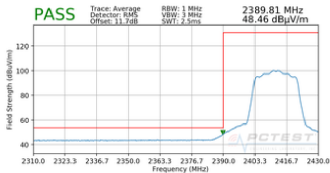
Plot 7-118. Radiated Restricted Lower Band Edge Measurement SISO ANT2 (Average)
