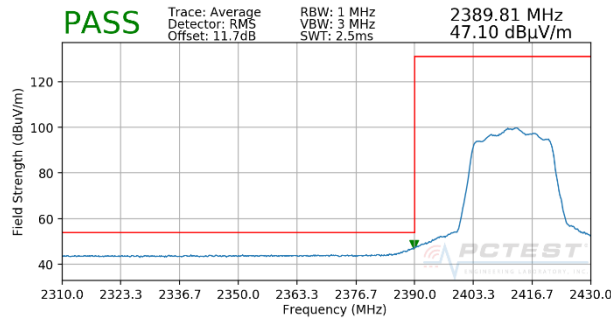
Plot 7-144. Radiated Restricted Band Edge Measurement MIMO with WCP (Average)
