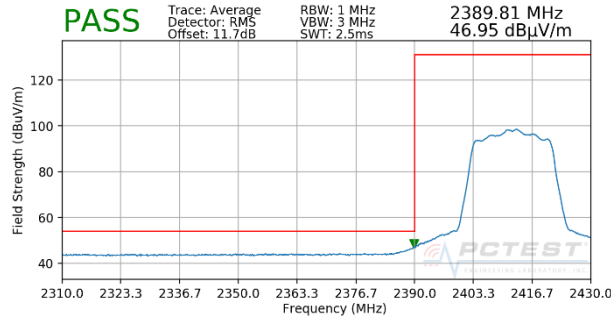
Plot 7-130. Radiated Restricted Band Edge Measurement SISO ANT2 with WCP (Average)
