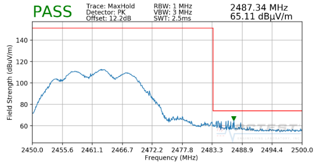
Plot 7-159. Radiated Restricted Band Edge Measurement CDD with WCP (Peak)
