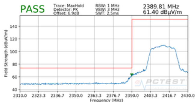
Plot 7-133. Radiated Restricted Lower Band Edge Measurement MIMO (Peak)
