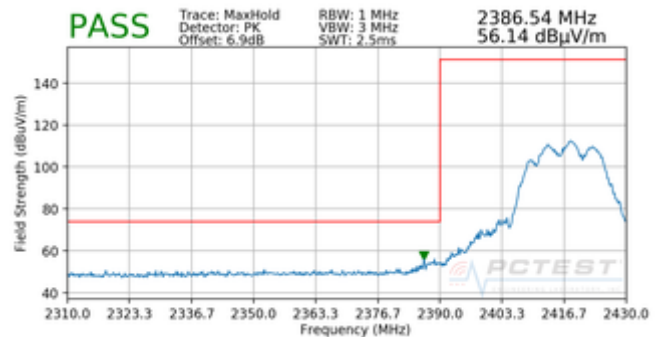
Plot 7-149. Radiated Restricted Lower Band Edge Measurement CDD (Peak)
