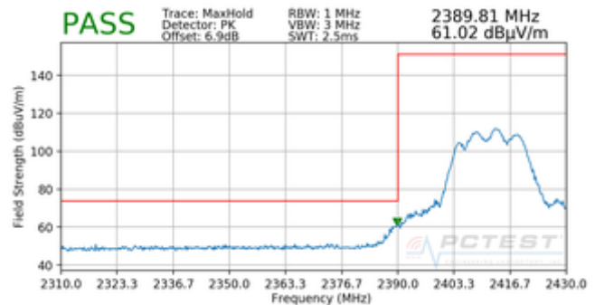
Plot 7-147. Radiated Restricted Lower Band Edge Measurement CDD (Peak)
