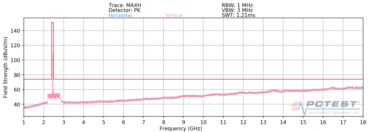
Plot 7-97. Radiated Spurious Plot above 1GHz SISO ANT1 (802.11b – Ch. 11)
