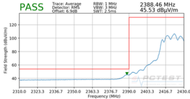
Plot 7-150. Radiated Restricted Lower Band Edge Measurement CDD (Average)
