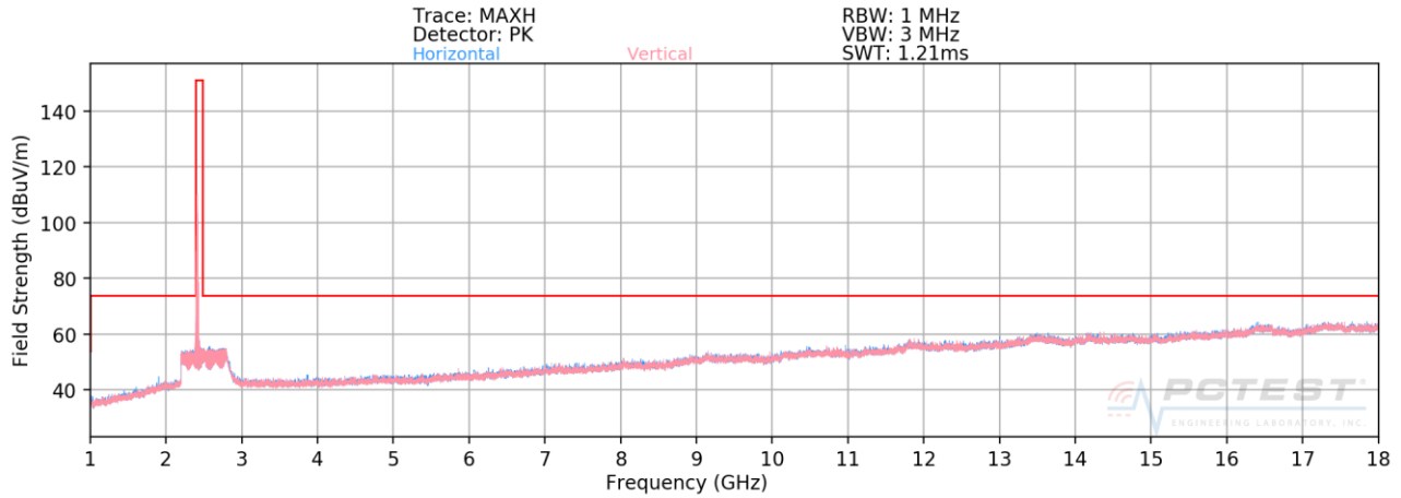
Plot 7-95. Radiated Spurious Plot above 1GHz SISO ANT1 (802.11b – Ch. 1)
