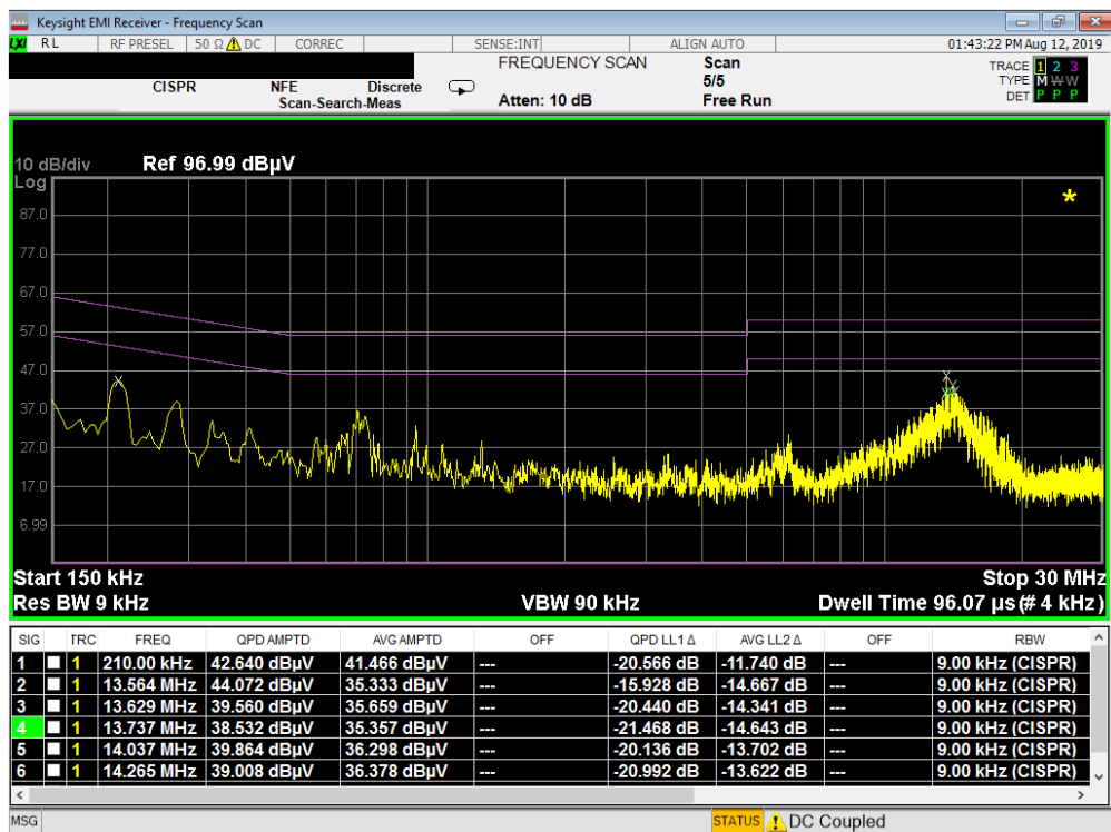
Plot 7-163. Line Conducted Plot with 802.11b (L1)
