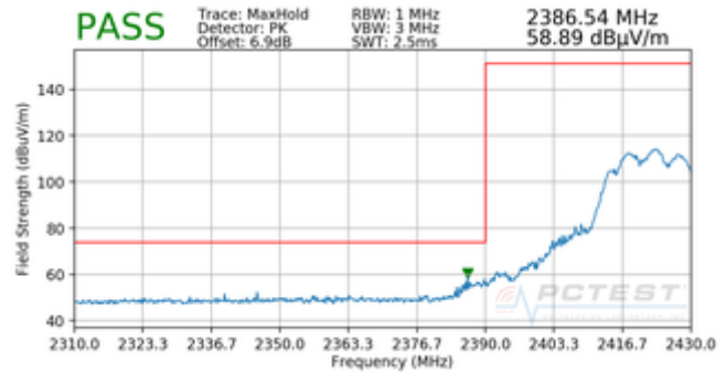
Plot 7-151. Radiated Restricted Lower Band Edge Measurement CDD (Peak)
