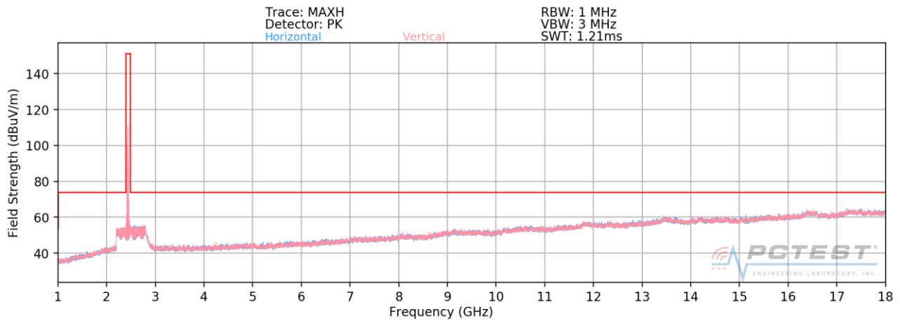
Plot 7-96. Radiated Spurious Plot above 1GHz SISO ANT1 (802.11b – Ch. 6)
