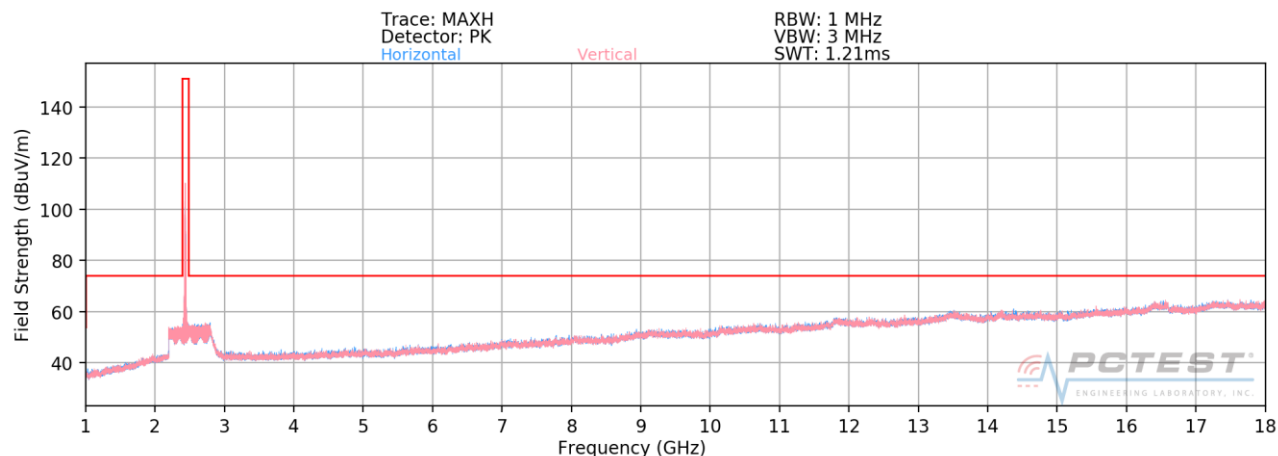
Plot 7-100. Radiated Spurious Plot above 1GHz SISO ANT2 (802.11b – Ch. 6)
