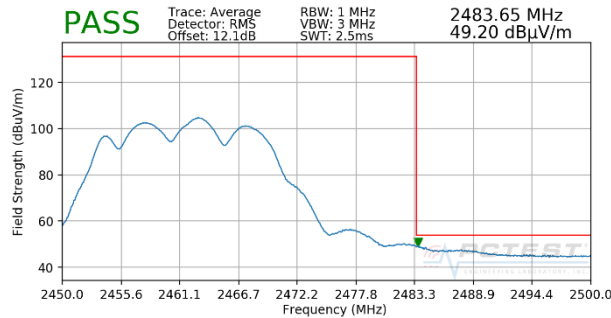
Plot 7-158. Radiated Restricted Band Edge Measurement CDD with WCP (Average)
