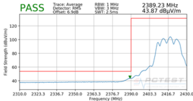
Plot 7-148. Radiated Restricted Lower Band Edge Measurement CDD (Average)
