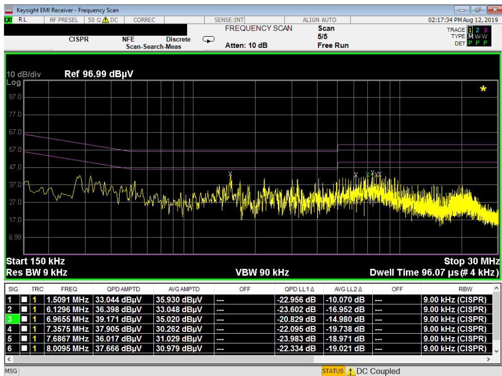
Plot 7-165. Line Conducted Plot with 802.11b (L1) with WCP
