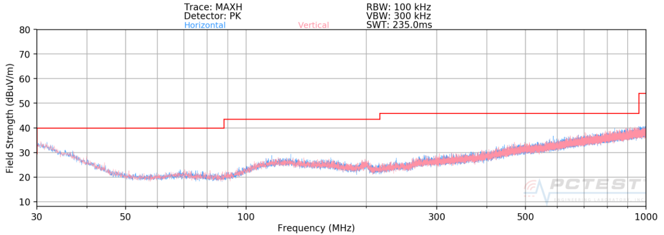
Plot 7-161. Radiated Spurious Plot below 1GHz SISO ANT2
