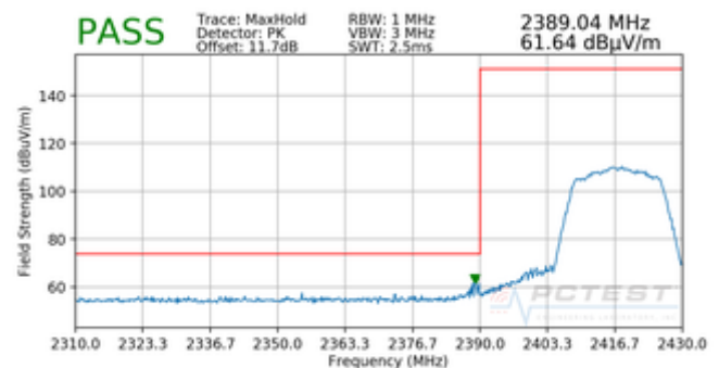
Plot 7-121. Radiated Restricted Lower Band Edge Measurement SISO ANT2 (Peak)
