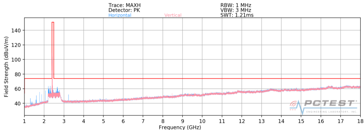
Plot 7-99. Radiated Spurious Plot above 1GHz SISO ANT2 (802.11b – Ch. 1)
