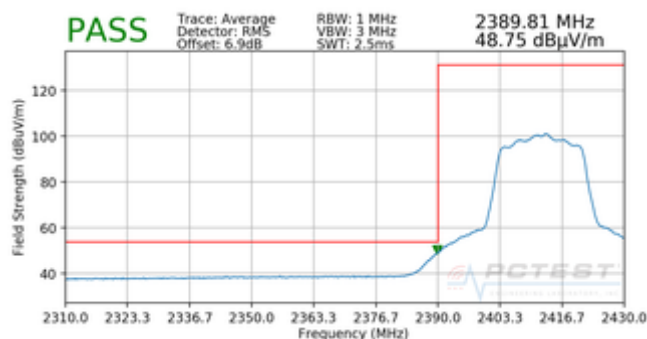
Plot 7-132. Radiated Restricted Lower Band Edge Measurement MIMO (Average)
