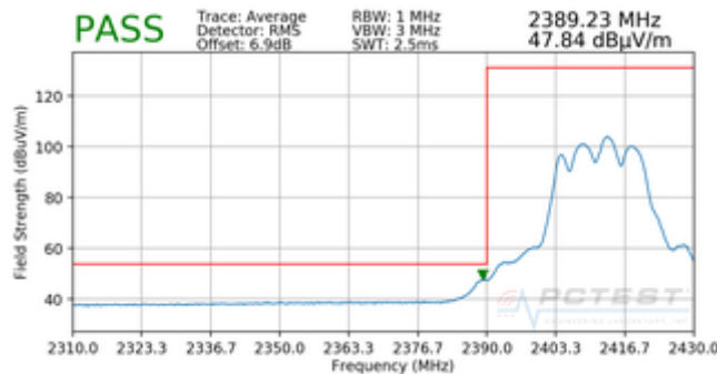
Plot 7-146. Radiated Restricted Lower Band Edge Measurement CDD (Average)
