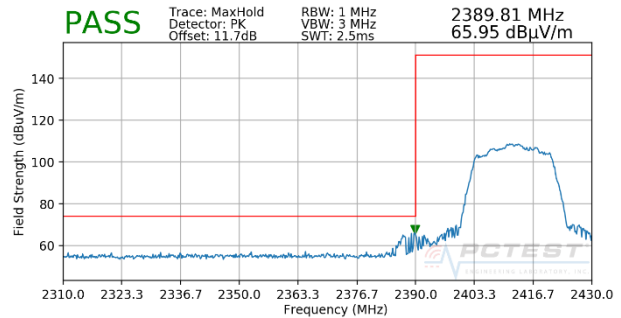
Plot 7-145. Radiated Restricted Band Edge Measurement MIMO with WCP (Peak)
