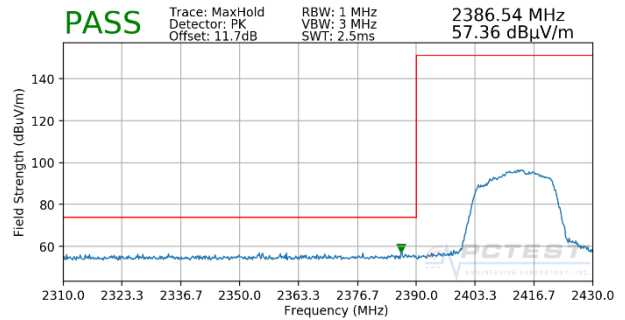
Plot 7-117. Radiated Restricted Band Edge Measurement SISO ANT1 with WCP (Peak)
