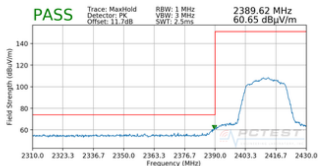
Plot 7-105. Radiated Restricted Lower Band Edge Measurement SISO ANT1 (Peak)
