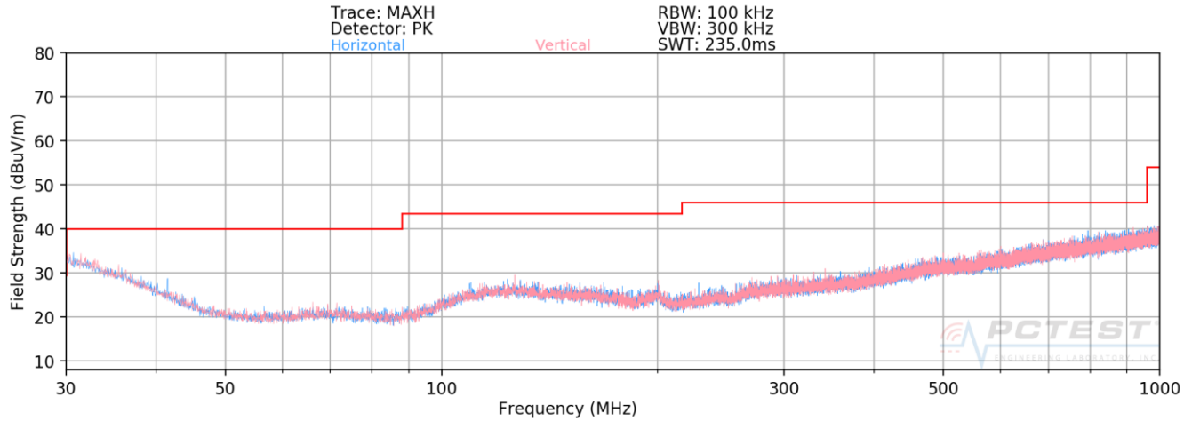
Plot 7-160. Radiated Spurious Plot below 1GHz SISO ANT1
