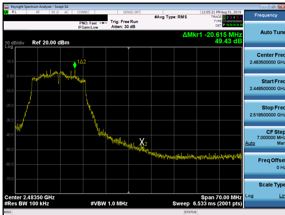
Plot 7-50. Band Edge Plot SISO ANT1 (802.11g – Ch. 11)
