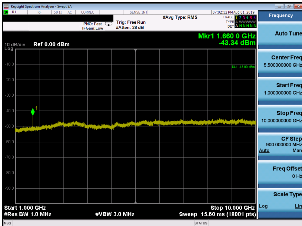
Plot 7-138. Conducted Spurious Plot (Band 26 - 15.0MHz QPSK - RB Size 1, RB Offset 0 - Mid Channel)
