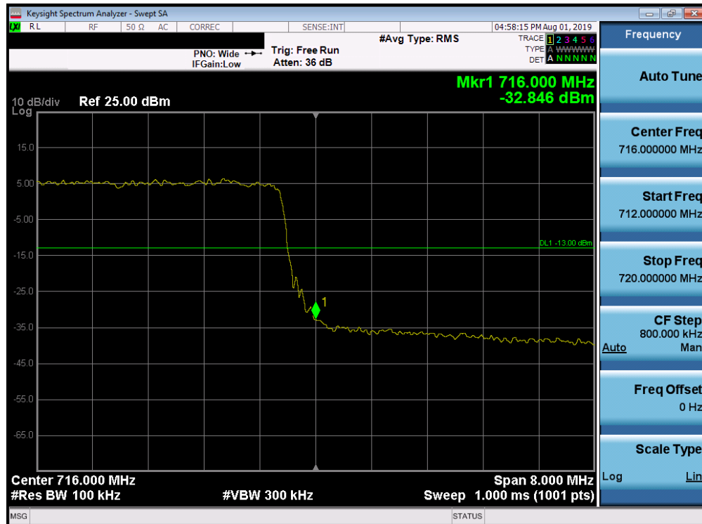
Plot 7-198. Upper Band Edge Plot (Band 12/17 - 10.0MHz QPSK - Full RB Configuration)
