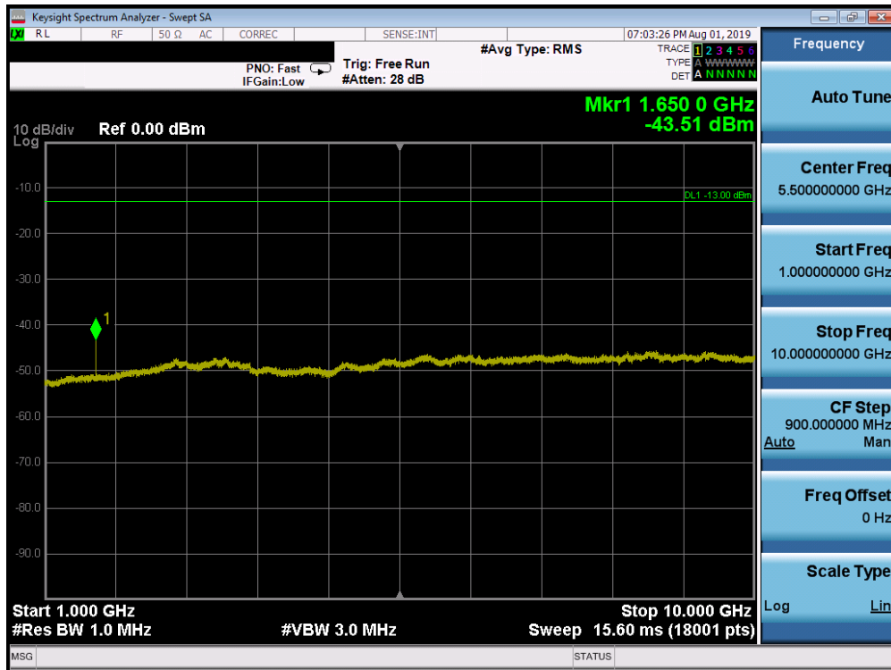
Plot 7-135. Conducted Spurious Plot (Band 26 - 15.0MHz QPSK - RB Size 1, RB Offset 0 - Low Channel)
