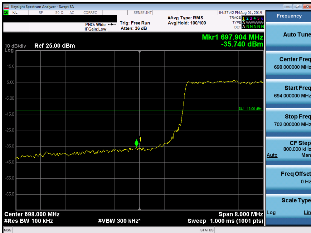
Plot 7-196. Lower Band Edge Plot (Band 12 - 10.0MHz QPSK - Full RB Configuration)
