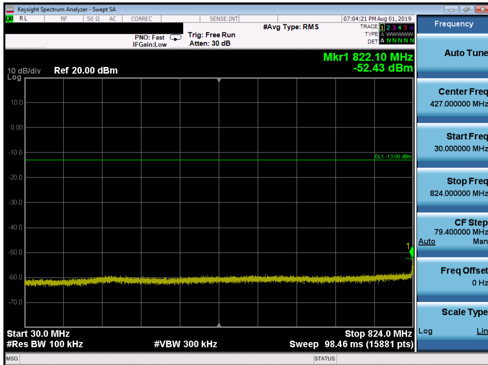
Plot 7-139. Conducted Spurious Plot (Band 26 - 15.0MHz QPSK - RB Size 1, RB Offset 0 - High Channel)
