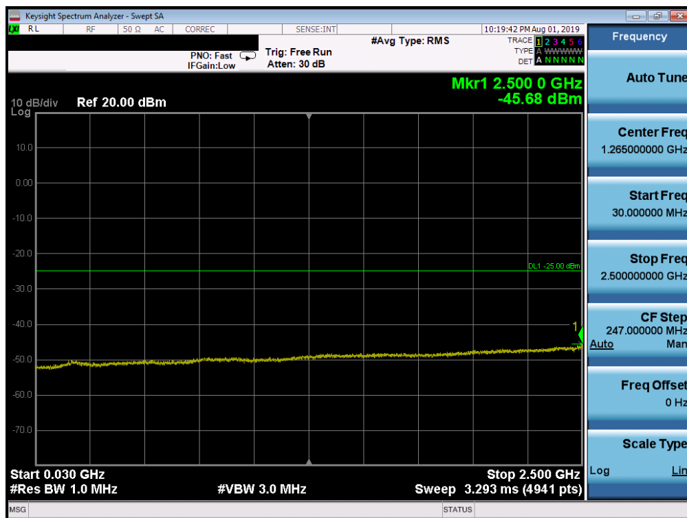
Plot 7-166. Conducted Spurious Plot (Band 7 - 20.0MHz QPSK - RB Size 1, RB Offset 0 - Mid Channel)
