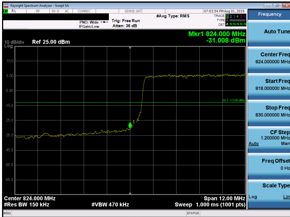
Plot 7-211. Lower Band Edge Plot (Band 26 - 15.0MHz QPSK - Full RB Configuration)
