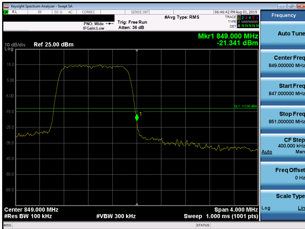
Plot 7-204. Upper Band Edge Plot (Band 26/5 - 1.4MHz QPSK - Full RB Configuration)
