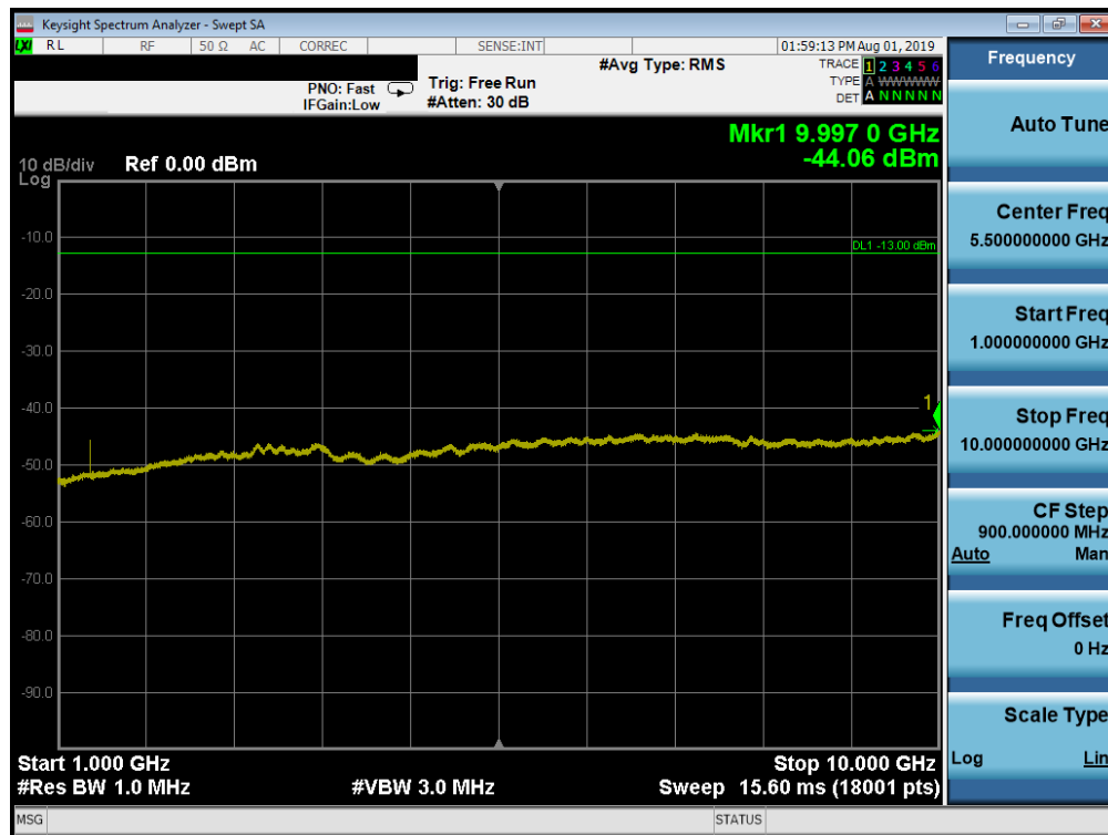
Plot 7-114. Conducted Spurious Plot (Band 71 - 10.0MHz QPSK - RB Size 1, RB Offset 0 - Low Channel)
