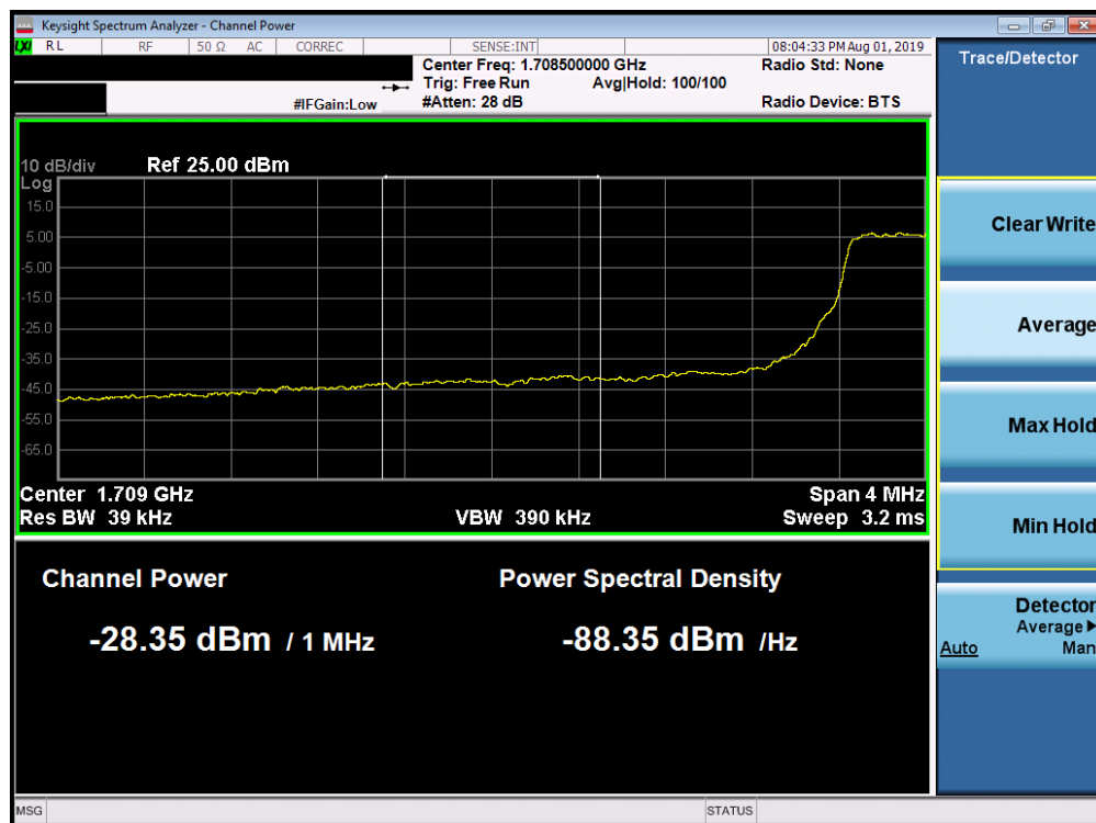
Plot 7-220. Lower Extended Band Edge Plot (Band 66/4 - 3.0MHz QPSK - Full RB Configuration)
