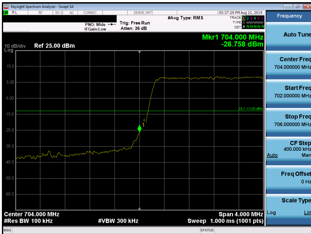
Plot 7-194. Lower Band Edge Plot (Band 17 - 5.0MHz QPSK - Full RB Configuration)
