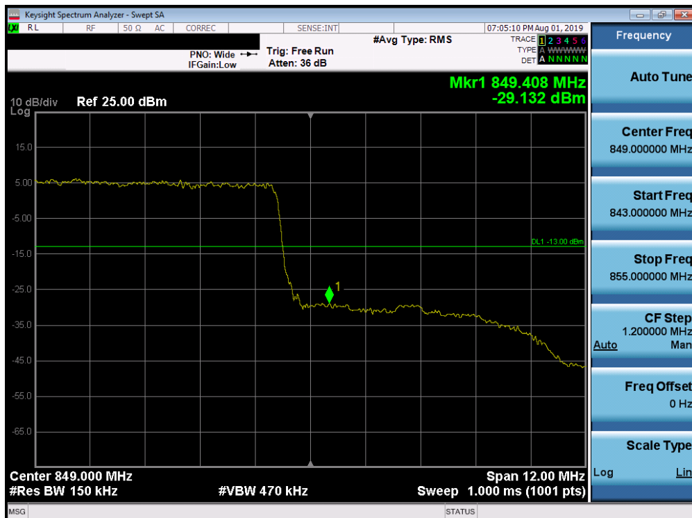
Plot 7-212. Upper Band Edge Plot (Band 26 - 15.0MHz QPSK - Full RB Configuration)
