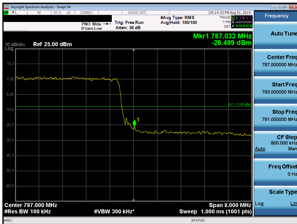
Plot 7-202. Upper Band Edge Plot (Band 13 - 10.0MHz QPSK - Full RB Configuration)
