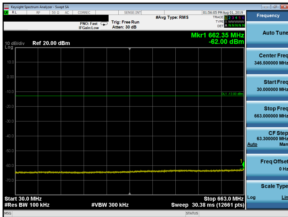
Plot 7-115. Conducted Spurious Plot (Band 71 - 10.0MHz QPSK - RB Size 1, RB Offset 0 - Mid Channel)
