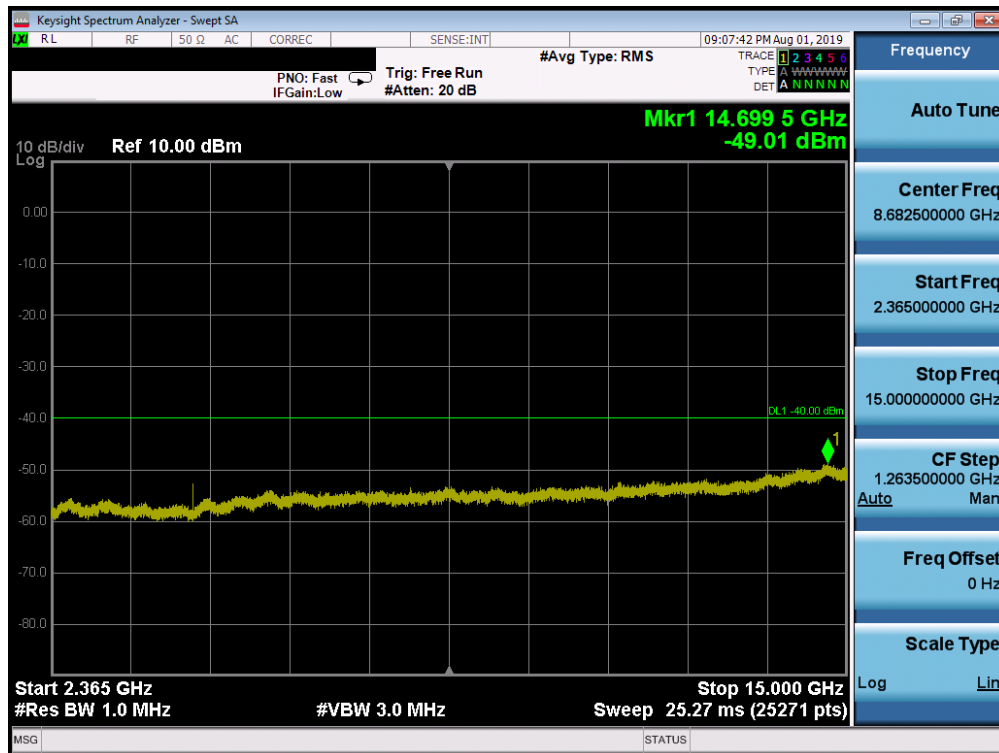
Plot 7-161. Conducted Spurious Plot (Band 30 - 10.0MHz QPSK - RB Size 1, RB Offset 0 – Mid Channel)
