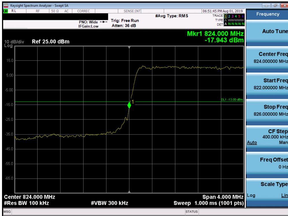
Plot 7-205. Lower Band Edge Plot (Band 26/5 - 3.0MHz QPSK - Full RB Configuration)
