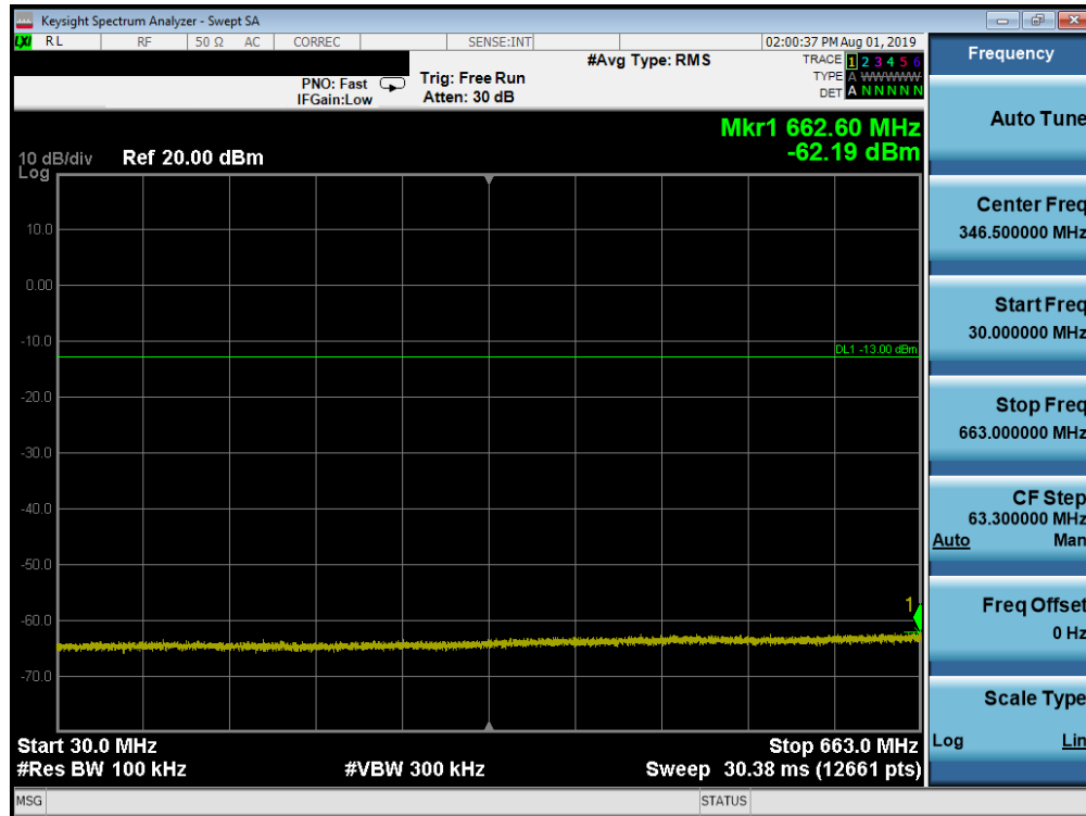
Plot 7-118. Conducted Spurious Plot (Band 71 - 10.0MHz QPSK - RB Size 1, RB Offset 0 - High Channel)
