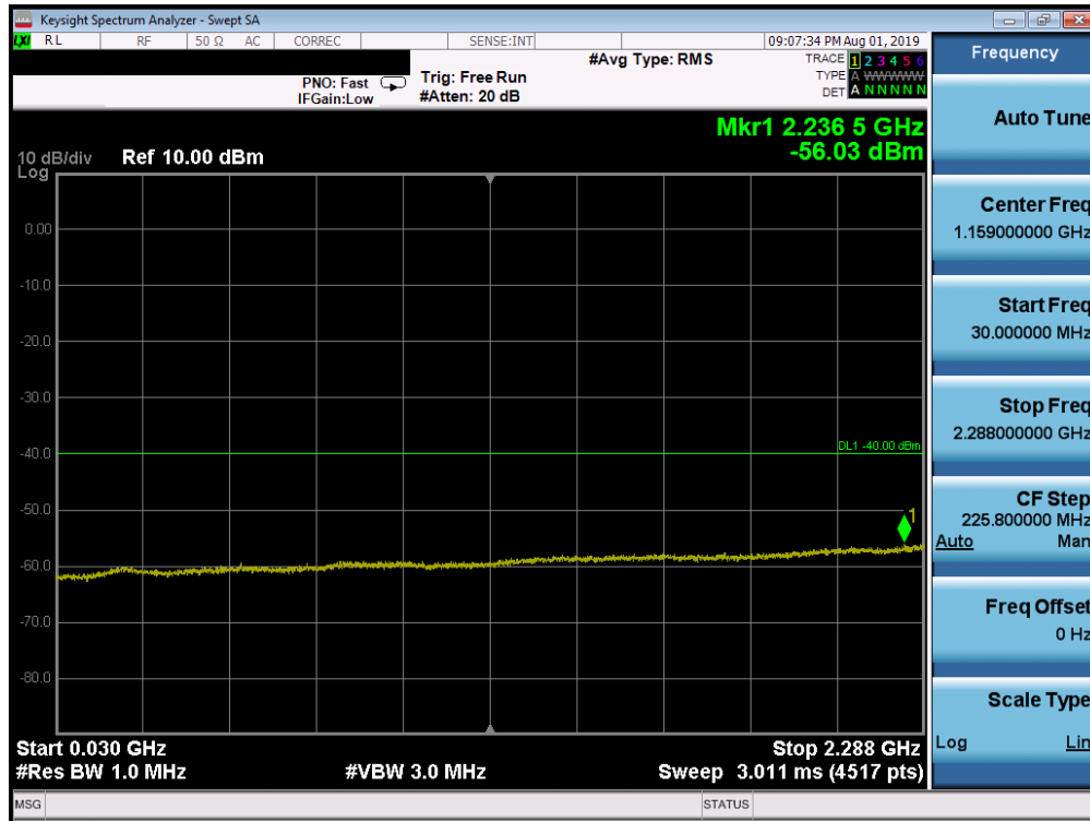
Plot 7-160. Conducted Spurious Plot (Band 30 - 10.0MHz QPSK - RB Size 1, RB Offset 0 – Mid Channel)
