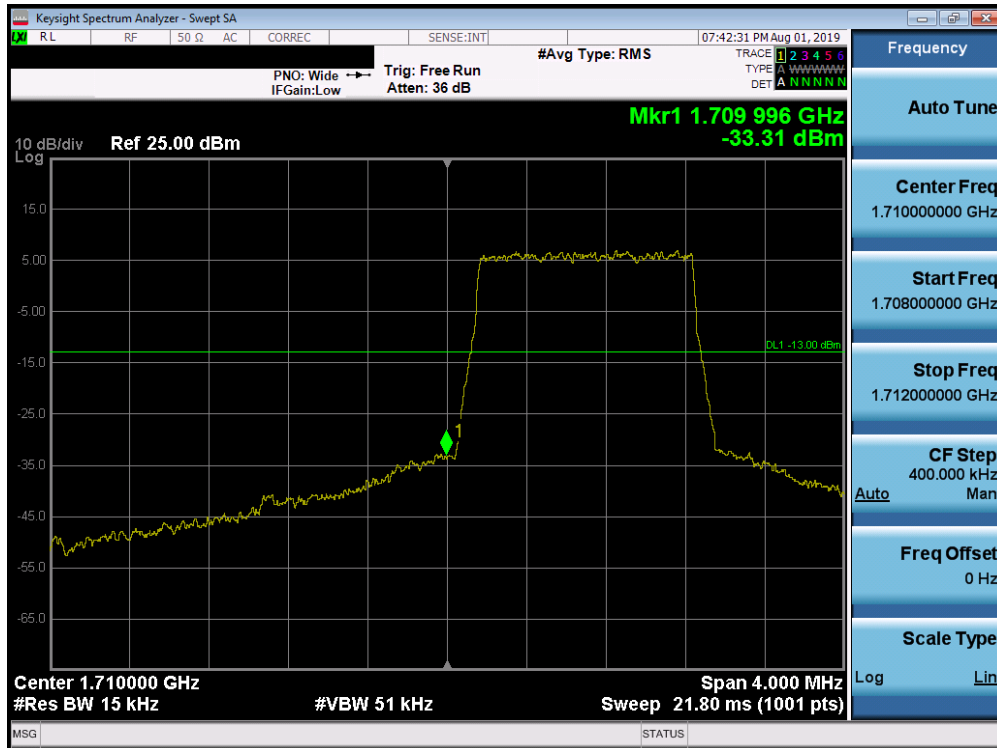
Plot 7-213. Lower Band Edge Plot (Band 66/4 - 1.4MHz QPSK - Full RB Configuration)
