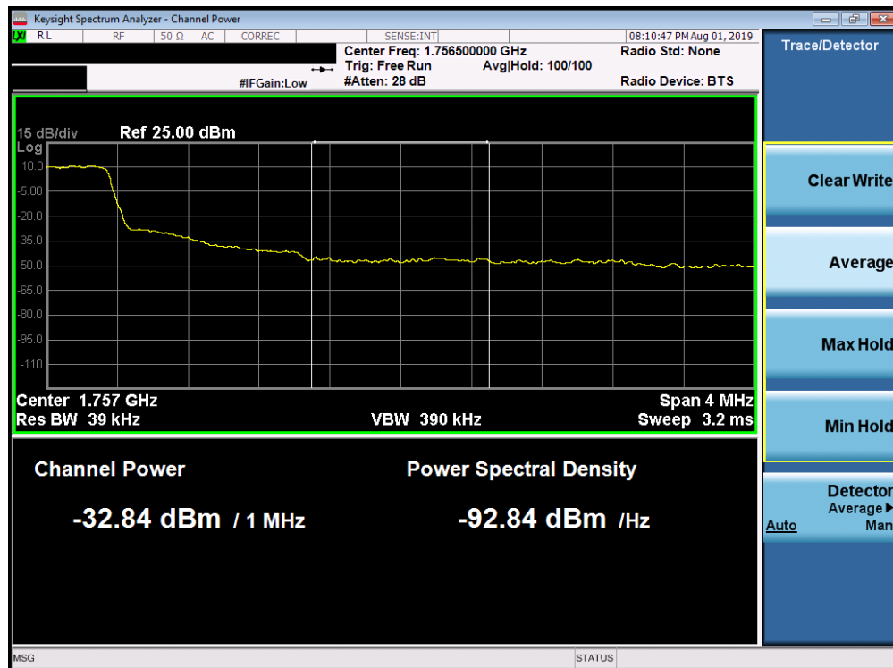
Plot 7-216. Upper Extended Band Edge Plot (Band 4 - 1.4MHz QPSK - Full RB Configuration)
