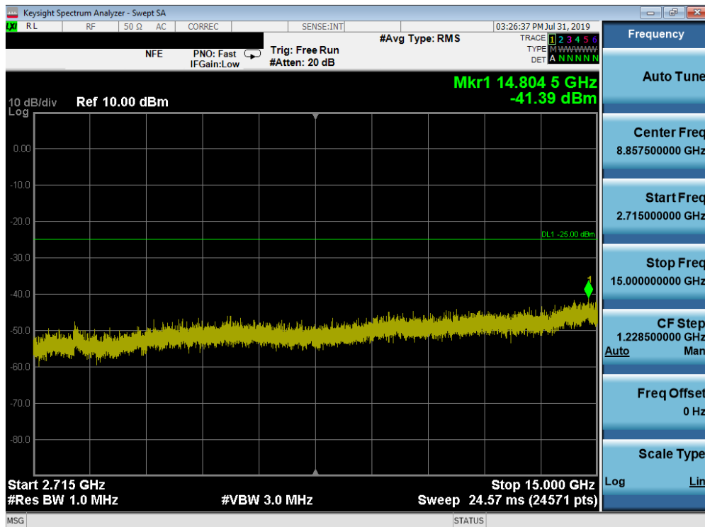
Plot 7-179. Conducted Spurious Plot (Band 41 (PC2) - 20.0MHz QPSK - RB Size 1, RB Offset 0 – High Channel)
