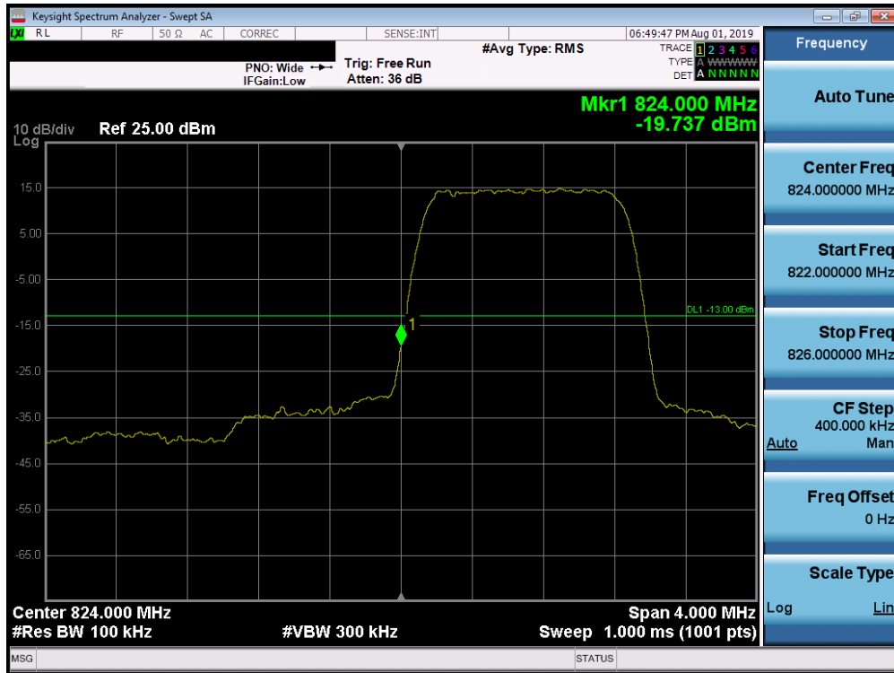
Plot 7-203. Lower Band Edge Plot (Band 26/5 - 1.4MHz QPSK - Full RB Configuration)
