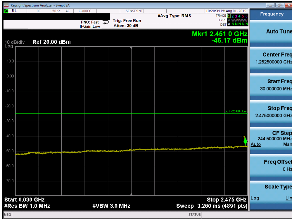
Plot 7-163. Conducted Spurious Plot (Band 7 - 20.0MHz QPSK - RB Size 1, RB Offset 0 - Low Channel)
