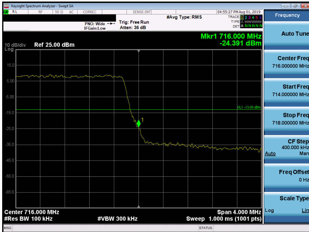
Plot 7-195. Upper Band Edge Plot (Band 12/17 - 5.0MHz QPSK - Full RB Configuration)
