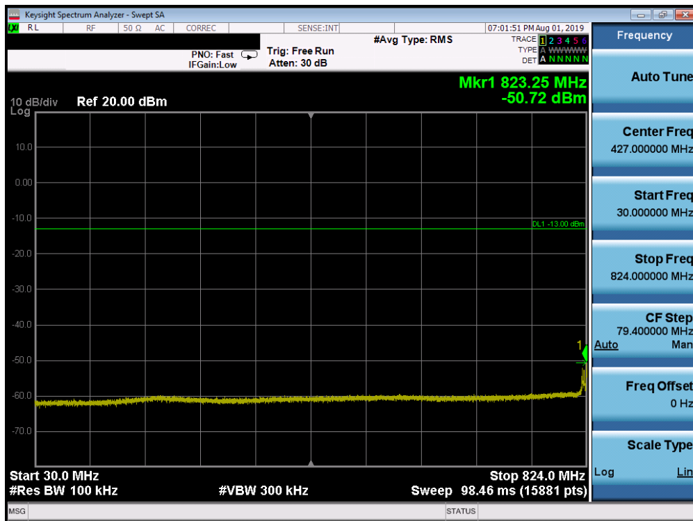
Plot 7-136. Conducted Spurious Plot (Band 26 - 15.0MHz QPSK - RB Size 1, RB Offset 0 - Mid Channel)
