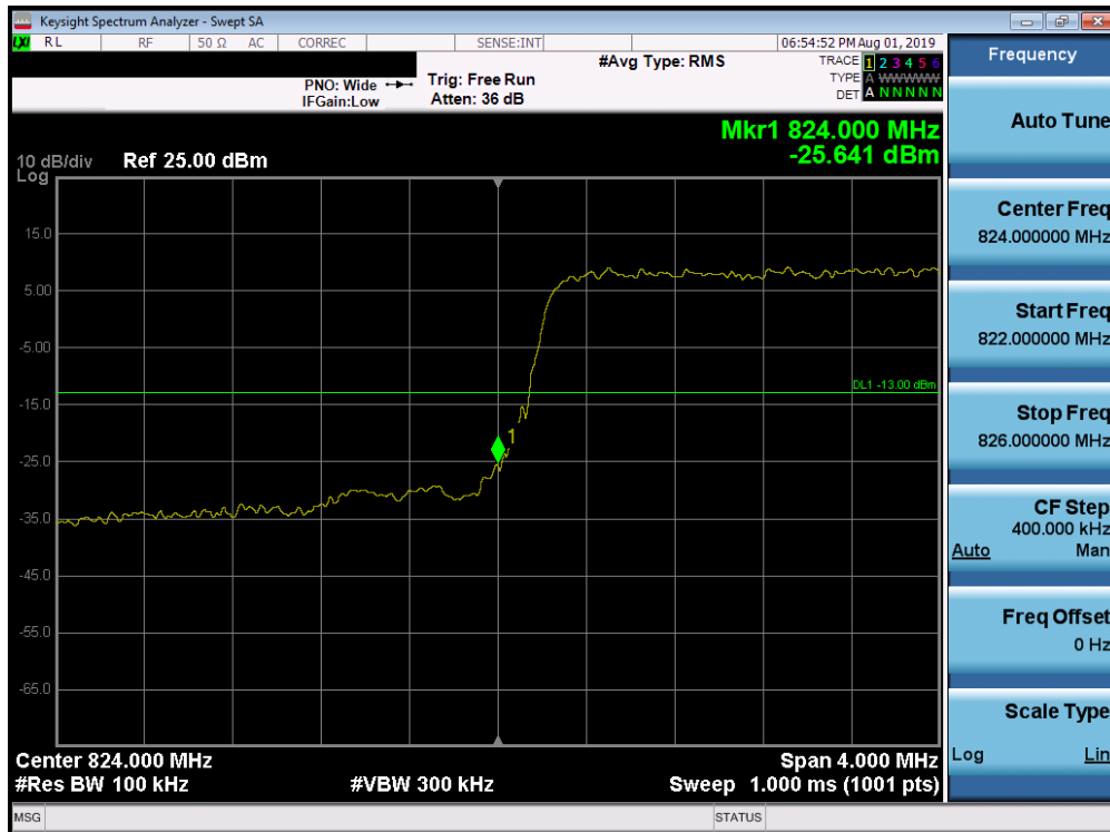
Plot 7-207. Lower Band Edge Plot (Band 26/5 - 5.0MHz QPSK - Full RB Configuration)
