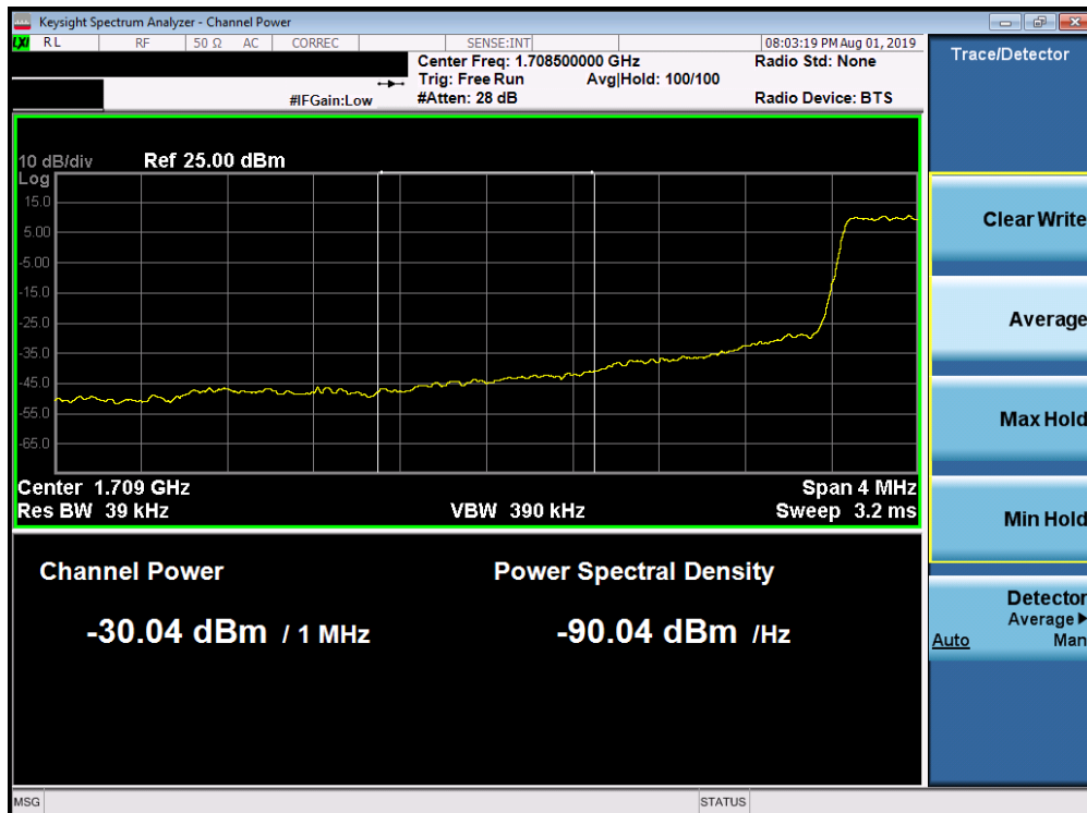
Plot 7-214. Lower Extended Band Edge Plot (Band 66/4 - 1.4MHz QPSK - Full RB Configuration)
