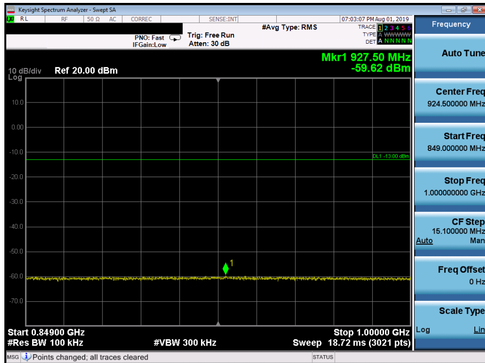
Plot 7-134. Conducted Spurious Plot (Band 26 - 15.0MHz QPSK - RB Size 1, RB Offset 0 - Low Channel)
