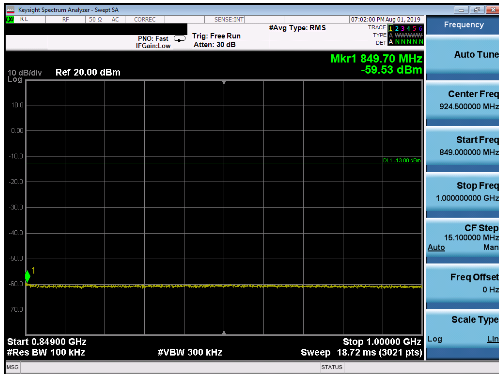
Plot 7-137. Conducted Spurious Plot (Band 26 - 15.0MHz QPSK - RB Size 1, RB Offset 0 - Mid Channel)
