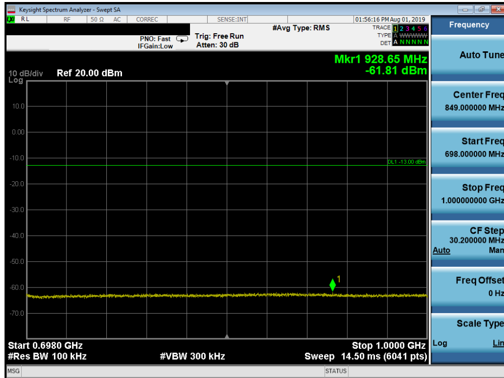
Plot 7-116. Conducted Spurious Plot (Band 71 - 10.0MHz QPSK - RB Size 1, RB Offset 0 - Mid Channel)
