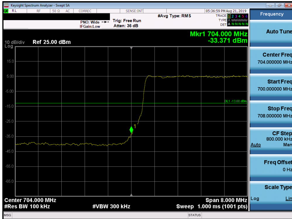
Plot 7-197. Lower Band Edge Plot (Band 17 - 10.0MHz QPSK - Full RB Configuration)
