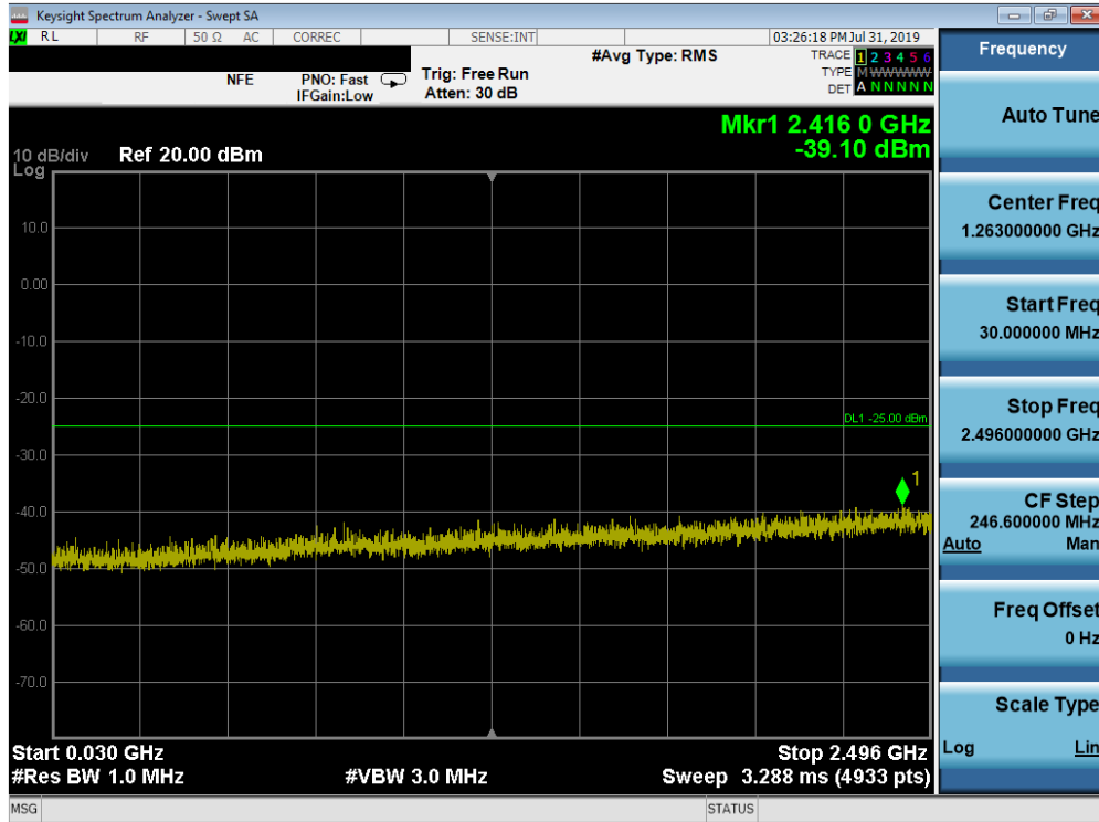
Plot 7-178. Conducted Spurious Plot (Band 41 (PC2) - 20.0MHz QPSK - RB Size 1, RB Offset 0 – High Channel)
