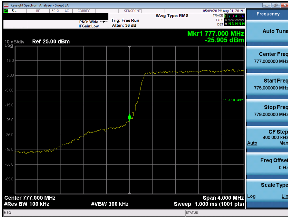
Plot 7-199. Lower Band Edge Plot (Band 13 - 5.0MHz QPSK - Full RB Configuration)
