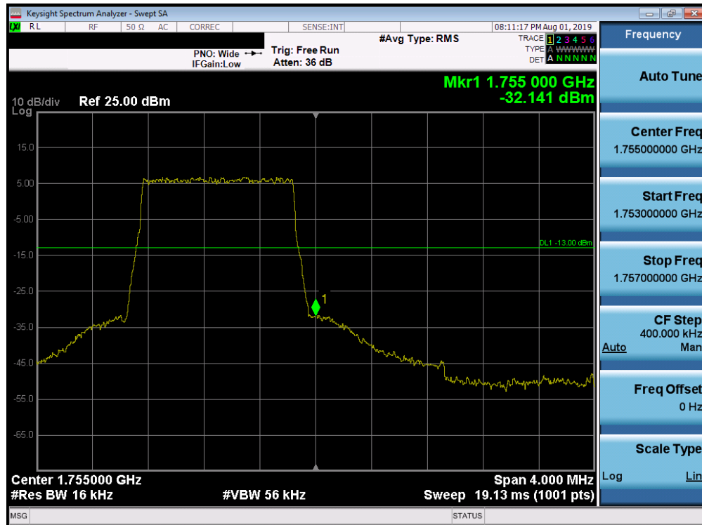
Plot 7-215. Upper Band Edge Plot (Band 4 - 1.4MHz QPSK - Full RB Configuration)
