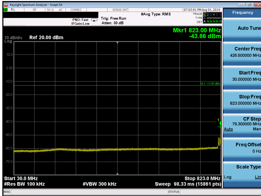
Plot 7-133. Conducted Spurious Plot (Band 26 - 15.0MHz QPSK - RB Size 1, RB Offset 0 - Low Channel)
