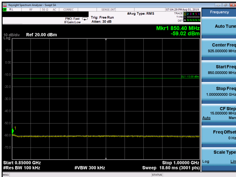
Plot 7-140. Conducted Spurious Plot (Band 26 - 15.0MHz QPSK - RB Size 1, RB Offset 0 - High Channel)
