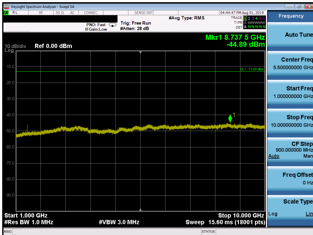
Plot 7-126. Conducted Spurious Plot (Band 12 /17 – 10.0MHz QPSK - RB Size 1, RB Offset 0 - Mid Channel)
