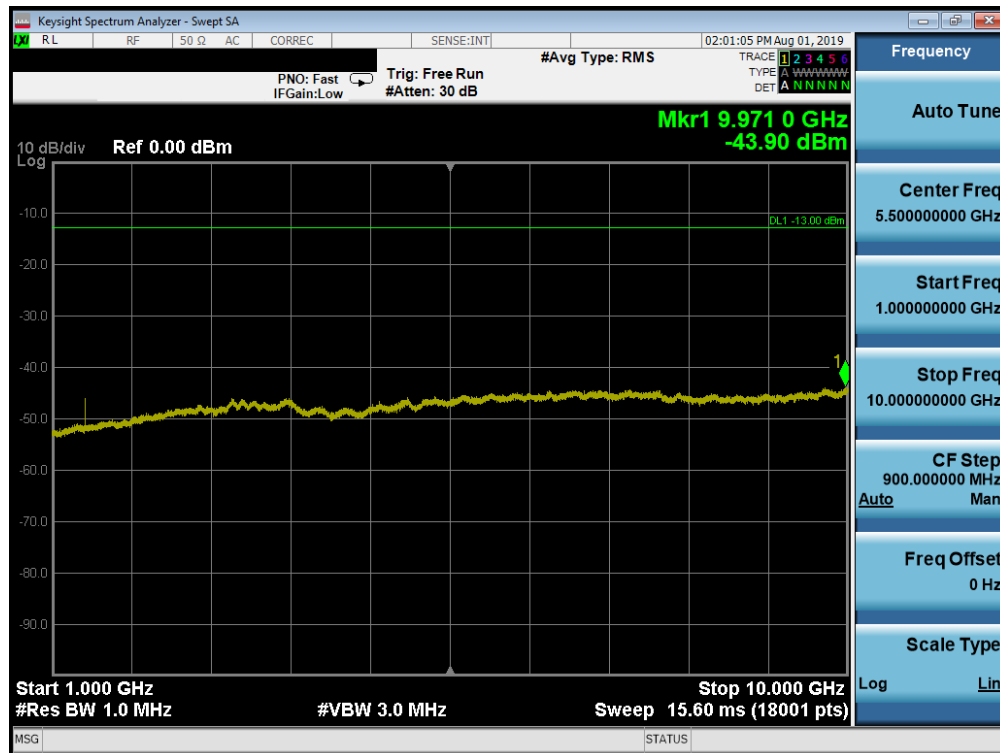
Plot 7-120. Conducted Spurious Plot (Band 71 - 10.0MHz QPSK - RB Size 1, RB Offset 0 - High Channel)
