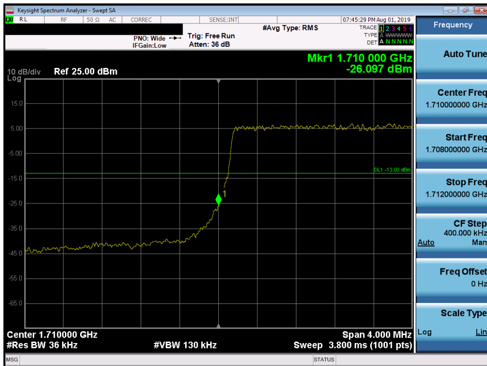
Plot 7-219. Lower Band Edge Plot (Band 66/4 - 3.0MHz QPSK - Full RB Configuration)
