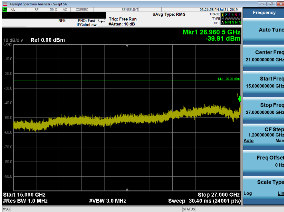
Plot 7-180. Conducted Spurious Plot (Band 41 (PC2) - 20.0MHz QPSK - RB Size 1, RB Offset 0 – High Channel)
