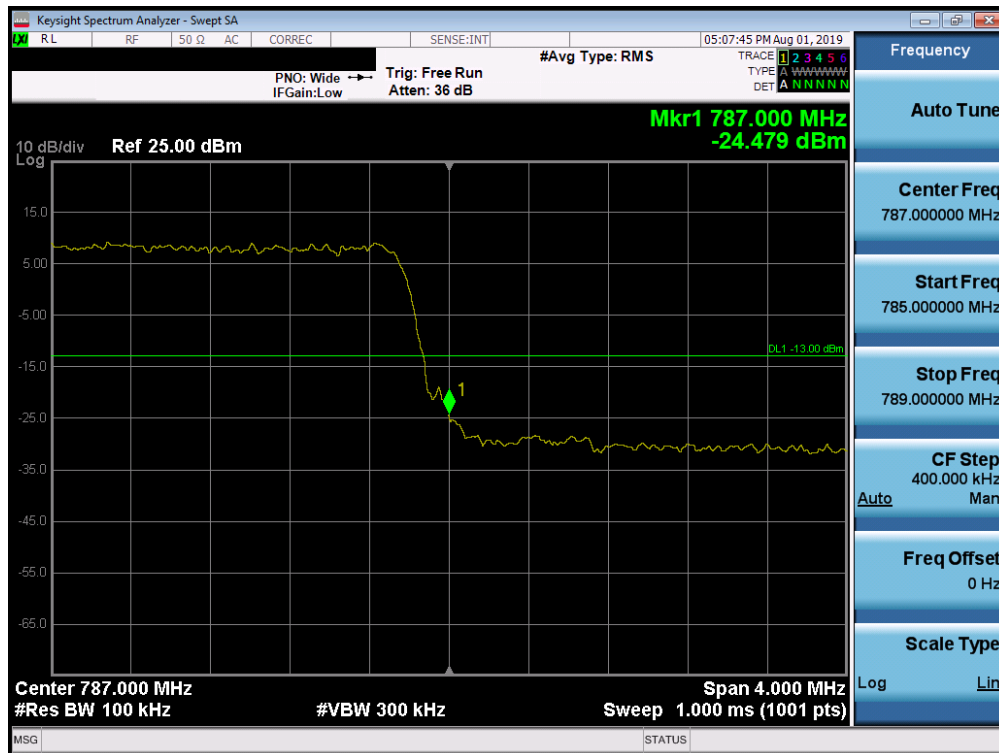
Plot 7-200. Upper Band Edge Plot (Band 13 - 5.0MHz QPSK - Full RB Configuration)
