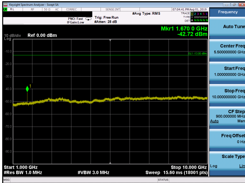
Plot 7-141. Conducted Spurious Plot (Band 26 - 15.0MHz QPSK - RB Size 1, RB Offset 0 - High Channel)
