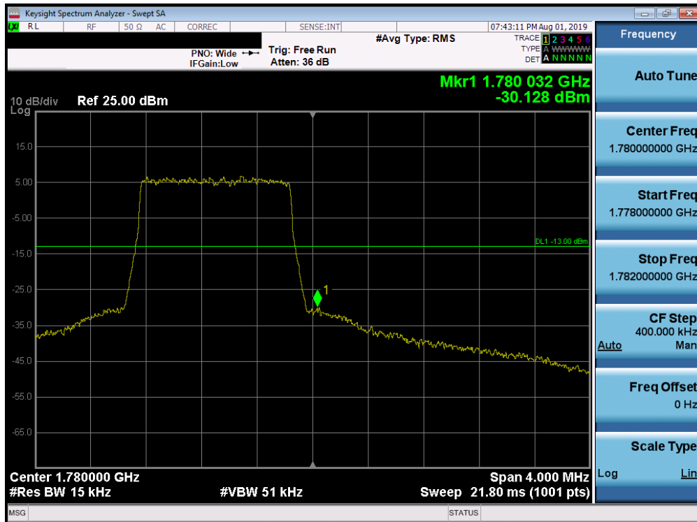
Plot 7-217. Upper Band Edge Plot (Band 66 - 1.4MHz QPSK - Full RB Configuration)
