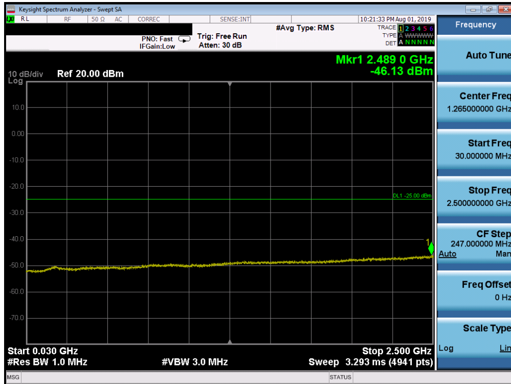
Plot 7-169. Conducted Spurious Plot (Band 7 - 20.0MHz QPSK - RB Size 1, RB Offset 0 – High Channel)
