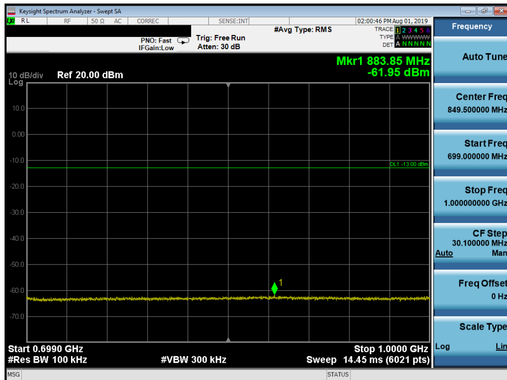
Plot 7-119. Conducted Spurious Plot (Band 71 - 10.0MHz QPSK - RB Size 1, RB Offset 0 - High Channel)
