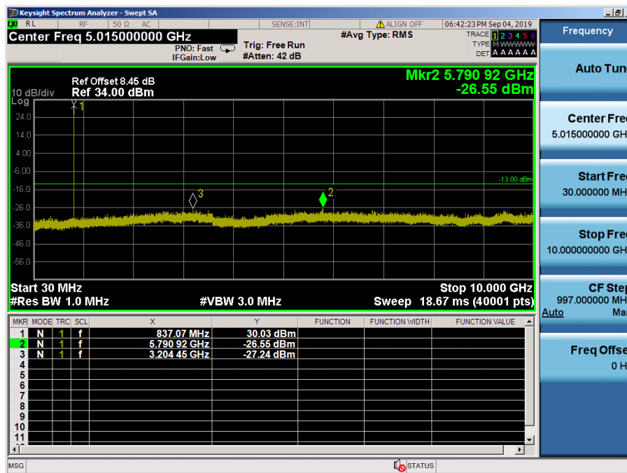
LTE Band 5 / 1.4MHz / 64QAM - RB Size/Offset (1/5) – Mid Channel
