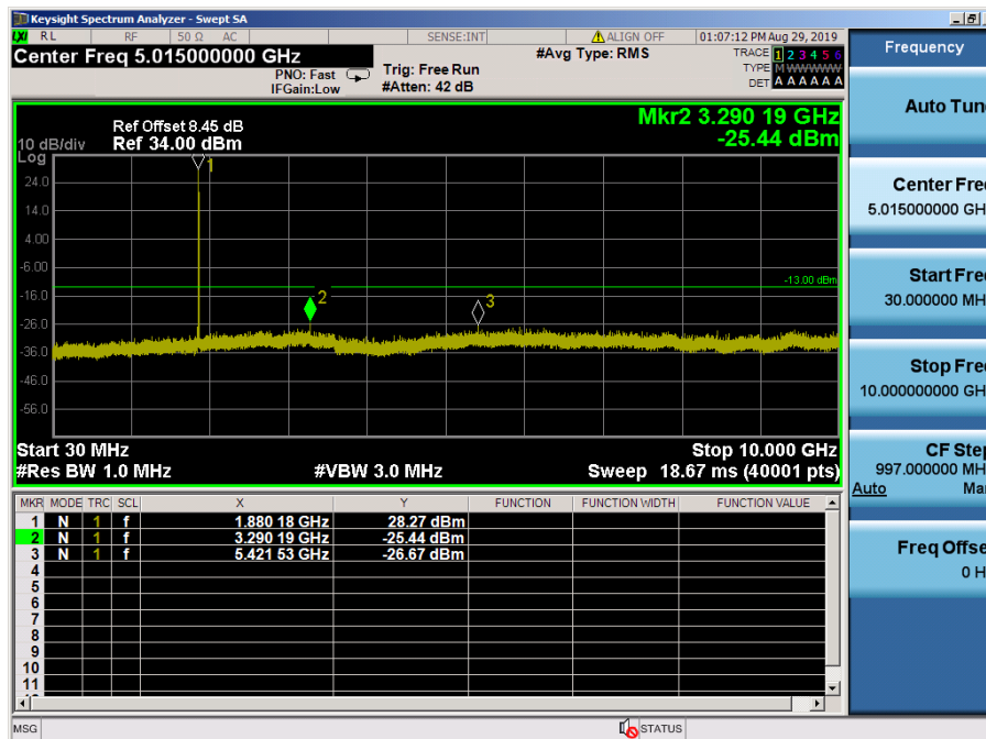
LTE Band 2 / 20MHz / 16QAM - RB Size/Offset (1/50)–Mid Channel
