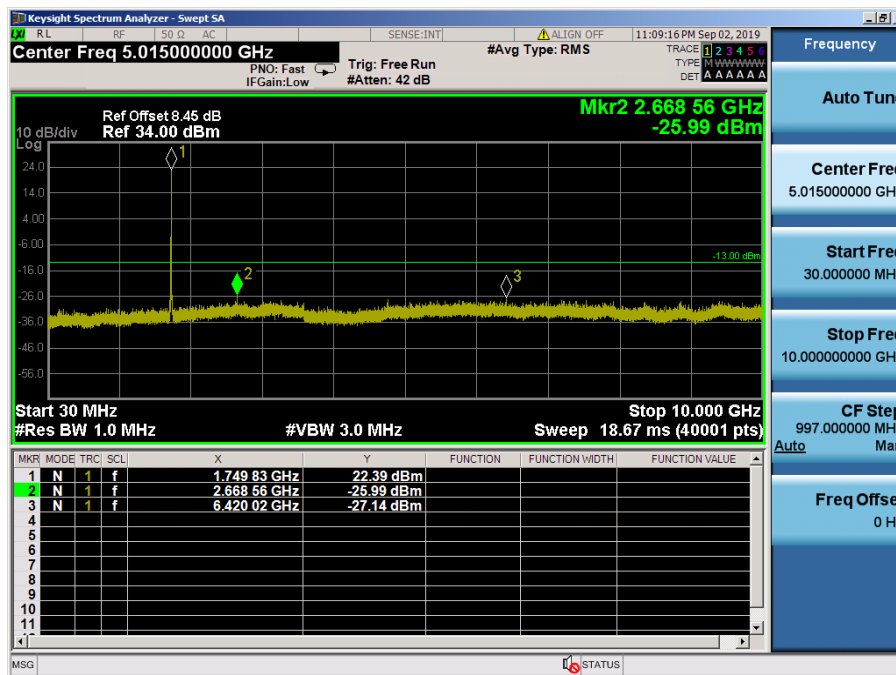
LTE Band 4 / 15MHz / 64QAM - RB Size/Offset (36/39) – High Channel
