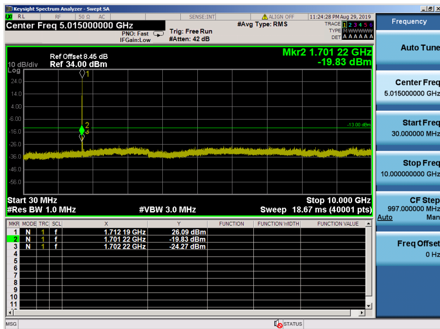
LTE Band 4 / 3MHz / QPSK - RB Size/Offset (8/4) – Low Channel
