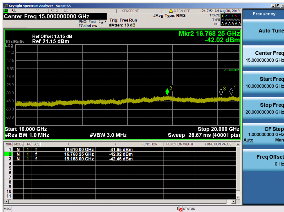
LTE Band 4 / 5MHz / QPSK - RB Size/Offset (1/0) – Low Channel
