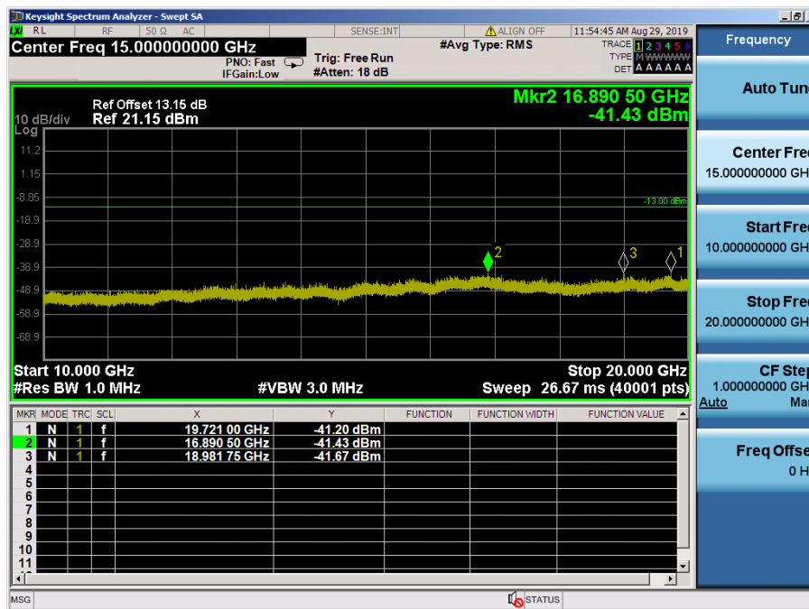
LTE Band 2 / 10MHz / 16QAM - RB Size/Offset (50/0) – High Channel
