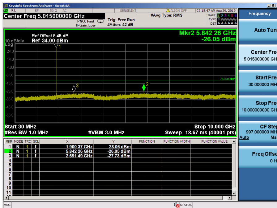
LTE Band 2 / 20MHz / QPSK - RB Size/Offset (1/50) – High Channel
