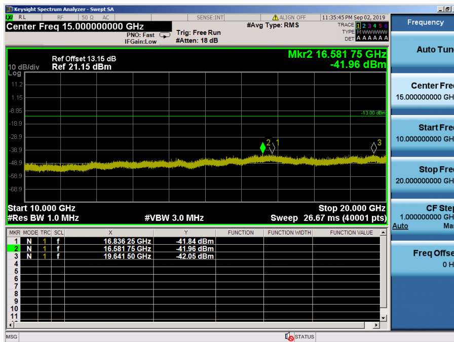
LTE Band 4 / 20MHz / 64QAM - RB Size/Offset (1/0)–Mid Channel
