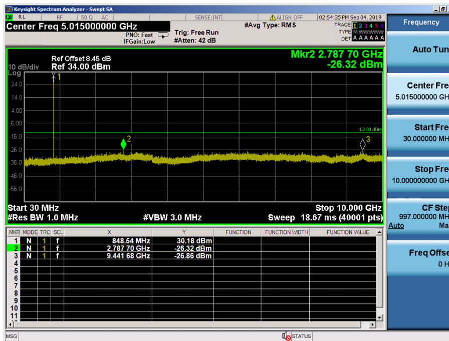
LTE Band 5 / 1.4MHz / 16QAM - RB Size/Offset (1/2) – High Channel
