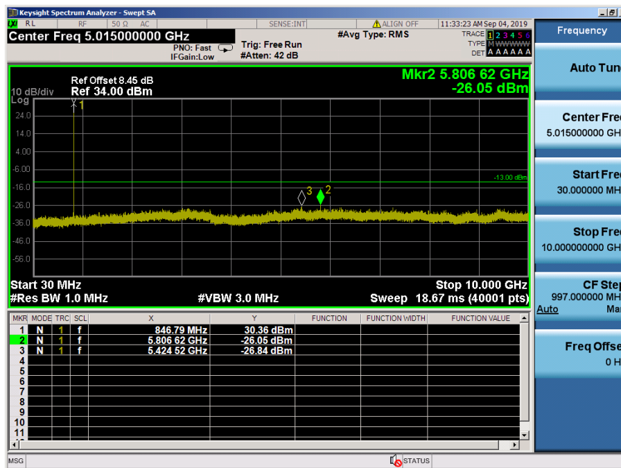
LTE Band 5 / 5MHz / QPSK - RB Size/Offset (1/12) – High Channel
