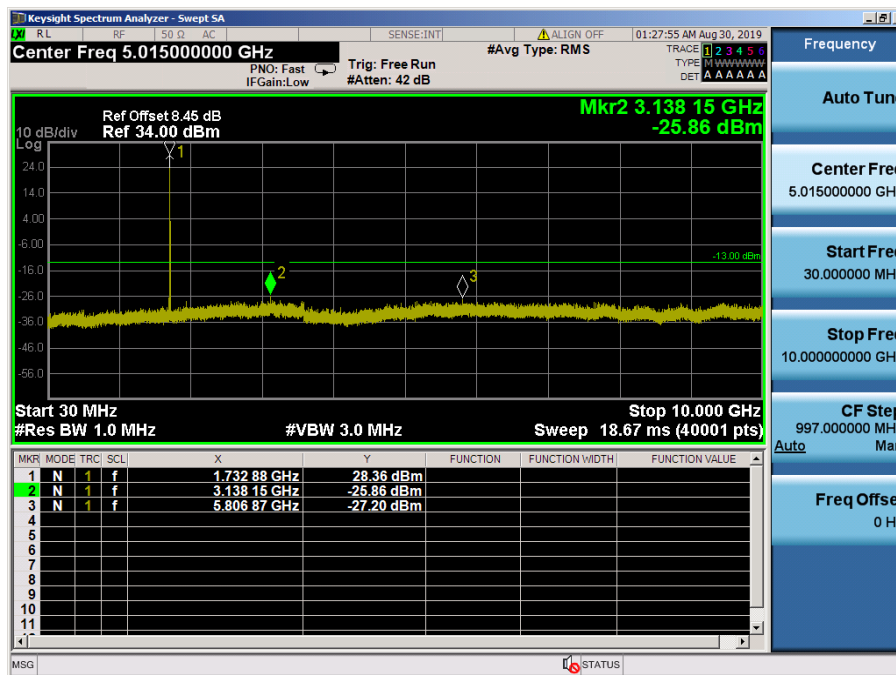
LTE Band 4 / 10MHz / QPSK - RB Size/Offset (1/25)– Mid Channel
