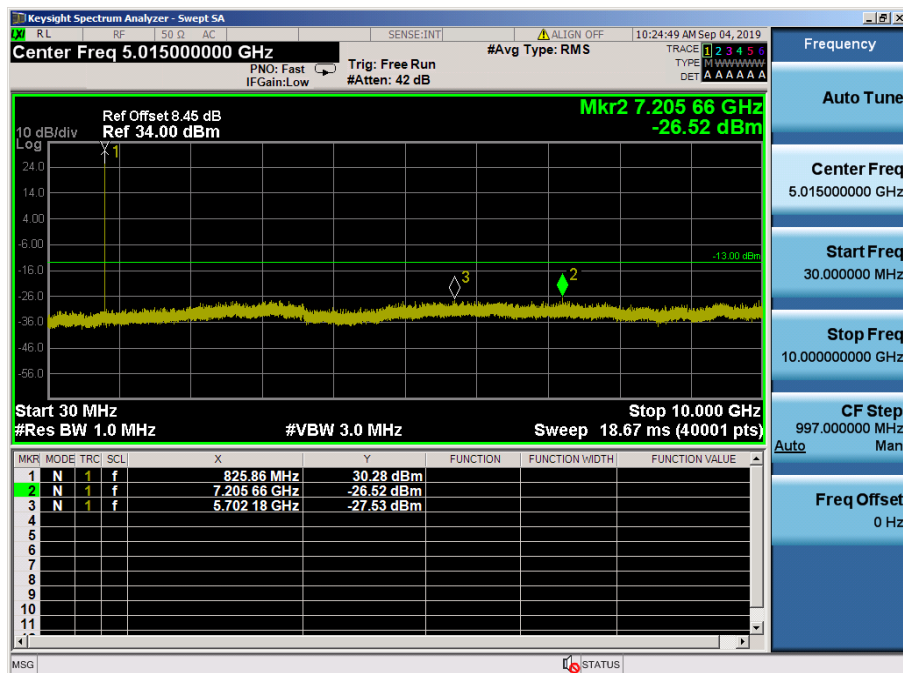
LTE Band 5 / 3MHz / QPSK - RB Size/Offset (1/7) – Low Channel
