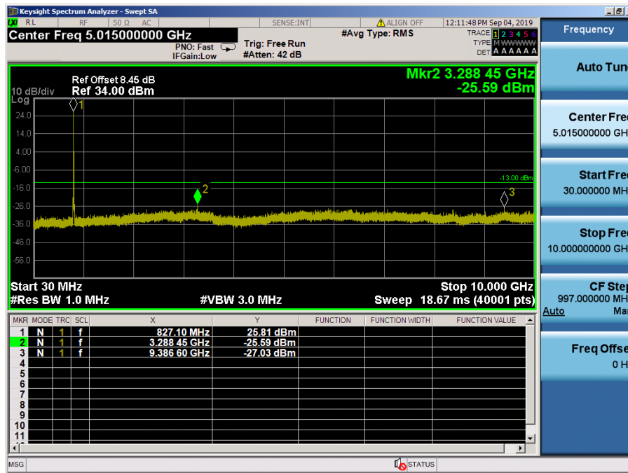
LTE Band 5 / 10MHz / QPSK - RB Size/Offset (25/0) – Low Channel
