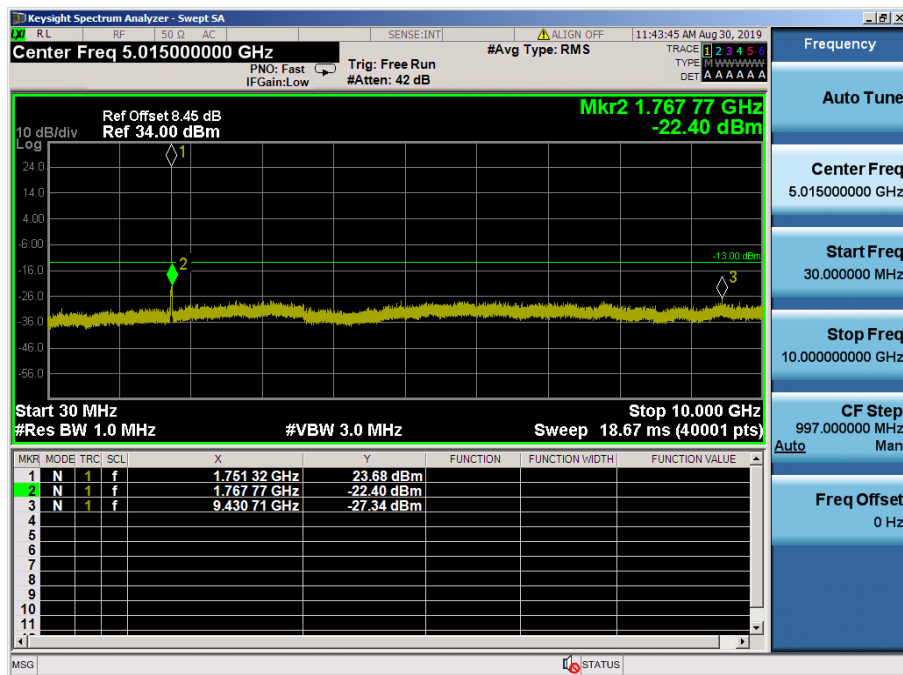
LTE Band 4 / 5MHz / 16QAM - RB Size/Offset (25/0) – High Channel
