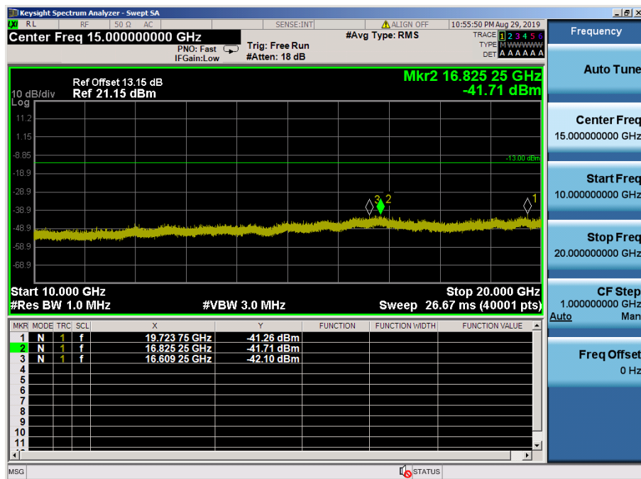
LTE Band 4 / 1.4MHz / QPSK - RB Size/Offset (6/0) – High Channel
