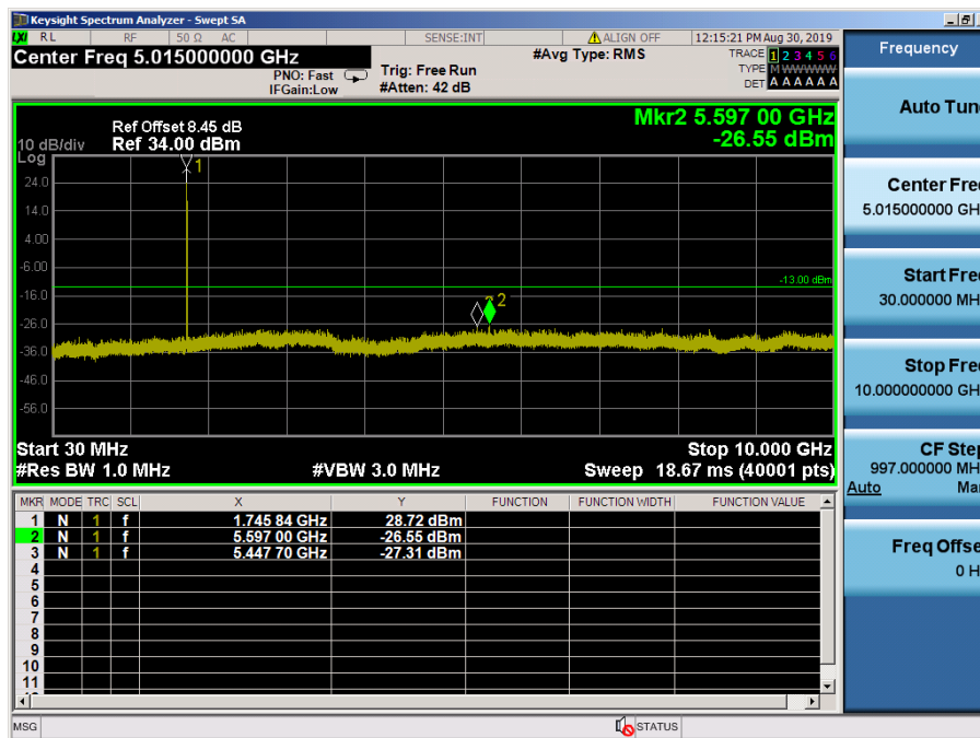
LTE Band 4 / 10MHz / 16QAM - RB Size/Offset (1/0) – High Channel
