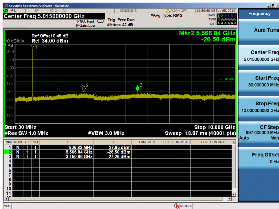
LTE Band 5 / 3MHz / 64QAM - RB Size/Offset (8/7) – Mid Channel
