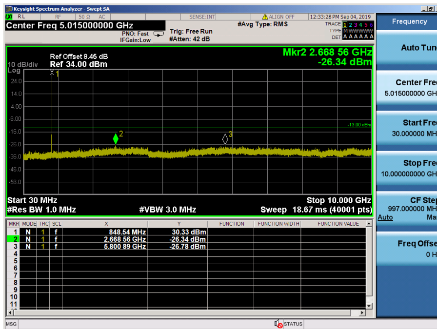
LTE Band 5 / 10MHz / QPSK - RB Size/Offset (1/49) – High Channel
