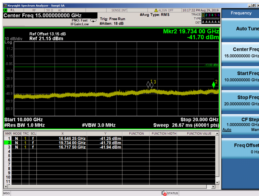
LTE Band 4 / 1.4MHz / QPSK - RB Size/Offset (8/0) – Low Channel
