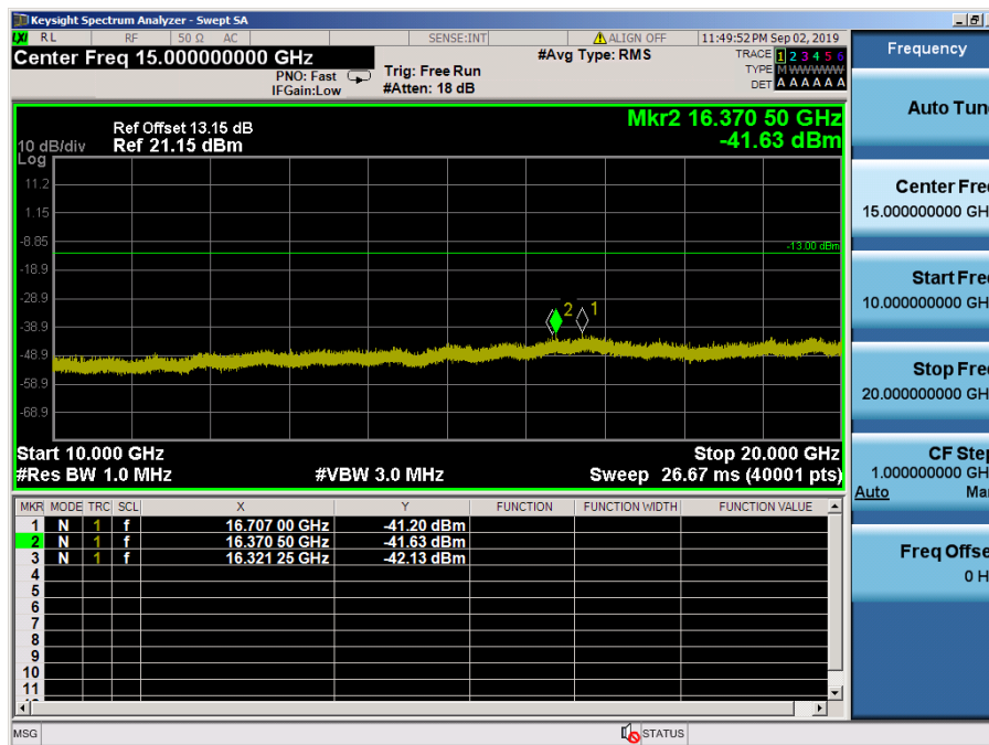
LTE Band 4 / 20MHz / 64QAM - RB Size/Offset (1/99) – High Channel
