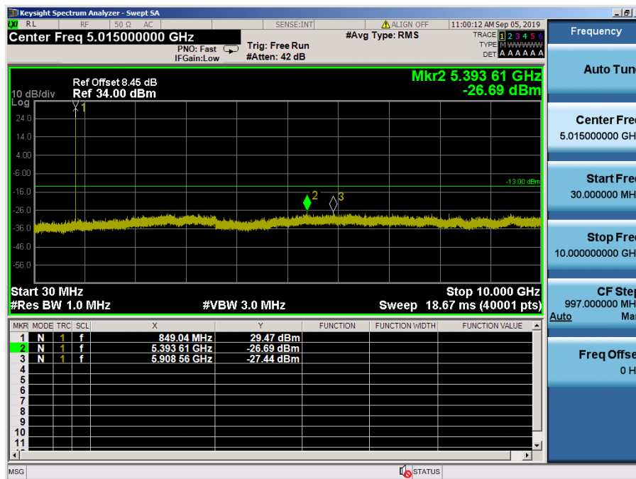
LTE Band 5 / 3MHz / 64QAM - RB Size/Offset (1/14) – High Channel
