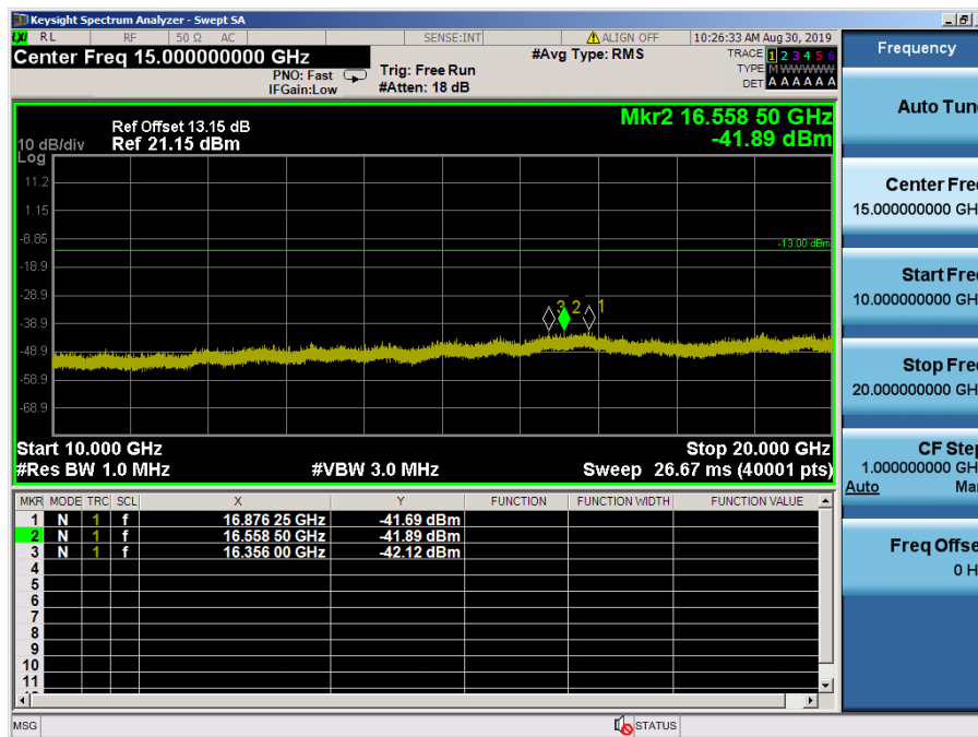
LTE Band 4 / 3MHz / 16QAM - RB Size/Offset (1/7) – High Channel
