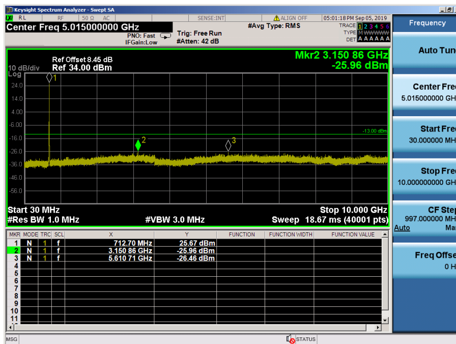
LTE Band 12, 17 / 10MHz / QPSK - RB Size/Offset (25/25) – High Channel
