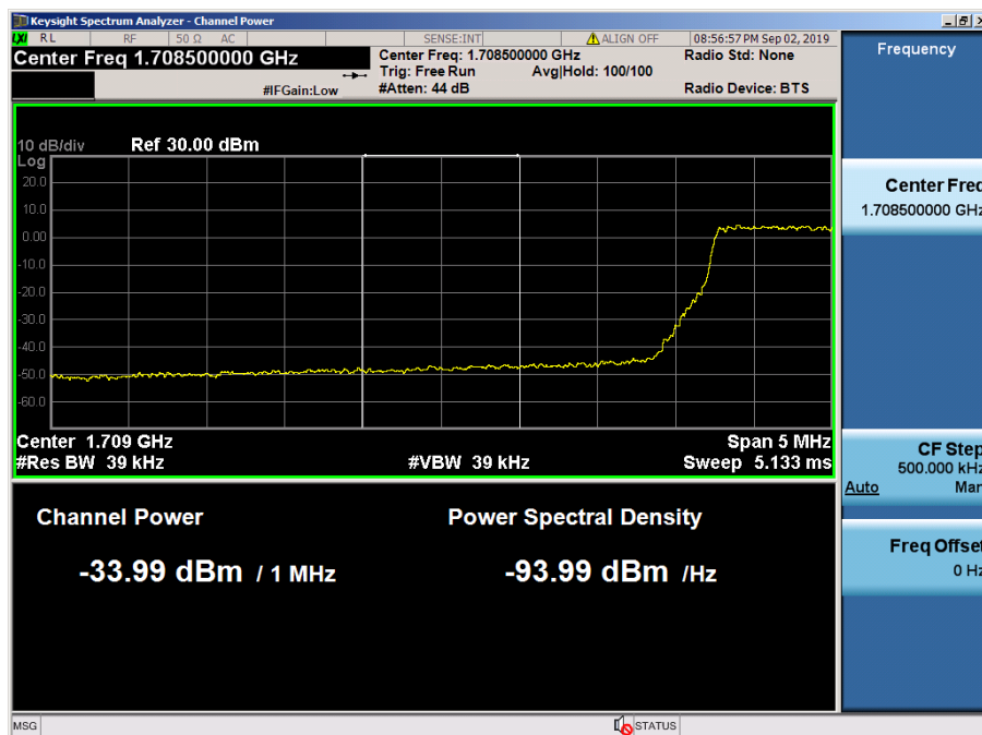
LTE Band 4 / 5MHz / 64QAM - RB Size/Offset (12/0)
