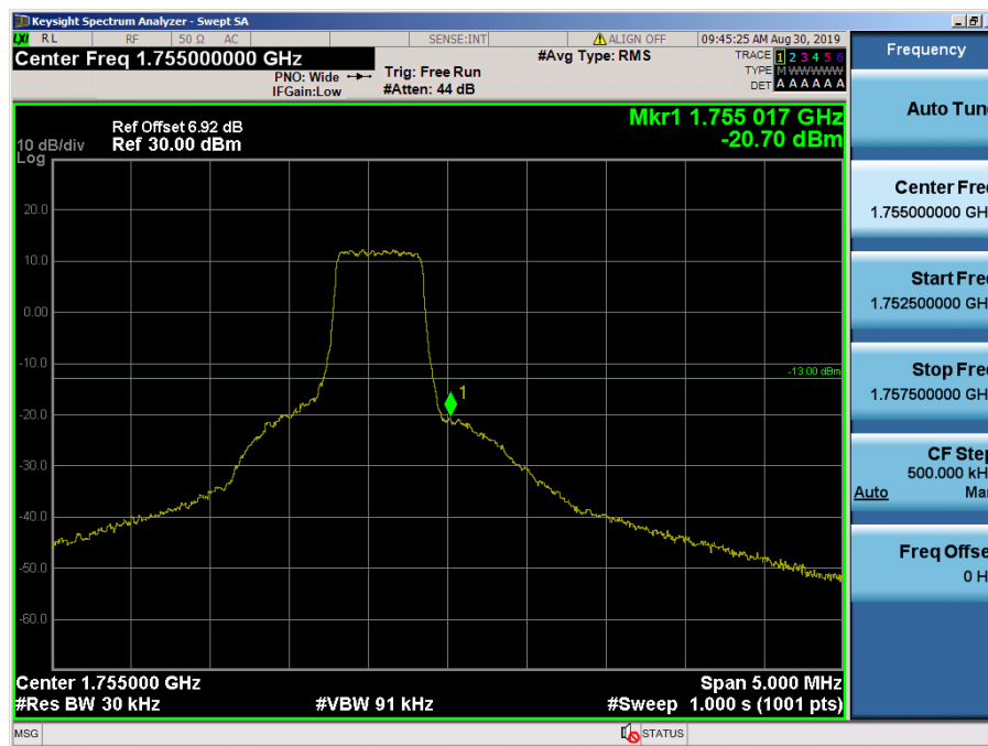
LTE Band 4 / 1.4MHz / 16QAM - RB Size/Offset (3/3)
