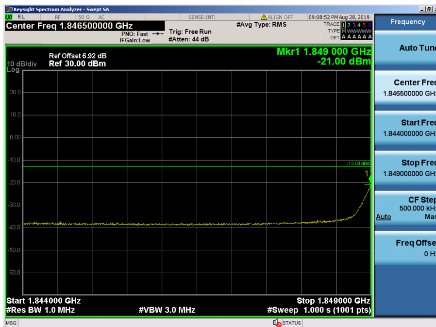
LTE Band 2 / 1.4MHz / QPSK - RB Size/Offset (1/2)
