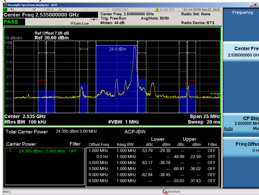
LTE Band 7 / 5MHz / QPSK - RB Size/Offset (1/14)
