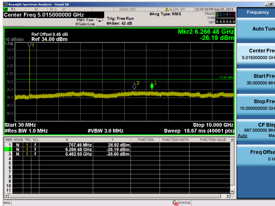
LTE Band 12 / 3MHz / 64QAM - RB Size/Offset (15/0) – Mid Channel
