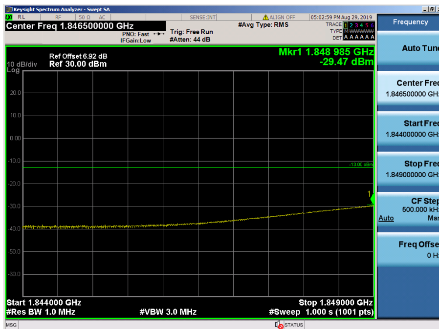
LTE Band 2 / 3MHz / 64QAM - RB Size/Offset (8/4)
