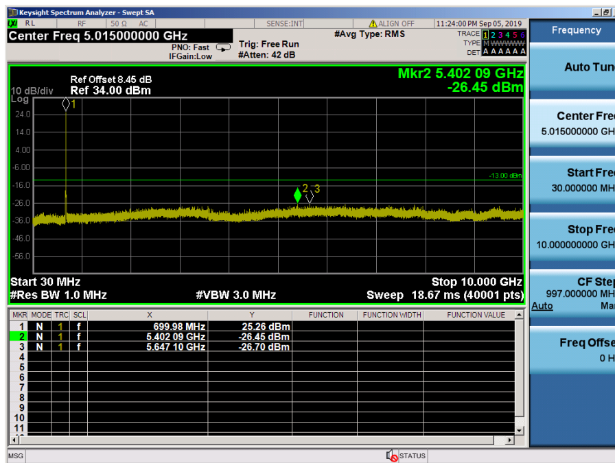
LTE Band 12, 17 / 5MHz / 64QAM - RB Size/Offset (25/0) – Low Channel
