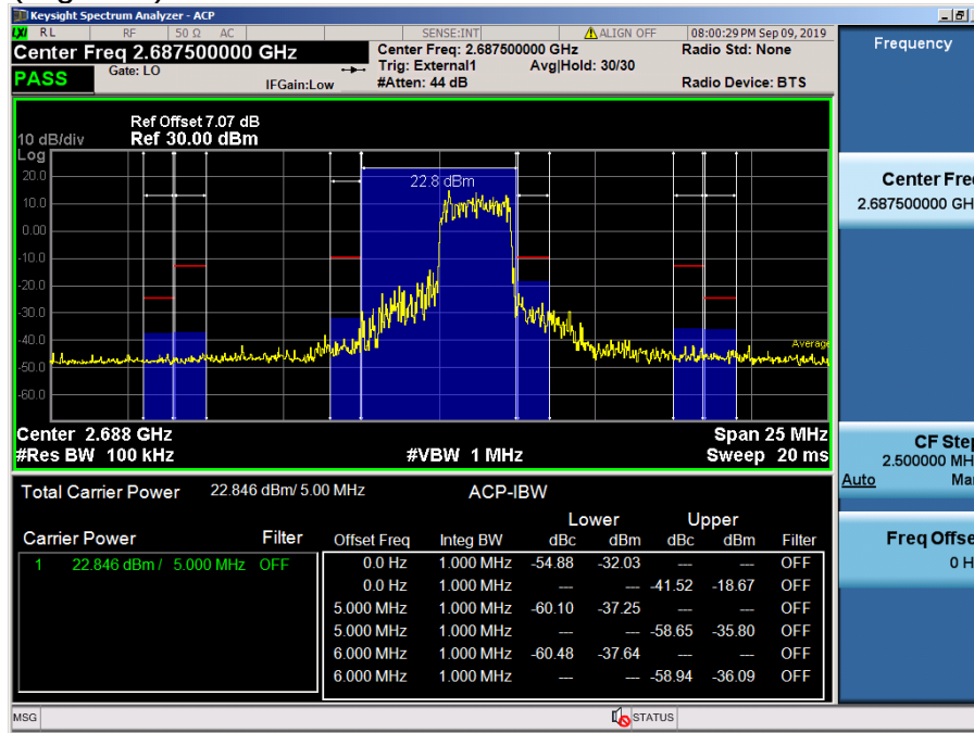
LTE Band 41 / 5MHz / QPSK - RB Size/Offset (12/13)
