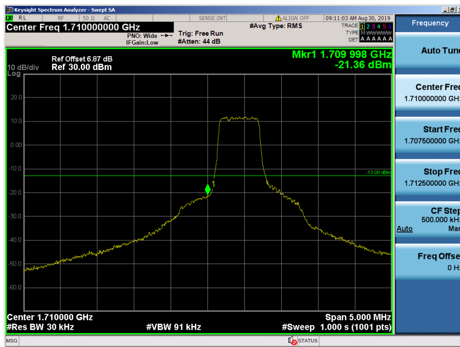
LTE Band 4 / 1.4MHz / 16QAM - RB Size/Offset (3/0)
