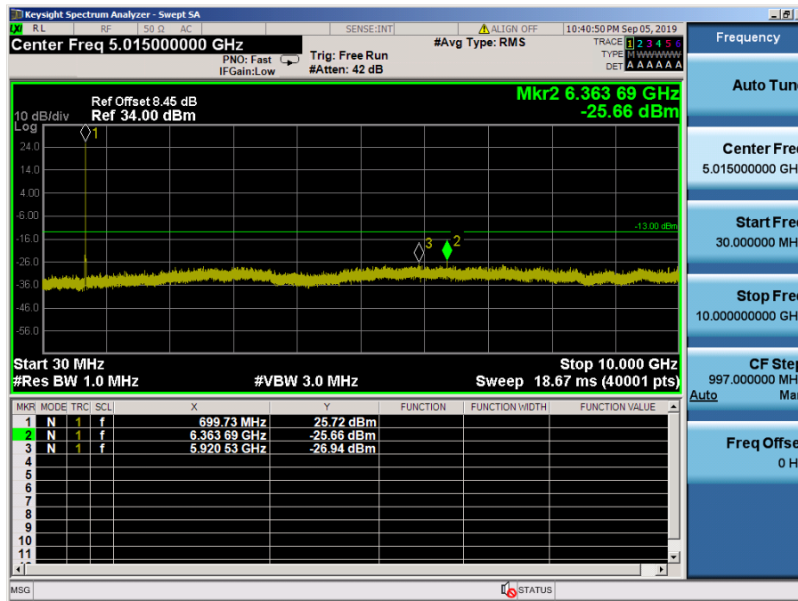
LTE Band 12 / 3MHz / 64QAM - RB Size/Offset (15/0) – Low Channel
