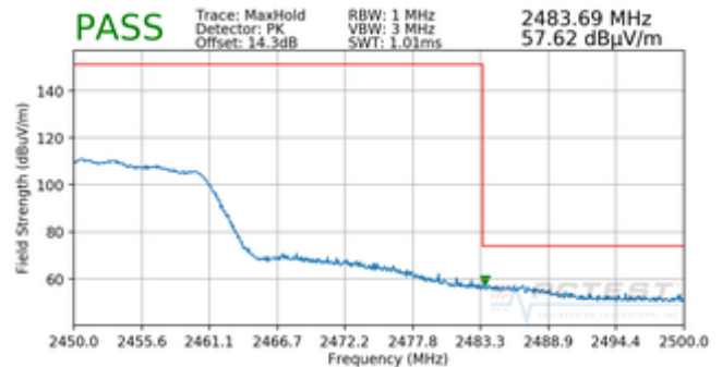
Plot 7-14. Radiated Restricted Upper Band Edge Measurement SISO ANT1 (Peak)
