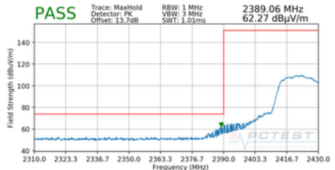
Plot 7-22. Radiated Restricted Lower Band Edge Measurement SISO ANT2 (Peak)
