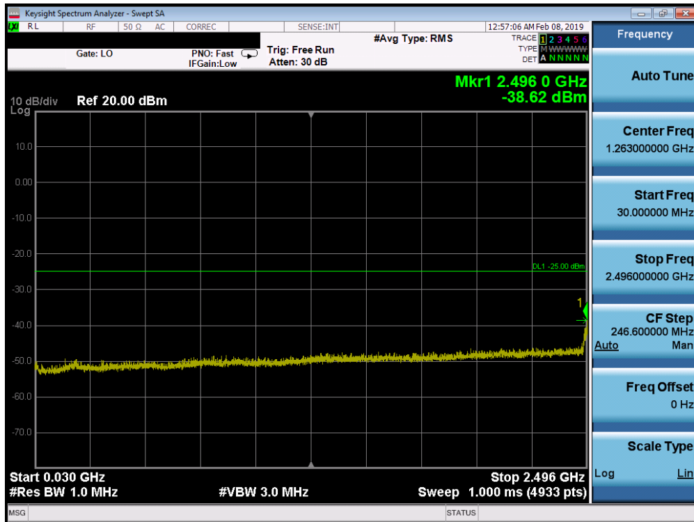
Plot 7-5. Conducted Spurious Plot (Band 41 – 20.0MHz QPSK – PCC 100/0 SCC 100/0 – Mid Channel)
