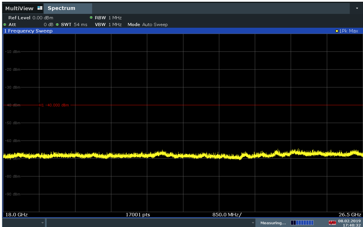
Plot 7-18. Radiated Spurious Plot 18GHz – 26.5GHz (Band 30) - H
