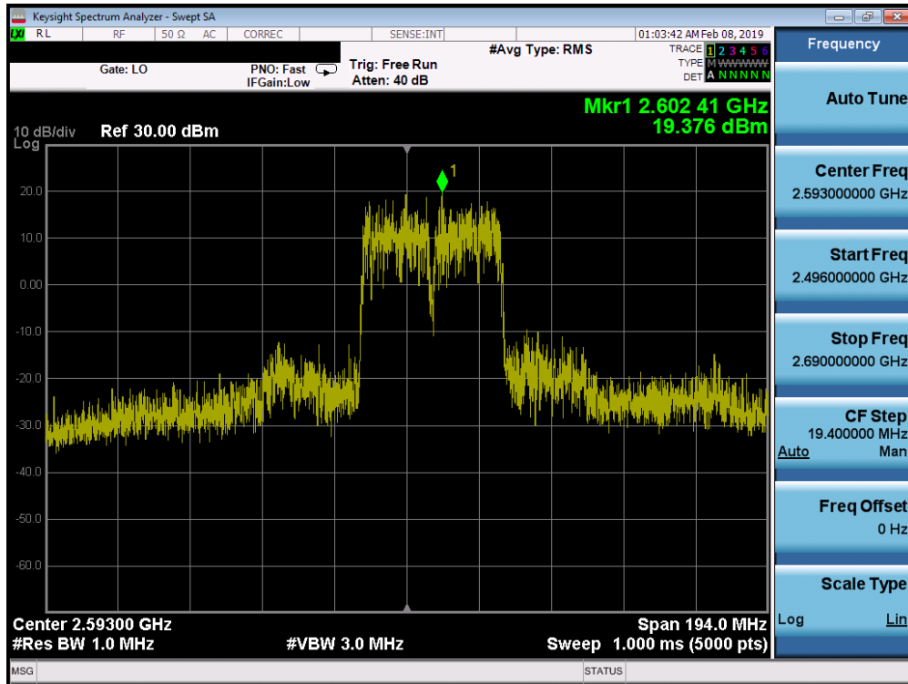
Plot 7-6. Conducted Spurious Plot (Band 41 – 20.0MHz QPSK – PCC 100/0 SCC 100/0 – Mid Channel)
