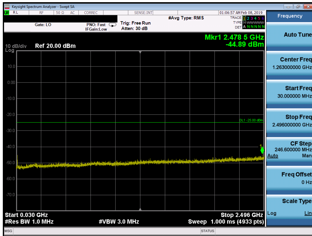
Plot 7-1. Conducted Spurious Plot (Band 41 – 20.0MHz QPSK – PCC 1/99 SCC 1/0 – Mid Channel)
