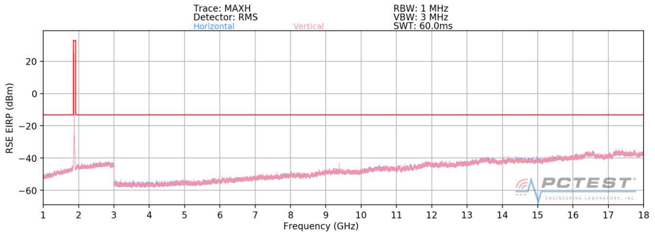
Plot 7-16. Radiated Spurious Plot above 1GHz (Band 25/2)
