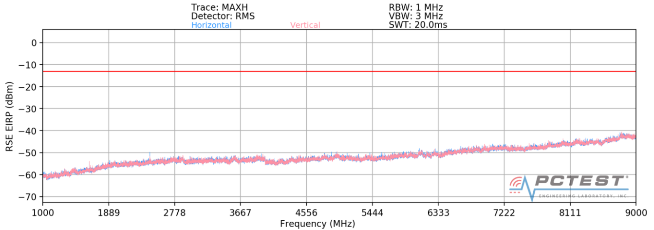
Plot 7-14. Radiated Spurious Plot above 1GHz (Band 26/5)
