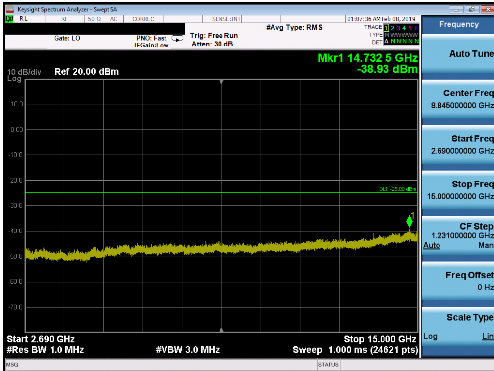
Plot 7-3. Conducted Spurious Plot (Band 41 – 20.0MHz QPSK – PCC 1/99 SCC 1/0 – Mid Channel)
