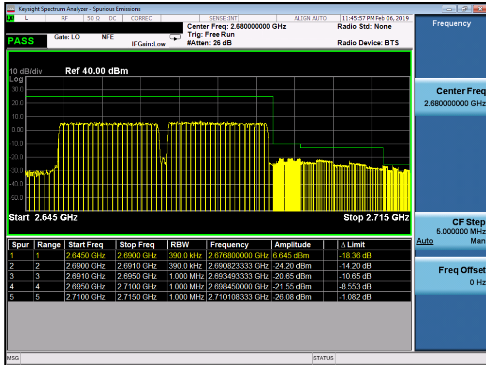
Plot 7-10. Upper ACP Plot (Band 41 QPSK – PCC:20 MHz SCC:20 MHz – Full RB)
