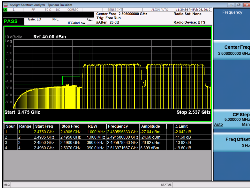
Plot 7-9. Lower ACP Plot (Band 41 QPSK – PCC:20 MHz SCC:20 MHz – Full RB)
