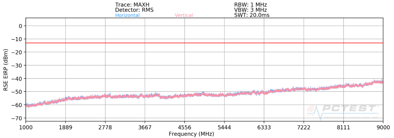
Plot 7-27. Radiated Spurious Plot (ULCA B5 PCC: RB 50 Offset 0, SCC: RB 50 Offset 0 – Low Channel)
