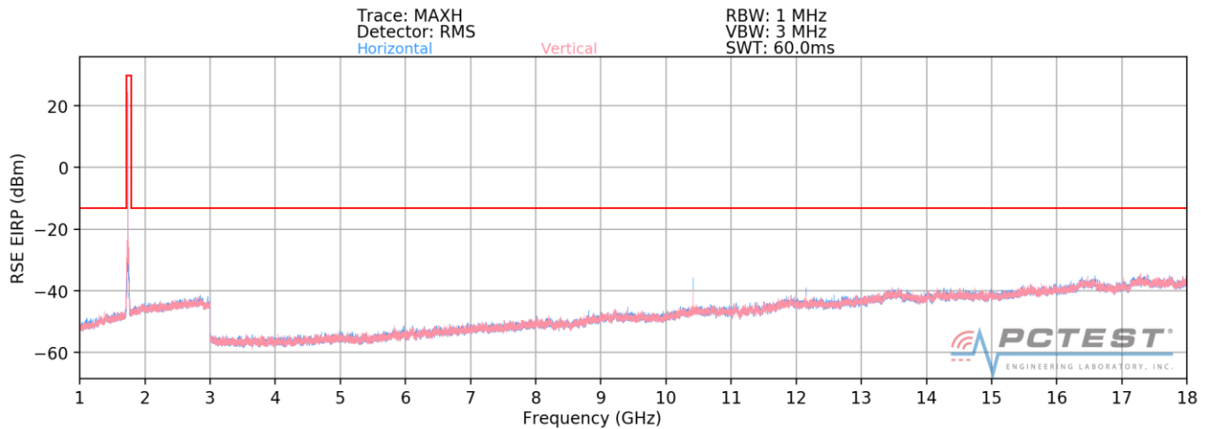
Plot 7-15. Radiated Spurious Plot above 1GHz (Band 66/4)
