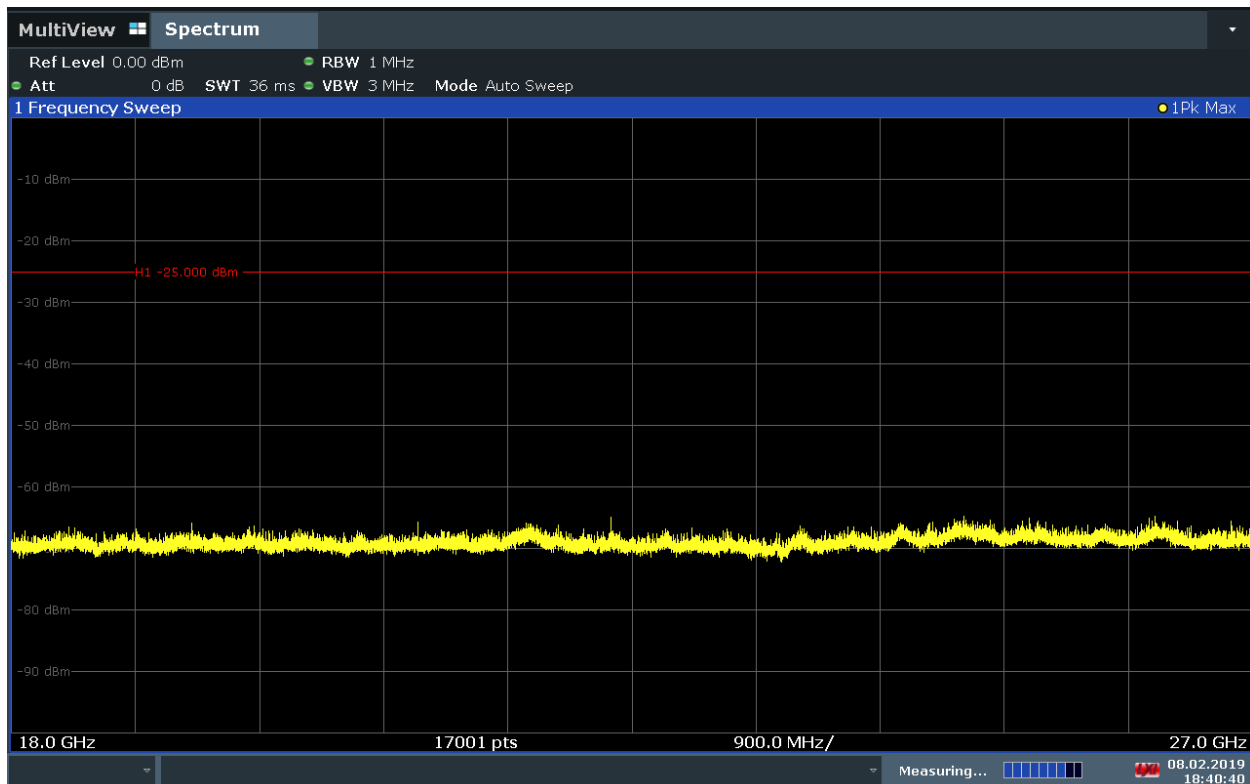
Plot 7-25. Radiated Spurious Plot 18GHz – 27GHz (Band 41 PC2) - V
