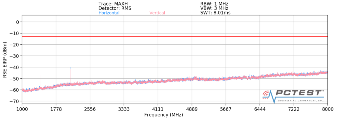
Plot 7-12. Radiated Spurious Plot above 1GHz (Band 17/12)
