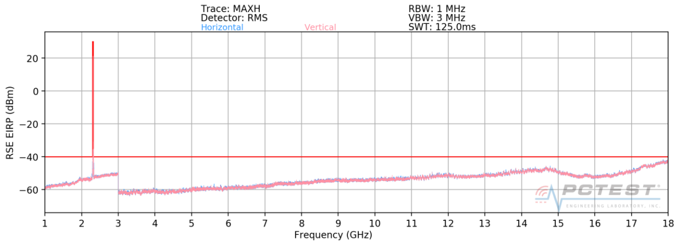
Plot 7-17. Radiated Spurious Plot 1GHz - 18GHz (Band 30)
