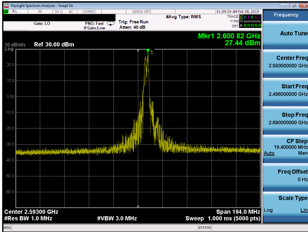
Plot 7-2. Conducted Spurious Plot (Band 41 – 20.0MHz QPSK – PCC 1/99 SCC 1/0 – Mid Channel)
