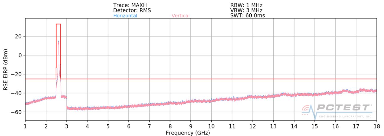
Plot 7-57. Radiated Spurious Plot (ULCA B41 PC2 PCC: RB 100 Offset 0, SCC: RB 100 Offset 0)
