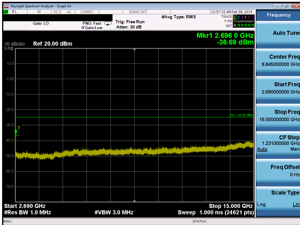
Plot 7-7. Conducted Spurious Plot (Band 41 – 20.0MHz QPSK – PCC 100/0 SCC 100/0 – Mid Channel)
