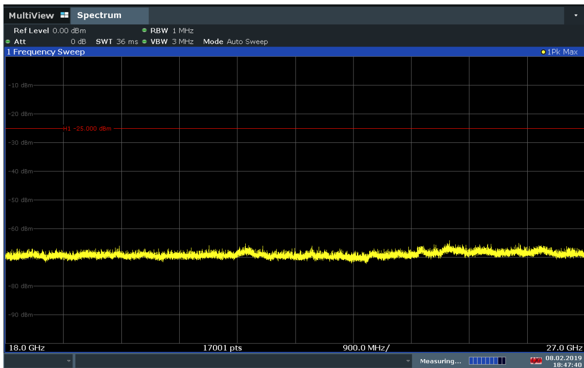
Plot 7-28. Radiated Spurious Plot 18GHz – 27GHz (Band 41 PC2 PCC: RB 1 Offset 99, SCC: RB 1 Offset 0) – H
