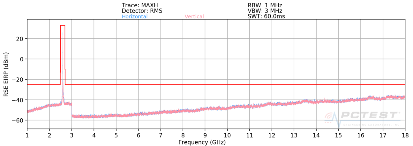
Plot 7-56. Radiated Spurious Plot (ULCA B41 PC2 PCC: RB 1 Offset 99, SCC: RB 1 Offset 0)
