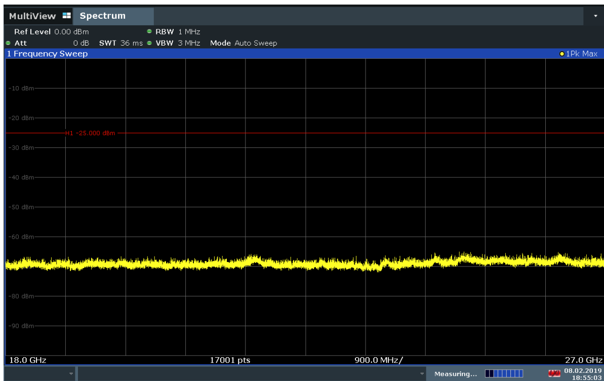
Plot 7-30. Radiated Spurious Plot 18GHz – 27GHz (Band 41 PC2 PCC: RB 100 Offset 0, SCC: RB 100 Offset 0) – H
