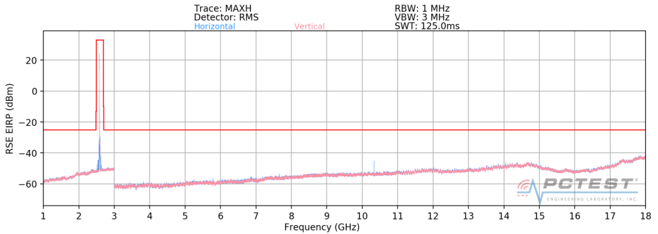
Plot 7-23. Radiated Spurious Plot 1GHz - 18GHz (Band 41 PC2)
