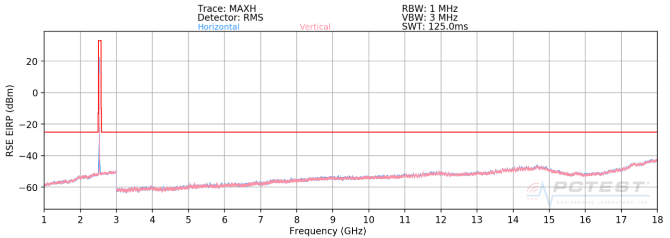
Plot 7-20. Radiated Spurious Plot 1GHz - 18GHz (Band 7)
