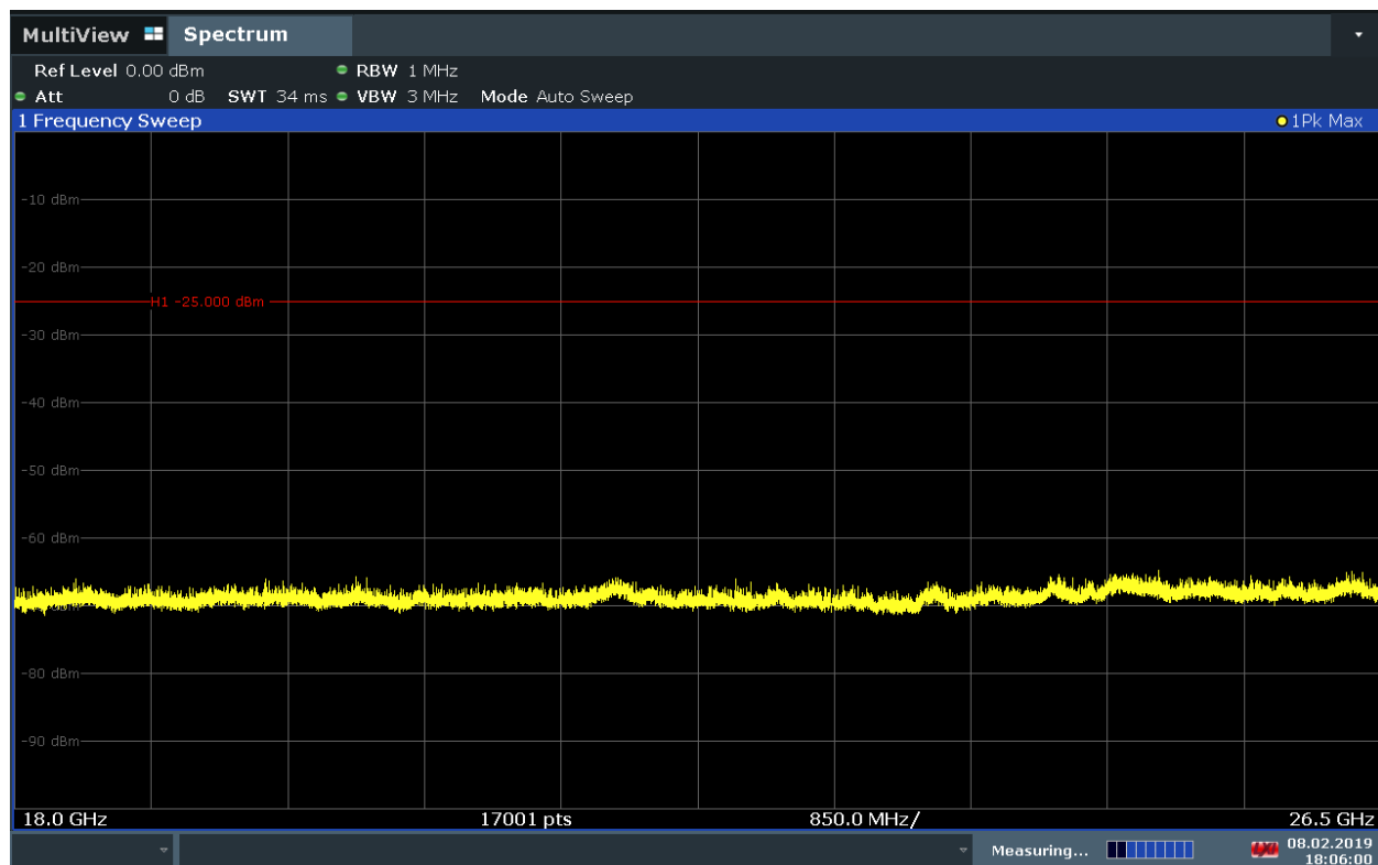
Plot 7-22. Radiated Spurious Plot 18GHz – 26.5GHz (Band 7) - V
