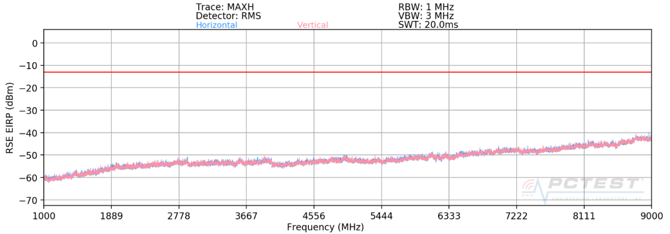
Plot 7-26. Radiated Spurious Plot (ULCA B5 PCC: RB 1 Offset 49, SCC: RB 1 Offset 0 – Low Channel)
