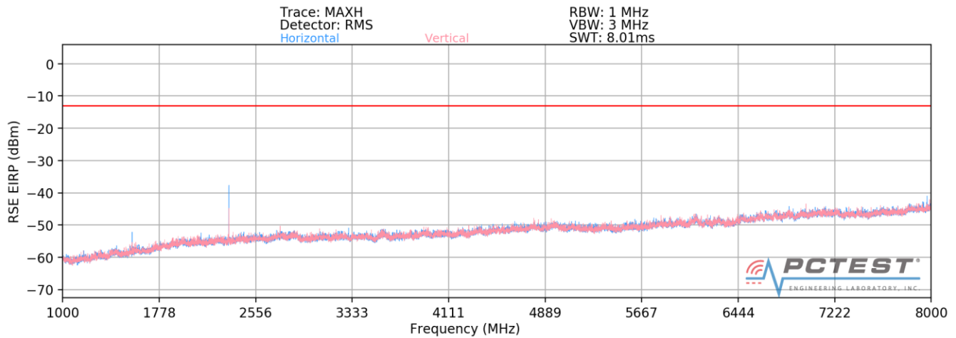
Plot 7-13. Radiated Spurious Plot above 1GHz (Band 13)
