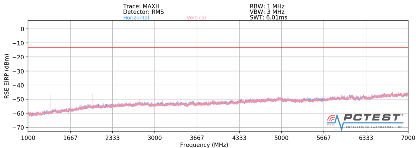
Plot 7-11. Radiated Spurious Plot above 1GHz (Band 71)
