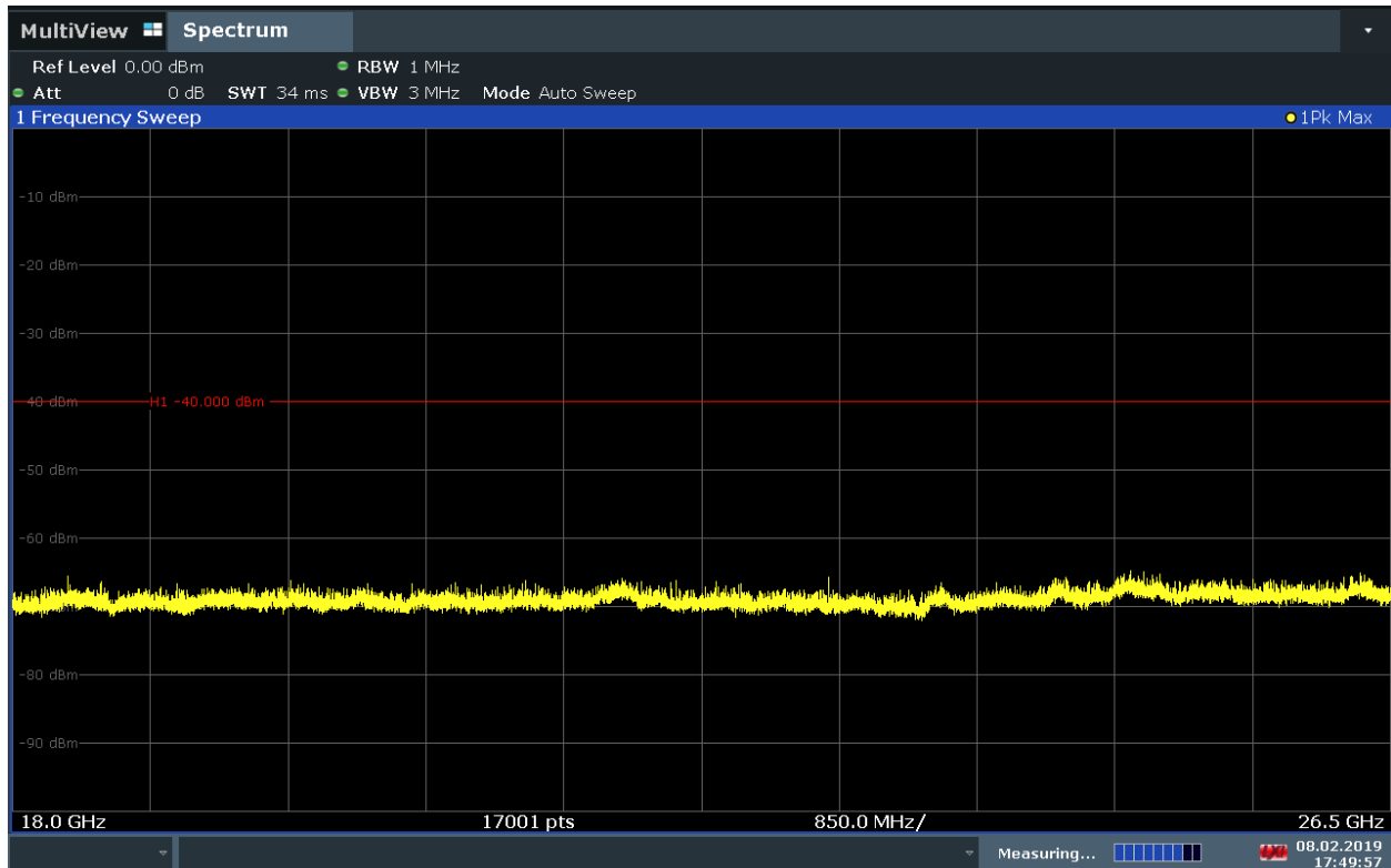
Plot 7-19. Radiated Spurious Plot 18GHz – 26.5GHz (Band 30) - V
