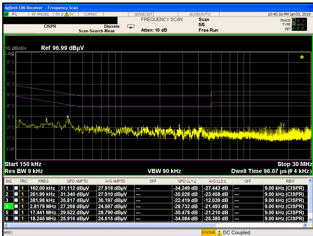
Plot 7-273. Line Conducted Plot with 802.11a UNII Band 2A (L1) on WCP
