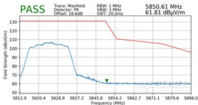
Plot 7-239. Radiated Upper Band Edge Plot (Peak – UNII Band 3)
