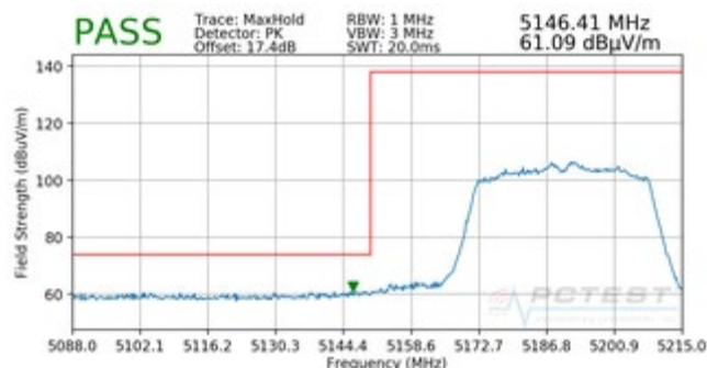
Plot 7-243. Radiated Lower Band Edge Plot (Peak - UNII Band 1)
