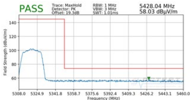
Plot 7-207. Radiated Band Edge Plot (Peak – WCP)
