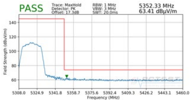
Plot 7-236. Radiated Upper Band Edge Plot (Peak - UNII Band 2A)
