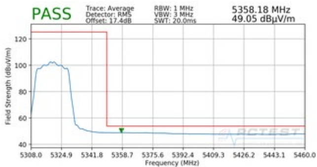
Plot 7-235. Radiated Upper Band Edge Plot (Average - UNII Band 2A)
