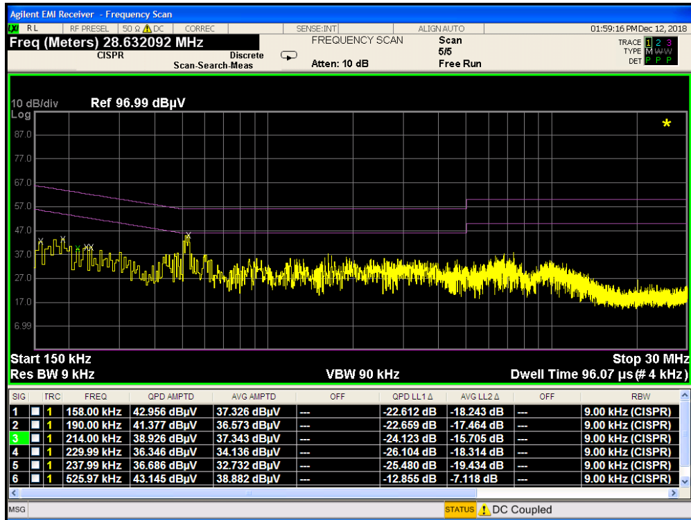
Plot 7-269. Line Conducted Plot with 802.11a UNII Band 3 (L1)
