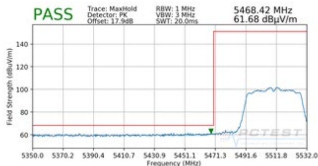
Plot 7-186. Radiated Lower Band Edge Plot (Peak – UNII Band 2C)
