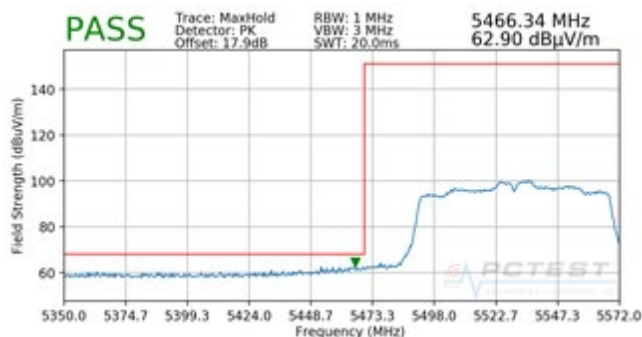
Plot 7-195. Radiated Lower Band Edge Plot (Peak – UNII Band 2C)
