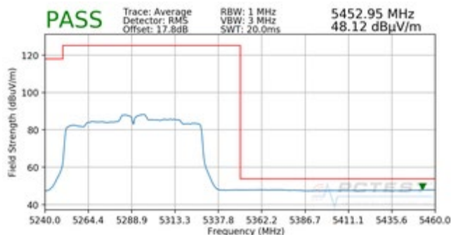
Plot 7-192. Radiated Upper Band Edge Plot (Average - UNII Band 2A)
