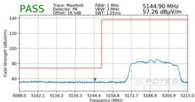
Plot 7-189. Radiated Band Edge Plot (Peak – WCP)
