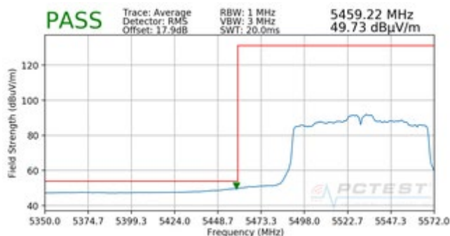
Plot 7-255. Radiated Lower Band Edge Plot (Average – UNII Band 2C)
