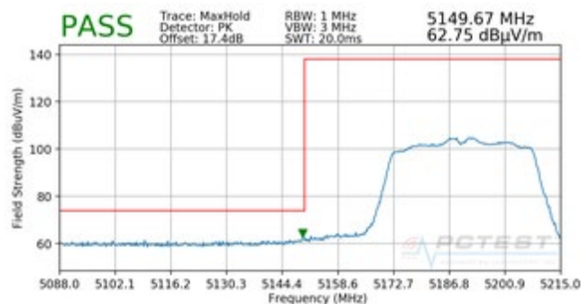
Plot 7-182. Radiated Lower Band Edge Plot (Peak - UNII Band 1)
