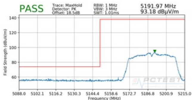
Plot 7-250. Radiated Band Edge Plot (Peak – WCP)
