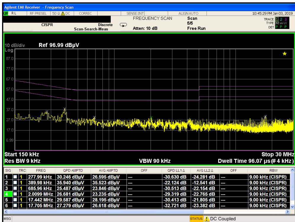
Plot 7-275. Line Conducted Plot with 802.11a UNII Band 2C (L1) on WCP
