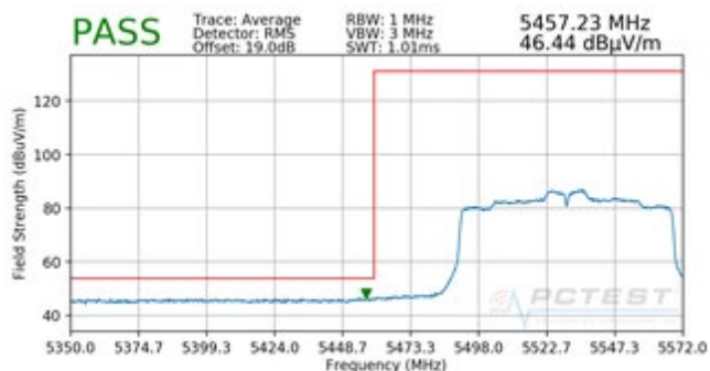
Plot 7-197. Radiated Band Edge Plot (Average – WCP)
