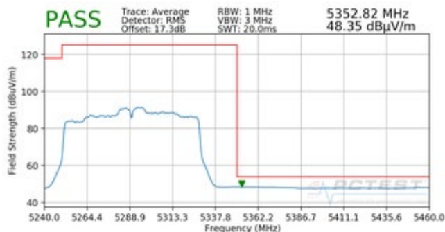
Plot 7-253. Radiated Upper Band Edge Plot (Average - UNII Band 2A)
