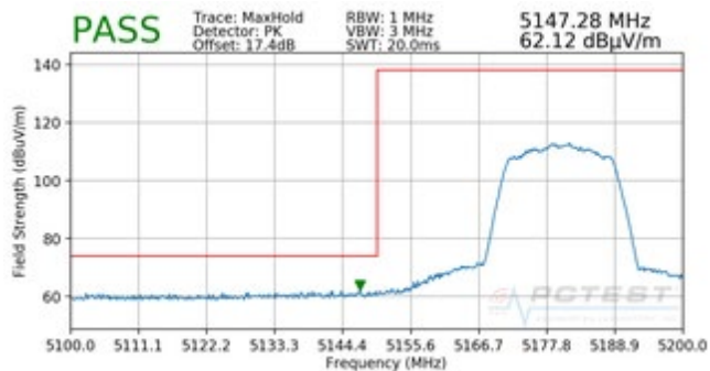
Plot 7-234. Radiated Lower Band Edge Plot (Peak - UNII Band 1)
