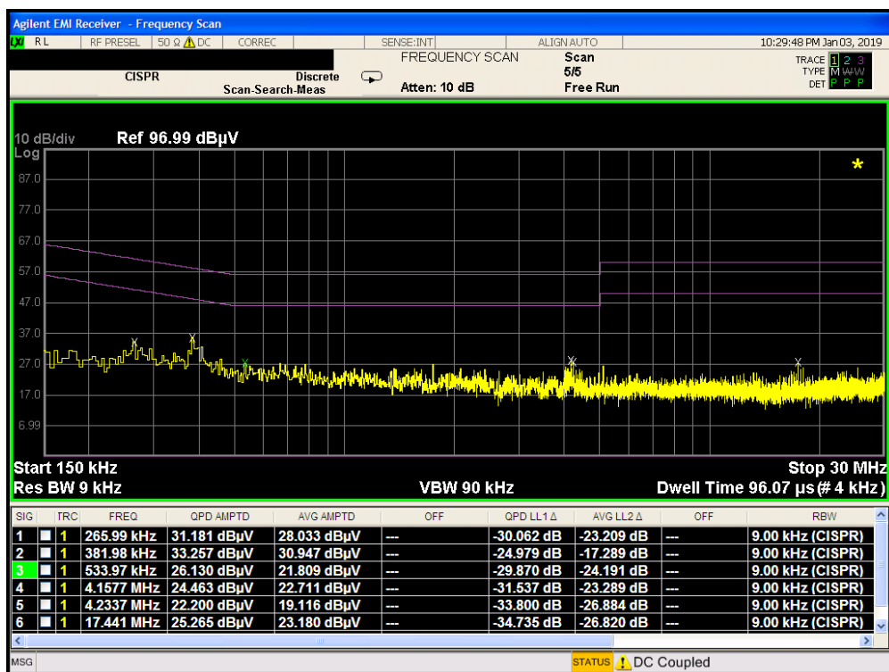
Plot 7-274. Line Conducted Plot with 802.11a UNII Band 2A (N) on WCP
