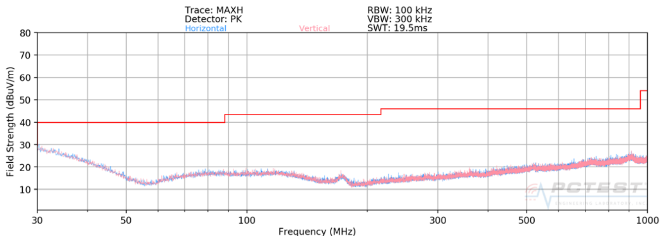
Plot 7-260. Radiated Spurious Plot below 1GHz
