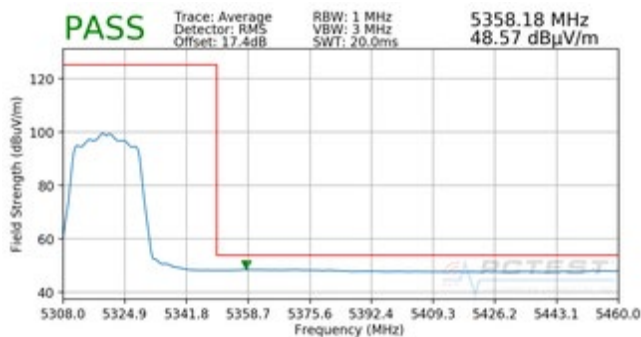
Plot 7-174. Radiated Upper Band Edge Plot (Average - UNII Band 2A)
