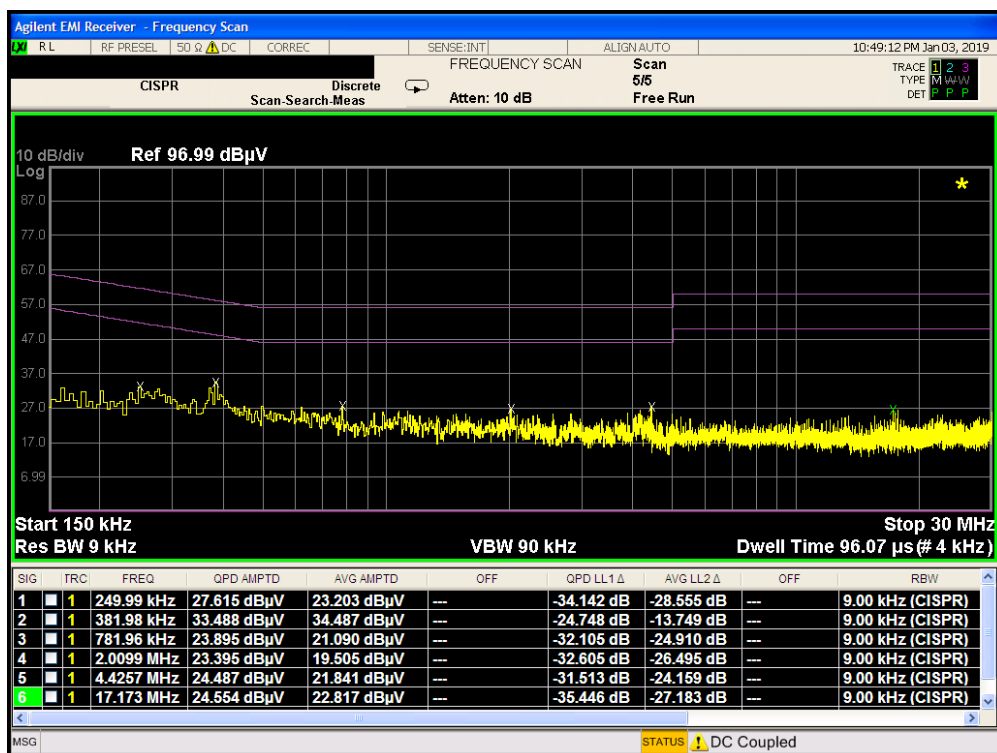
Plot 7-276. Line Conducted Plot with 802.11a UNII Band 2C (N) on WCP
