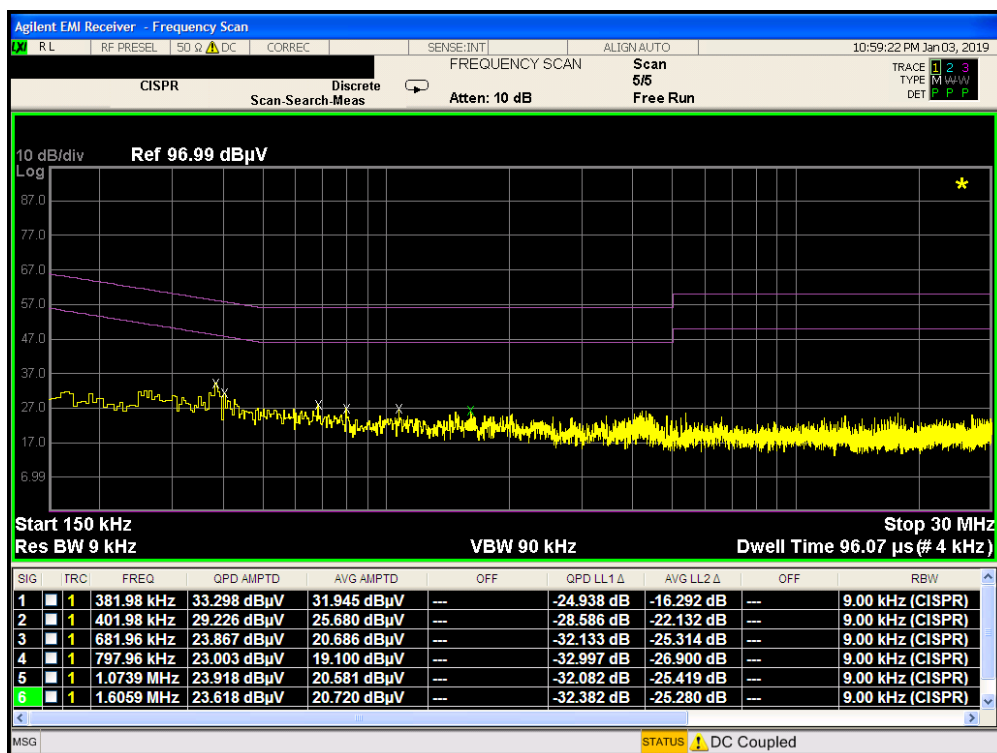
Plot 7-278. Line Conducted Plot with 802.11a UNII Band 3 (N) on WCP
