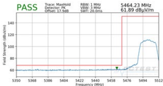
Plot 7-238. Radiated Lower Band Edge Plot (Peak – UNII Band 2C)
