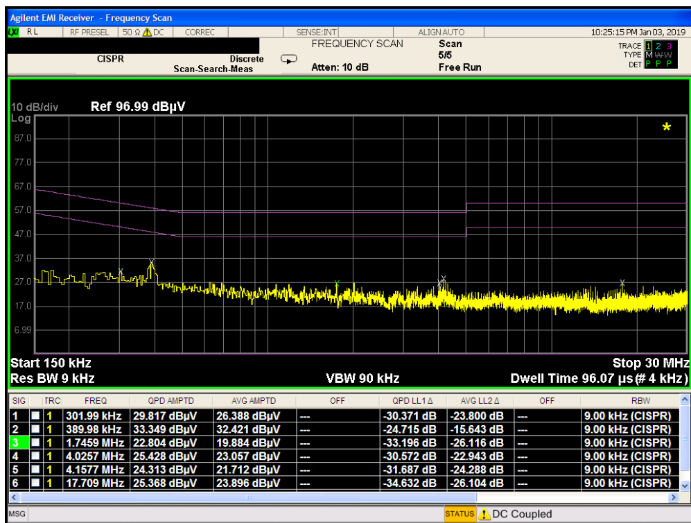
Plot 7-272. Line Conducted Plot with 802.11a UNII Band 1 (N) on WCP
