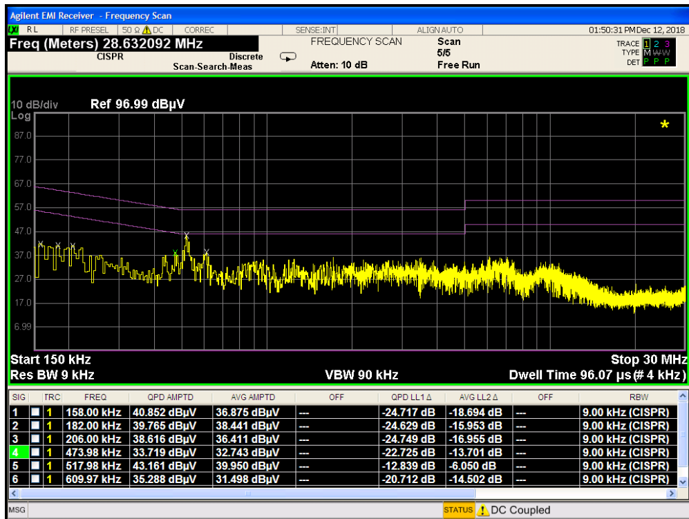
Plot 7-267. Line Conducted Plot with 802.11a UNII Band 2C (L1)
