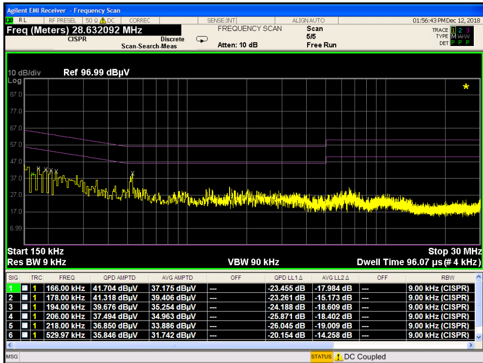
Plot 7-270. Line Conducted Plot with 802.11a UNII Band 3 (N)
