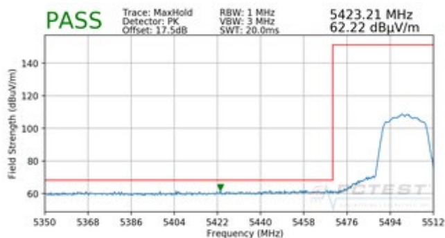
Plot 7-177. Radiated Lower Band Edge Plot (Peak – UNII Band 2C)
