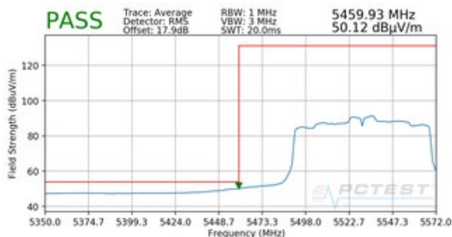
Plot 7-194. Radiated Lower Band Edge Plot (Average – UNII Band 2C)
