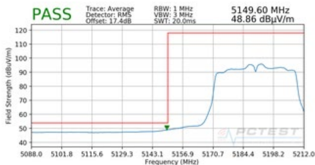
Plot 7-181. Radiated Lower Band Edge Plot (Average - UNII Band 1)
