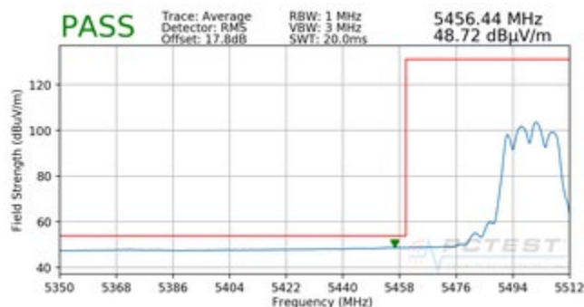
Plot 7-230. Radiated Lower Band Edge Plot (Average – UNII Band 2C)
