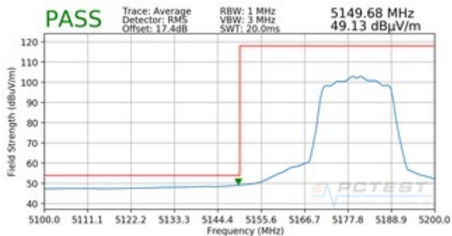
Plot 7-233. Radiated Lower Band Edge Plot (Average - UNII Band 1)
