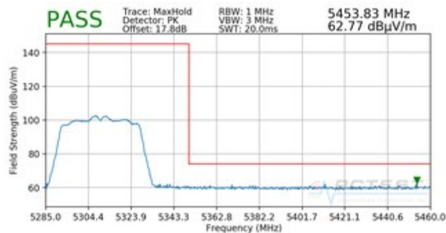
Plot 7-184. Radiated Upper Band Edge Plot (Peak - UNII Band 2A)
