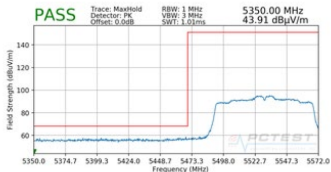
Plot 7-198. Radiated Band Edge Plot (Peak – WCP)
