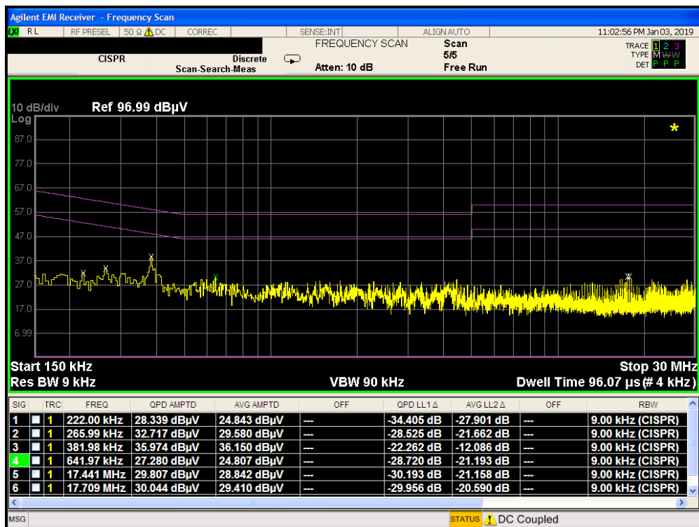
Plot 7-277. Line Conducted Plot with 802.11a UNII Band 3 (L1) on WCP
