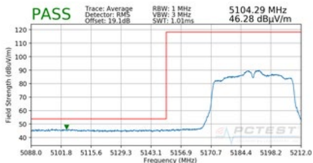
Plot 7-249. Radiated Band Edge Plot (Average – WCP)
