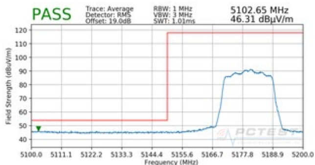
Plot 7-240. Radiated Band Edge Plot (Average – WCP)
