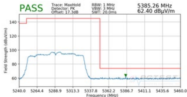
Plot 7-193. Radiated Upper Band Edge Plot (Peak - UNII Band 2A)
