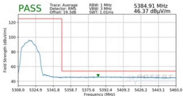
Plot 7-179. Radiated Band Edge Plot (Average – WCP)
