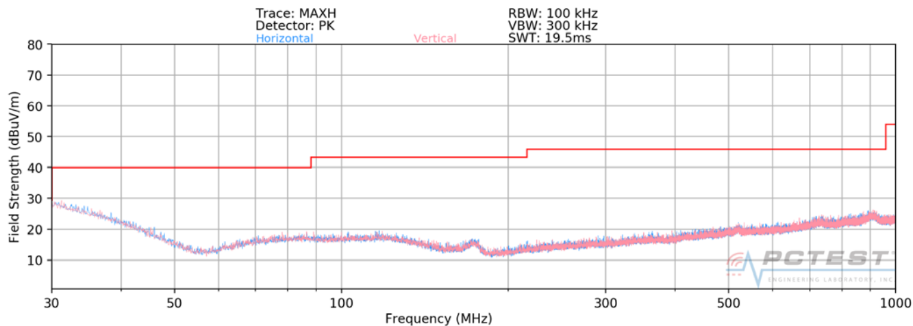
Plot 7-261. Radiated Spurious Plot below 1GHz
