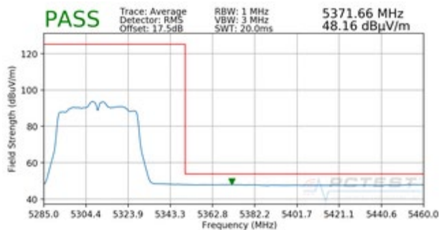
Plot 7-183. Radiated Upper Band Edge Plot (Average - UNII Band 2A)
