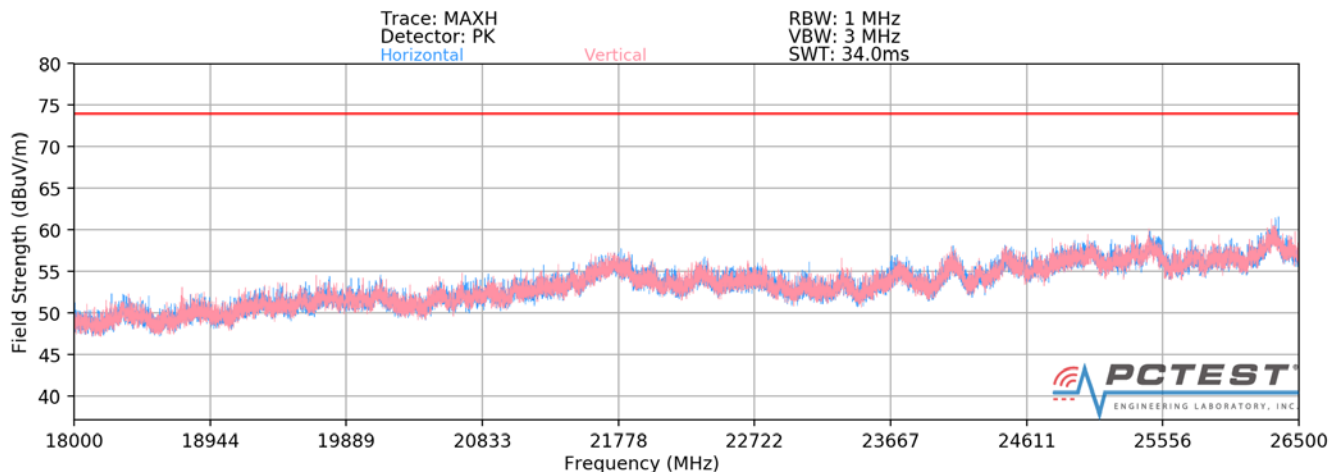
Plot 7-167. Radiated Spurious Plot 18GHz - 26.5GHz (802.11a)
