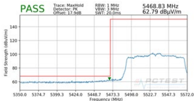
Plot 7-256. Radiated Lower Band Edge Plot (Peak – UNII Band 2C)
