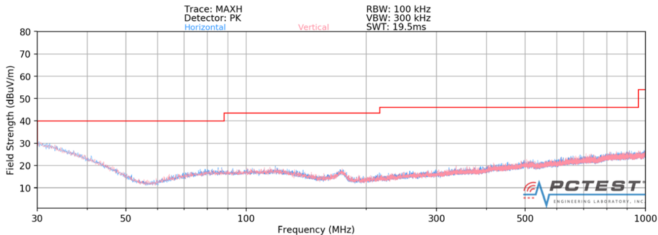
Plot 7-262. Radiated Spurious Plot below 1GHz (2.4GHz – 5GHz)
