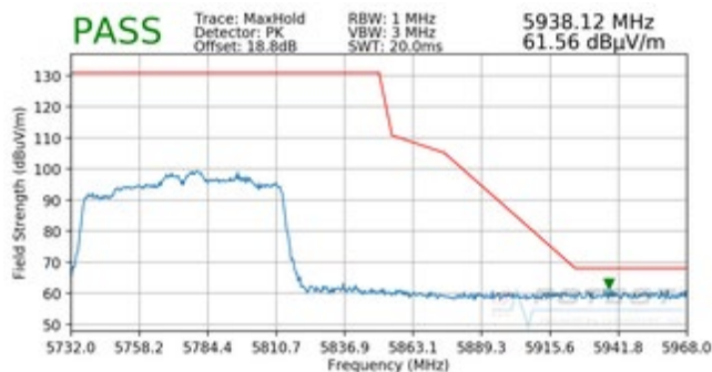
Plot 7-196. Radiated Upper Band Edge Plot (Peak – UNII Band 3)
