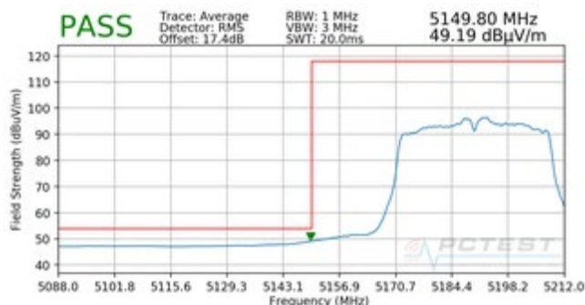
Plot 7-242. Radiated Lower Band Edge Plot (Average - UNII Band 1)
