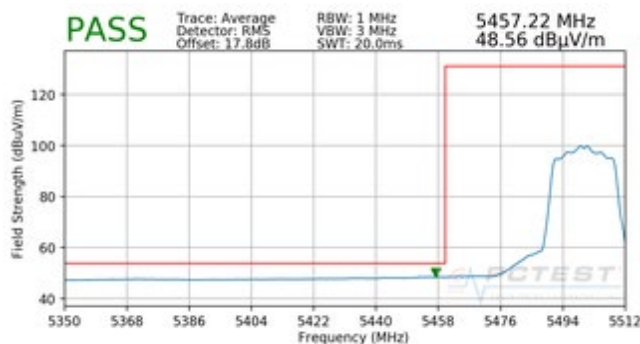
Plot 7-176. Radiated Lower Band Edge Plot (Average – UNII Band 2C)
