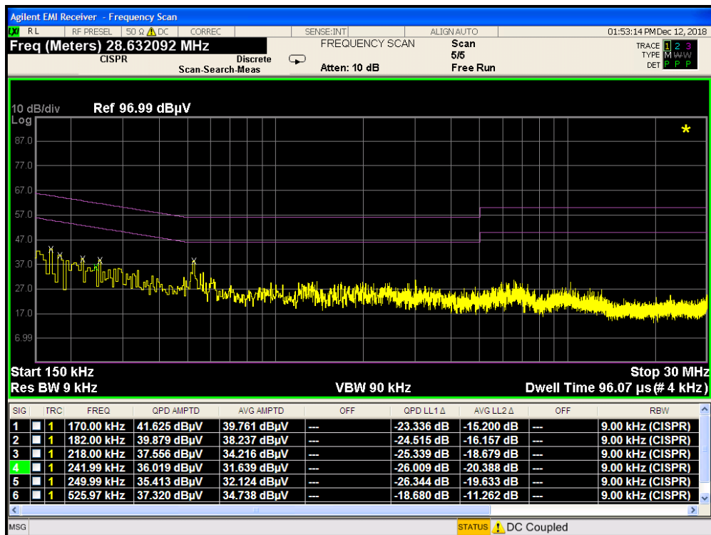
Plot 7-268. Line Conducted Plot with 802.11a UNII Band 2C (N)
