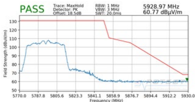
Plot 7-248. Radiated Upper Band Edge Plot (Peak – UNII Band 3)
