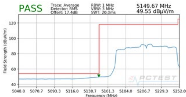
Plot 7-190. Radiated Lower Band Edge Plot (Average - UNII Band 1)
