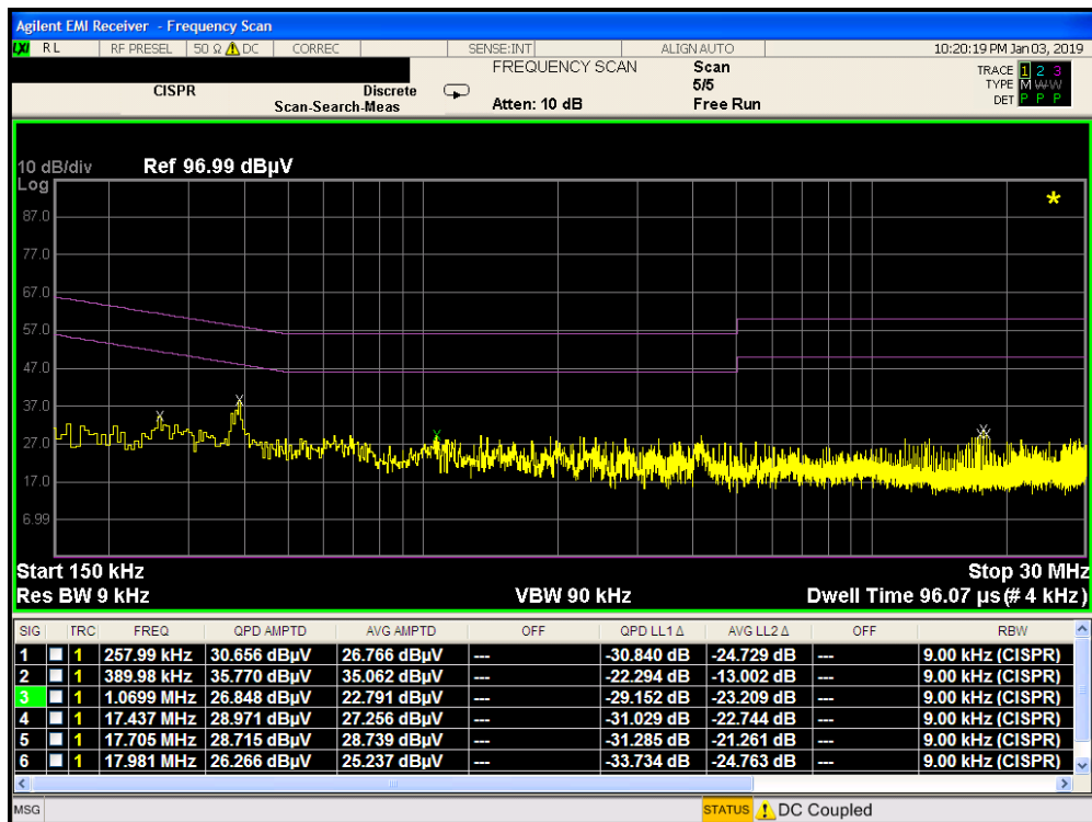
Plot 7-271. Line Conducted Plot with 802.11a UNII Band 1 (L1) on WCP
