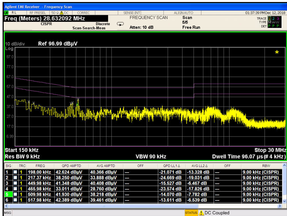
Plot 7-263. Line Conducted Plot with 802.11a UNII Band 1 (L1)
