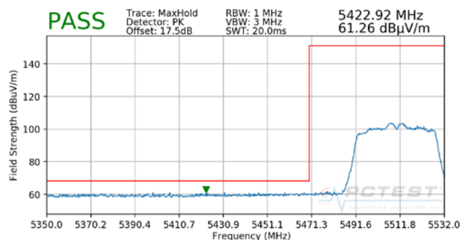
Plot 7-247. Radiated Lower Band Edge Plot (Peak – UNII Band 2C)
