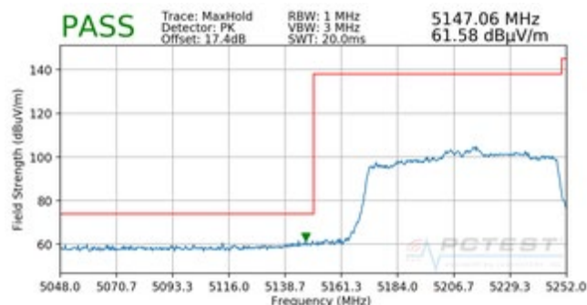
Plot 7-252. Radiated Lower Band Edge Plot (Peak - UNII Band 1)
