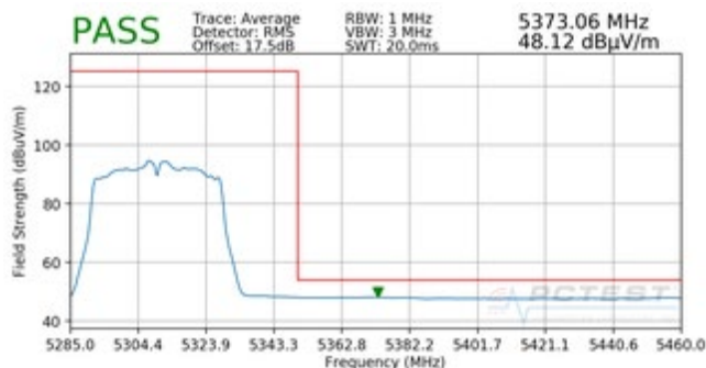
Plot 7-244. Radiated Upper Band Edge Plot (Average - UNII Band 2A)
