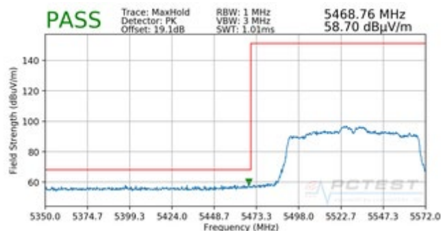
Plot 7-259. Radiated Band Edge Plot (Peak – WCP)
