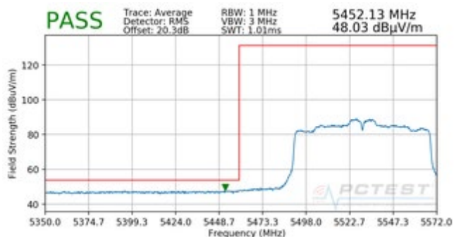
Plot 7-258. Radiated Band Edge Plot (Average – WCP)
