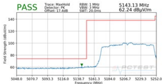
Plot 7-191. Radiated Lower Band Edge Plot (Peak - UNII Band 1)
