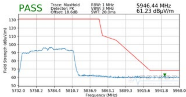
Plot 7-257. Radiated Upper Band Edge Plot (Peak – UNII Band 3)
