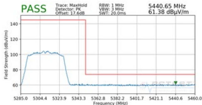
Plot 7-245. Radiated Upper Band Edge Plot (Peak - UNII Band 2A)
