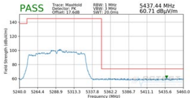
Plot 7-254. Radiated Upper Band Edge Plot (Peak - UNII Band 2A)
