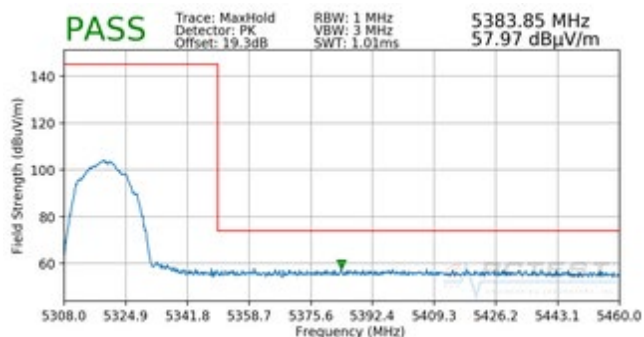
Plot 7-180. Radiated Band Edge Plot (Peak – WCP)
