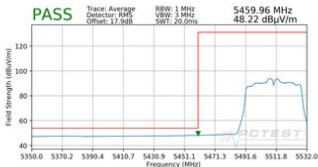
Plot 7-246. Radiated Lower Band Edge Plot (Average – UNII Band 2C)
