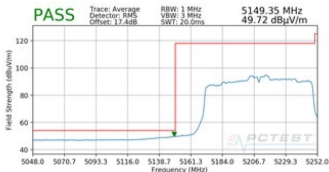
Plot 7-251. Radiated Lower Band Edge Plot (Average - UNII Band 1)
