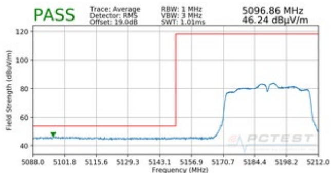
Plot 7-188. Radiated Band Edge Plot (Average – WCP)
