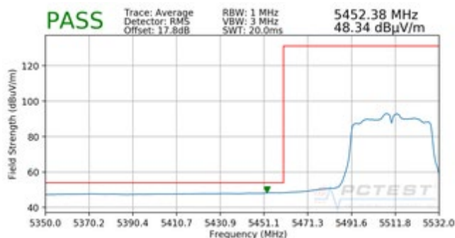
Plot 7-185. Radiated Lower Band Edge Plot (Average – UNII Band 2C)
