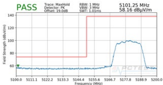
Plot 7-241. Radiated Band Edge Plot (Peak – WCP)
