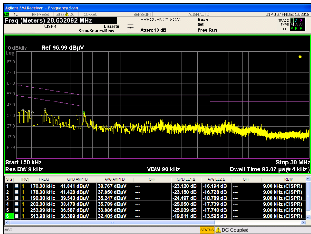
Plot 7-264. Line Conducted Plot with 802.11a UNII Band 1 (N)
