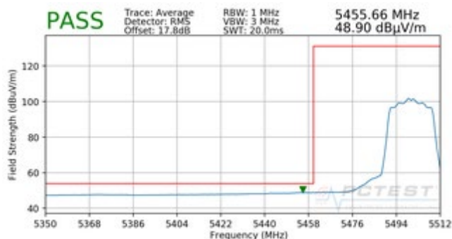
Plot 7-237. Radiated Lower Band Edge Plot (Average – UNII Band 2C)
