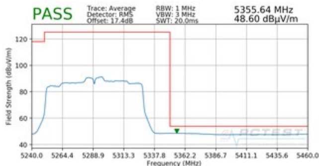
Plot 7-219. Radiated Upper Band Edge Plot (Average - UNII Band 2A)
