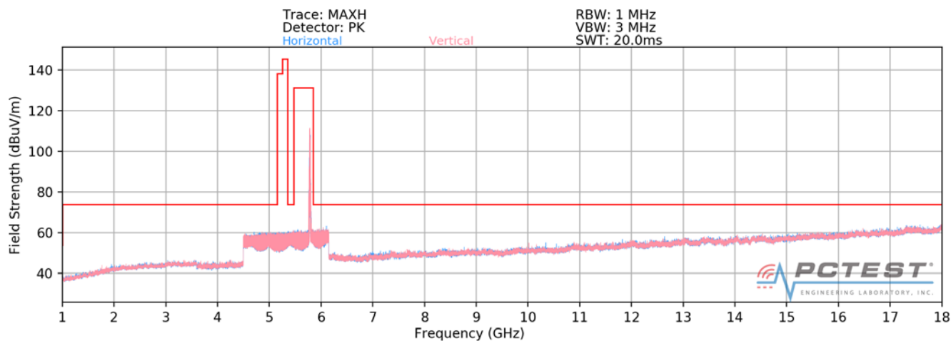
Plot 7-160. Radiated Spurious Plot above 1GHz (802.11a – U3 Ch. 157)
