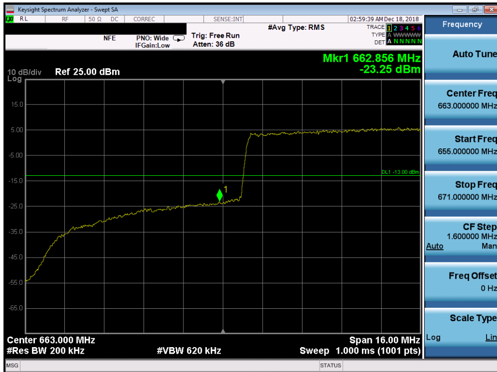
Plot 7-193. Lower Band Edge Plot (Band 71 - 20.0MHz QPSK - Full RB Configuration)
