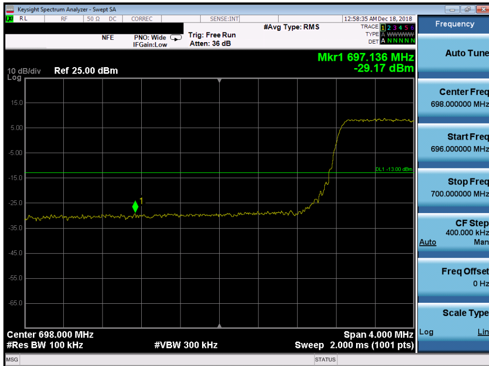
Plot 7-199. Lower Band Edge Plot (Band 12 - 5.0MHz QPSK - Full RB Configuration)
