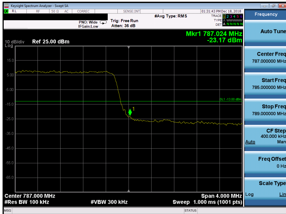
Plot 7-206. Upper Band Edge Plot (Band 13 - 5.0MHz QPSK - Full RB Configuration)
