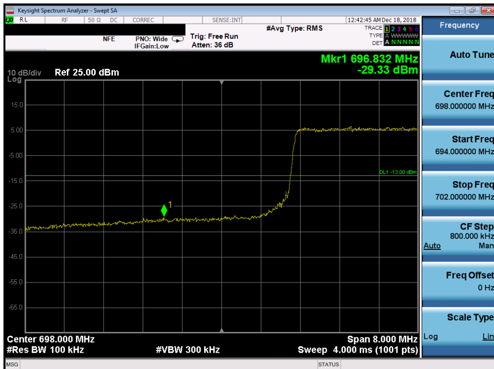
Plot 7-202. Lower Band Edge Plot (Band 12 - 10.0MHz QPSK - Full RB Configuration)
