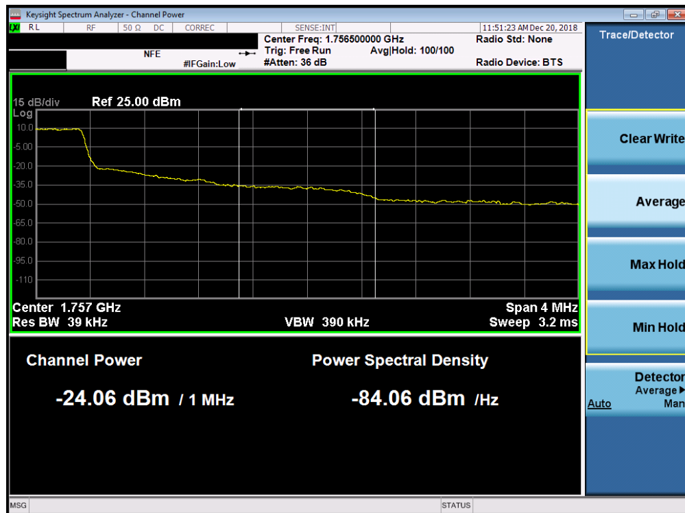
Plot 7-222. Upper Extended Band Edge Plot (Band 4 - 1.4MHz QPSK - Full RB Configuration)
