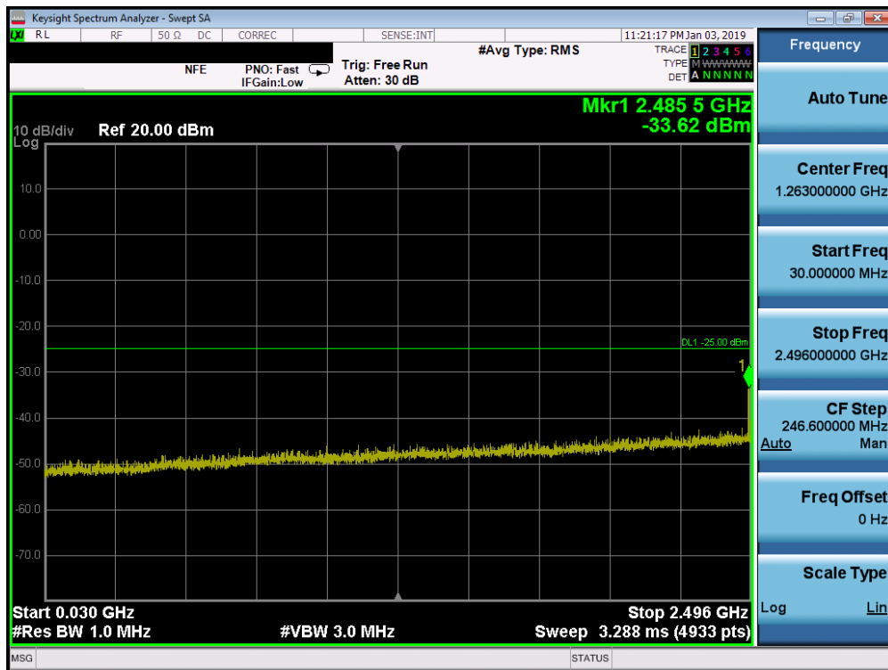
Plot 7-181. Conducted Spurious Plot (Band 41 - 20.0MHz QPSK - RB Size 1, RB Offset 0 - Mid Channel)
