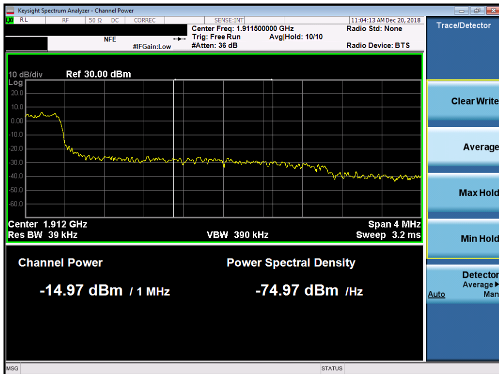
Plot 7-264. Upper Extended Band Edge Plot (Band 2 - 3.0MHz QPSK - Full RB Configuration)
