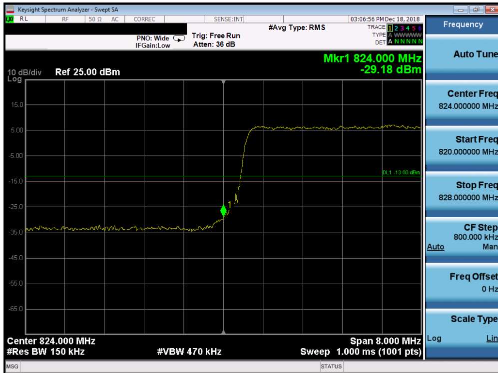
Plot 7-215. Lower Band Edge Plot (Band 26/5 - 10.0MHz QPSK - Full RB Configuration)
