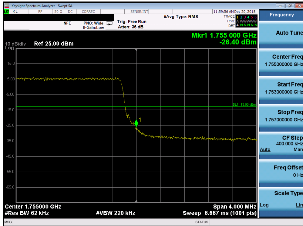
Plot 7-233. Upper Band Edge Plot (Band 4 - 5.0MHz QPSK - Full RB Configuration)
