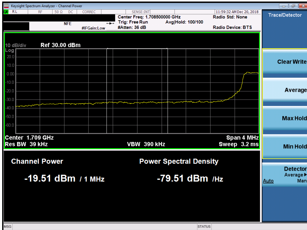
Plot 7-232. Lower Extended Band Edge Plot (Band 66/4 - 5.0MHz QPSK - Full RB Configuration)
