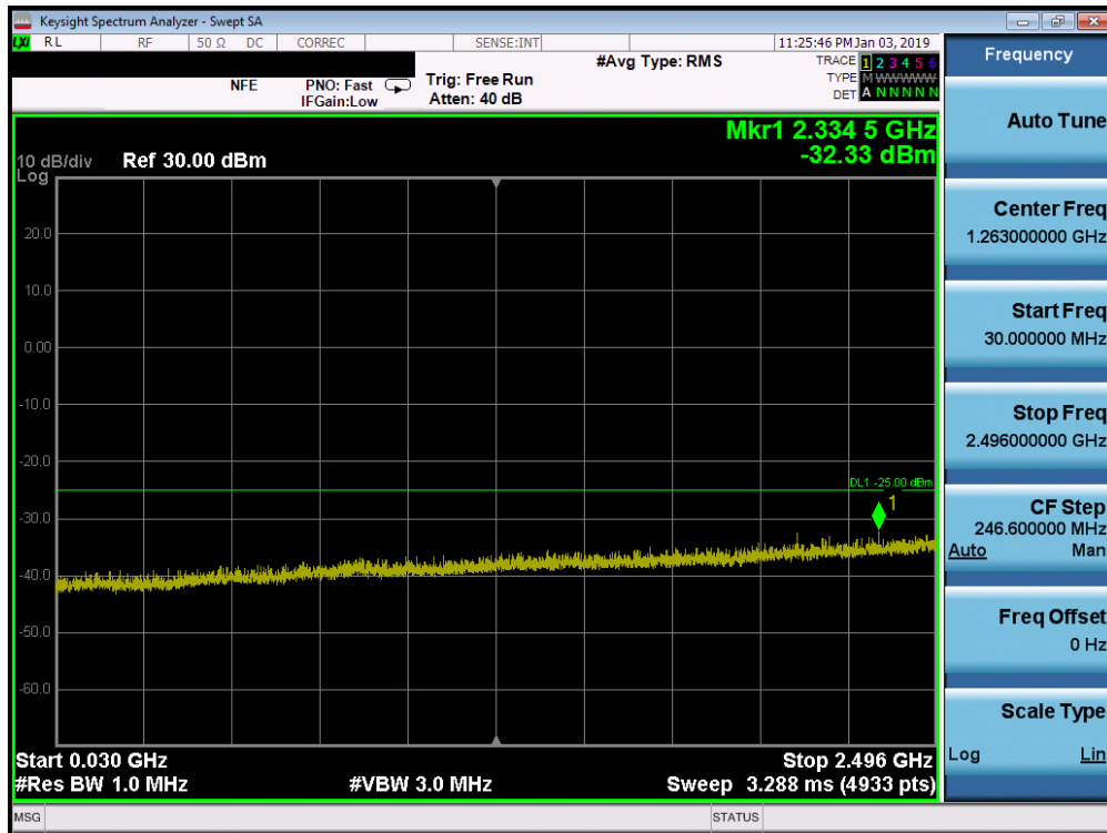
Plot 7-184. Conducted Spurious Plot (Band 41 - 20.0MHz QPSK - RB Size 1, RB Offset 0 - High Channel)
