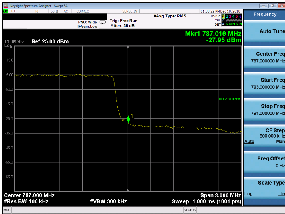
Plot 7-208. Upper Band Edge Plot (Band 13 - 10.0MHz QPSK - Full RB Configuration)
