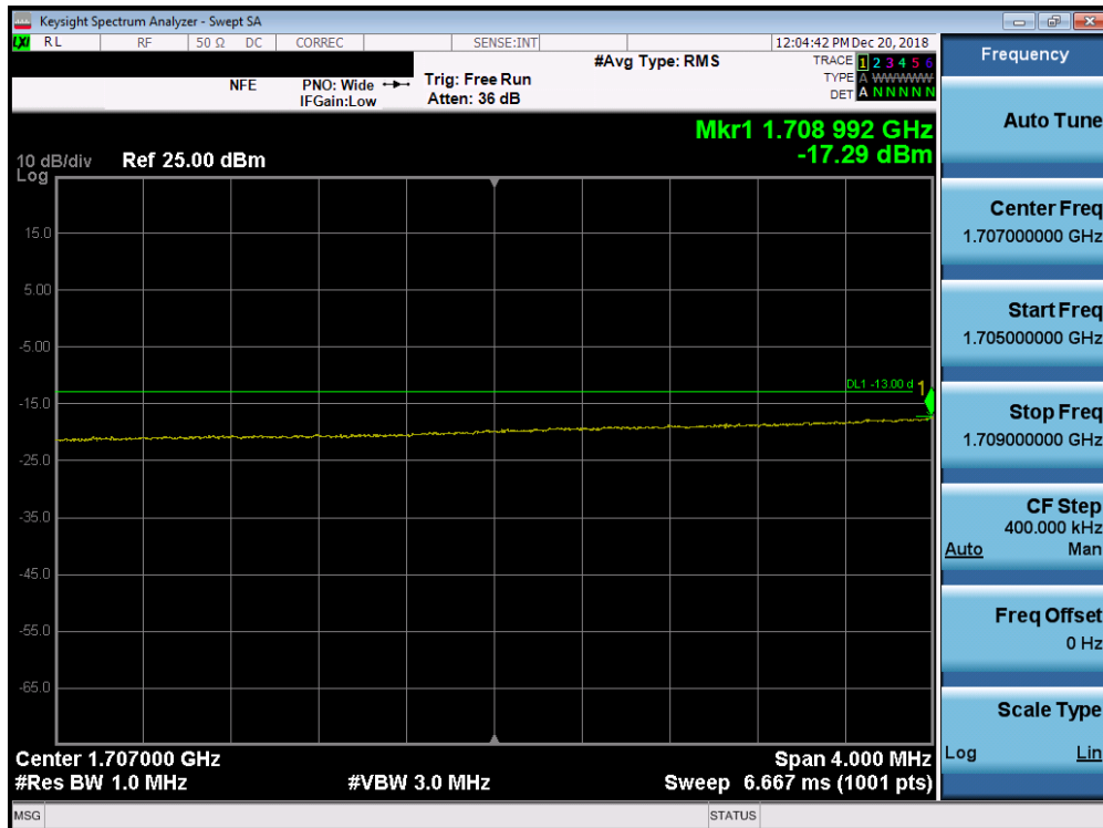
Plot 7-244. Lower Extended Band Edge Plot (Band 66/4 - 15.0MHz QPSK - Full RB Configuration)
