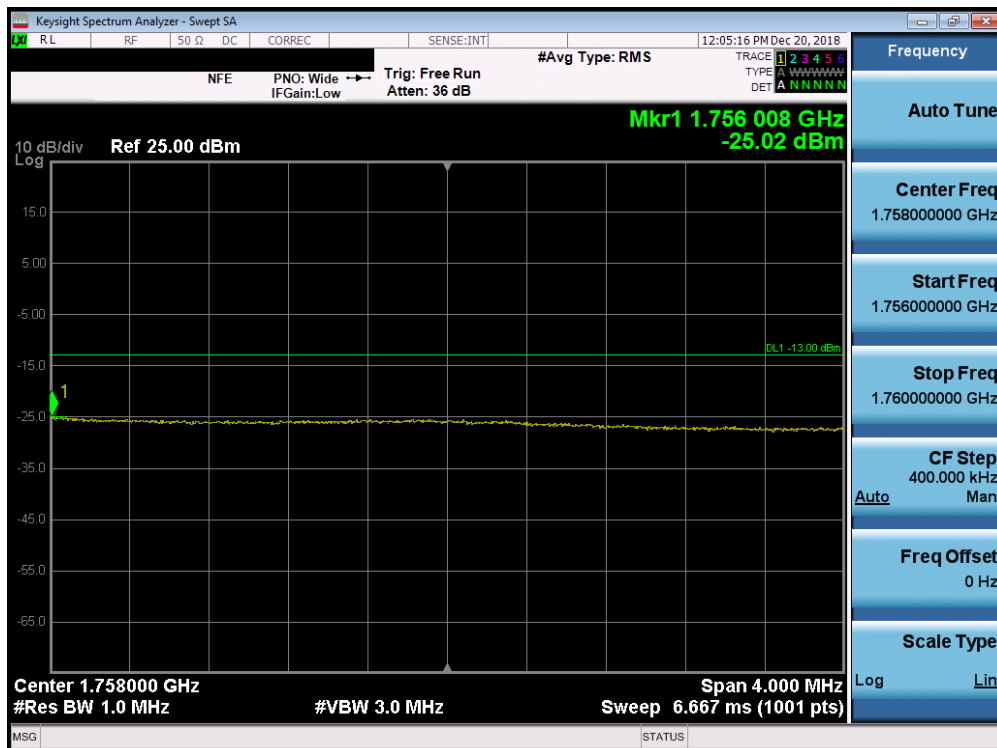
Plot 7-246. Upper Extended Band Edge Plot (Band 4 - 15.0MHz QPSK - Full RB Configuration)
