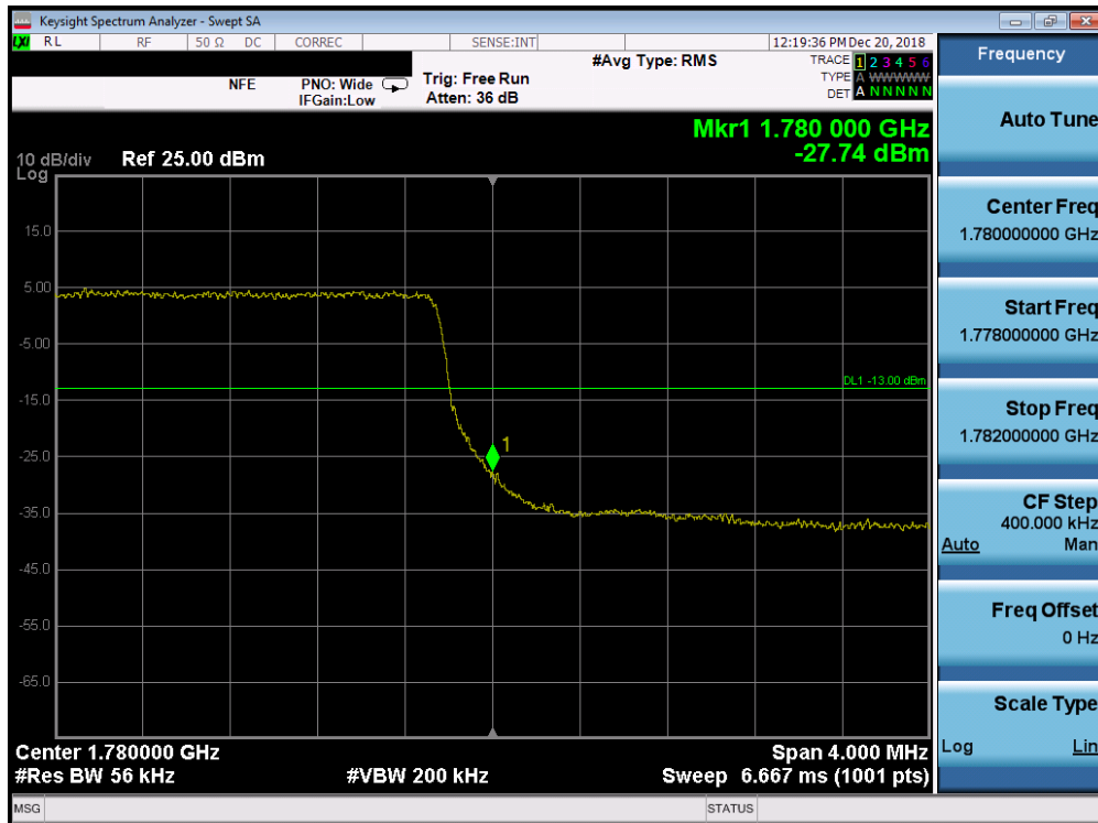
Plot 7-235. Upper Band Edge Plot (Band 66 - 5.0MHz QPSK - Full RB Configuration)
