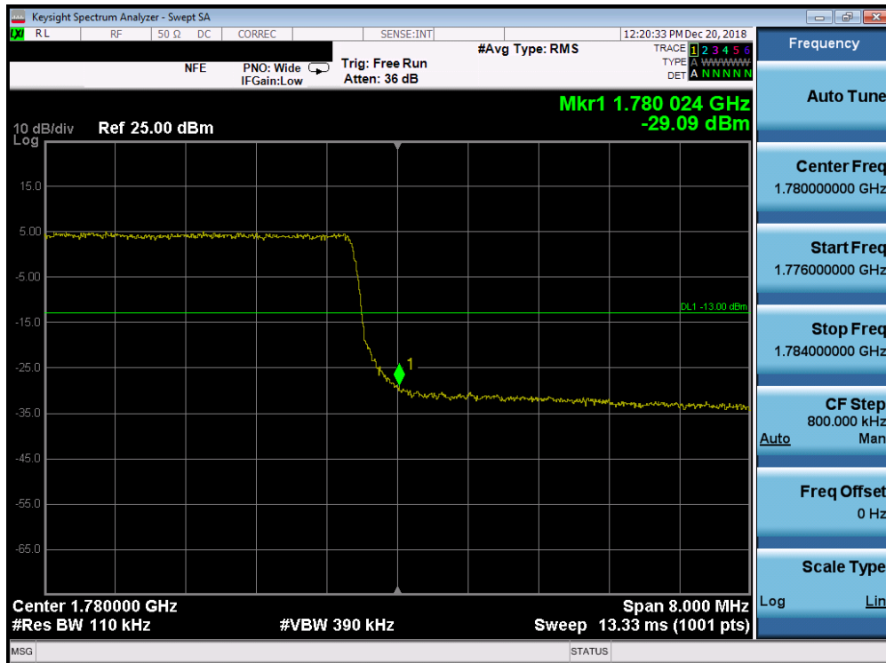
Plot 7-241. Upper Band Edge Plot (Band 66 - 10.0MHz QPSK - Full RB Configuration)
