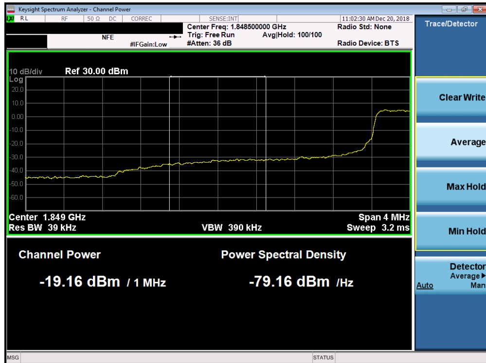
Plot 7-262. Lower Extended Band Edge Plot (Band 25/2 - 3.0MHz QPSK - Full RB Configuration)
