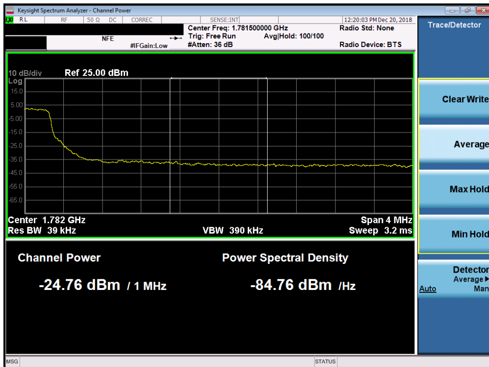
Plot 7-236. Upper Extended Band Edge Plot (Band 66 - 5.0MHz QPSK - Full RB Configuration)
