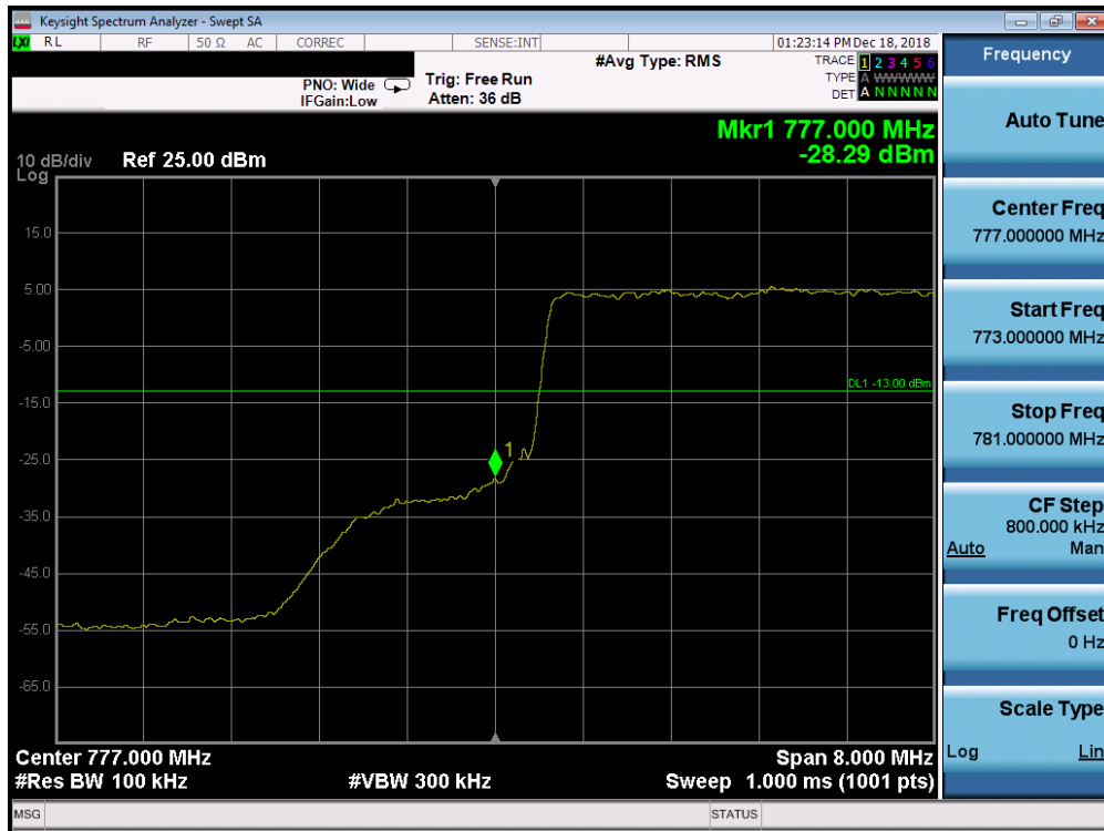
Plot 7-207. Lower Band Edge Plot (Band 13 - 10.0MHz QPSK - Full RB Configuration)
