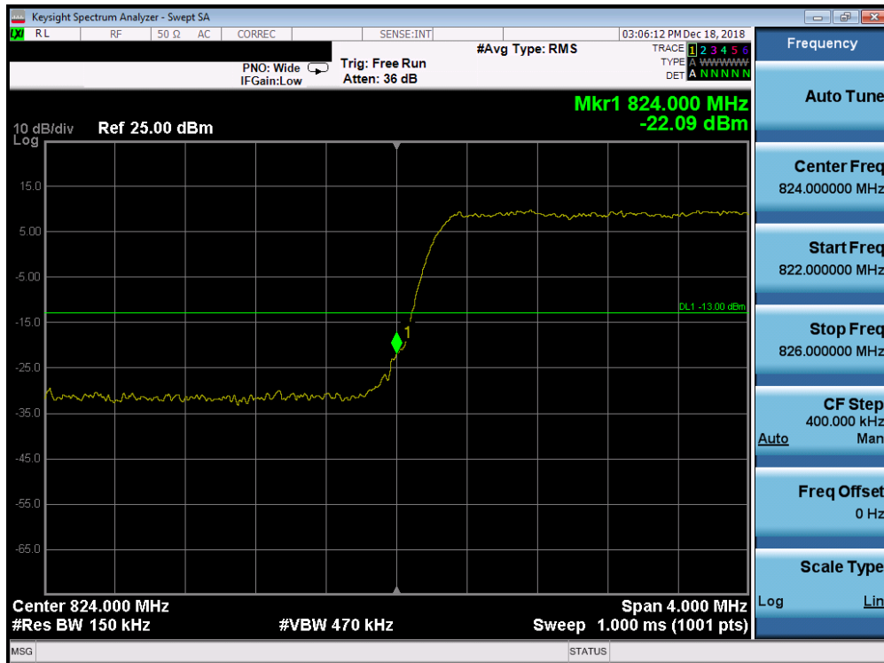
Plot 7-213. Lower Band Edge Plot (Band 26/5 - 5.0MHz QPSK - Full RB Configuration)
