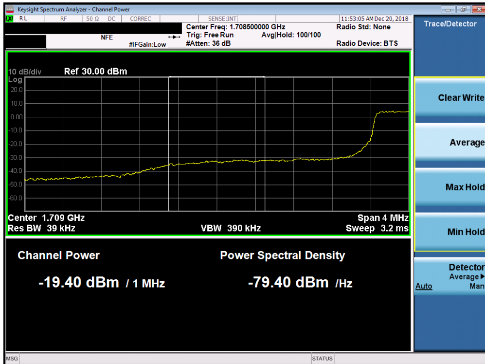
Plot 7-226. Lower Extended Band Edge Plot (Band 66/4 - 3.0MHz QPSK - Full RB Configuration)
