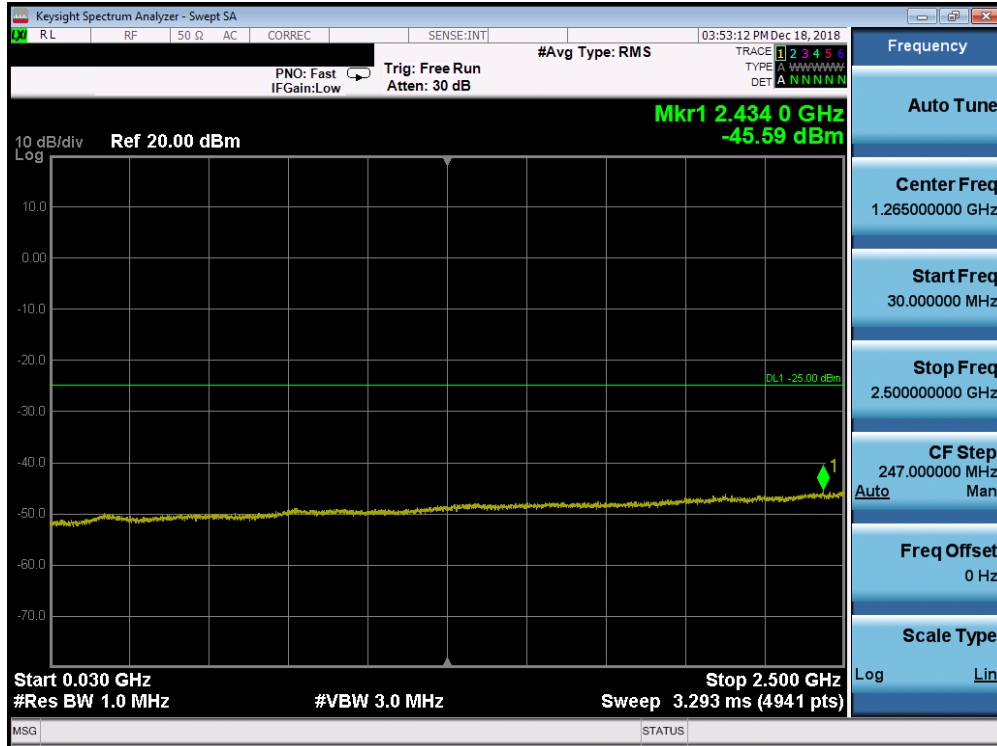
Plot 7-175. Conducted Spurious Plot (Band 7 - 20.0MHz QPSK - RB Size 1, RB Offset 0 - High Channel)
