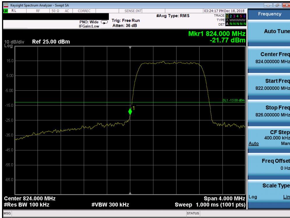
Plot 7-209. Lower Band Edge Plot (Band 26/5 - 1.4MHz QPSK - Full RB Configuration)
