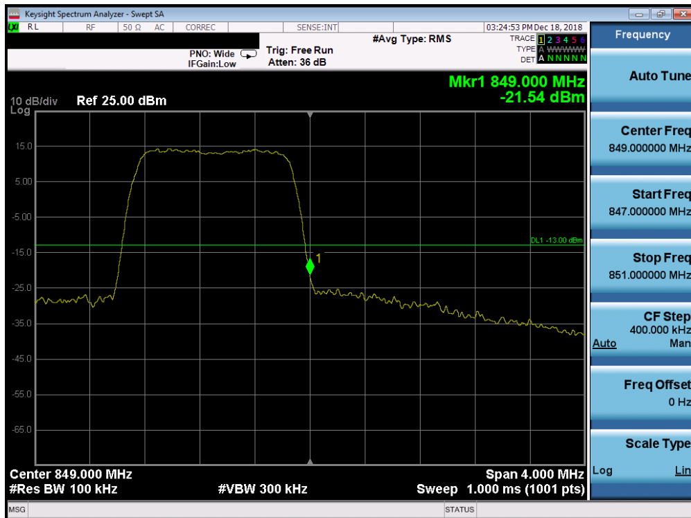
Plot 7-210. Upper Band Edge Plot (Band 26/5 - 1.4MHz QPSK - Full RB Configuration)
