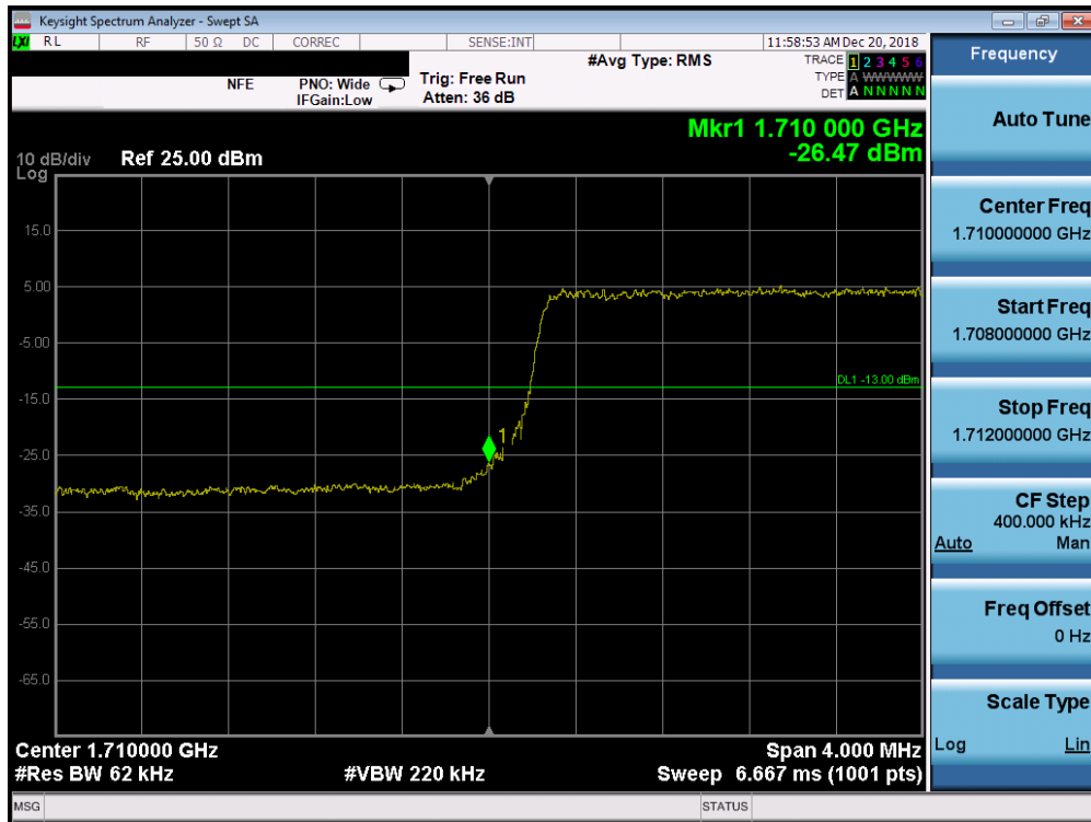
Plot 7-231. Lower Band Edge Plot (Band 66/4 - 5.0MHz QPSK - Full RB Configuration)
