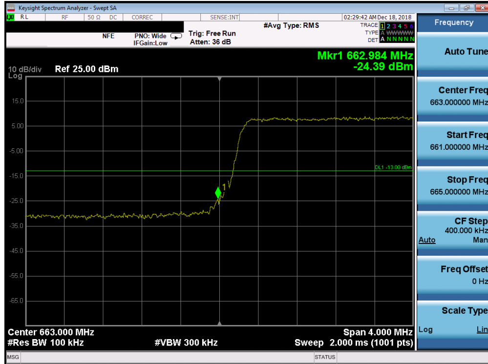
Plot 7-187. Lower Band Edge Plot (Band 71 - 5.0MHz QPSK - Full RB Configuration)
