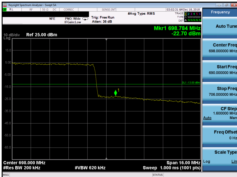
Plot 7-194. Upper Band Edge Plot (Band 71 - 20.0MHz QPSK - Full RB Configuration)
