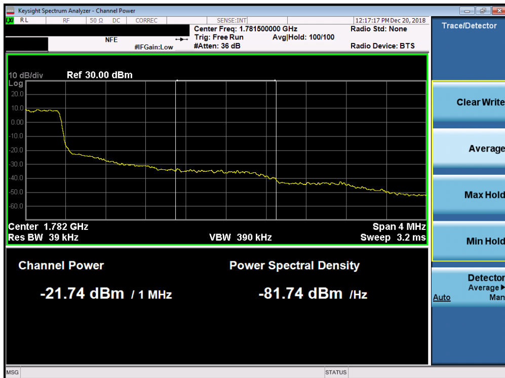
Plot 7-224. Upper Extended Band Edge Plot (Band 66 - 1.4MHz QPSK - Full RB Configuration)
