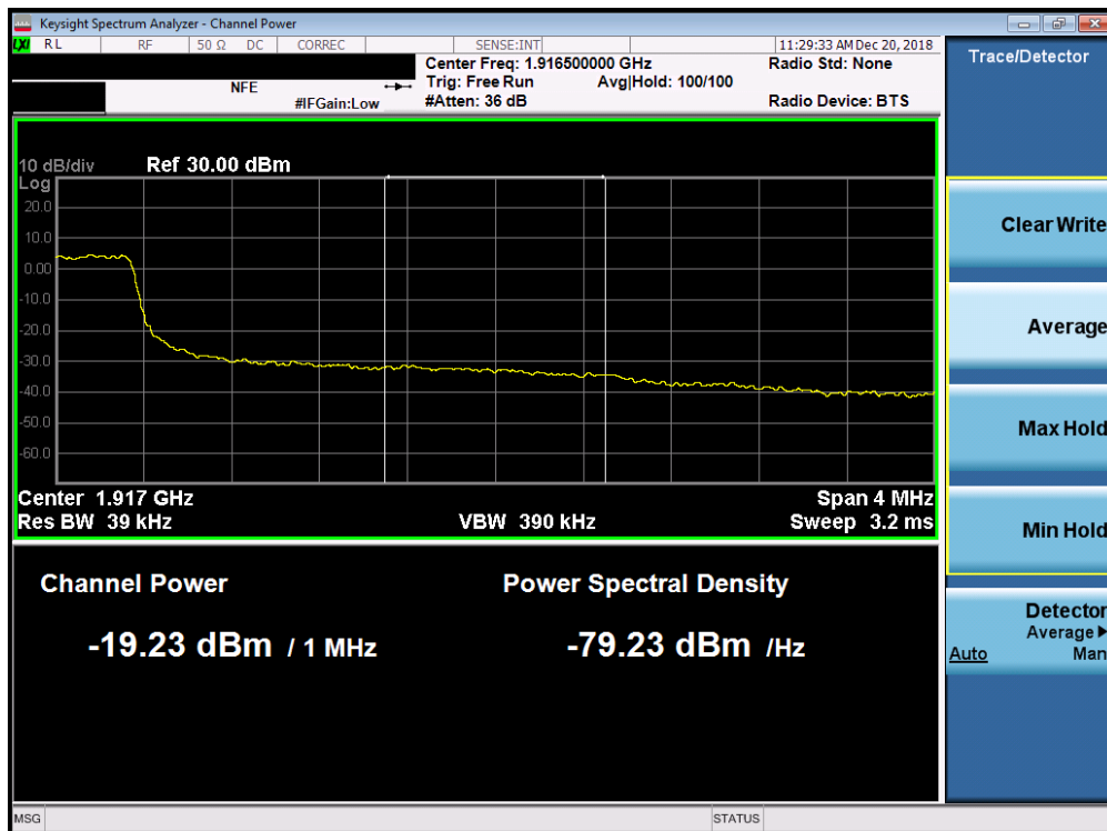
Plot 7-266. Upper Extended Band Edge Plot (Band 25 - 3.0MHz QPSK - Full RB Configuration)
