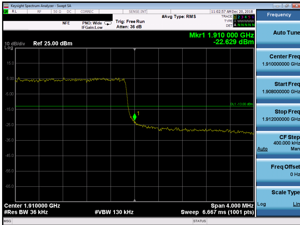
Plot 7-263. Upper Band Edge Plot (Band 2 - 3.0MHz QPSK - Full RB Configuration)
