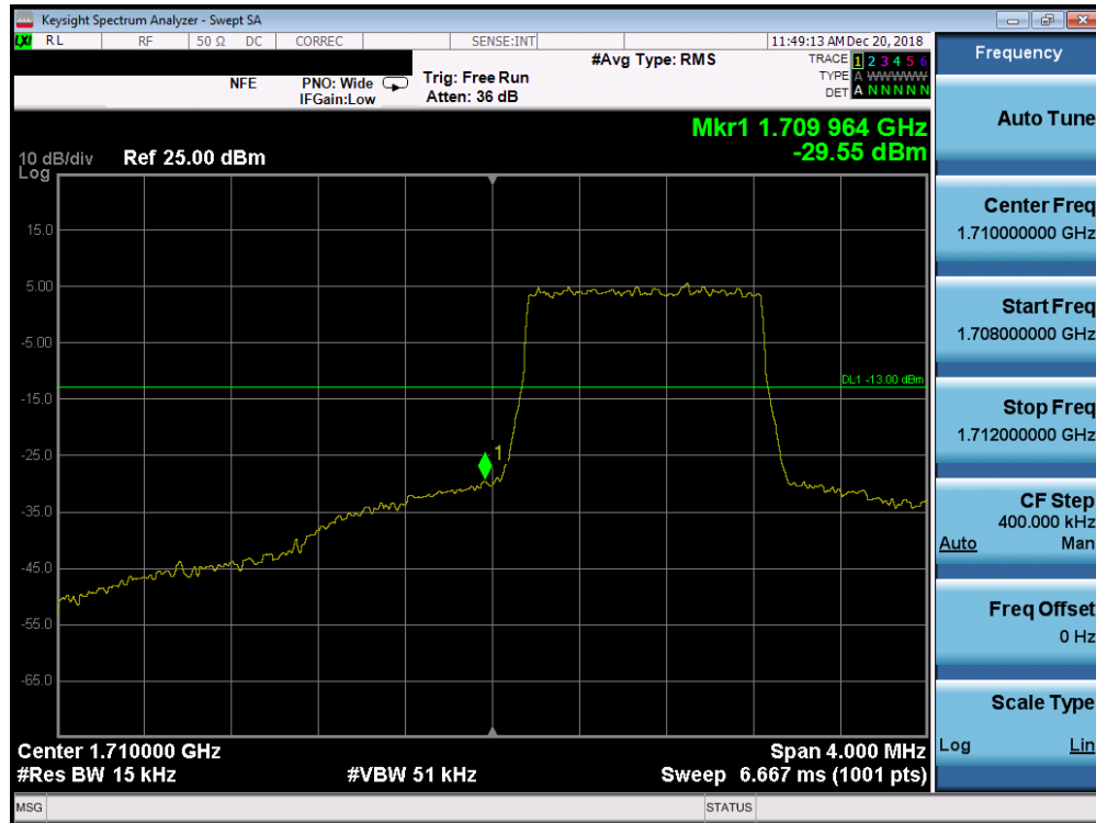
Plot 7-219. Lower Band Edge Plot (Band 66/4 - 1.4MHz QPSK - Full RB Configuration)
