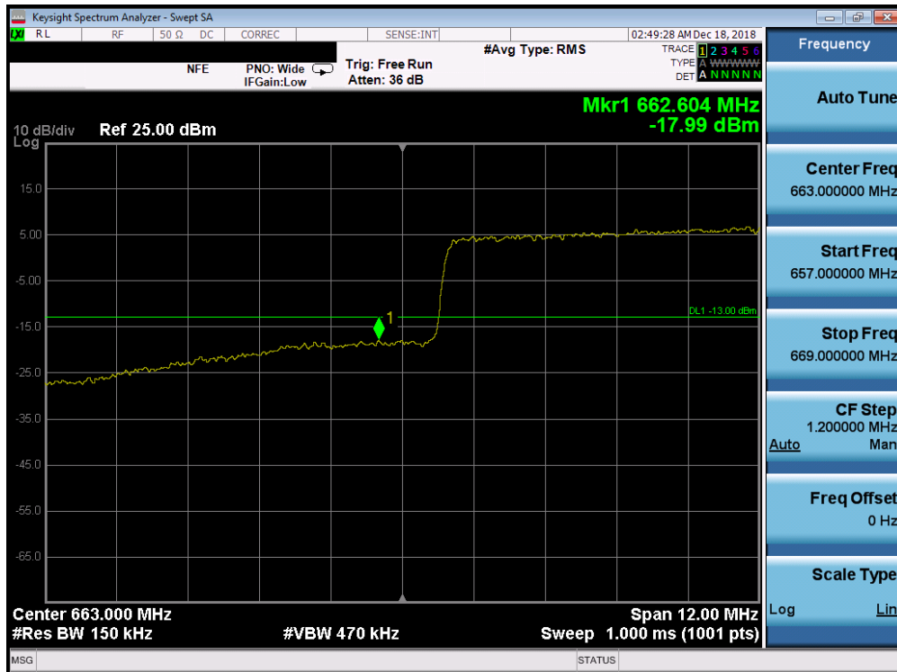
Plot 7-191. Lower Band Edge Plot (Band 71 - 15.0MHz QPSK - Full RB Configuration)
