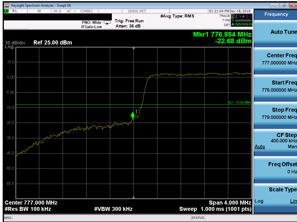
Plot 7-205. Lower Band Edge Plot (Band 13 - 5.0MHz QPSK - Full RB Configuration)
