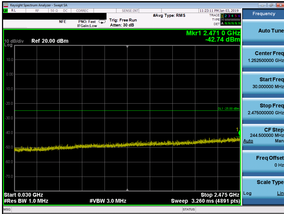
Plot 7-178. Conducted Spurious Plot (Band 41 PC - 20.0MHz QPSK - RB Size 1, RB Offset 0 - Low Channel)
