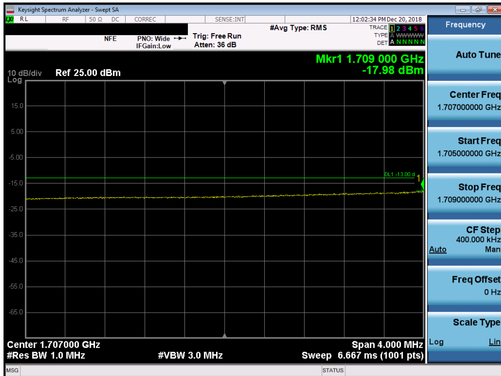
Plot 7-238. Lower Extended Band Edge Plot (Band 66/4 - 10.0MHz QPSK - Full RB Configuration)
