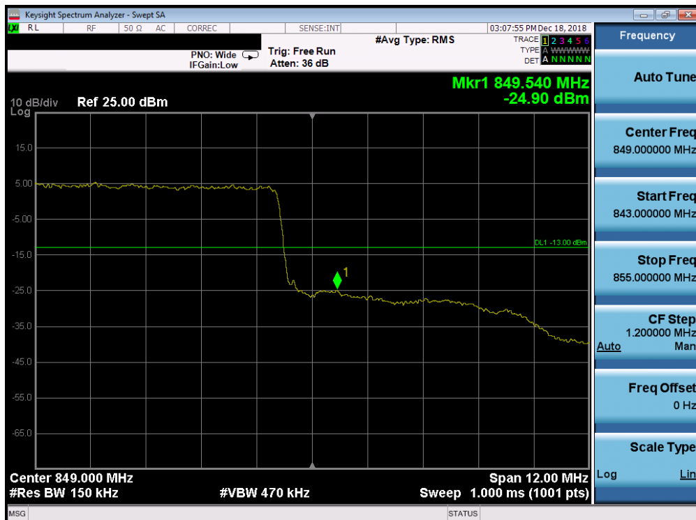
Plot 7-218. Upper Band Edge Plot (Band 26 - 15.0MHz QPSK - Full RB Configuration)
