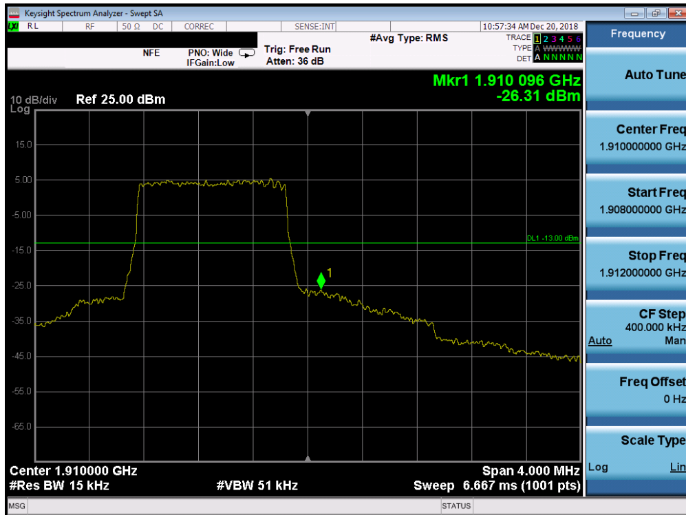
Plot 7-257. Upper Band Edge Plot (Band 2 - 1.4MHz QPSK - Full RB Configuration)
