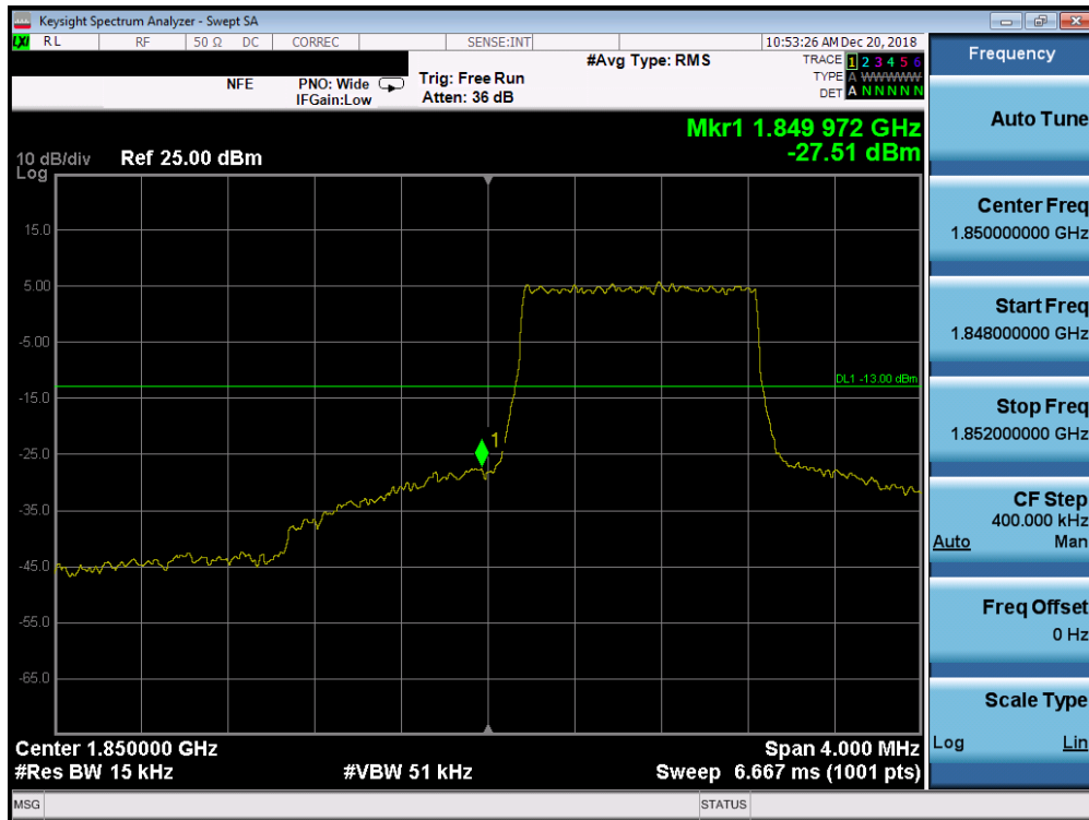
Plot 7-255. Lower Band Edge Plot (Band 25/2 - 1.4MHz QPSK - Full RB Configuration)
