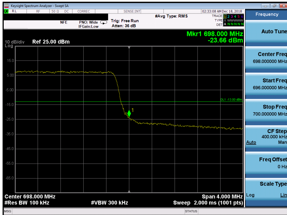
Plot 7-188. Upper Band Edge Plot (Band 71 - 5.0MHz QPSK - Full RB Configuration)
