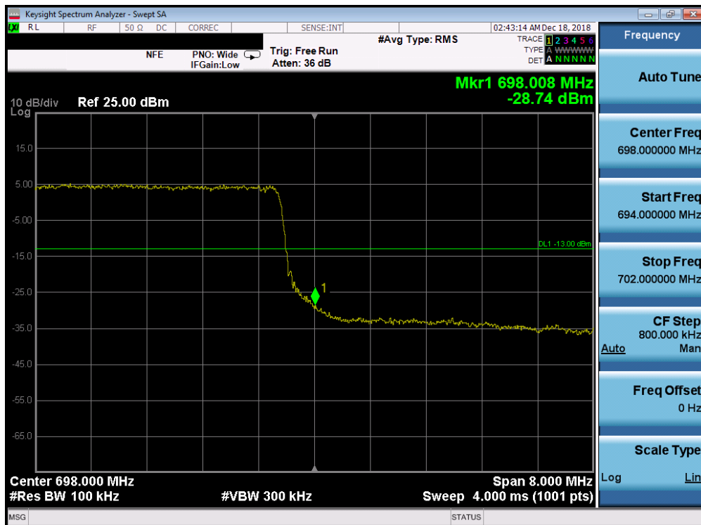
Plot 7-190. Upper Band Edge Plot (Band 71 - 10.0MHz QPSK - Full RB Configuration)
