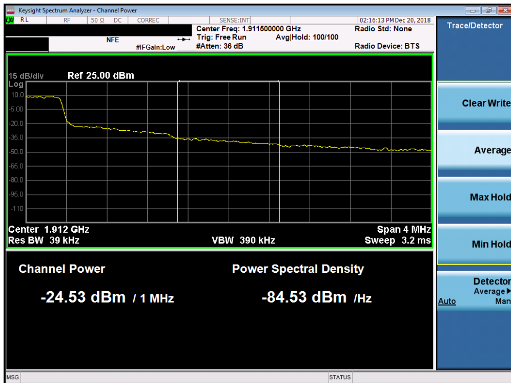
Plot 7-258. Upper Extended Band Edge Plot (Band 2 - 1.4MHz QPSK - Full RB Configuration)
