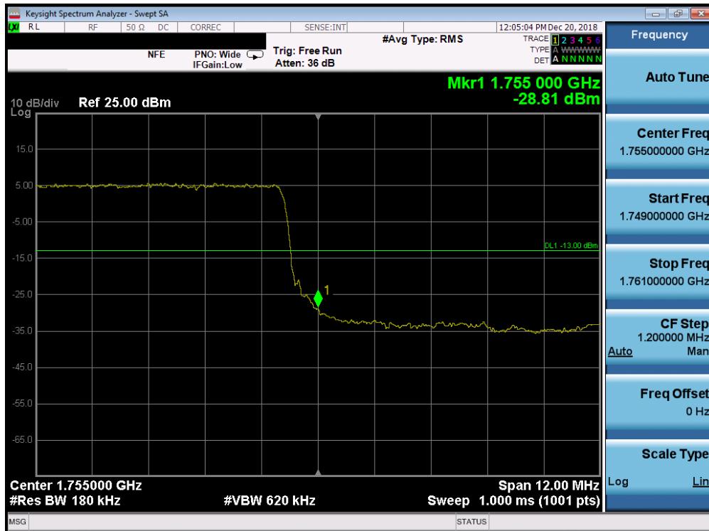
Plot 7-245. Upper Band Edge Plot (Band 4 - 15.0MHz QPSK - Full RB Configuration)
