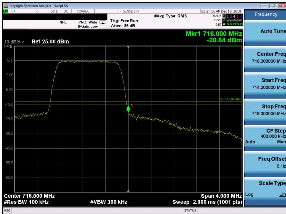
Plot 7-196. Upper Band Edge Plot (Band 12 - 1.4MHz QPSK - Full RB Configuration)
