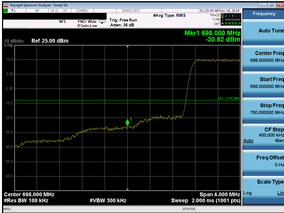
Plot 7-195. Lower Band Edge Plot (Band 12 - 1.4MHz QPSK - Full RB Configuration)
