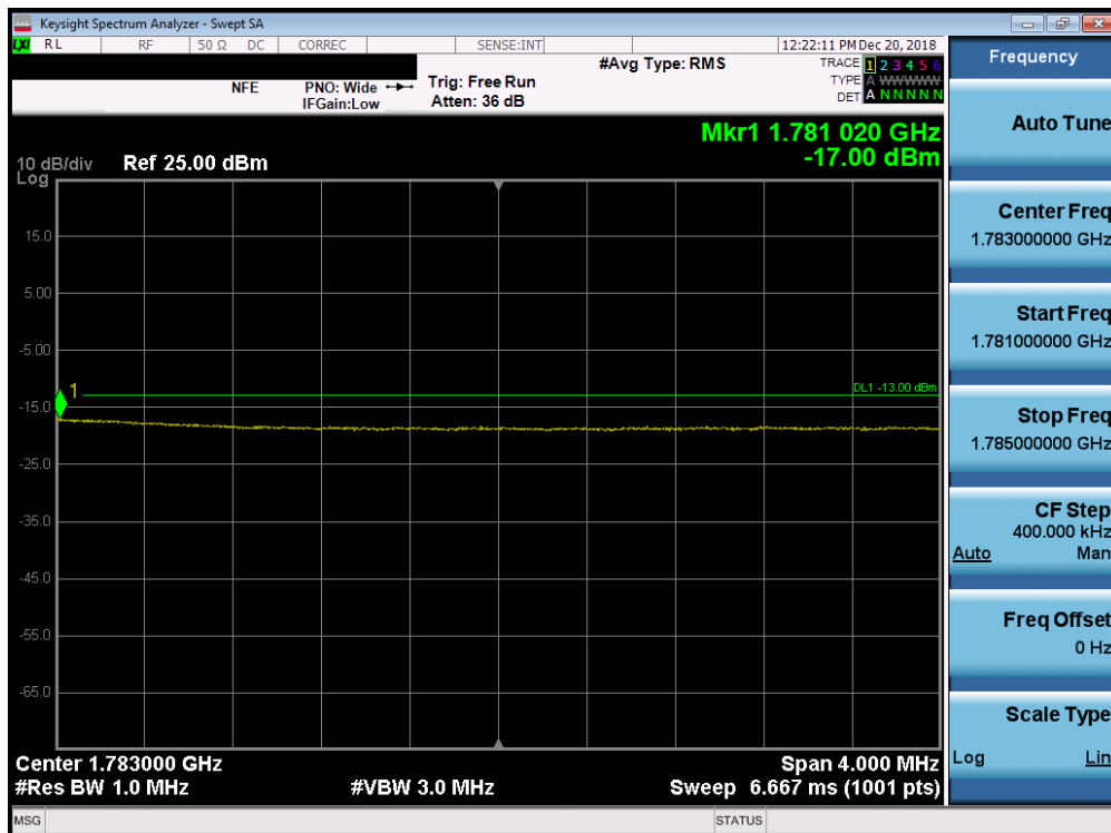
Plot 7-254. Upper Extended Band Edge Plot (Band 66 - 20.0MHz QPSK - Full RB Configuration)
