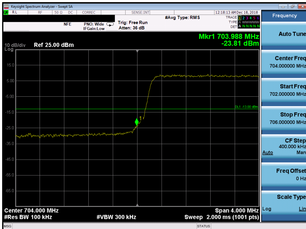
Plot 7-200. Lower Band Edge Plot (Band 17 - 5.0MHz QPSK - Full RB Configuration)
