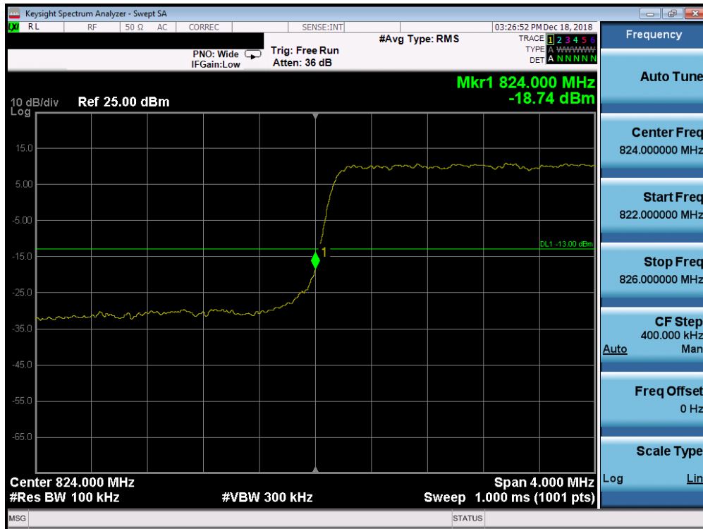
Plot 7-211. Lower Band Edge Plot (Band 26/5 - 3.0MHz QPSK - Full RB Configuration)
