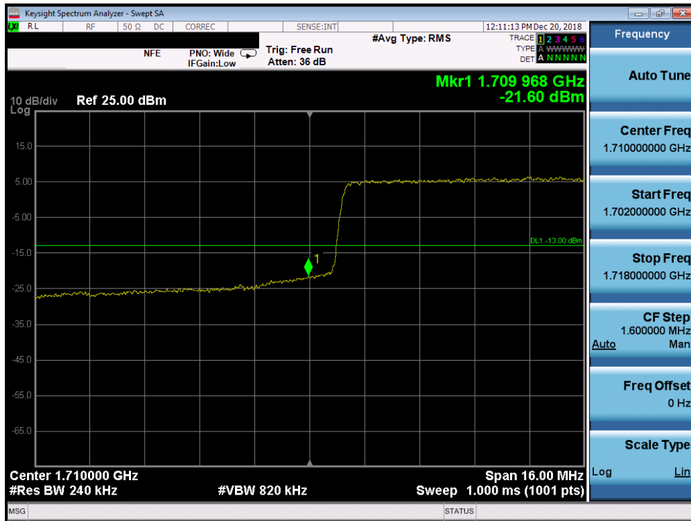
Plot 7-249. Lower Band Edge Plot (Band 66/4 - 20.0MHz QPSK - Full RB Configuration)
