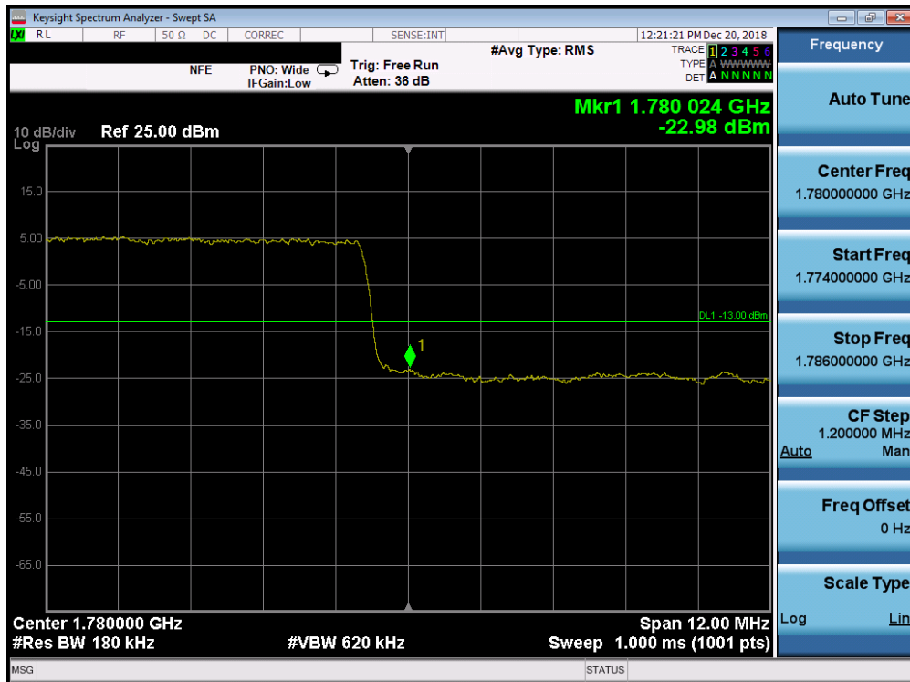
Plot 7-247. Upper Band Edge Plot (Band 66 - 15.0MHz QPSK - Full RB Configuration)
