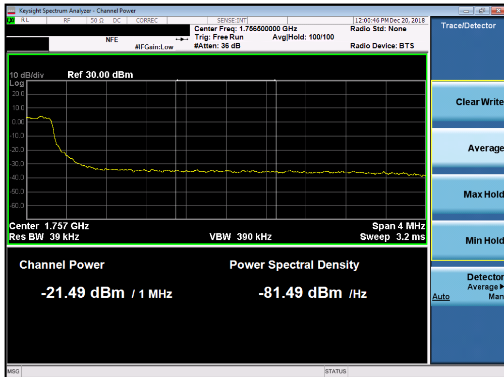
Plot 7-234. Upper Extended Band Edge Plot (Band 4 - 5.0MHz QPSK - Full RB Configuration)
