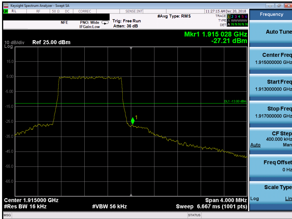
Plot 7-259. Upper Band Edge Plot (Band 25 - 1.4MHz QPSK - Full RB Configuration)
