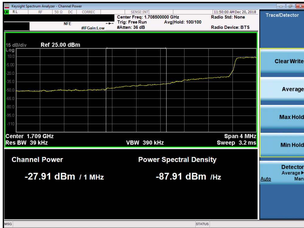
Plot 7-220. Lower Extended Band Edge Plot (Band 66/4 - 1.4MHz QPSK - Full RB Configuration)
