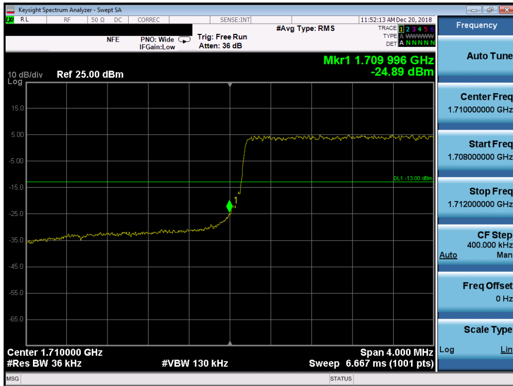
Plot 7-225. Lower Band Edge Plot (Band 66/4 - 3.0MHz QPSK - Full RB Configuration)
