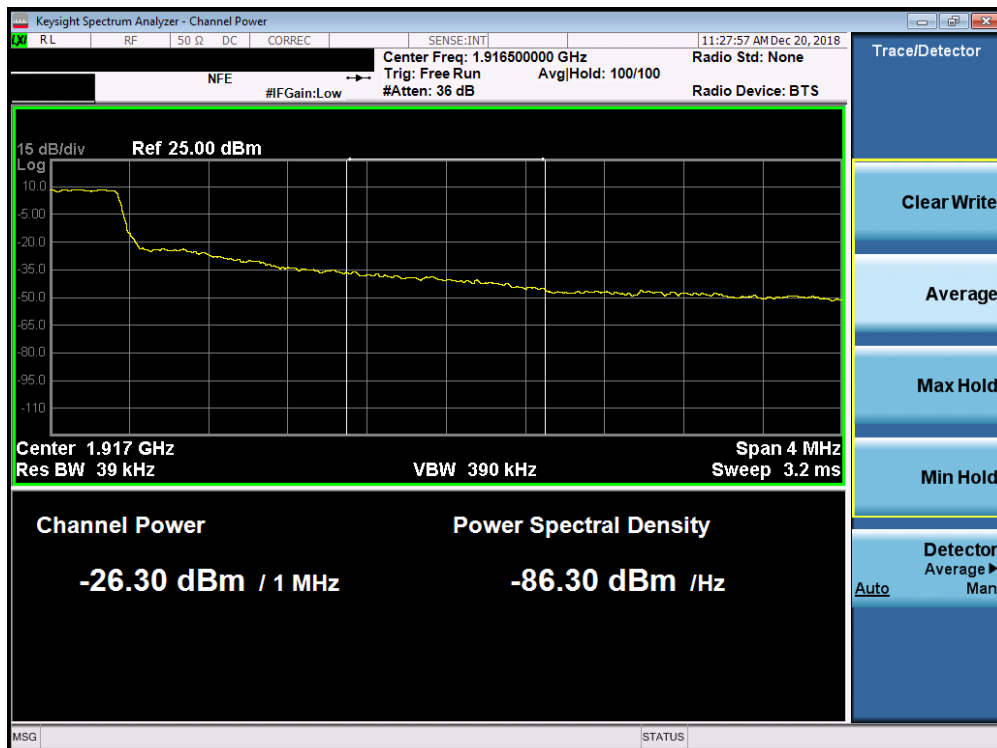
Plot 7-260. Upper Extended Band Edge Plot (Band 25 - 1.4MHz QPSK - Full RB Configuration)
