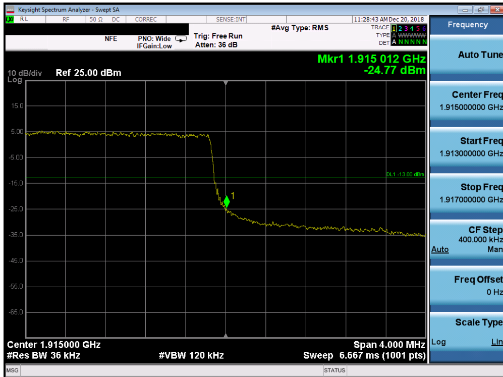
Plot 7-265. Upper Band Edge Plot (Band 25 - 3.0MHz QPSK - Full RB Configuration)
