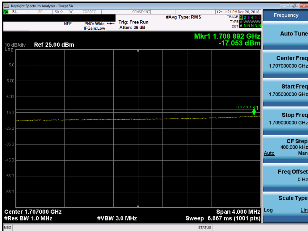
Plot 7-250. Lower Extended Band Edge Plot (Band 66/4 - 20.0MHz QPSK - Full RB Configuration)
