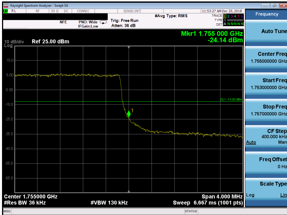
Plot 7-227. Upper Band Edge Plot (Band 4 - 3.0MHz QPSK - Full RB Configuration)
