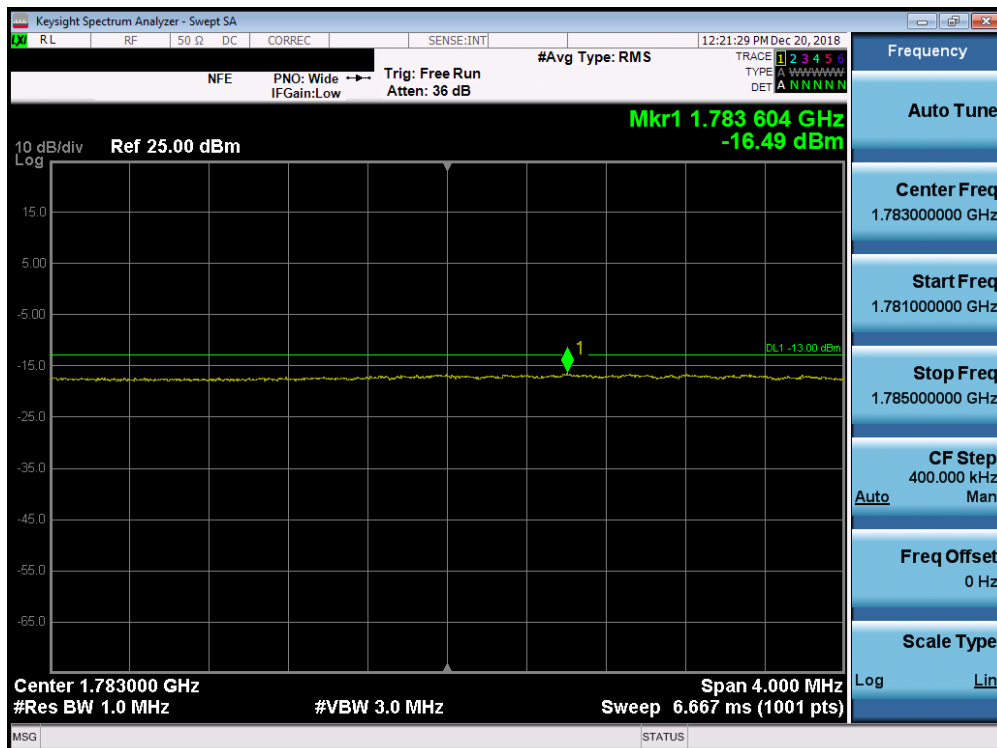
Plot 7-248. Upper Extended Band Edge Plot (Band 66 - 15.0MHz QPSK - Full RB Configuration)
