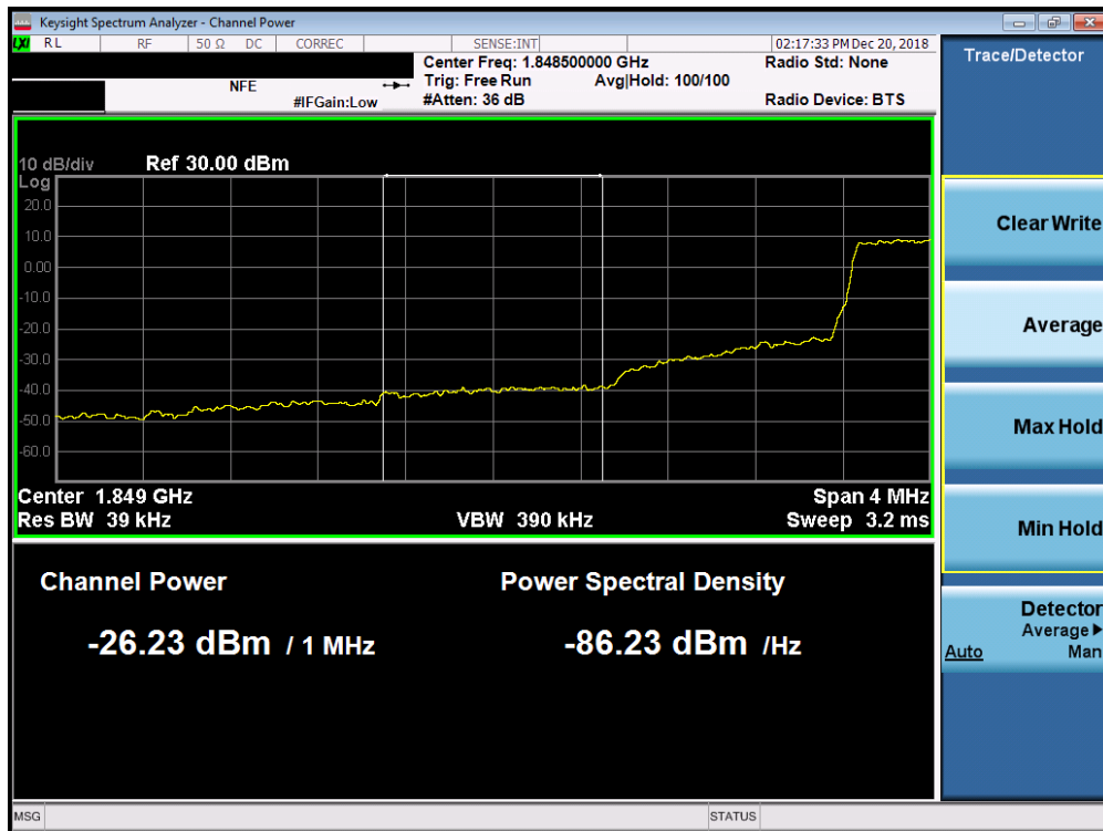
Plot 7-256. Lower Extended Band Edge Plot (Band 25/2 - 1.4MHz QPSK - Full RB Configuration)
