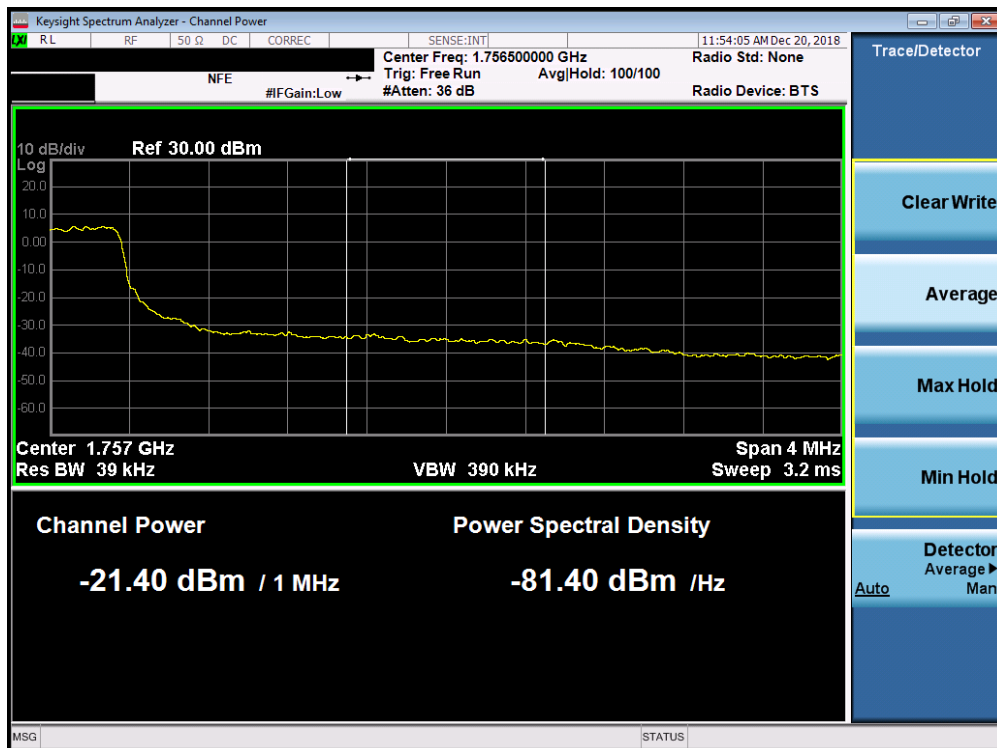
Plot 7-228. Upper Extended Band Edge Plot (Band 4 - 3.0MHz QPSK - Full RB Configuration)
