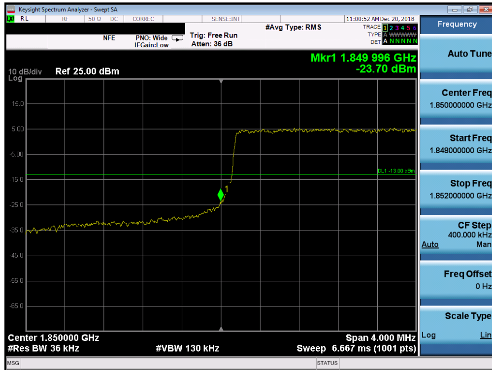
Plot 7-261. Lower Band Edge Plot (Band 25/2 - 3.0MHz QPSK - Full RB Configuration)
