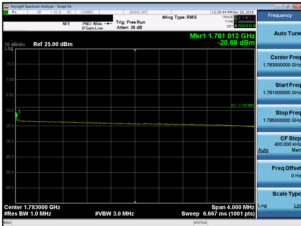
Plot 7-242. Upper Extended Band Edge Plot (Band 66 - 10.0MHz QPSK - Full RB Configuration)
