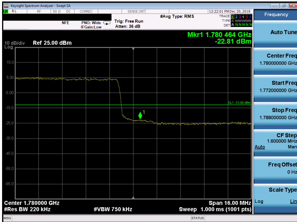
Plot 7-253. Upper Band Edge Plot (Band 66 - 20.0MHz QPSK - Full RB Configuration)
