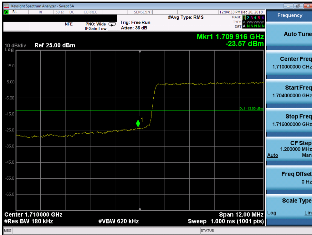
Plot 7-243. Lower Band Edge Plot (Band 66/4 - 15.0MHz QPSK - Full RB Configuration)
