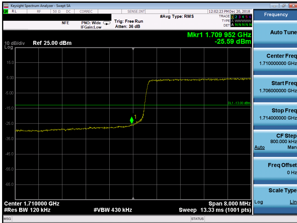
Plot 7-237. Lower Band Edge Plot (Band 66/4 - 10.0MHz QPSK - Full RB Configuration)
