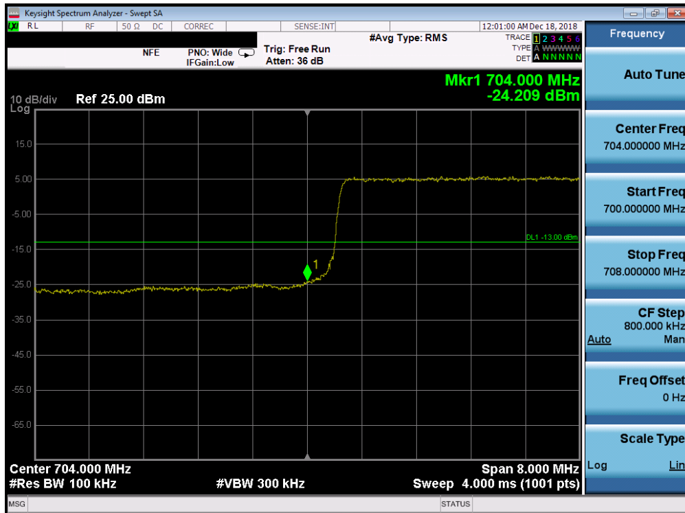
Plot 7-203. Lower Band Edge Plot (Band 17 - 10.0MHz QPSK - Full RB Configuration)
