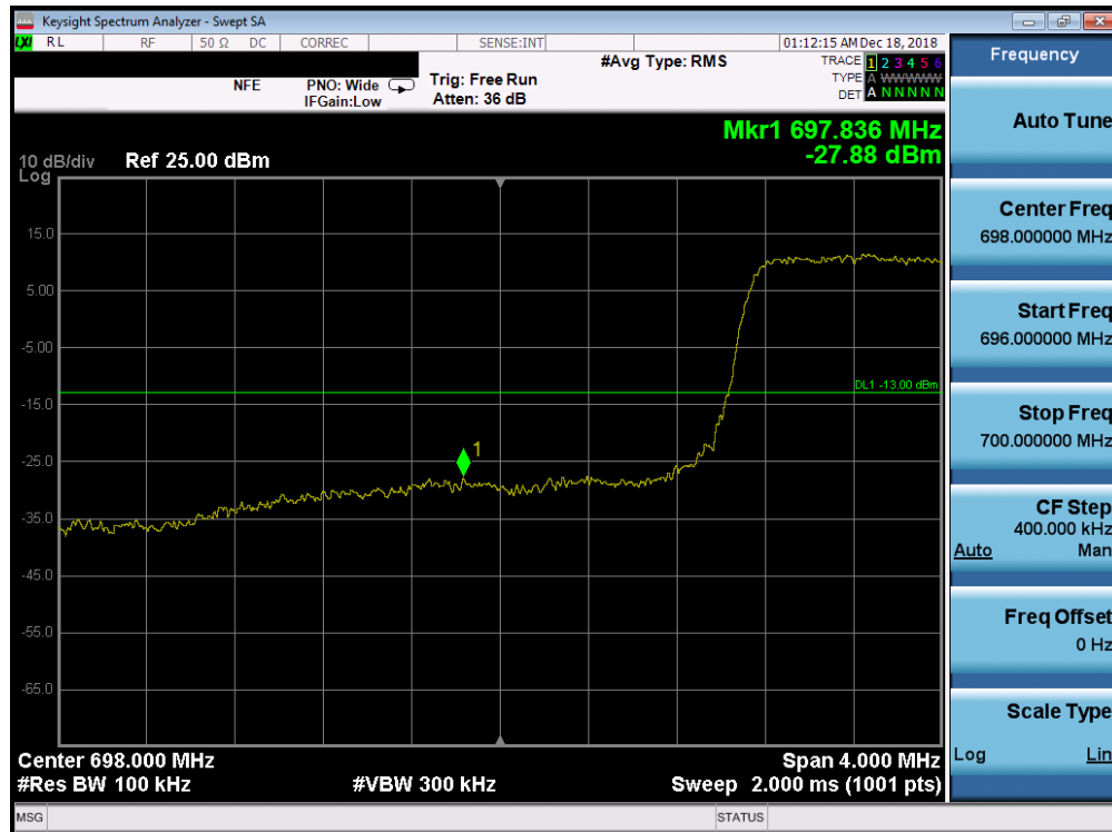
Plot 7-197. Lower Band Edge Plot (Band 12 - 3.0MHz QPSK - Full RB Configuration)
