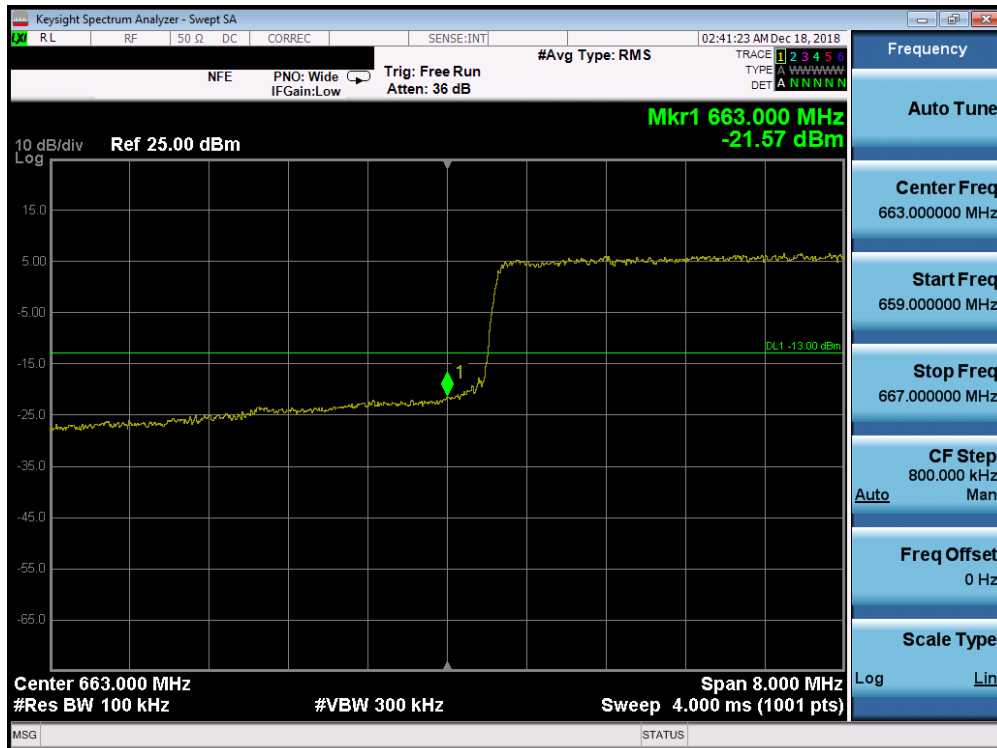
Plot 7-189. Lower Band Edge Plot (Band 71 - 10.0MHz QPSK - Full RB Configuration)
