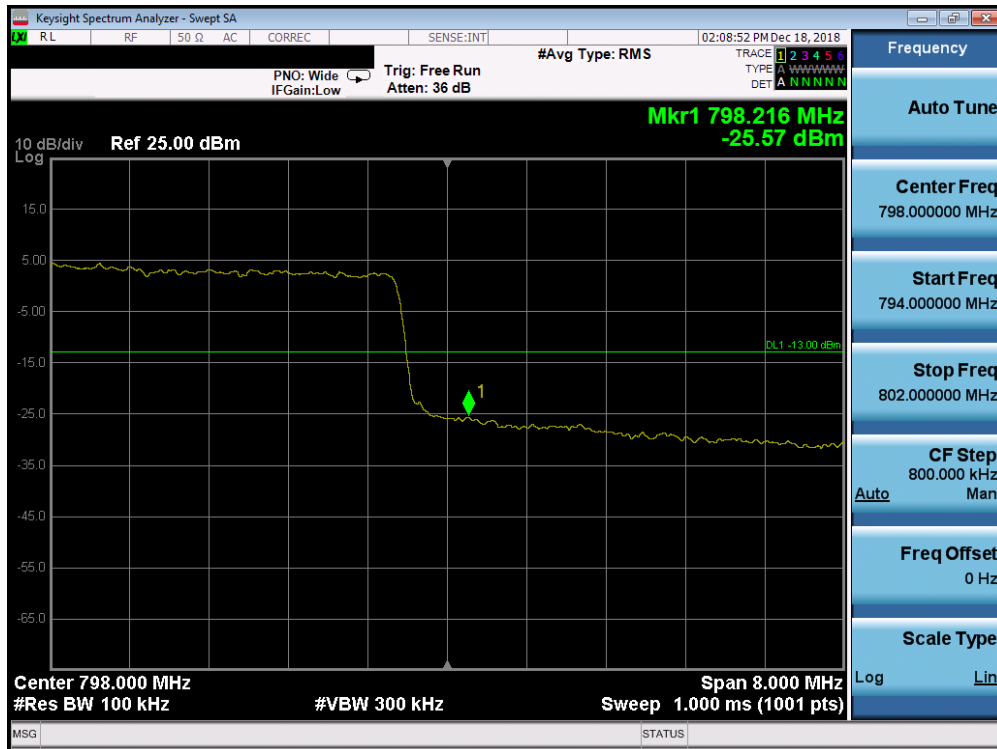
Plot 7-52. Upper Band Edge Plot (LTE Band 14, 10MHz QPSK – RB Size 50)
