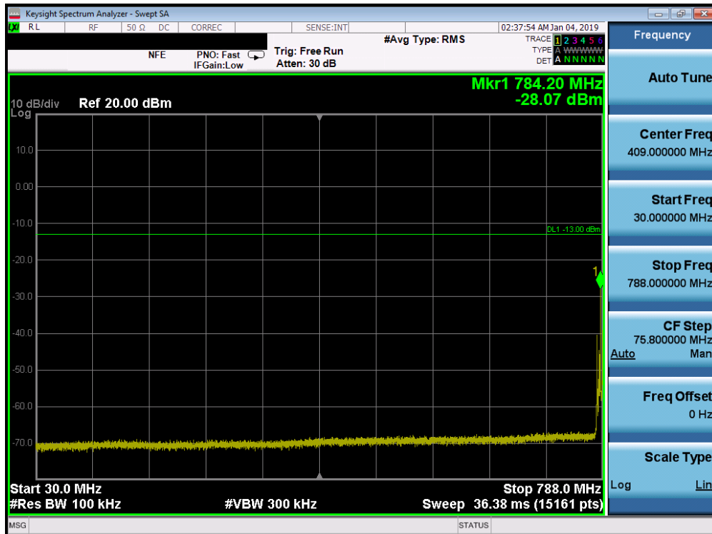
Plot 7-33. Conducted Spurious Plot (LTE Band 14, 10 MHz QPSK – RB Size 1, RB Offset 0)
