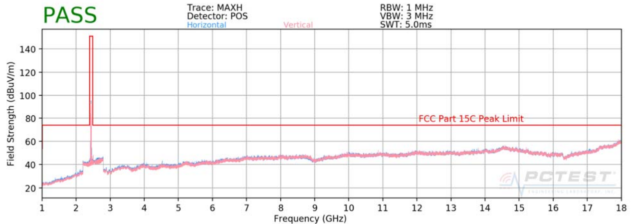
Plot 7-6. Radiated Spurious Plot above 1GHz SISO ANT2 (802.11b – Ch. 6)
