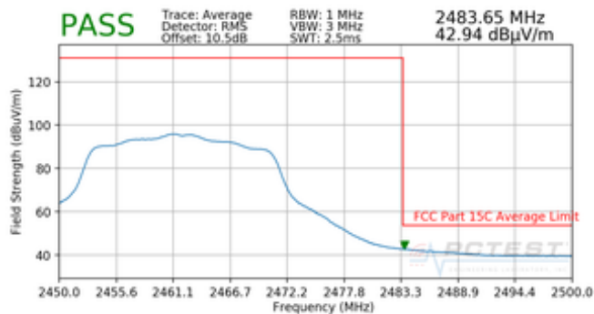
Plot 7-17. Radiated Restricted Upper Band Edge Measurement SISO ANT2 (Average)
