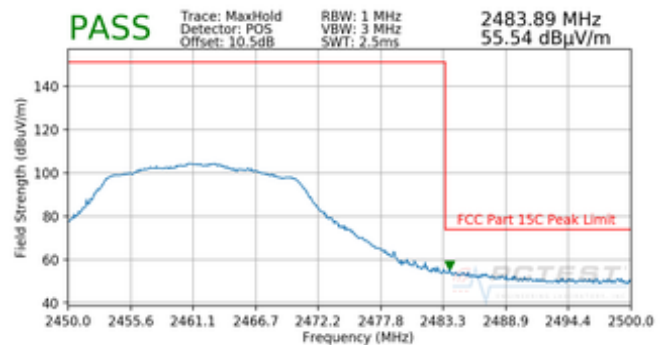
Plot 7-18. Radiated Restricted Upper Band Edge Measurement SISO ANT2 (Peak)
