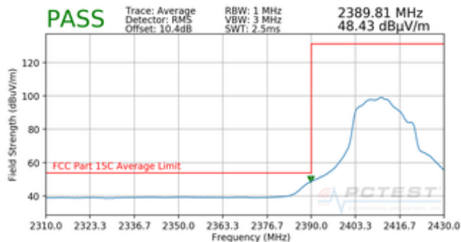
Plot 7-21. Radiated Restricted Lower Band Edge Measurement MIMO (Average)
