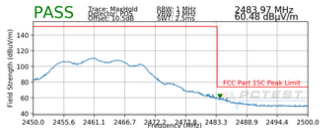
Plot 7-30. Radiated Restricted Upper Band Edge Measurement MIMO (Peak)
