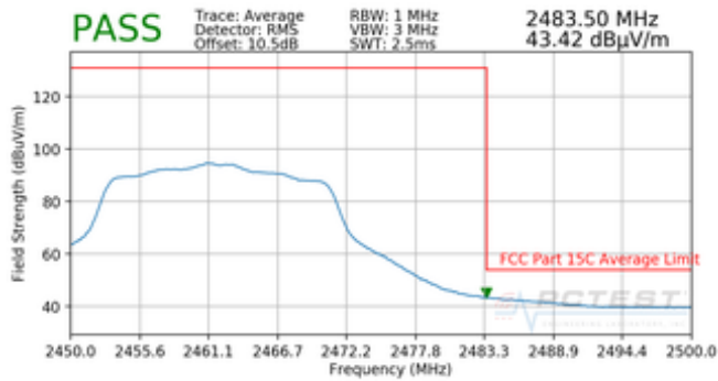
Plot 7-19. Radiated Restricted Band Edge Measurement SISO ANT2 with WCP (Average)
