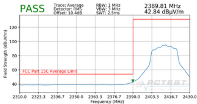
Plot 7-15. Radiated Restricted Lower Band Edge Measurement SISO ANT2 (Average)
