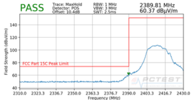
Plot 7-22. Radiated Restricted Lower Band Edge Measurement MIMO (Peak)
