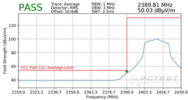
Plot 7-13. Radiated Restricted Band Edge Measurement SISO ANT1 with WCP (Average)
