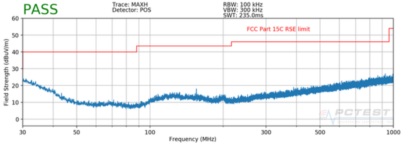
Plot 7-34. Radiated Spurious Plot below 1GHz SISO ANT2
