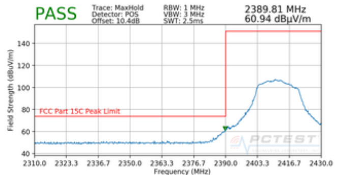
Plot 7-10. Radiated Restricted Lower Band Edge Measurement SISO ANT1 (Peak)
