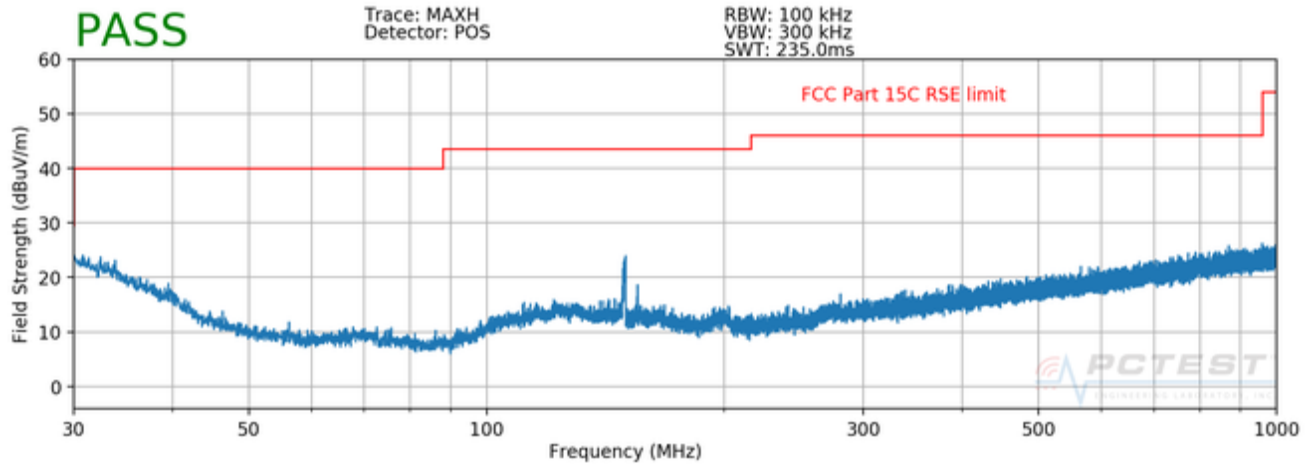
Plot 7-33. Radiated Spurious Plot below 1GHz SISO ANT1
