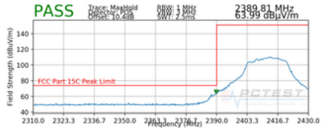
Plot 7-26. Radiated Restricted Band Edge Measurement MIMO with WCP (Peak)
