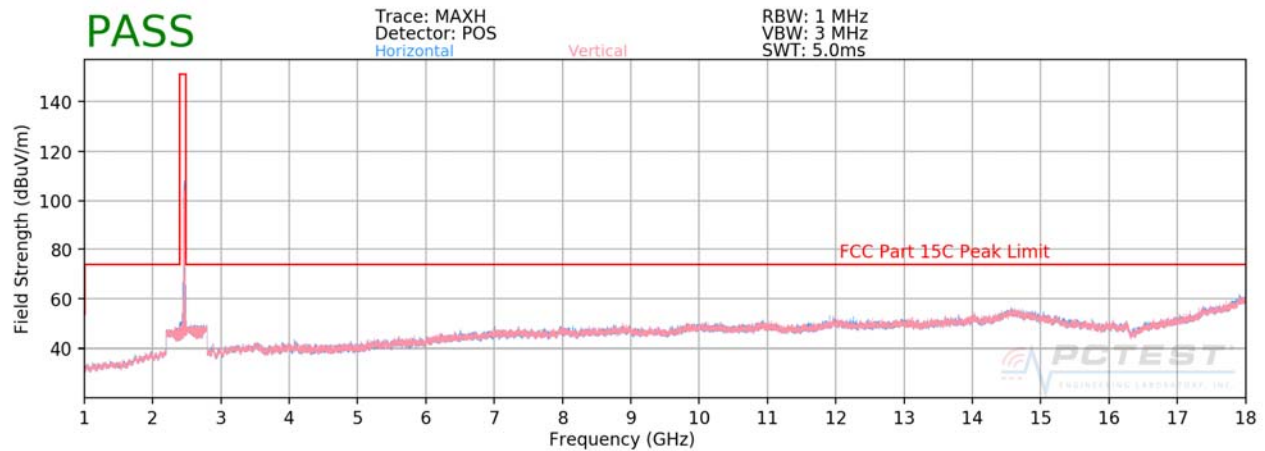
Plot 7-3. Radiated Spurious Plot above 1GHz SISO ANT1 (802.11b – Ch. 11)
