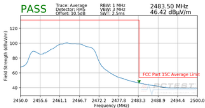
Plot 7-23. Radiated Restricted Upper Band Edge Measurement MIMO (Average)
