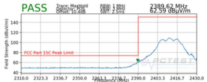
Plot 7-28. Radiated Restricted Lower Band Edge Measurement MIMO (Peak)
