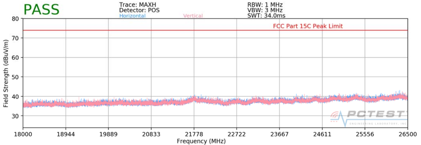
Plot 7-8. Radiated Spurious Plot above 18GHz SISO ANT2
