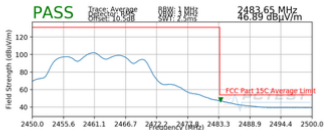
Plot 7-29. Radiated Restricted Upper Band Edge Measurement MIMO (Average)
