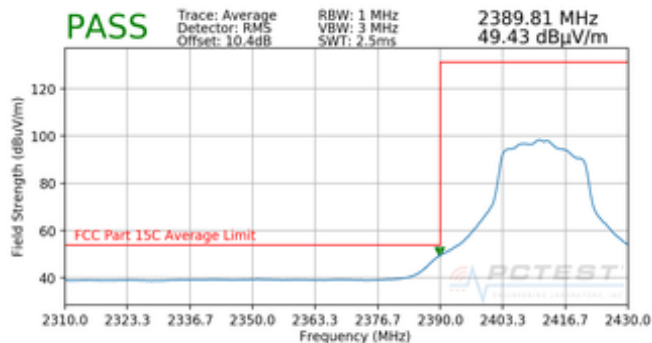
Plot 7-9. Radiated Restricted Lower Band Edge Measurement SISO ANT1 (Average)
