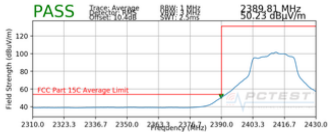
Plot 7-25. Radiated Restricted Band Edge Measurement MIMO with WCP (Average)
