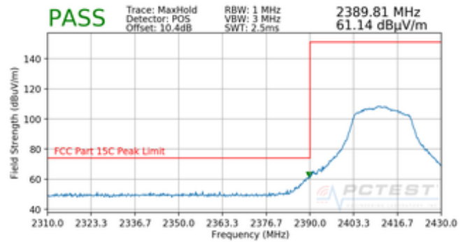
Plot 7-14. Radiated Restricted Band Edge Measurement SISO ANT1 with WCP (Peak)
