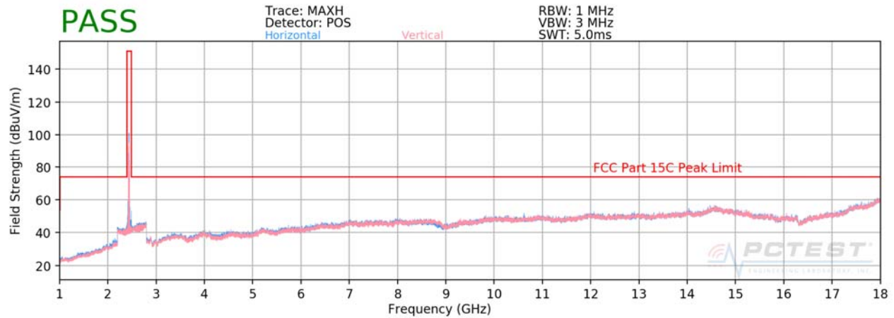
Plot 7-2. Radiated Spurious Plot above 1GHz SISO ANT1 (802.11b – Ch. 6)
