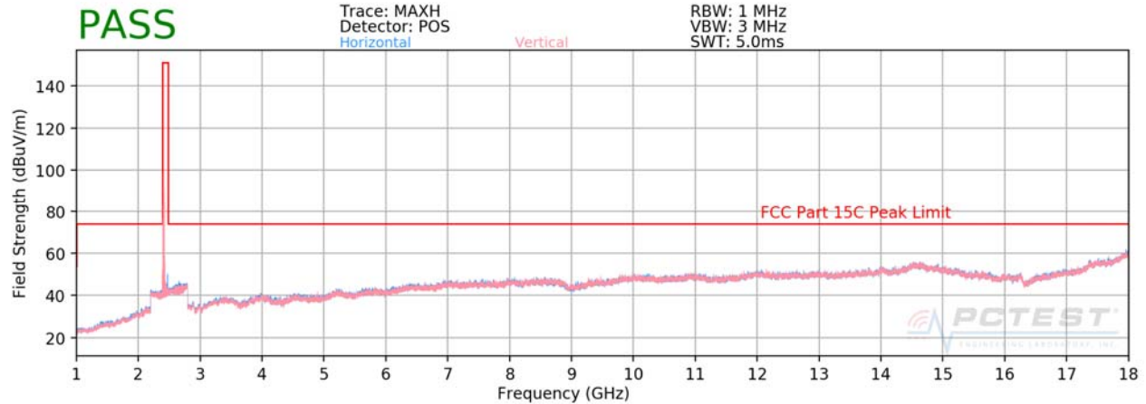
Plot 7-5. Radiated Spurious Plot above 1GHz SISO ANT2 (802.11b – Ch. 1)
