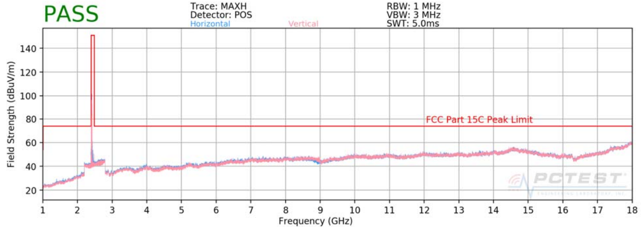
Plot 7-1. Radiated Spurious Plot above 1GHz SISO ANT1 (802.11b – Ch. 1)
