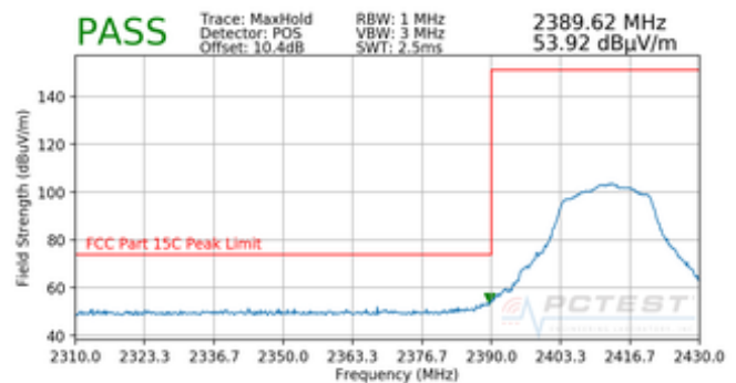
Plot 7-16. Radiated Restricted Lower Band Edge Measurement SISO ANT2 (Peak)
