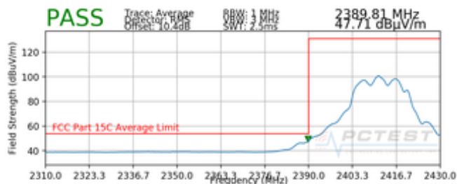
Plot 7-27. Radiated Restricted Lower Band Edge Measurement MIMO (Average)
