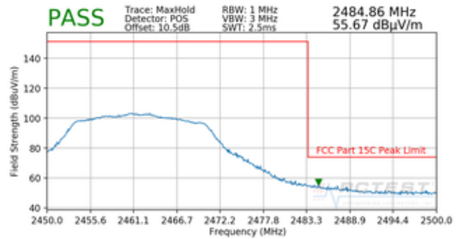
Plot 7-20. Radiated Restricted Band Edge Measurement SISO ANT2 with WCP (Peak)
