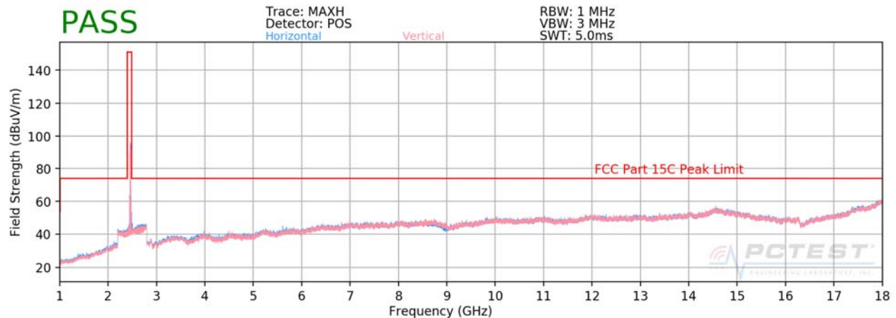
Plot 7-7. Radiated Spurious Plot above 1GHz SISO ANT2 (802.11b – Ch. 11)
