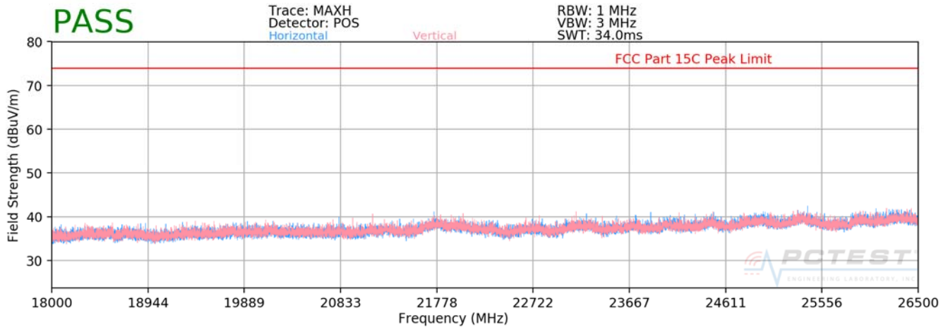
Plot 7-4. Radiated Spurious Plot above 18GHz SISO ANT1
