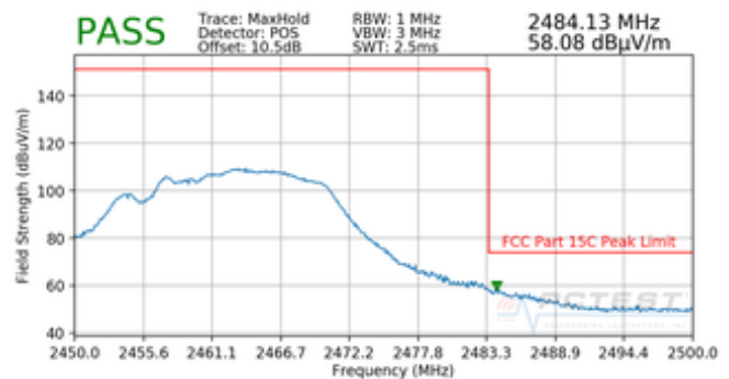
Plot 7-24. Radiated Restricted Upper Band Edge Measurement MIMO (Peak)
