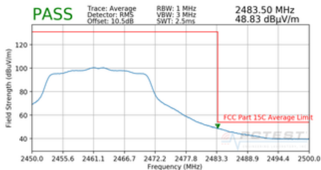
Plot 7-11. Radiated Restricted Upper Band Edge Measurement SISO ANT1 (Average)
