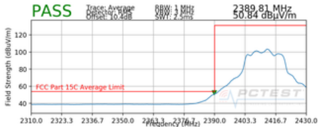
Plot 7-31. Radiated Restricted Band Edge Measurement MIMO with WCP (Average)
