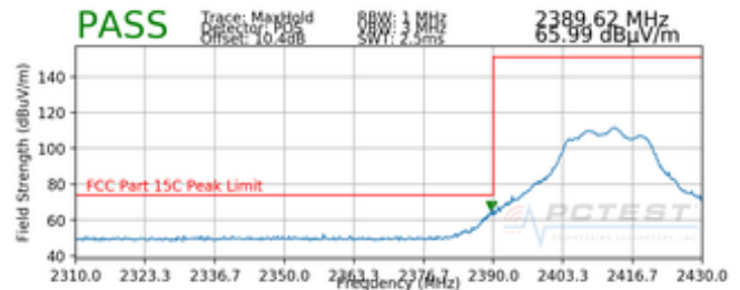
Plot 7-32. Radiated Restricted Band Edge Measurement MIMO with WCP (Peak)
