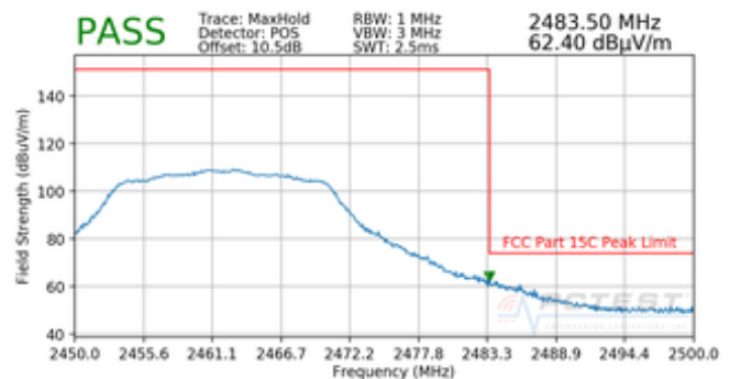
Plot 7-12. Radiated Restricted Upper Band Edge Measurement SISO ANT1 (Peak)
