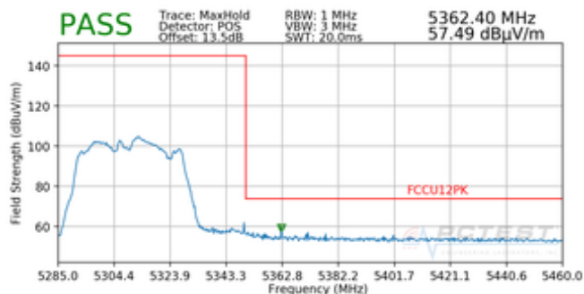
Plot 7-87. Radiated Band Edge Plot ANT (Peak – WCP)
