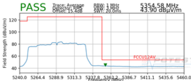
Plot 7-36. Radiated Upper Band Edge Plot SISO ANT1 (Average – UNII Band 2A)
