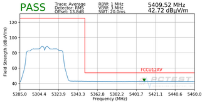
Plot 7-32. Radiated Band Edge Plot SISO ANT1 (Average – WCP)
