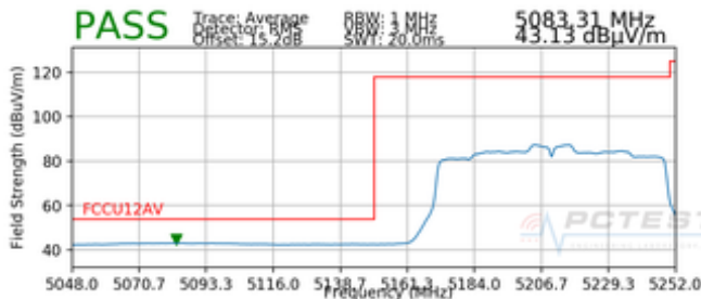
Plot 7-34. Radiated Lower Band Edge Plot SISO ANT1 (Average – UNII Band 1)
