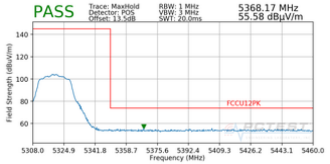
Plot 7-24. Radiated Band Edge Plot SISO ANT1 (Peak – WCP)
