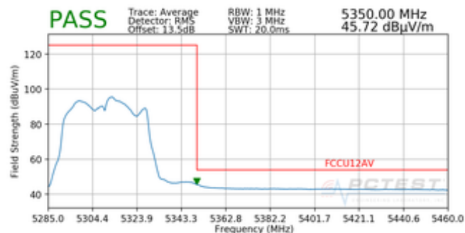
Plot 7-86. Radiated Band Edge Plot ANT (Average – WCP)
