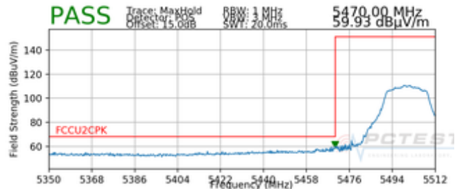
Plot 7-48. Radiated Lower Band Edge Plot SISO ANT2 (Peak – UNII Band 2C)
