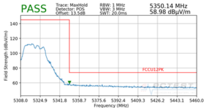
Plot 7-73. Radiated Upper Band Edge Plot MIMO (Peak – UNII Band 2A)
