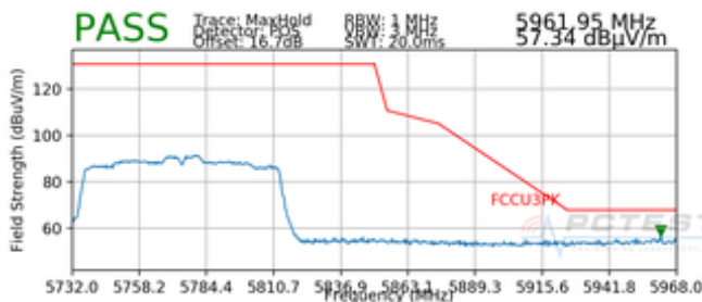
Plot 7-40. Radiated Upper Band Edge Plot SISO ANT1 (Peak – UNII Band 3)
