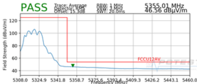
Plot 7-99. Radiated Upper Band Edge Plot MIMO (Average – UNII Band 2A)
