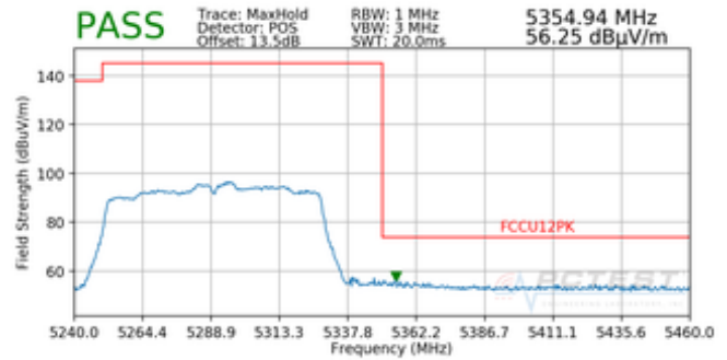
Plot 7-69. Radiated Band Edge Plot SISO ANT2 (Peak – WCP)
