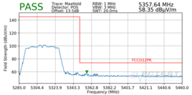
Plot 7-60. Radiated Band Edge Plot SISO ANT2 (Peak – WCP)
