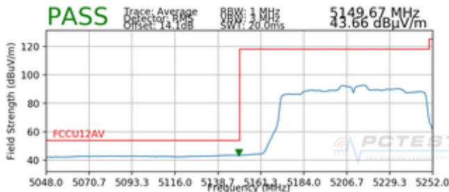
Plot 7-61. Radiated Lower Band Edge Plot SISO ANT2 (Average – UNII Band 1)
