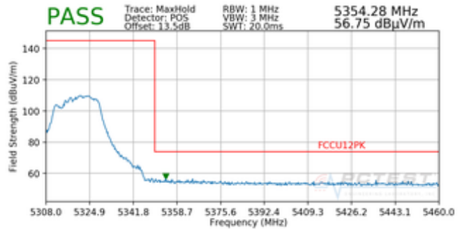
Plot 7-78. Radiated Band Edge Plot MIMO (Peak – WCP)
