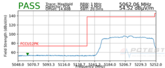
Plot 7-35. Radiated Lower Band Edge Plot SISO ANT1 (Peak – UNII Band 1)
