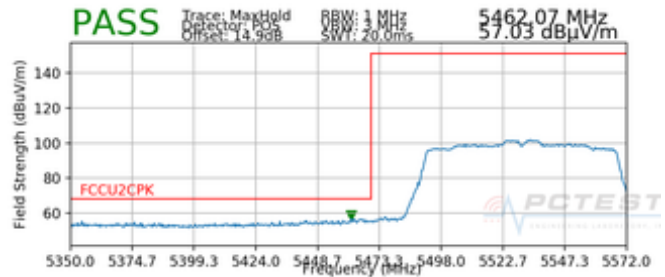
Plot 7-66. Radiated Lower Band Edge Plot SISO ANT2 (Peak – UNII Band 2C)
