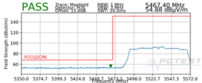
Plot 7-39. Radiated Lower Band Edge Plot SISO ANT1 (Peak – UNII Band 2C)
