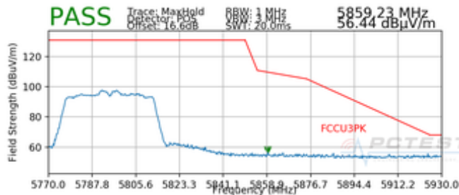
Plot 7-31. Radiated Upper Band Edge Plot SISO ANT1 (Peak – UNII Band 3)
