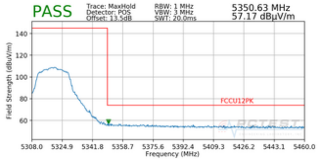
Plot 7-51. Radiated Band Edge Plot SISO ANT2 (Peak – WCP)
