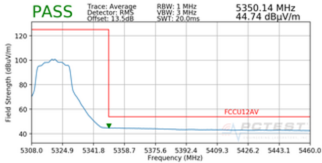
Plot 7-50. Radiated Band Edge Plot SISO ANT2 (Average – WCP)
