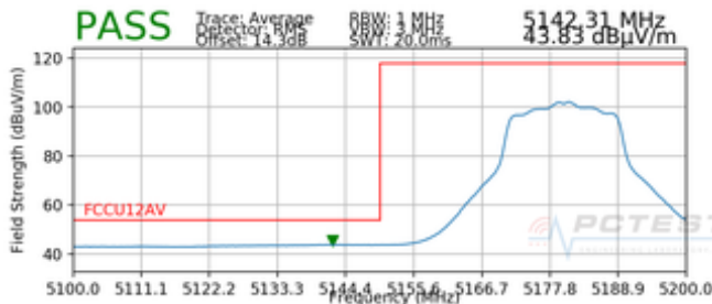
Plot 7-43. Radiated Lower Band Edge Plot SISO ANT2 (Average – UNII Band 1)
