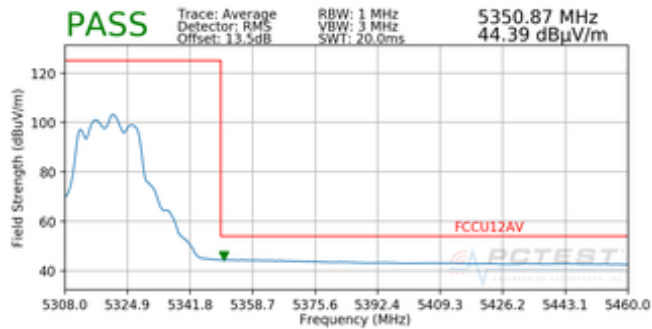
Plot 7-104. Radiated Band Edge Plot MIMO (Average – WCP)
