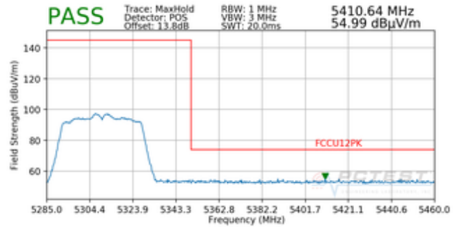
Plot 7-33. Radiated Band Edge Plot SISO ANT1 (Peak – WCP)
