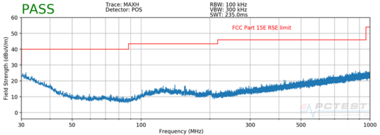
Plot 7-108. Radiated Spurious Plot below 1GHz (Simultaneous Transmission Config-1)
