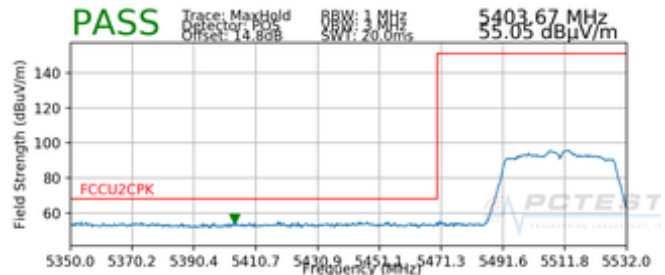
Plot 7-30. Radiated Lower Band Edge Plot SISO ANT1 (Peak – UNII Band 2C)
