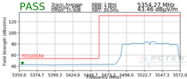
Plot 7-38. Radiated Lower Band Edge Plot SISO ANT1 (Average – UNII Band 2C)
