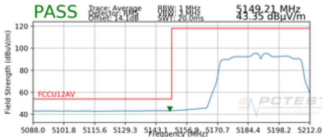
Plot 7-52. Radiated Lower Band Edge Plot SISO ANT2 (Average – UNII Band 1)
