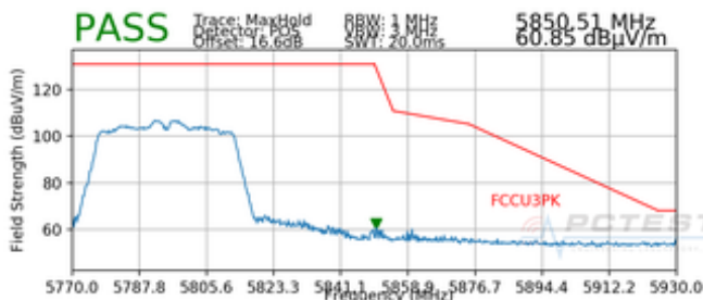
Plot 7-58. Radiated Upper Band Edge Plot SISO ANT2 (Peak – UNII Band 3)
