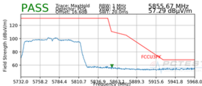
Plot 7-67. Radiated Upper Band Edge Plot SISO ANT2 (Peak – UNII Band 3)
