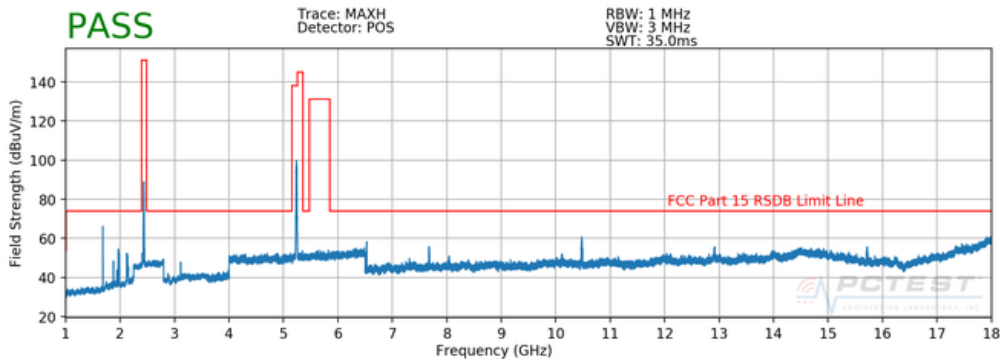
Plot 7-13. Radiated Spurious Plot above 1GHz (Simultaneous Transmission Config-1)
