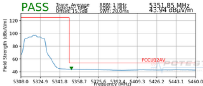
Plot 7-18. Radiated Upper Band Edge Plot SISO ANT1 (Average – UNII Band 2A)
