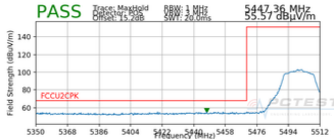
Plot 7-21. Radiated Lower Band Edge Plot SISO ANT1 (Peak – UNII Band 2C)
