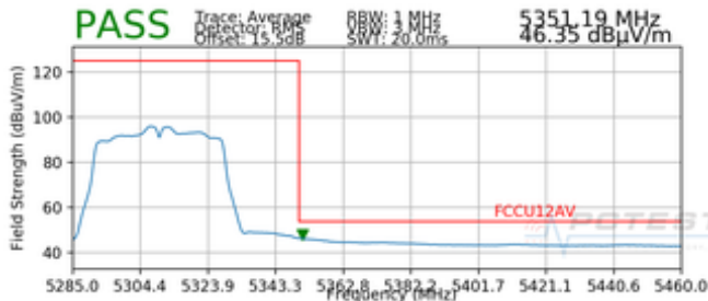
Plot 7-54. Radiated Upper Band Edge Plot SISO ANT2 (Average – UNII Band 2A)
