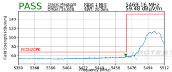
Plot 7-102. Radiated Lower Band Edge Plot MIMO (Peak – UNII Band 2C)
