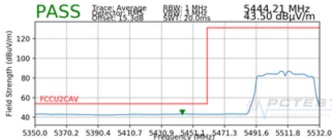
Plot 7-29. Radiated Lower Band Edge Plot SISO ANT1 (Average – UNII Band 2C)
