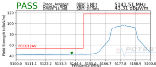
Plot 7-16. Radiated Lower Band Edge Plot SISO ANT1 (Average – UNII Band 1)
