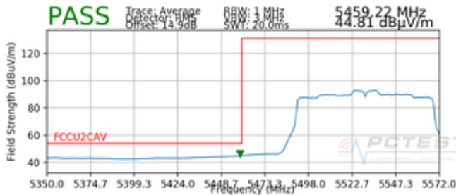
Plot 7-65. Radiated Lower Band Edge Plot SISO ANT2 (Average – UNII Band 2C)
