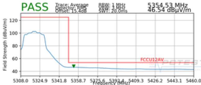
Plot 7-45. Radiated Upper Band Edge Plot SISO ANT2 (Average – UNII Band 2A)
