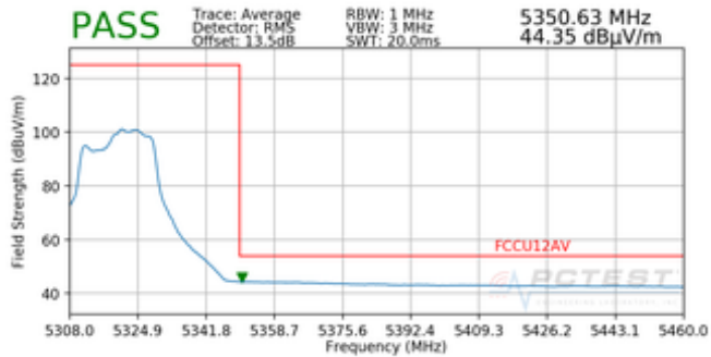
Plot 7-77. Radiated Band Edge Plot MIMO (Average – WCP)
