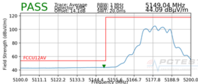
Plot 7-97. Radiated Lower Band Edge Plot MIMO (Average – UNII Band 1)
