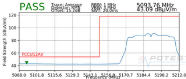
Plot 7-25. Radiated Lower Band Edge Plot SISO ANT1 (Average – UNII Band 1)
