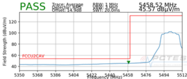
Plot 7-47. Radiated Lower Band Edge Plot SISO ANT2 (Average – UNII Band 2C)
