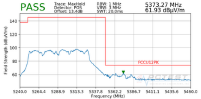
Plot 7-96. Radiated Band Edge Plot ANT (Peak – WCP)
