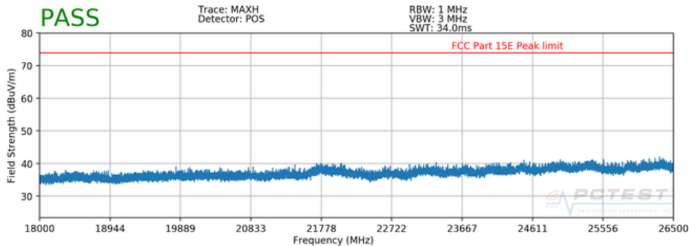
Plot 7-14. Radiated Spurious Plot 18GHz – 26.5GHz (Simultaneous Transmission Config-1)
