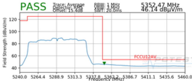
Plot 7-63. Radiated Upper Band Edge Plot SISO ANT2 (Average – UNII Band 2A)
