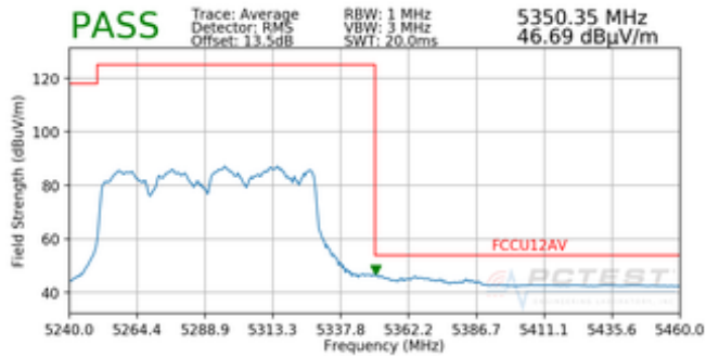
Plot 7-95. Radiated Band Edge Plot ANT (Average – WCP)
