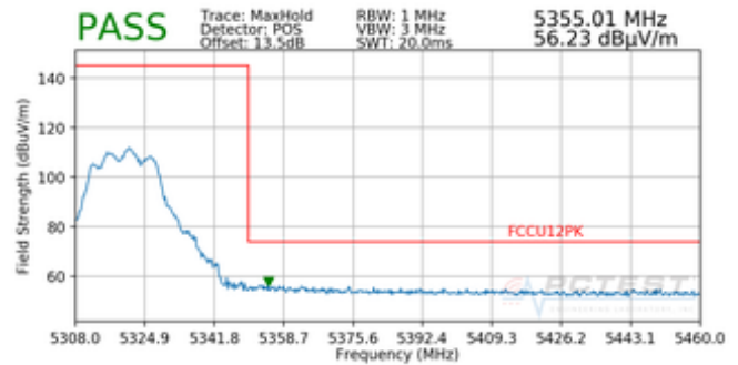
Plot 7-105. Radiated Band Edge Plot MIMO (Peak – WCP)
