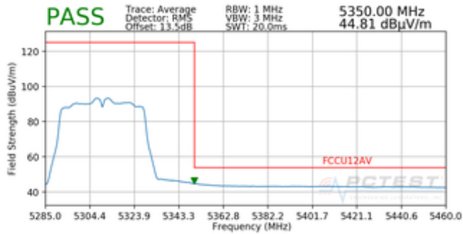
Plot 7-59. Radiated Band Edge Plot SISO ANT2 (Average – WCP)
