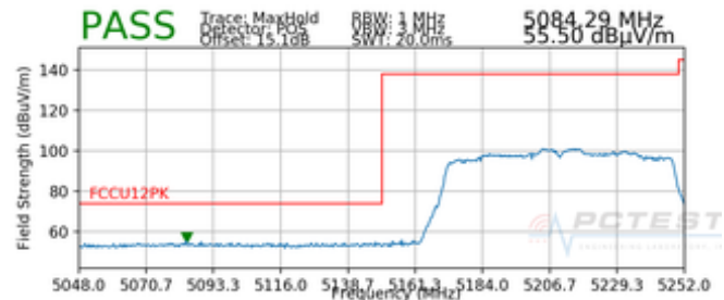
Plot 7-62. Radiated Lower Band Edge Plot SISO ANT2 (Peak – UNII Band 1)
