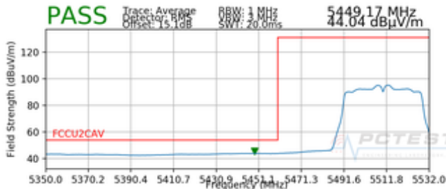
Plot 7-56. Radiated Lower Band Edge Plot SISO ANT2 (Average – UNII Band 2C)
