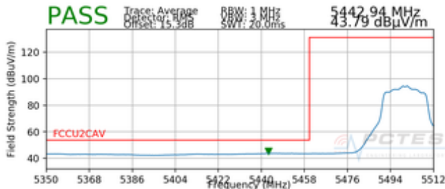
Plot 7-20. Radiated Lower Band Edge Plot SISO ANT1 (Average – UNII Band 2C)
