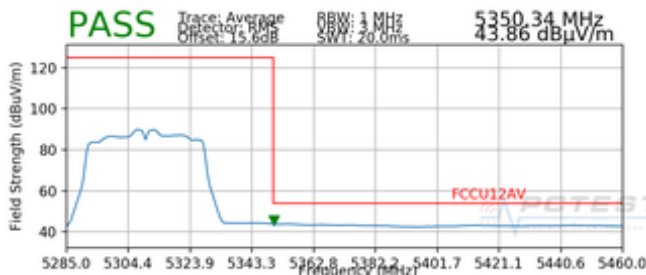
Plot 7-27. Radiated Upper Band Edge Plot SISO ANT1 (Average – UNII Band 2A)
