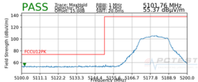
Plot 7-17. Radiated Lower Band Edge Plot SISO ANT1 (Peak – UNII Band 1)
