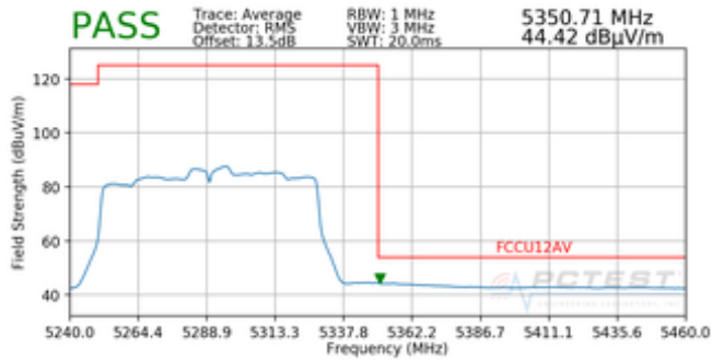
Plot 7-68. Radiated Band Edge Plot SISO ANT2 (Average – WCP)
