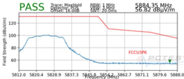
Plot 7-22. Radiated Upper Band Edge Plot SISO ANT1 (Peak – UNII Band 3)
