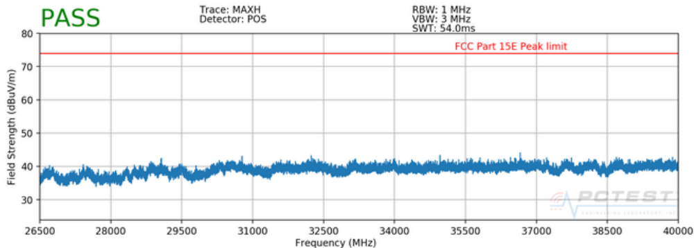
Plot 7-15. Radiated Spurious Plot above 26.5GHz (Simultaneous Transmission Config-1)
