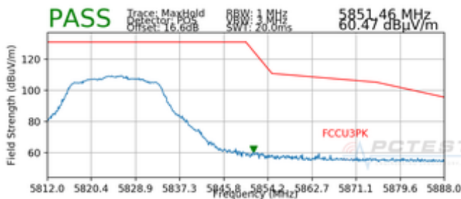
Plot 7-49. Radiated Upper Band Edge Plot SISO ANT2 (Peak – UNII Band 3)
