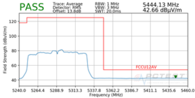
Plot 7-41. Radiated Band Edge Plot SISO ANT1 (Average – WCP)
