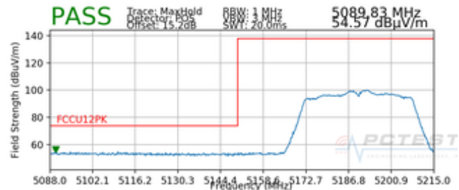
Plot 7-26. Radiated Lower Band Edge Plot SISO ANT1 (Peak – UNII Band 1)
