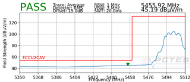
Plot 7-101. Radiated Lower Band Edge Plot MIMO (Average – UNII Band 2C)
