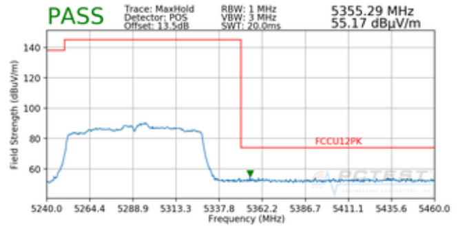
Plot 7-42. Radiated Band Edge Plot SISO ANT1 (Peak – WCP)
