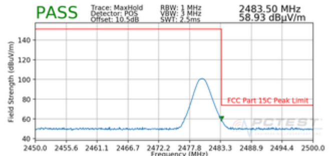
Plot 7-49. Radiated Restricted Upper Band Edge Measurement with WCP (Peak)
