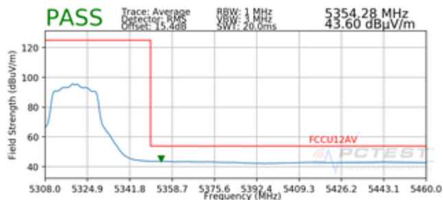
Plot 7-233. Radiated Band Edge Plot (Average – WCP)
