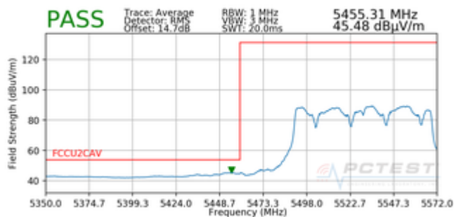
Plot 7-257. Radiated Lower Band Edge Plot (Average – UNII Band 2C)
