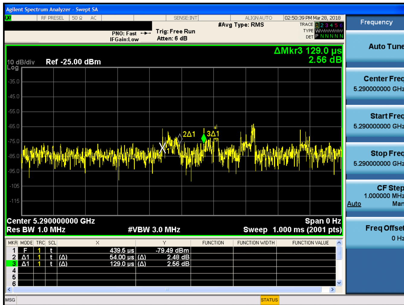
Figure 5-1. Band 2A Channel Loading
