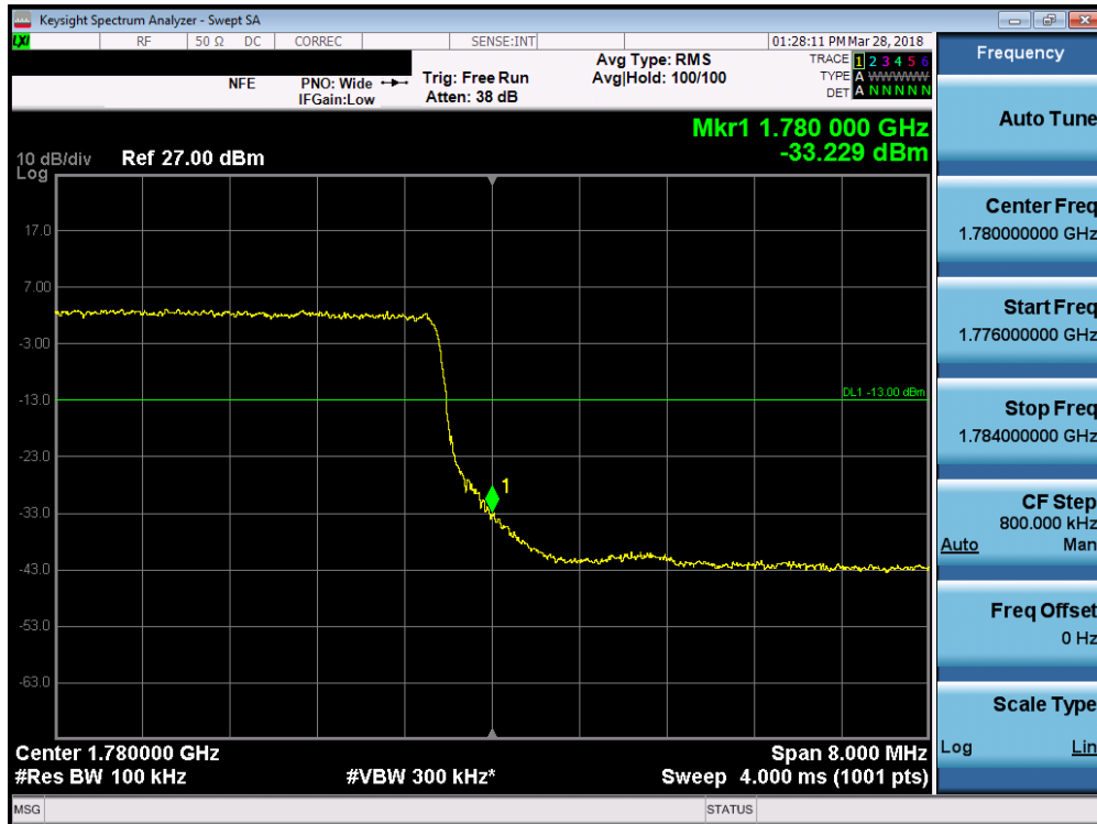
Plot 7-179. Upper Band Edge Plot (Band 66 - 10.0MHz QPSK - Full RB Configuration)
