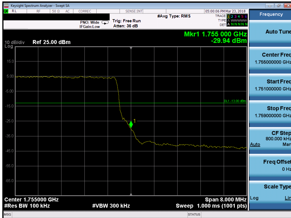
Plot 7-177. Upper Band Edge Plot (Band 4 - 10.0MHz QPSK - Full RB Configuration)
