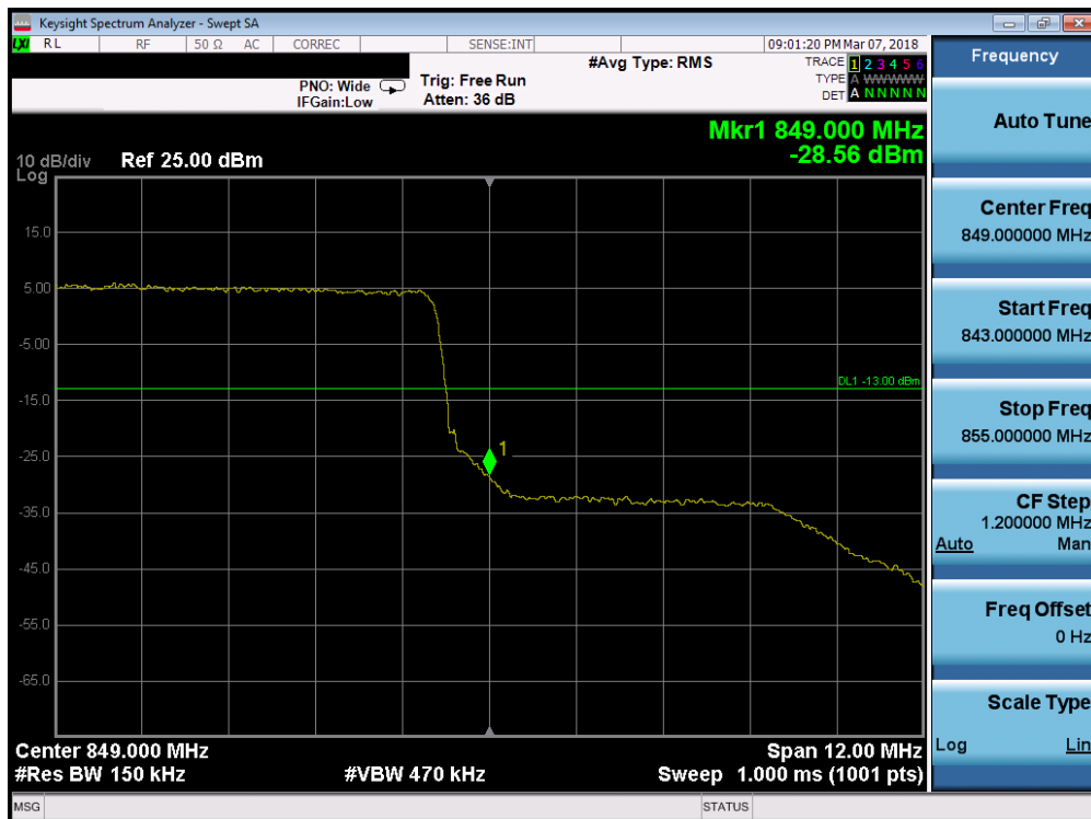
Plot 7-156. Upper Band Edge Plot (Band 26 - 15.0MHz QPSK - Full RB Configuration)
