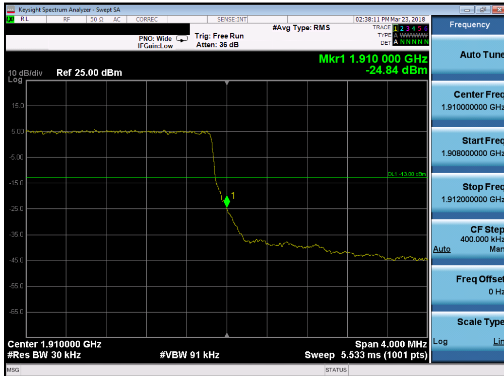
Plot 7-201. Upper Band Edge Plot (Band 2 - 3.0MHz QPSK - Full RB Configuration)
