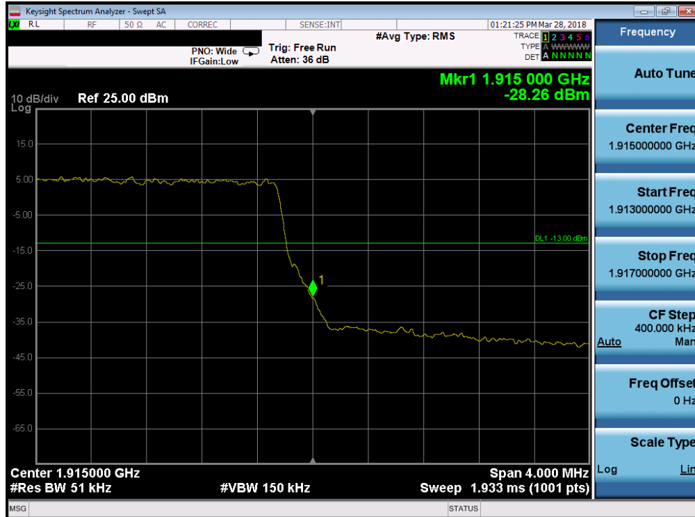
Plot 7-209. Upper Band Edge Plot (Band 25 - 5.0MHz QPSK - Full RB Configuration)
