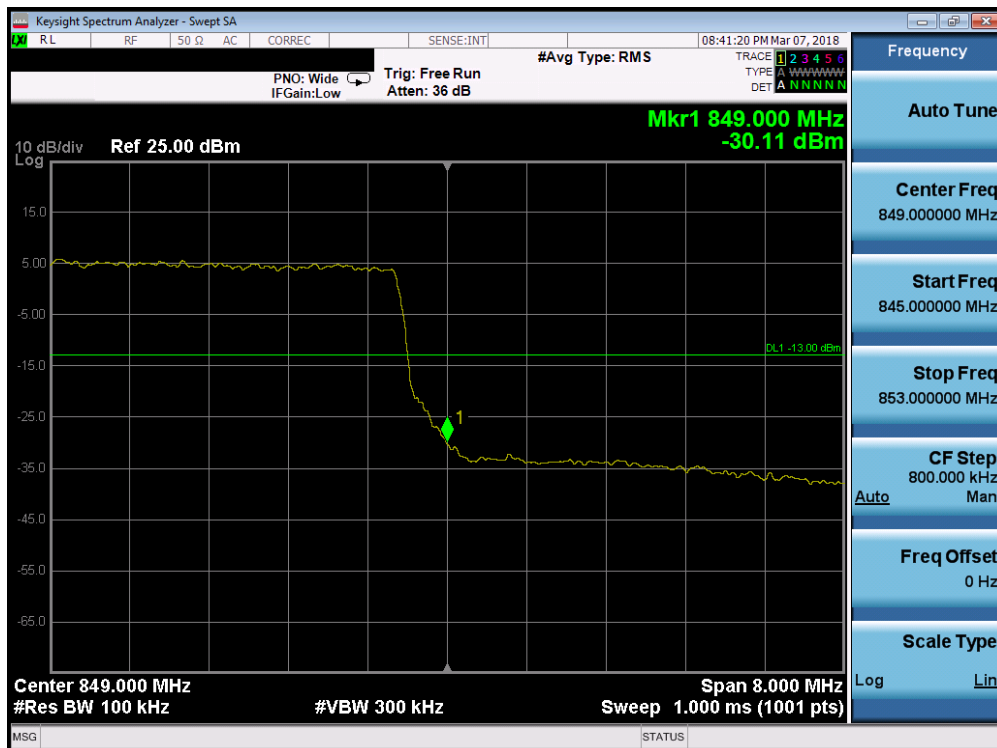
Plot 7-154. Upper Band Edge Plot (Band 26/5 - 10.0MHz QPSK - Full RB Configuration)
