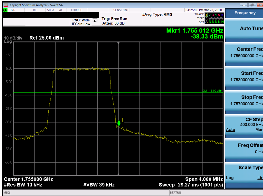
Plot 7-159. Upper Band Edge Plot (Band 4 - 1.4MHz QPSK - Full RB Configuration)
