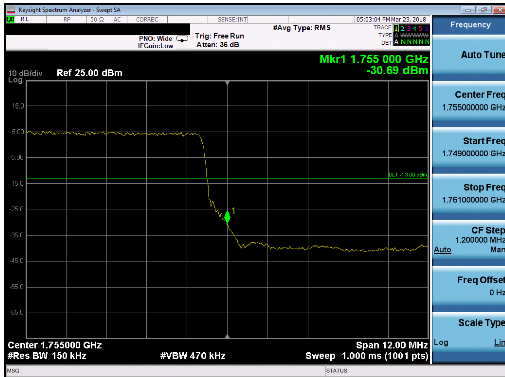
Plot 7-183. Upper Band Edge Plot (Band 4 - 15.0MHz QPSK - Full RB Configuration)
